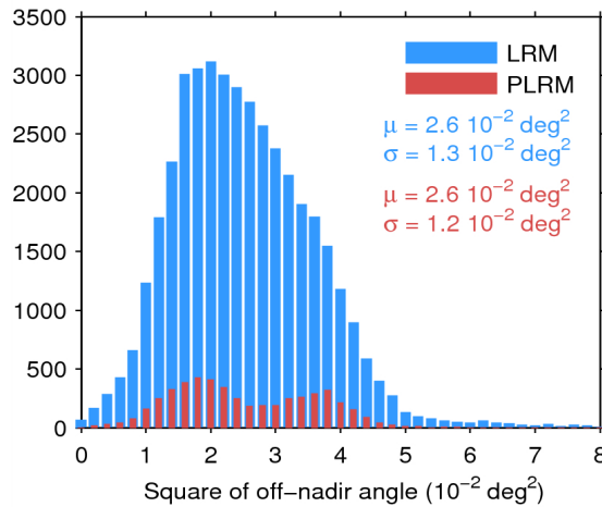
Figure 39. Histogram of flag-valid mispointing over oceans and lakes for LRM (blue) and PLRM (red) for 06/03/2015. Only positive values have been considered. The mean ( \mu ) and standard deviation ( \sigma ) are also shown. Note that values larger than 8 \cdot 10^{-2} \text{ deg}^2 are excluded from the histogram for the sake of readability but not from the computation of \mu and \sigma .
