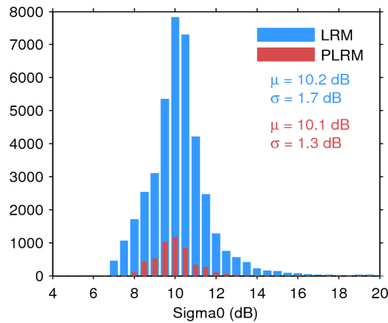
Figure 28. Histogram of science-valid sigma0 over oceans and lakes for LRM (blue) and PLRM (red) for 06/03/2015. The mean ( \mu ) and standard deviation ( \sigma ) are also shown. Note that values outside [4 20] dB are excluded from the histogram for the sake of readability but not from the computation of \mu and \sigma .
