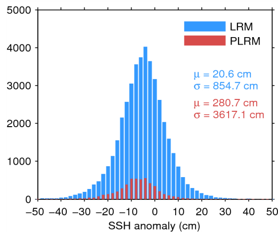
Figure 7. Histogram of flag-valid SSH anomaly over oceans and lakes for LRM (blue) and PLRM (red) for 06/03/2015. The mean ( \mu ) and standard deviation ( \sigma ) are also shown. Note that values outside [-50\ 50] cm are excluded from the histogram for the sake of readability but not from the computation of \mu and \sigma .
