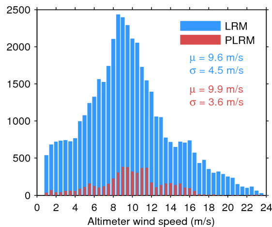
Figure 35. Histogram of science-valid wind over oceans and lakes for LRM (blue) and PLRM (red) for 06/03/2015. The mean ( \mu ) and standard deviation ( \sigma ) are also shown. Note that values larger than 24 m/s are excluded from the histogram for the sake of readability but not from the computation of \mu and \sigma .
