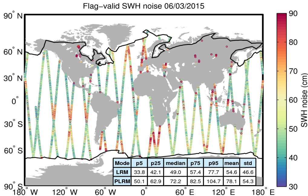
Figure 18. Geographical distribution of flag-valid 20-Hz SWH measurement noise over oceans and lakes for 06/03/2015. The statistical values shown in the table refer to the SWH noise and are calculated separately for LRM and PLRM regions. Measurements taken over polar polygons have been excluded from the computation of the statistical values. The black lines mark the outer limit of the Arctic and Antarctic polar polygons.
