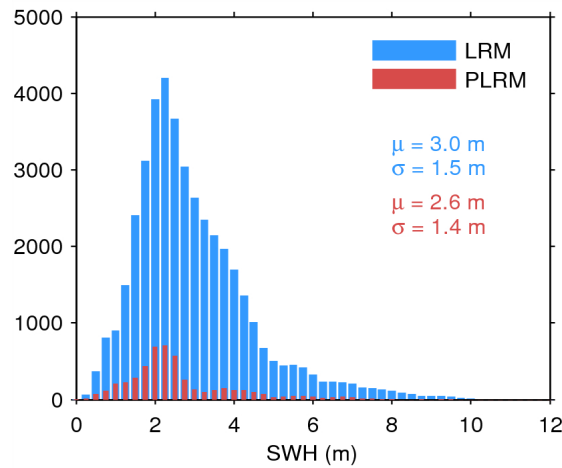
Figure 20. Histogram of science-valid SWH over oceans and lakes for LRM (blue) and PLRM (red) for 06/03/2015. The mean ( \mu ) and standard deviation ( \sigma ) are also shown. Note that values larger than 12 m are excluded from the histogram for the sake of readability but not from the computation of \mu and \sigma .
