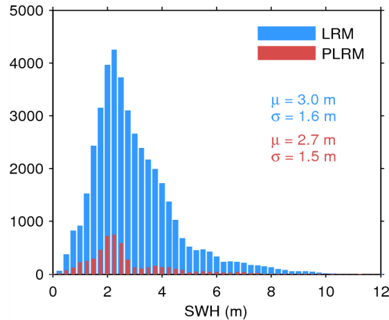
Figure 17. Histogram of flag-valid SWH over oceans and lakes for LRM (blue) and PLRM (red) for 06/03/2015. The mean ( \mu ) and standard deviation ( \sigma ) are also shown. Note that values larger than 12 m are excluded from the histogram for the sake of readability but not from the computation of \mu and \sigma .
