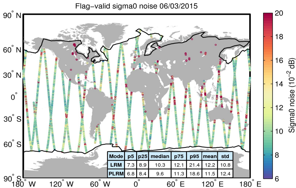
Figure 26. Geographical distribution of flag-valid 20-Hz sigma0 measurement noise over oceans and lakes for 06/03/2015. The statistical values shown in the table refer to the sigma0 noise and are calculated separately for LRM and PLRM regions. Measurements taken over polar polygons have been excluded from the computation of the statistical values. The black lines mark the outer limit of the Arctic and Antarctic polar polygons.
