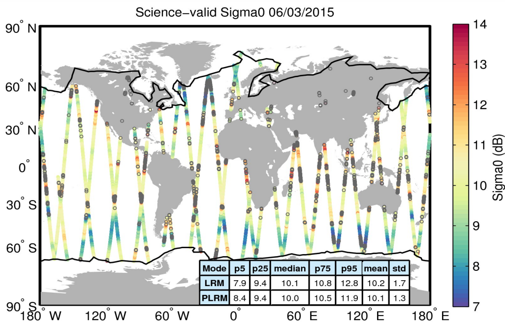
Figure 27. Geographical distribution of science-valid sigma0 data over oceans and lakes for 06/03/2015. The statistical values shown in the table refer to the sigma0 in dB and are calculated separately for LRM and PLRM regions. The black lines mark the outer limit of the Arctic and Antarctic polar polygons. Gray circles denote records that have been rejected based on the editing criteria described in Table 4.
