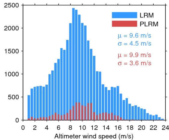
Figure 33. Histogram of flag-valid wind over oceans and lakes for LRM (blue) and PLRM (red) for 06/03/2015. The mean ( \mu ) and standard deviation ( \sigma ) are also shown. Note that values larger than 24 m/s are excluded from the histogram for the sake of readability but not from the computation of \mu and \sigma .
