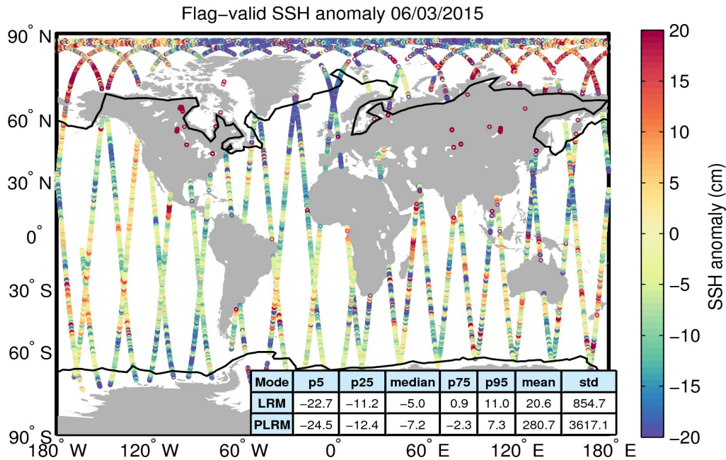
Figure 5. Geographical distribution of flag-valid 1-Hz SSH anomaly data over oceans and lakes for 06/03/2015. The statistical values shown in the table refer to the SSH anomaly in cm and are calculated separately for LRM and PLRM regions. Measurements taken over polar polygons have been excluded from the computation of the statistical values. The black lines mark the outer limit of the Arctic and Antarctic polar polygons.
