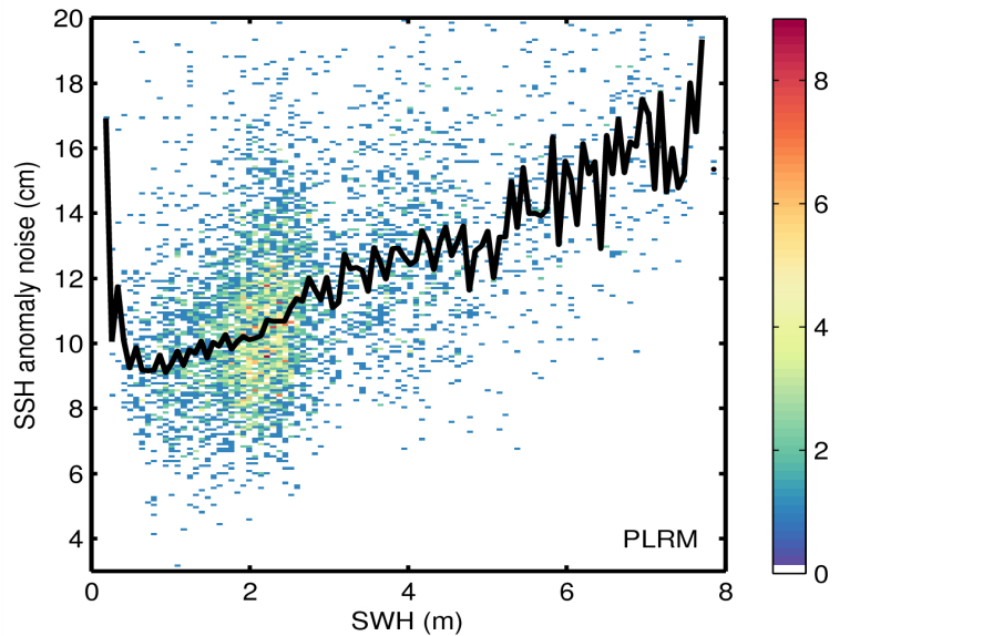
Figure 9. 2D histogram showing flag-valid SSH anomaly noise as a function of SWH for LRM (top) and PLRM (bottom) for 06/03/2015. The black line denotes the median SSH anomaly as a function of SWH.
