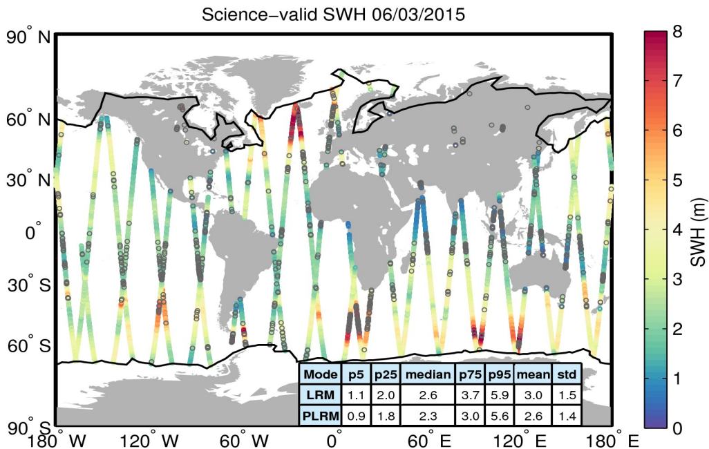
Figure 19. Geographical distribution of science-valid SWH data over oceans and lakes for 06/03/2015. The statistical values shown in the table refer to the SWH in m and are calculated separately for LRM and PLRM regions. The black lines mark the outer limit of the Arctic and Antarctic polar polygons. Gray circles denote records that have been rejected based on the editing criteria described in Table 3.
