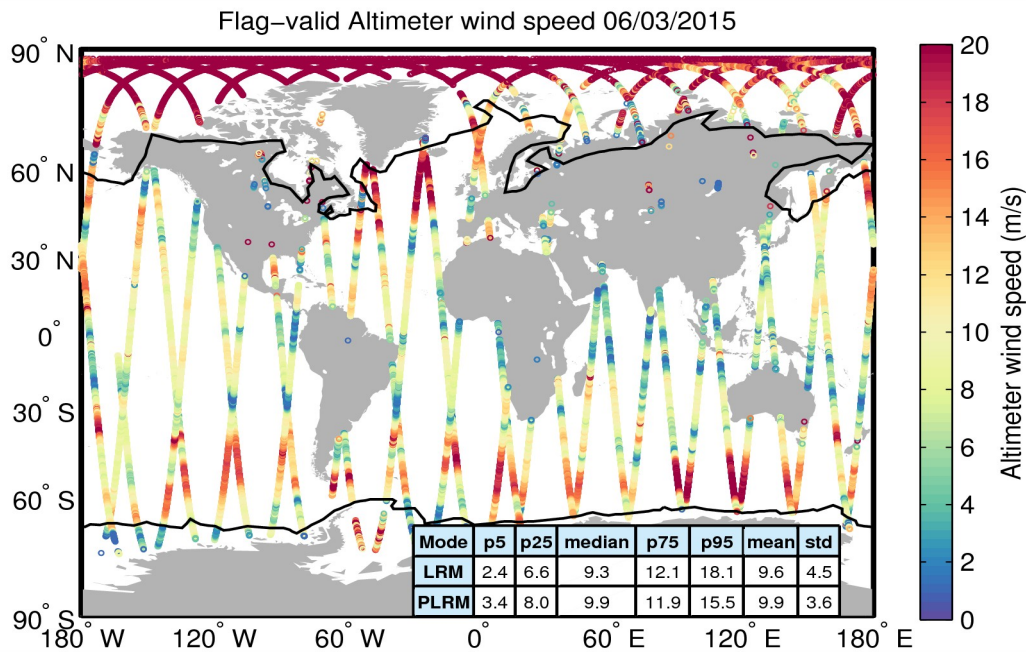
Figure 31. Geographical distribution of flag-valid wind data over oceans and lakes for 06/03/2015. The statistical values shown in the table refer to the wind in m/s and are calculated separately for LRM and PLRM regions. Measurements taken over polar polygons have been excluded from the computation of the statistical values. The black lines mark the outer limit of the Arctic and Antarctic polar polygons.
