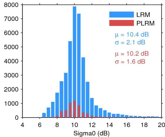
Figure 25. Histogram of flag-valid sigma0 over oceans and lakes for LRM (blue) and PLRM (red) for 06/03/2015. The mean ( \mu ) and standard deviation ( \sigma ) are also shown. Note that values outside [4 20] dB are excluded from the histogram for the sake of readability but not from the computation of \mu and \sigma .
