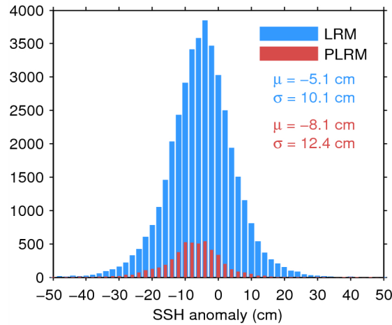
Figure 11. Histogram of science-valid SSH anomaly over oceans and lakes for LRM (blue) and PLRM (red) for 06/03/2015. The mean ( \mu ) and standard deviation ( \sigma ) are also shown. Note that values outside [-50 50] cm are excluded from the histogram for the sake of readability but not from the computation of \mu and \sigma .
