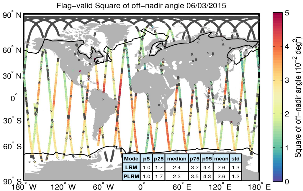
Figure 37. Geographical distribution of flag-valid mispointing data over oceans and lakes for 06/03/2015. The statistical values shown in the table refer to the mispointing in 10^{-2} \text{ deg}^2 and are calculated separately for LRM and PLRM regions. Measurements taken over polar polygons have been excluded from the computation of the statistical values. The black lines mark the outer limit of the Arctic and Antarctic polar polygons. Gray circles denote negative values.
