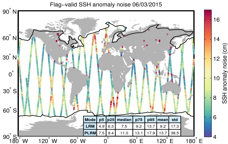
Figure 8. Geographical distribution of flag-valid 20-Hz SSH anomaly measurement noise over oceans and lakes for 06/03/2015. The statistical values shown in the table refer to the SSH anomaly noise and are calculated separately for LRM and PLRM regions. Measurements taken over polar polygons have been excluded from the computation of the statistical values. The black lines mark the outer limit of the Arctic and Antarctic polar polygons.
