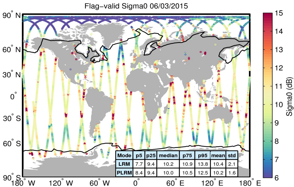
Figure 23. Geographical distribution of flag-valid sigma0 data over oceans and lakes for 06/03/2015. The statistical values shown in the table refer to the sigma0 in dB and are calculated separately for LRM and PLRM regions. Measurements taken over polar polygons have been excluded from the computation of the statistical values. The black lines mark the outer limit of the Arctic and Antarctic polar polygons.
