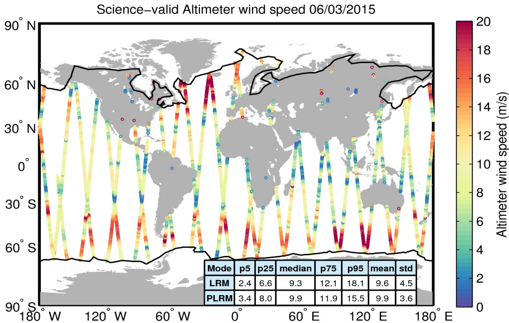
Figure 34. Geographical distribution of science-valid wind data over oceans and lakes for 06/03/2015. The statistical values shown in the table refer to the wind in m/s and are calculated separately for LRM and PLRM regions. The black lines mark the outer limit of the Arctic and Antarctic polar polygons. Gray circles denote records that have been rejected based on the editing criteria described in Table 5.
