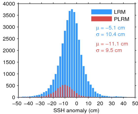
Figure 11. Histogram of science-valid SSH anomaly over oceans and lakes for LRM (blue) and PLRM (red) for 05/03/2015. The mean ( \mu ) and standard deviation ( \sigma ) are also shown. Note that values outside [-50 50] cm are excluded from the histogram for the sake of readability but not from the computation of \mu and \sigma .
