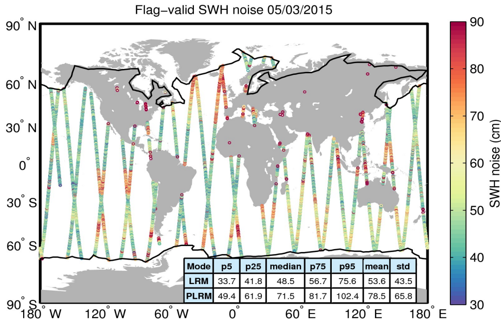
Figure 18. Geographical distribution of flag-valid 20-Hz SWH measurement noise over oceans and lakes for 05/03/2015. The statistical values shown in the table refer to the SWH noise and are calculated separately for LRM and PLRM regions. Measurements taken over polar polygons have been excluded from the computation of the statistical values. The black lines mark the outer limit of the Arctic and Antarctic polar polygons.
