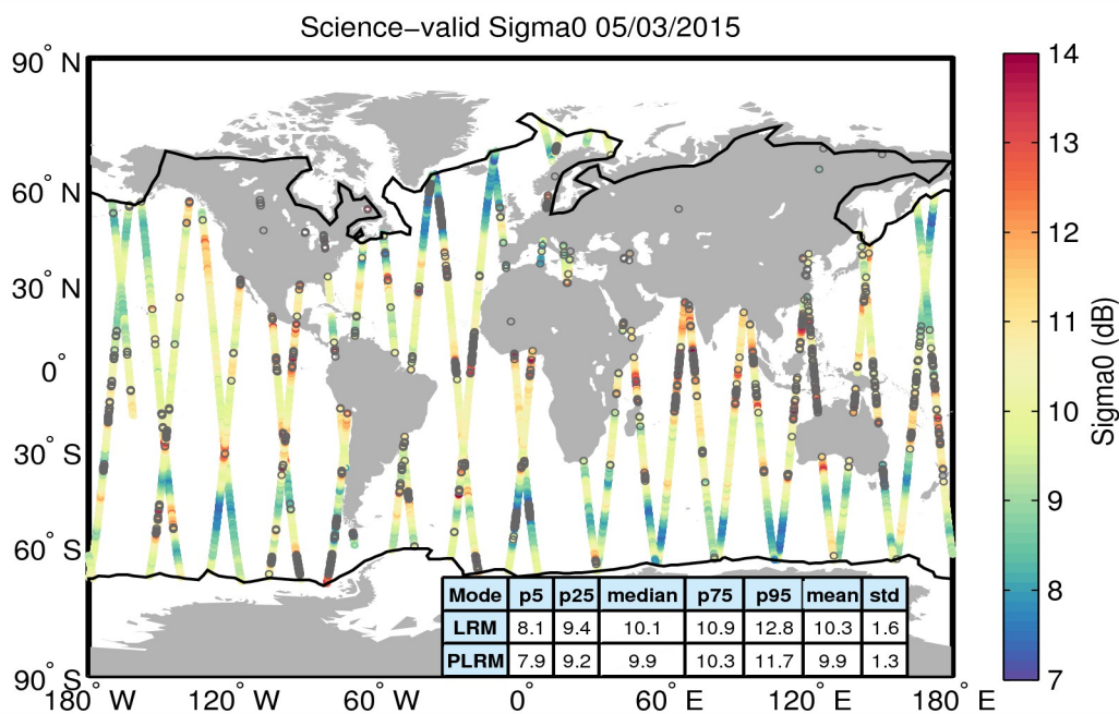
Figure 27. Geographical distribution of science-valid sigma0 data over oceans and lakes for 05/03/2015. The statistical values shown in the table refer to the sigma0 in dB and are calculated separately for LRM and PLRM regions. The black lines mark the outer limit of the Arctic and Antarctic polar polygons. Gray circles denote records that have been rejected based on the editing criteria described in Table 4.
