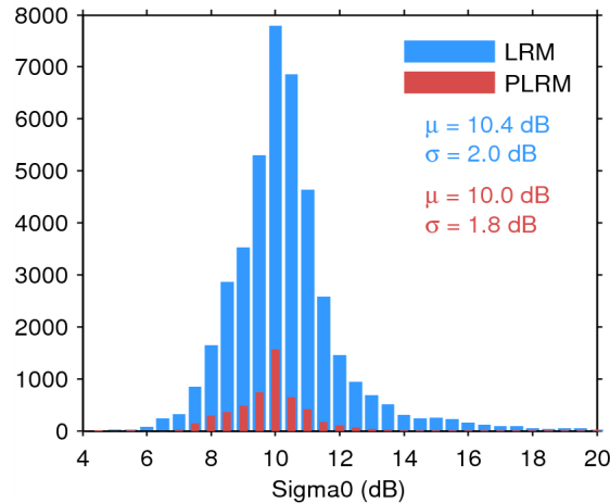
Figure 25. Histogram of flag-valid sigma0 over oceans and lakes for LRM (blue) and PLRM (red) for 05/03/2015. The mean ( \mu ) and standard deviation ( \sigma ) are also shown. Note that values outside [4 20] dB are excluded from the histogram for the sake of readability but not from the computation of \mu and \sigma .
