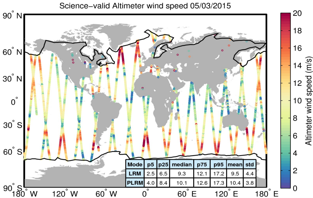
Figure 34. Geographical distribution of science-valid wind data over oceans and lakes for 05/03/2015. The statistical values shown in the table refer to the wind in m/s and are calculated separately for LRM and PLRM regions. The black lines mark the outer limit of the Arctic and Antarctic polar polygons. Gray circles denote records that have been rejected based on the editing criteria described in Table 5.
