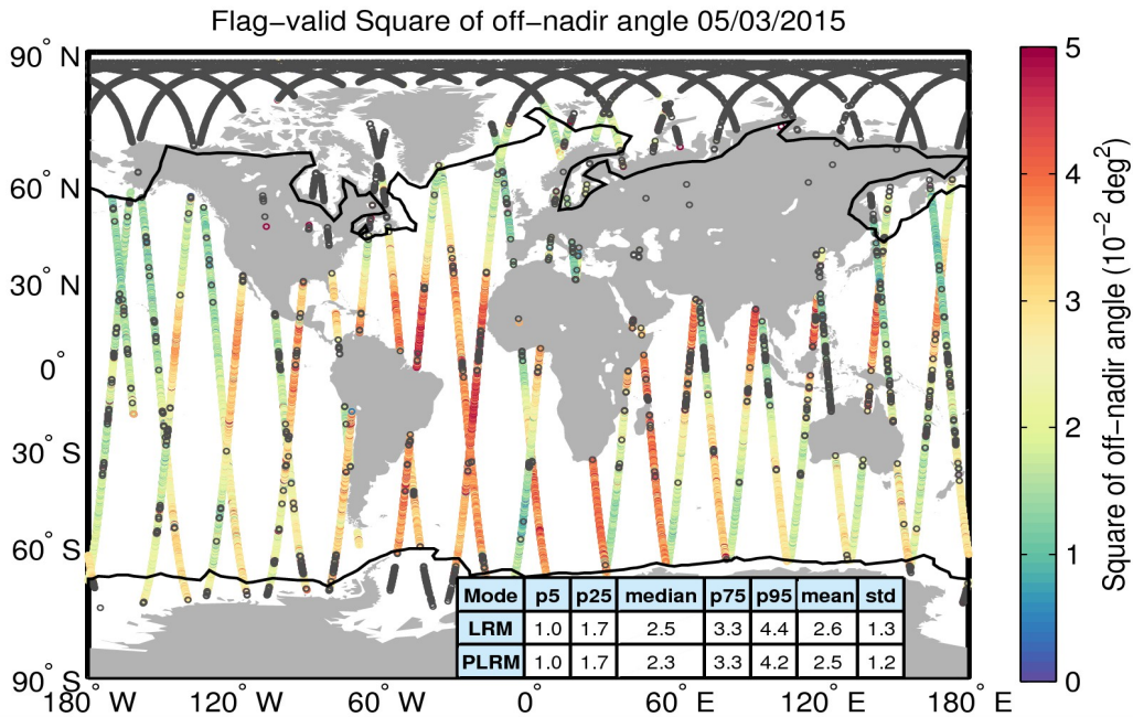
Figure 37. Geographical distribution of flag-valid mispointing data over oceans and lakes for 05/03/2015. The statistical values shown in the table refer to the mispointing in 10^{-2} \text{ deg}^2 and are calculated separately for LRM and PLRM regions. Measurements taken over polar polygons have been excluded from the computation of the statistical values. The black lines mark the outer limit of the Arctic and Antarctic polar polygons. Gray circles denote negative values.
