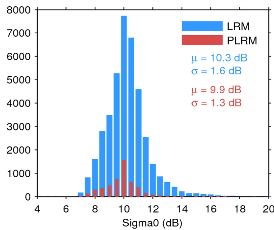
Figure 28. Histogram of science-valid sigma0 over oceans and lakes for LRM (blue) and PLRM (red) for 05/03/2015. The mean ( \mu ) and standard deviation ( \sigma ) are also shown. Note that values outside [4 20] dB are excluded from the histogram for the sake of readability but not from the computation of \mu and \sigma .
