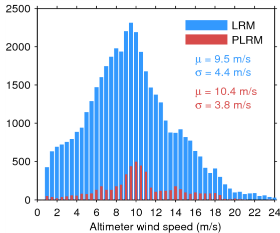
Figure 33. Histogram of flag-valid wind over oceans and lakes for LRM (blue) and PLRM (red) for 05/03/2015. The mean ( \mu ) and standard deviation ( \sigma ) are also shown. Note that values larger than 24 m/s are excluded from the histogram for the sake of readability but not from the computation of \mu and \sigma .
