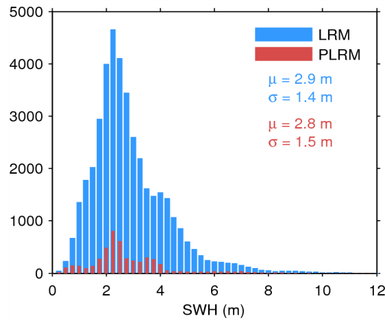
Figure 20. Histogram of science-valid SWH over oceans and lakes for LRM (blue) and PLRM (red) for 05/03/2015. The mean ( \mu ) and standard deviation ( \sigma ) are also shown. Note that values larger than 12 m are excluded from the histogram for the sake of readability but not from the computation of \mu and \sigma .
