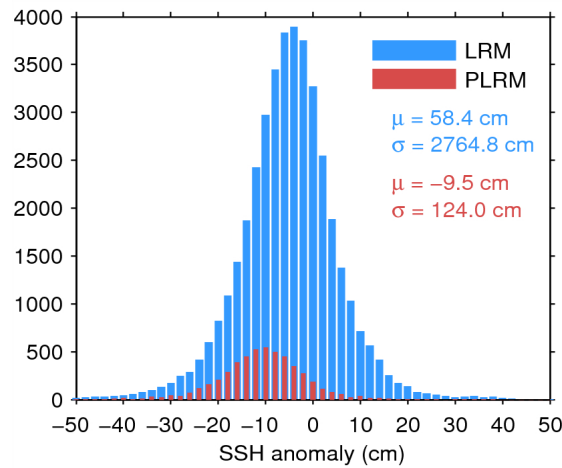
Figure 7. Histogram of flag-valid SSH anomaly over oceans and lakes for LRM (blue) and PLRM (red) for 05/03/2015. The mean ( \mu ) and standard deviation ( \sigma ) are also shown. Note that values outside [-50\ 50] cm are excluded from the histogram for the sake of readability but not from the computation of \mu and \sigma .
