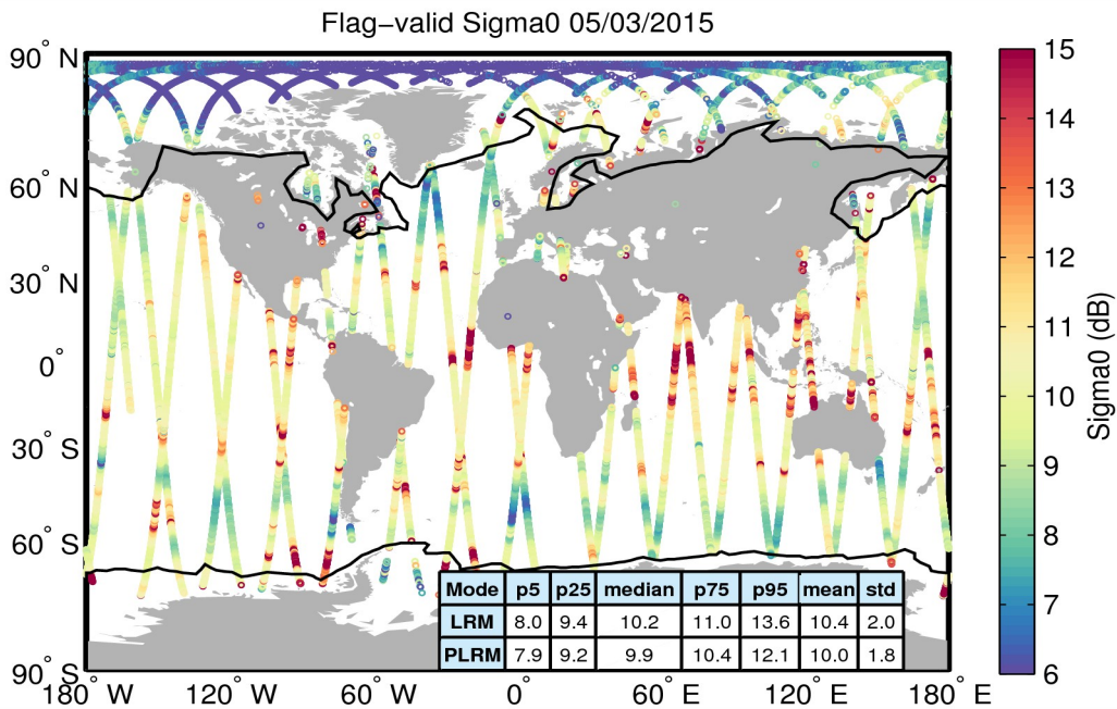
Figure 23. Geographical distribution of flag-valid sigma0 data over oceans and lakes for 05/03/2015. The statistical values shown in the table refer to the sigma0 in dB and are calculated separately for LRM and PLRM regions. Measurements taken over polar polygons have been excluded from the computation of the statistical values. The black lines mark the outer limit of the Arctic and Antarctic polar polygons.
