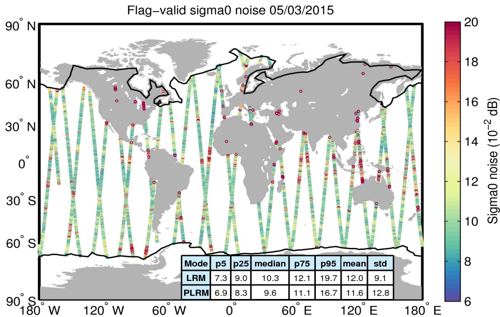
Figure 26. Geographical distribution of flag-valid 20-Hz sigma0 measurement noise over oceans and lakes for 05/03/2015. The statistical values shown in the table refer to the sigma0 noise and are calculated separately for LRM and PLRM regions. Measurements taken over polar polygons have been excluded from the computation of the statistical values. The black lines mark the outer limit of the Arctic and Antarctic polar polygons.
