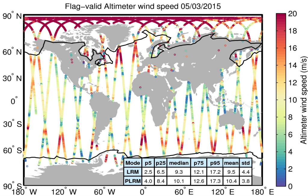
Figure 31. Geographical distribution of flag-valid wind data over oceans and lakes for 05/03/2015. The statistical values shown in the table refer to the wind in m/s and are calculated separately for LRM and PLRM regions. Measurements taken over polar polygons have been excluded from the computation of the statistical values. The black lines mark the outer limit of the Arctic and Antarctic polar polygons.
