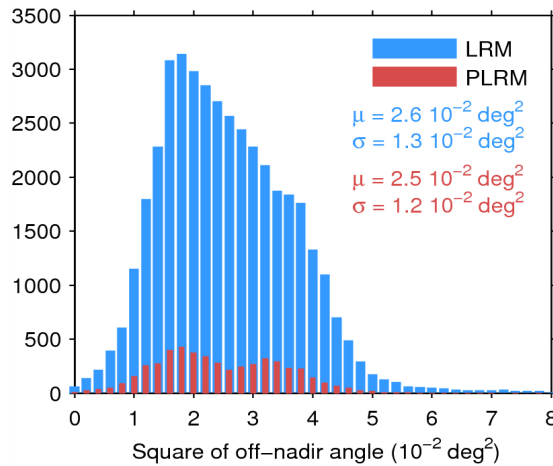
Figure 39. Histogram of flag-valid mispointing over oceans and lakes for LRM (blue) and PLRM (red) for 05/03/2015. Only positive values have been considered. The mean ( \mu ) and standard deviation ( \sigma ) are also shown. Note that values larger than 8 \cdot 10^{-2} \text{ deg}^2 are excluded from the histogram for the sake of readability but not from the computation of \mu and \sigma .
