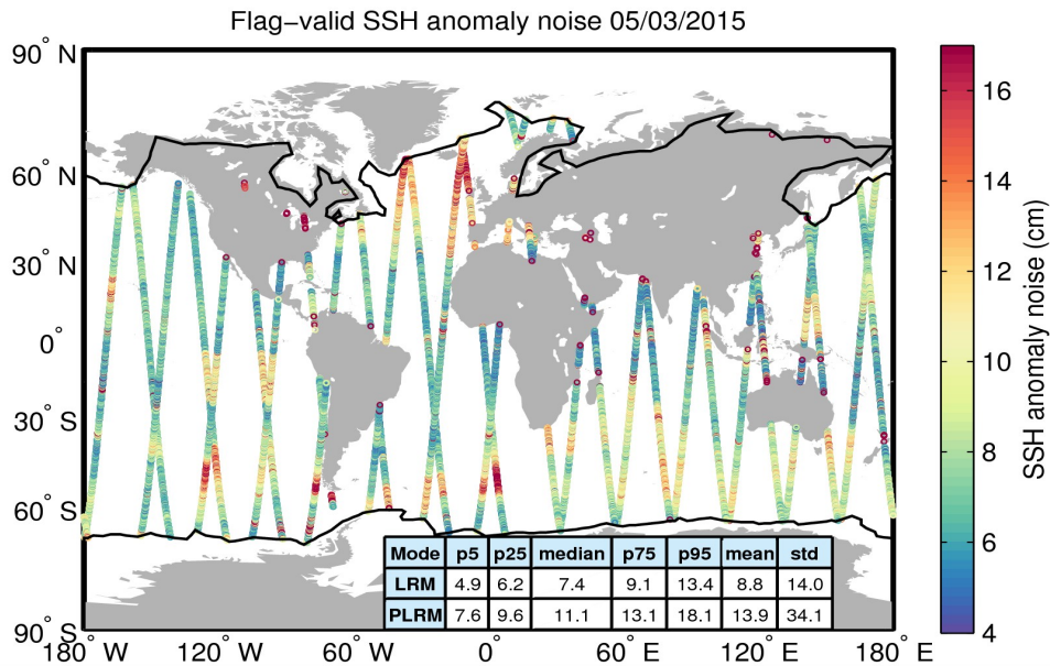
Figure 8. Geographical distribution of flag-valid 20-Hz SSH anomaly measurement noise over oceans and lakes for 05/03/2015. The statistical values shown in the table refer to the SSH anomaly noise and are calculated separately for LRM and PLRM regions. Measurements taken over polar polygons have been excluded from the computation of the statistical values. The black lines mark the outer limit of the Arctic and Antarctic polar polygons.
