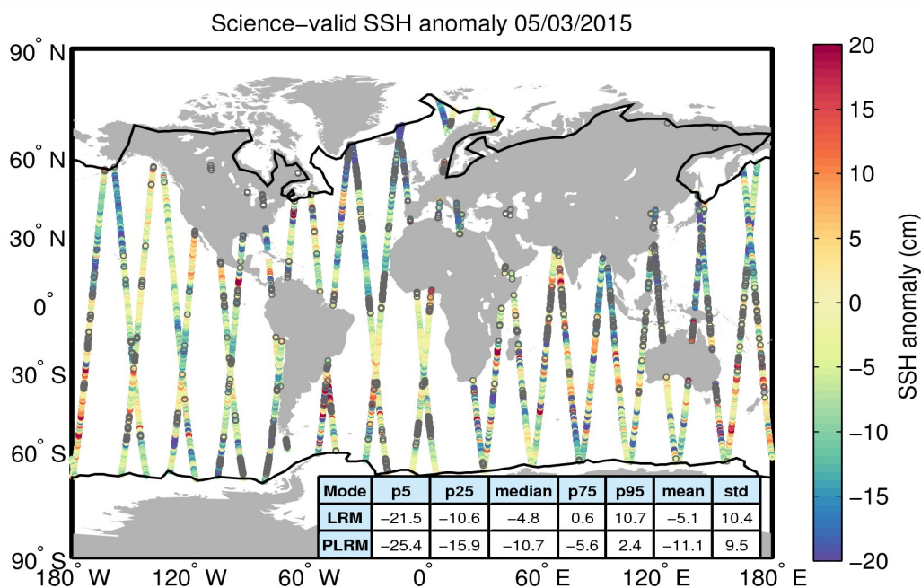
Figure 10. Geographical distribution of science-valid SSH anomaly data over oceans and lakes for 05/03/2015. The statistical values shown in the table refer to the SSH anomaly in cm and are calculated separately for LRM and PLRM regions. The black lines mark the outer limit of the Arctic and Antarctic polar polygons. Gray circles denote records that have been rejected based on the editing criteria described in Table 2.
