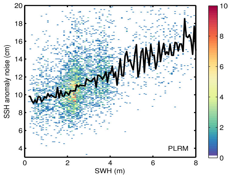
Figure 9. 2D histogram showing flag-valid SSH anomaly noise as a function of SWH for LRM (top) and PLRM (bottom) for 05/03/2015. The black line denotes the median SSH anomaly as a function of SWH.
