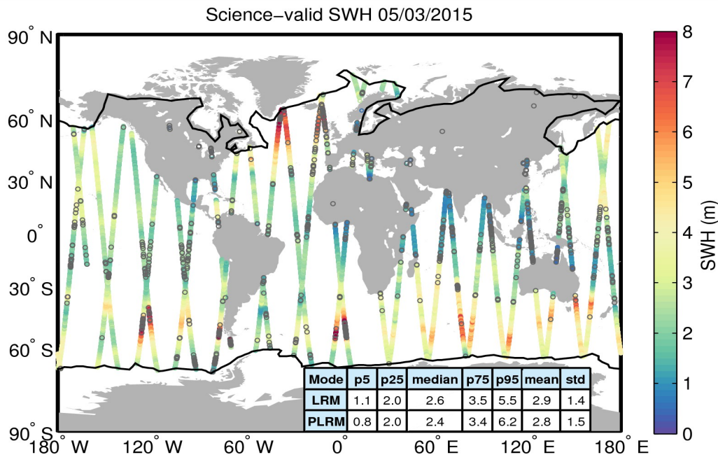
Figure 19. Geographical distribution of science-valid SWH data over oceans and lakes for 05/03/2015. The statistical values shown in the table refer to the SWH in m and are calculated separately for LRM and PLRM regions. The black lines mark the outer limit of the Arctic and Antarctic polar polygons. Gray circles denote records that have been rejected based on the editing criteria described in Table 3.
