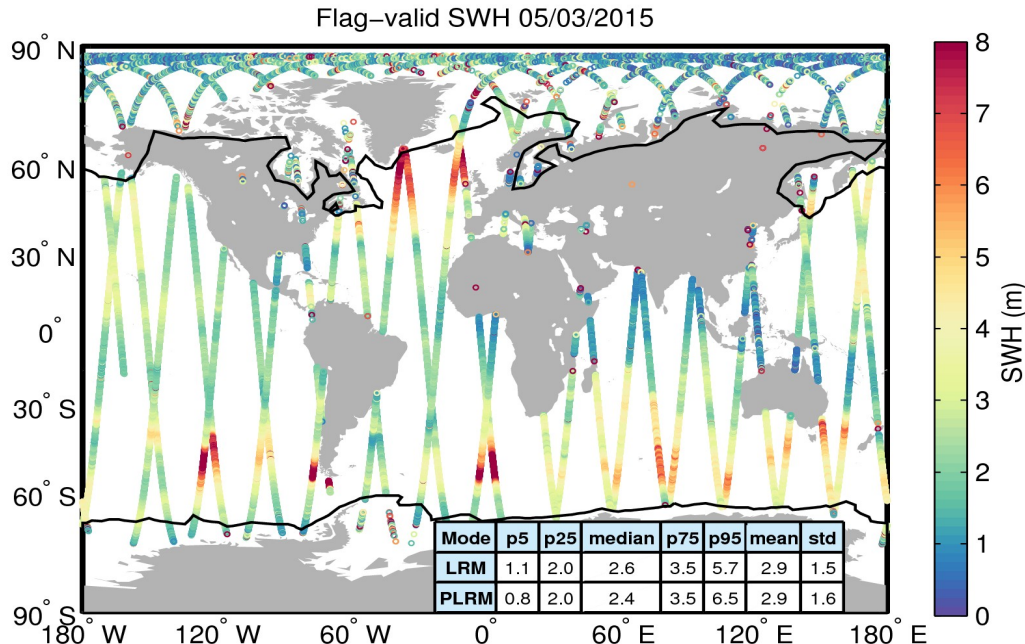
Figure 15. Geographical distribution of flag-valid SWH data over oceans and lakes for 05/03/2015. The statistical values shown in the table refer to the SWH in m and are calculated separately for LRM and PLRM regions. Measurements taken over polar polygons have been excluded from the computation of the statistical values. The black lines mark the outer limit of the Arctic and Antarctic polar polygons.
