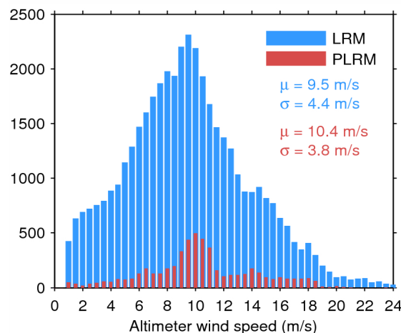
Figure 35. Histogram of science-valid wind over oceans and lakes for LRM (blue) and PLRM (red) for 05/03/2015. The mean ( \mu ) and standard deviation ( \sigma ) are also shown. Note that values larger than 24 m/s are excluded from the histogram for the sake of readability but not from the computation of \mu and \sigma .
