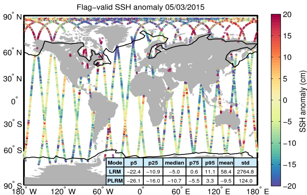
Figure 5. Geographical distribution of flag-valid 1-Hz SSH anomaly data over oceans and lakes for 05/03/2015. The statistical values shown in the table refer to the SSH anomaly in cm and are calculated separately for LRM and PLRM regions. Measurements taken over polar polygons have been excluded from the computation of the statistical values. The black lines mark the outer limit of the Arctic and Antarctic polar polygons.
