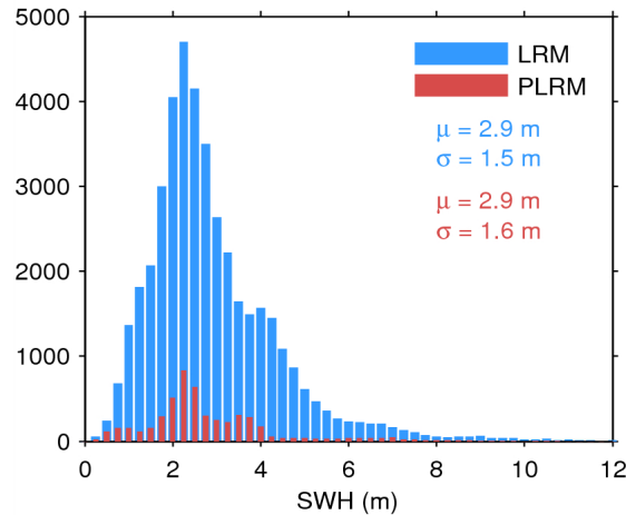
Figure 17. Histogram of flag-valid SWH over oceans and lakes for LRM (blue) and PLRM (red) for 05/03/2015. The mean ( \mu ) and standard deviation ( \sigma ) are also shown. Note that values larger than 12 m are excluded from the histogram for the sake of readability but not from the computation of \mu and \sigma .
