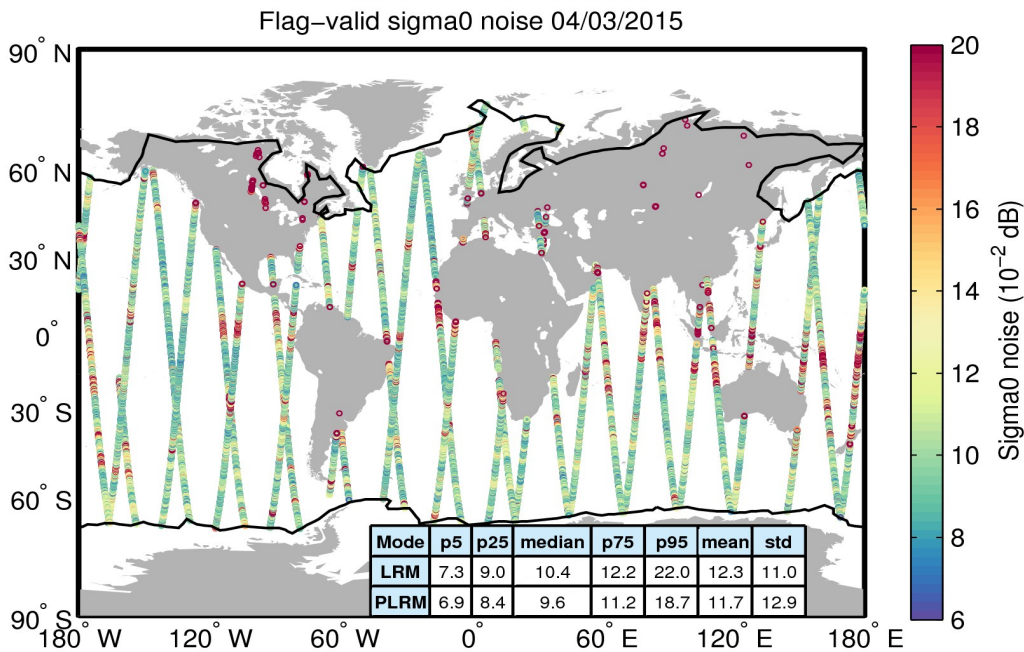
Figure 26. Geographical distribution of flag-valid 20-Hz sigma0 measurement noise over oceans and lakes for 04/03/2015. The statistical values shown in the table refer to the sigma0 noise and are calculated separately for LRM and PLRM regions. Measurements taken over polar polygons have been excluded from the computation of the statistical values. The black lines mark the outer limit of the Arctic and Antarctic polar polygons.
