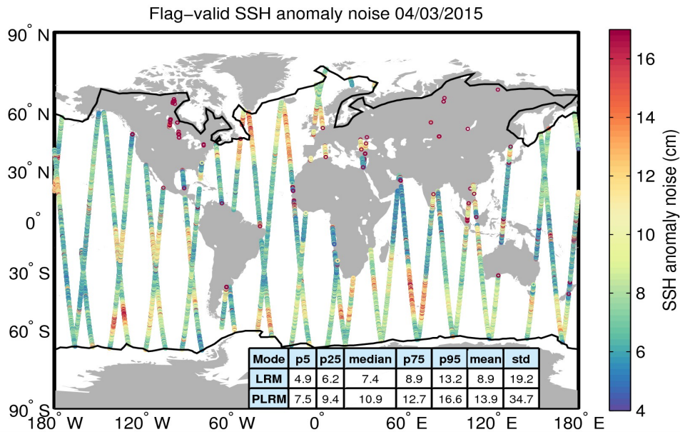
Figure 8. Geographical distribution of flag-valid 20-Hz SSH anomaly measurement noise over oceans and lakes for 04/03/2015. The statistical values shown in the table refer to the SSH anomaly noise and are calculated separately for LRM and PLRM regions. Measurements taken over polar polygons have been excluded from the computation of the statistical values. The black lines mark the outer limit of the Arctic and Antarctic polar polygons.
