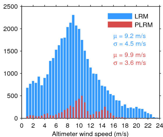
Figure 33. Histogram of flag-valid wind over oceans and lakes for LRM (blue) and PLRM (red) for 04/03/2015. The mean ( \mu ) and standard deviation ( \sigma ) are also shown. Note that values larger than 24 m/s are excluded from the histogram for the sake of readability but not from the computation of \mu and \sigma .
