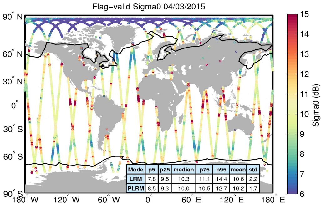
Figure 23. Geographical distribution of flag-valid sigma0 data over oceans and lakes for 04/03/2015. The statistical values shown in the table refer to the sigma0 in dB and are calculated separately for LRM and PLRM regions. Measurements taken over polar polygons have been excluded from the computation of the statistical values. The black lines mark the outer limit of the Arctic and Antarctic polar polygons.
