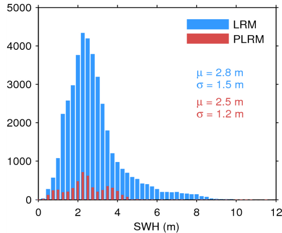
Figure 17. Histogram of flag-valid SWH over oceans and lakes for LRM (blue) and PLRM (red) for 04/03/2015. The mean ( \mu ) and standard deviation ( \sigma ) are also shown. Note that values larger than 12 m are excluded from the histogram for the sake of readability but not from the computation of \mu and \sigma .
