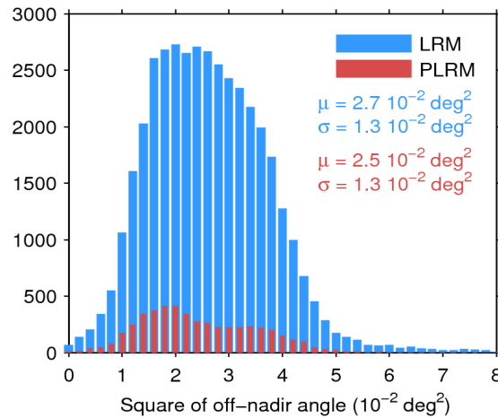
Figure 39. Histogram of flag-valid mispointing over oceans and lakes for LRM (blue) and PLRM (red) for 04/03/2015. Only positive values have been considered. The mean ( \mu ) and standard deviation ( \sigma ) are also shown. Note that values larger than 8 \cdot 10^{-2} \text{ deg}^2 are excluded from the histogram for the sake of readability but not from the computation of \mu and \sigma .
