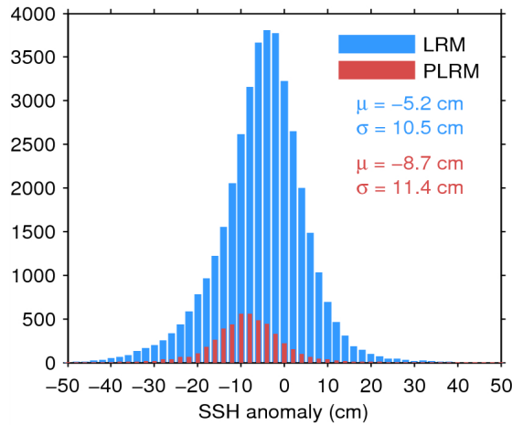
Figure 11. Histogram of science-valid SSH anomaly over oceans and lakes for LRM (blue) and PLRM (red) for 04/03/2015. The mean ( \mu ) and standard deviation ( \sigma ) are also shown. Note that values outside [-50\ 50] cm are excluded from the histogram for the sake of readability but not from the computation of \mu and \sigma .
