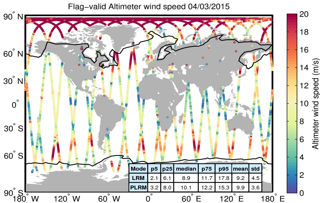
Figure 31. Geographical distribution of flag-valid wind data over oceans and lakes for 04/03/2015. The statistical values shown in the table refer to the wind in m/s and are calculated separately for LRM and PLRM regions. Measurements taken over polar polygons have been excluded from the computation of the statistical values. The black lines mark the outer limit of the Arctic and Antarctic polar polygons.
