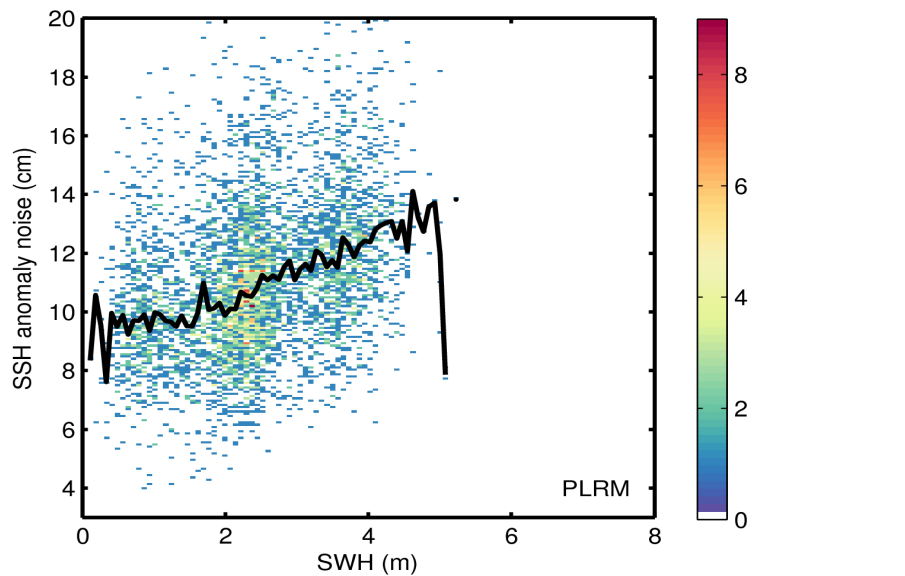
Figure 9. 2D histogram showing flag-valid SSH anomaly noise as a function of SWH for LRM (top) and PLRM (bottom) for 04/03/2015. The black line denotes the median SSH anomaly as a function of SWH.
