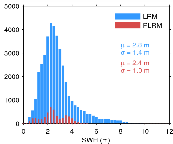
Figure 20. Histogram of science-valid SWH over oceans and lakes for LRM (blue) and PLRM (red) for 04/03/2015. The mean ( \mu ) and standard deviation ( \sigma ) are also shown. Note that values larger than 12 m are excluded from the histogram for the sake of readability but not from the computation of \mu and \sigma .
