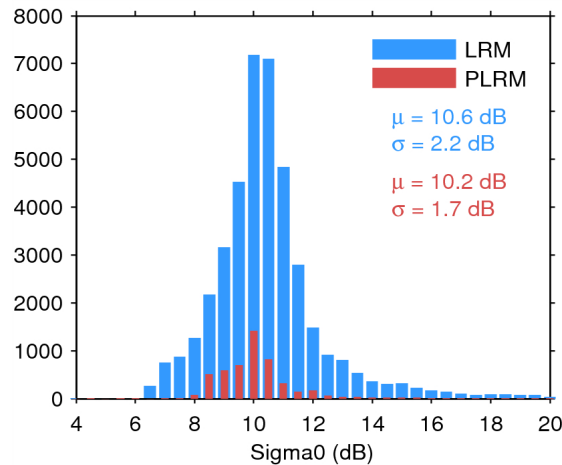
Figure 25. Histogram of flag-valid sigma0 over oceans and lakes for LRM (blue) and PLRM (red) for 04/03/2015. The mean ( \mu ) and standard deviation ( \sigma ) are also shown. Note that values outside [4 20] dB are excluded from the histogram for the sake of readability but not from the computation of \mu and \sigma .
