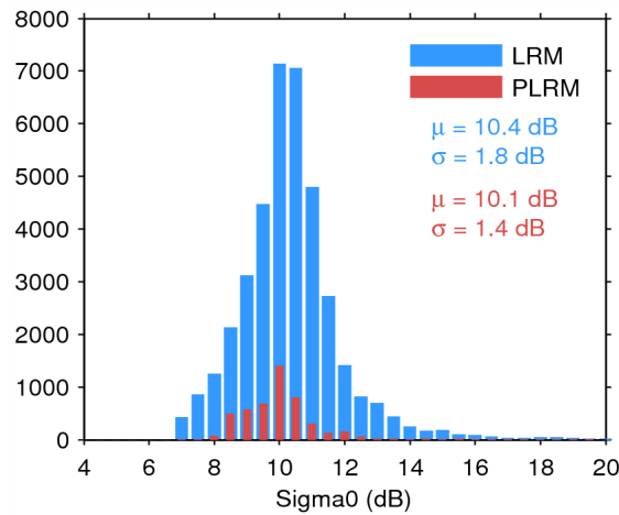
Figure 28. Histogram of science-valid sigma0 over oceans and lakes for LRM (blue) and PLRM (red) for 04/03/2015. The mean ( \mu ) and standard deviation ( \sigma ) are also shown. Note that values outside [4 20] dB are excluded from the histogram for the sake of readability but not from the computation of \mu and \sigma .
