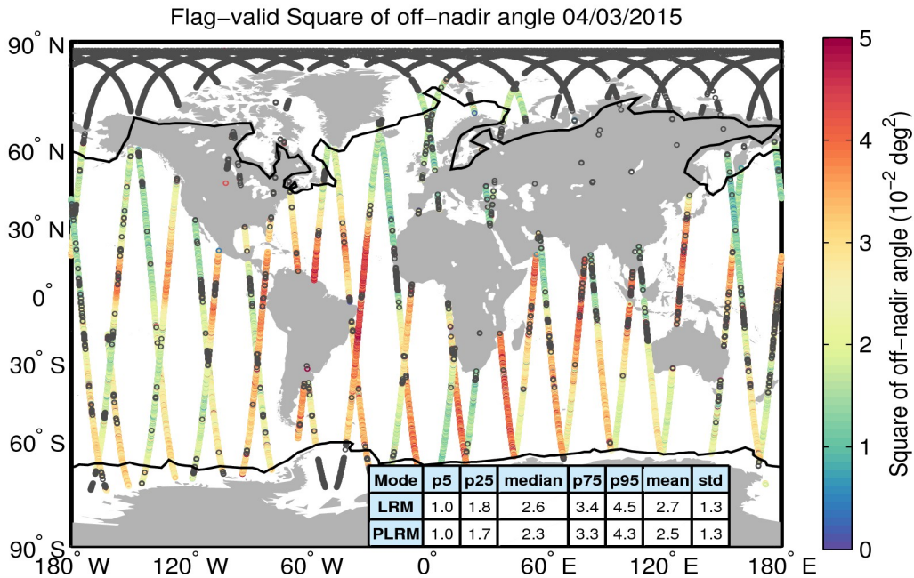
Figure 37. Geographical distribution of flag-valid mispointing data over oceans and lakes for 04/03/2015. The statistical values shown in the table refer to the mispointing in 10^{-2} \text{ deg}^2 and are calculated separately for LRM and PLRM regions. Measurements taken over polar polygons have been excluded from the computation of the statistical values. The black lines mark the outer limit of the Arctic and Antarctic polar polygons. Gray circles denote negative values.
