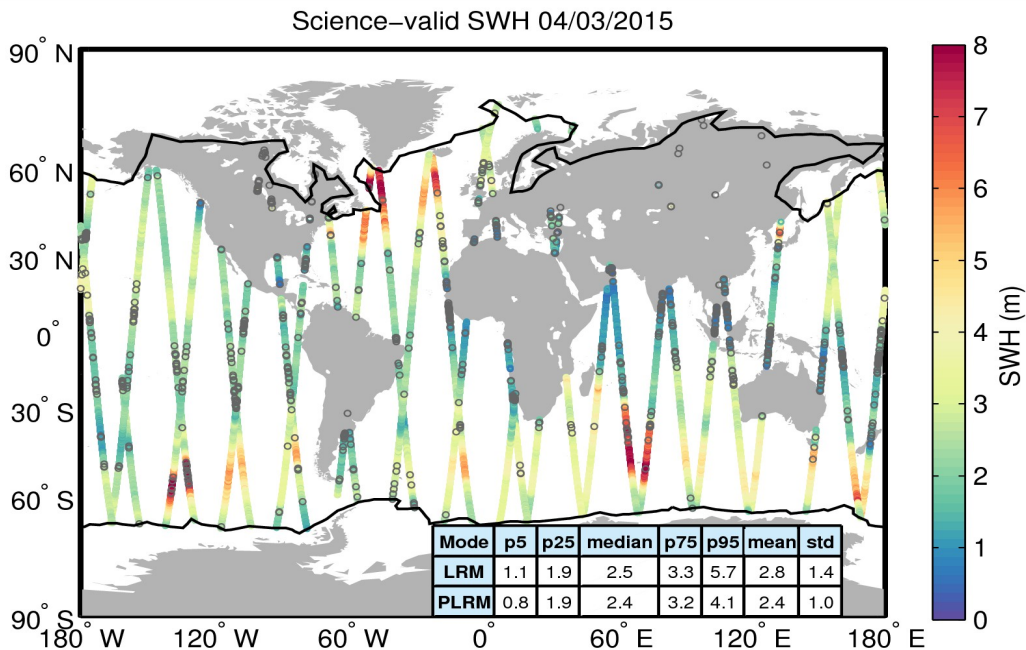
Figure 19. Geographical distribution of science-valid SWH data over oceans and lakes for 04/03/2015. The statistical values shown in the table refer to the SWH in m and are calculated separately for LRM and PLRM regions. The black lines mark the outer limit of the Arctic and Antarctic polar polygons. Gray circles denote records that have been rejected based on the editing criteria described in Table 3.
