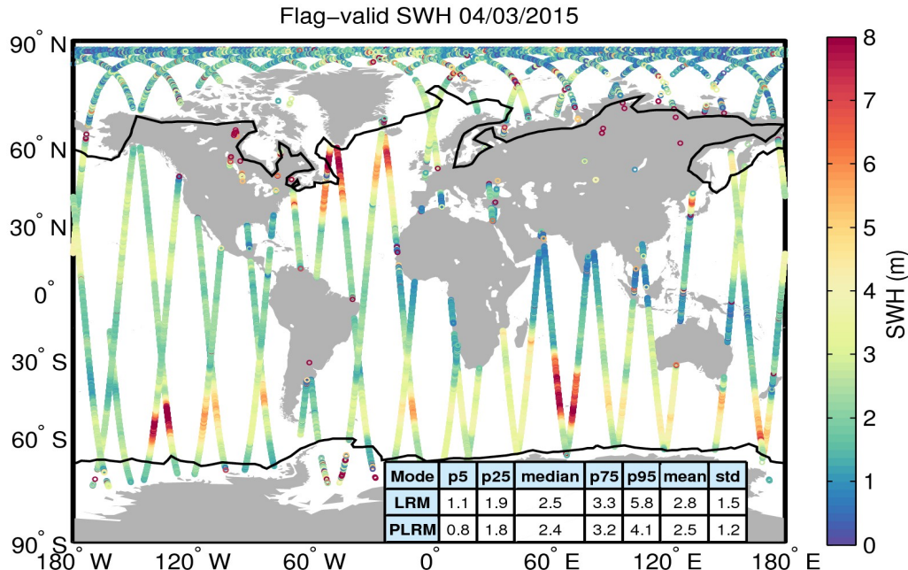
Figure 15. Geographical distribution of flag-valid SWH data over oceans and lakes for 04/03/2015. The statistical values shown in the table refer to the SWH in m and are calculated separately for LRM and PLRM regions. Measurements taken over polar polygons have been excluded from the computation of the statistical values. The black lines mark the outer limit of the Arctic and Antarctic polar polygons.
