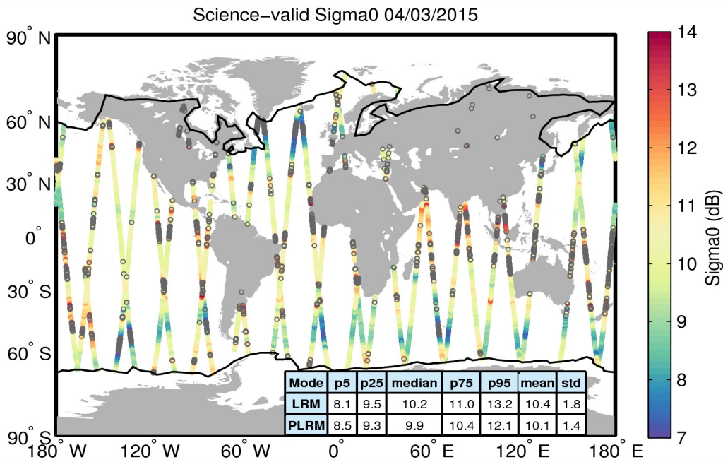
Figure 27. Geographical distribution of science-valid sigma0 data over oceans and lakes for 04/03/2015. The statistical values shown in the table refer to the sigma0 in dB and are calculated separately for LRM and PLRM regions. The black lines mark the outer limit of the Arctic and Antarctic polar polygons. Gray circles denote records that have been rejected based on the editing criteria described in Table 4.
