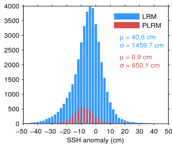
Figure 7. Histogram of flag-valid SSH anomaly over oceans and lakes for LRM (blue) and PLRM (red) for 04/03/2015. The mean ( \mu ) and standard deviation ( \sigma ) are also shown. Note that values outside [-50 \ 50] cm are excluded from the histogram for the sake of readability but not from the computation of \mu and \sigma .
