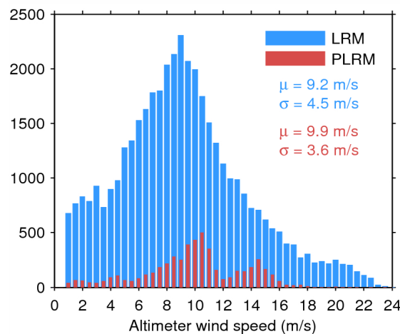
Figure 35. Histogram of science-valid wind over oceans and lakes for LRM (blue) and PLRM (red) for 04/03/2015. The mean ( \mu ) and standard deviation ( \sigma ) are also shown. Note that values larger than 24 m/s are excluded from the histogram for the sake of readability but not from the computation of \mu and \sigma .
