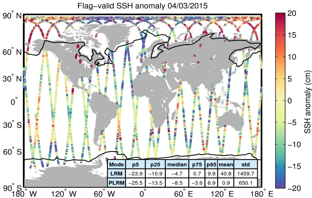
Figure 5. Geographical distribution of flag-valid 1-Hz SSH anomaly data over oceans and lakes for 04/03/2015. The statistical values shown in the table refer to the SSH anomaly in cm and are calculated separately for LRM and PLRM regions. Measurements taken over polar polygons have been excluded from the computation of the statistical values. The black lines mark the outer limit of the Arctic and Antarctic polar polygons.
