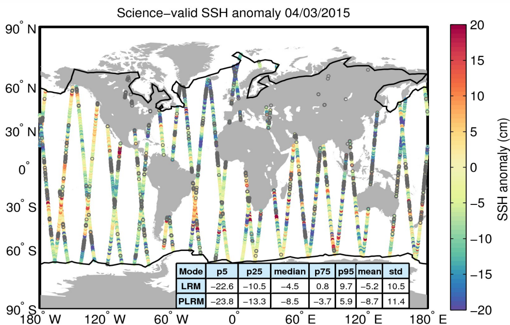
Figure 10. Geographical distribution of science-valid SSH anomaly data over oceans and lakes for 04/03/2015. The statistical values shown in the table refer to the SSH anomaly in cm and are calculated separately for LRM and PLRM regions. The black lines mark the outer limit of the Arctic and Antarctic polar polygons. Gray circles denote records that have been rejected based on the editing criteria described in Table 2.
