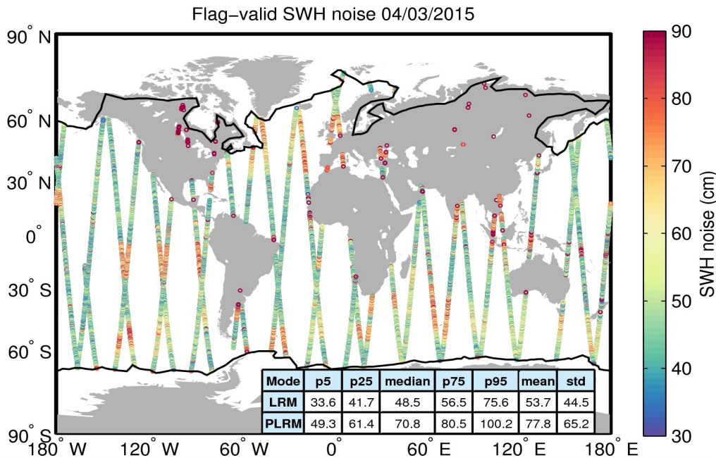
Figure 18. Geographical distribution of flag-valid 20-Hz SWH measurement noise over oceans and lakes for 04/03/2015. The statistical values shown in the table refer to the SWH noise and are calculated separately for LRM and PLRM regions. Measurements taken over polar polygons have been excluded from the computation of the statistical values. The black lines mark the outer limit of the Arctic and Antarctic polar polygons.
