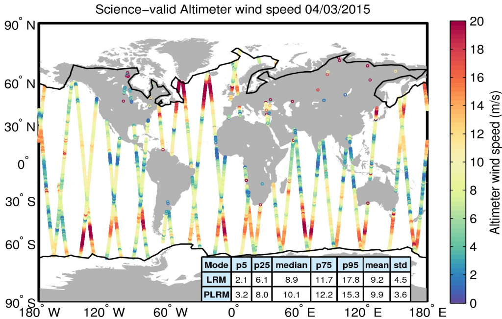
Figure 34. Geographical distribution of science-valid wind data over oceans and lakes for 04/03/2015. The statistical values shown in the table refer to the wind in m/s and are calculated separately for LRM and PLRM regions. The black lines mark the outer limit of the Arctic and Antarctic polar polygons. Gray circles denote records that have been rejected based on the editing criteria described in Table 5.
