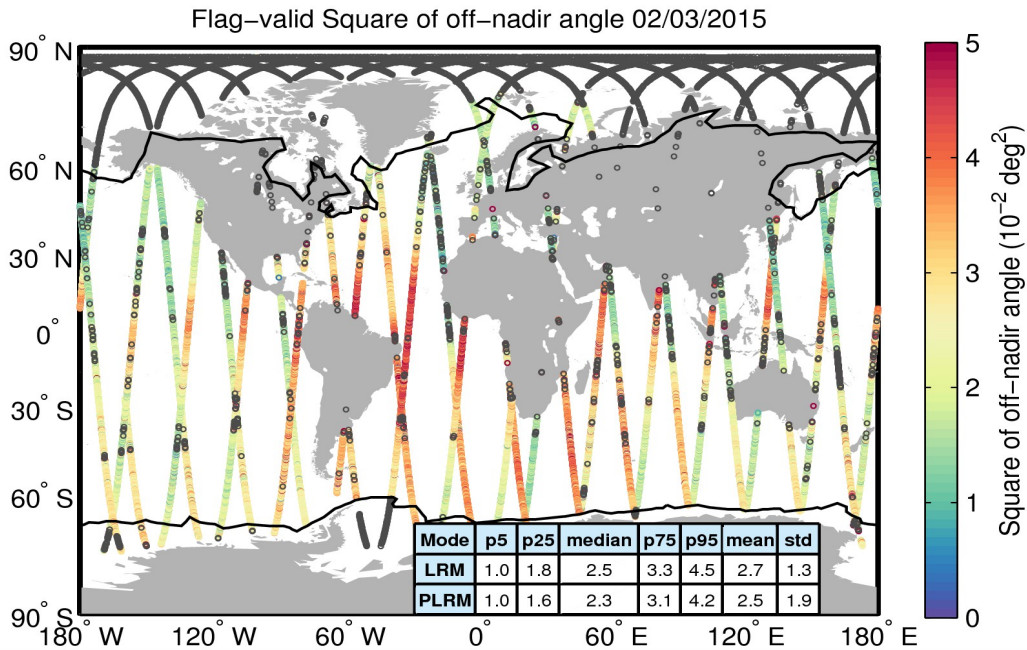
Figure 37. Geographical distribution of flag-valid mispointing data over oceans and lakes for 02/03/2015. The statistical values shown in the table refer to the mispointing in 10^{-2} \text{ deg}^2 and are calculated separately for LRM and PLRM regions. Measurements taken over polar polygons have been excluded from the computation of the statistical values. The black lines mark the outer limit of the Arctic and Antarctic polar polygons. Gray circles denote negative values.
