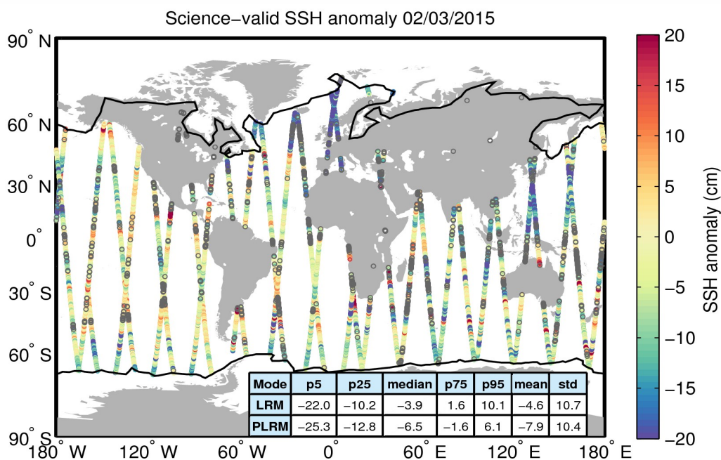
Figure 10. Geographical distribution of science-valid SSH anomaly data over oceans and lakes for 02/03/2015. The statistical values shown in the table refer to the SSH anomaly in cm and are calculated separately for LRM and PLRM regions. The black lines mark the outer limit of the Arctic and Antarctic polar polygons. Gray circles denote records that have been rejected based on the editing criteria described in Table 2.
