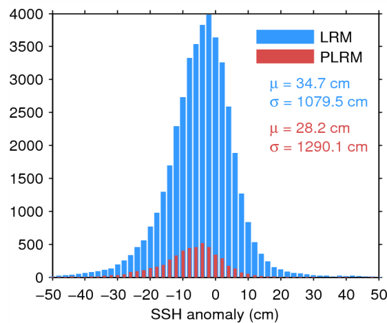
Figure 7. Histogram of flag-valid SSH anomaly over oceans and lakes for LRM (blue) and PLRM (red) for 02/03/2015. The mean ( \mu ) and standard deviation ( \sigma ) are also shown. Note that values outside [-50\ 50] cm are excluded from the histogram for the sake of readability but not from the computation of \mu and \sigma .
