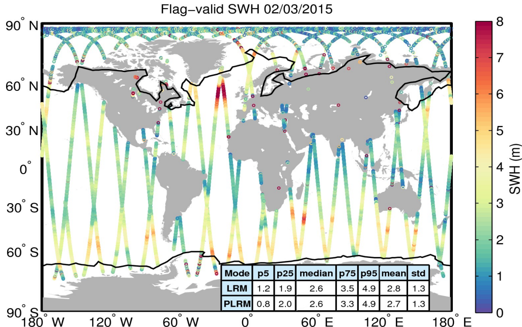
Figure 15. Geographical distribution of flag-valid SWH data over oceans and lakes for 02/03/2015. The statistical values shown in the table refer to the SWH in m and are calculated separately for LRM and PLRM regions. Measurements taken over polar polygons have been excluded from the computation of the statistical values. The black lines mark the outer limit of the Arctic and Antarctic polar polygons.
