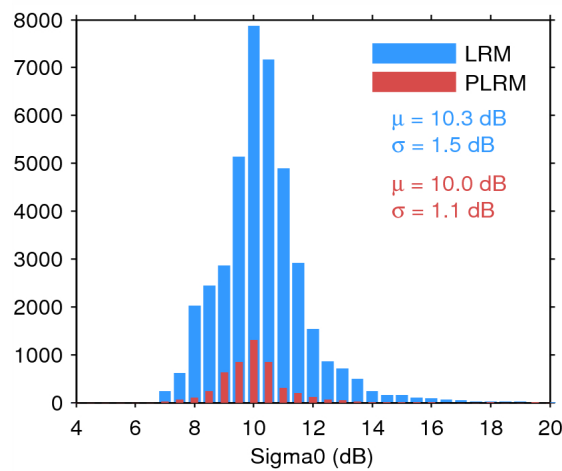
Figure 28. Histogram of science-valid sigma0 over oceans and lakes for LRM (blue) and PLRM (red) for 02/03/2015. The mean ( \mu ) and standard deviation ( \sigma ) are also shown. Note that values outside [4 20] dB are excluded from the histogram for the sake of readability but not from the computation of \mu and \sigma .
