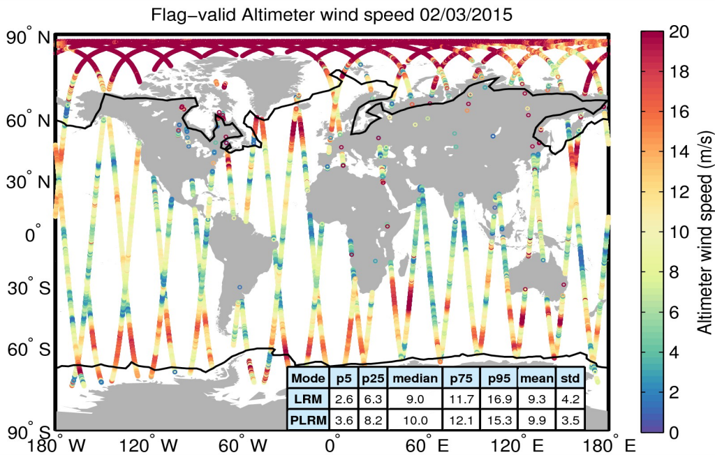
Figure 31. Geographical distribution of flag-valid wind data over oceans and lakes for 02/03/2015. The statistical values shown in the table refer to the wind in m/s and are calculated separately for LRM and PLRM regions. Measurements taken over polar polygons have been excluded from the computation of the statistical values. The black lines mark the outer limit of the Arctic and Antarctic polar polygons.
