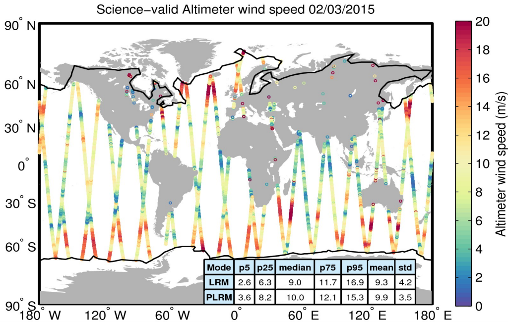
Figure 34. Geographical distribution of science-valid wind data over oceans and lakes for 02/03/2015. The statistical values shown in the table refer to the wind in m/s and are calculated separately for LRM and PLRM regions. The black lines mark the outer limit of the Arctic and Antarctic polar polygons. Gray circles denote records that have been rejected based on the editing criteria described in Table 5.
