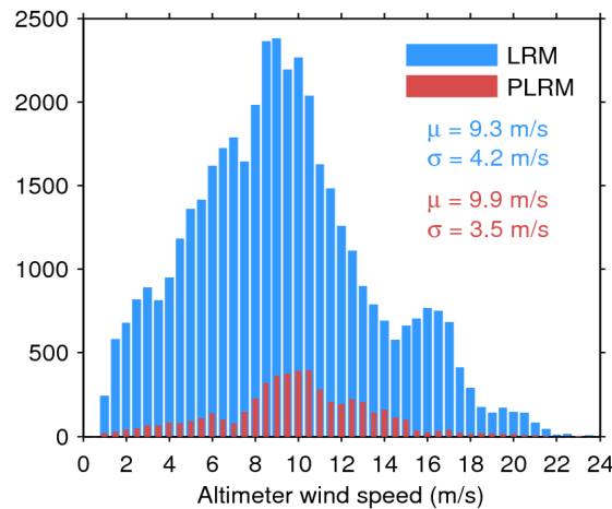
Figure 33. Histogram of flag-valid wind over oceans and lakes for LRM (blue) and PLRM (red) for 02/03/2015. The mean ( \mu ) and standard deviation ( \sigma ) are also shown. Note that values larger than 24 m/s are excluded from the histogram for the sake of readability but not from the computation of \mu and \sigma .
