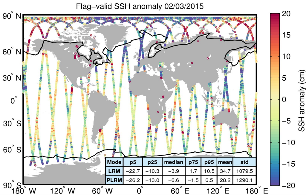
Figure 5. Geographical distribution of flag-valid 1-Hz SSH anomaly data over oceans and lakes for 02/03/2015. The statistical values shown in the table refer to the SSH anomaly in cm and are calculated separately for LRM and PLRM regions. Measurements taken over polar polygons have been excluded from the computation of the statistical values. The black lines mark the outer limit of the Arctic and Antarctic polar polygons.
