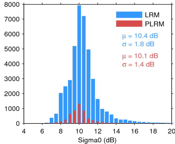
Figure 25. Histogram of flag-valid sigma0 over oceans and lakes for LRM (blue) and PLRM (red) for 02/03/2015. The mean ( \mu ) and standard deviation ( \sigma ) are also shown. Note that values outside [4 20] dB are excluded from the histogram for the sake of readability but not from the computation of \mu and \sigma .
