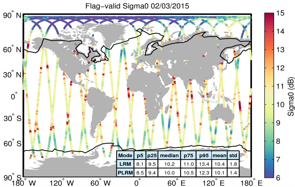
Figure 23. Geographical distribution of flag-valid sigma0 data over oceans and lakes for 02/03/2015. The statistical values shown in the table refer to the sigma0 in dB and are calculated separately for LRM and PLRM regions. Measurements taken over polar polygons have been excluded from the computation of the statistical values. The black lines mark the outer limit of the Arctic and Antarctic polar polygons.
