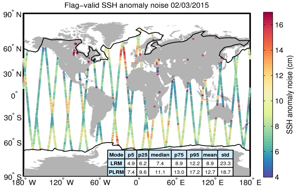
Figure 8. Geographical distribution of flag-valid 20-Hz SSH anomaly measurement noise over oceans and lakes for 02/03/2015. The statistical values shown in the table refer to the SSH anomaly noise and are calculated separately for LRM and PLRM regions. Measurements taken over polar polygons have been excluded from the computation of the statistical values. The black lines mark the outer limit of the Arctic and Antarctic polar polygons.
