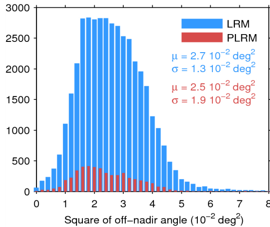
Figure 39. Histogram of flag-valid mispointing over oceans and lakes for LRM (blue) and PLRM (red) for 02/03/2015. Only positive values have been considered. The mean ( \mu ) and standard deviation ( \sigma ) are also shown. Note that values larger than 8 \cdot 10^{-2} \text{ deg}^2 are excluded from the histogram for the sake of readability but not from the computation of \mu and \sigma .
