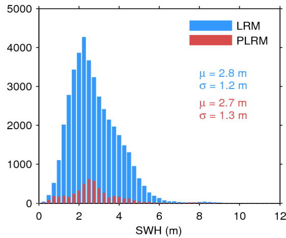
Figure 20. Histogram of science-valid SWH over oceans and lakes for LRM (blue) and PLRM (red) for 02/03/2015. The mean ( \mu ) and standard deviation ( \sigma ) are also shown. Note that values larger than 12 m are excluded from the histogram for the sake of readability but not from the computation of \mu and \sigma .
