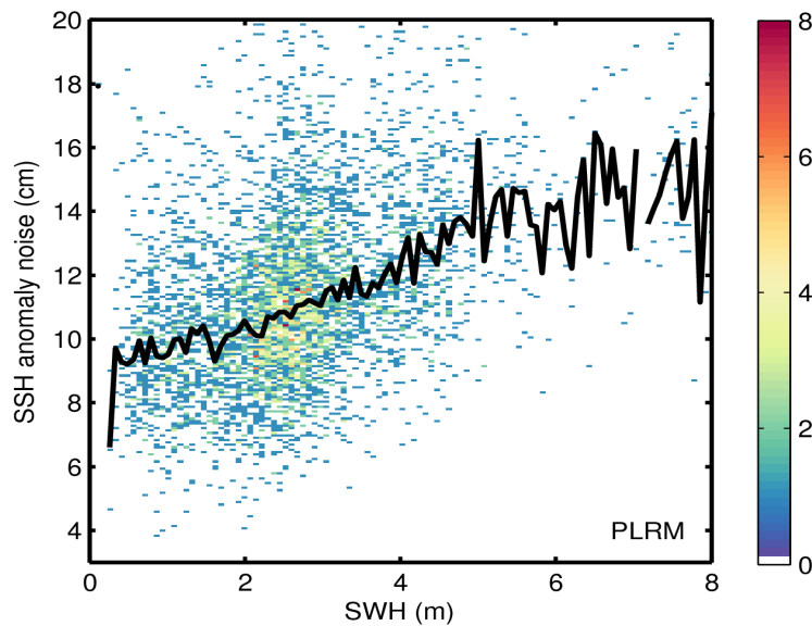
Figure 9. 2D histogram showing flag-valid SSH anomaly noise as a function of SWH for LRM (top) and PLRM (bottom) for 02/03/2015. The black line denotes the median SSH anomaly as a function of SWH.
