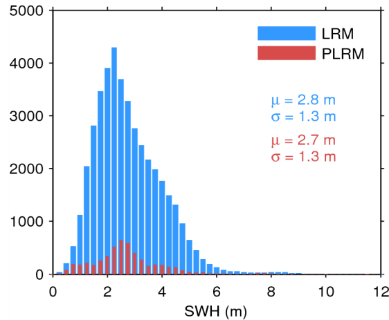
Figure 17. Histogram of flag-valid SWH over oceans and lakes for LRM (blue) and PLRM (red) for 02/03/2015. The mean ( \mu ) and standard deviation ( \sigma ) are also shown. Note that values larger than 12 m are excluded from the histogram for the sake of readability but not from the computation of \mu and \sigma .
