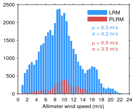
Figure 35. Histogram of science-valid wind over oceans and lakes for LRM (blue) and PLRM (red) for 02/03/2015. The mean ( \mu ) and standard deviation ( \sigma ) are also shown. Note that values larger than 24 m/s are excluded from the histogram for the sake of readability but not from the computation of \mu and \sigma .
