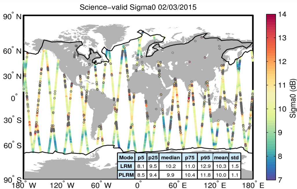
Figure 27. Geographical distribution of science-valid sigma0 data over oceans and lakes for 02/03/2015. The statistical values shown in the table refer to the sigma0 in dB and are calculated separately for LRM and PLRM regions. The black lines mark the outer limit of the Arctic and Antarctic polar polygons. Gray circles denote records that have been rejected based on the editing criteria described in Table 4.
