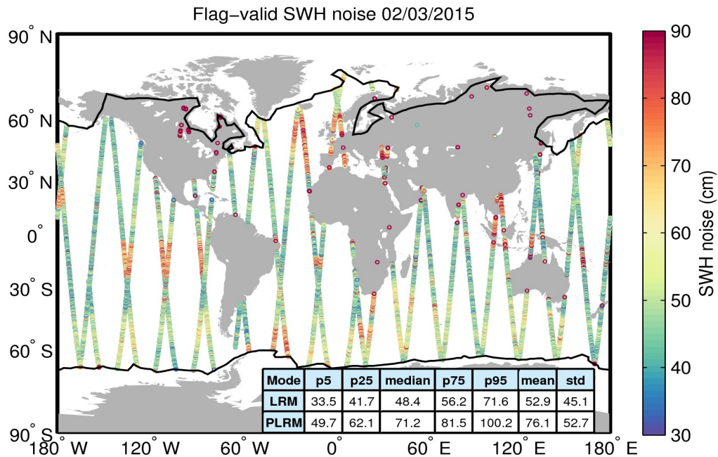
Figure 18. Geographical distribution of flag-valid 20-Hz SWH measurement noise over oceans and lakes for 02/03/2015. The statistical values shown in the table refer to the SWH noise and are calculated separately for LRM and PLRM regions. Measurements taken over polar polygons have been excluded from the computation of the statistical values. The black lines mark the outer limit of the Arctic and Antarctic polar polygons.
