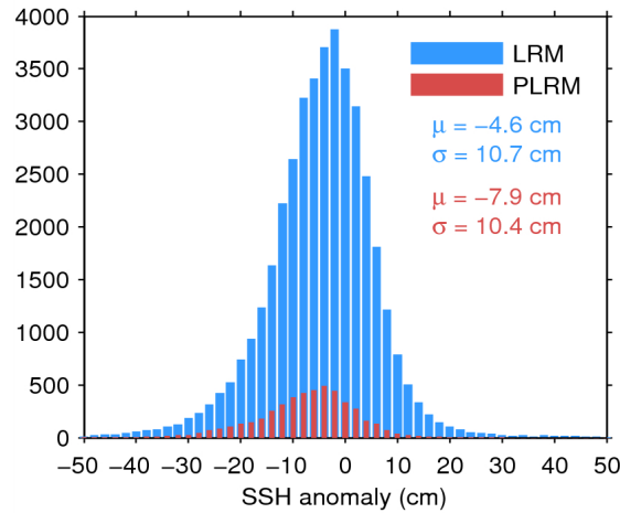
Figure 11. Histogram of science-valid SSH anomaly over oceans and lakes for LRM (blue) and PLRM (red) for 02/03/2015. The mean ( \mu ) and standard deviation ( \sigma ) are also shown. Note that values outside [-50\ 50] cm are excluded from the histogram for the sake of readability but not from the computation of \mu and \sigma .
