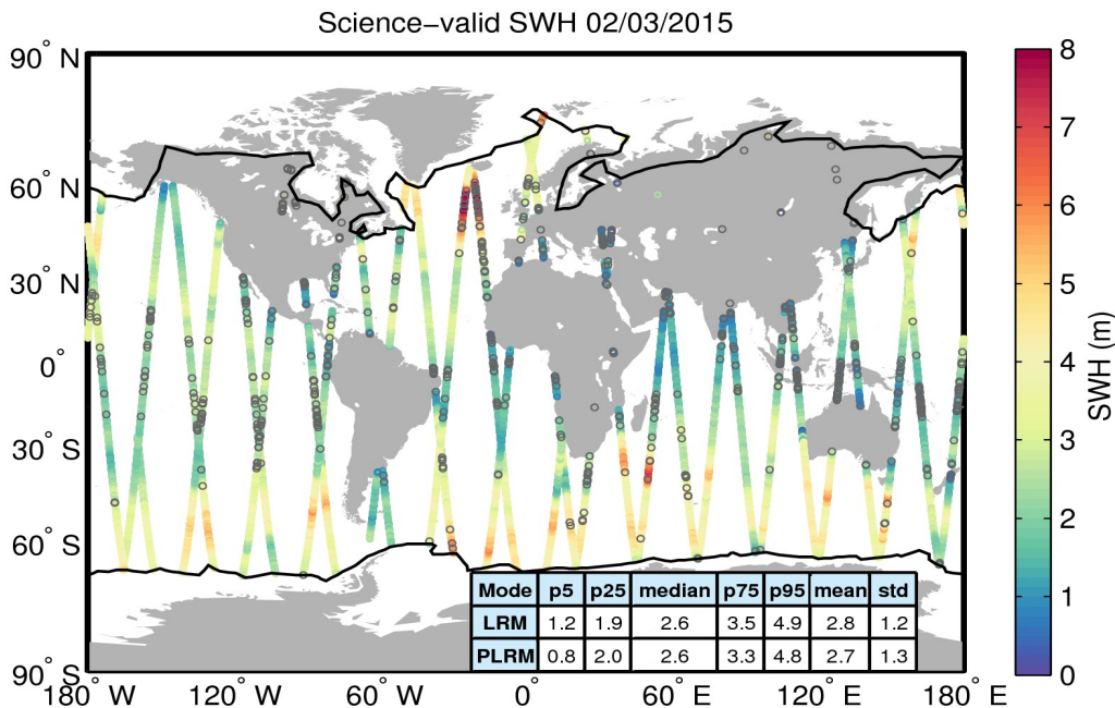
Figure 19. Geographical distribution of science-valid SWH data over oceans and lakes for 02/03/2015. The statistical values shown in the table refer to the SWH in m and are calculated separately for LRM and PLRM regions. The black lines mark the outer limit of the Arctic and Antarctic polar polygons. Gray circles denote records that have been rejected based on the editing criteria described in Table 3.
