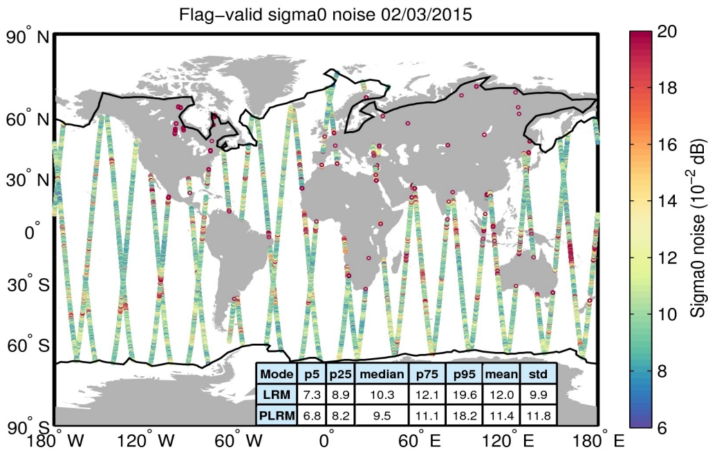
Figure 26. Geographical distribution of flag-valid 20-Hz sigma0 measurement noise over oceans and lakes for 02/03/2015. The statistical values shown in the table refer to the sigma0 noise and are calculated separately for LRM and PLRM regions. Measurements taken over polar polygons have been excluded from the computation of the statistical values. The black lines mark the outer limit of the Arctic and Antarctic polar polygons.
