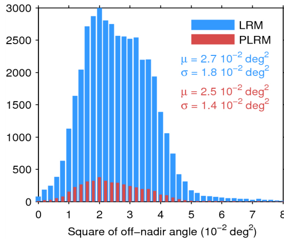
Figure 39. Histogram of flag-valid mispointing over oceans and lakes for LRM (blue) and PLRM (red) for 26/01/2015. Only positive values have been considered. The mean ( \mu ) and standard deviation ( \sigma ) are also shown. Note that values larger than 8 \cdot 10^{-2} \text{ deg}^2 are excluded from the histogram for the sake of readability but not from the computation of \mu and \sigma .
