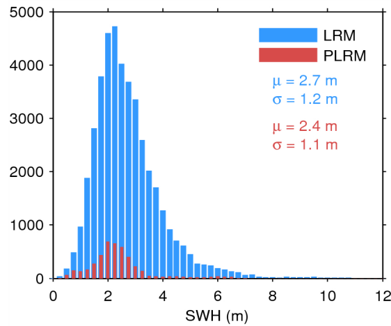
Figure 20. Histogram of science-valid SWH over oceans and lakes for LRM (blue) and PLRM (red) for 26/01/2015. The mean ( \mu ) and standard deviation ( \sigma ) are also shown. Note that values larger than 12 m are excluded from the histogram for the sake of readability but not from the computation of \mu and \sigma .
