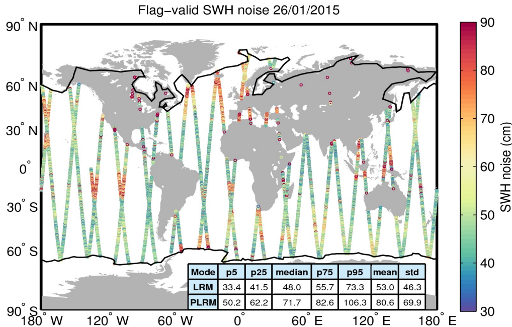
Figure 18. Geographical distribution of flag-valid 20-Hz SWH measurement noise over oceans and lakes for 26/01/2015. The statistical values shown in the table refer to the SWH noise and are calculated separately for LRM and PLRM regions. Measurements taken over polar polygons have been excluded from the computation of the statistical values. The black lines mark the outer limit of the Arctic and Antarctic polar polygons.
