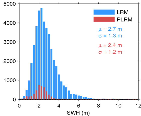
Figure 17. Histogram of flag-valid SWH over oceans and lakes for LRM (blue) and PLRM (red) for 26/01/2015. The mean ( \mu ) and standard deviation ( \sigma ) are also shown. Note that values larger than 12 m are excluded from the histogram for the sake of readability but not from the computation of \mu and \sigma .
