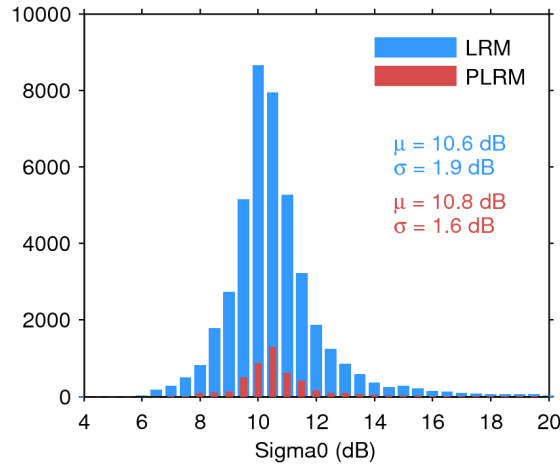
Figure 25. Histogram of flag-valid sigma0 over oceans and lakes for LRM (blue) and PLRM (red) for 26/01/2015. The mean ( \mu ) and standard deviation ( \sigma ) are also shown. Note that values outside [4 20] dB are excluded from the histogram for the sake of readability but not from the computation of \mu and \sigma .
