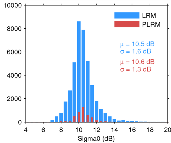
Figure 28. Histogram of science-valid sigma0 over oceans and lakes for LRM (blue) and PLRM (red) for 26/01/2015. The mean ( \mu ) and standard deviation ( \sigma ) are also shown. Note that values outside [4 20] dB are excluded from the histogram for the sake of readability but not from the computation of \mu and \sigma .
