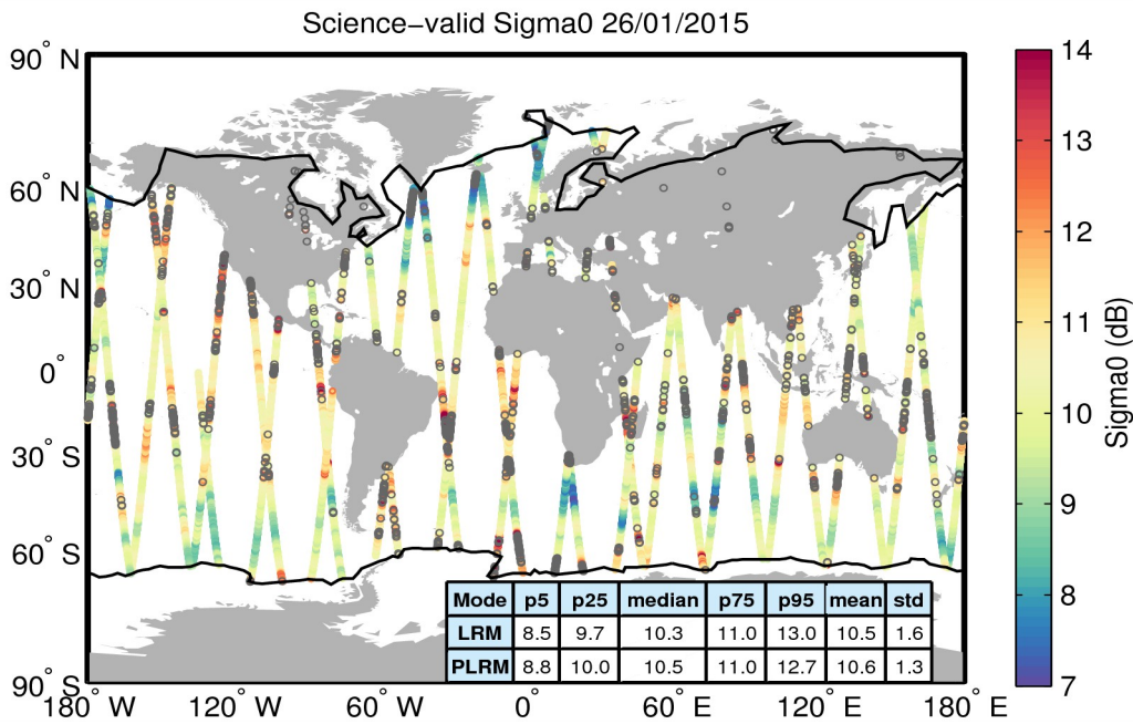
Figure 27. Geographical distribution of science-valid sigma0 data over oceans and lakes for 26/01/2015. The statistical values shown in the table refer to the sigma0 in dB and are calculated separately for LRM and PLRM regions. The black lines mark the outer limit of the Arctic and Antarctic polar polygons. Gray circles denote records that have been rejected based on the editing criteria described in Table 4.
