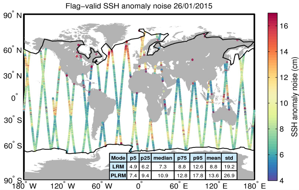
Figure 8. Geographical distribution of flag-valid 20-Hz SSH anomaly measurement noise over oceans and lakes for 26/01/2015. The statistical values shown in the table refer to the SSH anomaly noise and are calculated separately for LRM and PLRM regions. Measurements taken over polar polygons have been excluded from the computation of the statistical values. The black lines mark the outer limit of the Arctic and Antarctic polar polygons.
