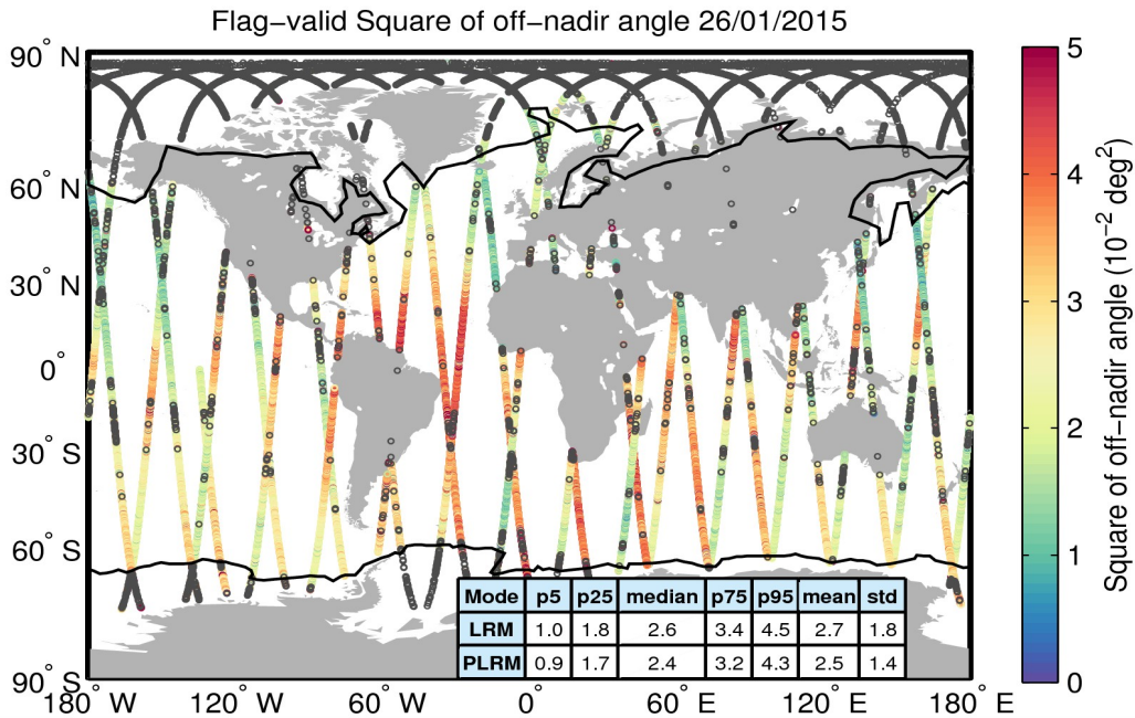
Figure 37. Geographical distribution of flag-valid mispointing data over oceans and lakes for 26/01/2015. The statistical values shown in the table refer to the mispointing in 10^{-2} \text{ deg}^2 and are calculated separately for LRM and PLRM regions. Measurements taken over polar polygons have been excluded from the computation of the statistical values. The black lines mark the outer limit of the Arctic and Antarctic polar polygons. Gray circles denote negative values.
