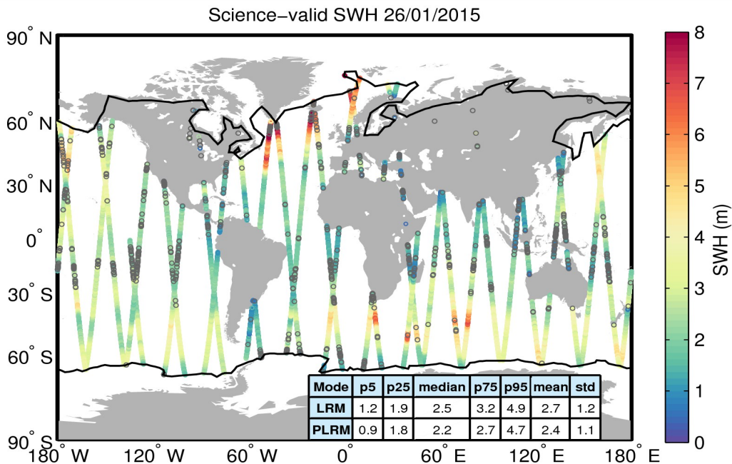
Figure 19. Geographical distribution of science-valid SWH data over oceans and lakes for 26/01/2015. The statistical values shown in the table refer to the SWH in m and are calculated separately for LRM and PLRM regions. The black lines mark the outer limit of the Arctic and Antarctic polar polygons. Gray circles denote records that have been rejected based on the editing criteria described in Table 3.
