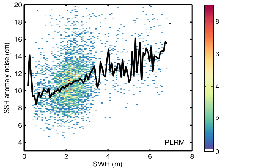
Figure 9. 2D histogram showing flag-valid SSH anomaly noise as a function of SWH for LRM (top) and PLRM (bottom) for 26/01/2015. The black line denotes the median SSH anomaly as a function of SWH.
