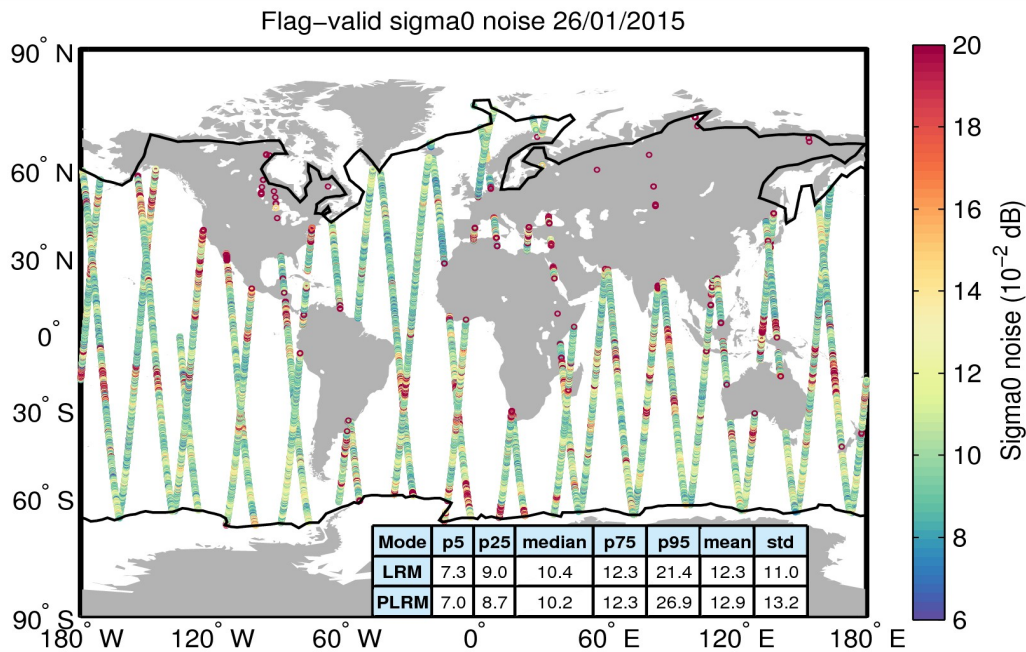
Figure 26. Geographical distribution of flag-valid 20-Hz sigma0 measurement noise over oceans and lakes for 26/01/2015. The statistical values shown in the table refer to the sigma0 noise and are calculated separately for LRM and PLRM regions. Measurements taken over polar polygons have been excluded from the computation of the statistical values. The black lines mark the outer limit of the Arctic and Antarctic polar polygons.
