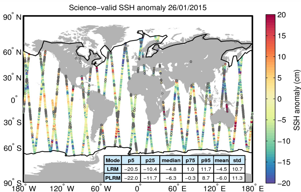
Figure 10. Geographical distribution of science-valid SSH anomaly data over oceans and lakes for 26/01/2015. The statistical values shown in the table refer to the SSH anomaly in cm and are calculated separately for LRM and PLRM regions. The black lines mark the outer limit of the Arctic and Antarctic polar polygons. Gray circles denote records that have been rejected based on the editing criteria described in Table 2.
