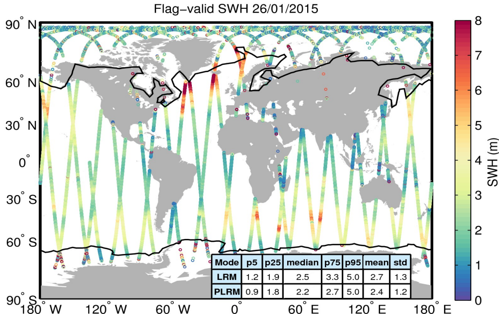
Figure 15. Geographical distribution of flag-valid SWH data over oceans and lakes for 26/01/2015. The statistical values shown in the table refer to the SWH in m and are calculated separately for LRM and PLRM regions. Measurements taken over polar polygons have been excluded from the computation of the statistical values. The black lines mark the outer limit of the Arctic and Antarctic polar polygons.
