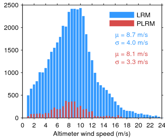
Figure 33. Histogram of flag-valid wind over oceans and lakes for LRM (blue) and PLRM (red) for 26/01/2015. The mean ( \mu ) and standard deviation ( \sigma ) are also shown. Note that values larger than 24 m/s are excluded from the histogram for the sake of readability but not from the computation of \mu and \sigma .
