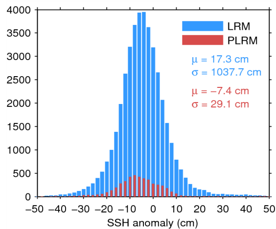
Figure 7. Histogram of flag-valid SSH anomaly over oceans and lakes for LRM (blue) and PLRM (red) for 26/01/2015. The mean ( \mu ) and standard deviation ( \sigma ) are also shown. Note that values outside [-50\ 50] cm are excluded from the histogram for the sake of readability but not from the computation of \mu and \sigma .
