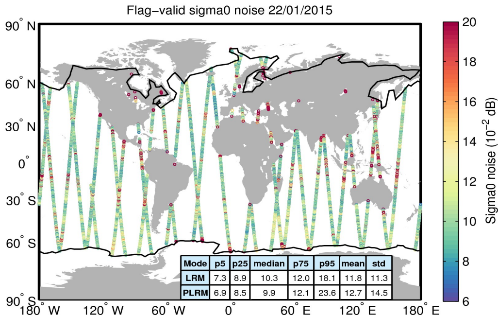
Figure 26. Geographical distribution of flag-valid 20-Hz sigma0 measurement noise over oceans and lakes for 22/01/2015. The statistical values shown in the table refer to the sigma0 noise and are calculated separately for LRM and PLRM regions. Measurements taken over polar polygons have been excluded from the computation of the statistical values. The black lines mark the outer limit of the Arctic and Antarctic polar polygons.
