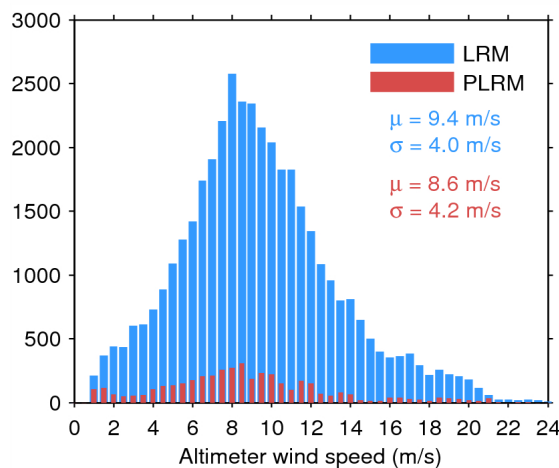
Figure 35. Histogram of science-valid wind over oceans and lakes for LRM (blue) and PLRM (red) for 22/01/2015. The mean ( \mu ) and standard deviation ( \sigma ) are also shown. Note that values larger than 24 m/s are excluded from the histogram for the sake of readability but not from the computation of \mu and \sigma .
