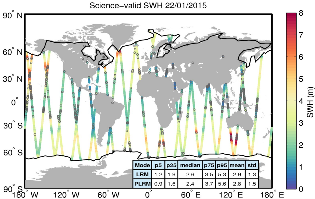
Figure 19. Geographical distribution of science-valid SWH data over oceans and lakes for 22/01/2015. The statistical values shown in the table refer to the SWH in m and are calculated separately for LRM and PLRM regions. The black lines mark the outer limit of the Arctic and Antarctic polar polygons. Gray circles denote records that have been rejected based on the editing criteria described in Table 3.
