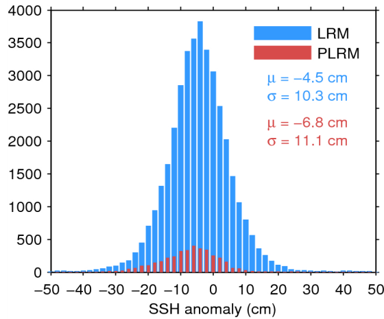
Figure 11. Histogram of science-valid SSH anomaly over oceans and lakes for LRM (blue) and PLRM (red) for 22/01/2015. The mean ( \mu ) and standard deviation ( \sigma ) are also shown. Note that values outside [-50 50] cm are excluded from the histogram for the sake of readability but not from the computation of \mu and \sigma .
