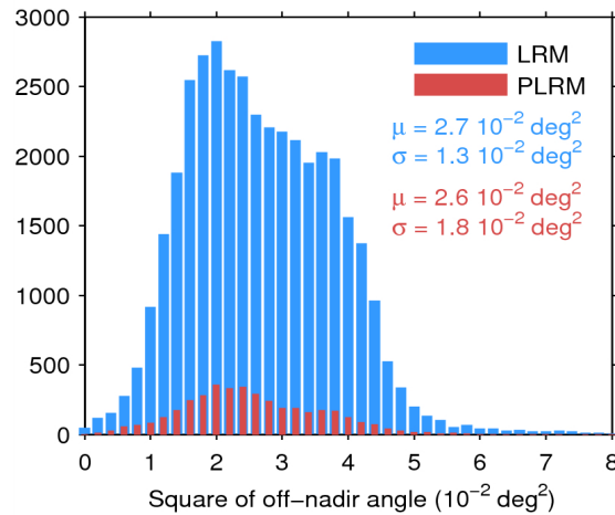
Figure 39. Histogram of flag-valid mispointing over oceans and lakes for LRM (blue) and PLRM (red) for 22/01/2015. Only positive values have been considered. The mean ( \mu ) and standard deviation ( \sigma ) are also shown. Note that values larger than 8 \cdot 10^{-2} \text{ deg}^2 are excluded from the histogram for the sake of readability but not from the computation of \mu and \sigma .
