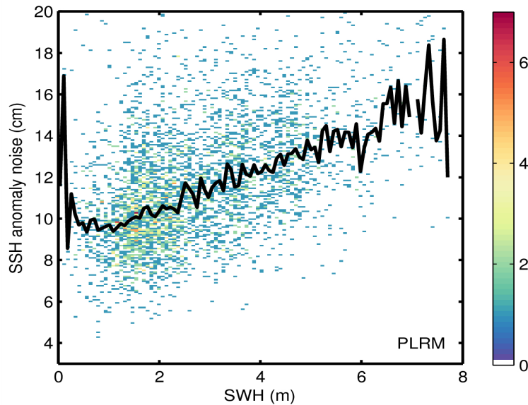
Figure 9. 2D histogram showing flag-valid SSH anomaly noise as a function of SWH for LRM (top) and PLRM (bottom) for 22/01/2015. The black line denotes the median SSH anomaly as a function of SWH.
