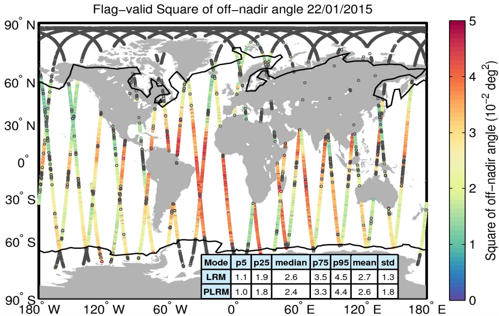
Figure 37. Geographical distribution of flag-valid mispointing data over oceans and lakes for 22/01/2015. The statistical values shown in the table refer to the mispointing in 10^{-2} \text{ deg}^2 and are calculated separately for LRM and PLRM regions. Measurements taken over polar polygons have been excluded from the computation of the statistical values. The black lines mark the outer limit of the Arctic and Antarctic polar polygons. Gray circles denote negative values.
