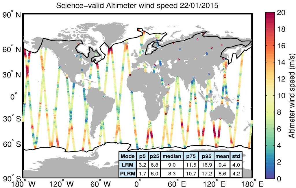
Figure 34. Geographical distribution of science-valid wind data over oceans and lakes for 22/01/2015. The statistical values shown in the table refer to the wind in m/s and are calculated separately for LRM and PLRM regions. The black lines mark the outer limit of the Arctic and Antarctic polar polygons. Gray circles denote records that have been rejected based on the editing criteria described in Table 5.
