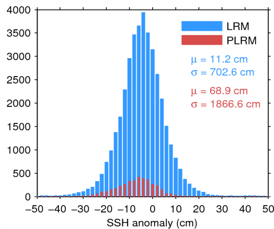
Figure 7. Histogram of flag-valid SSH anomaly over oceans and lakes for LRM (blue) and PLRM (red) for 22/01/2015. The mean ( \mu ) and standard deviation ( \sigma ) are also shown. Note that values outside [-50\ 50] cm are excluded from the histogram for the sake of readability but not from the computation of \mu and \sigma .
