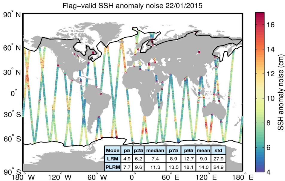
Figure 8. Geographical distribution of flag-valid 20-Hz SSH anomaly measurement noise over oceans and lakes for 22/01/2015. The statistical values shown in the table refer to the SSH anomaly noise and are calculated separately for LRM and PLRM regions. Measurements taken over polar polygons have been excluded from the computation of the statistical values. The black lines mark the outer limit of the Arctic and Antarctic polar polygons.
