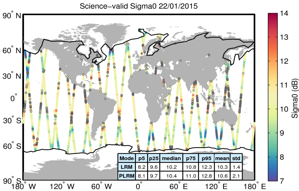
Figure 27. Geographical distribution of science-valid sigma0 data over oceans and lakes for 22/01/2015. The statistical values shown in the table refer to the sigma0 in dB and are calculated separately for LRM and PLRM regions. The black lines mark the outer limit of the Arctic and Antarctic polar polygons. Gray circles denote records that have been rejected based on the editing criteria described in Table 4.
