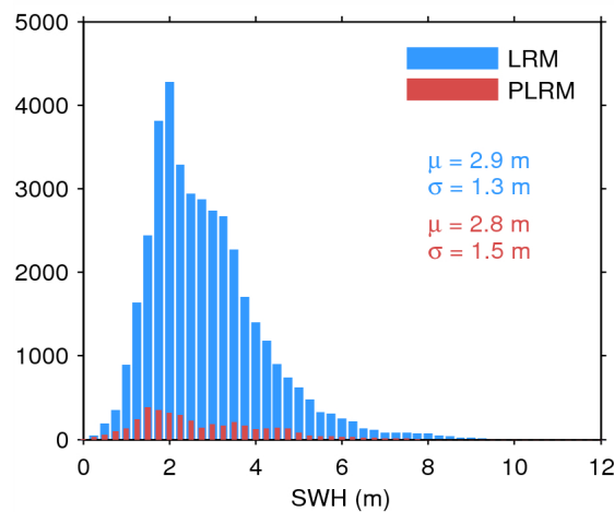
Figure 20. Histogram of science-valid SWH over oceans and lakes for LRM (blue) and PLRM (red) for 22/01/2015. The mean ( \mu ) and standard deviation ( \sigma ) are also shown. Note that values larger than 12 m are excluded from the histogram for the sake of readability but not from the computation of \mu and \sigma .
