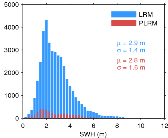
Figure 17. Histogram of flag-valid SWH over oceans and lakes for LRM (blue) and PLRM (red) for 22/01/2015. The mean ( \mu ) and standard deviation ( \sigma ) are also shown. Note that values larger than 12 m are excluded from the histogram for the sake of readability but not from the computation of \mu and \sigma .
