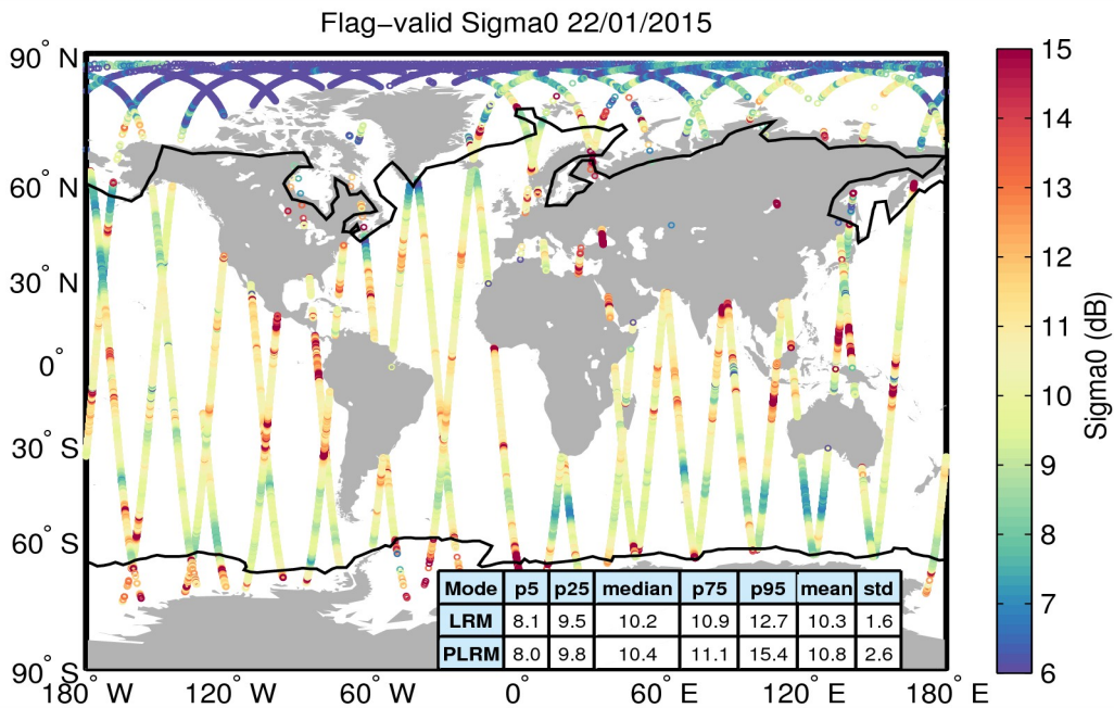
Figure 23. Geographical distribution of flag-valid sigma0 data over oceans and lakes for 22/01/2015. The statistical values shown in the table refer to the sigma0 in dB and are calculated separately for LRM and PLRM regions. Measurements taken over polar polygons have been excluded from the computation of the statistical values. The black lines mark the outer limit of the Arctic and Antarctic polar polygons.
