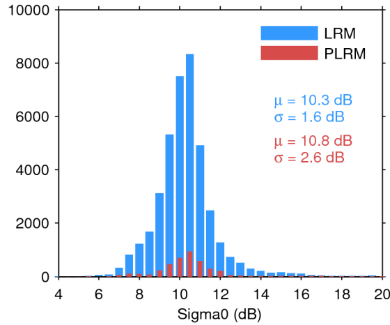
Figure 25. Histogram of flag-valid sigma0 over oceans and lakes for LRM (blue) and PLRM (red) for 22/01/2015. The mean ( \mu ) and standard deviation ( \sigma ) are also shown. Note that values outside [4 20] dB are excluded from the histogram for the sake of readability but not from the computation of \mu and \sigma .
