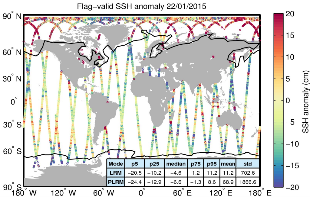
Figure 5. Geographical distribution of flag-valid 1-Hz SSH anomaly data over oceans and lakes for 22/01/2015. The statistical values shown in the table refer to the SSH anomaly in cm and are calculated separately for LRM and PLRM regions. Measurements taken over polar polygons have been excluded from the computation of the statistical values. The black lines mark the outer limit of the Arctic and Antarctic polar polygons.
