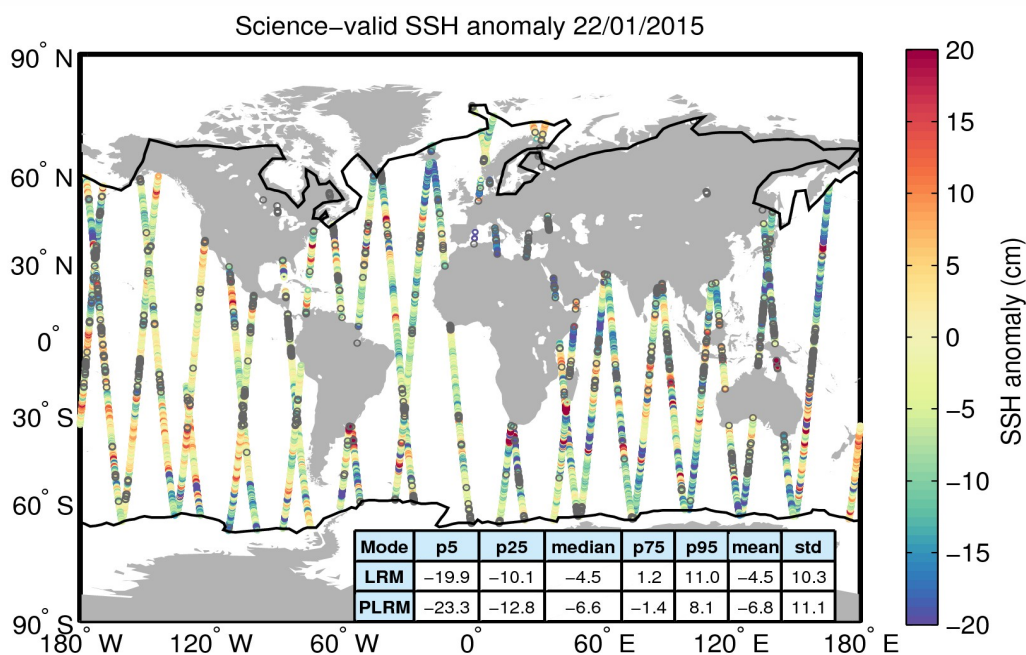
Figure 10. Geographical distribution of science-valid SSH anomaly data over oceans and lakes for 22/01/2015. The statistical values shown in the table refer to the SSH anomaly in cm and are calculated separately for LRM and PLRM regions. The black lines mark the outer limit of the Arctic and Antarctic polar polygons. Gray circles denote records that have been rejected based on the editing criteria described in Table 2.
