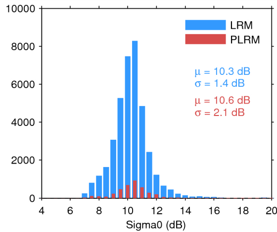
Figure 28. Histogram of science-valid sigma0 over oceans and lakes for LRM (blue) and PLRM (red) for 22/01/2015. The mean ( \mu ) and standard deviation ( \sigma ) are also shown. Note that values outside [4 20] dB are excluded from the histogram for the sake of readability but not from the computation of \mu and \sigma .
