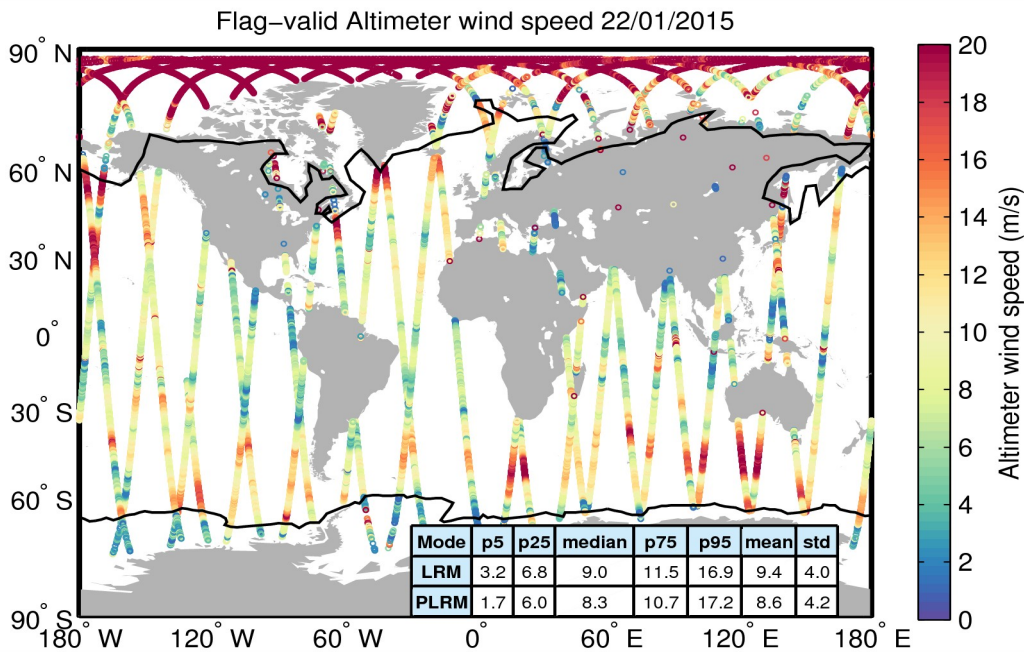
Figure 31. Geographical distribution of flag-valid wind data over oceans and lakes for 22/01/2015. The statistical values shown in the table refer to the wind in m/s and are calculated separately for LRM and PLRM regions. Measurements taken over polar polygons have been excluded from the computation of the statistical values. The black lines mark the outer limit of the Arctic and Antarctic polar polygons.
