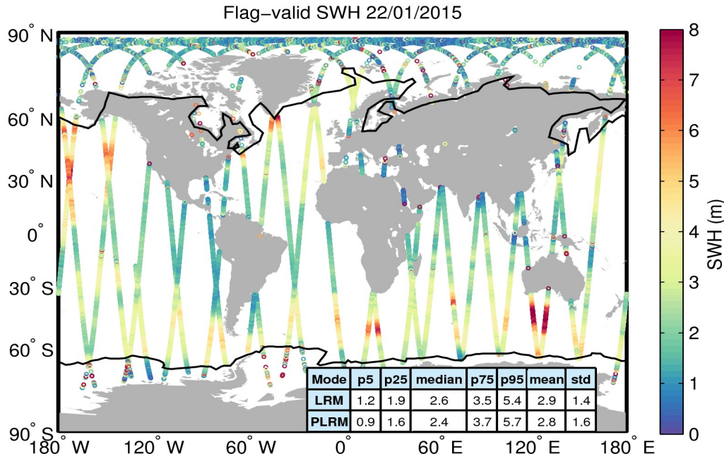
Figure 15. Geographical distribution of flag-valid SWH data over oceans and lakes for 22/01/2015. The statistical values shown in the table refer to the SWH in m and are calculated separately for LRM and PLRM regions. Measurements taken over polar polygons have been excluded from the computation of the statistical values. The black lines mark the outer limit of the Arctic and Antarctic polar polygons.
