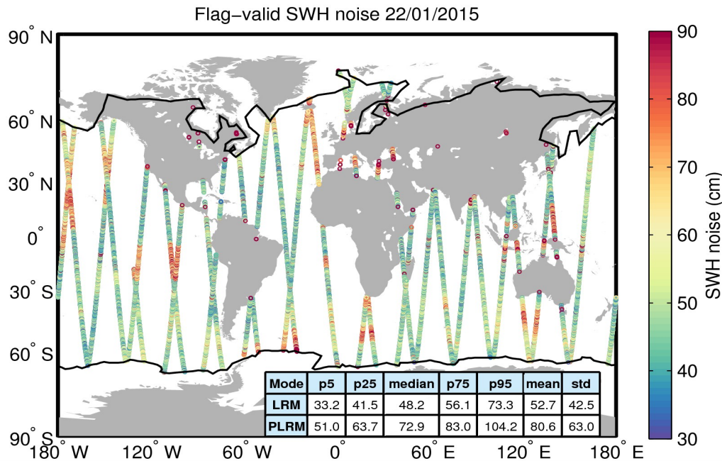
Figure 18. Geographical distribution of flag-valid 20-Hz SWH measurement noise over oceans and lakes for 22/01/2015. The statistical values shown in the table refer to the SWH noise and are calculated separately for LRM and PLRM regions. Measurements taken over polar polygons have been excluded from the computation of the statistical values. The black lines mark the outer limit of the Arctic and Antarctic polar polygons.
