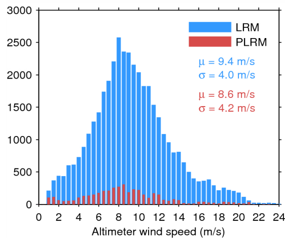
Figure 33. Histogram of flag-valid wind over oceans and lakes for LRM (blue) and PLRM (red) for 22/01/2015. The mean ( \mu ) and standard deviation ( \sigma ) are also shown. Note that values larger than 24 m/s are excluded from the histogram for the sake of readability but not from the computation of \mu and \sigma .
