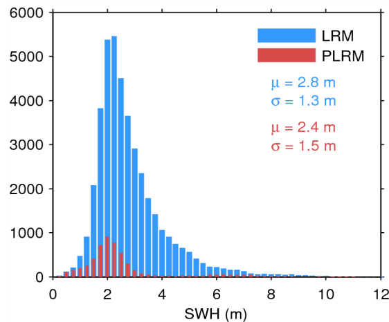
Figure 17. Histogram of flag-valid SWH over oceans and lakes for LRM (blue) and PLRM (red) for 13/01/2015. The mean ( \mu ) and standard deviation ( \sigma ) are also shown. Note that values larger than 12 m are excluded from the histogram for the sake of readability but not from the computation of \mu and \sigma .
