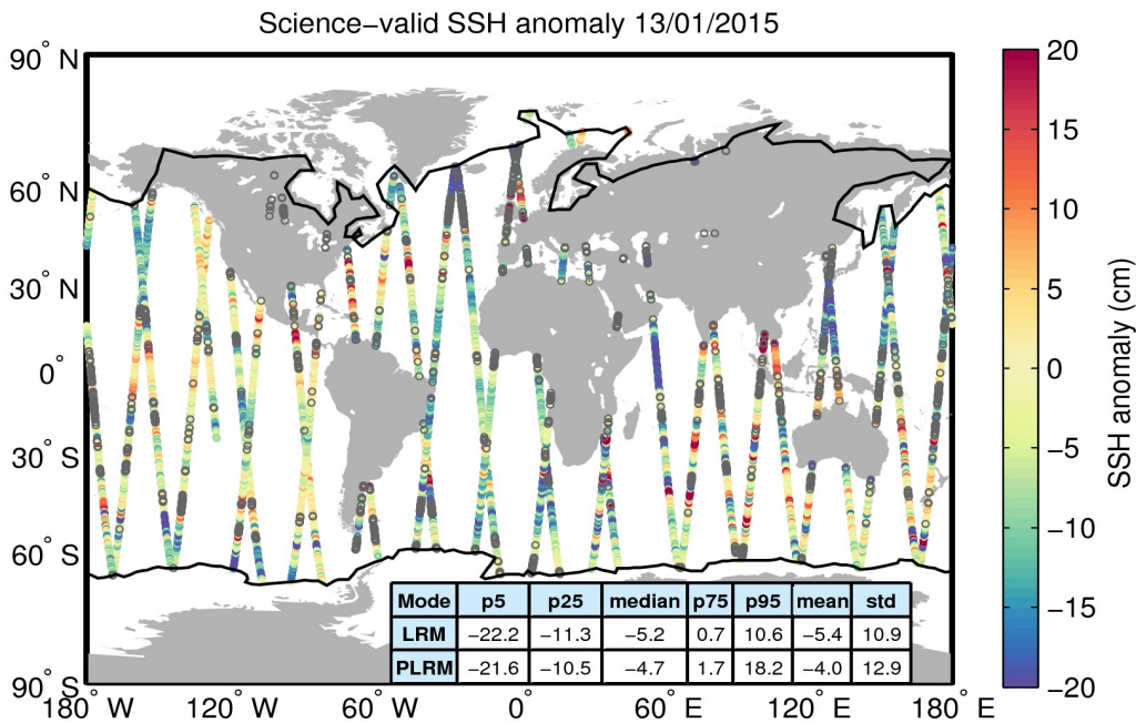
Figure 10. Geographical distribution of science-valid SSH anomaly data over oceans and lakes for 13/01/2015. The statistical values shown in the table refer to the SSH anomaly in cm and are calculated separately for LRM and PLRM regions. The black lines mark the outer limit of the Arctic and Antarctic polar polygons. Gray circles denote records that have been rejected based on the editing criteria described in Table 2.
