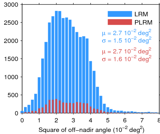
Figure 39. Histogram of flag-valid mispointing over oceans and lakes for LRM (blue) and PLRM (red) for 13/01/2015. Only positive values have been considered. The mean ( \mu ) and standard deviation ( \sigma ) are also shown. Note that values larger than 8 \cdot 10^{-2} \text{ deg}^2 are excluded from the histogram for the sake of readability but not from the computation of \mu and \sigma .
