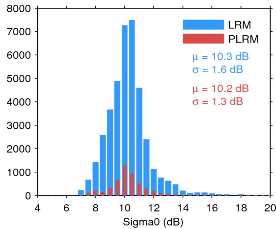
Figure 28. Histogram of science-valid sigma0 over oceans and lakes for LRM (blue) and PLRM (red) for 13/01/2015. The mean ( \mu ) and standard deviation ( \sigma ) are also shown. Note that values outside [4 20] dB are excluded from the histogram for the sake of readability but not from the computation of \mu and \sigma .
