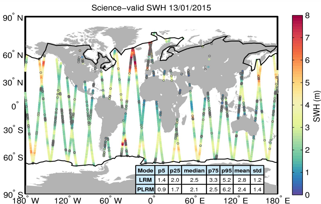
Figure 19. Geographical distribution of science-valid SWH data over oceans and lakes for 13/01/2015. The statistical values shown in the table refer to the SWH in m and are calculated separately for LRM and PLRM regions. The black lines mark the outer limit of the Arctic and Antarctic polar polygons. Gray circles denote records that have been rejected based on the editing criteria described in Table 3.
