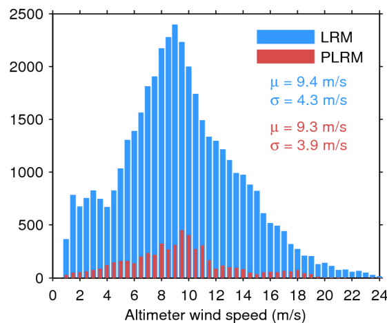
Figure 35. Histogram of science-valid wind over oceans and lakes for LRM (blue) and PLRM (red) for 13/01/2015. The mean ( \mu ) and standard deviation ( \sigma ) are also shown. Note that values larger than 24 m/s are excluded from the histogram for the sake of readability but not from the computation of \mu and \sigma .
