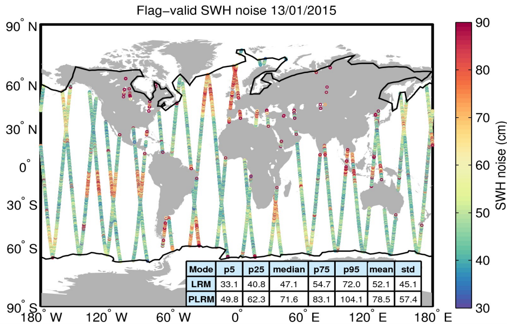
Figure 18. Geographical distribution of flag-valid 20-Hz SWH measurement noise over oceans and lakes for 13/01/2015. The statistical values shown in the table refer to the SWH noise and are calculated separately for LRM and PLRM regions. Measurements taken over polar polygons have been excluded from the computation of the statistical values. The black lines mark the outer limit of the Arctic and Antarctic polar polygons.
