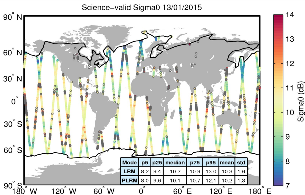
Figure 27. Geographical distribution of science-valid sigma0 data over oceans and lakes for 13/01/2015. The statistical values shown in the table refer to the sigma0 in dB and are calculated separately for LRM and PLRM regions. The black lines mark the outer limit of the Arctic and Antarctic polar polygons. Gray circles denote records that have been rejected based on the editing criteria described in Table 4.
