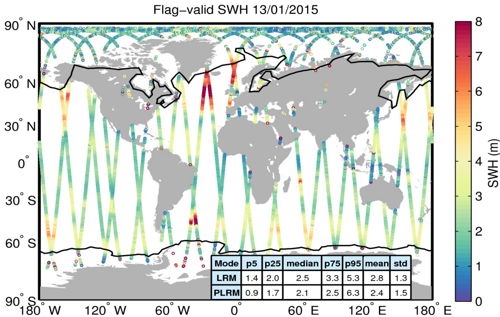
Figure 15. Geographical distribution of flag-valid SWH data over oceans and lakes for 13/01/2015. The statistical values shown in the table refer to the SWH in m and are calculated separately for LRM and PLRM regions. Measurements taken over polar polygons have been excluded from the computation of the statistical values. The black lines mark the outer limit of the Arctic and Antarctic polar polygons.
