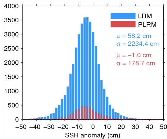
Figure 7. Histogram of flag-valid SSH anomaly over oceans and lakes for LRM (blue) and PLRM (red) for 13/01/2015. The mean ( \mu ) and standard deviation ( \sigma ) are also shown. Note that values outside [-50\ 50] cm are excluded from the histogram for the sake of readability but not from the computation of \mu and \sigma .
