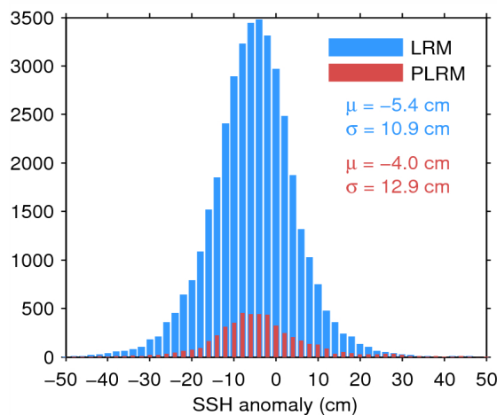
Figure 11. Histogram of science-valid SSH anomaly over oceans and lakes for LRM (blue) and PLRM (red) for 13/01/2015. The mean ( \mu ) and standard deviation ( \sigma ) are also shown. Note that values outside [-50 50] cm are excluded from the histogram for the sake of readability but not from the computation of \mu and \sigma .
