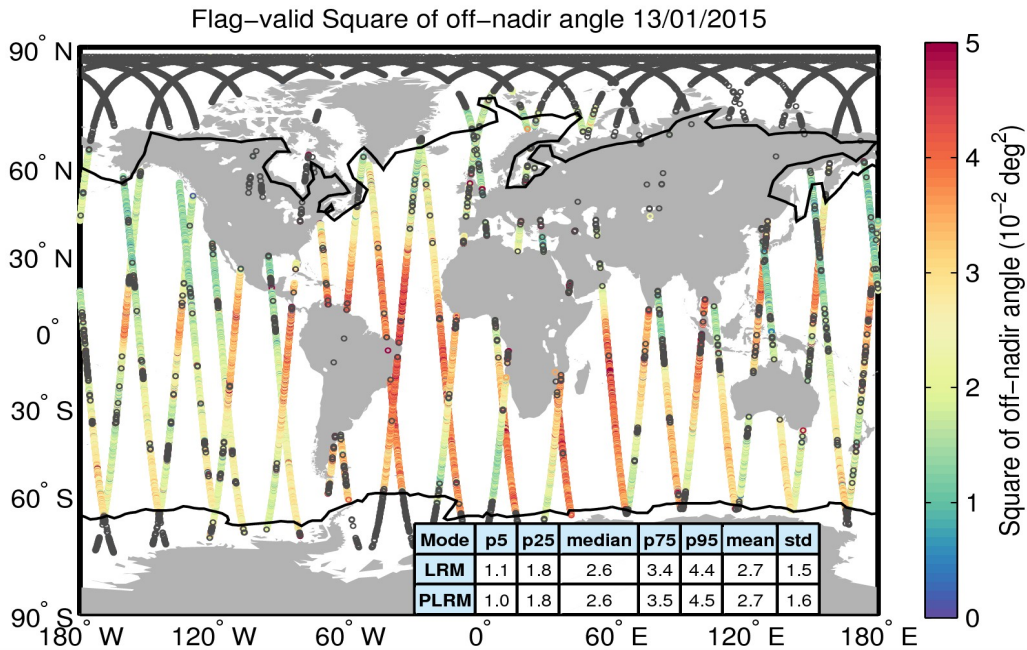
Figure 37. Geographical distribution of flag-valid mispointing data over oceans and lakes for 13/01/2015. The statistical values shown in the table refer to the mispointing in 10^{-2} \text{ deg}^2 and are calculated separately for LRM and PLRM regions. Measurements taken over polar polygons have been excluded from the computation of the statistical values. The black lines mark the outer limit of the Arctic and Antarctic polar polygons. Gray circles denote negative values.
