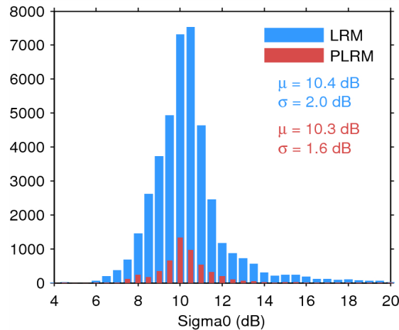
Figure 25. Histogram of flag-valid sigma0 over oceans and lakes for LRM (blue) and PLRM (red) for 13/01/2015. The mean ( \mu ) and standard deviation ( \sigma ) are also shown. Note that values outside [4 20] dB are excluded from the histogram for the sake of readability but not from the computation of \mu and \sigma .
