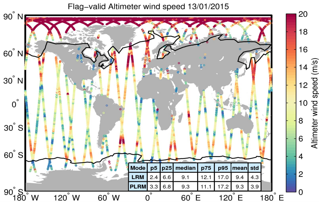
Figure 31. Geographical distribution of flag-valid wind data over oceans and lakes for 13/01/2015. The statistical values shown in the table refer to the wind in m/s and are calculated separately for LRM and PLRM regions. Measurements taken over polar polygons have been excluded from the computation of the statistical values. The black lines mark the outer limit of the Arctic and Antarctic polar polygons.
