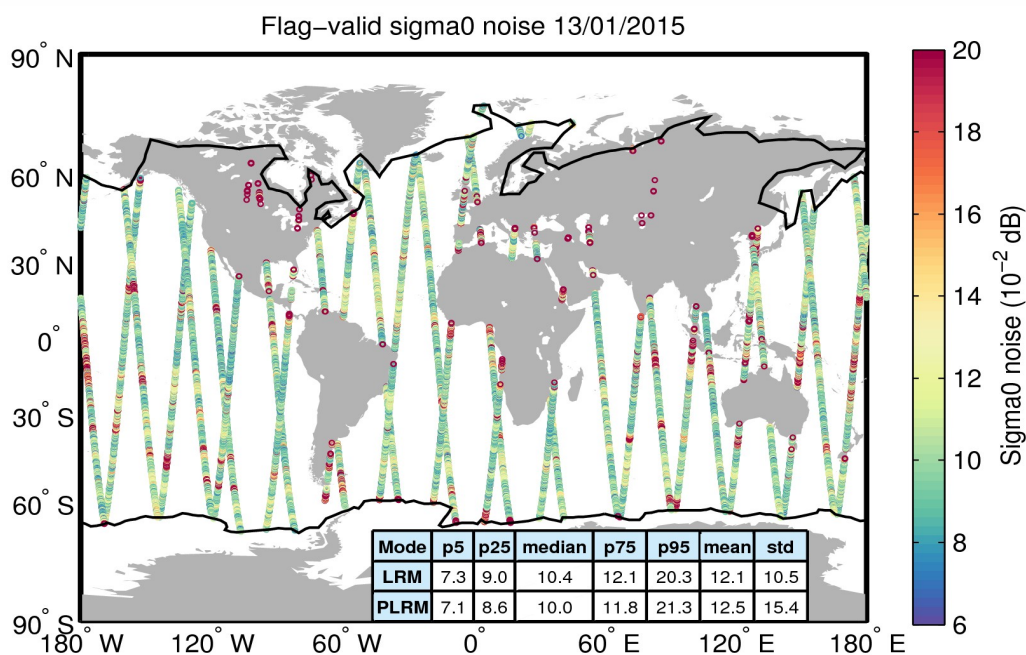
Figure 26. Geographical distribution of flag-valid 20-Hz sigma0 measurement noise over oceans and lakes for 13/01/2015. The statistical values shown in the table refer to the sigma0 noise and are calculated separately for LRM and PLRM regions. Measurements taken over polar polygons have been excluded from the computation of the statistical values. The black lines mark the outer limit of the Arctic and Antarctic polar polygons.
