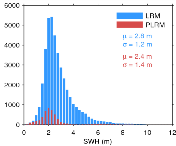
Figure 20. Histogram of science-valid SWH over oceans and lakes for LRM (blue) and PLRM (red) for 13/01/2015. The mean ( \mu ) and standard deviation ( \sigma ) are also shown. Note that values larger than 12 m are excluded from the histogram for the sake of readability but not from the computation of \mu and \sigma .
