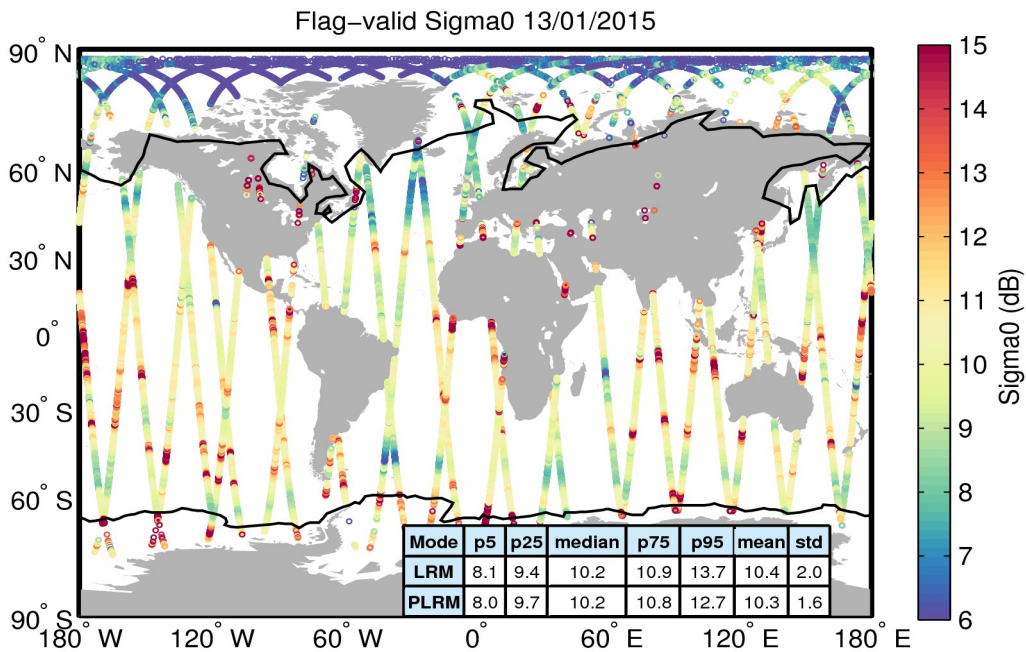
Figure 23. Geographical distribution of flag-valid sigma0 data over oceans and lakes for 13/01/2015. The statistical values shown in the table refer to the sigma0 in dB and are calculated separately for LRM and PLRM regions. Measurements taken over polar polygons have been excluded from the computation of the statistical values. The black lines mark the outer limit of the Arctic and Antarctic polar polygons.
