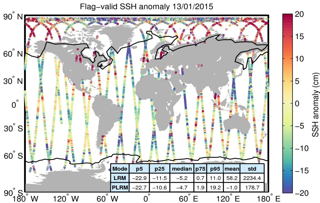
Figure 5. Geographical distribution of flag-valid 1-Hz SSH anomaly data over oceans and lakes for 13/01/2015. The statistical values shown in the table refer to the SSH anomaly in cm and are calculated separately for LRM and PLRM regions. Measurements taken over polar polygons have been excluded from the computation of the statistical values. The black lines mark the outer limit of the Arctic and Antarctic polar polygons.
