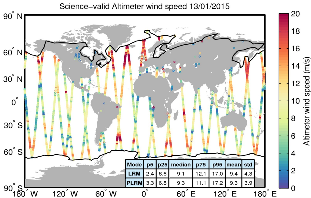
Figure 34. Geographical distribution of science-valid wind data over oceans and lakes for 13/01/2015. The statistical values shown in the table refer to the wind in m/s and are calculated separately for LRM and PLRM regions. The black lines mark the outer limit of the Arctic and Antarctic polar polygons. Gray circles denote records that have been rejected based on the editing criteria described in Table 5.
