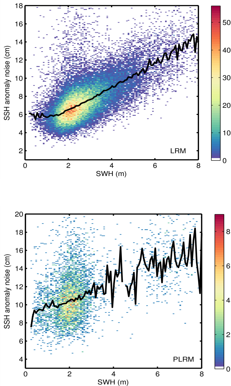
Figure 9. 2D histogram showing flag-valid SSH anomaly noise as a function of SWH for LRM (top) and PLRM (bottom) for 13/01/2015. The black line denotes the median SSH anomaly as a function of SWH.
