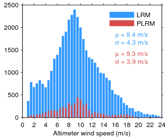
Figure 33. Histogram of flag-valid wind over oceans and lakes for LRM (blue) and PLRM (red) for 13/01/2015. The mean ( \mu ) and standard deviation ( \sigma ) are also shown. Note that values larger than 24 m/s are excluded from the histogram for the sake of readability but not from the computation of \mu and \sigma .
