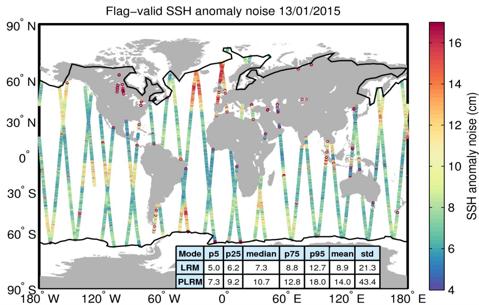
Figure 8. Geographical distribution of flag-valid 20-Hz SSH anomaly measurement noise over oceans and lakes for 13/01/2015. The statistical values shown in the table refer to the SSH anomaly noise and are calculated separately for LRM and PLRM regions. Measurements taken over polar polygons have been excluded from the computation of the statistical values. The black lines mark the outer limit of the Arctic and Antarctic polar polygons.
