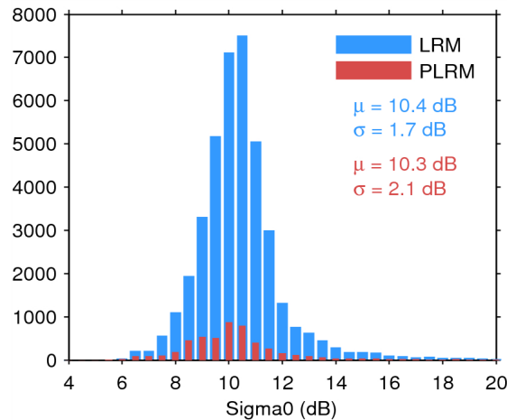
Figure 25. Histogram of flag-valid sigma0 over oceans and lakes for LRM (blue) and PLRM (red) for 12/01/2015. The mean ( \mu ) and standard deviation ( \sigma ) are also shown. Note that values outside [4 20] dB are excluded from the histogram for the sake of readability but not from the computation of \mu and \sigma .
