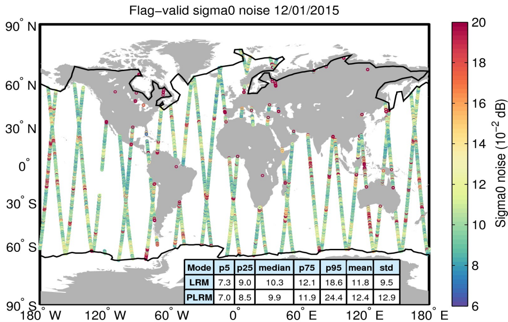
Figure 26. Geographical distribution of flag-valid 20-Hz sigma0 measurement noise over oceans and lakes for 12/01/2015. The statistical values shown in the table refer to the sigma0 noise and are calculated separately for LRM and PLRM regions. Measurements taken over polar polygons have been excluded from the computation of the statistical values. The black lines mark the outer limit of the Arctic and Antarctic polar polygons.
