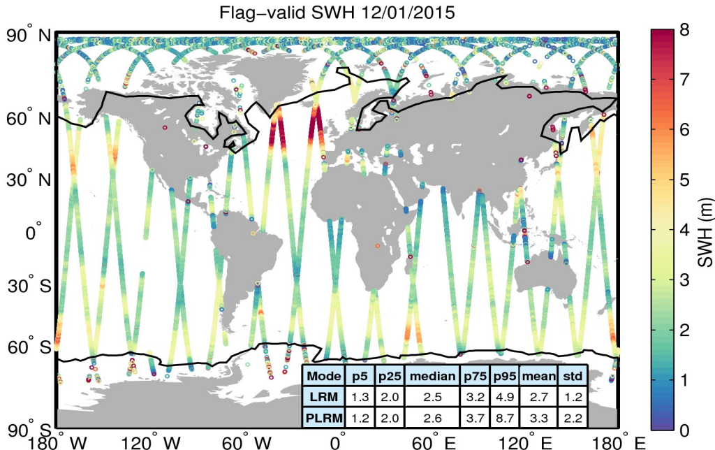
Figure 15. Geographical distribution of flag-valid SWH data over oceans and lakes for 12/01/2015. The statistical values shown in the table refer to the SWH in m and are calculated separately for LRM and PLRM regions. Measurements taken over polar polygons have been excluded from the computation of the statistical values. The black lines mark the outer limit of the Arctic and Antarctic polar polygons.
