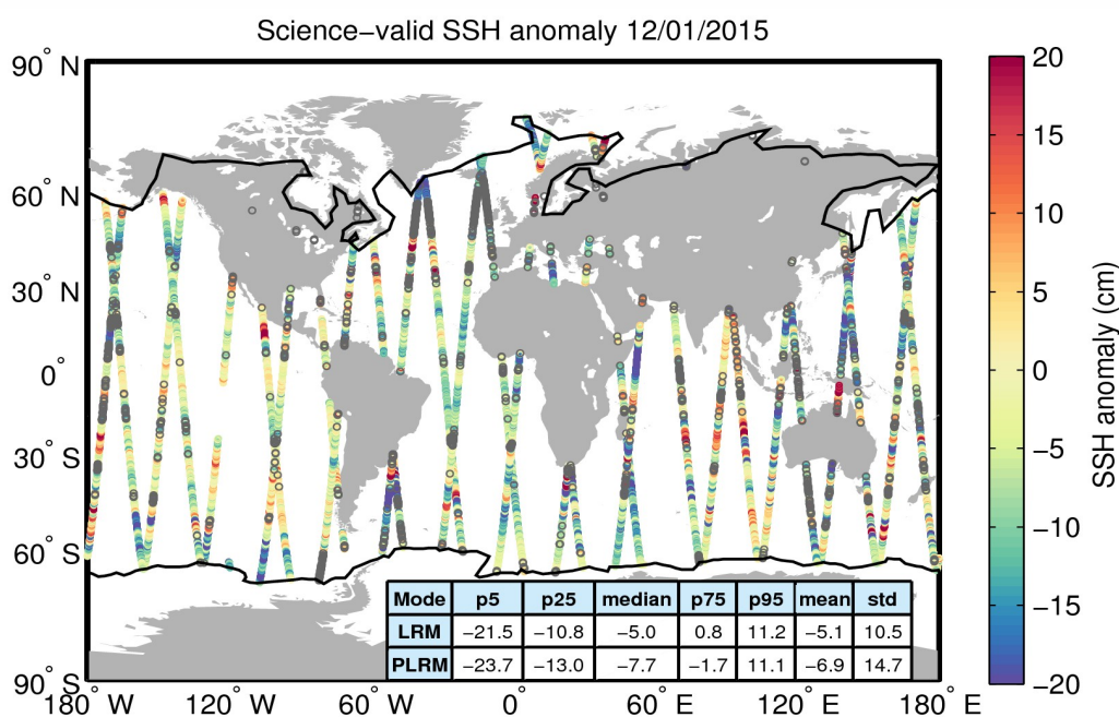
Figure 10. Geographical distribution of science-valid SSH anomaly data over oceans and lakes for 12/01/2015. The statistical values shown in the table refer to the SSH anomaly in cm and are calculated separately for LRM and PLRM regions. The black lines mark the outer limit of the Arctic and Antarctic polar polygons. Gray circles denote records that have been rejected based on the editing criteria described in Table 2.
