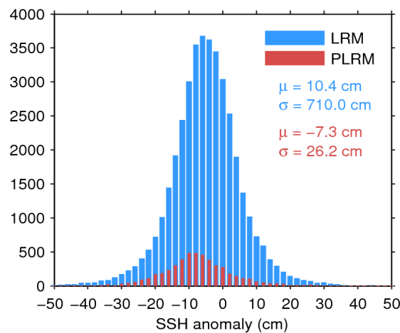
Figure 7. Histogram of flag-valid SSH anomaly over oceans and lakes for LRM (blue) and PLRM (red) for 12/01/2015. The mean ( \mu ) and standard deviation ( \sigma ) are also shown. Note that values outside [-50\ 50] cm are excluded from the histogram for the sake of readability but not from the computation of \mu and \sigma .
