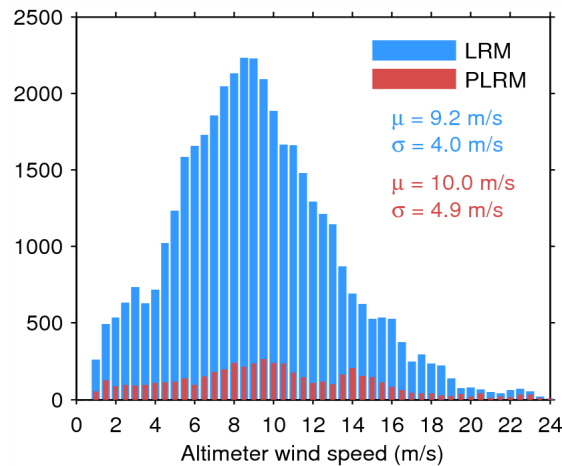
Figure 33. Histogram of flag-valid wind over oceans and lakes for LRM (blue) and PLRM (red) for 12/01/2015. The mean ( \mu ) and standard deviation ( \sigma ) are also shown. Note that values larger than 24 m/s are excluded from the histogram for the sake of readability but not from the computation of \mu and \sigma .
