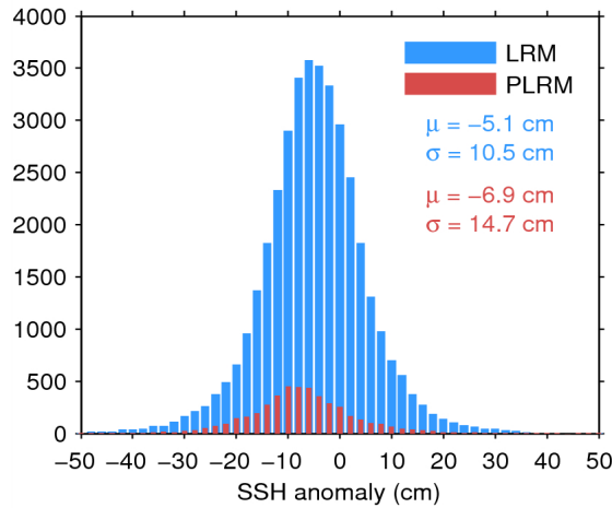
Figure 11. Histogram of science-valid SSH anomaly over oceans and lakes for LRM (blue) and PLRM (red) for 12/01/2015. The mean ( \mu ) and standard deviation ( \sigma ) are also shown. Note that values outside [-50\ 50] cm are excluded from the histogram for the sake of readability but not from the computation of \mu and \sigma .
