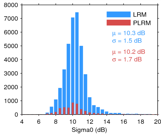
Figure 28. Histogram of science-valid sigma0 over oceans and lakes for LRM (blue) and PLRM (red) for 12/01/2015. The mean ( \mu ) and standard deviation ( \sigma ) are also shown. Note that values outside [4 20] dB are excluded from the histogram for the sake of readability but not from the computation of \mu and \sigma .
