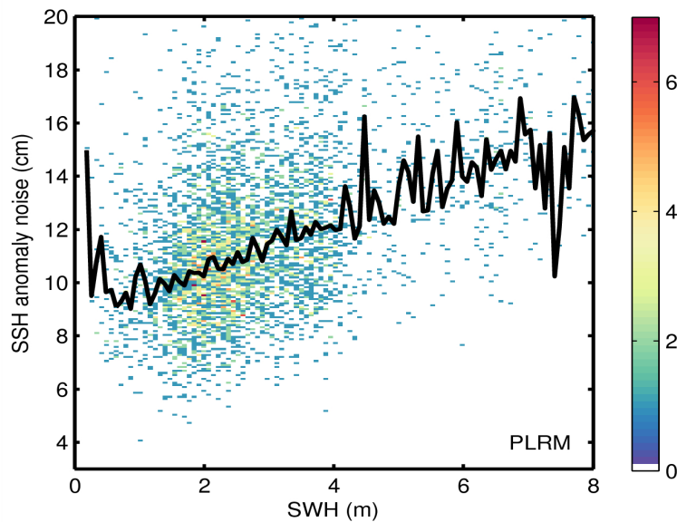
Figure 9. 2D histogram showing flag-valid SSH anomaly noise as a function of SWH for LRM (top) and PLRM (bottom) for 12/01/2015. The black line denotes the median SSH anomaly as a function of SWH.
