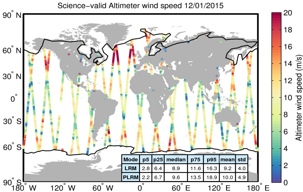
Figure 34. Geographical distribution of science-valid wind data over oceans and lakes for 12/01/2015. The statistical values shown in the table refer to the wind in m/s and are calculated separately for LRM and PLRM regions. The black lines mark the outer limit of the Arctic and Antarctic polar polygons. Gray circles denote records that have been rejected based on the editing criteria described in Table 5.
