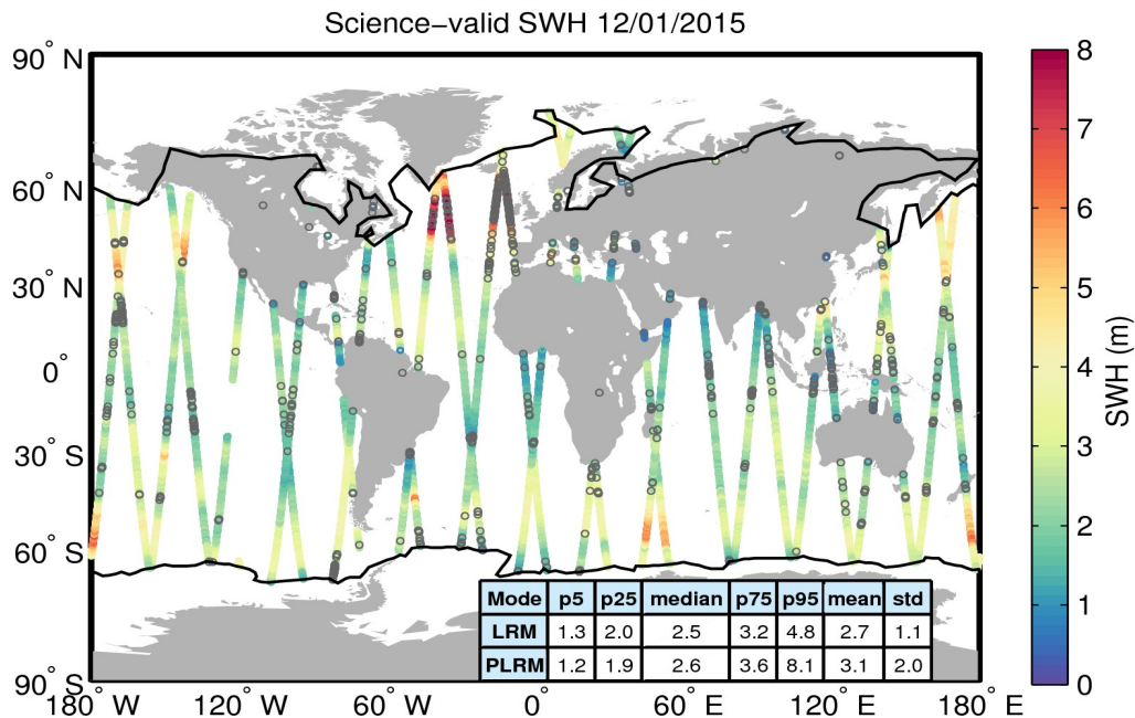
Figure 19. Geographical distribution of science-valid SWH data over oceans and lakes for 12/01/2015. The statistical values shown in the table refer to the SWH in m and are calculated separately for LRM and PLRM regions. The black lines mark the outer limit of the Arctic and Antarctic polar polygons. Gray circles denote records that have been rejected based on the editing criteria described in Table 3.
