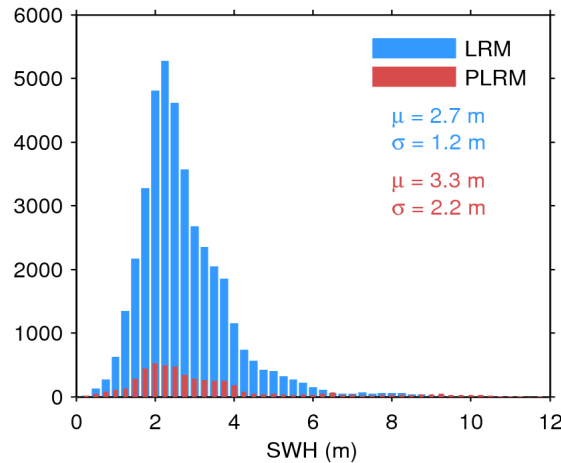
Figure 17. Histogram of flag-valid SWH over oceans and lakes for LRM (blue) and PLRM (red) for 12/01/2015. The mean ( \mu ) and standard deviation ( \sigma ) are also shown. Note that values larger than 12 m are excluded from the histogram for the sake of readability but not from the computation of \mu and \sigma .
