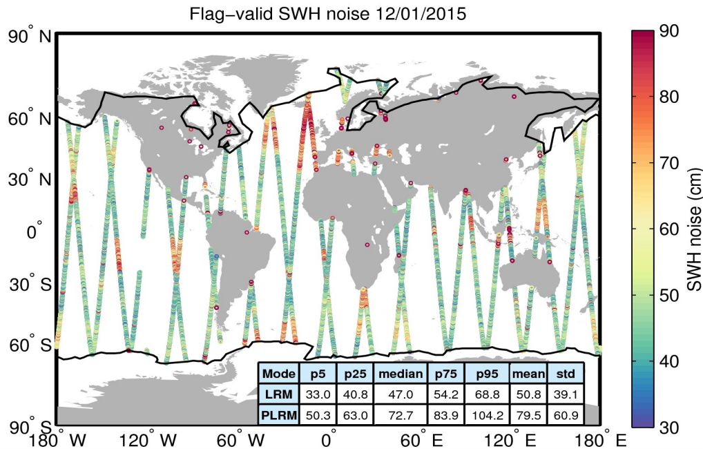
Figure 18. Geographical distribution of flag-valid 20-Hz SWH measurement noise over oceans and lakes for 12/01/2015. The statistical values shown in the table refer to the SWH noise and are calculated separately for LRM and PLRM regions. Measurements taken over polar polygons have been excluded from the computation of the statistical values. The black lines mark the outer limit of the Arctic and Antarctic polar polygons.
