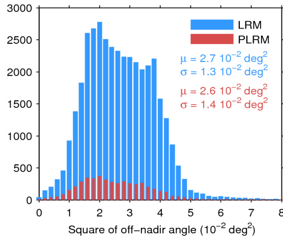
Figure 39. Histogram of flag-valid mispointing over oceans and lakes for LRM (blue) and PLRM (red) for 12/01/2015. Only positive values have been considered. The mean ( \mu ) and standard deviation ( \sigma ) are also shown. Note that values larger than 8 \cdot 10^{-2} \text{ deg}^2 are excluded from the histogram for the sake of readability but not from the computation of \mu and \sigma .
