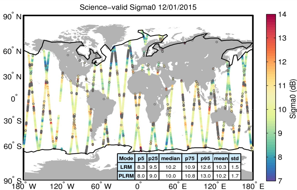
Figure 27. Geographical distribution of science-valid sigma0 data over oceans and lakes for 12/01/2015. The statistical values shown in the table refer to the sigma0 in dB and are calculated separately for LRM and PLRM regions. The black lines mark the outer limit of the Arctic and Antarctic polar polygons. Gray circles denote records that have been rejected based on the editing criteria described in Table 4.
