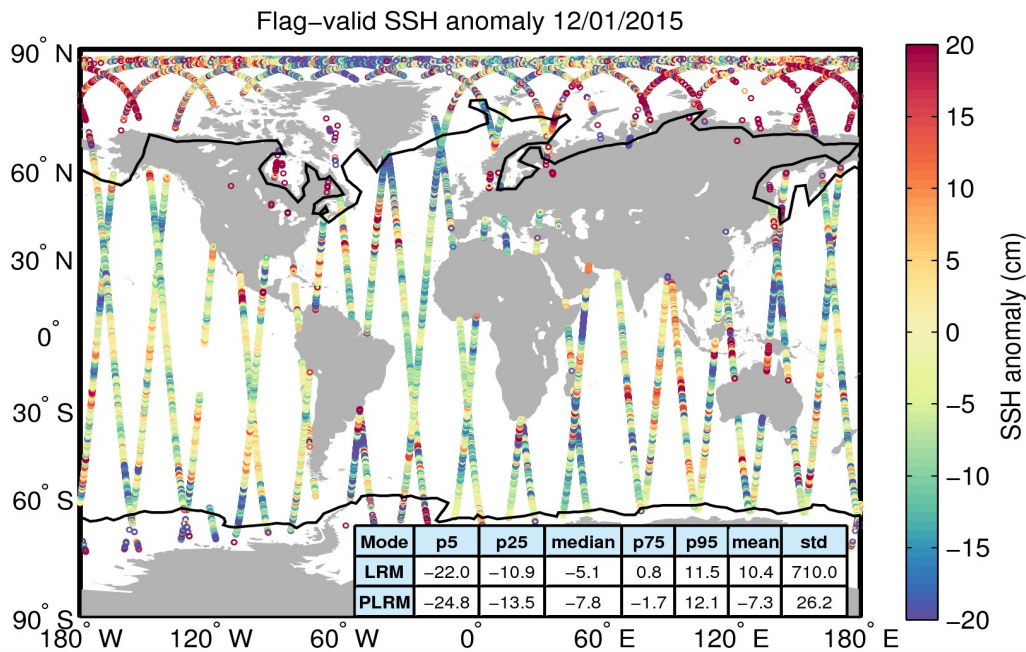
Figure 5. Geographical distribution of flag-valid 1-Hz SSH anomaly data over oceans and lakes for 12/01/2015. The statistical values shown in the table refer to the SSH anomaly in cm and are calculated separately for LRM and PLRM regions. Measurements taken over polar polygons have been excluded from the computation of the statistical values. The black lines mark the outer limit of the Arctic and Antarctic polar polygons.
