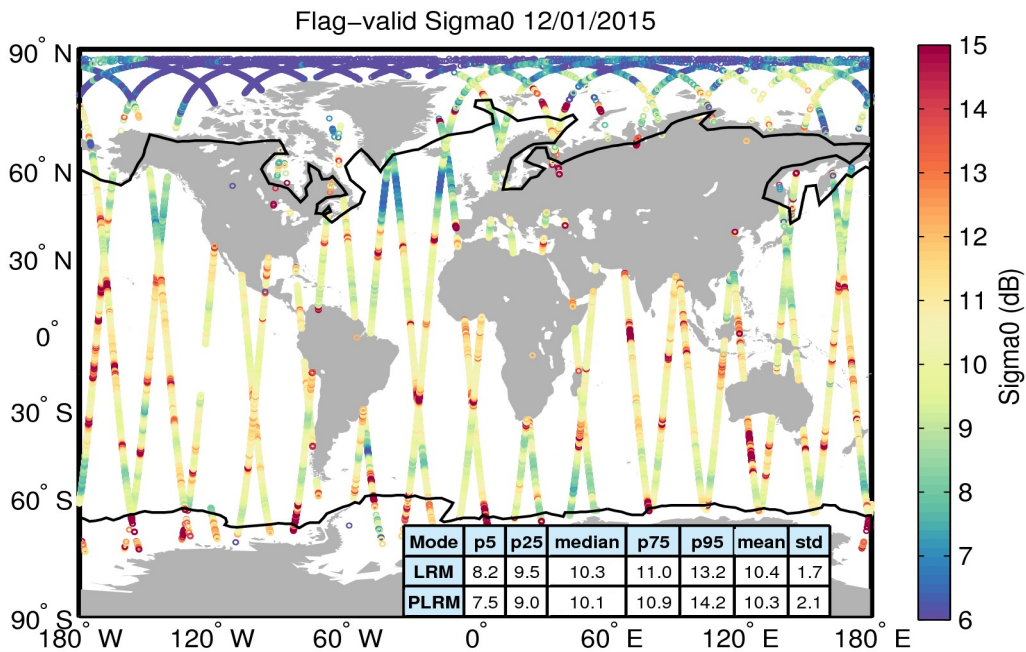
Figure 23. Geographical distribution of flag-valid sigma0 data over oceans and lakes for 12/01/2015. The statistical values shown in the table refer to the sigma0 in dB and are calculated separately for LRM and PLRM regions. Measurements taken over polar polygons have been excluded from the computation of the statistical values. The black lines mark the outer limit of the Arctic and Antarctic polar polygons.
