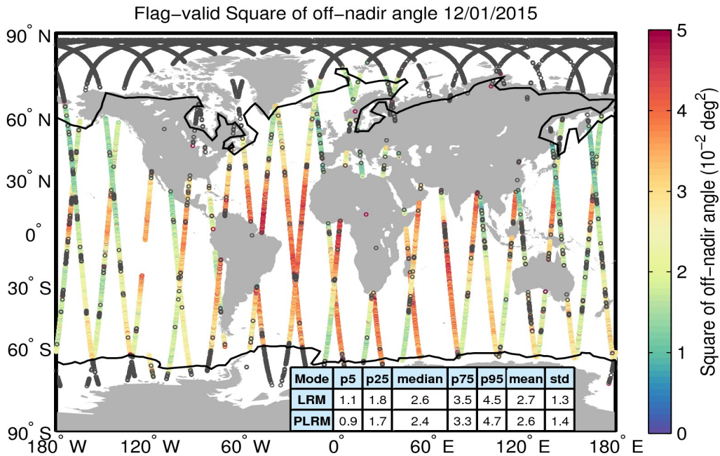
Figure 37. Geographical distribution of flag-valid mispointing data over oceans and lakes for 12/01/2015. The statistical values shown in the table refer to the mispointing in 10^{-2} \text{ deg}^2 and are calculated separately for LRM and PLRM regions. Measurements taken over polar polygons have been excluded from the computation of the statistical values. The black lines mark the outer limit of the Arctic and Antarctic polar polygons. Gray circles denote negative values.
