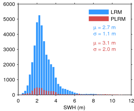
Figure 20. Histogram of science-valid SWH over oceans and lakes for LRM (blue) and PLRM (red) for 12/01/2015. The mean ( \mu ) and standard deviation ( \sigma ) are also shown. Note that values larger than 12 m are excluded from the histogram for the sake of readability but not from the computation of \mu and \sigma .
