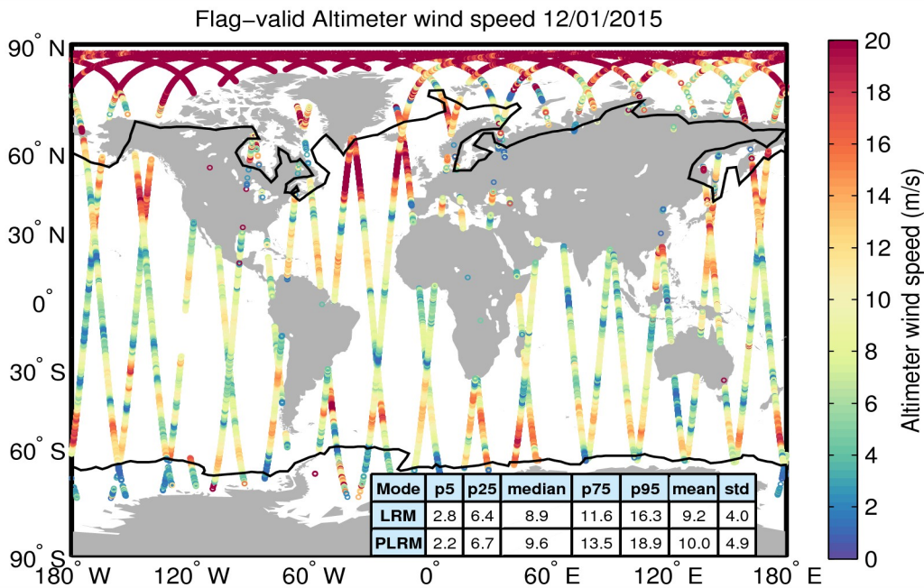
Figure 31. Geographical distribution of flag-valid wind data over oceans and lakes for 12/01/2015. The statistical values shown in the table refer to the wind in m/s and are calculated separately for LRM and PLRM regions. Measurements taken over polar polygons have been excluded from the computation of the statistical values. The black lines mark the outer limit of the Arctic and Antarctic polar polygons.
