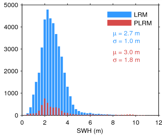
Figure 20. Histogram of science-valid SWH over oceans and lakes for LRM (blue) and PLRM (red) for 10/01/2015. The mean ( \mu ) and standard deviation ( \sigma ) are also shown. Note that values larger than 12 m are excluded from the histogram for the sake of readability but not from the computation of \mu and \sigma .
