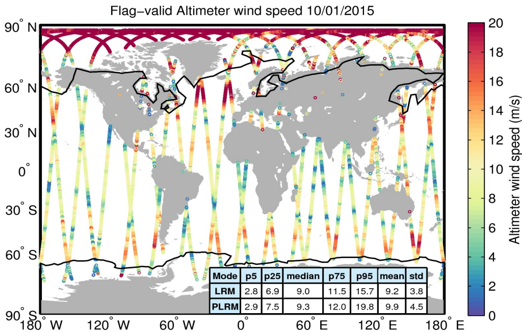
Figure 31. Geographical distribution of flag-valid wind data over oceans and lakes for 10/01/2015. The statistical values shown in the table refer to the wind in m/s and are calculated separately for LRM and PLRM regions. Measurements taken over polar polygons have been excluded from the computation of the statistical values. The black lines mark the outer limit of the Arctic and Antarctic polar polygons.
