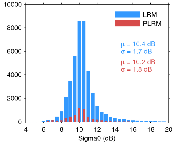
Figure 25. Histogram of flag-valid sigma0 over oceans and lakes for LRM (blue) and PLRM (red) for 10/01/2015. The mean ( \mu ) and standard deviation ( \sigma ) are also shown. Note that values outside [4 20] dB are excluded from the histogram for the sake of readability but not from the computation of \mu and \sigma .
