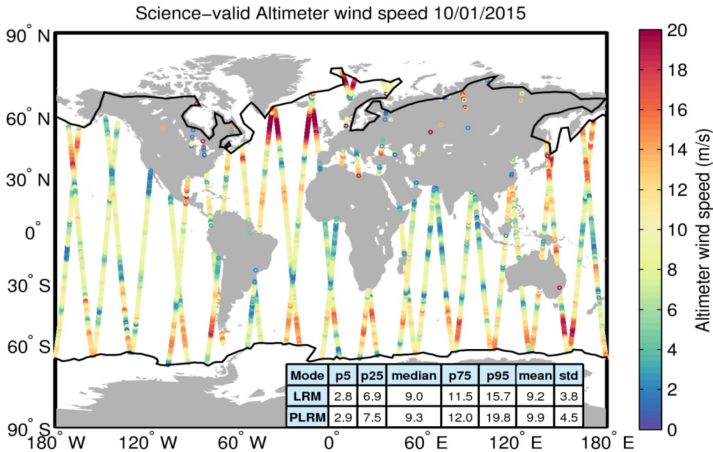
Figure 34. Geographical distribution of science-valid wind data over oceans and lakes for 10/01/2015. The statistical values shown in the table refer to the wind in m/s and are calculated separately for LRM and PLRM regions. The black lines mark the outer limit of the Arctic and Antarctic polar polygons. Gray circles denote records that have been rejected based on the editing criteria described in Table 5.
