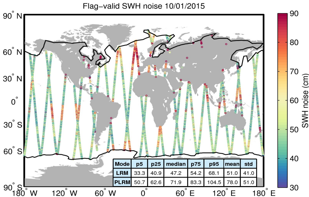
Figure 18. Geographical distribution of flag-valid 20-Hz SWH measurement noise over oceans and lakes for 10/01/2015. The statistical values shown in the table refer to the SWH noise and are calculated separately for LRM and PLRM regions. Measurements taken over polar polygons have been excluded from the computation of the statistical values. The black lines mark the outer limit of the Arctic and Antarctic polar polygons.
