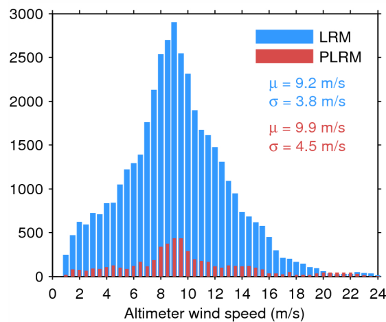
Figure 33. Histogram of flag-valid wind over oceans and lakes for LRM (blue) and PLRM (red) for 10/01/2015. The mean ( \mu ) and standard deviation ( \sigma ) are also shown. Note that values larger than 24 m/s are excluded from the histogram for the sake of readability but not from the computation of \mu and \sigma .
