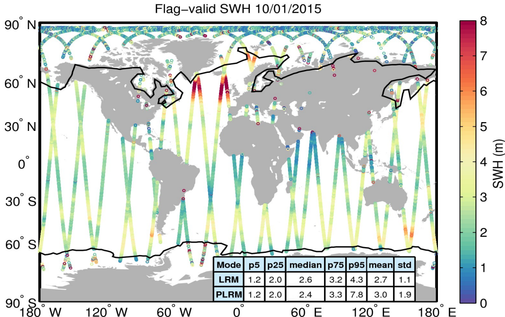
Figure 15. Geographical distribution of flag-valid SWH data over oceans and lakes for 10/01/2015. The statistical values shown in the table refer to the SWH in m and are calculated separately for LRM and PLRM regions. Measurements taken over polar polygons have been excluded from the computation of the statistical values. The black lines mark the outer limit of the Arctic and Antarctic polar polygons.
