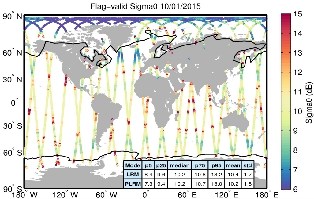
Figure 23. Geographical distribution of flag-valid sigma0 data over oceans and lakes for 10/01/2015. The statistical values shown in the table refer to the sigma0 in dB and are calculated separately for LRM and PLRM regions. Measurements taken over polar polygons have been excluded from the computation of the statistical values. The black lines mark the outer limit of the Arctic and Antarctic polar polygons.
