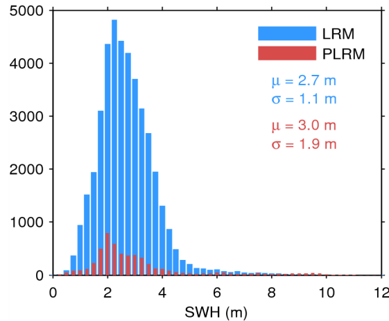
Figure 17. Histogram of flag-valid SWH over oceans and lakes for LRM (blue) and PLRM (red) for 10/01/2015. The mean ( \mu ) and standard deviation ( \sigma ) are also shown. Note that values larger than 12 m are excluded from the histogram for the sake of readability but not from the computation of \mu and \sigma .
