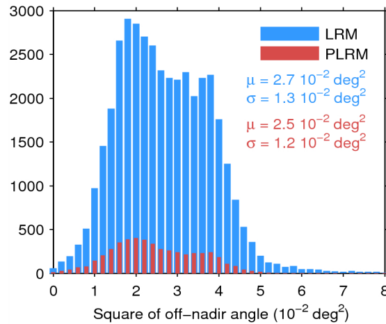
Figure 39. Histogram of flag-valid mispointing over oceans and lakes for LRM (blue) and PLRM (red) for 10/01/2015. Only positive values have been considered. The mean ( \mu ) and standard deviation ( \sigma ) are also shown. Note that values larger than 8 \cdot 10^{-2} \text{ deg}^2 are excluded from the histogram for the sake of readability but not from the computation of \mu and \sigma .
