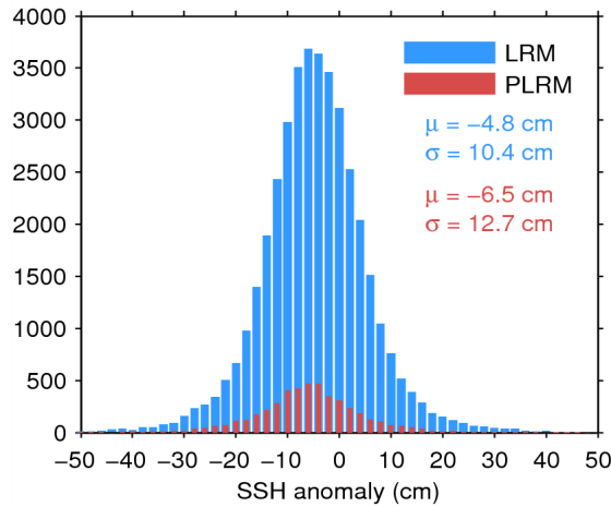
Figure 11. Histogram of science-valid SSH anomaly over oceans and lakes for LRM (blue) and PLRM (red) for 10/01/2015. The mean ( \mu ) and standard deviation ( \sigma ) are also shown. Note that values outside [-50\ 50] cm are excluded from the histogram for the sake of readability but not from the computation of \mu and \sigma .
