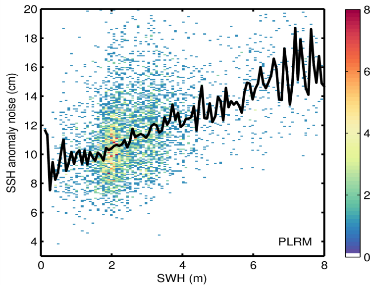
Figure 9. 2D histogram showing flag-valid SSH anomaly noise as a function of SWH for LRM (top) and PLRM (bottom) for 10/01/2015. The black line denotes the median SSH anomaly as a function of SWH.
