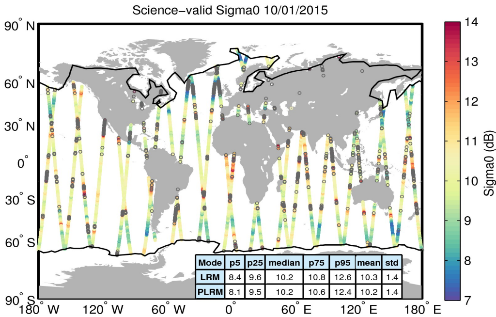
Figure 27. Geographical distribution of science-valid sigma0 data over oceans and lakes for 10/01/2015. The statistical values shown in the table refer to the sigma0 in dB and are calculated separately for LRM and PLRM regions. The black lines mark the outer limit of the Arctic and Antarctic polar polygons. Gray circles denote records that have been rejected based on the editing criteria described in Table 4.
