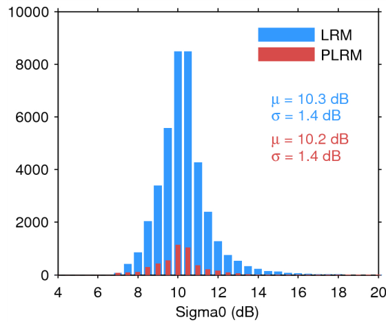
Figure 28. Histogram of science-valid sigma0 over oceans and lakes for LRM (blue) and PLRM (red) for 10/01/2015. The mean ( \mu ) and standard deviation ( \sigma ) are also shown. Note that values outside [4 20] dB are excluded from the histogram for the sake of readability but not from the computation of \mu and \sigma .
