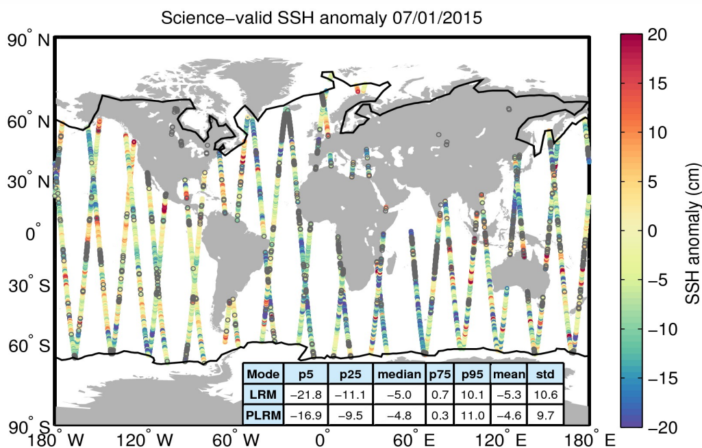
Figure 10. Geographical distribution of science-valid SSH anomaly data over oceans and lakes for 07/01/2015. The statistical values shown in the table refer to the SSH anomaly in cm and are calculated separately for LRM and PLRM regions. The black lines mark the outer limit of the Arctic and Antarctic polar polygons. Gray circles denote records that have been rejected based on the editing criteria described in Table 2.
