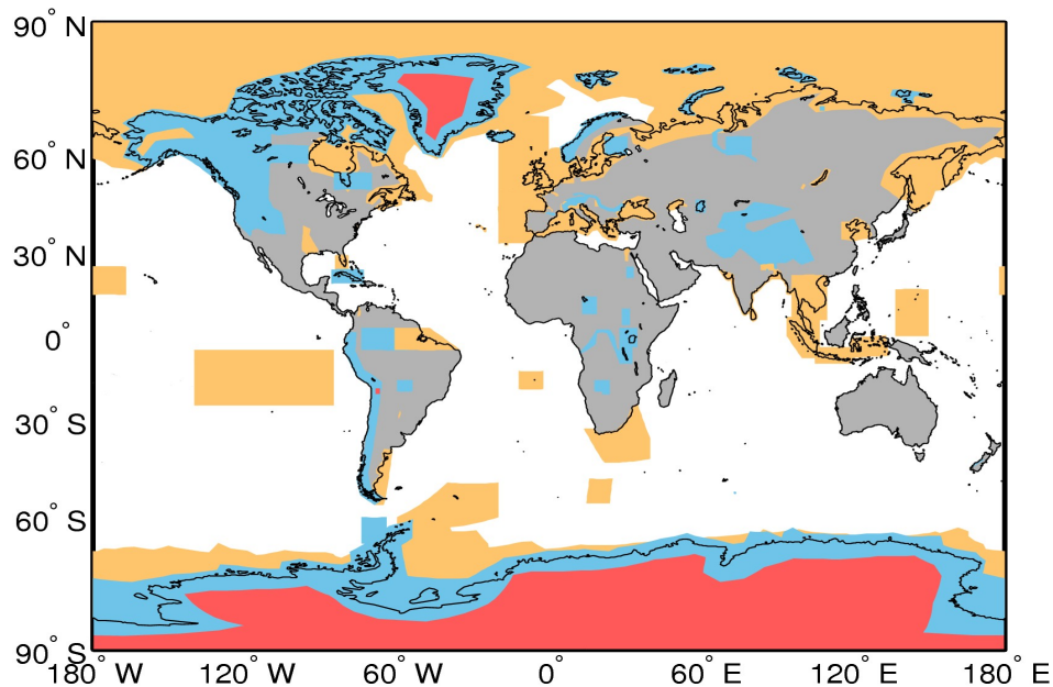
Figure A1. Extent of the regions defining the geographical mode mask for 07/01/2015. The regions where SAR, and SARIn are operated are denoted by the orange and blue polygons, respectively. LRM is operated over areas of the continental ice sheets (red polygons) and over oceans and land not covered by other modes.
