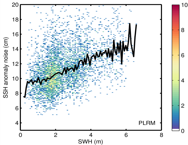
Figure 9. 2D histogram showing flag-valid SSH anomaly noise as a function of SWH for LRM (top) and PLRM (bottom) for 07/01/2015. The black line denotes the median SSH anomaly as a function of SWH.
