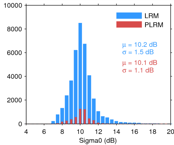
Figure 28. Histogram of science-valid sigma0 over oceans and lakes for LRM (blue) and PLRM (red) for 07/01/2015. The mean ( \mu ) and standard deviation ( \sigma ) are also shown. Note that values outside [4 20] dB are excluded from the histogram for the sake of readability but not from the computation of \mu and \sigma .
