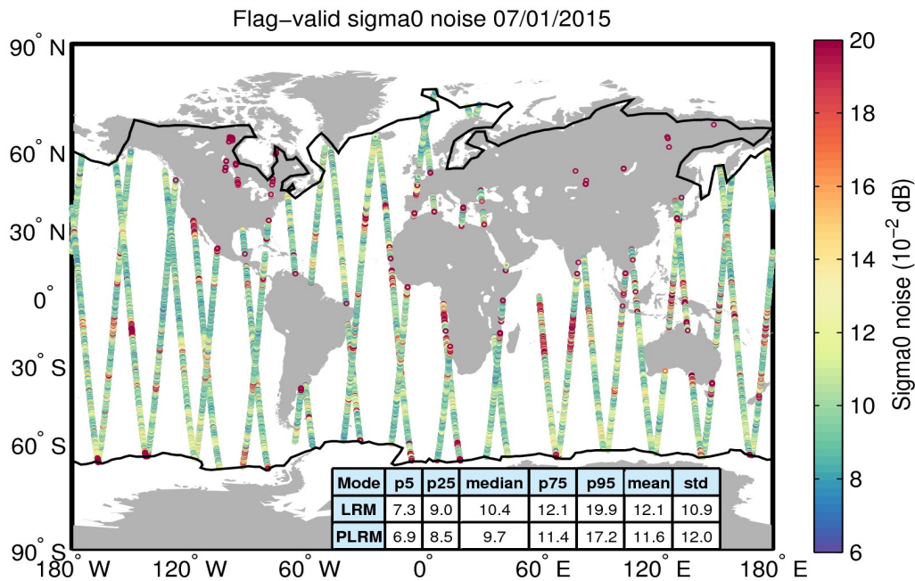
Figure 26. Geographical distribution of flag-valid 20-Hz sigma0 measurement noise over oceans and lakes for 07/01/2015. The statistical values shown in the table refer to the sigma0 noise and are calculated separately for LRM and PLRM regions. Measurements taken over polar polygons have been excluded from the computation of the statistical values. The black lines mark the outer limit of the Arctic and Antarctic polar polygons.
