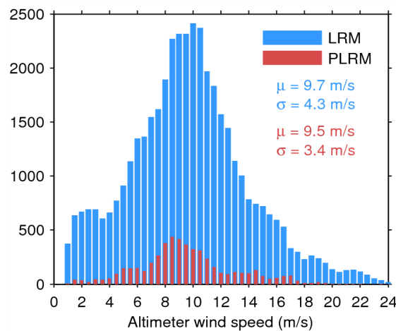
Figure 33. Histogram of flag-valid wind over oceans and lakes for LRM (blue) and PLRM (red) for 07/01/2015. The mean ( \mu ) and standard deviation ( \sigma ) are also shown. Note that values larger than 24 m/s are excluded from the histogram for the sake of readability but not from the computation of \mu and \sigma .
