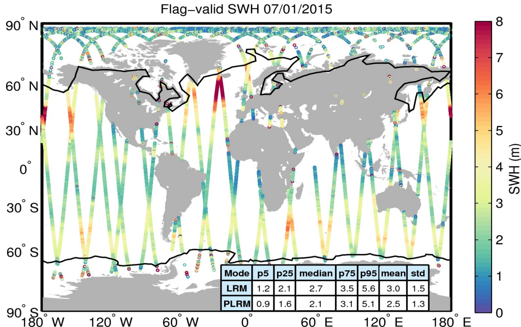
Figure 15. Geographical distribution of flag-valid SWH data over oceans and lakes for 07/01/2015. The statistical values shown in the table refer to the SWH in m and are calculated separately for LRM and PLRM regions. Measurements taken over polar polygons have been excluded from the computation of the statistical values. The black lines mark the outer limit of the Arctic and Antarctic polar polygons.
