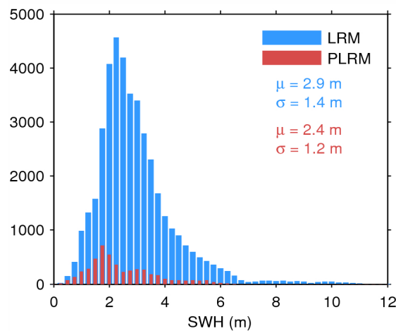
Figure 20. Histogram of science-valid SWH over oceans and lakes for LRM (blue) and PLRM (red) for 07/01/2015. The mean ( \mu ) and standard deviation ( \sigma ) are also shown. Note that values larger than 12 m are excluded from the histogram for the sake of readability but not from the computation of \mu and \sigma .
