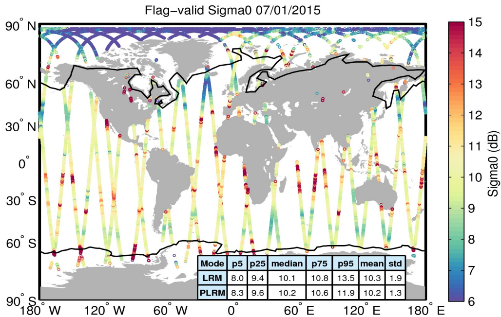
Figure 23. Geographical distribution of flag-valid sigma0 data over oceans and lakes for 07/01/2015. The statistical values shown in the table refer to the sigma0 in dB and are calculated separately for LRM and PLRM regions. Measurements taken over polar polygons have been excluded from the computation of the statistical values. The black lines mark the outer limit of the Arctic and Antarctic polar polygons.
