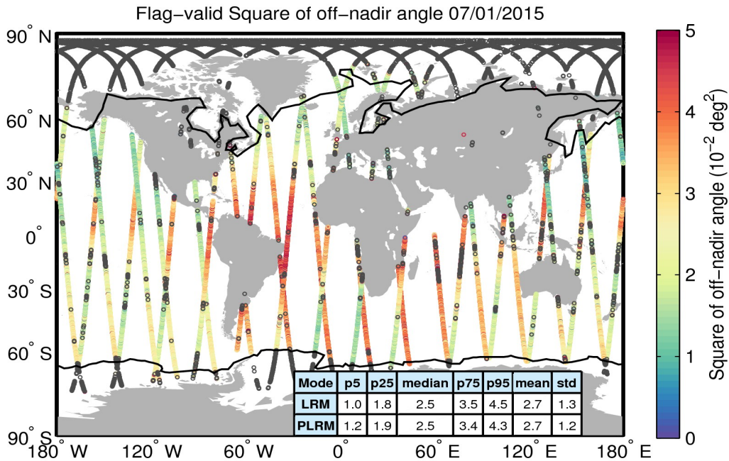
Figure 37. Geographical distribution of flag-valid mispointing data over oceans and lakes for 07/01/2015. The statistical values shown in the table refer to the mispointing in 10^{-2} \text{ deg}^2 and are calculated separately for LRM and PLRM regions. Measurements taken over polar polygons have been excluded from the computation of the statistical values. The black lines mark the outer limit of the Arctic and Antarctic polar polygons. Gray circles denote negative values.
