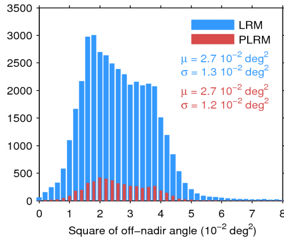
Figure 39. Histogram of flag-valid mispointing over oceans and lakes for LRM (blue) and PLRM (red) for 07/01/2015. Only positive values have been considered. The mean ( \mu ) and standard deviation ( \sigma ) are also shown. Note that values larger than 8 \cdot 10^{-2} \text{ deg}^2 are excluded from the histogram for the sake of readability but not from the computation of \mu and \sigma .
