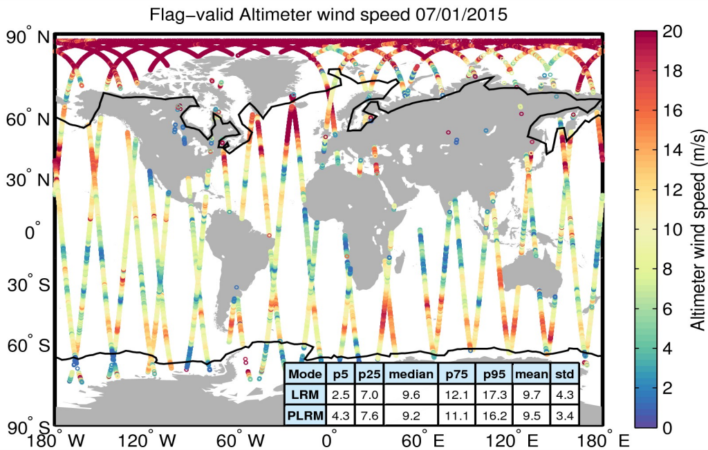
Figure 31. Geographical distribution of flag-valid wind data over oceans and lakes for 07/01/2015. The statistical values shown in the table refer to the wind in m/s and are calculated separately for LRM and PLRM regions. Measurements taken over polar polygons have been excluded from the computation of the statistical values. The black lines mark the outer limit of the Arctic and Antarctic polar polygons.
