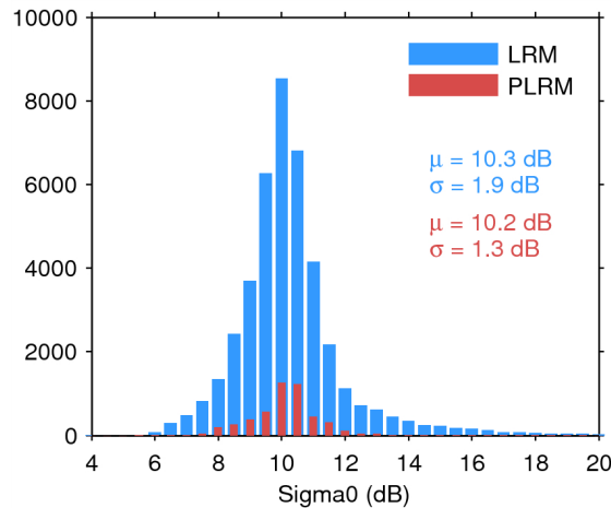
Figure 25. Histogram of flag-valid sigma0 over oceans and lakes for LRM (blue) and PLRM (red) for 07/01/2015. The mean ( \mu ) and standard deviation ( \sigma ) are also shown. Note that values outside [4 20] dB are excluded from the histogram for the sake of readability but not from the computation of \mu and \sigma .
