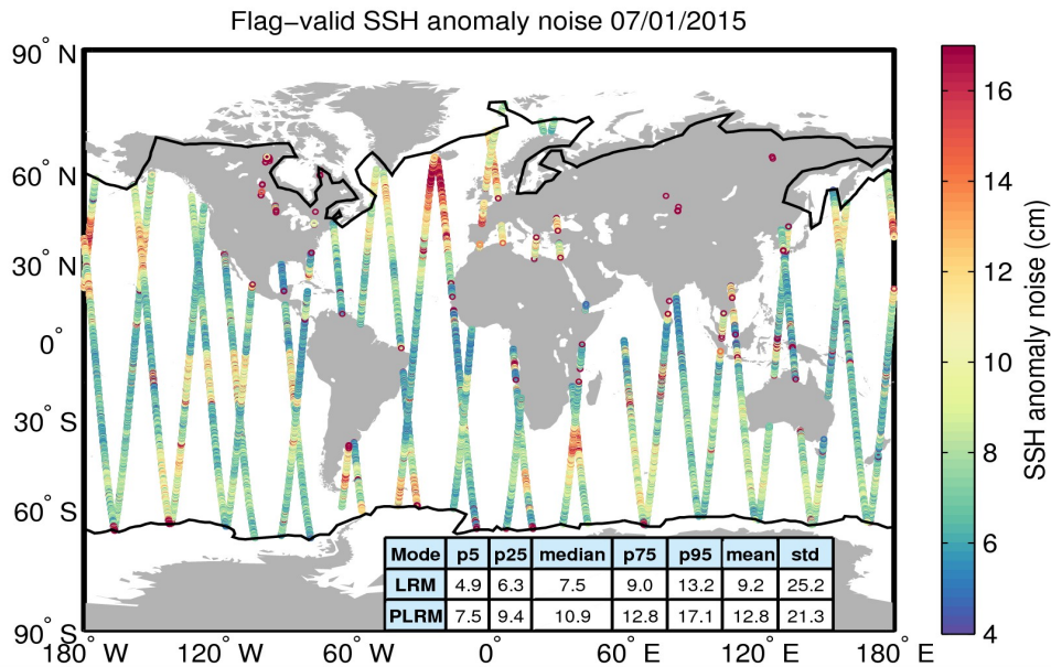
Figure 8. Geographical distribution of flag-valid 20-Hz SSH anomaly measurement noise over oceans and lakes for 07/01/2015. The statistical values shown in the table refer to the SSH anomaly noise and are calculated separately for LRM and PLRM regions. Measurements taken over polar polygons have been excluded from the computation of the statistical values. The black lines mark the outer limit of the Arctic and Antarctic polar polygons.
