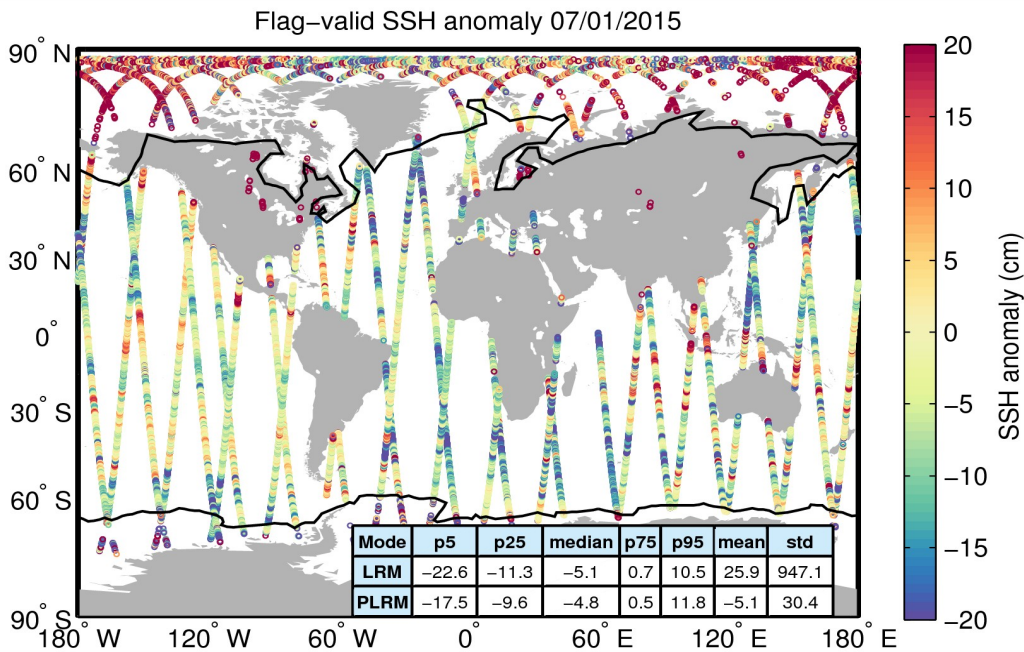
Figure 5. Geographical distribution of flag-valid 1-Hz SSH anomaly data over oceans and lakes for 07/01/2015. The statistical values shown in the table refer to the SSH anomaly in cm and are calculated separately for LRM and PLRM regions. Measurements taken over polar polygons have been excluded from the computation of the statistical values. The black lines mark the outer limit of the Arctic and Antarctic polar polygons.
