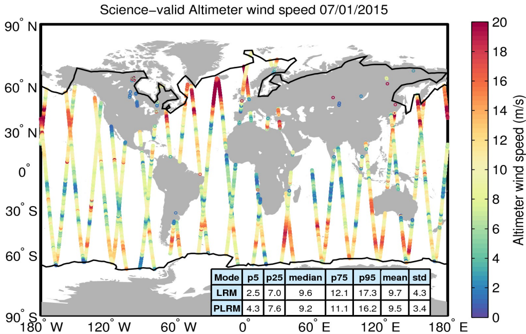
Figure 34. Geographical distribution of science-valid wind data over oceans and lakes for 07/01/2015. The statistical values shown in the table refer to the wind in m/s and are calculated separately for LRM and PLRM regions. The black lines mark the outer limit of the Arctic and Antarctic polar polygons. Gray circles denote records that have been rejected based on the editing criteria described in Table 5.
