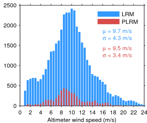
Figure 35. Histogram of science-valid wind over oceans and lakes for LRM (blue) and PLRM (red) for 07/01/2015. The mean ( \mu ) and standard deviation ( \sigma ) are also shown. Note that values larger than 24 m/s are excluded from the histogram for the sake of readability but not from the computation of \mu and \sigma .
