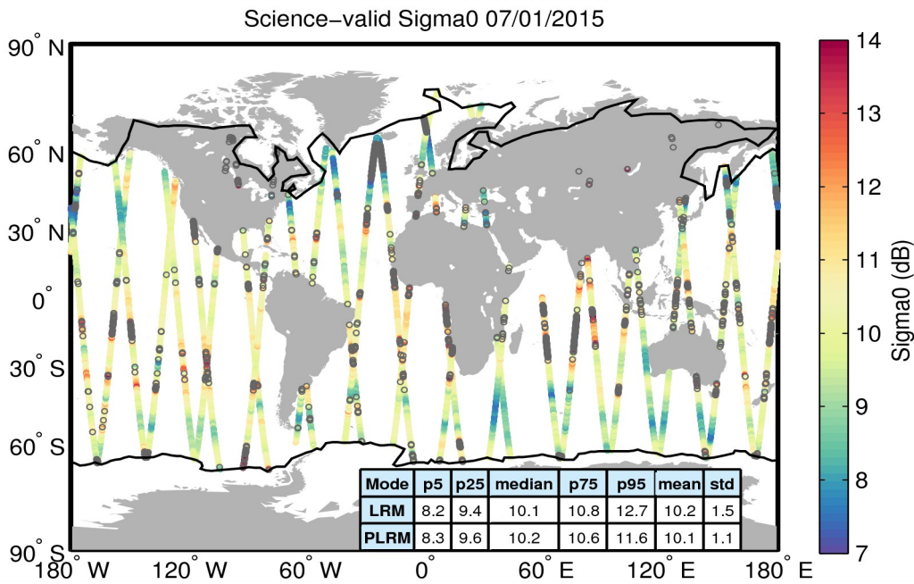
Figure 27. Geographical distribution of science-valid sigma0 data over oceans and lakes for 07/01/2015. The statistical values shown in the table refer to the sigma0 in dB and are calculated separately for LRM and PLRM regions. The black lines mark the outer limit of the Arctic and Antarctic polar polygons. Gray circles denote records that have been rejected based on the editing criteria described in Table 4.
