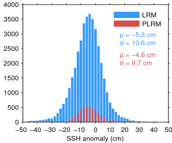
Figure 11. Histogram of science-valid SSH anomaly over oceans and lakes for LRM (blue) and PLRM (red) for 07/01/2015. The mean ( \mu ) and standard deviation ( \sigma ) are also shown. Note that values outside [-50 50] cm are excluded from the histogram for the sake of readability but not from the computation of \mu and \sigma .
