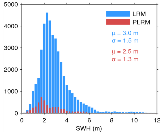
Figure 17. Histogram of flag-valid SWH over oceans and lakes for LRM (blue) and PLRM (red) for 07/01/2015. The mean ( \mu ) and standard deviation ( \sigma ) are also shown. Note that values larger than 12 m are excluded from the histogram for the sake of readability but not from the computation of \mu and \sigma .
