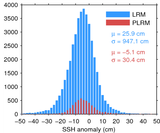
Figure 7. Histogram of flag-valid SSH anomaly over oceans and lakes for LRM (blue) and PLRM (red) for 07/01/2015. The mean ( \mu ) and standard deviation ( \sigma ) are also shown. Note that values outside [-50\ 50] cm are excluded from the histogram for the sake of readability but not from the computation of \mu and \sigma .
