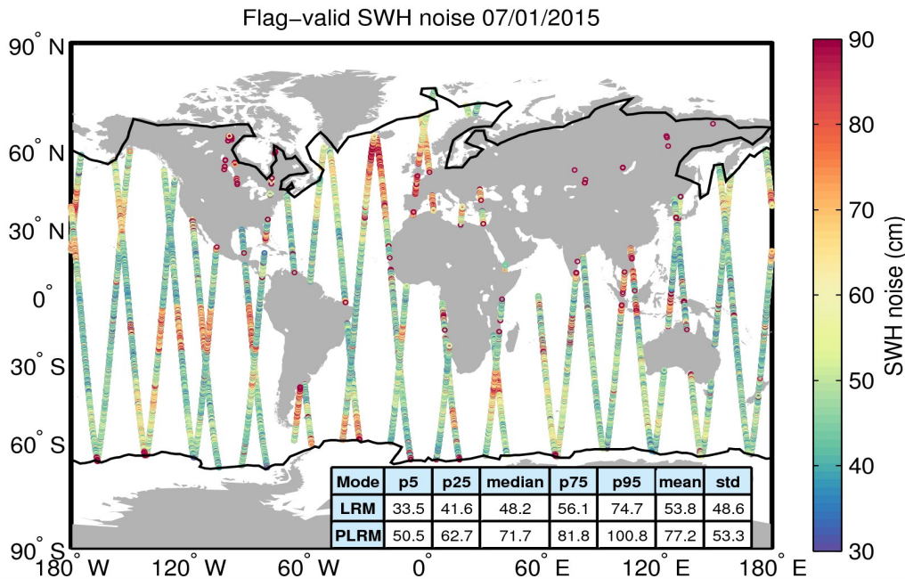
Figure 18. Geographical distribution of flag-valid 20-Hz SWH measurement noise over oceans and lakes for 07/01/2015. The statistical values shown in the table refer to the SWH noise and are calculated separately for LRM and PLRM regions. Measurements taken over polar polygons have been excluded from the computation of the statistical values. The black lines mark the outer limit of the Arctic and Antarctic polar polygons.
