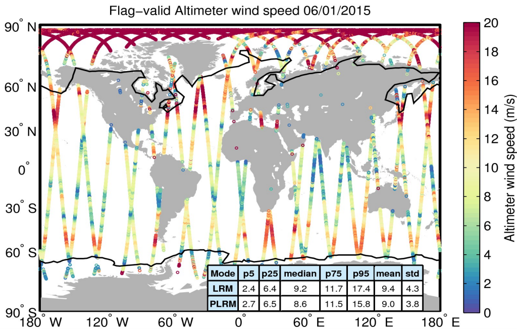
Figure 31. Geographical distribution of flag-valid wind data over oceans and lakes for 06/01/2015. The statistical values shown in the table refer to the wind in m/s and are calculated separately for LRM and PLRM regions. Measurements taken over polar polygons have been excluded from the computation of the statistical values. The black lines mark the outer limit of the Arctic and Antarctic polar polygons.
