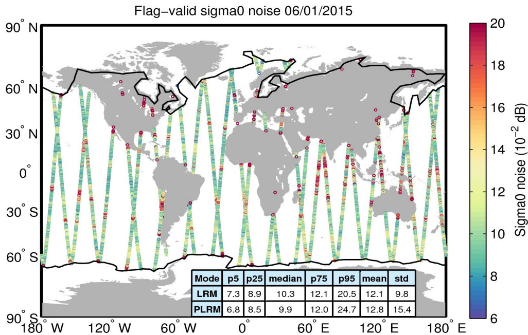
Figure 26. Geographical distribution of flag-valid 20-Hz sigma0 measurement noise over oceans and lakes for 06/01/2015. The statistical values shown in the table refer to the sigma0 noise and are calculated separately for LRM and PLRM regions. Measurements taken over polar polygons have been excluded from the computation of the statistical values. The black lines mark the outer limit of the Arctic and Antarctic polar polygons.
