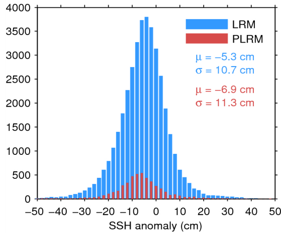
Figure 11. Histogram of science-valid SSH anomaly over oceans and lakes for LRM (blue) and PLRM (red) for 06/01/2015. The mean ( \mu ) and standard deviation ( \sigma ) are also shown. Note that values outside [-50\ 50] cm are excluded from the histogram for the sake of readability but not from the computation of \mu and \sigma .
