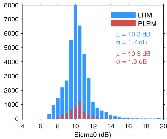
Figure 28. Histogram of science-valid sigma0 over oceans and lakes for LRM (blue) and PLRM (red) for 06/01/2015. The mean ( \mu ) and standard deviation ( \sigma ) are also shown. Note that values outside [4 20] dB are excluded from the histogram for the sake of readability but not from the computation of \mu and \sigma .
