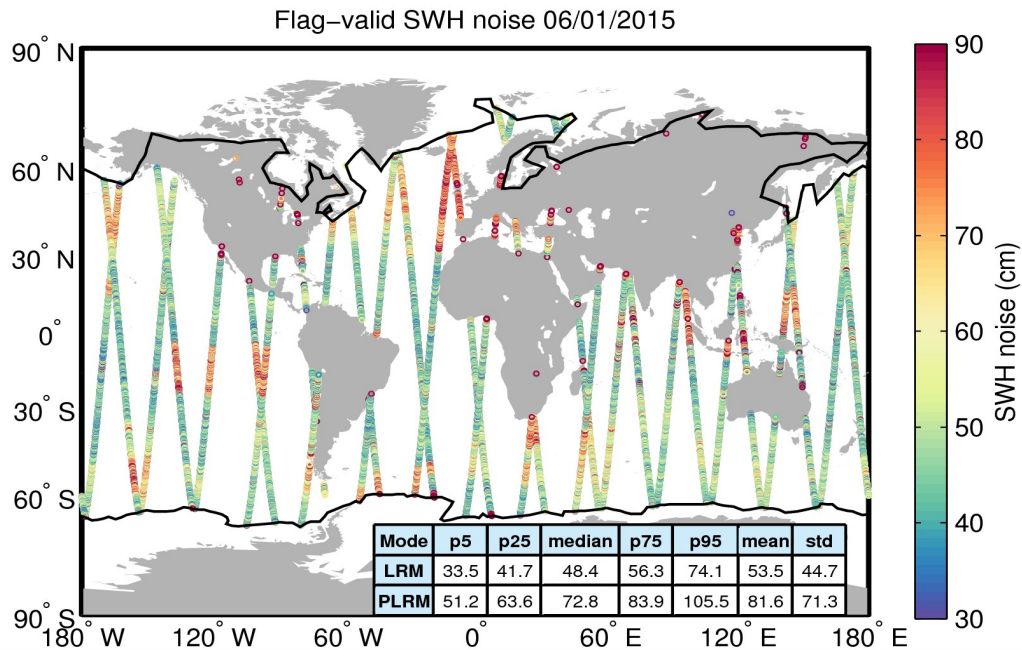
Figure 18. Geographical distribution of flag-valid 20-Hz SWH measurement noise over oceans and lakes for 06/01/2015. The statistical values shown in the table refer to the SWH noise and are calculated separately for LRM and PLRM regions. Measurements taken over polar polygons have been excluded from the computation of the statistical values. The black lines mark the outer limit of the Arctic and Antarctic polar polygons.
