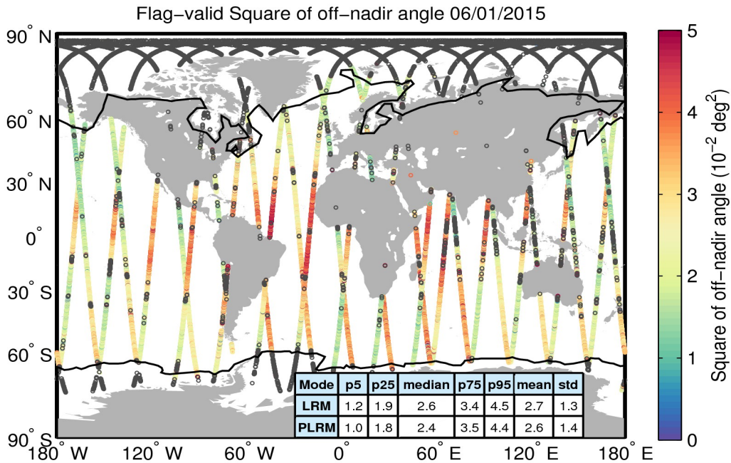
Figure 37. Geographical distribution of flag-valid mispointing data over oceans and lakes for 06/01/2015. The statistical values shown in the table refer to the mispointing in 10^{-2} \text{ deg}^2 and are calculated separately for LRM and PLRM regions. Measurements taken over polar polygons have been excluded from the computation of the statistical values. The black lines mark the outer limit of the Arctic and Antarctic polar polygons. Gray circles denote negative values.
