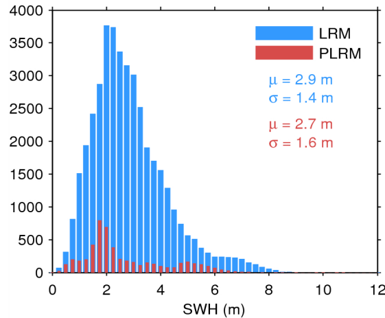
Figure 17. Histogram of flag-valid SWH over oceans and lakes for LRM (blue) and PLRM (red) for 06/01/2015. The mean ( \mu ) and standard deviation ( \sigma ) are also shown. Note that values larger than 12 m are excluded from the histogram for the sake of readability but not from the computation of \mu and \sigma .
