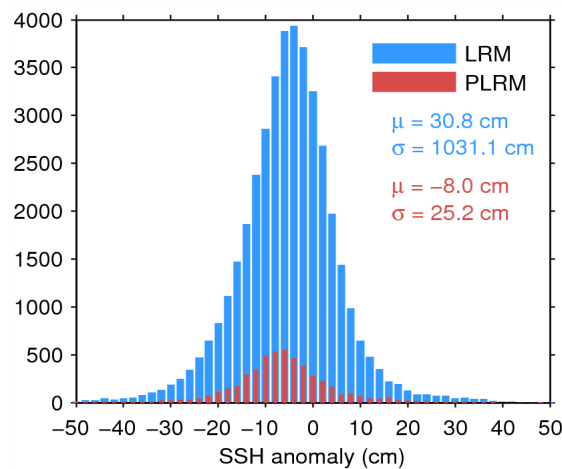
Figure 7. Histogram of flag-valid SSH anomaly over oceans and lakes for LRM (blue) and PLRM (red) for 06/01/2015. The mean ( \mu ) and standard deviation ( \sigma ) are also shown. Note that values outside [-50 \ 50] cm are excluded from the histogram for the sake of readability but not from the computation of \mu and \sigma .
