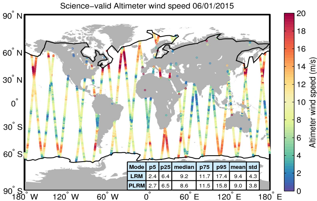
Figure 34. Geographical distribution of science-valid wind data over oceans and lakes for 06/01/2015. The statistical values shown in the table refer to the wind in m/s and are calculated separately for LRM and PLRM regions. The black lines mark the outer limit of the Arctic and Antarctic polar polygons. Gray circles denote records that have been rejected based on the editing criteria described in Table 5.
