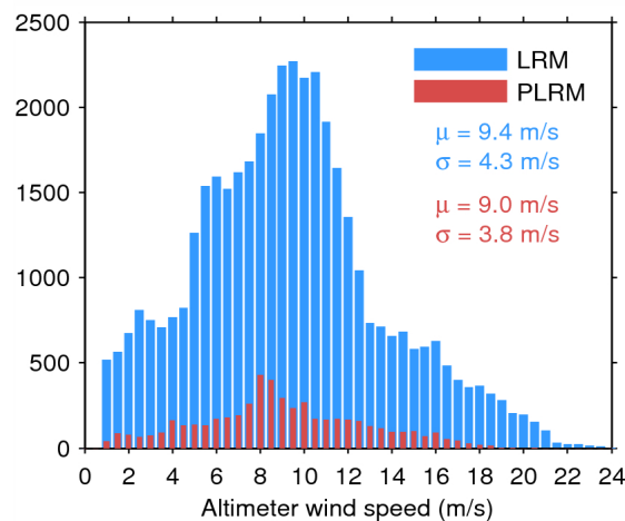
Figure 35. Histogram of science-valid wind over oceans and lakes for LRM (blue) and PLRM (red) for 06/01/2015. The mean ( \mu ) and standard deviation ( \sigma ) are also shown. Note that values larger than 24 m/s are excluded from the histogram for the sake of readability but not from the computation of \mu and \sigma .
