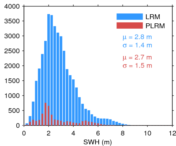
Figure 20. Histogram of science-valid SWH over oceans and lakes for LRM (blue) and PLRM (red) for 06/01/2015. The mean ( \mu ) and standard deviation ( \sigma ) are also shown. Note that values larger than 12 m are excluded from the histogram for the sake of readability but not from the computation of \mu and \sigma .
