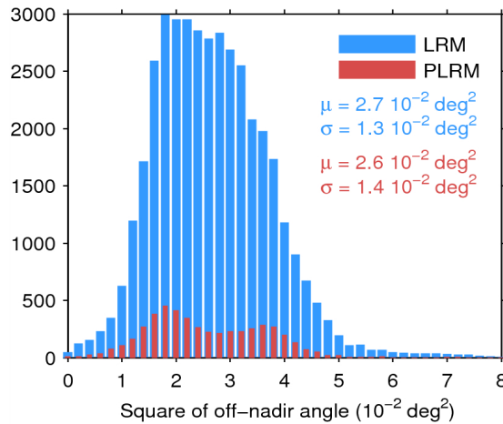
Figure 39. Histogram of flag-valid mispointing over oceans and lakes for LRM (blue) and PLRM (red) for 06/01/2015. Only positive values have been considered. The mean ( \mu ) and standard deviation ( \sigma ) are also shown. Note that values larger than 8 \cdot 10^{-2} \text{ deg}^2 are excluded from the histogram for the sake of readability but not from the computation of \mu and \sigma .
