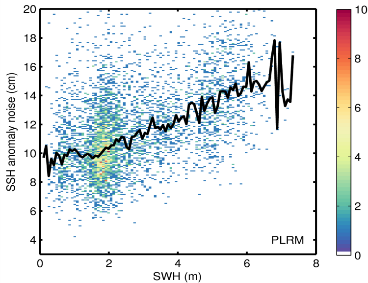
Figure 9. 2D histogram showing flag-valid SSH anomaly noise as a function of SWH for LRM (top) and PLRM (bottom) for 06/01/2015. The black line denotes the median SSH anomaly as a function of SWH.
