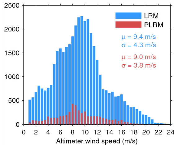
Figure 33. Histogram of flag-valid wind over oceans and lakes for LRM (blue) and PLRM (red) for 06/01/2015. The mean ( \mu ) and standard deviation ( \sigma ) are also shown. Note that values larger than 24 m/s are excluded from the histogram for the sake of readability but not from the computation of \mu and \sigma .
