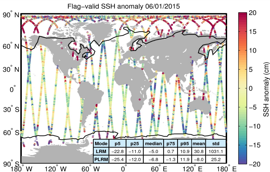
Figure 5. Geographical distribution of flag-valid 1-Hz SSH anomaly data over oceans and lakes for 06/01/2015. The statistical values shown in the table refer to the SSH anomaly in cm and are calculated separately for LRM and PLRM regions. Measurements taken over polar polygons have been excluded from the computation of the statistical values. The black lines mark the outer limit of the Arctic and Antarctic polar polygons.
