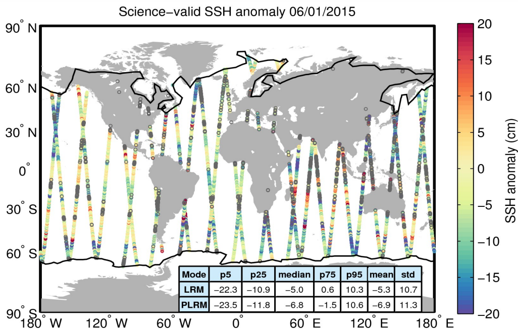
Figure 10. Geographical distribution of science-valid SSH anomaly data over oceans and lakes for 06/01/2015. The statistical values shown in the table refer to the SSH anomaly in cm and are calculated separately for LRM and PLRM regions. The black lines mark the outer limit of the Arctic and Antarctic polar polygons. Gray circles denote records that have been rejected based on the editing criteria described in Table 2.
