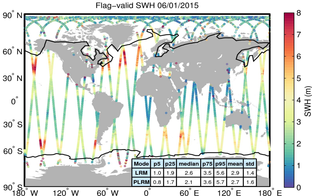
Figure 15. Geographical distribution of flag-valid SWH data over oceans and lakes for 06/01/2015. The statistical values shown in the table refer to the SWH in m and are calculated separately for LRM and PLRM regions. Measurements taken over polar polygons have been excluded from the computation of the statistical values. The black lines mark the outer limit of the Arctic and Antarctic polar polygons.
