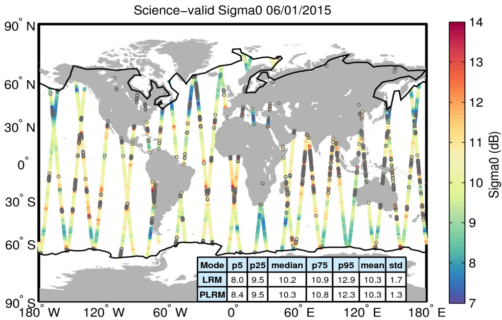
Figure 27. Geographical distribution of science-valid sigma0 data over oceans and lakes for 06/01/2015. The statistical values shown in the table refer to the sigma0 in dB and are calculated separately for LRM and PLRM regions. The black lines mark the outer limit of the Arctic and Antarctic polar polygons. Gray circles denote records that have been rejected based on the editing criteria described in Table 4.
