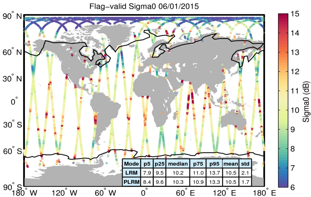
Figure 23. Geographical distribution of flag-valid sigma0 data over oceans and lakes for 06/01/2015. The statistical values shown in the table refer to the sigma0 in dB and are calculated separately for LRM and PLRM regions. Measurements taken over polar polygons have been excluded from the computation of the statistical values. The black lines mark the outer limit of the Arctic and Antarctic polar polygons.
