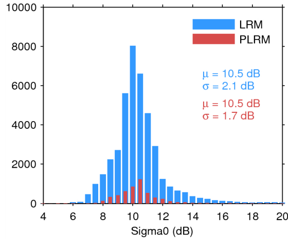
Figure 25. Histogram of flag-valid sigma0 over oceans and lakes for LRM (blue) and PLRM (red) for 06/01/2015. The mean ( \mu ) and standard deviation ( \sigma ) are also shown. Note that values outside [4 20] dB are excluded from the histogram for the sake of readability but not from the computation of \mu and \sigma .
