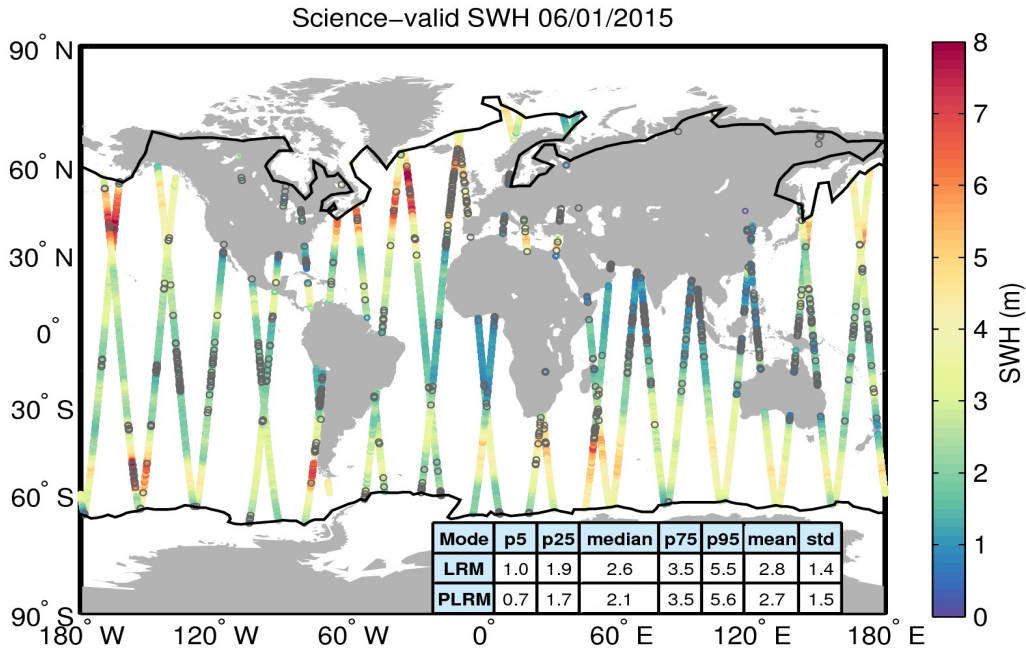
Figure 19. Geographical distribution of science-valid SWH data over oceans and lakes for 06/01/2015. The statistical values shown in the table refer to the SWH in m and are calculated separately for LRM and PLRM regions. The black lines mark the outer limit of the Arctic and Antarctic polar polygons. Gray circles denote records that have been rejected based on the editing criteria described in Table 3.
