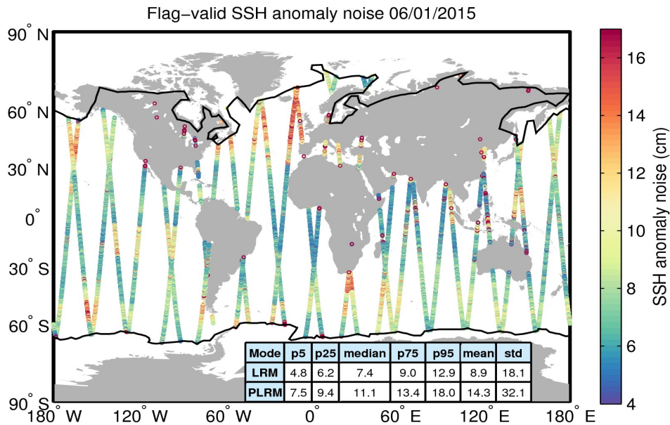
Figure 8. Geographical distribution of flag-valid 20-Hz SSH anomaly measurement noise over oceans and lakes for 06/01/2015. The statistical values shown in the table refer to the SSH anomaly noise and are calculated separately for LRM and PLRM regions. Measurements taken over polar polygons have been excluded from the computation of the statistical values. The black lines mark the outer limit of the Arctic and Antarctic polar polygons.
