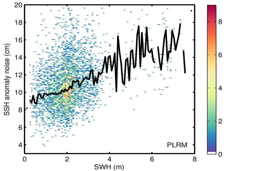
Figure 9. 2D histogram showing flag-valid SSH anomaly noise as a function of SWH for LRM (top) and PLRM (bottom) for 05/01/2015. The black line denotes the median SSH anomaly as a function of SWH.
