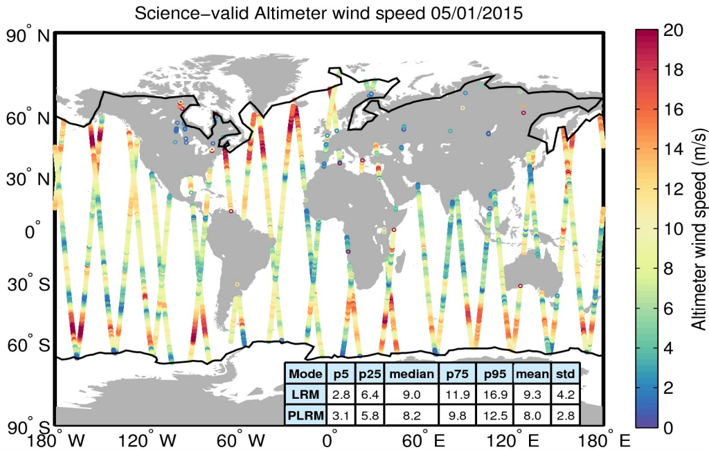
Figure 34. Geographical distribution of science-valid wind data over oceans and lakes for 05/01/2015. The statistical values shown in the table refer to the wind in m/s and are calculated separately for LRM and PLRM regions. The black lines mark the outer limit of the Arctic and Antarctic polar polygons. Gray circles denote records that have been rejected based on the editing criteria described in Table 5.
