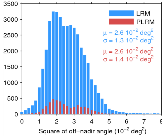
Figure 39. Histogram of flag-valid mispointing over oceans and lakes for LRM (blue) and PLRM (red) for 05/01/2015. Only positive values have been considered. The mean ( \mu ) and standard deviation ( \sigma ) are also shown. Note that values larger than 8 \cdot 10^{-2} \text{ deg}^2 are excluded from the histogram for the sake of readability but not from the computation of \mu and \sigma .
