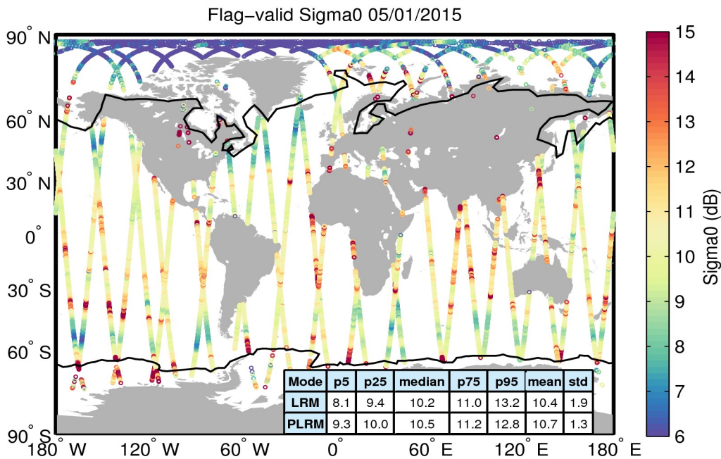
Figure 23. Geographical distribution of flag-valid sigma0 data over oceans and lakes for 05/01/2015. The statistical values shown in the table refer to the sigma0 in dB and are calculated separately for LRM and PLRM regions. Measurements taken over polar polygons have been excluded from the computation of the statistical values. The black lines mark the outer limit of the Arctic and Antarctic polar polygons.
