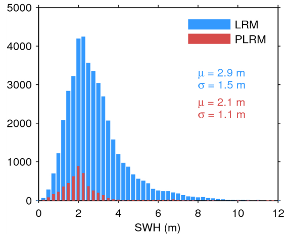
Figure 17. Histogram of flag-valid SWH over oceans and lakes for LRM (blue) and PLRM (red) for 05/01/2015. The mean ( \mu ) and standard deviation ( \sigma ) are also shown. Note that values larger than 12 m are excluded from the histogram for the sake of readability but not from the computation of \mu and \sigma .
