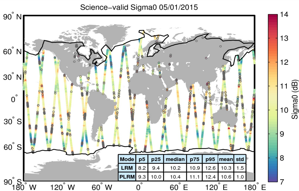
Figure 27. Geographical distribution of science-valid sigma0 data over oceans and lakes for 05/01/2015. The statistical values shown in the table refer to the sigma0 in dB and are calculated separately for LRM and PLRM regions. The black lines mark the outer limit of the Arctic and Antarctic polar polygons. Gray circles denote records that have been rejected based on the editing criteria described in Table 4.
