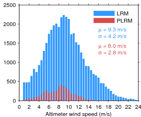
Figure 35. Histogram of science-valid wind over oceans and lakes for LRM (blue) and PLRM (red) for 05/01/2015. The mean ( \mu ) and standard deviation ( \sigma ) are also shown. Note that values larger than 24 m/s are excluded from the histogram for the sake of readability but not from the computation of \mu and \sigma .
