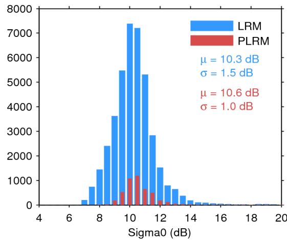
Figure 28. Histogram of science-valid sigma0 over oceans and lakes for LRM (blue) and PLRM (red) for 05/01/2015. The mean ( \mu ) and standard deviation ( \sigma ) are also shown. Note that values outside [4 20] dB are excluded from the histogram for the sake of readability but not from the computation of \mu and \sigma .
