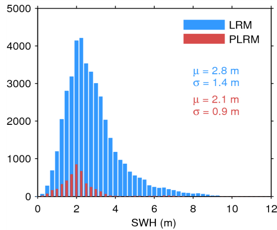
Figure 20. Histogram of science-valid SWH over oceans and lakes for LRM (blue) and PLRM (red) for 05/01/2015. The mean ( \mu ) and standard deviation ( \sigma ) are also shown. Note that values larger than 12 m are excluded from the histogram for the sake of readability but not from the computation of \mu and \sigma .
