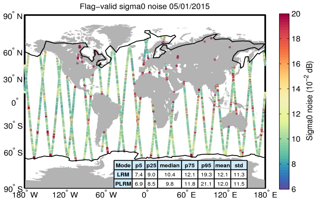
Figure 26. Geographical distribution of flag-valid 20-Hz sigma0 measurement noise over oceans and lakes for 05/01/2015. The statistical values shown in the table refer to the sigma0 noise and are calculated separately for LRM and PLRM regions. Measurements taken over polar polygons have been excluded from the computation of the statistical values. The black lines mark the outer limit of the Arctic and Antarctic polar polygons.
