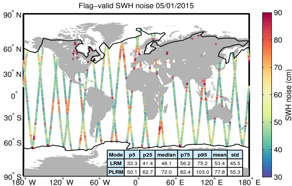
Figure 18. Geographical distribution of flag-valid 20-Hz SWH measurement noise over oceans and lakes for 05/01/2015. The statistical values shown in the table refer to the SWH noise and are calculated separately for LRM and PLRM regions. Measurements taken over polar polygons have been excluded from the computation of the statistical values. The black lines mark the outer limit of the Arctic and Antarctic polar polygons.
