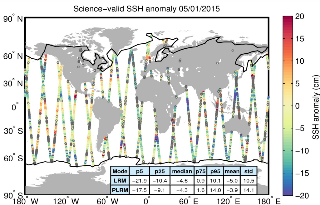
Figure 10. Geographical distribution of science-valid SSH anomaly data over oceans and lakes for 05/01/2015. The statistical values shown in the table refer to the SSH anomaly in cm and are calculated separately for LRM and PLRM regions. The black lines mark the outer limit of the Arctic and Antarctic polar polygons. Gray circles denote records that have been rejected based on the editing criteria described in Table 2.
