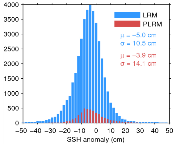
Figure 11. Histogram of science-valid SSH anomaly over oceans and lakes for LRM (blue) and PLRM (red) for 05/01/2015. The mean ( \mu ) and standard deviation ( \sigma ) are also shown. Note that values outside [-50\ 50] cm are excluded from the histogram for the sake of readability but not from the computation of \mu and \sigma .
