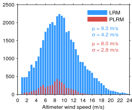
Figure 33. Histogram of flag-valid wind over oceans and lakes for LRM (blue) and PLRM (red) for 05/01/2015. The mean ( \mu ) and standard deviation ( \sigma ) are also shown. Note that values larger than 24 m/s are excluded from the histogram for the sake of readability but not from the computation of \mu and \sigma .
