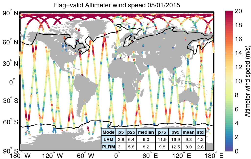
Figure 31. Geographical distribution of flag-valid wind data over oceans and lakes for 05/01/2015. The statistical values shown in the table refer to the wind in m/s and are calculated separately for LRM and PLRM regions. Measurements taken over polar polygons have been excluded from the computation of the statistical values. The black lines mark the outer limit of the Arctic and Antarctic polar polygons.
