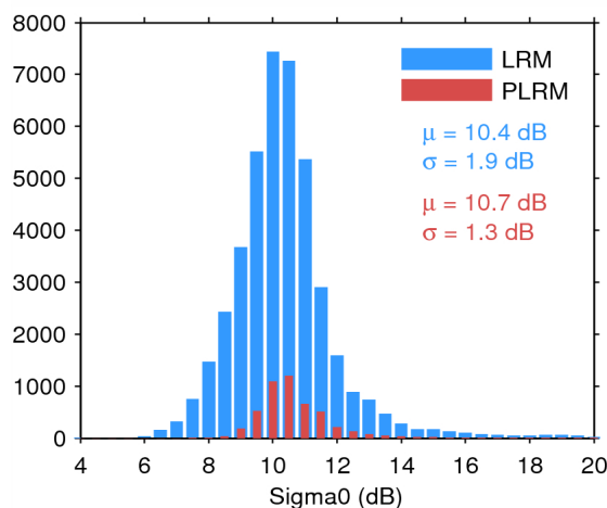
Figure 25. Histogram of flag-valid sigma0 over oceans and lakes for LRM (blue) and PLRM (red) for 05/01/2015. The mean ( \mu ) and standard deviation ( \sigma ) are also shown. Note that values outside [4 20] dB are excluded from the histogram for the sake of readability but not from the computation of \mu and \sigma .
