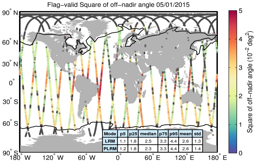
Figure 37. Geographical distribution of flag-valid mispointing data over oceans and lakes for 05/01/2015. The statistical values shown in the table refer to the mispointing in 10^{-2} \text{ deg}^2 and are calculated separately for LRM and PLRM regions. Measurements taken over polar polygons have been excluded from the computation of the statistical values. The black lines mark the outer limit of the Arctic and Antarctic polar polygons. Gray circles denote negative values.
