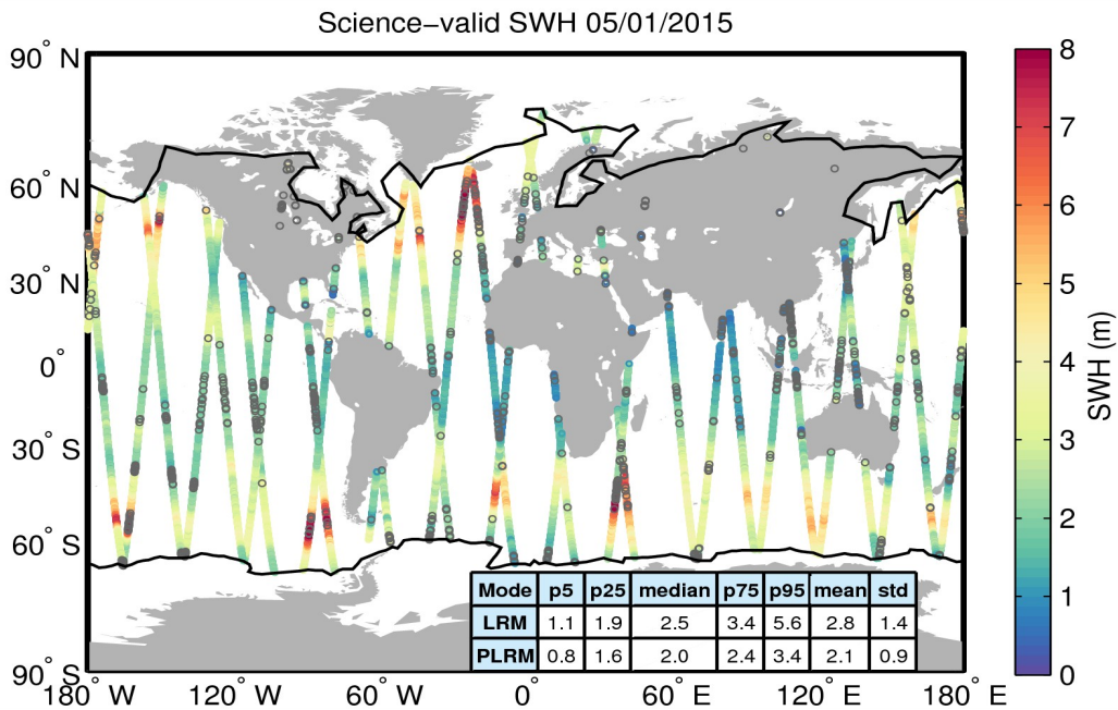
Figure 19. Geographical distribution of science-valid SWH data over oceans and lakes for 05/01/2015. The statistical values shown in the table refer to the SWH in m and are calculated separately for LRM and PLRM regions. The black lines mark the outer limit of the Arctic and Antarctic polar polygons. Gray circles denote records that have been rejected based on the editing criteria described in Table 3.
