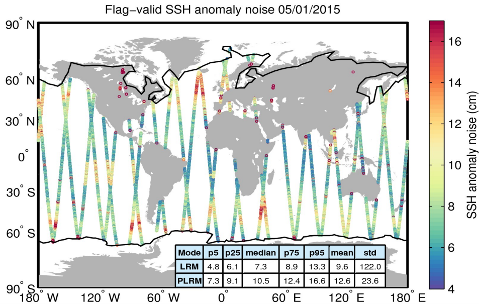
Figure 8. Geographical distribution of flag-valid 20-Hz SSH anomaly measurement noise over oceans and lakes for 05/01/2015. The statistical values shown in the table refer to the SSH anomaly noise and are calculated separately for LRM and PLRM regions. Measurements taken over polar polygons have been excluded from the computation of the statistical values. The black lines mark the outer limit of the Arctic and Antarctic polar polygons.
