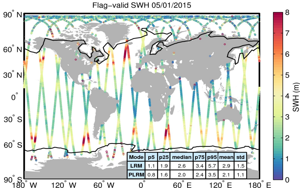
Figure 15. Geographical distribution of flag-valid SWH data over oceans and lakes for 05/01/2015. The statistical values shown in the table refer to the SWH in m and are calculated separately for LRM and PLRM regions. Measurements taken over polar polygons have been excluded from the computation of the statistical values. The black lines mark the outer limit of the Arctic and Antarctic polar polygons.
