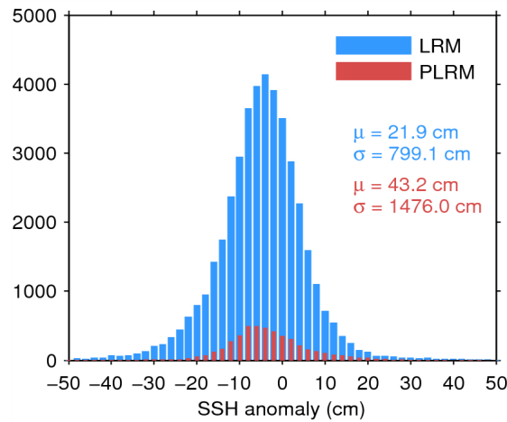
Figure 7. Histogram of flag-valid SSH anomaly over oceans and lakes for LRM (blue) and PLRM (red) for 05/01/2015. The mean ( \mu ) and standard deviation ( \sigma ) are also shown. Note that values outside [-50\ 50] cm are excluded from the histogram for the sake of readability but not from the computation of \mu and \sigma .
