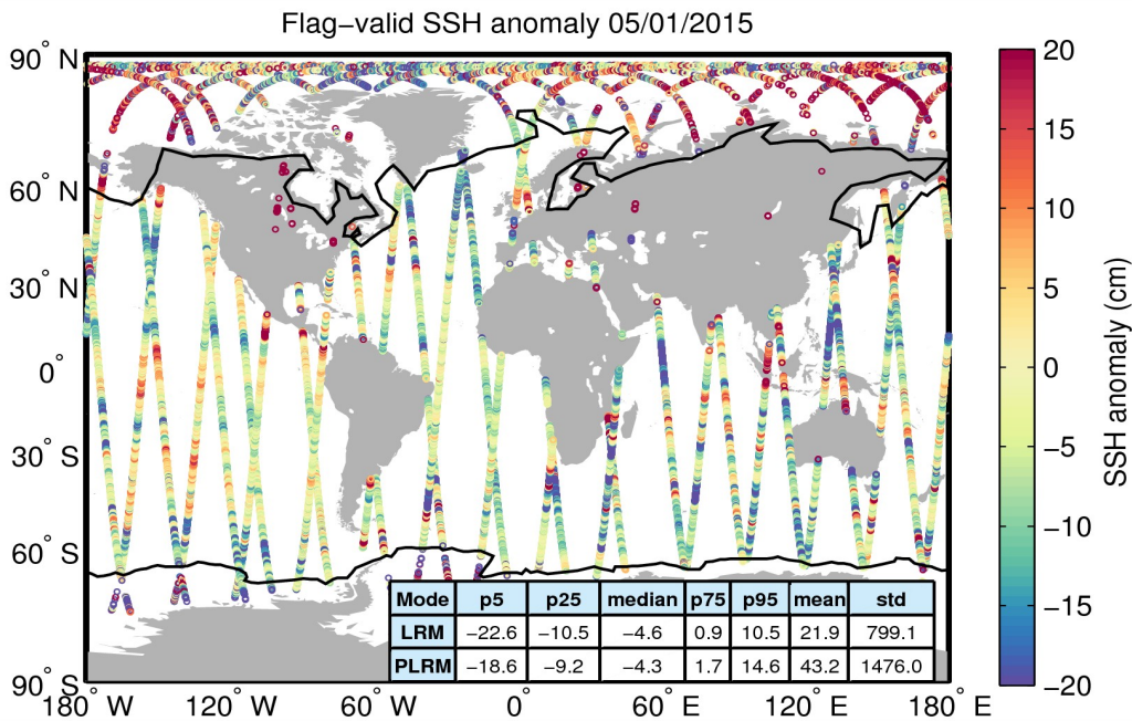
Figure 5. Geographical distribution of flag-valid 1-Hz SSH anomaly data over oceans and lakes for 05/01/2015. The statistical values shown in the table refer to the SSH anomaly in cm and are calculated separately for LRM and PLRM regions. Measurements taken over polar polygons have been excluded from the computation of the statistical values. The black lines mark the outer limit of the Arctic and Antarctic polar polygons.
