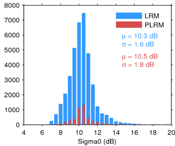
Figure 28. Histogram of science-valid sigma0 over oceans and lakes for LRM (blue) and PLRM (red) for 04/01/2015. The mean ( \mu ) and standard deviation ( \sigma ) are also shown. Note that values outside [4 20] dB are excluded from the histogram for the sake of readability but not from the computation of \mu and \sigma .
