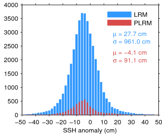
Figure 7. Histogram of flag-valid SSH anomaly over oceans and lakes for LRM (blue) and PLRM (red) for 04/01/2015. The mean ( \mu ) and standard deviation ( \sigma ) are also shown. Note that values outside [-50\ 50] cm are excluded from the histogram for the sake of readability but not from the computation of \mu and \sigma .
