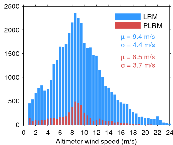
Figure 35. Histogram of science-valid wind over oceans and lakes for LRM (blue) and PLRM (red) for 04/01/2015. The mean ( \mu ) and standard deviation ( \sigma ) are also shown. Note that values larger than 24 m/s are excluded from the histogram for the sake of readability but not from the computation of \mu and \sigma .
