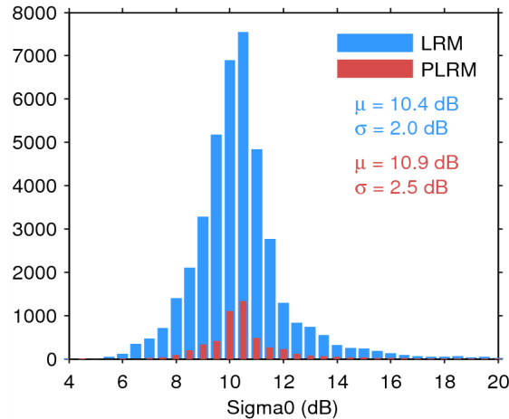
Figure 25. Histogram of flag-valid sigma0 over oceans and lakes for LRM (blue) and PLRM (red) for 04/01/2015. The mean ( \mu ) and standard deviation ( \sigma ) are also shown. Note that values outside [4 20] dB are excluded from the histogram for the sake of readability but not from the computation of \mu and \sigma .
