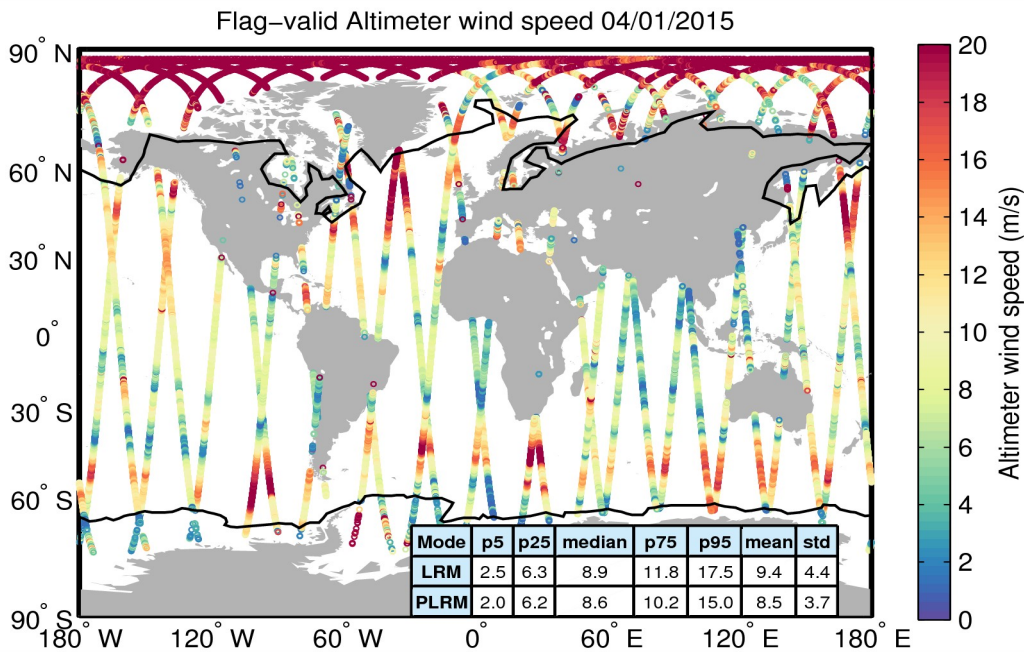
Figure 31. Geographical distribution of flag-valid wind data over oceans and lakes for 04/01/2015. The statistical values shown in the table refer to the wind in m/s and are calculated separately for LRM and PLRM regions. Measurements taken over polar polygons have been excluded from the computation of the statistical values. The black lines mark the outer limit of the Arctic and Antarctic polar polygons.
