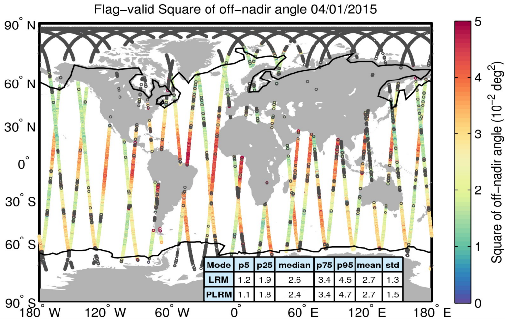
Figure 37. Geographical distribution of flag-valid mispointing data over oceans and lakes for 04/01/2015. The statistical values shown in the table refer to the mispointing in 10^{-2} \text{ deg}^2 and are calculated separately for LRM and PLRM regions. Measurements taken over polar polygons have been excluded from the computation of the statistical values. The black lines mark the outer limit of the Arctic and Antarctic polar polygons. Gray circles denote negative values.
