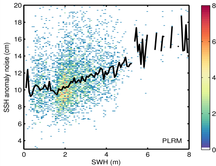
Figure 9. 2D histogram showing flag-valid SSH anomaly noise as a function of SWH for LRM (top) and PLRM (bottom) for 04/01/2015. The black line denotes the median SSH anomaly as a function of SWH.
