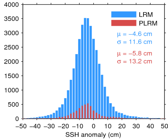
Figure 11. Histogram of science-valid SSH anomaly over oceans and lakes for LRM (blue) and PLRM (red) for 04/01/2015. The mean ( \mu ) and standard deviation ( \sigma ) are also shown. Note that values outside [-50 50] cm are excluded from the histogram for the sake of readability but not from the computation of \mu and \sigma .
