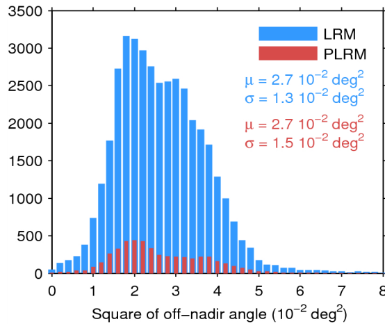
Figure 39. Histogram of flag-valid mispointing over oceans and lakes for LRM (blue) and PLRM (red) for 04/01/2015. Only positive values have been considered. The mean ( \mu ) and standard deviation ( \sigma ) are also shown. Note that values larger than 8 \cdot 10^{-2} \text{ deg}^2 are excluded from the histogram for the sake of readability but not from the computation of \mu and \sigma .
