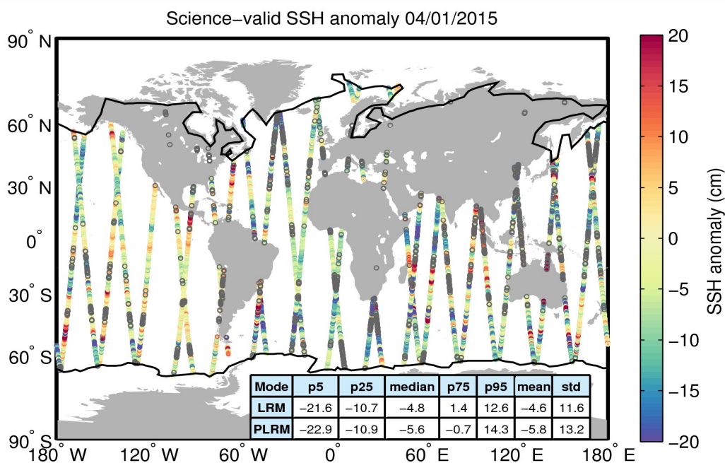
Figure 10. Geographical distribution of science-valid SSH anomaly data over oceans and lakes for 04/01/2015. The statistical values shown in the table refer to the SSH anomaly in cm and are calculated separately for LRM and PLRM regions. The black lines mark the outer limit of the Arctic and Antarctic polar polygons. Gray circles denote records that have been rejected based on the editing criteria described in Table 2.
