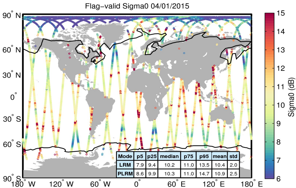
Figure 23. Geographical distribution of flag-valid sigma0 data over oceans and lakes for 04/01/2015. The statistical values shown in the table refer to the sigma0 in dB and are calculated separately for LRM and PLRM regions. Measurements taken over polar polygons have been excluded from the computation of the statistical values. The black lines mark the outer limit of the Arctic and Antarctic polar polygons.
