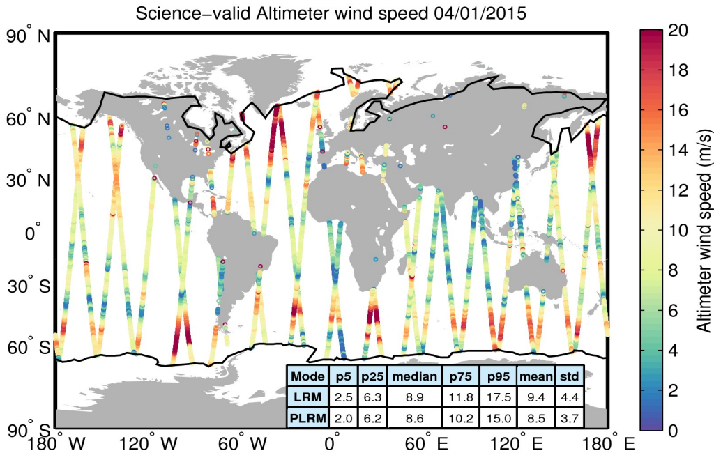
Figure 34. Geographical distribution of science-valid wind data over oceans and lakes for 04/01/2015. The statistical values shown in the table refer to the wind in m/s and are calculated separately for LRM and PLRM regions. The black lines mark the outer limit of the Arctic and Antarctic polar polygons. Gray circles denote records that have been rejected based on the editing criteria described in Table 5.
