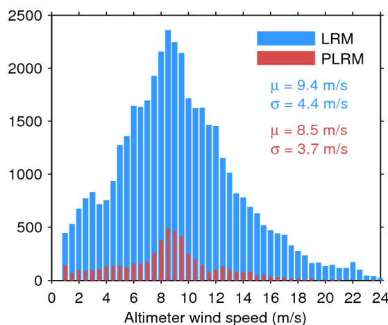
Figure 33. Histogram of flag-valid wind over oceans and lakes for LRM (blue) and PLRM (red) for 04/01/2015. The mean ( \mu ) and standard deviation ( \sigma ) are also shown. Note that values larger than 24 m/s are excluded from the histogram for the sake of readability but not from the computation of \mu and \sigma .
