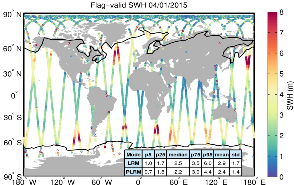
Figure 15. Geographical distribution of flag-valid SWH data over oceans and lakes for 04/01/2015. The statistical values shown in the table refer to the SWH in m and are calculated separately for LRM and PLRM regions. Measurements taken over polar polygons have been excluded from the computation of the statistical values. The black lines mark the outer limit of the Arctic and Antarctic polar polygons.
