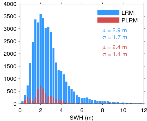
Figure 17. Histogram of flag-valid SWH over oceans and lakes for LRM (blue) and PLRM (red) for 04/01/2015. The mean ( \mu ) and standard deviation ( \sigma ) are also shown. Note that values larger than 12 m are excluded from the histogram for the sake of readability but not from the computation of \mu and \sigma .
