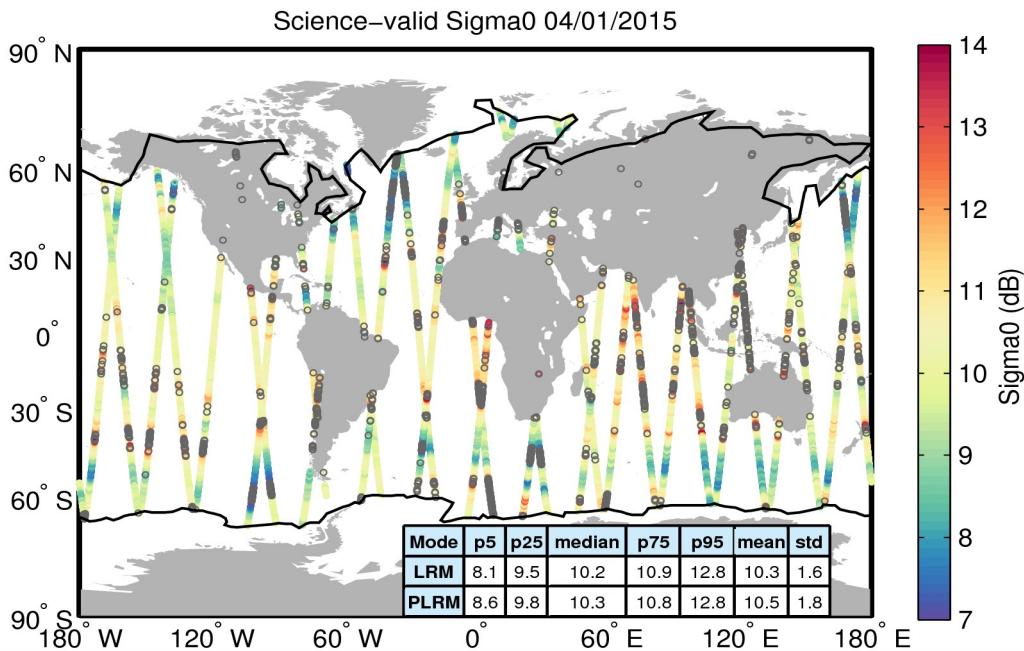
Figure 27. Geographical distribution of science-valid sigma0 data over oceans and lakes for 04/01/2015. The statistical values shown in the table refer to the sigma0 in dB and are calculated separately for LRM and PLRM regions. The black lines mark the outer limit of the Arctic and Antarctic polar polygons. Gray circles denote records that have been rejected based on the editing criteria described in Table 4.
