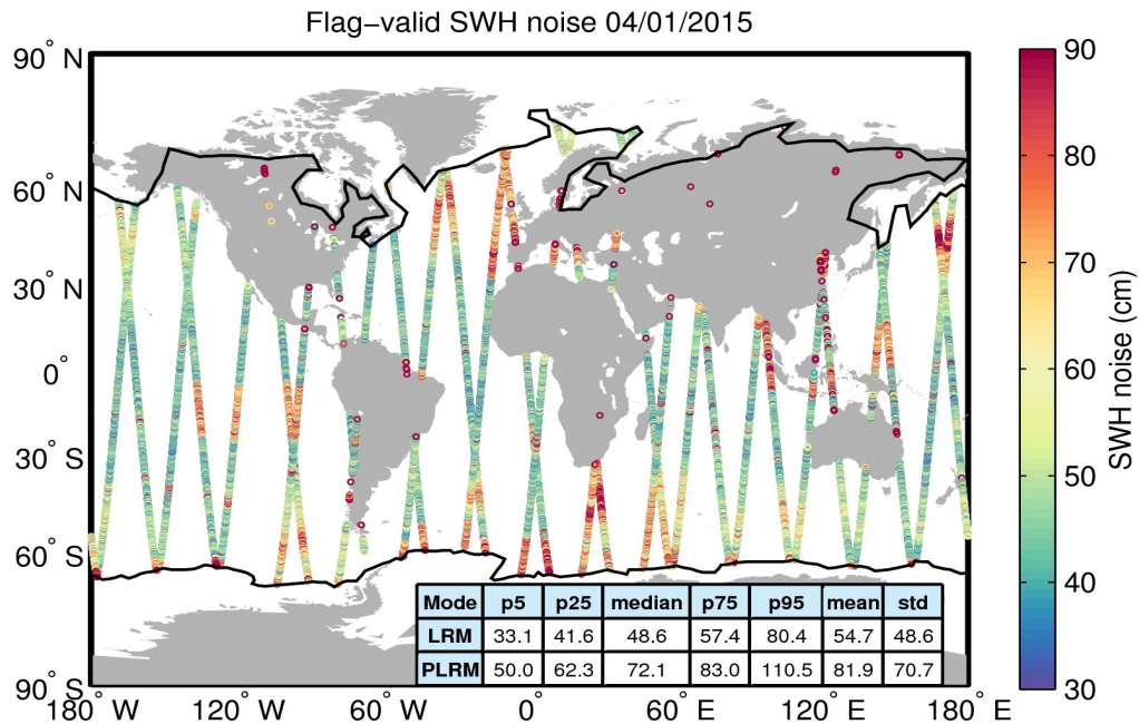
Figure 18. Geographical distribution of flag-valid 20-Hz SWH measurement noise over oceans and lakes for 04/01/2015. The statistical values shown in the table refer to the SWH noise and are calculated separately for LRM and PLRM regions. Measurements taken over polar polygons have been excluded from the computation of the statistical values. The black lines mark the outer limit of the Arctic and Antarctic polar polygons.
