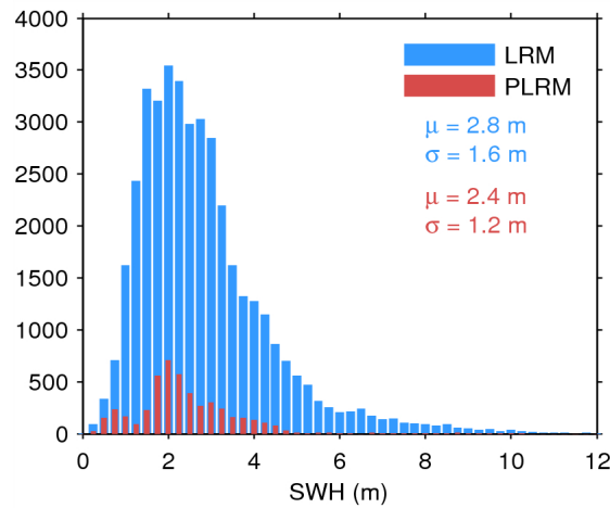
Figure 20. Histogram of science-valid SWH over oceans and lakes for LRM (blue) and PLRM (red) for 04/01/2015. The mean ( \mu ) and standard deviation ( \sigma ) are also shown. Note that values larger than 12 m are excluded from the histogram for the sake of readability but not from the computation of \mu and \sigma .
