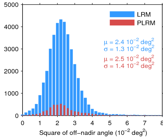
Figure 39. Histogram of flag-valid mispointing over oceans and lakes for LRM (blue) and PLRM (red) for 07/11/2014. Only positive values have been considered. The mean ( \mu ) and standard deviation ( \sigma ) are also shown. Note that values larger than 8 \cdot 10^{-2} \text{ deg}^2 are excluded from the histogram for the sake of readability but not from the computation of \mu and \sigma .
