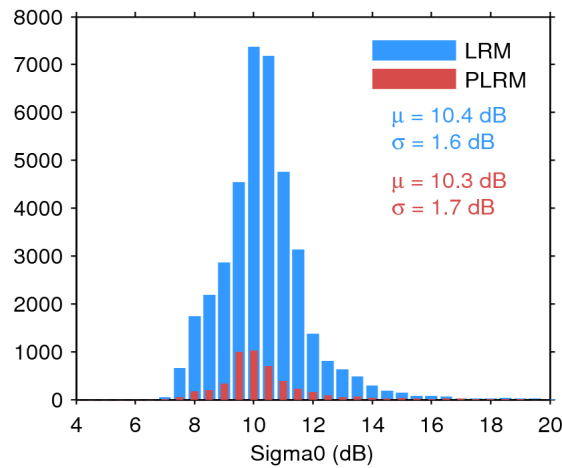
Figure 28. Histogram of science-valid sigma0 over oceans and lakes for LRM (blue) and PLRM (red) for 07/11/2014. The mean ( \mu ) and standard deviation ( \sigma ) are also shown. Note that values outside [4 20] dB are excluded from the histogram for the sake of readability but not from the computation of \mu and \sigma .
