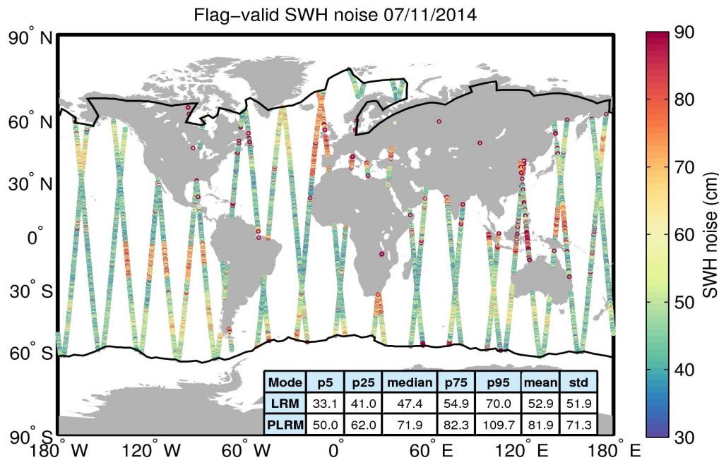
Figure 18. Geographical distribution of flag-valid 20-Hz SWH measurement noise over oceans and lakes for 07/11/2014. The statistical values shown in the table refer to the SWH noise and are calculated separately for LRM and PLRM regions. Measurements taken over polar polygons have been excluded from the computation of the statistical values. The black lines mark the outer limit of the Arctic and Antarctic polar polygons.
