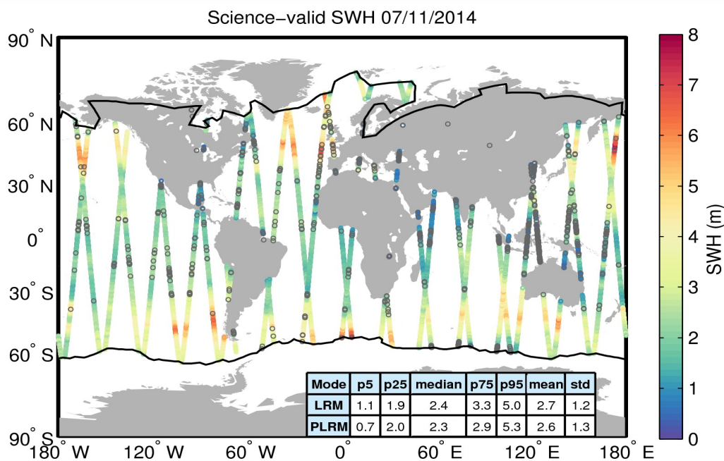
Figure 19. Geographical distribution of science-valid SWH data over oceans and lakes for 07/11/2014. The statistical values shown in the table refer to the SWH in m and are calculated separately for LRM and PLRM regions. The black lines mark the outer limit of the Arctic and Antarctic polar polygons. Gray circles denote records that have been rejected based on the editing criteria described in Table 3.
