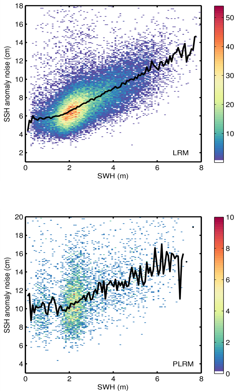
Figure 9. 2D histogram showing flag-valid SSH anomaly noise as a function of SWH for LRM (top) and PLRM (bottom) for 07/11/2014. The black line denotes the median SSH anomaly as a function of SWH.
