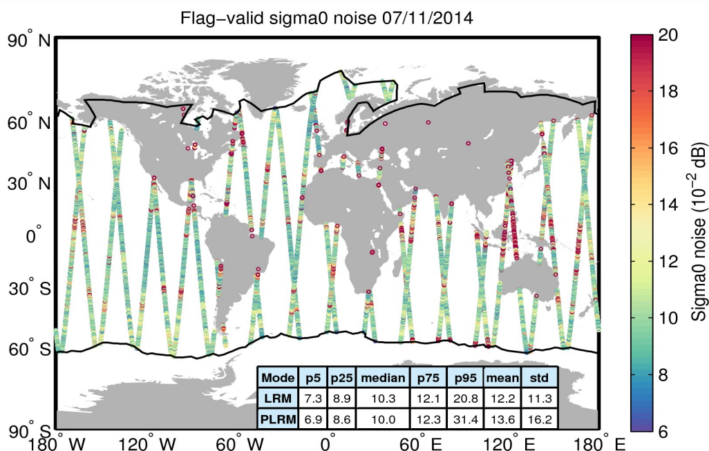
Figure 26. Geographical distribution of flag-valid 20-Hz sigma0 measurement noise over oceans and lakes for 07/11/2014. The statistical values shown in the table refer to the sigma0 noise and are calculated separately for LRM and PLRM regions. Measurements taken over polar polygons have been excluded from the computation of the statistical values. The black lines mark the outer limit of the Arctic and Antarctic polar polygons.
