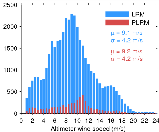
Figure 35. Histogram of science-valid wind over oceans and lakes for LRM (blue) and PLRM (red) for 07/11/2014. The mean ( \mu ) and standard deviation ( \sigma ) are also shown. Note that values larger than 24 m/s are excluded from the histogram for the sake of readability but not from the computation of \mu and \sigma .
