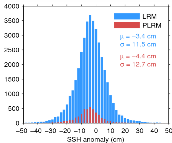
Figure 11. Histogram of science-valid SSH anomaly over oceans and lakes for LRM (blue) and PLRM (red) for 07/11/2014. The mean ( \mu ) and standard deviation ( \sigma ) are also shown. Note that values outside [-50 50] cm are excluded from the histogram for the sake of readability but not from the computation of \mu and \sigma .
