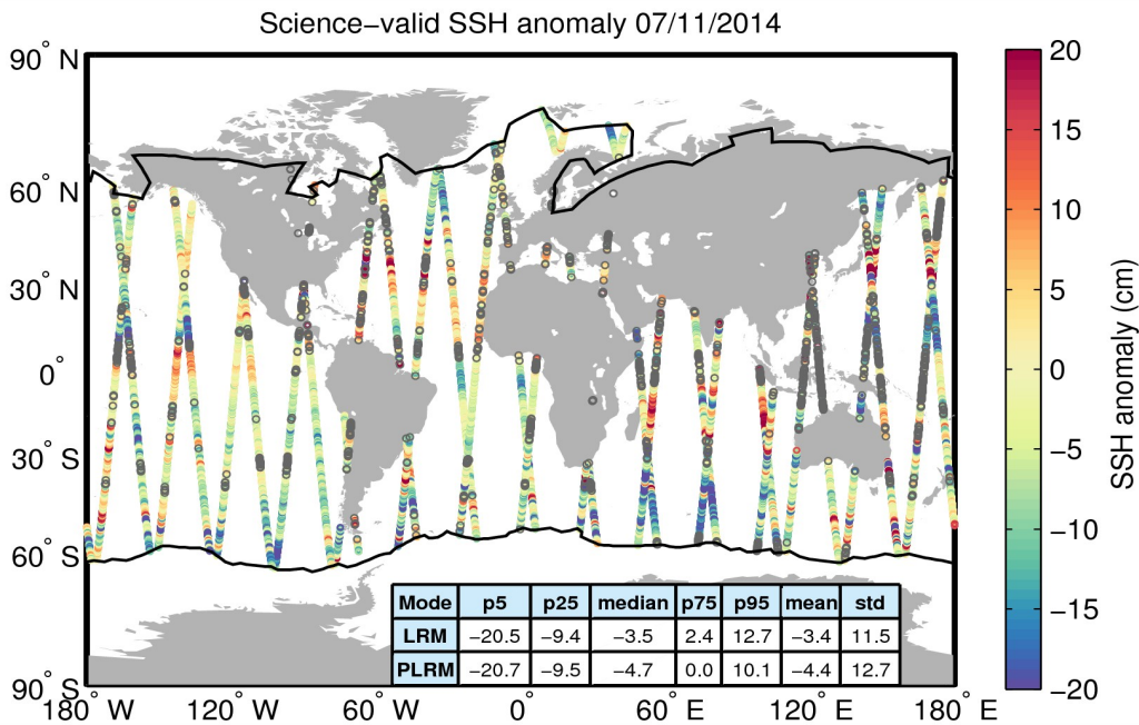
Figure 10. Geographical distribution of science-valid SSH anomaly data over oceans and lakes for 07/11/2014. The statistical values shown in the table refer to the SSH anomaly in cm and are calculated separately for LRM and PLRM regions. The black lines mark the outer limit of the Arctic and Antarctic polar polygons. Gray circles denote records that have been rejected based on the editing criteria described in Table 2.
