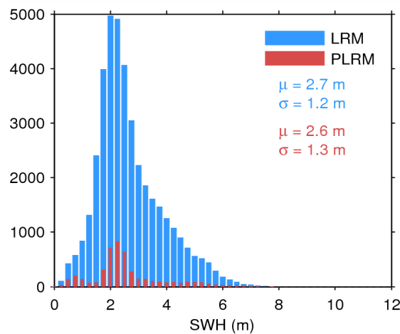
Figure 20. Histogram of science-valid SWH over oceans and lakes for LRM (blue) and PLRM (red) for 07/11/2014. The mean ( \mu ) and standard deviation ( \sigma ) are also shown. Note that values larger than 12 m are excluded from the histogram for the sake of readability but not from the computation of \mu and \sigma .
