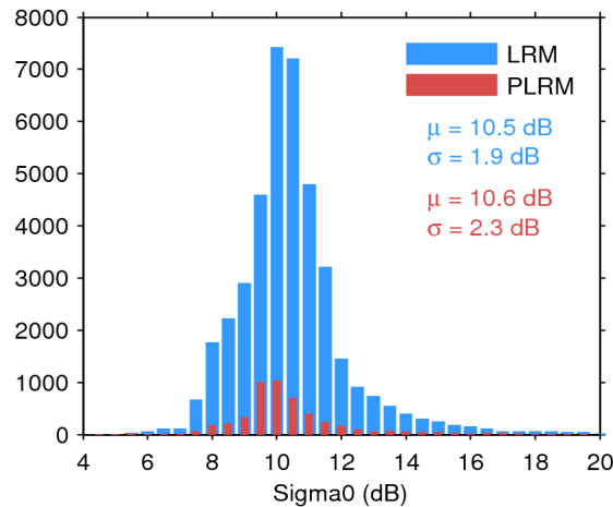
Figure 25. Histogram of flag-valid sigma0 over oceans and lakes for LRM (blue) and PLRM (red) for 07/11/2014. The mean ( \mu ) and standard deviation ( \sigma ) are also shown. Note that values outside [4 20] dB are excluded from the histogram for the sake of readability but not from the computation of \mu and \sigma .
