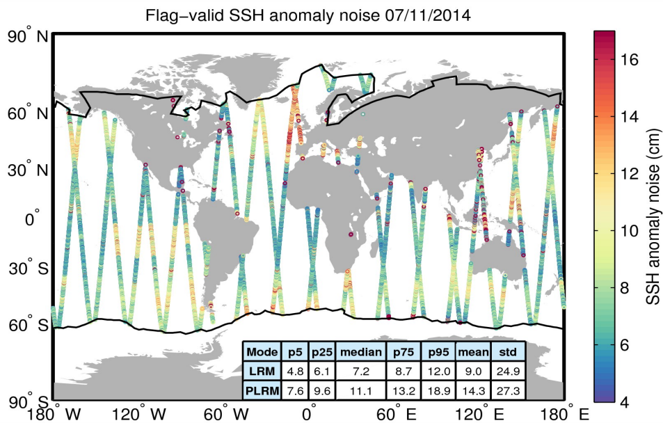
Figure 8. Geographical distribution of flag-valid 20-Hz SSH anomaly measurement noise over oceans and lakes for 07/11/2014. The statistical values shown in the table refer to the SSH anomaly noise and are calculated separately for LRM and PLRM regions. Measurements taken over polar polygons have been excluded from the computation of the statistical values. The black lines mark the outer limit of the Arctic and Antarctic polar polygons.
