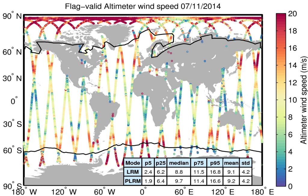
Figure 31. Geographical distribution of flag-valid wind data over oceans and lakes for 07/11/2014. The statistical values shown in the table refer to the wind in m/s and are calculated separately for LRM and PLRM regions. Measurements taken over polar polygons have been excluded from the computation of the statistical values. The black lines mark the outer limit of the Arctic and Antarctic polar polygons.
