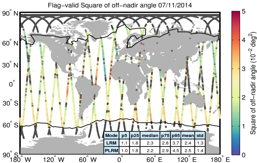
Figure 37. Geographical distribution of flag-valid mispointing data over oceans and lakes for 07/11/2014. The statistical values shown in the table refer to the mispointing in 10^{-2} \text{ deg}^2 and are calculated separately for LRM and PLRM regions. Measurements taken over polar polygons have been excluded from the computation of the statistical values. The black lines mark the outer limit of the Arctic and Antarctic polar polygons. Gray circles denote negative values.
