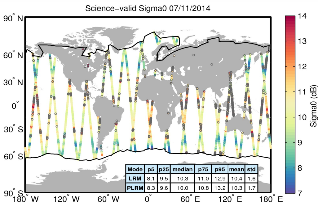
Figure 27. Geographical distribution of science-valid sigma0 data over oceans and lakes for 07/11/2014. The statistical values shown in the table refer to the sigma0 in dB and are calculated separately for LRM and PLRM regions. The black lines mark the outer limit of the Arctic and Antarctic polar polygons. Gray circles denote records that have been rejected based on the editing criteria described in Table 4.
