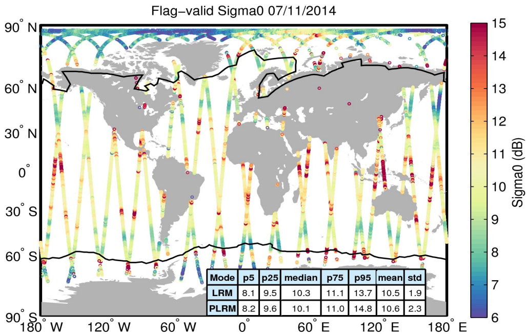
Figure 23. Geographical distribution of flag-valid sigma0 data over oceans and lakes for 07/11/2014. The statistical values shown in the table refer to the sigma0 in dB and are calculated separately for LRM and PLRM regions. Measurements taken over polar polygons have been excluded from the computation of the statistical values. The black lines mark the outer limit of the Arctic and Antarctic polar polygons.
