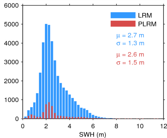
Figure 17. Histogram of flag-valid SWH over oceans and lakes for LRM (blue) and PLRM (red) for 07/11/2014. The mean ( \mu ) and standard deviation ( \sigma ) are also shown. Note that values larger than 12 m are excluded from the histogram for the sake of readability but not from the computation of \mu and \sigma .
