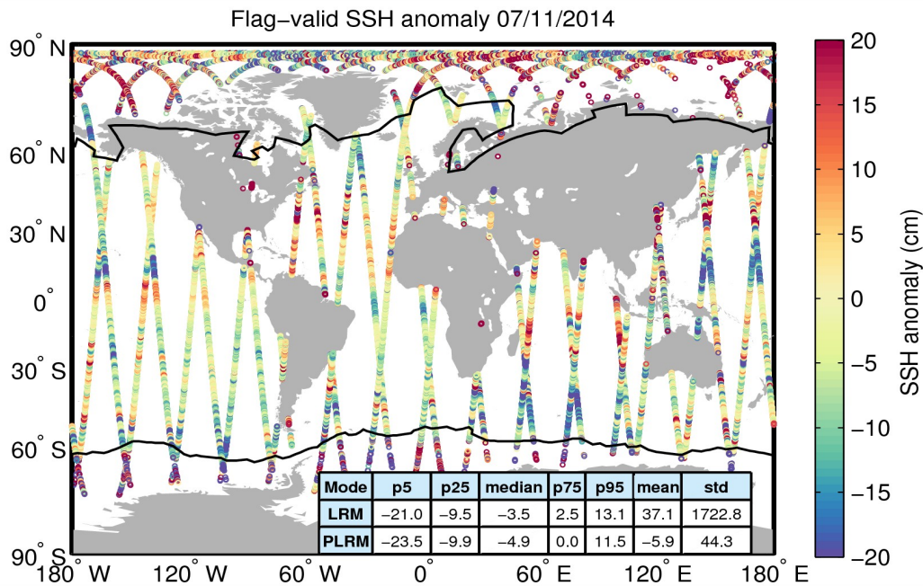
Figure 5. Geographical distribution of flag-valid 1-Hz SSH anomaly data over oceans and lakes for 07/11/2014. The statistical values shown in the table refer to the SSH anomaly in cm and are calculated separately for LRM and PLRM regions. Measurements taken over polar polygons have been excluded from the computation of the statistical values. The black lines mark the outer limit of the Arctic and Antarctic polar polygons.
