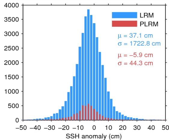
Figure 7. Histogram of flag-valid SSH anomaly over oceans and lakes for LRM (blue) and PLRM (red) for 07/11/2014. The mean ( \mu ) and standard deviation ( \sigma ) are also shown. Note that values outside [-50\ 50] cm are excluded from the histogram for the sake of readability but not from the computation of \mu and \sigma .
