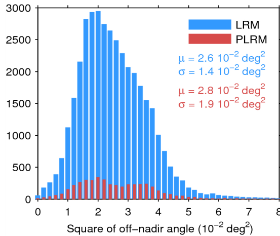
Figure 39. Histogram of flag-valid mispointing over oceans and lakes for LRM (blue) and PLRM (red) for 23/10/2014. Only positive values have been considered. The mean ( \mu ) and standard deviation ( \sigma ) are also shown. Note that values larger than 8 \cdot 10^{-2} \text{ deg}^2 are excluded from the histogram for the sake of readability but not from the computation of \mu and \sigma .
