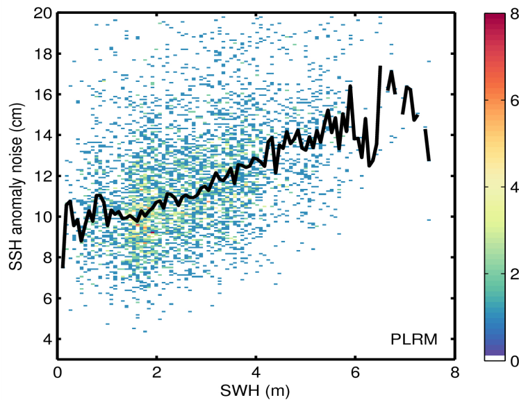
Figure 9. 2D histogram showing flag-valid SSH anomaly noise as a function of SWH for LRM (top) and PLRM (bottom) for 23/10/2014. The black line denotes the median SSH anomaly as a function of SWH.
