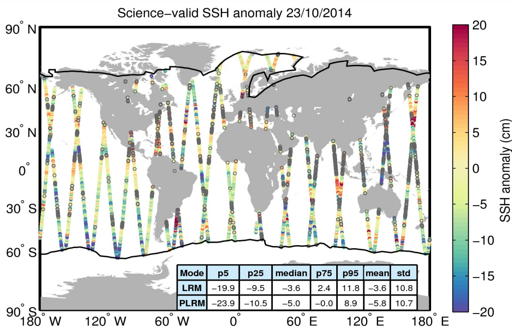
Figure 10. Geographical distribution of science-valid SSH anomaly data over oceans and lakes for 23/10/2014. The statistical values shown in the table refer to the SSH anomaly in cm and are calculated separately for LRM and PLRM regions. The black lines mark the outer limit of the Arctic and Antarctic polar polygons. Gray circles denote records that have been rejected based on the editing criteria described in Table 2.
