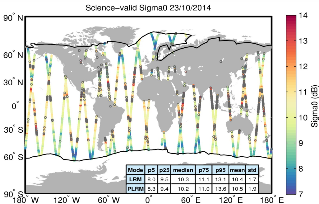
Figure 27. Geographical distribution of science-valid sigma0 data over oceans and lakes for 23/10/2014. The statistical values shown in the table refer to the sigma0 in dB and are calculated separately for LRM and PLRM regions. The black lines mark the outer limit of the Arctic and Antarctic polar polygons. Gray circles denote records that have been rejected based on the editing criteria described in Table 4.
