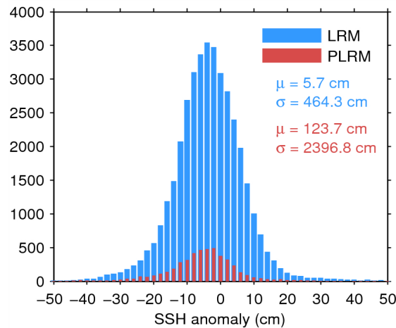
Figure 7. Histogram of flag-valid SSH anomaly over oceans and lakes for LRM (blue) and PLRM (red) for 23/10/2014. The mean ( \mu ) and standard deviation ( \sigma ) are also shown. Note that values outside [-50\ 50] cm are excluded from the histogram for the sake of readability but not from the computation of \mu and \sigma .
