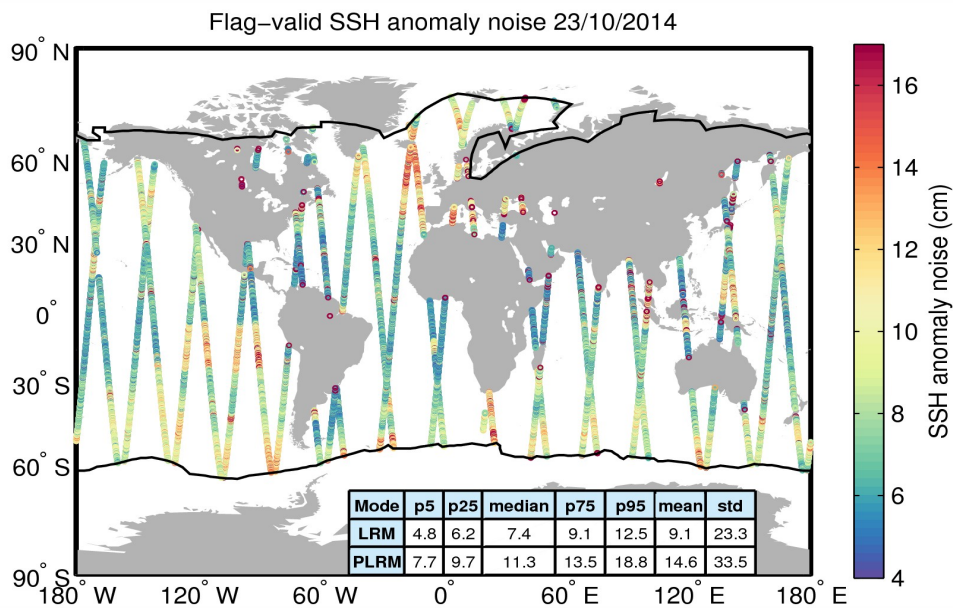
Figure 8. Geographical distribution of flag-valid 20-Hz SSH anomaly measurement noise over oceans and lakes for 23/10/2014. The statistical values shown in the table refer to the SSH anomaly noise and are calculated separately for LRM and PLRM regions. Measurements taken over polar polygons have been excluded from the computation of the statistical values. The black lines mark the outer limit of the Arctic and Antarctic polar polygons.
