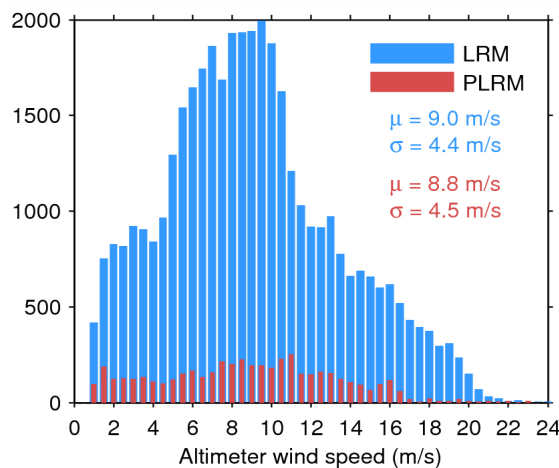
Figure 35. Histogram of science-valid wind over oceans and lakes for LRM (blue) and PLRM (red) for 23/10/2014. The mean ( \mu ) and standard deviation ( \sigma ) are also shown. Note that values larger than 24 m/s are excluded from the histogram for the sake of readability but not from the computation of \mu and \sigma .
