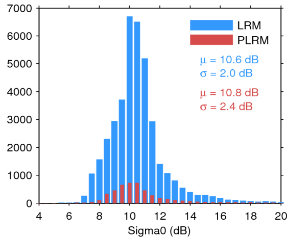
Figure 25. Histogram of flag-valid sigma0 over oceans and lakes for LRM (blue) and PLRM (red) for 23/10/2014. The mean ( \mu ) and standard deviation ( \sigma ) are also shown. Note that values outside [4 20] dB are excluded from the histogram for the sake of readability but not from the computation of \mu and \sigma .
