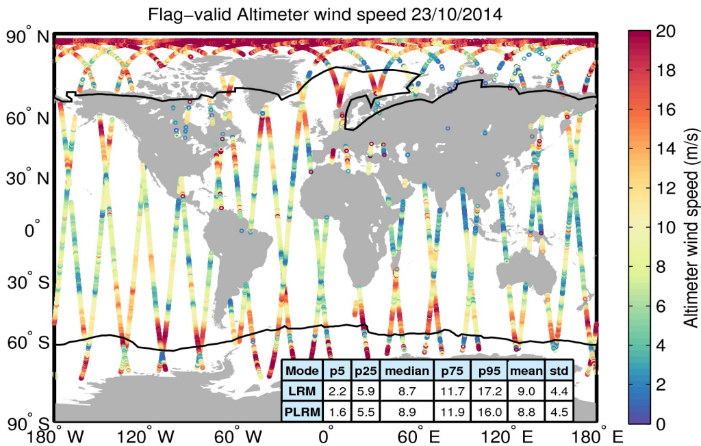
Figure 31. Geographical distribution of flag-valid wind data over oceans and lakes for 23/10/2014. The statistical values shown in the table refer to the wind in m/s and are calculated separately for LRM and PLRM regions. Measurements taken over polar polygons have been excluded from the computation of the statistical values. The black lines mark the outer limit of the Arctic and Antarctic polar polygons.
