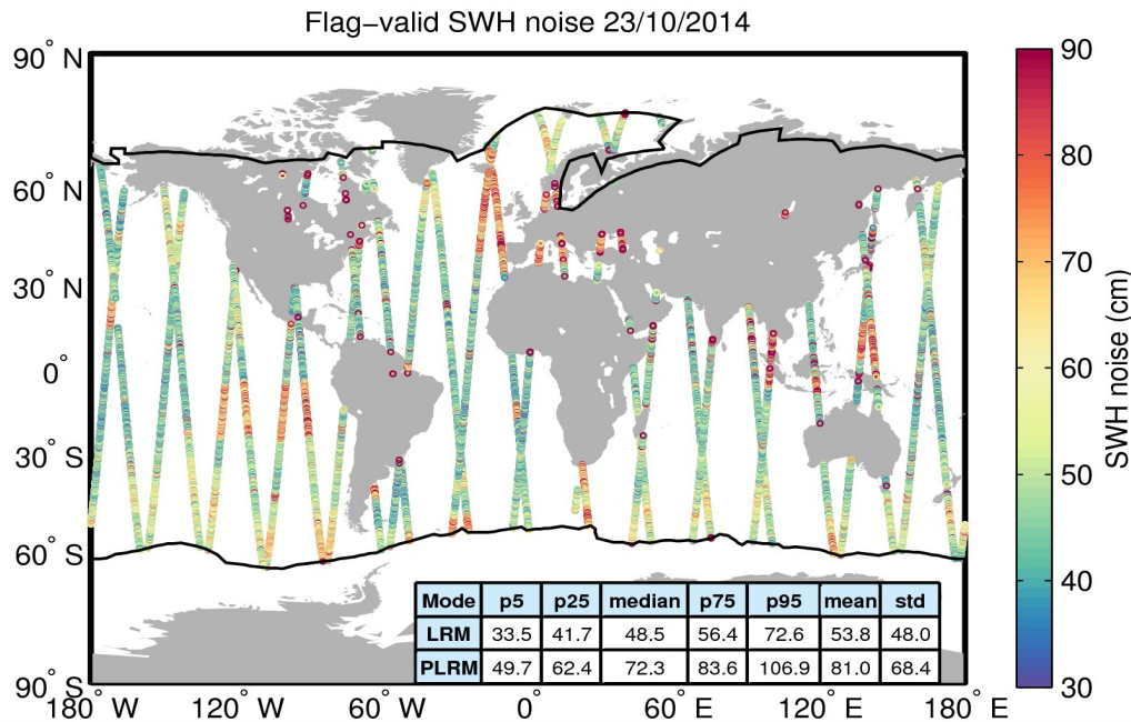
Figure 18. Geographical distribution of flag-valid 20-Hz SWH measurement noise over oceans and lakes for 23/10/2014. The statistical values shown in the table refer to the SWH noise and are calculated separately for LRM and PLRM regions. Measurements taken over polar polygons have been excluded from the computation of the statistical values. The black lines mark the outer limit of the Arctic and Antarctic polar polygons.
