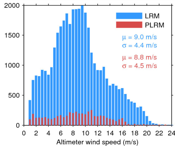
Figure 33. Histogram of flag-valid wind over oceans and lakes for LRM (blue) and PLRM (red) for 23/10/2014. The mean ( \mu ) and standard deviation ( \sigma ) are also shown. Note that values larger than 24 m/s are excluded from the histogram for the sake of readability but not from the computation of \mu and \sigma .
