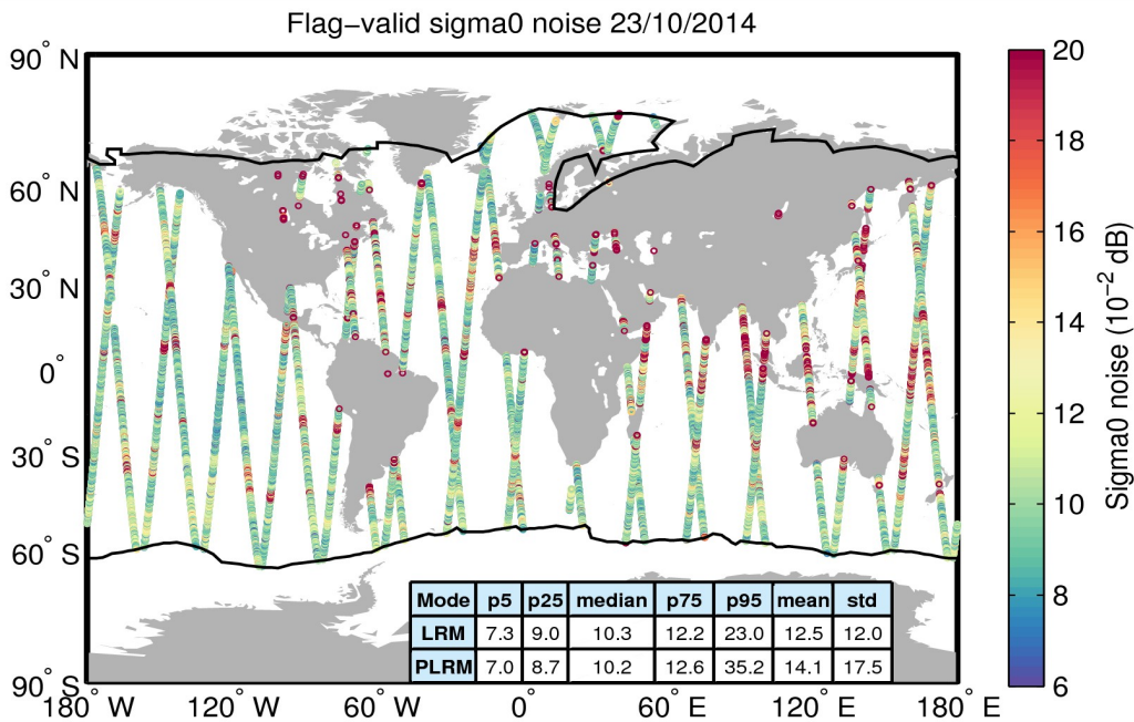
Figure 26. Geographical distribution of flag-valid 20-Hz sigma0 measurement noise over oceans and lakes for 23/10/2014. The statistical values shown in the table refer to the sigma0 noise and are calculated separately for LRM and PLRM regions. Measurements taken over polar polygons have been excluded from the computation of the statistical values. The black lines mark the outer limit of the Arctic and Antarctic polar polygons.
