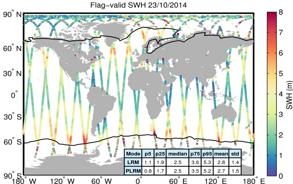
Figure 15. Geographical distribution of flag-valid SWH data over oceans and lakes for 23/10/2014. The statistical values shown in the table refer to the SWH in m and are calculated separately for LRM and PLRM regions. Measurements taken over polar polygons have been excluded from the computation of the statistical values. The black lines mark the outer limit of the Arctic and Antarctic polar polygons.
