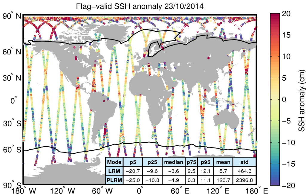
Figure 5. Geographical distribution of flag-valid 1-Hz SSH anomaly data over oceans and lakes for 23/10/2014. The statistical values shown in the table refer to the SSH anomaly in cm and are calculated separately for LRM and PLRM regions. Measurements taken over polar polygons have been excluded from the computation of the statistical values. The black lines mark the outer limit of the Arctic and Antarctic polar polygons.
