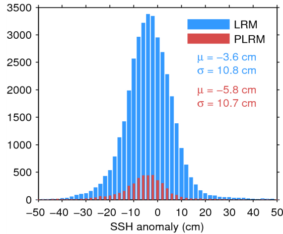
Figure 11. Histogram of science-valid SSH anomaly over oceans and lakes for LRM (blue) and PLRM (red) for 23/10/2014. The mean ( \mu ) and standard deviation ( \sigma ) are also shown. Note that values outside [-50 50] cm are excluded from the histogram for the sake of readability but not from the computation of \mu and \sigma .
