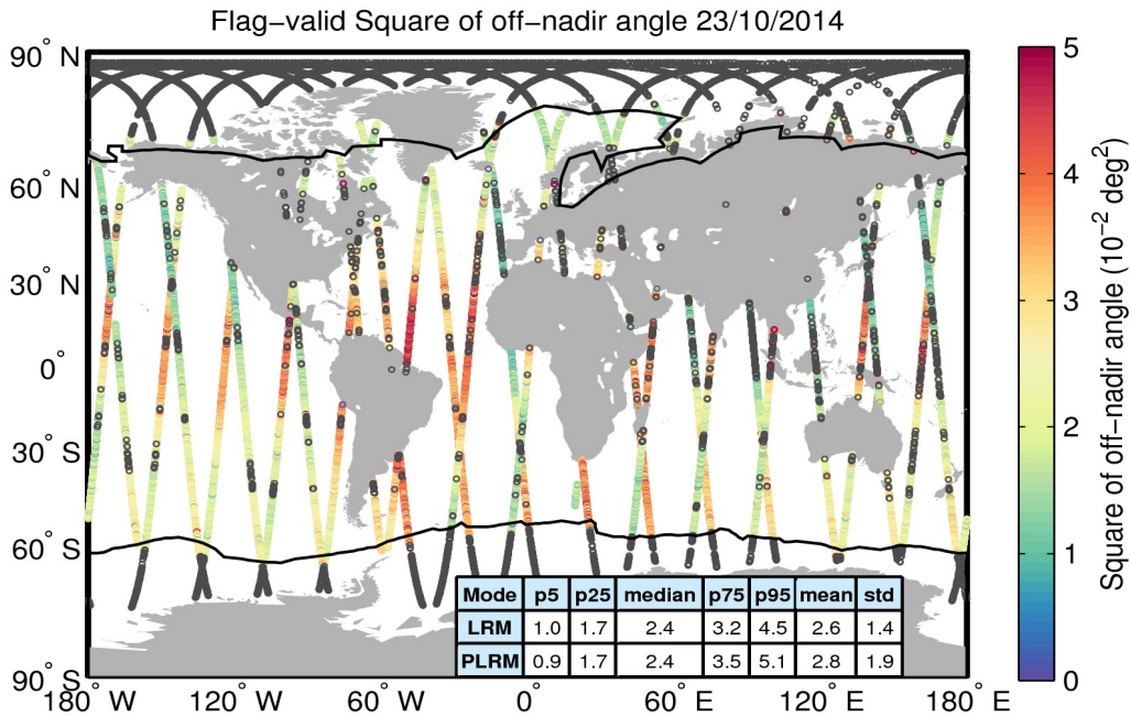
Figure 37. Geographical distribution of flag-valid mispointing data over oceans and lakes for 23/10/2014. The statistical values shown in the table refer to the mispointing in 10^{-2} \text{ deg}^2 and are calculated separately for LRM and PLRM regions. Measurements taken over polar polygons have been excluded from the computation of the statistical values. The black lines mark the outer limit of the Arctic and Antarctic polar polygons. Gray circles denote negative values.
