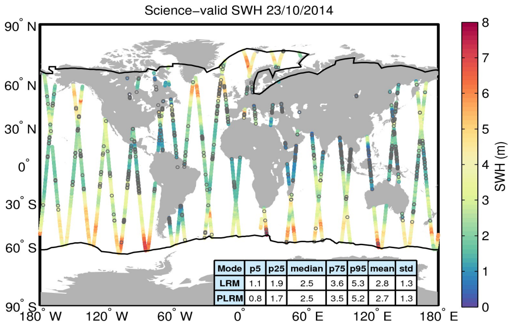
Figure 19. Geographical distribution of science-valid SWH data over oceans and lakes for 23/10/2014. The statistical values shown in the table refer to the SWH in m and are calculated separately for LRM and PLRM regions. The black lines mark the outer limit of the Arctic and Antarctic polar polygons. Gray circles denote records that have been rejected based on the editing criteria described in Table 3.
