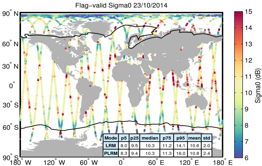
Figure 23. Geographical distribution of flag-valid sigma0 data over oceans and lakes for 23/10/2014. The statistical values shown in the table refer to the sigma0 in dB and are calculated separately for LRM and PLRM regions. Measurements taken over polar polygons have been excluded from the computation of the statistical values. The black lines mark the outer limit of the Arctic and Antarctic polar polygons.
