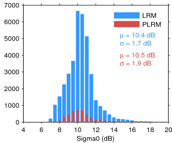
Figure 28. Histogram of science-valid sigma0 over oceans and lakes for LRM (blue) and PLRM (red) for 23/10/2014. The mean ( \mu ) and standard deviation ( \sigma ) are also shown. Note that values outside [4 20] dB are excluded from the histogram for the sake of readability but not from the computation of \mu and \sigma .
