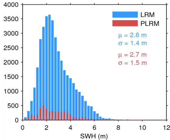
Figure 17. Histogram of flag-valid SWH over oceans and lakes for LRM (blue) and PLRM (red) for 23/10/2014. The mean ( \mu ) and standard deviation ( \sigma ) are also shown. Note that values larger than 12 m are excluded from the histogram for the sake of readability but not from the computation of \mu and \sigma .
