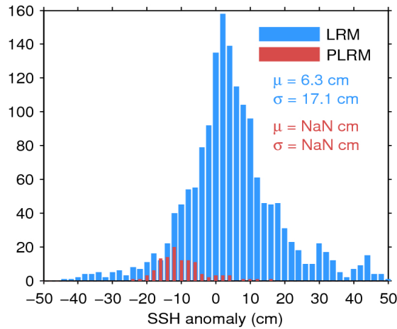
Figure 11. Histogram of science-valid SSH anomaly over oceans and lakes for LRM (blue) and PLRM (red) for 03/10/2014. The mean ( \mu ) and standard deviation ( \sigma ) are also shown. Note that values outside [-50\ 50] cm are excluded from the histogram for the sake of readability but not from the computation of \mu and \sigma .
