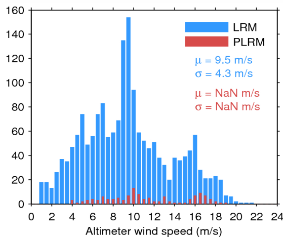
Figure 35. Histogram of science-valid wind over oceans and lakes for LRM (blue) and PLRM (red) for 03/10/2014. The mean ( \mu ) and standard deviation ( \sigma ) are also shown. Note that values larger than 24 m/s are excluded from the histogram for the sake of readability but not from the computation of \mu and \sigma .
