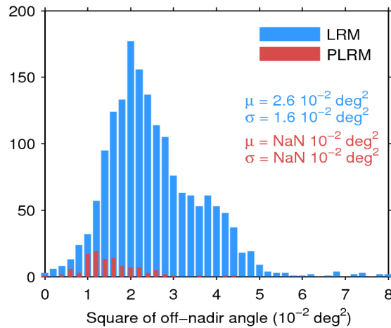
Figure 39. Histogram of flag-valid mispointing over oceans and lakes for LRM (blue) and PLRM (red) for 03/10/2014. Only positive values have been considered. The mean ( \mu ) and standard deviation ( \sigma ) are also shown. Note that values larger than 8 \cdot 10^{-2} \text{ deg}^2 are excluded from the histogram for the sake of readability but not from the computation of \mu and \sigma .
