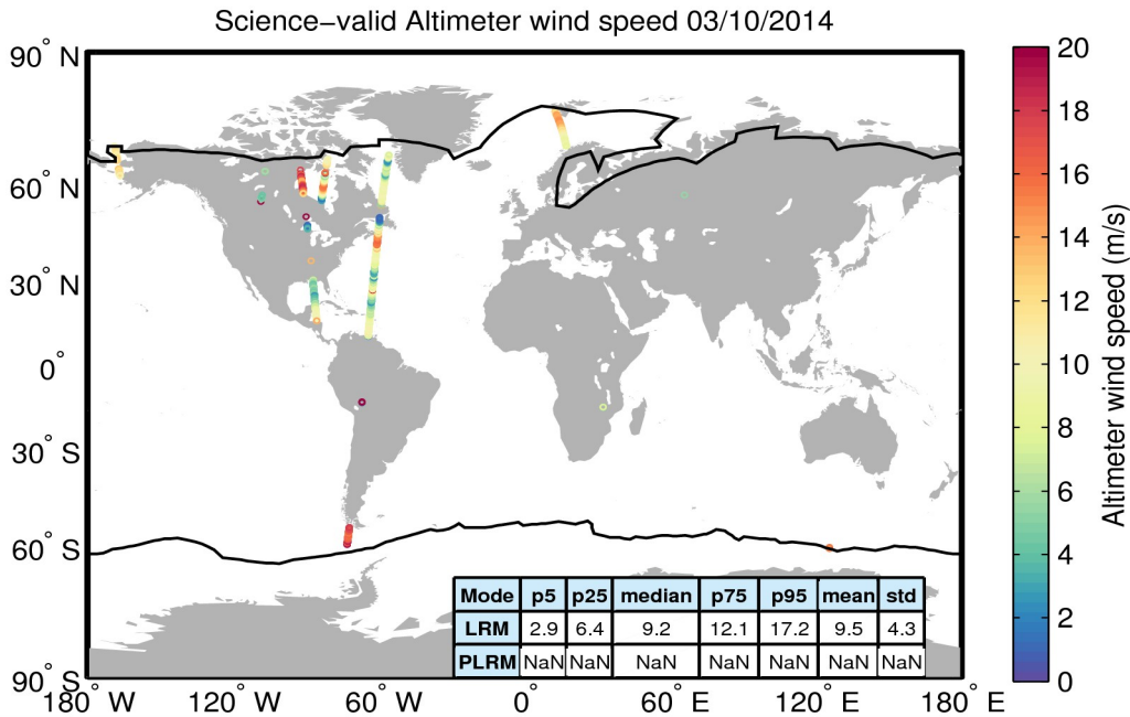
Figure 34. Geographical distribution of science-valid wind data over oceans and lakes for 03/10/2014. The statistical values shown in the table refer to the wind in m/s and are calculated separately for LRM and PLRM regions. The black lines mark the outer limit of the Arctic and Antarctic polar polygons. Gray circles denote records that have been rejected based on the editing criteria described in Table 5.
