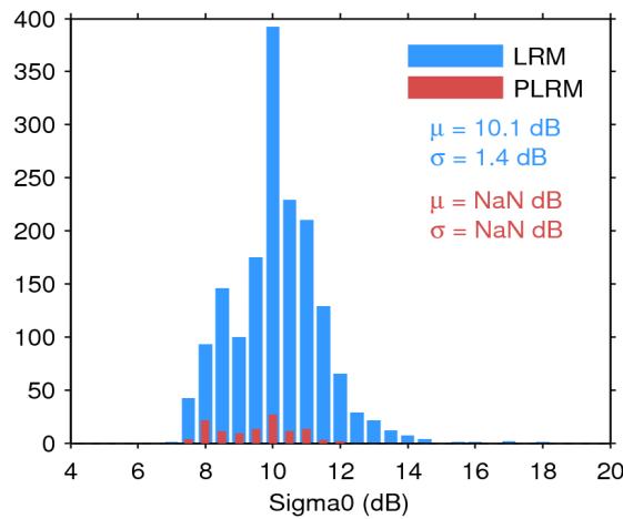
Figure 28. Histogram of science-valid sigma0 over oceans and lakes for LRM (blue) and PLRM (red) for 03/10/2014. The mean ( \mu ) and standard deviation ( \sigma ) are also shown. Note that values outside [4 20] dB are excluded from the histogram for the sake of readability but not from the computation of \mu and \sigma .
