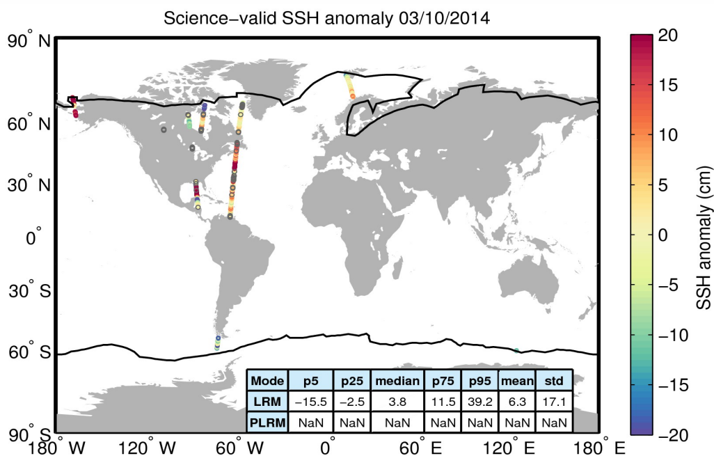
Figure 10. Geographical distribution of science-valid SSH anomaly data over oceans and lakes for 03/10/2014. The statistical values shown in the table refer to the SSH anomaly in cm and are calculated separately for LRM and PLRM regions. The black lines mark the outer limit of the Arctic and Antarctic polar polygons. Gray circles denote records that have been rejected based on the editing criteria described in Table 2.
