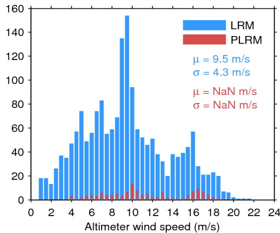
Figure 33. Histogram of flag-valid wind over oceans and lakes for LRM (blue) and PLRM (red) for 03/10/2014. The mean ( \mu ) and standard deviation ( \sigma ) are also shown. Note that values larger than 24 m/s are excluded from the histogram for the sake of readability but not from the computation of \mu and \sigma .
