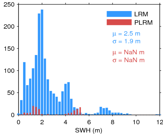
Figure 17. Histogram of flag-valid SWH over oceans and lakes for LRM (blue) and PLRM (red) for 03/10/2014. The mean ( \mu ) and standard deviation ( \sigma ) are also shown. Note that values larger than 12 m are excluded from the histogram for the sake of readability but not from the computation of \mu and \sigma .
