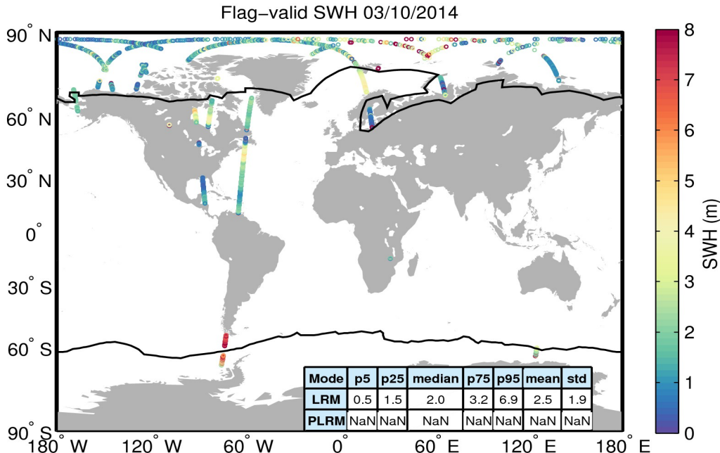
Figure 15. Geographical distribution of flag-valid SWH data over oceans and lakes for 03/10/2014. The statistical values shown in the table refer to the SWH in m and are calculated separately for LRM and PLRM regions. Measurements taken over polar polygons have been excluded from the computation of the statistical values. The black lines mark the outer limit of the Arctic and Antarctic polar polygons.
