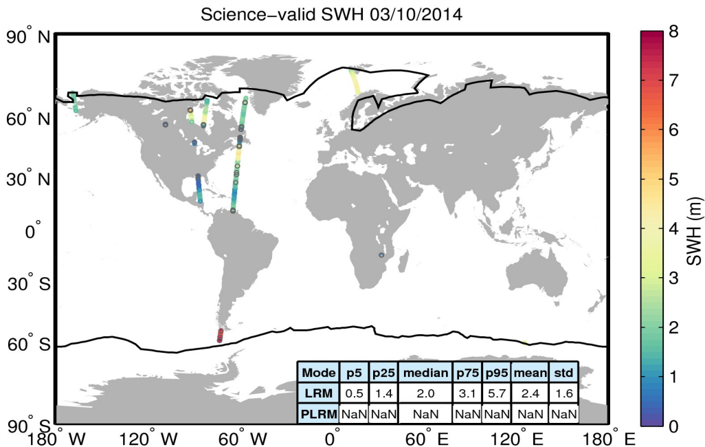
Figure 19. Geographical distribution of science-valid SWH data over oceans and lakes for 03/10/2014. The statistical values shown in the table refer to the SWH in m and are calculated separately for LRM and PLRM regions. The black lines mark the outer limit of the Arctic and Antarctic polar polygons. Gray circles denote records that have been rejected based on the editing criteria described in Table 3.
