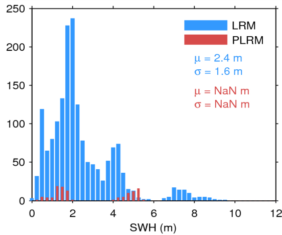
Figure 20. Histogram of science-valid SWH over oceans and lakes for LRM (blue) and PLRM (red) for 03/10/2014. The mean ( \mu ) and standard deviation ( \sigma ) are also shown. Note that values larger than 12 m are excluded from the histogram for the sake of readability but not from the computation of \mu and \sigma .
