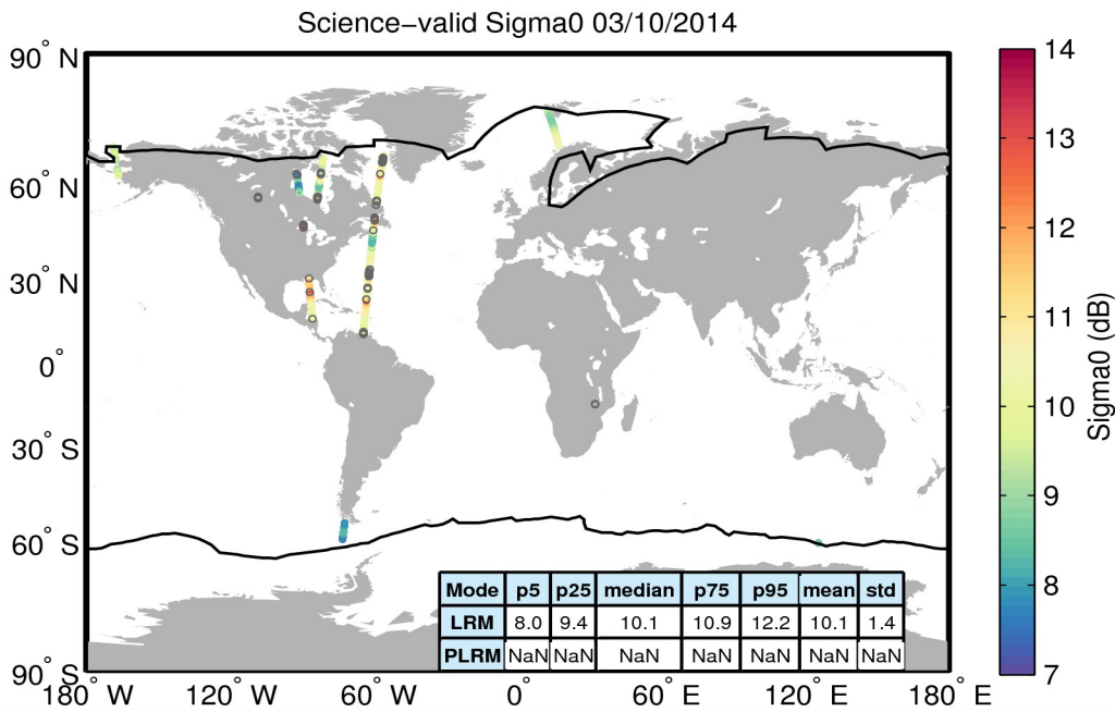
Figure 27. Geographical distribution of science-valid sigma0 data over oceans and lakes for 03/10/2014. The statistical values shown in the table refer to the sigma0 in dB and are calculated separately for LRM and PLRM regions. The black lines mark the outer limit of the Arctic and Antarctic polar polygons. Gray circles denote records that have been rejected based on the editing criteria described in Table 4.
