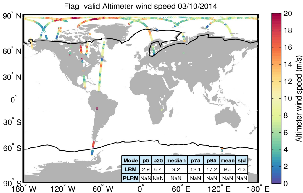
Figure 31. Geographical distribution of flag-valid wind data over oceans and lakes for 03/10/2014. The statistical values shown in the table refer to the wind in m/s and are calculated separately for LRM and PLRM regions. Measurements taken over polar polygons have been excluded from the computation of the statistical values. The black lines mark the outer limit of the Arctic and Antarctic polar polygons.
