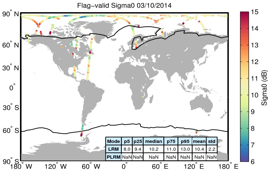
Figure 23. Geographical distribution of flag-valid sigma0 data over oceans and lakes for 03/10/2014. The statistical values shown in the table refer to the sigma0 in dB and are calculated separately for LRM and PLRM regions. Measurements taken over polar polygons have been excluded from the computation of the statistical values. The black lines mark the outer limit of the Arctic and Antarctic polar polygons.
