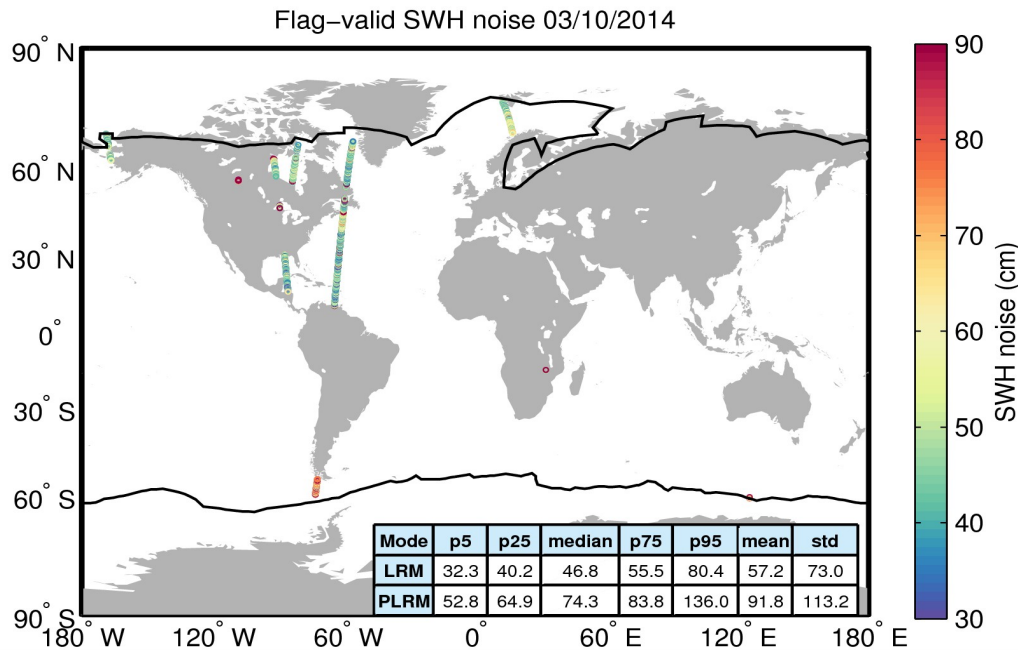
Figure 18. Geographical distribution of flag-valid 20-Hz SWH measurement noise over oceans and lakes for 03/10/2014. The statistical values shown in the table refer to the SWH noise and are calculated separately for LRM and PLRM regions. Measurements taken over polar polygons have been excluded from the computation of the statistical values. The black lines mark the outer limit of the Arctic and Antarctic polar polygons.
