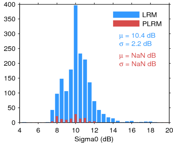
Figure 25. Histogram of flag-valid sigma0 over oceans and lakes for LRM (blue) and PLRM (red) for 03/10/2014. The mean ( \mu ) and standard deviation ( \sigma ) are also shown. Note that values outside [4 20] dB are excluded from the histogram for the sake of readability but not from the computation of \mu and \sigma .
