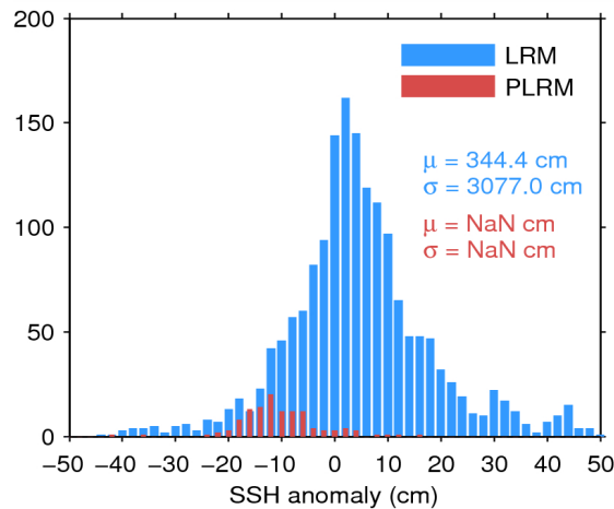
Figure 7. Histogram of flag-valid SSH anomaly over oceans and lakes for LRM (blue) and PLRM (red) for 03/10/2014. The mean ( \mu ) and standard deviation ( \sigma ) are also shown. Note that values outside [-50\ 50] cm are excluded from the histogram for the sake of readability but not from the computation of \mu and \sigma .
