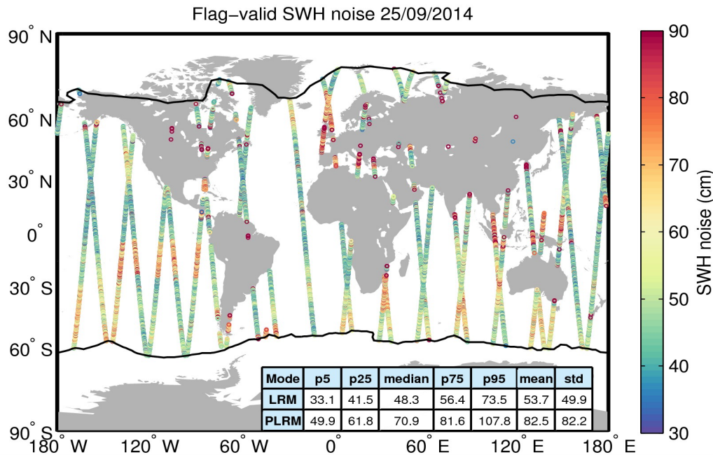
Figure 18. Geographical distribution of flag-valid 20-Hz SWH measurement noise over oceans and lakes for 25/09/2014. The statistical values shown in the table refer to the SWH noise and are calculated separately for LRM and PLRM regions. Measurements taken over polar polygons have been excluded from the computation of the statistical values. The black lines mark the outer limit of the Arctic and Antarctic polar polygons.
