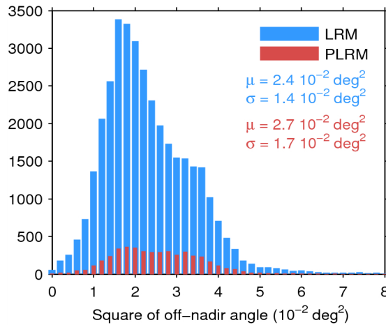
Figure 39. Histogram of flag-valid mispointing over oceans and lakes for LRM (blue) and PLRM (red) for 25/09/2014. Only positive values have been considered. The mean ( \mu ) and standard deviation ( \sigma ) are also shown. Note that values larger than 8 \cdot 10^{-2} \text{ deg}^2 are excluded from the histogram for the sake of readability but not from the computation of \mu and \sigma .
