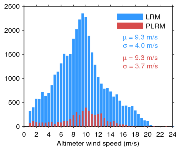
Figure 35. Histogram of science-valid wind over oceans and lakes for LRM (blue) and PLRM (red) for 25/09/2014. The mean ( \mu ) and standard deviation ( \sigma ) are also shown. Note that values larger than 24 m/s are excluded from the histogram for the sake of readability but not from the computation of \mu and \sigma .
