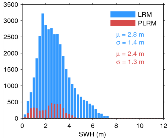
Figure 17. Histogram of flag-valid SWH over oceans and lakes for LRM (blue) and PLRM (red) for 25/09/2014. The mean ( \mu ) and standard deviation ( \sigma ) are also shown. Note that values larger than 12 m are excluded from the histogram for the sake of readability but not from the computation of \mu and \sigma .
