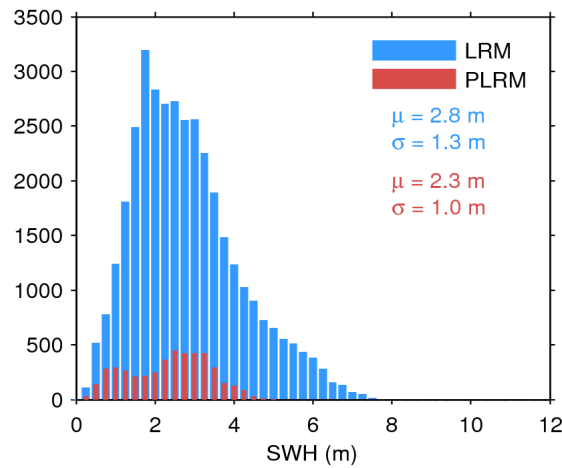
Figure 20. Histogram of science-valid SWH over oceans and lakes for LRM (blue) and PLRM (red) for 25/09/2014. The mean ( \mu ) and standard deviation ( \sigma ) are also shown. Note that values larger than 12 m are excluded from the histogram for the sake of readability but not from the computation of \mu and \sigma .
