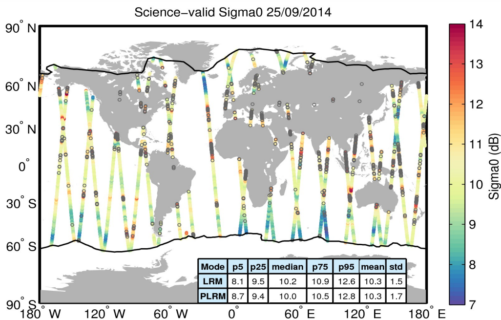
Figure 27. Geographical distribution of science-valid sigma0 data over oceans and lakes for 25/09/2014. The statistical values shown in the table refer to the sigma0 in dB and are calculated separately for LRM and PLRM regions. The black lines mark the outer limit of the Arctic and Antarctic polar polygons. Gray circles denote records that have been rejected based on the editing criteria described in Table 4.
