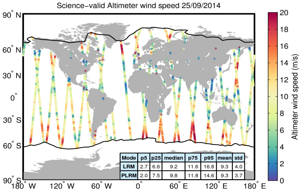
Figure 34. Geographical distribution of science-valid wind data over oceans and lakes for 25/09/2014. The statistical values shown in the table refer to the wind in m/s and are calculated separately for LRM and PLRM regions. The black lines mark the outer limit of the Arctic and Antarctic polar polygons. Gray circles denote records that have been rejected based on the editing criteria described in Table 5.
