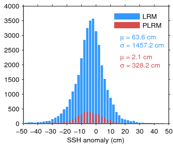
Figure 7. Histogram of flag-valid SSH anomaly over oceans and lakes for LRM (blue) and PLRM (red) for 25/09/2014. The mean ( \mu ) and standard deviation ( \sigma ) are also shown. Note that values outside [-50\ 50] cm are excluded from the histogram for the sake of readability but not from the computation of \mu and \sigma .
