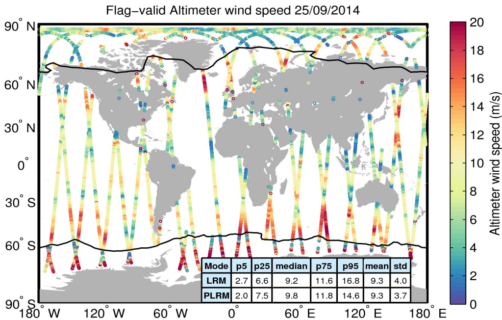
Figure 31. Geographical distribution of flag-valid wind data over oceans and lakes for 25/09/2014. The statistical values shown in the table refer to the wind in m/s and are calculated separately for LRM and PLRM regions. Measurements taken over polar polygons have been excluded from the computation of the statistical values. The black lines mark the outer limit of the Arctic and Antarctic polar polygons.
