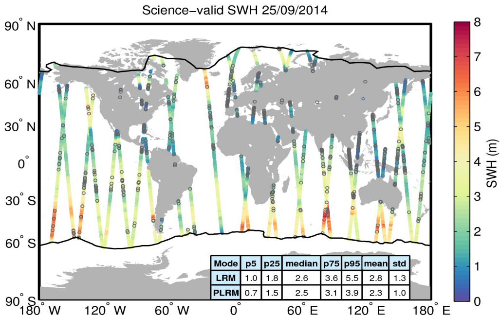
Figure 19. Geographical distribution of science-valid SWH data over oceans and lakes for 25/09/2014. The statistical values shown in the table refer to the SWH in m and are calculated separately for LRM and PLRM regions. The black lines mark the outer limit of the Arctic and Antarctic polar polygons. Gray circles denote records that have been rejected based on the editing criteria described in Table 3.
