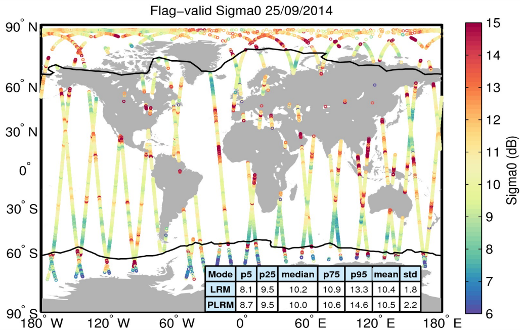
Figure 23. Geographical distribution of flag-valid sigma0 data over oceans and lakes for 25/09/2014. The statistical values shown in the table refer to the sigma0 in dB and are calculated separately for LRM and PLRM regions. Measurements taken over polar polygons have been excluded from the computation of the statistical values. The black lines mark the outer limit of the Arctic and Antarctic polar polygons.
