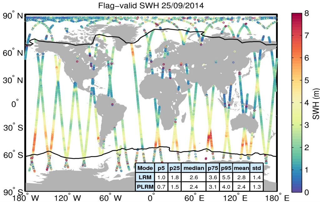
Figure 15. Geographical distribution of flag-valid SWH data over oceans and lakes for 25/09/2014. The statistical values shown in the table refer to the SWH in m and are calculated separately for LRM and PLRM regions. Measurements taken over polar polygons have been excluded from the computation of the statistical values. The black lines mark the outer limit of the Arctic and Antarctic polar polygons.
