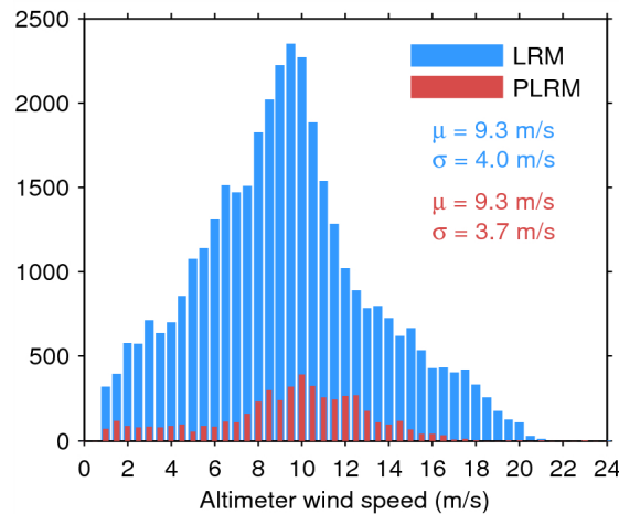
Figure 33. Histogram of flag-valid wind over oceans and lakes for LRM (blue) and PLRM (red) for 25/09/2014. The mean ( \mu ) and standard deviation ( \sigma ) are also shown. Note that values larger than 24 m/s are excluded from the histogram for the sake of readability but not from the computation of \mu and \sigma .
