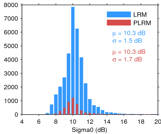
Figure 28. Histogram of science-valid sigma0 over oceans and lakes for LRM (blue) and PLRM (red) for 25/09/2014. The mean ( \mu ) and standard deviation ( \sigma ) are also shown. Note that values outside [4 20] dB are excluded from the histogram for the sake of readability but not from the computation of \mu and \sigma .
