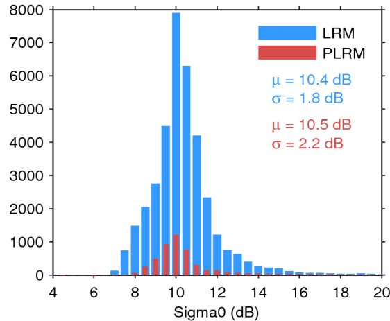
Figure 25. Histogram of flag-valid sigma0 over oceans and lakes for LRM (blue) and PLRM (red) for 25/09/2014. The mean ( \mu ) and standard deviation ( \sigma ) are also shown. Note that values outside [4 20] dB are excluded from the histogram for the sake of readability but not from the computation of \mu and \sigma .
