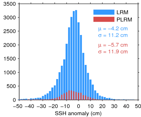
Figure 11. Histogram of science-valid SSH anomaly over oceans and lakes for LRM (blue) and PLRM (red) for 25/09/2014. The mean ( \mu ) and standard deviation ( \sigma ) are also shown. Note that values outside [-50\ 50] cm are excluded from the histogram for the sake of readability but not from the computation of \mu and \sigma .
