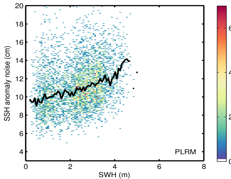
Figure 9. 2D histogram showing flag-valid SSH anomaly noise as a function of SWH for LRM (top) and PLRM (bottom) for 25/09/2014. The black line denotes the median SSH anomaly as a function of SWH.
