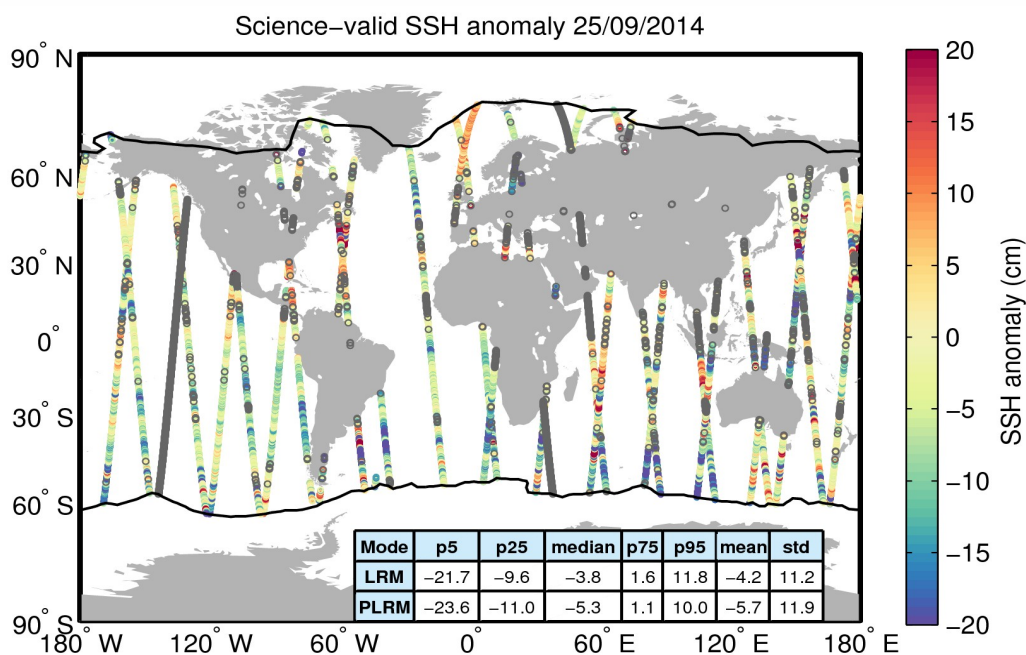
Figure 10. Geographical distribution of science-valid SSH anomaly data over oceans and lakes for 25/09/2014. The statistical values shown in the table refer to the SSH anomaly in cm and are calculated separately for LRM and PLRM regions. The black lines mark the outer limit of the Arctic and Antarctic polar polygons. Gray circles denote records that have been rejected based on the editing criteria described in Table 2.
