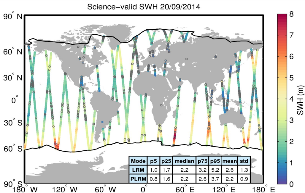
Figure 19. Geographical distribution of science-valid SWH data over oceans and lakes for 20/09/2014. The statistical values shown in the table refer to the SWH in m and are calculated separately for LRM and PLRM regions. The black lines mark the outer limit of the Arctic and Antarctic polar polygons. Gray circles denote records that have been rejected based on the editing criteria described in Table 3.
