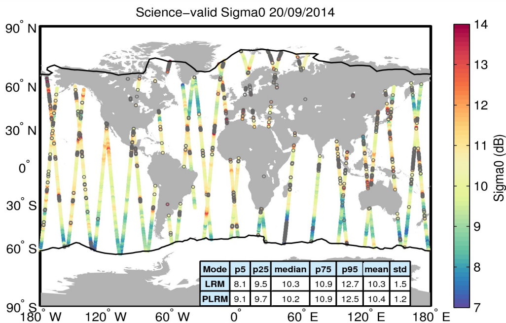
Figure 27. Geographical distribution of science-valid sigma0 data over oceans and lakes for 20/09/2014. The statistical values shown in the table refer to the sigma0 in dB and are calculated separately for LRM and PLRM regions. The black lines mark the outer limit of the Arctic and Antarctic polar polygons. Gray circles denote records that have been rejected based on the editing criteria described in Table 4.
