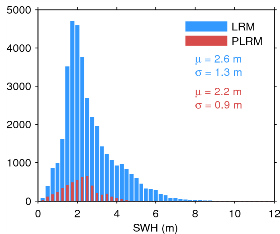
Figure 20. Histogram of science-valid SWH over oceans and lakes for LRM (blue) and PLRM (red) for 20/09/2014. The mean ( \mu ) and standard deviation ( \sigma ) are also shown. Note that values larger than 12 m are excluded from the histogram for the sake of readability but not from the computation of \mu and \sigma .
