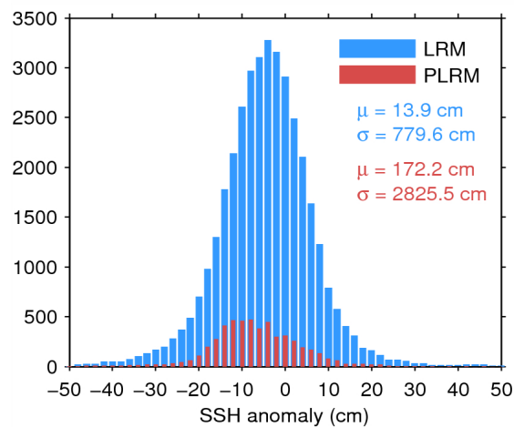
Figure 7. Histogram of flag-valid SSH anomaly over oceans and lakes for LRM (blue) and PLRM (red) for 20/09/2014. The mean ( \mu ) and standard deviation ( \sigma ) are also shown. Note that values outside [-50\ 50] cm are excluded from the histogram for the sake of readability but not from the computation of \mu and \sigma .
