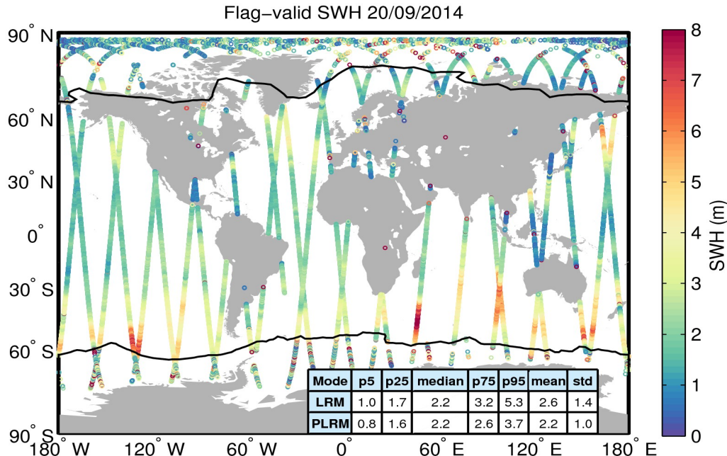
Figure 15. Geographical distribution of flag-valid SWH data over oceans and lakes for 20/09/2014. The statistical values shown in the table refer to the SWH in m and are calculated separately for LRM and PLRM regions. Measurements taken over polar polygons have been excluded from the computation of the statistical values. The black lines mark the outer limit of the Arctic and Antarctic polar polygons.
