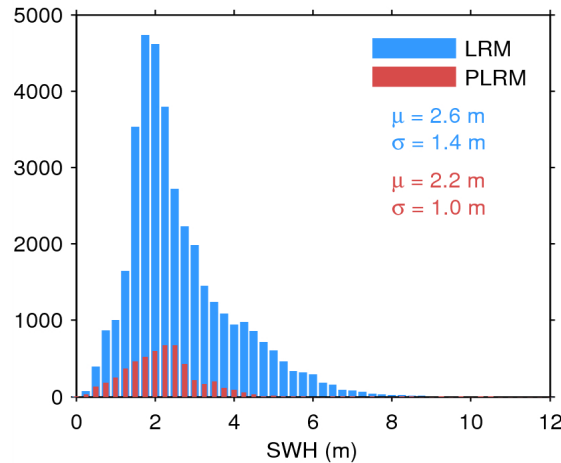
Figure 17. Histogram of flag-valid SWH over oceans and lakes for LRM (blue) and PLRM (red) for 20/09/2014. The mean ( \mu ) and standard deviation ( \sigma ) are also shown. Note that values larger than 12 m are excluded from the histogram for the sake of readability but not from the computation of \mu and \sigma .
