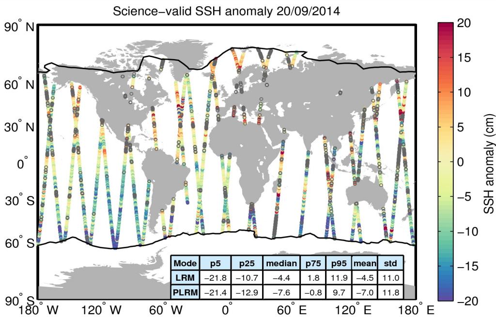
Figure 10. Geographical distribution of science-valid SSH anomaly data over oceans and lakes for 20/09/2014. The statistical values shown in the table refer to the SSH anomaly in cm and are calculated separately for LRM and PLRM regions. The black lines mark the outer limit of the Arctic and Antarctic polar polygons. Gray circles denote records that have been rejected based on the editing criteria described in Table 2.
