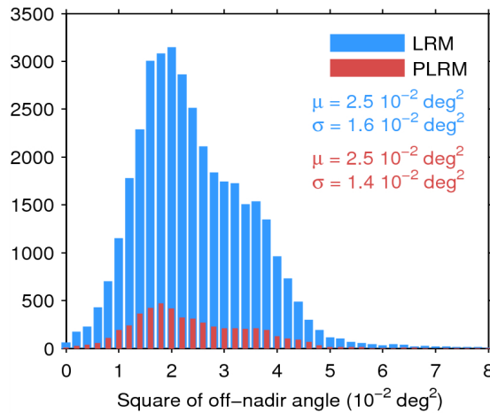
Figure 39. Histogram of flag-valid mispointing over oceans and lakes for LRM (blue) and PLRM (red) for 20/09/2014. Only positive values have been considered. The mean ( \mu ) and standard deviation ( \sigma ) are also shown. Note that values larger than 8 \cdot 10^{-2} \text{ deg}^2 are excluded from the histogram for the sake of readability but not from the computation of \mu and \sigma .
