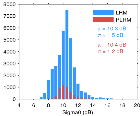
Figure 28. Histogram of science-valid sigma0 over oceans and lakes for LRM (blue) and PLRM (red) for 20/09/2014. The mean ( \mu ) and standard deviation ( \sigma ) are also shown. Note that values outside [4 20] dB are excluded from the histogram for the sake of readability but not from the computation of \mu and \sigma .
