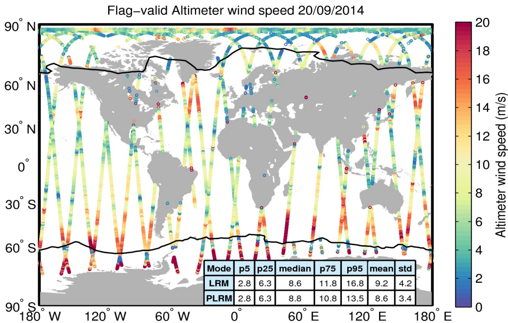
Figure 31. Geographical distribution of flag-valid wind data over oceans and lakes for 20/09/2014. The statistical values shown in the table refer to the wind in m/s and are calculated separately for LRM and PLRM regions. Measurements taken over polar polygons have been excluded from the computation of the statistical values. The black lines mark the outer limit of the Arctic and Antarctic polar polygons.
