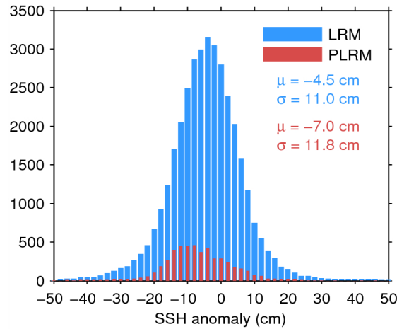
Figure 11. Histogram of science-valid SSH anomaly over oceans and lakes for LRM (blue) and PLRM (red) for 20/09/2014. The mean ( \mu ) and standard deviation ( \sigma ) are also shown. Note that values outside [-50\ 50] cm are excluded from the histogram for the sake of readability but not from the computation of \mu and \sigma .
