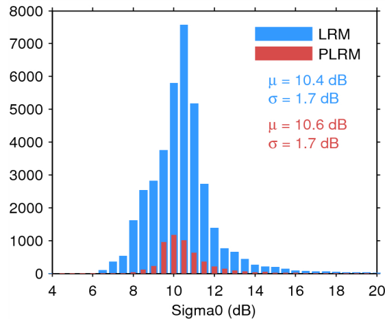
Figure 25. Histogram of flag-valid sigma0 over oceans and lakes for LRM (blue) and PLRM (red) for 20/09/2014. The mean ( \mu ) and standard deviation ( \sigma ) are also shown. Note that values outside [4 20] dB are excluded from the histogram for the sake of readability but not from the computation of \mu and \sigma .
