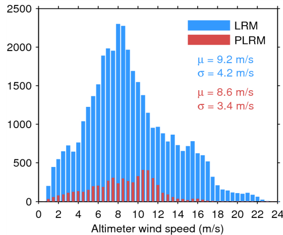
Figure 33. Histogram of flag-valid wind over oceans and lakes for LRM (blue) and PLRM (red) for 20/09/2014. The mean ( \mu ) and standard deviation ( \sigma ) are also shown. Note that values larger than 24 m/s are excluded from the histogram for the sake of readability but not from the computation of \mu and \sigma .
