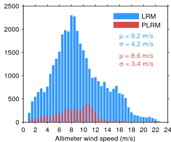
Figure 35. Histogram of science-valid wind over oceans and lakes for LRM (blue) and PLRM (red) for 20/09/2014. The mean ( \mu ) and standard deviation ( \sigma ) are also shown. Note that values larger than 24 m/s are excluded from the histogram for the sake of readability but not from the computation of \mu and \sigma .
