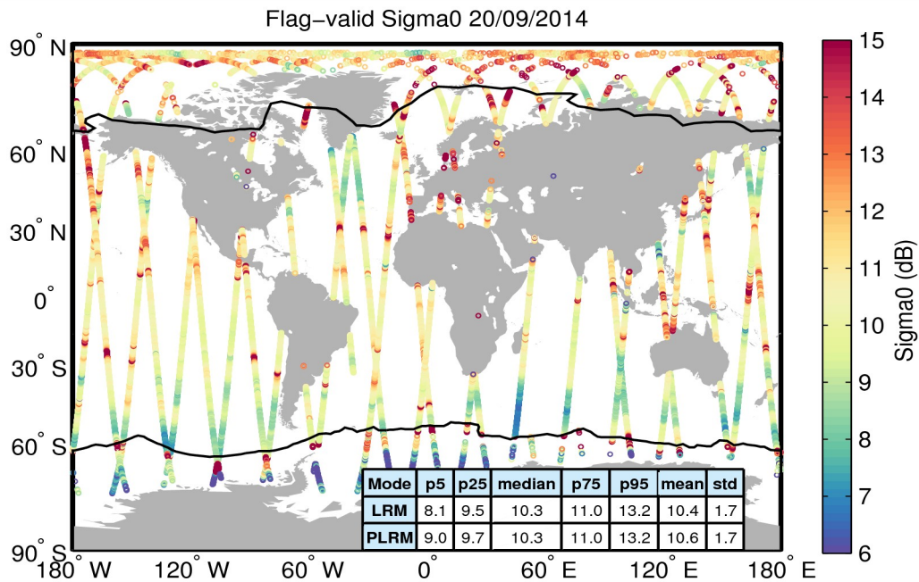
Figure 23. Geographical distribution of flag-valid sigma0 data over oceans and lakes for 20/09/2014. The statistical values shown in the table refer to the sigma0 in dB and are calculated separately for LRM and PLRM regions. Measurements taken over polar polygons have been excluded from the computation of the statistical values. The black lines mark the outer limit of the Arctic and Antarctic polar polygons.
