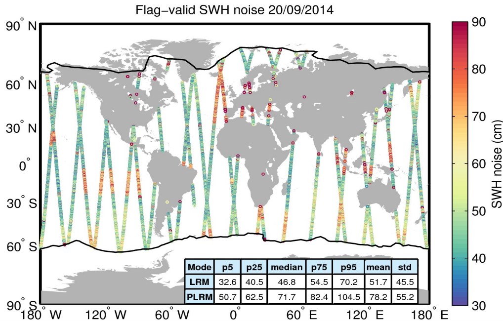
Figure 18. Geographical distribution of flag-valid 20-Hz SWH measurement noise over oceans and lakes for 20/09/2014. The statistical values shown in the table refer to the SWH noise and are calculated separately for LRM and PLRM regions. Measurements taken over polar polygons have been excluded from the computation of the statistical values. The black lines mark the outer limit of the Arctic and Antarctic polar polygons.
