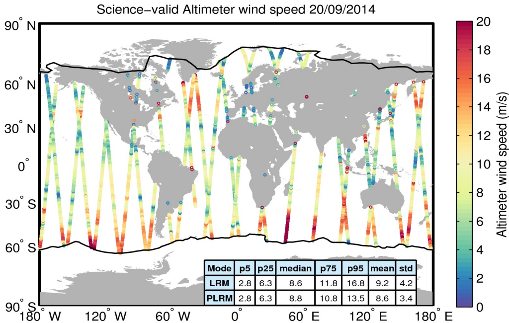
Figure 34. Geographical distribution of science-valid wind data over oceans and lakes for 20/09/2014. The statistical values shown in the table refer to the wind in m/s and are calculated separately for LRM and PLRM regions. The black lines mark the outer limit of the Arctic and Antarctic polar polygons. Gray circles denote records that have been rejected based on the editing criteria described in Table 5.
