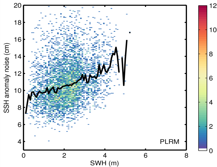
Figure 9. 2D histogram showing flag-valid SSH anomaly noise as a function of SWH for LRM (top) and PLRM (bottom) for 20/09/2014. The black line denotes the median SSH anomaly as a function of SWH.
