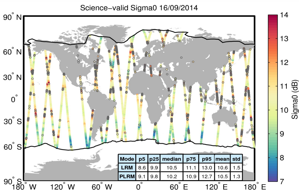
Figure 27. Geographical distribution of science-valid sigma0 data over oceans and lakes for 16/09/2014. The statistical values shown in the table refer to the sigma0 in dB and are calculated separately for LRM and PLRM regions. The black lines mark the outer limit of the Arctic and Antarctic polar polygons. Gray circles denote records that have been rejected based on the editing criteria described in Table 4.
