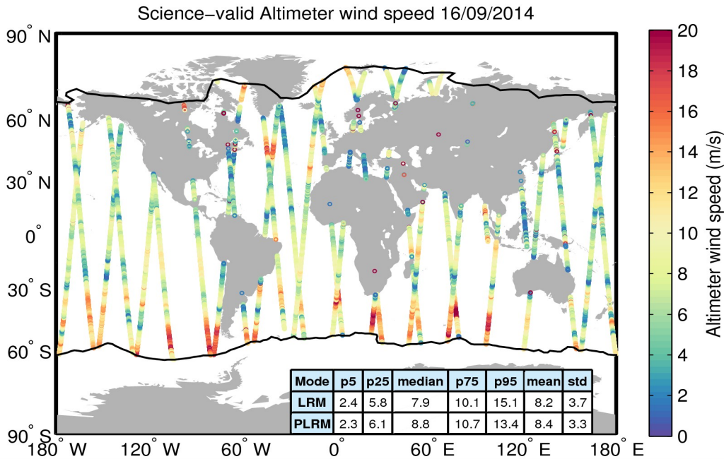
Figure 34. Geographical distribution of science-valid wind data over oceans and lakes for 16/09/2014. The statistical values shown in the table refer to the wind in m/s and are calculated separately for LRM and PLRM regions. The black lines mark the outer limit of the Arctic and Antarctic polar polygons. Gray circles denote records that have been rejected based on the editing criteria described in Table 5.
