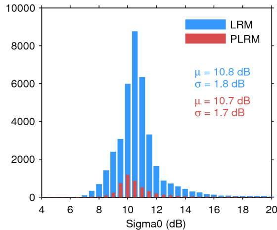
Figure 25. Histogram of flag-valid sigma0 over oceans and lakes for LRM (blue) and PLRM (red) for 16/09/2014. The mean ( \mu ) and standard deviation ( \sigma ) are also shown. Note that values outside [4 20] dB are excluded from the histogram for the sake of readability but not from the computation of \mu and \sigma .
