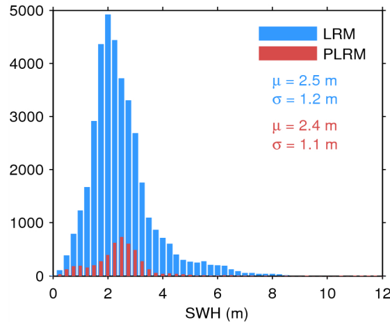
Figure 17. Histogram of flag-valid SWH over oceans and lakes for LRM (blue) and PLRM (red) for 16/09/2014. The mean ( \mu ) and standard deviation ( \sigma ) are also shown. Note that values larger than 12 m are excluded from the histogram for the sake of readability but not from the computation of \mu and \sigma .
