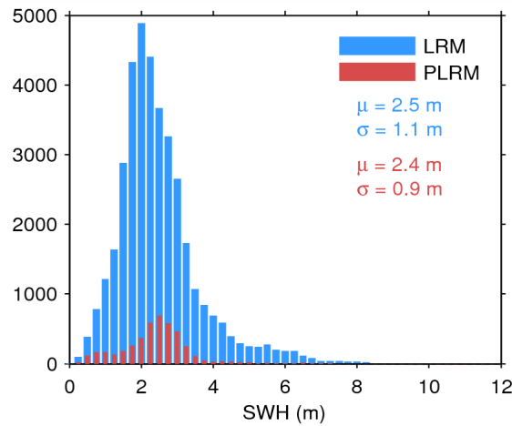
Figure 20. Histogram of science-valid SWH over oceans and lakes for LRM (blue) and PLRM (red) for 16/09/2014. The mean ( \mu ) and standard deviation ( \sigma ) are also shown. Note that values larger than 12 m are excluded from the histogram for the sake of readability but not from the computation of \mu and \sigma .
