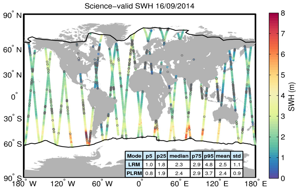
Figure 19. Geographical distribution of science-valid SWH data over oceans and lakes for 16/09/2014. The statistical values shown in the table refer to the SWH in m and are calculated separately for LRM and PLRM regions. The black lines mark the outer limit of the Arctic and Antarctic polar polygons. Gray circles denote records that have been rejected based on the editing criteria described in Table 3.
