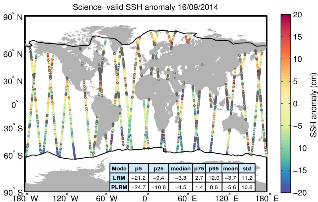
Figure 10. Geographical distribution of science-valid SSH anomaly data over oceans and lakes for 16/09/2014. The statistical values shown in the table refer to the SSH anomaly in cm and are calculated separately for LRM and PLRM regions. The black lines mark the outer limit of the Arctic and Antarctic polar polygons. Gray circles denote records that have been rejected based on the editing criteria described in Table 2.
