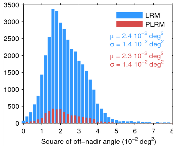
Figure 39. Histogram of flag-valid mispointing over oceans and lakes for LRM (blue) and PLRM (red) for 16/09/2014. Only positive values have been considered. The mean ( \mu ) and standard deviation ( \sigma ) are also shown. Note that values larger than 8 \cdot 10^{-2} \text{ deg}^2 are excluded from the histogram for the sake of readability but not from the computation of \mu and \sigma .
