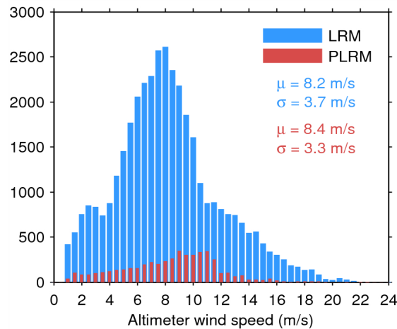
Figure 33. Histogram of flag-valid wind over oceans and lakes for LRM (blue) and PLRM (red) for 16/09/2014. The mean ( \mu ) and standard deviation ( \sigma ) are also shown. Note that values larger than 24 m/s are excluded from the histogram for the sake of readability but not from the computation of \mu and \sigma .
