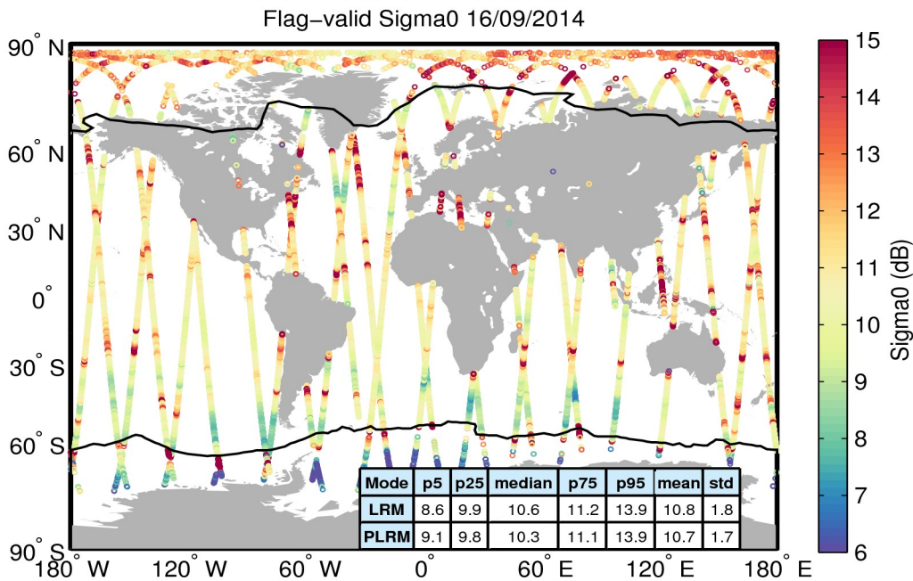
Figure 23. Geographical distribution of flag-valid sigma0 data over oceans and lakes for 16/09/2014. The statistical values shown in the table refer to the sigma0 in dB and are calculated separately for LRM and PLRM regions. Measurements taken over polar polygons have been excluded from the computation of the statistical values. The black lines mark the outer limit of the Arctic and Antarctic polar polygons.
