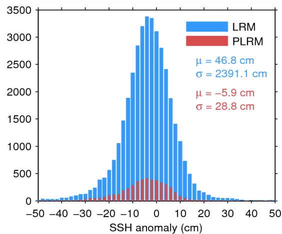
Figure 7. Histogram of flag-valid SSH anomaly over oceans and lakes for LRM (blue) and PLRM (red) for 16/09/2014. The mean ( \mu ) and standard deviation ( \sigma ) are also shown. Note that values outside [-50\ 50] cm are excluded from the histogram for the sake of readability but not from the computation of \mu and \sigma .
