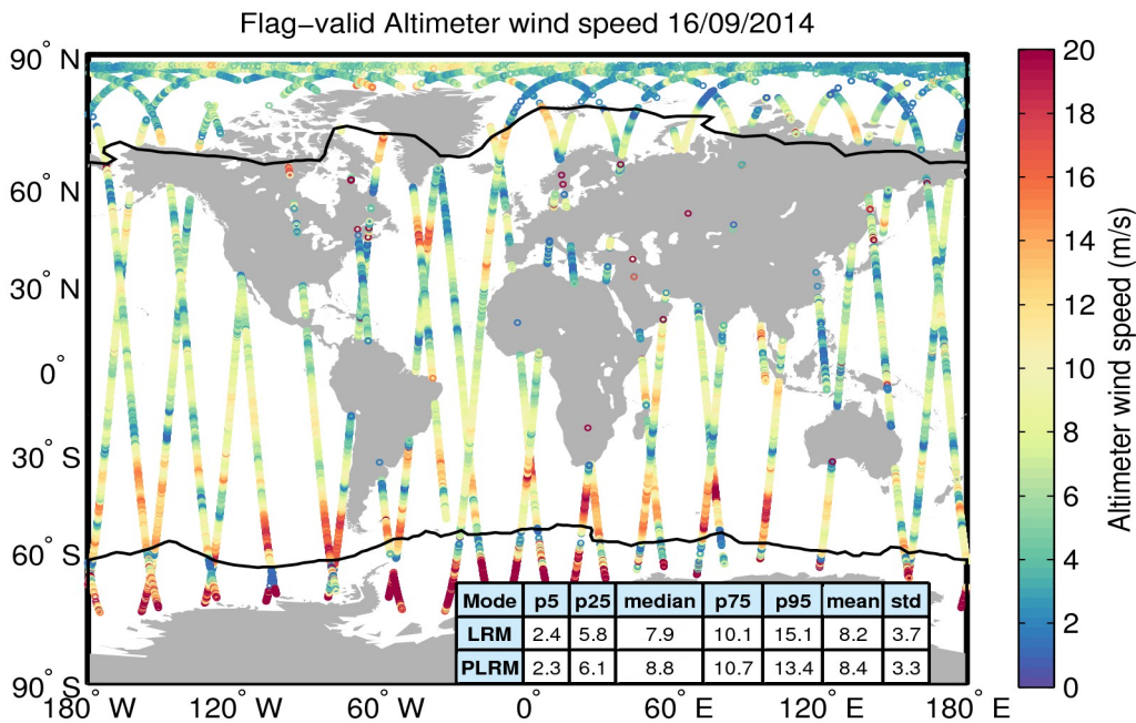
Figure 31. Geographical distribution of flag-valid wind data over oceans and lakes for 16/09/2014. The statistical values shown in the table refer to the wind in m/s and are calculated separately for LRM and PLRM regions. Measurements taken over polar polygons have been excluded from the computation of the statistical values. The black lines mark the outer limit of the Arctic and Antarctic polar polygons.
