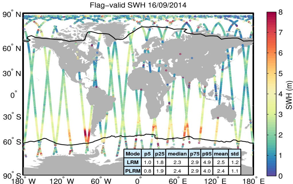
Figure 15. Geographical distribution of flag-valid SWH data over oceans and lakes for 16/09/2014. The statistical values shown in the table refer to the SWH in m and are calculated separately for LRM and PLRM regions. Measurements taken over polar polygons have been excluded from the computation of the statistical values. The black lines mark the outer limit of the Arctic and Antarctic polar polygons.
