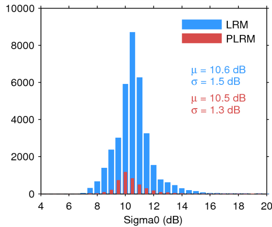
Figure 28. Histogram of science-valid sigma0 over oceans and lakes for LRM (blue) and PLRM (red) for 16/09/2014. The mean ( \mu ) and standard deviation ( \sigma ) are also shown. Note that values outside [4 20] dB are excluded from the histogram for the sake of readability but not from the computation of \mu and \sigma .
