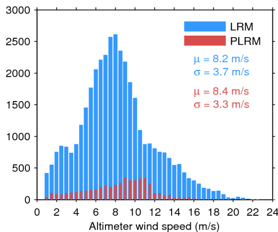
Figure 35. Histogram of science-valid wind over oceans and lakes for LRM (blue) and PLRM (red) for 16/09/2014. The mean ( \mu ) and standard deviation ( \sigma ) are also shown. Note that values larger than 24 m/s are excluded from the histogram for the sake of readability but not from the computation of \mu and \sigma .
