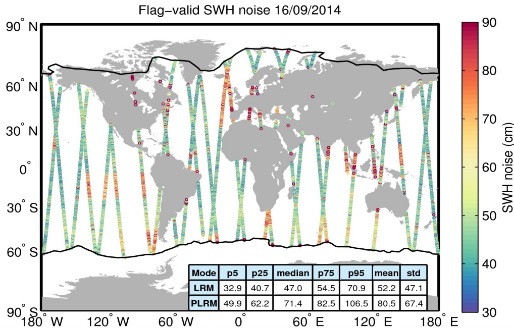
Figure 18. Geographical distribution of flag-valid 20-Hz SWH measurement noise over oceans and lakes for 16/09/2014. The statistical values shown in the table refer to the SWH noise and are calculated separately for LRM and PLRM regions. Measurements taken over polar polygons have been excluded from the computation of the statistical values. The black lines mark the outer limit of the Arctic and Antarctic polar polygons.
