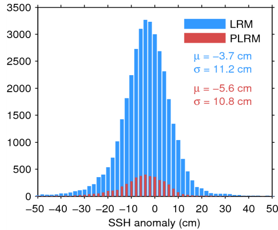
Figure 11. Histogram of science-valid SSH anomaly over oceans and lakes for LRM (blue) and PLRM (red) for 16/09/2014. The mean ( \mu ) and standard deviation ( \sigma ) are also shown. Note that values outside [-50\ 50] cm are excluded from the histogram for the sake of readability but not from the computation of \mu and \sigma .
