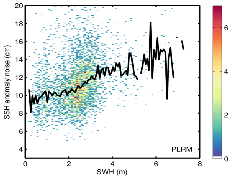
Figure 9. 2D histogram showing flag-valid SSH anomaly noise as a function of SWH for LRM (top) and PLRM (bottom) for 16/09/2014. The black line denotes the median SSH anomaly as a function of SWH.
