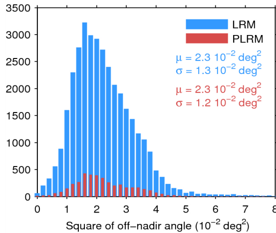
Figure 39. Histogram of flag-valid mispointing over oceans and lakes for LRM (blue) and PLRM (red) for 15/09/2014. Only positive values have been considered. The mean ( \mu ) and standard deviation ( \sigma ) are also shown. Note that values larger than 8 \cdot 10^{-2} \text{ deg}^2 are excluded from the histogram for the sake of readability but not from the computation of \mu and \sigma .
