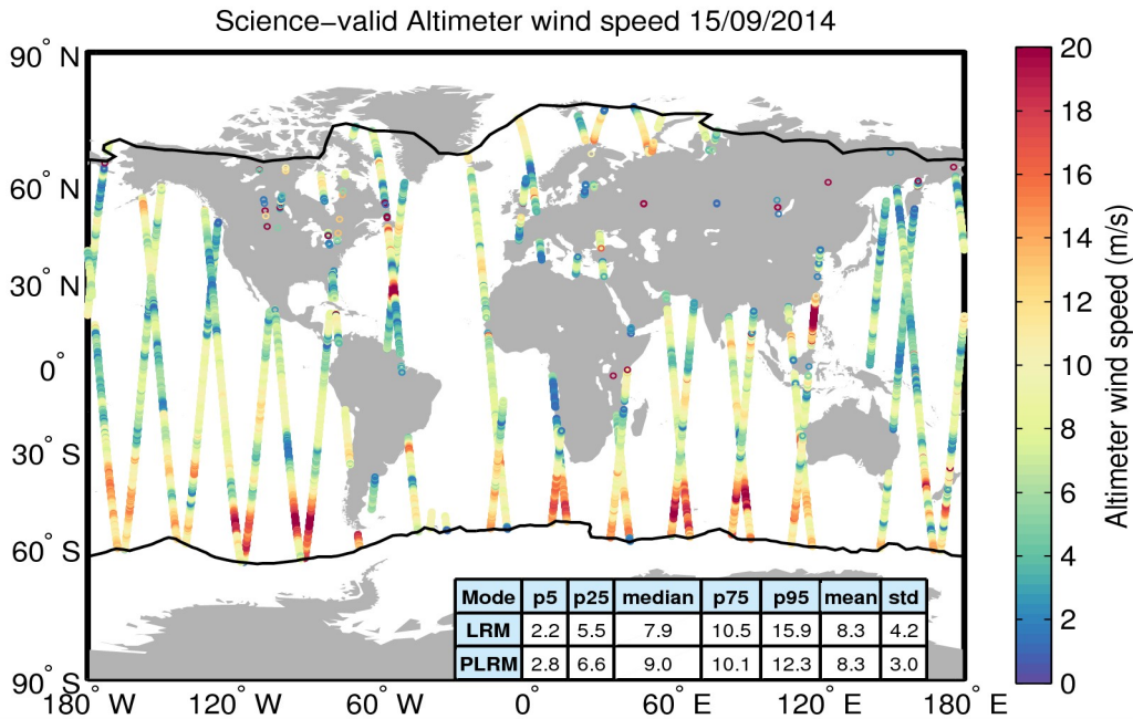
Figure 34. Geographical distribution of science-valid wind data over oceans and lakes for 15/09/2014. The statistical values shown in the table refer to the wind in m/s and are calculated separately for LRM and PLRM regions. The black lines mark the outer limit of the Arctic and Antarctic polar polygons. Gray circles denote records that have been rejected based on the editing criteria described in Table 5.
