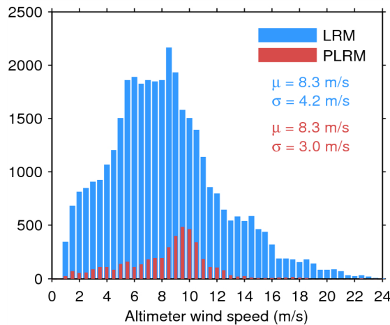
Figure 33. Histogram of flag-valid wind over oceans and lakes for LRM (blue) and PLRM (red) for 15/09/2014. The mean ( \mu ) and standard deviation ( \sigma ) are also shown. Note that values larger than 24 m/s are excluded from the histogram for the sake of readability but not from the computation of \mu and \sigma .
