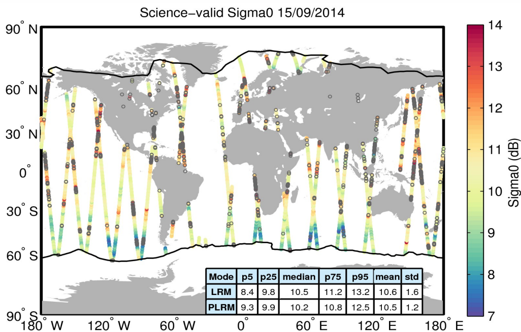
Figure 27. Geographical distribution of science-valid sigma0 data over oceans and lakes for 15/09/2014. The statistical values shown in the table refer to the sigma0 in dB and are calculated separately for LRM and PLRM regions. The black lines mark the outer limit of the Arctic and Antarctic polar polygons. Gray circles denote records that have been rejected based on the editing criteria described in Table 4.
