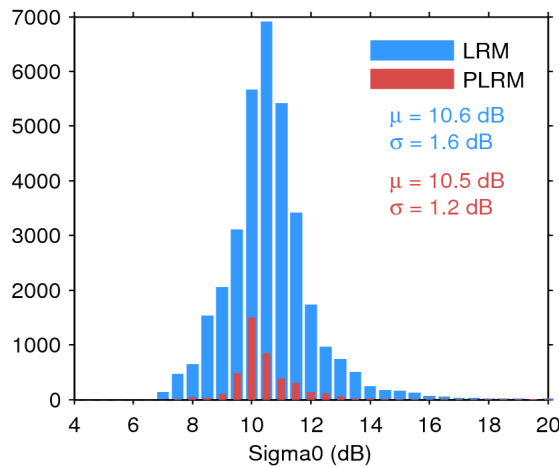
Figure 28. Histogram of science-valid sigma0 over oceans and lakes for LRM (blue) and PLRM (red) for 15/09/2014. The mean ( \mu ) and standard deviation ( \sigma ) are also shown. Note that values outside [4 20] dB are excluded from the histogram for the sake of readability but not from the computation of \mu and \sigma .
