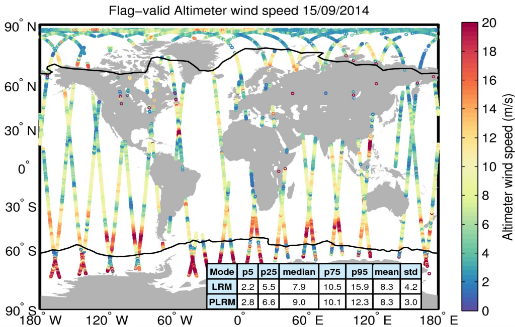
Figure 31. Geographical distribution of flag-valid wind data over oceans and lakes for 15/09/2014. The statistical values shown in the table refer to the wind in m/s and are calculated separately for LRM and PLRM regions. Measurements taken over polar polygons have been excluded from the computation of the statistical values. The black lines mark the outer limit of the Arctic and Antarctic polar polygons.
