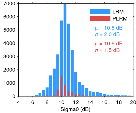
Figure 25. Histogram of flag-valid sigma0 over oceans and lakes for LRM (blue) and PLRM (red) for 15/09/2014. The mean ( \mu ) and standard deviation ( \sigma ) are also shown. Note that values outside [4 20] dB are excluded from the histogram for the sake of readability but not from the computation of \mu and \sigma .
