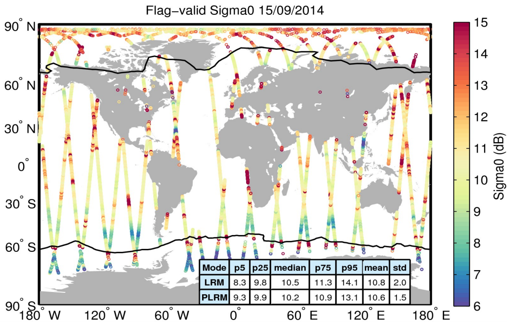
Figure 23. Geographical distribution of flag-valid sigma0 data over oceans and lakes for 15/09/2014. The statistical values shown in the table refer to the sigma0 in dB and are calculated separately for LRM and PLRM regions. Measurements taken over polar polygons have been excluded from the computation of the statistical values. The black lines mark the outer limit of the Arctic and Antarctic polar polygons.
