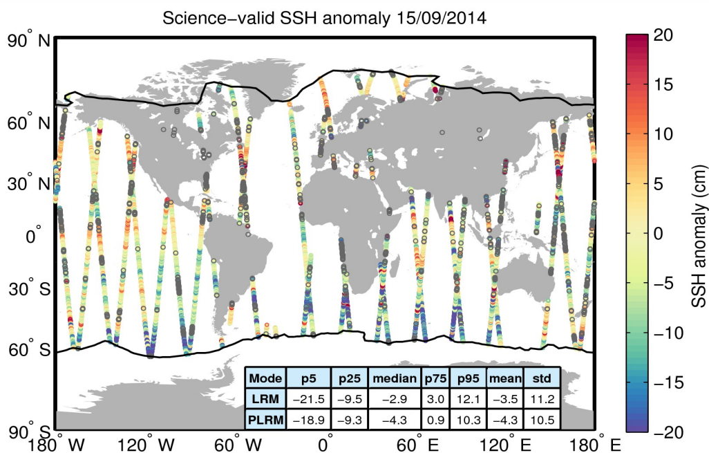
Figure 10. Geographical distribution of science-valid SSH anomaly data over oceans and lakes for 15/09/2014. The statistical values shown in the table refer to the SSH anomaly in cm and are calculated separately for LRM and PLRM regions. The black lines mark the outer limit of the Arctic and Antarctic polar polygons. Gray circles denote records that have been rejected based on the editing criteria described in Table 2.
