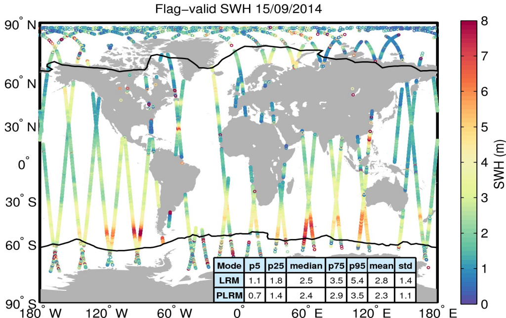
Figure 15. Geographical distribution of flag-valid SWH data over oceans and lakes for 15/09/2014. The statistical values shown in the table refer to the SWH in m and are calculated separately for LRM and PLRM regions. Measurements taken over polar polygons have been excluded from the computation of the statistical values. The black lines mark the outer limit of the Arctic and Antarctic polar polygons.
