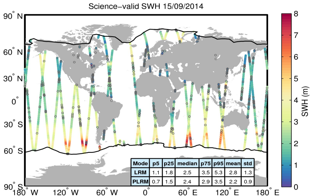
Figure 19. Geographical distribution of science-valid SWH data over oceans and lakes for 15/09/2014. The statistical values shown in the table refer to the SWH in m and are calculated separately for LRM and PLRM regions. The black lines mark the outer limit of the Arctic and Antarctic polar polygons. Gray circles denote records that have been rejected based on the editing criteria described in Table 3.
