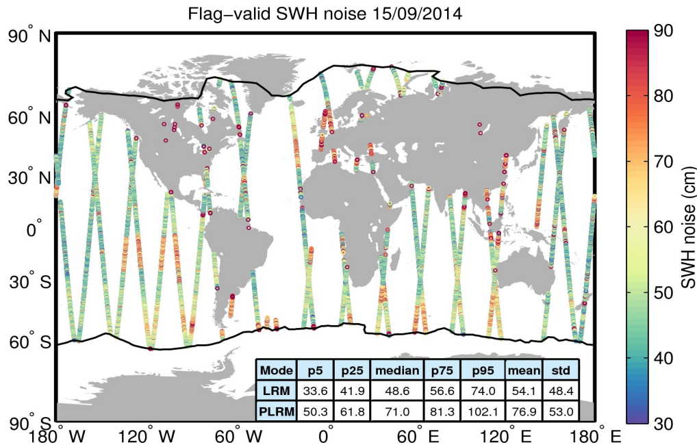
Figure 18. Geographical distribution of flag-valid 20-Hz SWH measurement noise over oceans and lakes for 15/09/2014. The statistical values shown in the table refer to the SWH noise and are calculated separately for LRM and PLRM regions. Measurements taken over polar polygons have been excluded from the computation of the statistical values. The black lines mark the outer limit of the Arctic and Antarctic polar polygons.
