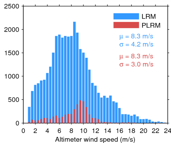
Figure 35. Histogram of science-valid wind over oceans and lakes for LRM (blue) and PLRM (red) for 15/09/2014. The mean ( \mu ) and standard deviation ( \sigma ) are also shown. Note that values larger than 24 m/s are excluded from the histogram for the sake of readability but not from the computation of \mu and \sigma .
