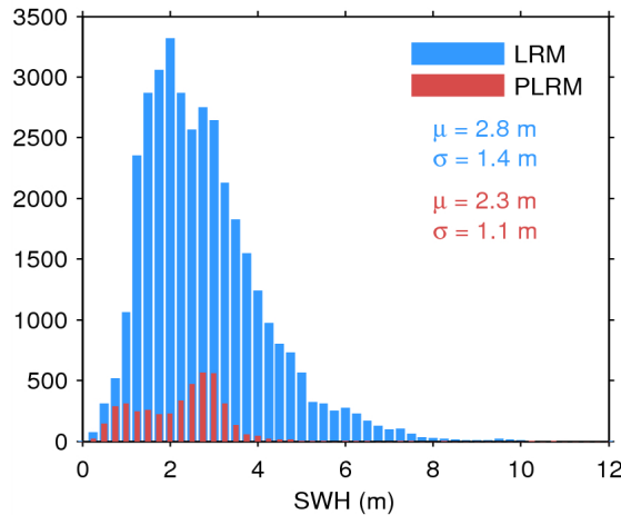
Figure 17. Histogram of flag-valid SWH over oceans and lakes for LRM (blue) and PLRM (red) for 15/09/2014. The mean ( \mu ) and standard deviation ( \sigma ) are also shown. Note that values larger than 12 m are excluded from the histogram for the sake of readability but not from the computation of \mu and \sigma .
