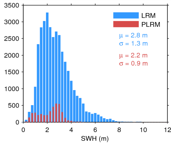
Figure 20. Histogram of science-valid SWH over oceans and lakes for LRM (blue) and PLRM (red) for 15/09/2014. The mean ( \mu ) and standard deviation ( \sigma ) are also shown. Note that values larger than 12 m are excluded from the histogram for the sake of readability but not from the computation of \mu and \sigma .
