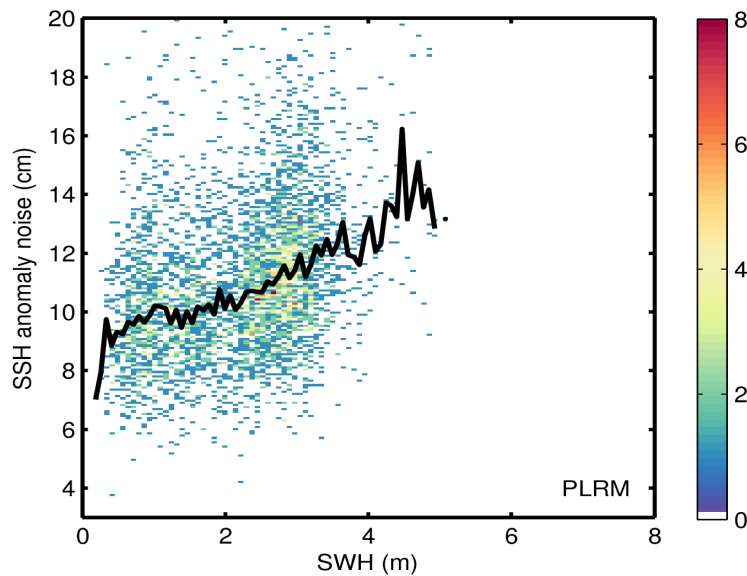
Figure 9. 2D histogram showing flag-valid SSH anomaly noise as a function of SWH for LRM (top) and PLRM (bottom) for 15/09/2014. The black line denotes the median SSH anomaly as a function of SWH.
