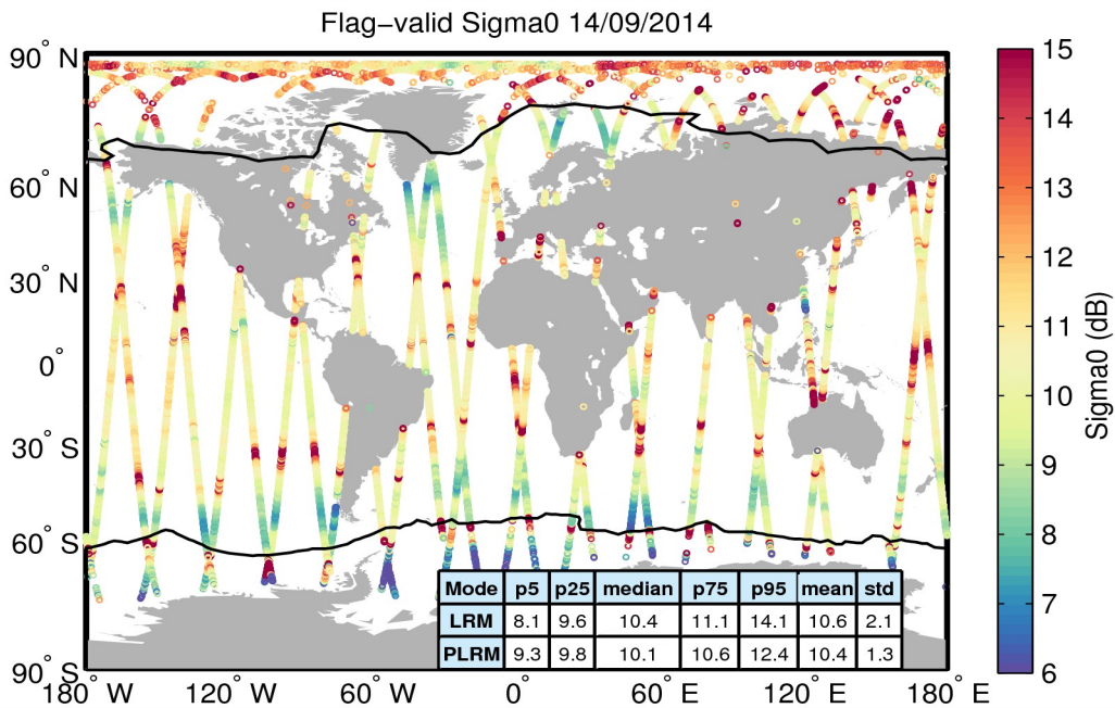
Figure 23. Geographical distribution of flag-valid sigma0 data over oceans and lakes for 14/09/2014. The statistical values shown in the table refer to the sigma0 in dB and are calculated separately for LRM and PLRM regions. Measurements taken over polar polygons have been excluded from the computation of the statistical values. The black lines mark the outer limit of the Arctic and Antarctic polar polygons.
