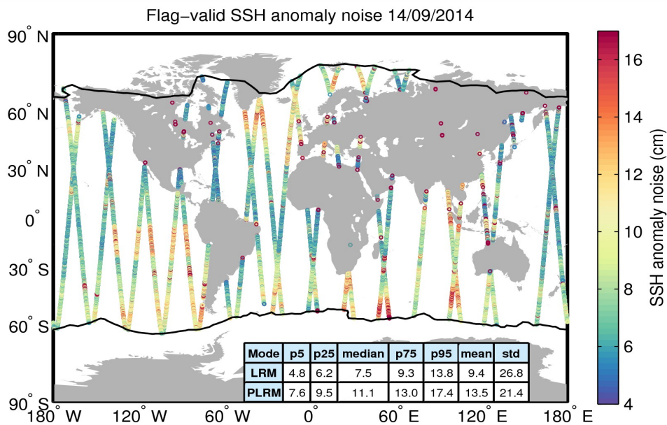
Figure 8. Geographical distribution of flag-valid 20-Hz SSH anomaly measurement noise over oceans and lakes for 14/09/2014. The statistical values shown in the table refer to the SSH anomaly noise and are calculated separately for LRM and PLRM regions. Measurements taken over polar polygons have been excluded from the computation of the statistical values. The black lines mark the outer limit of the Arctic and Antarctic polar polygons.
