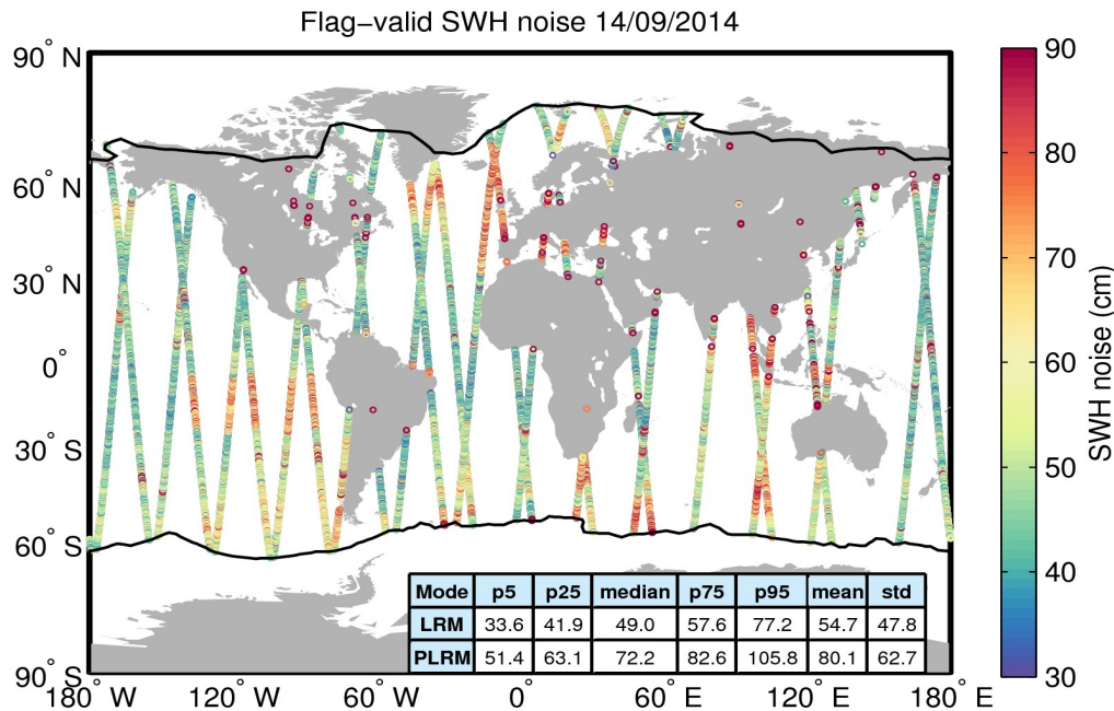
Figure 18. Geographical distribution of flag-valid 20-Hz SWH measurement noise over oceans and lakes for 14/09/2014. The statistical values shown in the table refer to the SWH noise and are calculated separately for LRM and PLRM regions. Measurements taken over polar polygons have been excluded from the computation of the statistical values. The black lines mark the outer limit of the Arctic and Antarctic polar polygons.
