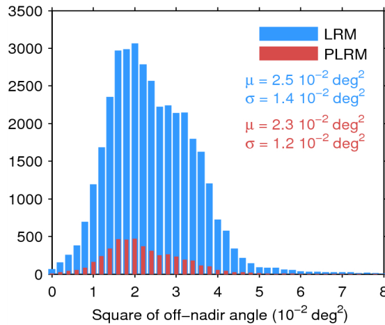
Figure 39. Histogram of flag-valid mispointing over oceans and lakes for LRM (blue) and PLRM (red) for 14/09/2014. Only positive values have been considered. The mean ( \mu ) and standard deviation ( \sigma ) are also shown. Note that values larger than 8 \cdot 10^{-2} \text{ deg}^2 are excluded from the histogram for the sake of readability but not from the computation of \mu and \sigma .
