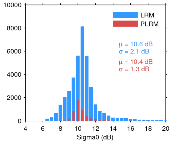
Figure 25. Histogram of flag-valid sigma0 over oceans and lakes for LRM (blue) and PLRM (red) for 14/09/2014. The mean ( \mu ) and standard deviation ( \sigma ) are also shown. Note that values outside [4 20] dB are excluded from the histogram for the sake of readability but not from the computation of \mu and \sigma .
