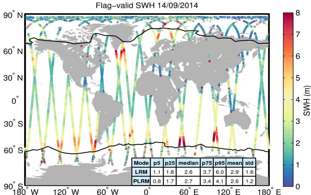
Figure 15. Geographical distribution of flag-valid SWH data over oceans and lakes for 14/09/2014. The statistical values shown in the table refer to the SWH in m and are calculated separately for LRM and PLRM regions. Measurements taken over polar polygons have been excluded from the computation of the statistical values. The black lines mark the outer limit of the Arctic and Antarctic polar polygons.
