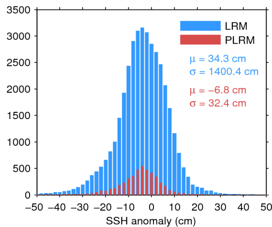
Figure 7. Histogram of flag-valid SSH anomaly over oceans and lakes for LRM (blue) and PLRM (red) for 14/09/2014. The mean ( \mu ) and standard deviation ( \sigma ) are also shown. Note that values outside [-50 50] cm are excluded from the histogram for the sake of readability but not from the computation of \mu and \sigma .
