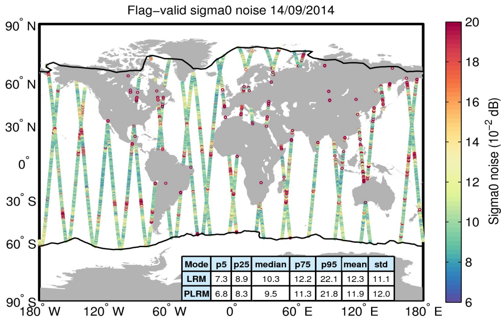
Figure 26. Geographical distribution of flag-valid 20-Hz sigma0 measurement noise over oceans and lakes for 14/09/2014. The statistical values shown in the table refer to the sigma0 noise and are calculated separately for LRM and PLRM regions. Measurements taken over polar polygons have been excluded from the computation of the statistical values. The black lines mark the outer limit of the Arctic and Antarctic polar polygons.
