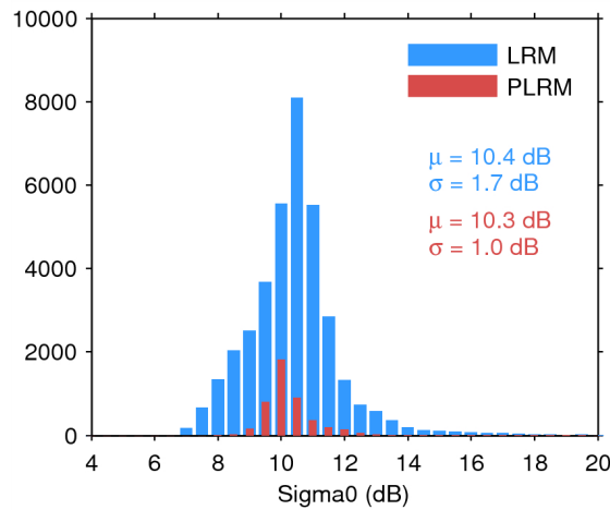
Figure 28. Histogram of science-valid sigma0 over oceans and lakes for LRM (blue) and PLRM (red) for 14/09/2014. The mean ( \mu ) and standard deviation ( \sigma ) are also shown. Note that values outside [4 20] dB are excluded from the histogram for the sake of readability but not from the computation of \mu and \sigma .
