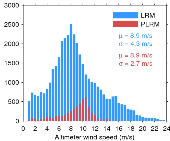
Figure 33. Histogram of flag-valid wind over oceans and lakes for LRM (blue) and PLRM (red) for 14/09/2014. The mean ( \mu ) and standard deviation ( \sigma ) are also shown. Note that values larger than 24 m/s are excluded from the histogram for the sake of readability but not from the computation of \mu and \sigma .
