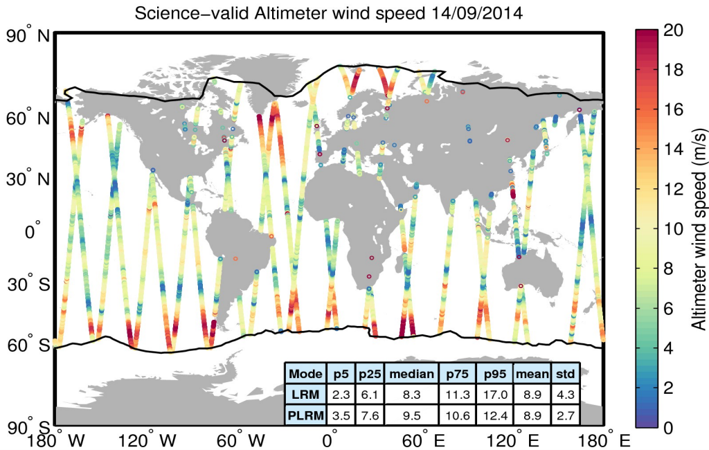
Figure 34. Geographical distribution of science-valid wind data over oceans and lakes for 14/09/2014. The statistical values shown in the table refer to the wind in m/s and are calculated separately for LRM and PLRM regions. The black lines mark the outer limit of the Arctic and Antarctic polar polygons. Gray circles denote records that have been rejected based on the editing criteria described in Table 5.
