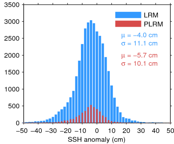
Figure 11. Histogram of science-valid SSH anomaly over oceans and lakes for LRM (blue) and PLRM (red) for 14/09/2014. The mean ( \mu ) and standard deviation ( \sigma ) are also shown. Note that values outside [-50\ 50] cm are excluded from the histogram for the sake of readability but not from the computation of \mu and \sigma .
