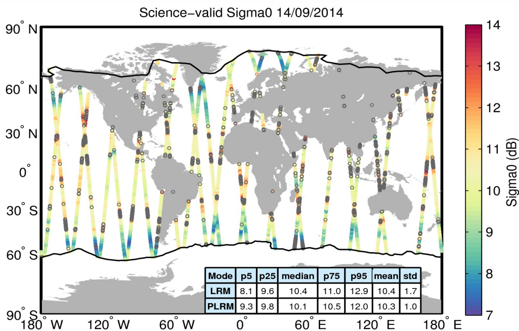
Figure 27. Geographical distribution of science-valid sigma0 data over oceans and lakes for 14/09/2014. The statistical values shown in the table refer to the sigma0 in dB and are calculated separately for LRM and PLRM regions. The black lines mark the outer limit of the Arctic and Antarctic polar polygons. Gray circles denote records that have been rejected based on the editing criteria described in Table 4.
