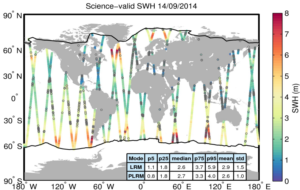
Figure 19. Geographical distribution of science-valid SWH data over oceans and lakes for 14/09/2014. The statistical values shown in the table refer to the SWH in m and are calculated separately for LRM and PLRM regions. The black lines mark the outer limit of the Arctic and Antarctic polar polygons. Gray circles denote records that have been rejected based on the editing criteria described in Table 3.
