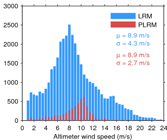
Figure 35. Histogram of science-valid wind over oceans and lakes for LRM (blue) and PLRM (red) for 14/09/2014. The mean ( \mu ) and standard deviation ( \sigma ) are also shown. Note that values larger than 24 m/s are excluded from the histogram for the sake of readability but not from the computation of \mu and \sigma .
