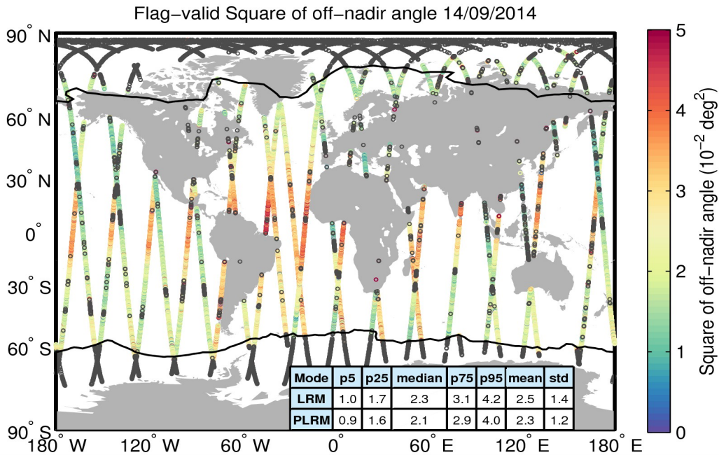
Figure 37. Geographical distribution of flag-valid mispointing data over oceans and lakes for 14/09/2014. The statistical values shown in the table refer to the mispointing in 10^{-2} \text{ deg}^2 and are calculated separately for LRM and PLRM regions. Measurements taken over polar polygons have been excluded from the computation of the statistical values. The black lines mark the outer limit of the Arctic and Antarctic polar polygons. Gray circles denote negative values.
