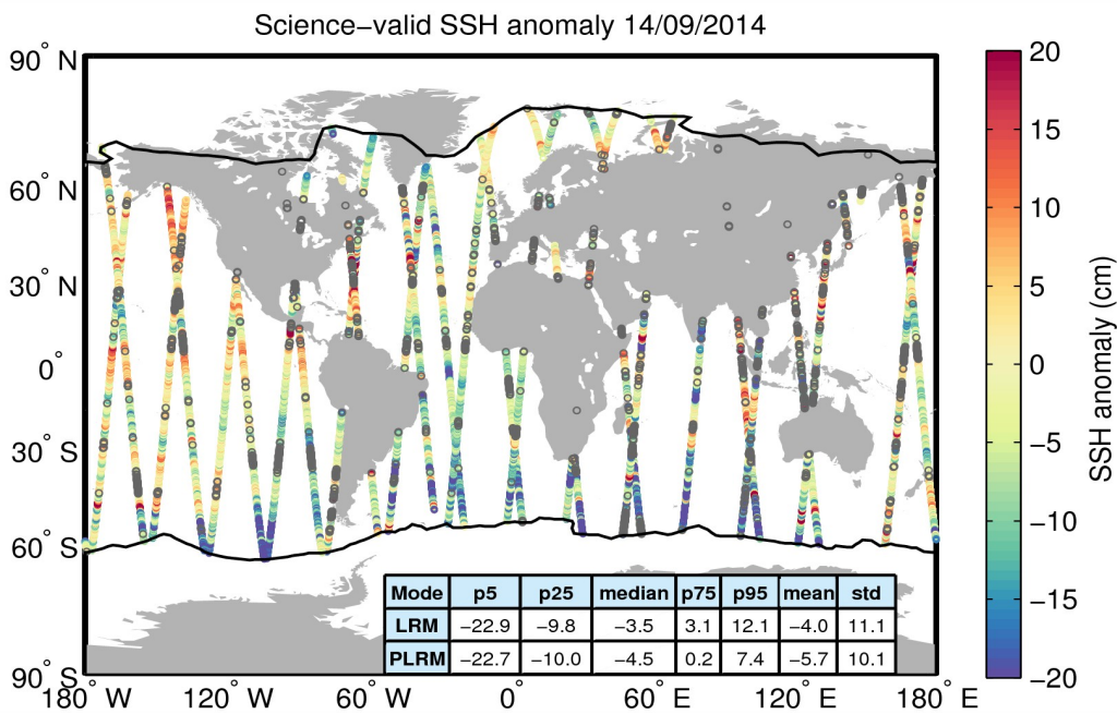
Figure 10. Geographical distribution of science-valid SSH anomaly data over oceans and lakes for 14/09/2014. The statistical values shown in the table refer to the SSH anomaly in cm and are calculated separately for LRM and PLRM regions. The black lines mark the outer limit of the Arctic and Antarctic polar polygons. Gray circles denote records that have been rejected based on the editing criteria described in Table 2.
