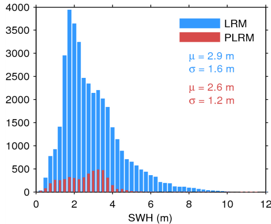
Figure 17. Histogram of flag-valid SWH over oceans and lakes for LRM (blue) and PLRM (red) for 14/09/2014. The mean ( \mu ) and standard deviation ( \sigma ) are also shown. Note that values larger than 12 m are excluded from the histogram for the sake of readability but not from the computation of \mu and \sigma .
