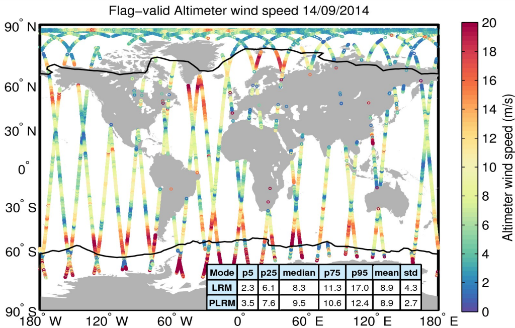
Figure 31. Geographical distribution of flag-valid wind data over oceans and lakes for 14/09/2014. The statistical values shown in the table refer to the wind in m/s and are calculated separately for LRM and PLRM regions. Measurements taken over polar polygons have been excluded from the computation of the statistical values. The black lines mark the outer limit of the Arctic and Antarctic polar polygons.
