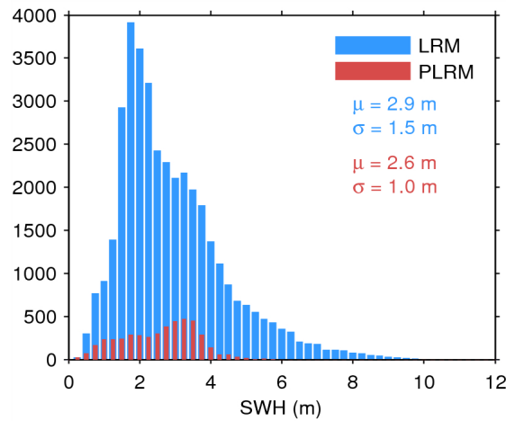
Figure 20. Histogram of science-valid SWH over oceans and lakes for LRM (blue) and PLRM (red) for 14/09/2014. The mean ( \mu ) and standard deviation ( \sigma ) are also shown. Note that values larger than 12 m are excluded from the histogram for the sake of readability but not from the computation of \mu and \sigma .
