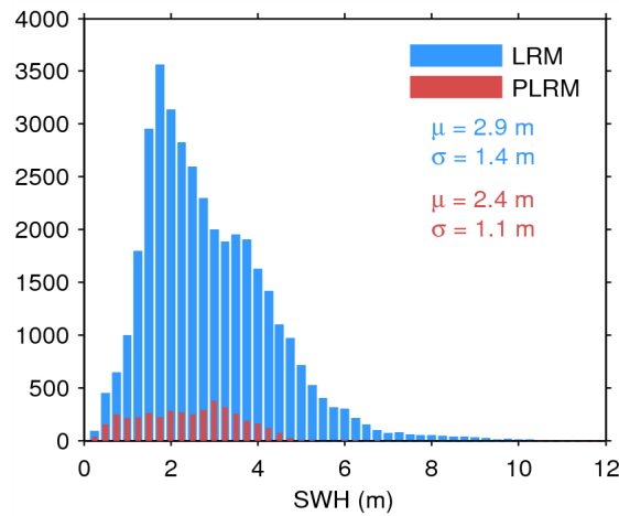
Figure 20. Histogram of science-valid SWH over oceans and lakes for LRM (blue) and PLRM (red) for 13/09/2014. The mean ( \mu ) and standard deviation ( \sigma ) are also shown. Note that values larger than 12 m are excluded from the histogram for the sake of readability but not from the computation of \mu and \sigma .
