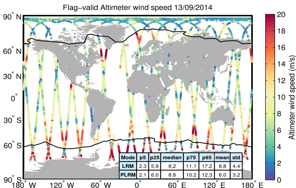
Figure 31. Geographical distribution of flag-valid wind data over oceans and lakes for 13/09/2014. The statistical values shown in the table refer to the wind in m/s and are calculated separately for LRM and PLRM regions. Measurements taken over polar polygons have been excluded from the computation of the statistical values. The black lines mark the outer limit of the Arctic and Antarctic polar polygons.
