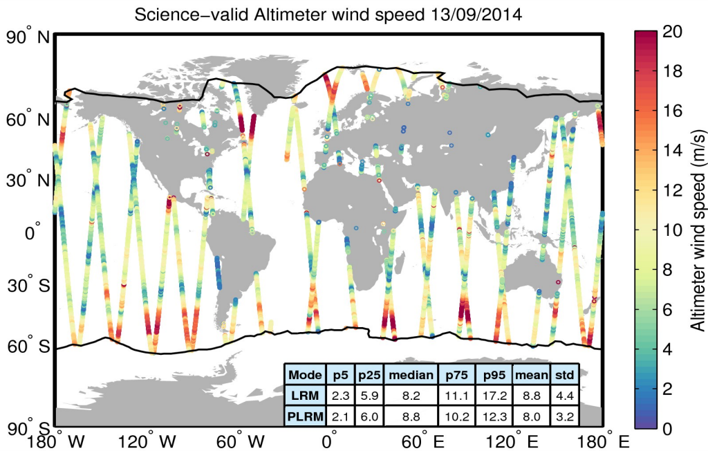
Figure 34. Geographical distribution of science-valid wind data over oceans and lakes for 13/09/2014. The statistical values shown in the table refer to the wind in m/s and are calculated separately for LRM and PLRM regions. The black lines mark the outer limit of the Arctic and Antarctic polar polygons. Gray circles denote records that have been rejected based on the editing criteria described in Table 5.
