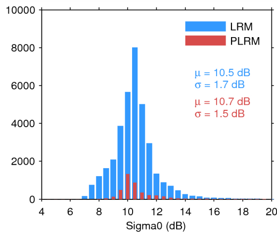
Figure 28. Histogram of science-valid sigma0 over oceans and lakes for LRM (blue) and PLRM (red) for 13/09/2014. The mean ( \mu ) and standard deviation ( \sigma ) are also shown. Note that values outside [4 20] dB are excluded from the histogram for the sake of readability but not from the computation of \mu and \sigma .
