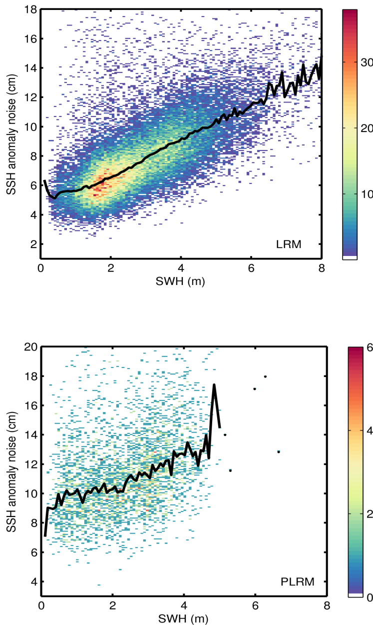
Figure 9. 2D histogram showing flag-valid SSH anomaly noise as a function of SWH for LRM (top) and PLRM (bottom) for 13/09/2014. The black line denotes the median SSH anomaly as a function of SWH.
