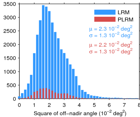
Figure 39. Histogram of flag-valid mispointing over oceans and lakes for LRM (blue) and PLRM (red) for 13/09/2014. Only positive values have been considered. The mean ( \mu ) and standard deviation ( \sigma ) are also shown. Note that values larger than 8 \cdot 10^{-2} \text{ deg}^2 are excluded from the histogram for the sake of readability but not from the computation of \mu and \sigma .
