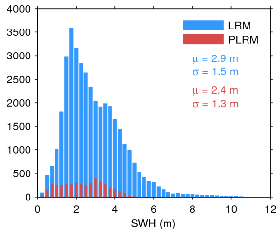
Figure 17. Histogram of flag-valid SWH over oceans and lakes for LRM (blue) and PLRM (red) for 13/09/2014. The mean ( \mu ) and standard deviation ( \sigma ) are also shown. Note that values larger than 12 m are excluded from the histogram for the sake of readability but not from the computation of \mu and \sigma .
