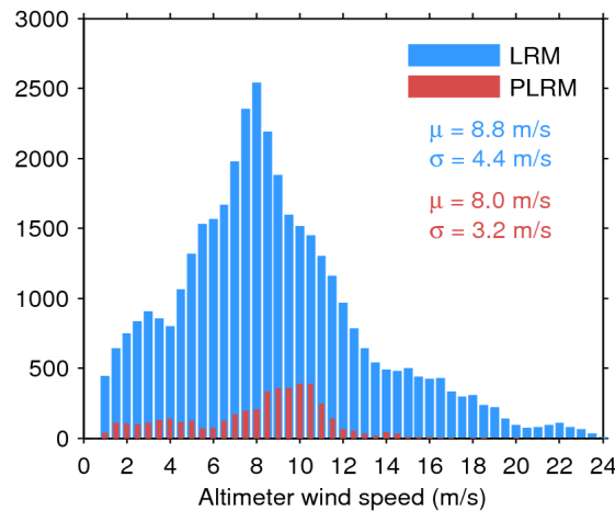
Figure 33. Histogram of flag-valid wind over oceans and lakes for LRM (blue) and PLRM (red) for 13/09/2014. The mean ( \mu ) and standard deviation ( \sigma ) are also shown. Note that values larger than 24 m/s are excluded from the histogram for the sake of readability but not from the computation of \mu and \sigma .
