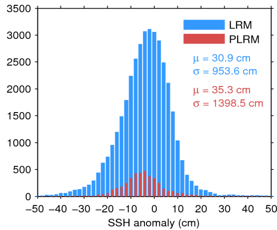
Figure 7. Histogram of flag-valid SSH anomaly over oceans and lakes for LRM (blue) and PLRM (red) for 13/09/2014. The mean ( \mu ) and standard deviation ( \sigma ) are also shown. Note that values outside [-50\ 50] cm are excluded from the histogram for the sake of readability but not from the computation of \mu and \sigma .
