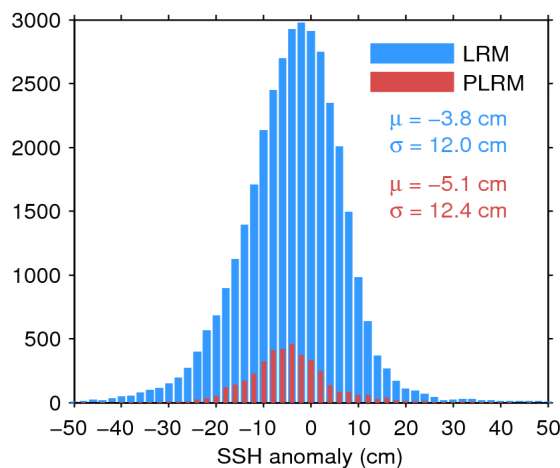
Figure 11. Histogram of science-valid SSH anomaly over oceans and lakes for LRM (blue) and PLRM (red) for 13/09/2014. The mean ( \mu ) and standard deviation ( \sigma ) are also shown. Note that values outside [-50 \ 50] cm are excluded from the histogram for the sake of readability but not from the computation of \mu and \sigma .
