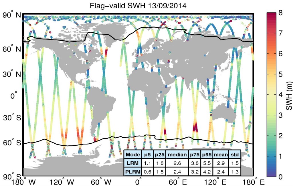
Figure 15. Geographical distribution of flag-valid SWH data over oceans and lakes for 13/09/2014. The statistical values shown in the table refer to the SWH in m and are calculated separately for LRM and PLRM regions. Measurements taken over polar polygons have been excluded from the computation of the statistical values. The black lines mark the outer limit of the Arctic and Antarctic polar polygons.
