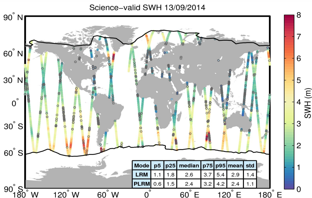
Figure 19. Geographical distribution of science-valid SWH data over oceans and lakes for 13/09/2014. The statistical values shown in the table refer to the SWH in m and are calculated separately for LRM and PLRM regions. The black lines mark the outer limit of the Arctic and Antarctic polar polygons. Gray circles denote records that have been rejected based on the editing criteria described in Table 3.
