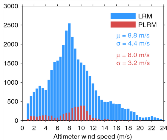
Figure 35. Histogram of science-valid wind over oceans and lakes for LRM (blue) and PLRM (red) for 13/09/2014. The mean ( \mu ) and standard deviation ( \sigma ) are also shown. Note that values larger than 24 m/s are excluded from the histogram for the sake of readability but not from the computation of \mu and \sigma .
