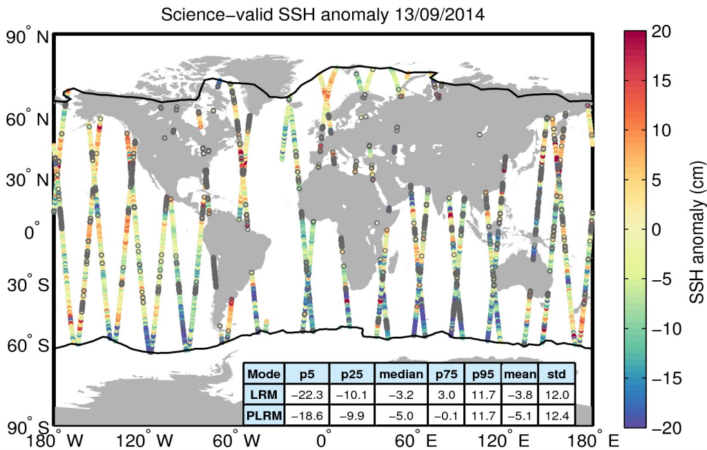
Figure 10. Geographical distribution of science-valid SSH anomaly data over oceans and lakes for 13/09/2014. The statistical values shown in the table refer to the SSH anomaly in cm and are calculated separately for LRM and PLRM regions. The black lines mark the outer limit of the Arctic and Antarctic polar polygons. Gray circles denote records that have been rejected based on the editing criteria described in Table 2.
