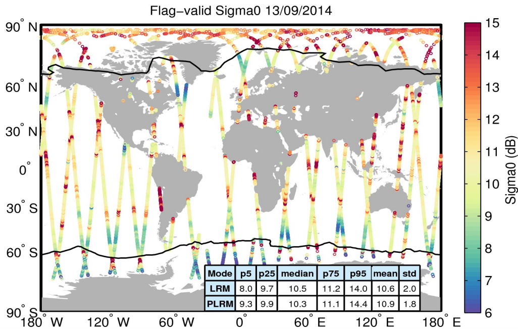
Figure 23. Geographical distribution of flag-valid sigma0 data over oceans and lakes for 13/09/2014. The statistical values shown in the table refer to the sigma0 in dB and are calculated separately for LRM and PLRM regions. Measurements taken over polar polygons have been excluded from the computation of the statistical values. The black lines mark the outer limit of the Arctic and Antarctic polar polygons.
