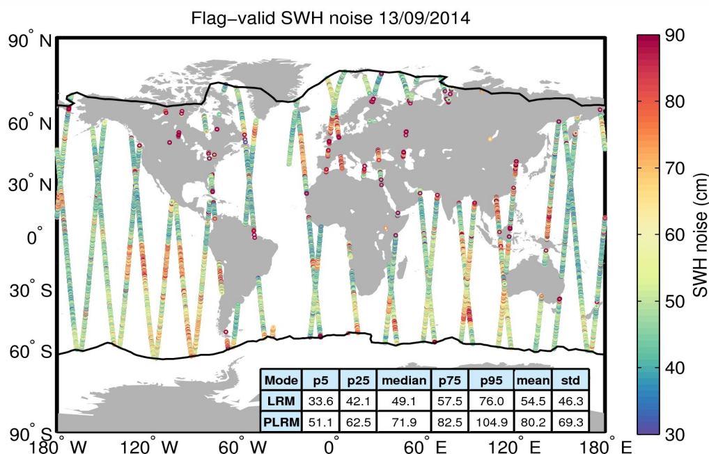
Figure 18. Geographical distribution of flag-valid 20-Hz SWH measurement noise over oceans and lakes for 13/09/2014. The statistical values shown in the table refer to the SWH noise and are calculated separately for LRM and PLRM regions. Measurements taken over polar polygons have been excluded from the computation of the statistical values. The black lines mark the outer limit of the Arctic and Antarctic polar polygons.
