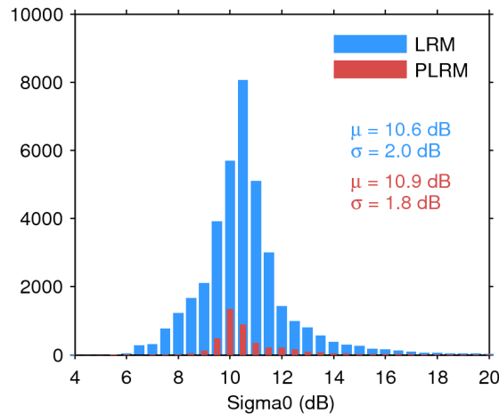
Figure 25. Histogram of flag-valid sigma0 over oceans and lakes for LRM (blue) and PLRM (red) for 13/09/2014. The mean ( \mu ) and standard deviation ( \sigma ) are also shown. Note that values outside [4 20] dB are excluded from the histogram for the sake of readability but not from the computation of \mu and \sigma .
