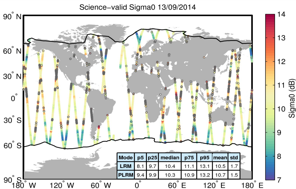
Figure 27. Geographical distribution of science-valid sigma0 data over oceans and lakes for 13/09/2014. The statistical values shown in the table refer to the sigma0 in dB and are calculated separately for LRM and PLRM regions. The black lines mark the outer limit of the Arctic and Antarctic polar polygons. Gray circles denote records that have been rejected based on the editing criteria described in Table 4.
