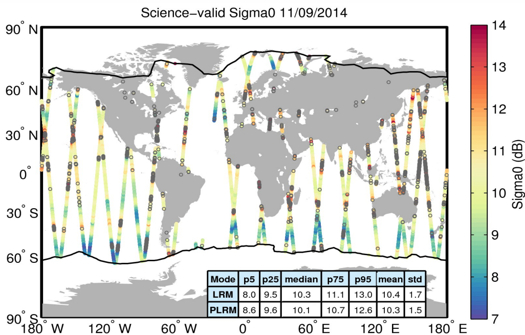
Figure 27. Geographical distribution of science-valid sigma0 data over oceans and lakes for 11/09/2014. The statistical values shown in the table refer to the sigma0 in dB and are calculated separately for LRM and PLRM regions. The black lines mark the outer limit of the Arctic and Antarctic polar polygons. Gray circles denote records that have been rejected based on the editing criteria described in Table 4.
