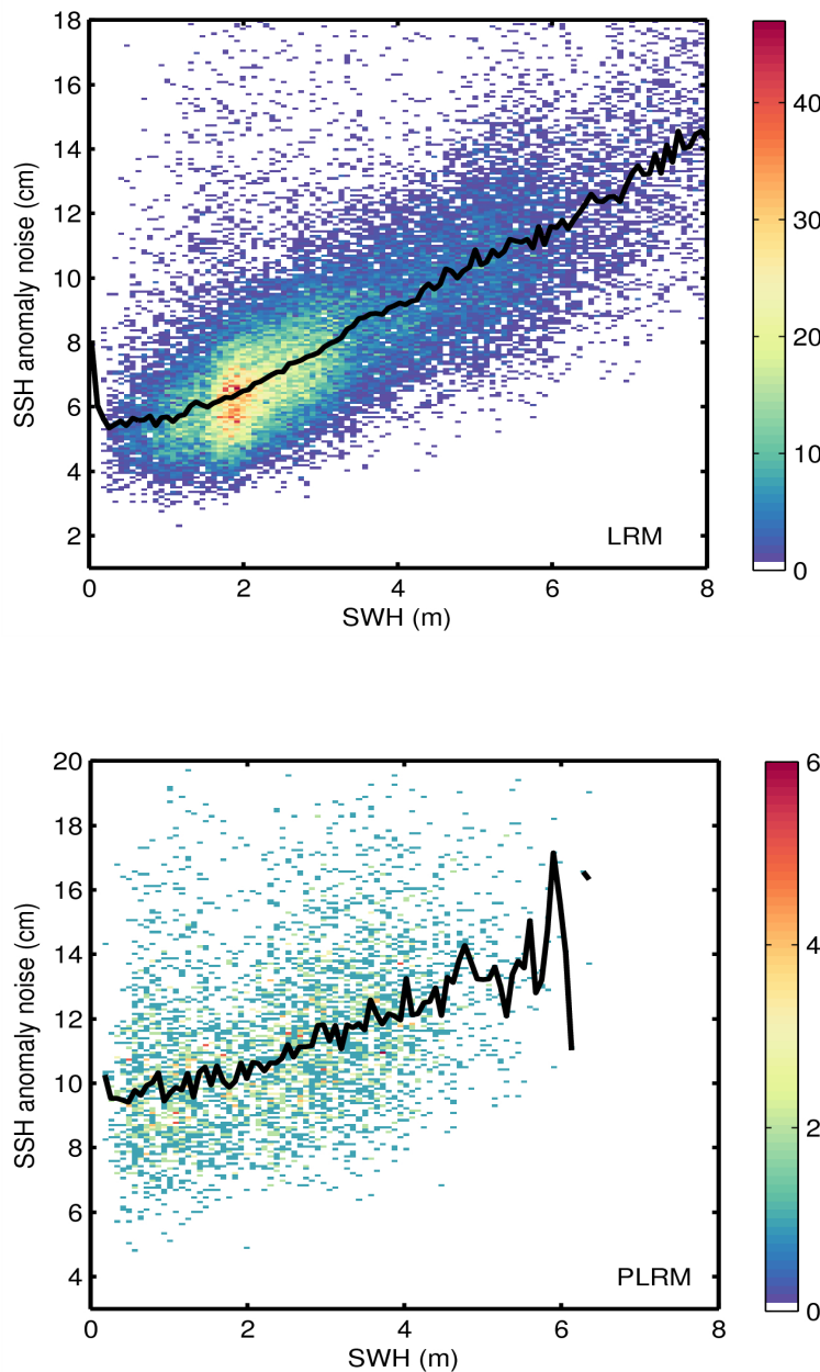
Figure 9. 2D histogram showing flag-valid SSH anomaly noise as a function of SWH for LRM (top) and PLRM (bottom) for 11/09/2014. The black line denotes the median SSH anomaly as a function of SWH.
