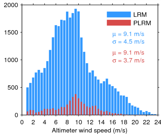
Figure 33. Histogram of flag-valid wind over oceans and lakes for LRM (blue) and PLRM (red) for 11/09/2014. The mean ( \mu ) and standard deviation ( \sigma ) are also shown. Note that values larger than 24 m/s are excluded from the histogram for the sake of readability but not from the computation of \mu and \sigma .
