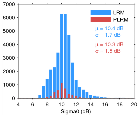
Figure 28. Histogram of science-valid sigma0 over oceans and lakes for LRM (blue) and PLRM (red) for 11/09/2014. The mean ( \mu ) and standard deviation ( \sigma ) are also shown. Note that values outside [4 20] dB are excluded from the histogram for the sake of readability but not from the computation of \mu and \sigma .
