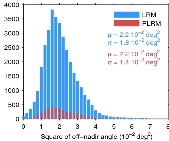
Figure 39. Histogram of flag-valid mispointing over oceans and lakes for LRM (blue) and PLRM (red) for 11/09/2014. Only positive values have been considered. The mean ( \mu ) and standard deviation ( \sigma ) are also shown. Note that values larger than 8 \cdot 10^{-2} \text{ deg}^2 are excluded from the histogram for the sake of readability but not from the computation of \mu and \sigma .
