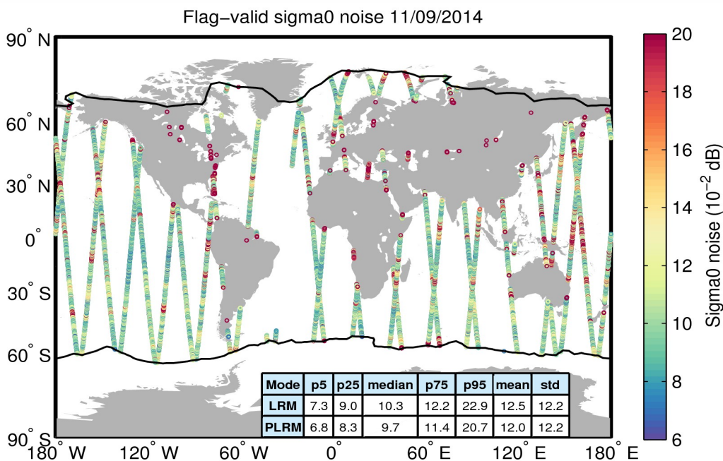
Figure 26. Geographical distribution of flag-valid 20-Hz sigma0 measurement noise over oceans and lakes for 11/09/2014. The statistical values shown in the table refer to the sigma0 noise and are calculated separately for LRM and PLRM regions. Measurements taken over polar polygons have been excluded from the computation of the statistical values. The black lines mark the outer limit of the Arctic and Antarctic polar polygons.
