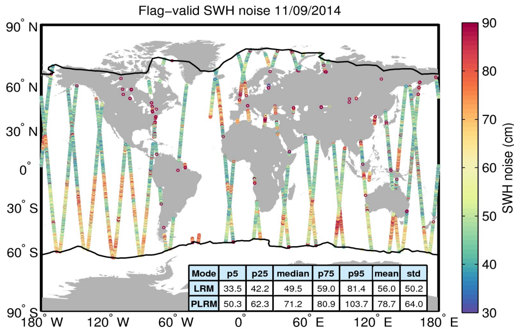
Figure 18. Geographical distribution of flag-valid 20-Hz SWH measurement noise over oceans and lakes for 11/09/2014. The statistical values shown in the table refer to the SWH noise and are calculated separately for LRM and PLRM regions. Measurements taken over polar polygons have been excluded from the computation of the statistical values. The black lines mark the outer limit of the Arctic and Antarctic polar polygons.
