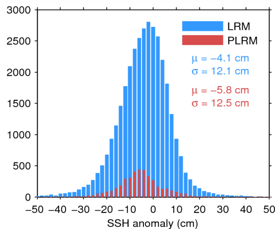
Figure 11. Histogram of science-valid SSH anomaly over oceans and lakes for LRM (blue) and PLRM (red) for 11/09/2014. The mean ( \mu ) and standard deviation ( \sigma ) are also shown. Note that values outside [-50 50] cm are excluded from the histogram for the sake of readability but not from the computation of \mu and \sigma .
