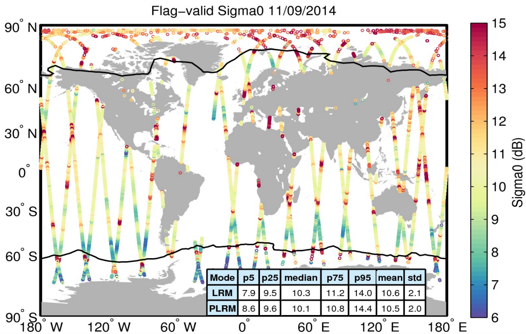
Figure 23. Geographical distribution of flag-valid sigma0 data over oceans and lakes for 11/09/2014. The statistical values shown in the table refer to the sigma0 in dB and are calculated separately for LRM and PLRM regions. Measurements taken over polar polygons have been excluded from the computation of the statistical values. The black lines mark the outer limit of the Arctic and Antarctic polar polygons.
