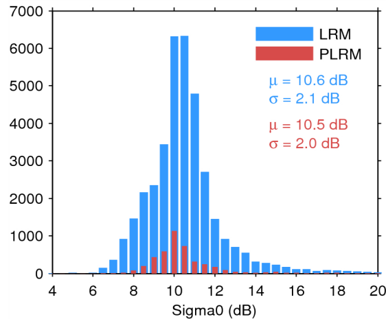
Figure 25. Histogram of flag-valid sigma0 over oceans and lakes for LRM (blue) and PLRM (red) for 11/09/2014. The mean ( \mu ) and standard deviation ( \sigma ) are also shown. Note that values outside [4 20] dB are excluded from the histogram for the sake of readability but not from the computation of \mu and \sigma .
