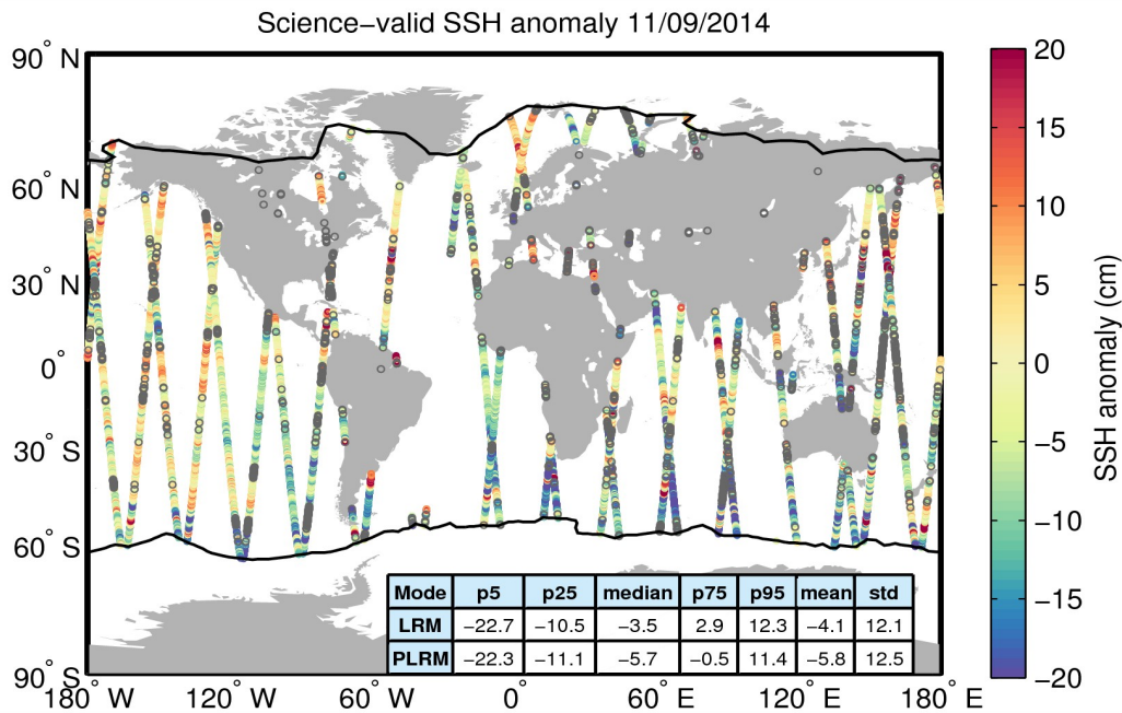
Figure 10. Geographical distribution of science-valid SSH anomaly data over oceans and lakes for 11/09/2014. The statistical values shown in the table refer to the SSH anomaly in cm and are calculated separately for LRM and PLRM regions. The black lines mark the outer limit of the Arctic and Antarctic polar polygons. Gray circles denote records that have been rejected based on the editing criteria described in Table 2.
