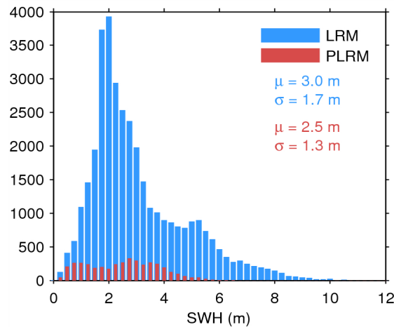
Figure 20. Histogram of science-valid SWH over oceans and lakes for LRM (blue) and PLRM (red) for 11/09/2014. The mean ( \mu ) and standard deviation ( \sigma ) are also shown. Note that values larger than 12 m are excluded from the histogram for the sake of readability but not from the computation of \mu and \sigma .
