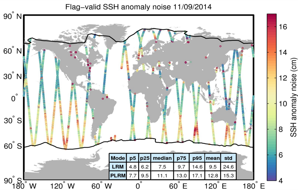
Figure 8. Geographical distribution of flag-valid 20-Hz SSH anomaly measurement noise over oceans and lakes for 11/09/2014. The statistical values shown in the table refer to the SSH anomaly noise and are calculated separately for LRM and PLRM regions. Measurements taken over polar polygons have been excluded from the computation of the statistical values. The black lines mark the outer limit of the Arctic and Antarctic polar polygons.
