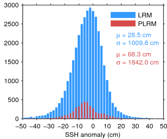
Figure 7. Histogram of flag-valid SSH anomaly over oceans and lakes for LRM (blue) and PLRM (red) for 11/09/2014. The mean ( \mu ) and standard deviation ( \sigma ) are also shown. Note that values outside [-50\ 50] cm are excluded from the histogram for the sake of readability but not from the computation of \mu and \sigma .
