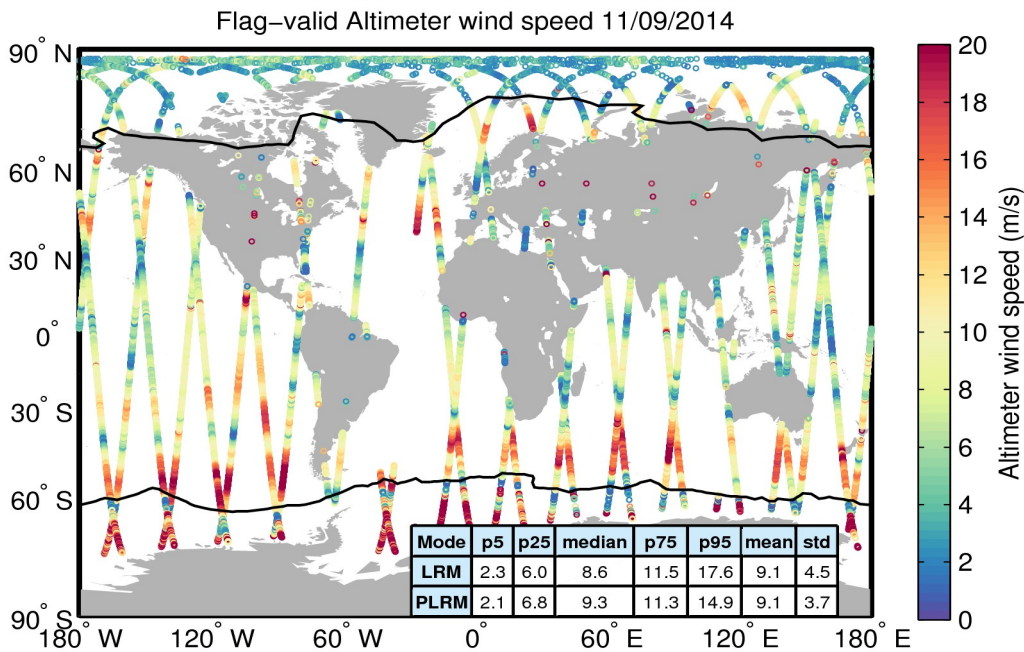
Figure 31. Geographical distribution of flag-valid wind data over oceans and lakes for 11/09/2014. The statistical values shown in the table refer to the wind in m/s and are calculated separately for LRM and PLRM regions. Measurements taken over polar polygons have been excluded from the computation of the statistical values. The black lines mark the outer limit of the Arctic and Antarctic polar polygons.
