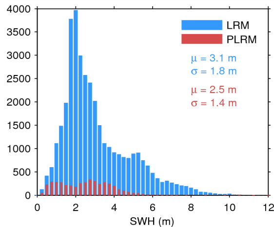
Figure 17. Histogram of flag-valid SWH over oceans and lakes for LRM (blue) and PLRM (red) for 11/09/2014. The mean ( \mu ) and standard deviation ( \sigma ) are also shown. Note that values larger than 12 m are excluded from the histogram for the sake of readability but not from the computation of \mu and \sigma .
