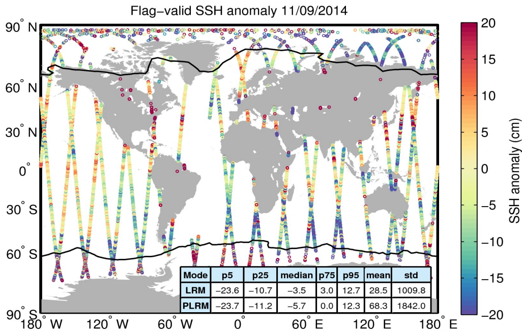
Figure 5. Geographical distribution of flag-valid 1-Hz SSH anomaly data over oceans and lakes for 11/09/2014. The statistical values shown in the table refer to the SSH anomaly in cm and are calculated separately for LRM and PLRM regions. Measurements taken over polar polygons have been excluded from the computation of the statistical values. The black lines mark the outer limit of the Arctic and Antarctic polar polygons.
