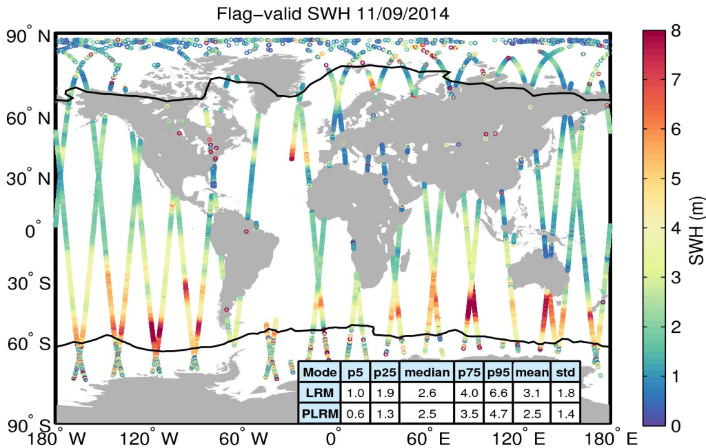
Figure 15. Geographical distribution of flag-valid SWH data over oceans and lakes for 11/09/2014. The statistical values shown in the table refer to the SWH in m and are calculated separately for LRM and PLRM regions. Measurements taken over polar polygons have been excluded from the computation of the statistical values. The black lines mark the outer limit of the Arctic and Antarctic polar polygons.
