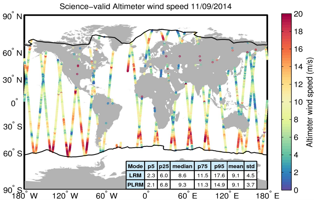
Figure 34. Geographical distribution of science-valid wind data over oceans and lakes for 11/09/2014. The statistical values shown in the table refer to the wind in m/s and are calculated separately for LRM and PLRM regions. The black lines mark the outer limit of the Arctic and Antarctic polar polygons. Gray circles denote records that have been rejected based on the editing criteria described in Table 5.
