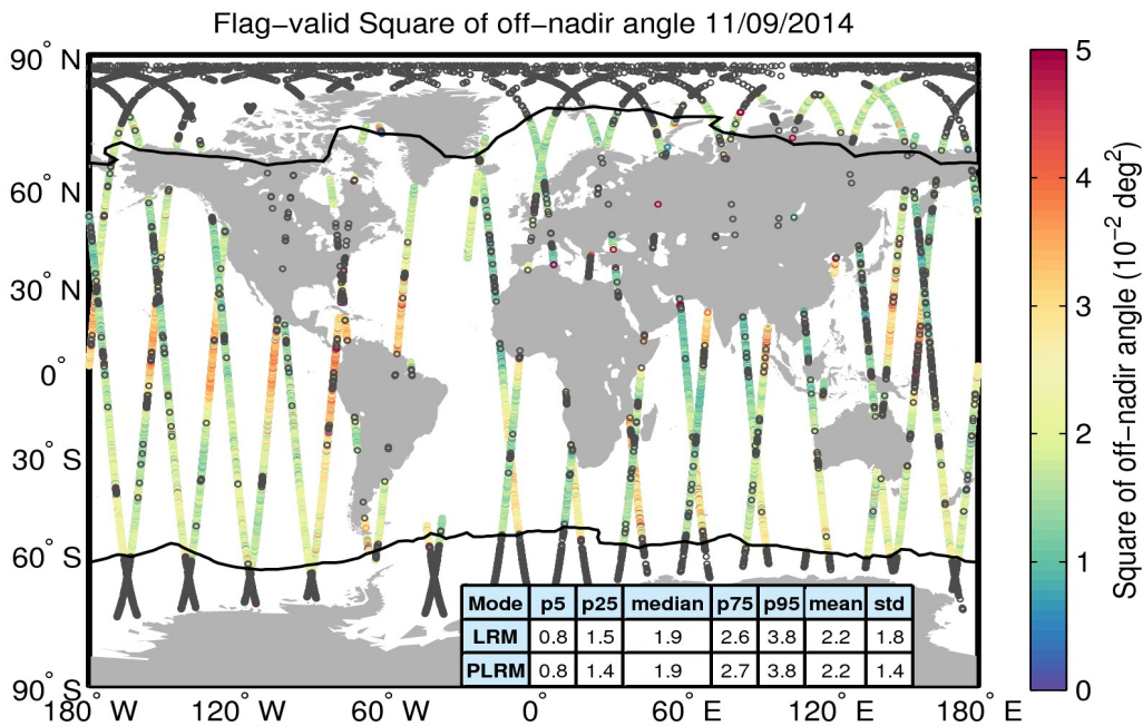
Figure 37. Geographical distribution of flag-valid mispointing data over oceans and lakes for 11/09/2014. The statistical values shown in the table refer to the mispointing in 10^{-2} \text{ deg}^2 and are calculated separately for LRM and PLRM regions. Measurements taken over polar polygons have been excluded from the computation of the statistical values. The black lines mark the outer limit of the Arctic and Antarctic polar polygons. Gray circles denote negative values.
