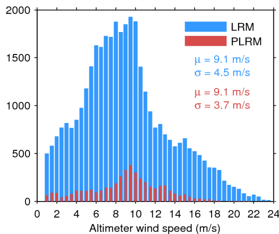
Figure 35. Histogram of science-valid wind over oceans and lakes for LRM (blue) and PLRM (red) for 11/09/2014. The mean ( \mu ) and standard deviation ( \sigma ) are also shown. Note that values larger than 24 m/s are excluded from the histogram for the sake of readability but not from the computation of \mu and \sigma .
