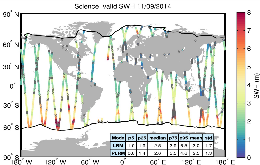
Figure 19. Geographical distribution of science-valid SWH data over oceans and lakes for 11/09/2014. The statistical values shown in the table refer to the SWH in m and are calculated separately for LRM and PLRM regions. The black lines mark the outer limit of the Arctic and Antarctic polar polygons. Gray circles denote records that have been rejected based on the editing criteria described in Table 3.
