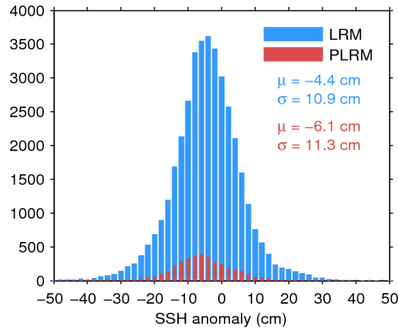
Figure 11. Histogram of science-valid SSH anomaly over oceans and lakes for LRM (blue) and PLRM (red) for 06/09/2014. The mean ( \mu ) and standard deviation ( \sigma ) are also shown. Note that values outside [-50\ 50] cm are excluded from the histogram for the sake of readability but not from the computation of \mu and \sigma .
