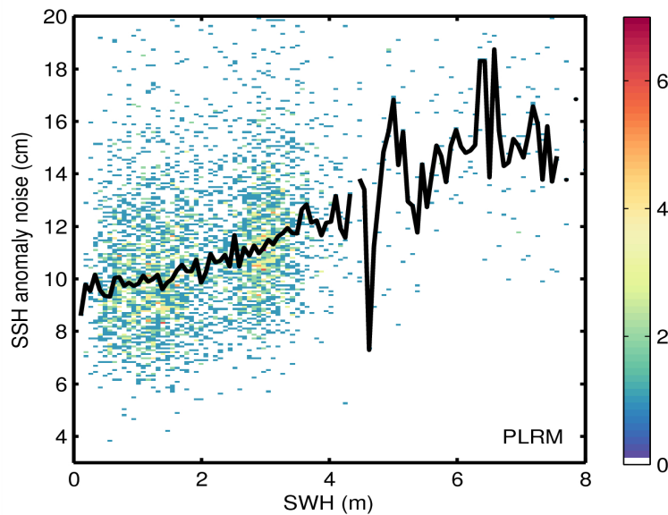
Figure 9. 2D histogram showing flag-valid SSH anomaly noise as a function of SWH for LRM (top) and PLRM (bottom) for 06/09/2014. The black line denotes the median SSH anomaly as a function of SWH.
