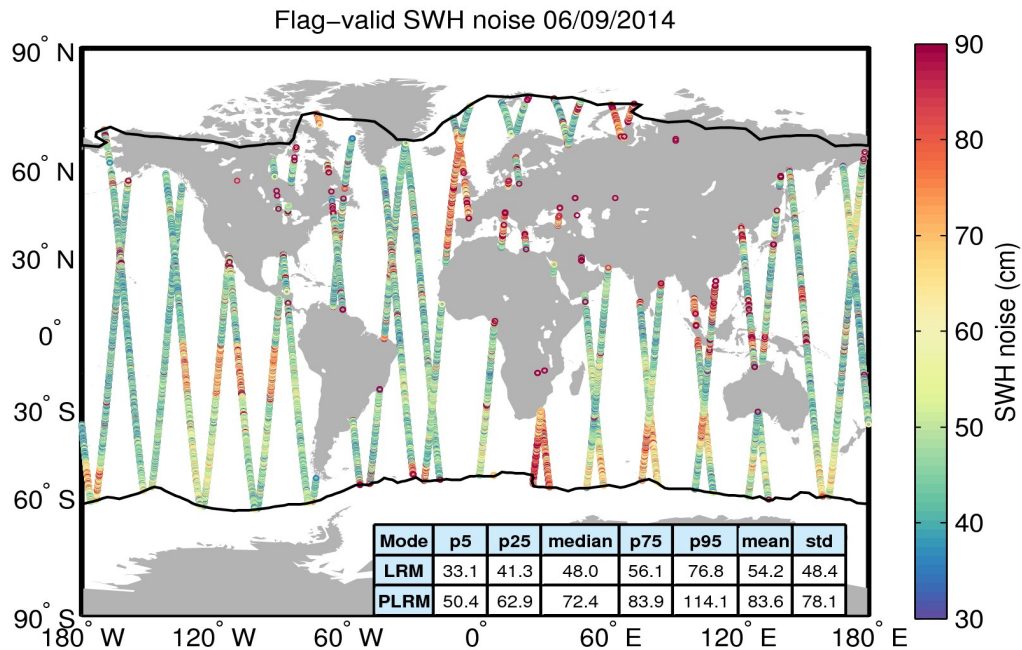
Figure 18. Geographical distribution of flag-valid 20-Hz SWH measurement noise over oceans and lakes for 06/09/2014. The statistical values shown in the table refer to the SWH noise and are calculated separately for LRM and PLRM regions. Measurements taken over polar polygons have been excluded from the computation of the statistical values. The black lines mark the outer limit of the Arctic and Antarctic polar polygons.
