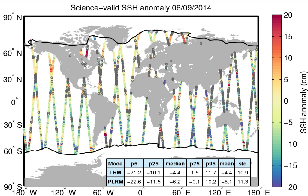
Figure 10. Geographical distribution of science-valid SSH anomaly data over oceans and lakes for 06/09/2014. The statistical values shown in the table refer to the SSH anomaly in cm and are calculated separately for LRM and PLRM regions. The black lines mark the outer limit of the Arctic and Antarctic polar polygons. Gray circles denote records that have been rejected based on the editing criteria described in Table 2.
