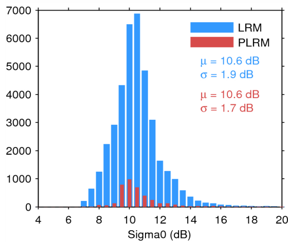
Figure 28. Histogram of science-valid sigma0 over oceans and lakes for LRM (blue) and PLRM (red) for 06/09/2014. The mean ( \mu ) and standard deviation ( \sigma ) are also shown. Note that values outside [4 20] dB are excluded from the histogram for the sake of readability but not from the computation of \mu and \sigma .
