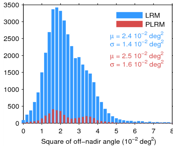
Figure 39. Histogram of flag-valid mispointing over oceans and lakes for LRM (blue) and PLRM (red) for 06/09/2014. Only positive values have been considered. The mean ( \mu ) and standard deviation ( \sigma ) are also shown. Note that values larger than 8 \cdot 10^{-2} \text{ deg}^2 are excluded from the histogram for the sake of readability but not from the computation of \mu and \sigma .
