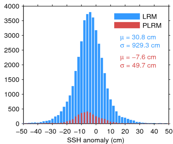
Figure 7. Histogram of flag-valid SSH anomaly over oceans and lakes for LRM (blue) and PLRM (red) for 06/09/2014. The mean ( \mu ) and standard deviation ( \sigma ) are also shown. Note that values outside [-50\ 50] cm are excluded from the histogram for the sake of readability but not from the computation of \mu and \sigma .
