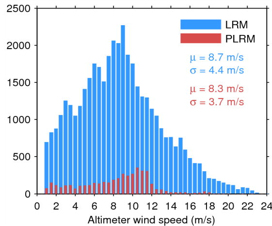
Figure 33. Histogram of flag-valid wind over oceans and lakes for LRM (blue) and PLRM (red) for 06/09/2014. The mean ( \mu ) and standard deviation ( \sigma ) are also shown. Note that values larger than 24 m/s are excluded from the histogram for the sake of readability but not from the computation of \mu and \sigma .
