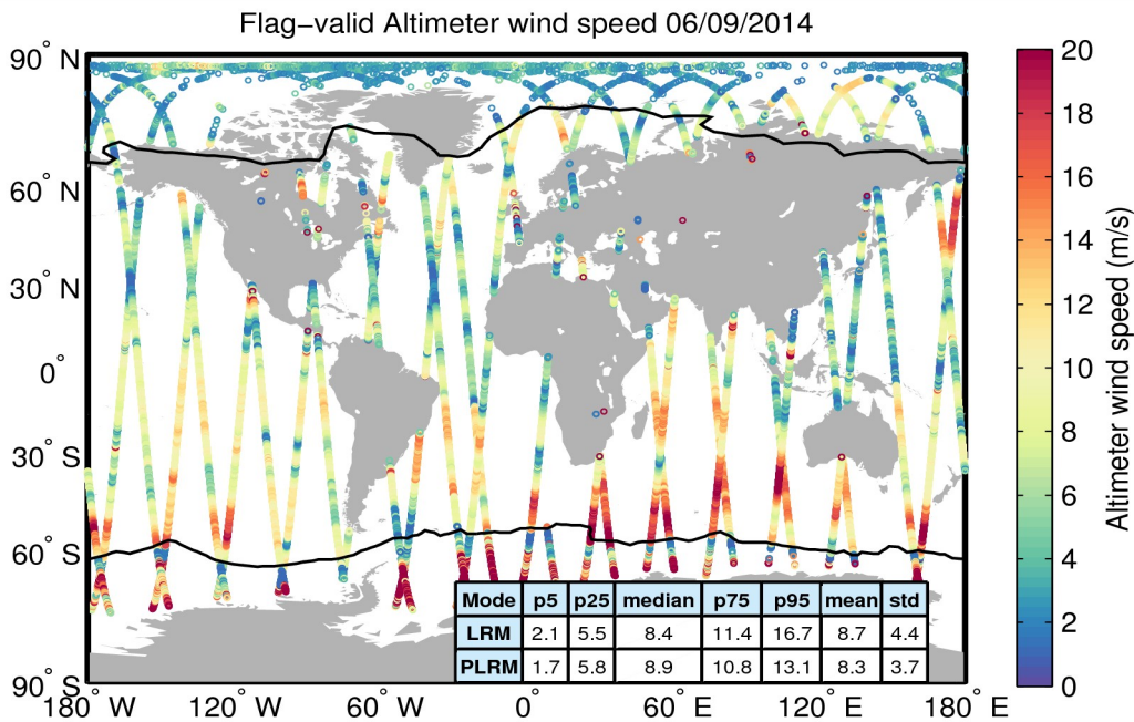
Figure 31. Geographical distribution of flag-valid wind data over oceans and lakes for 06/09/2014. The statistical values shown in the table refer to the wind in m/s and are calculated separately for LRM and PLRM regions. Measurements taken over polar polygons have been excluded from the computation of the statistical values. The black lines mark the outer limit of the Arctic and Antarctic polar polygons.
