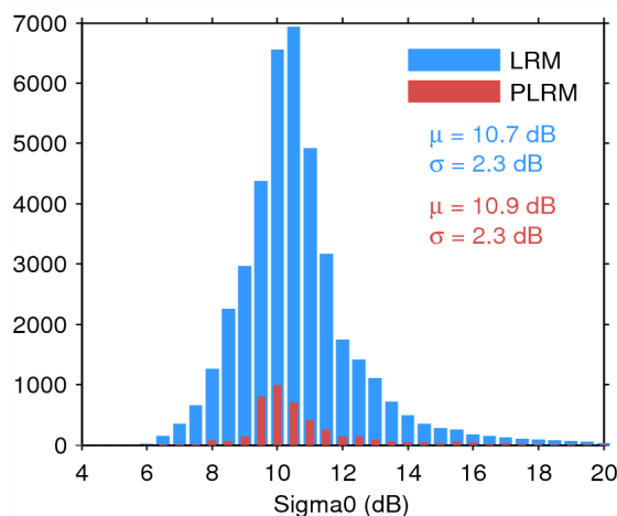
Figure 25. Histogram of flag-valid sigma0 over oceans and lakes for LRM (blue) and PLRM (red) for 06/09/2014. The mean ( \mu ) and standard deviation ( \sigma ) are also shown. Note that values outside [4 20] dB are excluded from the histogram for the sake of readability but not from the computation of \mu and \sigma .
