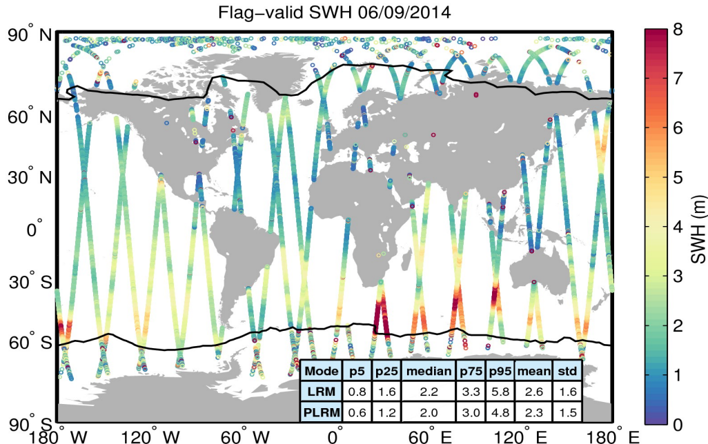
Figure 15. Geographical distribution of flag-valid SWH data over oceans and lakes for 06/09/2014. The statistical values shown in the table refer to the SWH in m and are calculated separately for LRM and PLRM regions. Measurements taken over polar polygons have been excluded from the computation of the statistical values. The black lines mark the outer limit of the Arctic and Antarctic polar polygons.
