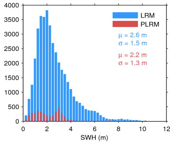
Figure 20. Histogram of science-valid SWH over oceans and lakes for LRM (blue) and PLRM (red) for 06/09/2014. The mean ( \mu ) and standard deviation ( \sigma ) are also shown. Note that values larger than 12 m are excluded from the histogram for the sake of readability but not from the computation of \mu and \sigma .
