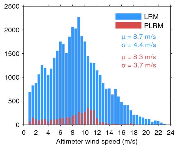
Figure 35. Histogram of science-valid wind over oceans and lakes for LRM (blue) and PLRM (red) for 06/09/2014. The mean ( \mu ) and standard deviation ( \sigma ) are also shown. Note that values larger than 24 m/s are excluded from the histogram for the sake of readability but not from the computation of \mu and \sigma .
