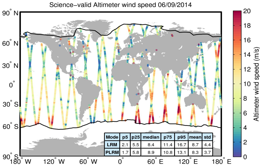
Figure 34. Geographical distribution of science-valid wind data over oceans and lakes for 06/09/2014. The statistical values shown in the table refer to the wind in m/s and are calculated separately for LRM and PLRM regions. The black lines mark the outer limit of the Arctic and Antarctic polar polygons. Gray circles denote records that have been rejected based on the editing criteria described in Table 5.
