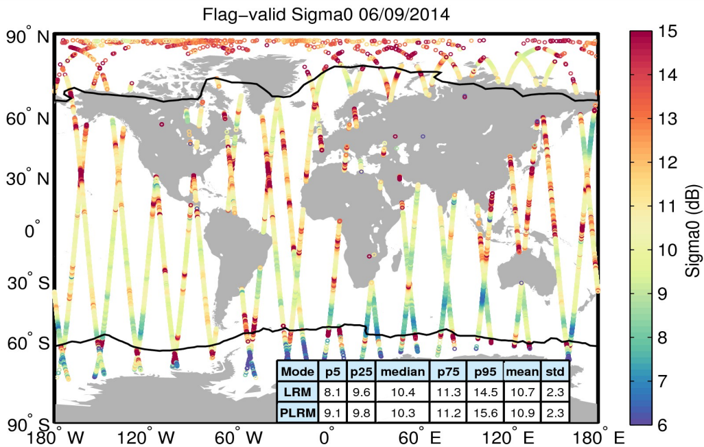
Figure 23. Geographical distribution of flag-valid sigma0 data over oceans and lakes for 06/09/2014. The statistical values shown in the table refer to the sigma0 in dB and are calculated separately for LRM and PLRM regions. Measurements taken over polar polygons have been excluded from the computation of the statistical values. The black lines mark the outer limit of the Arctic and Antarctic polar polygons.
