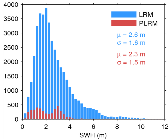
Figure 17. Histogram of flag-valid SWH over oceans and lakes for LRM (blue) and PLRM (red) for 06/09/2014. The mean ( \mu ) and standard deviation ( \sigma ) are also shown. Note that values larger than 12 m are excluded from the histogram for the sake of readability but not from the computation of \mu and \sigma .
