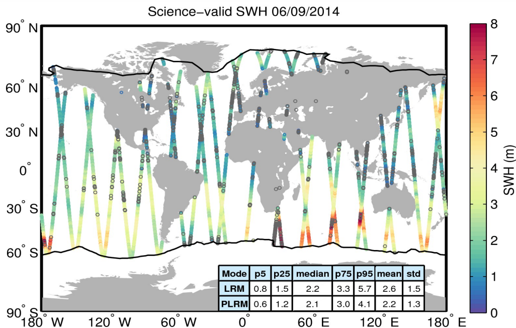
Figure 19. Geographical distribution of science-valid SWH data over oceans and lakes for 06/09/2014. The statistical values shown in the table refer to the SWH in m and are calculated separately for LRM and PLRM regions. The black lines mark the outer limit of the Arctic and Antarctic polar polygons. Gray circles denote records that have been rejected based on the editing criteria described in Table 3.
