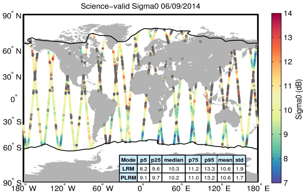
Figure 27. Geographical distribution of science-valid sigma0 data over oceans and lakes for 06/09/2014. The statistical values shown in the table refer to the sigma0 in dB and are calculated separately for LRM and PLRM regions. The black lines mark the outer limit of the Arctic and Antarctic polar polygons. Gray circles denote records that have been rejected based on the editing criteria described in Table 4.
