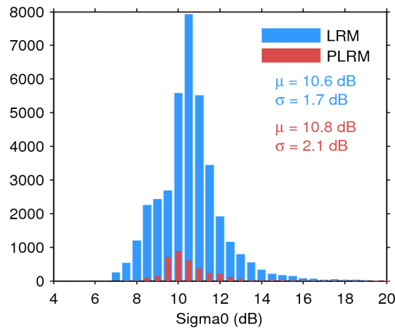
Figure 28. Histogram of science-valid sigma0 over oceans and lakes for LRM (blue) and PLRM (red) for 04/09/2014. The mean ( \mu ) and standard deviation ( \sigma ) are also shown. Note that values outside [4 20] dB are excluded from the histogram for the sake of readability but not from the computation of \mu and \sigma .
