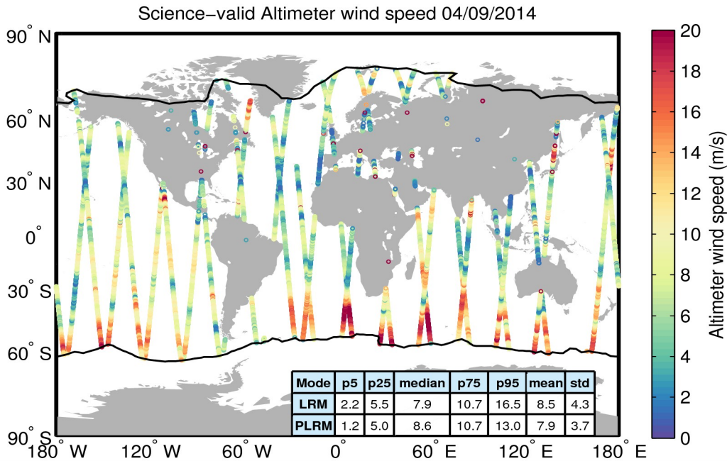
Figure 34. Geographical distribution of science-valid wind data over oceans and lakes for 04/09/2014. The statistical values shown in the table refer to the wind in m/s and are calculated separately for LRM and PLRM regions. The black lines mark the outer limit of the Arctic and Antarctic polar polygons. Gray circles denote records that have been rejected based on the editing criteria described in Table 5.
