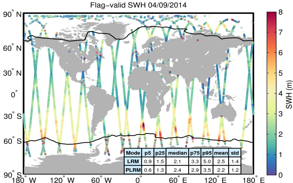
Figure 15. Geographical distribution of flag-valid SWH data over oceans and lakes for 04/09/2014. The statistical values shown in the table refer to the SWH in m and are calculated separately for LRM and PLRM regions. Measurements taken over polar polygons have been excluded from the computation of the statistical values. The black lines mark the outer limit of the Arctic and Antarctic polar polygons.
