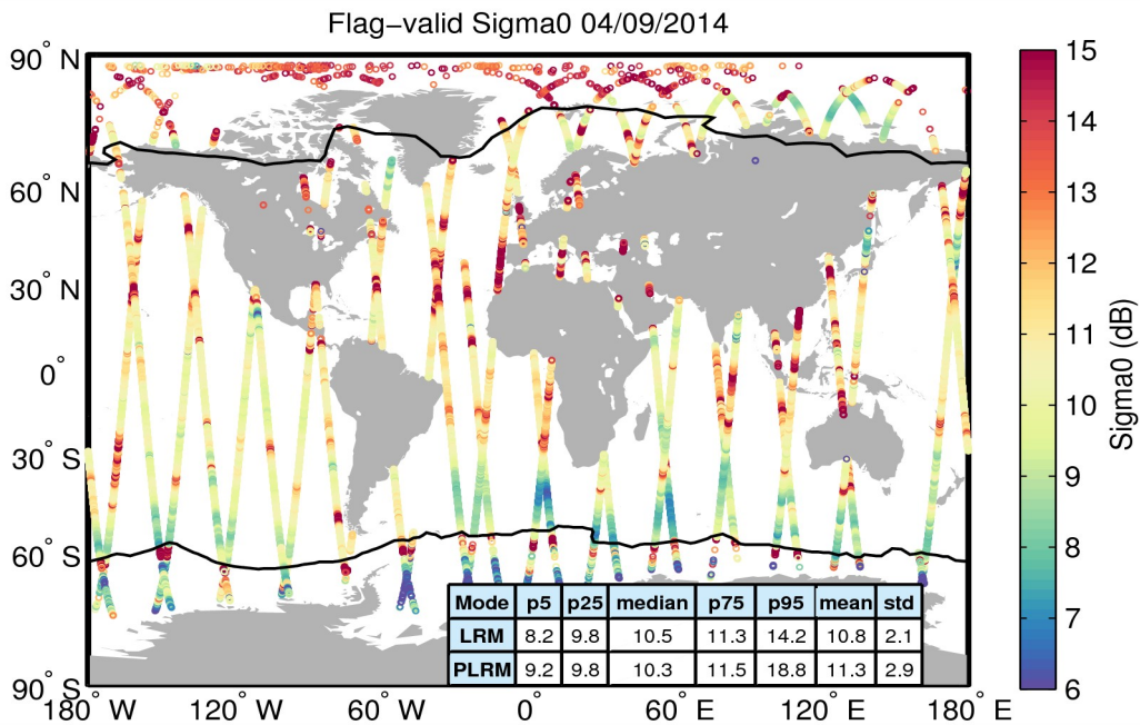
Figure 23. Geographical distribution of flag-valid sigma0 data over oceans and lakes for 04/09/2014. The statistical values shown in the table refer to the sigma0 in dB and are calculated separately for LRM and PLRM regions. Measurements taken over polar polygons have been excluded from the computation of the statistical values. The black lines mark the outer limit of the Arctic and Antarctic polar polygons.
