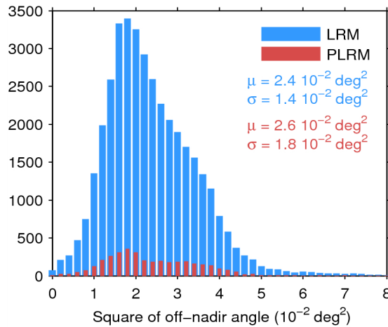
Figure 39. Histogram of flag-valid mispointing over oceans and lakes for LRM (blue) and PLRM (red) for 04/09/2014. Only positive values have been considered. The mean ( \mu ) and standard deviation ( \sigma ) are also shown. Note that values larger than 8 \cdot 10^{-2} \text{ deg}^2 are excluded from the histogram for the sake of readability but not from the computation of \mu and \sigma .
