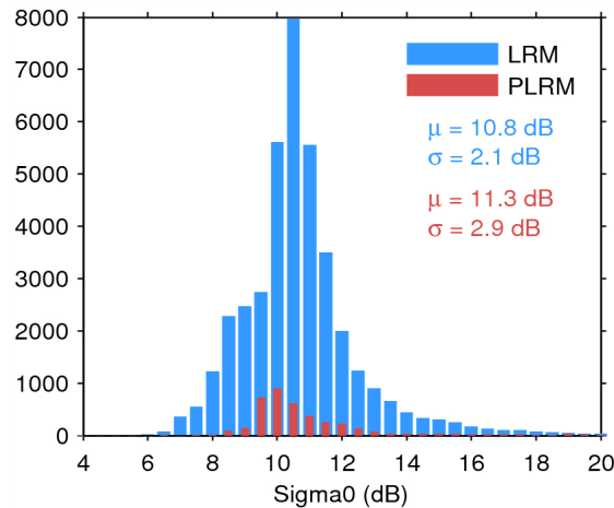
Figure 25. Histogram of flag-valid sigma0 over oceans and lakes for LRM (blue) and PLRM (red) for 04/09/2014. The mean ( \mu ) and standard deviation ( \sigma ) are also shown. Note that values outside [4 20] dB are excluded from the histogram for the sake of readability but not from the computation of \mu and \sigma .
