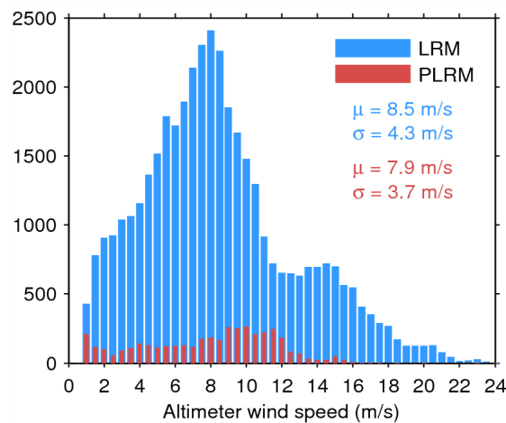
Figure 33. Histogram of flag-valid wind over oceans and lakes for LRM (blue) and PLRM (red) for 04/09/2014. The mean ( \mu ) and standard deviation ( \sigma ) are also shown. Note that values larger than 24 m/s are excluded from the histogram for the sake of readability but not from the computation of \mu and \sigma .
