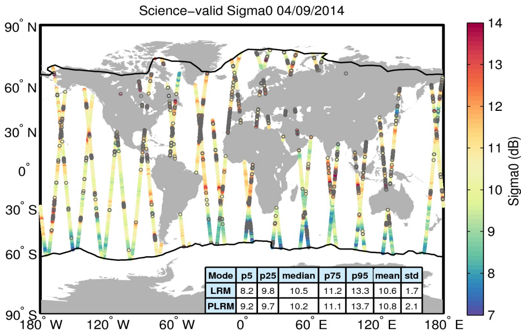
Figure 27. Geographical distribution of science-valid sigma0 data over oceans and lakes for 04/09/2014. The statistical values shown in the table refer to the sigma0 in dB and are calculated separately for LRM and PLRM regions. The black lines mark the outer limit of the Arctic and Antarctic polar polygons. Gray circles denote records that have been rejected based on the editing criteria described in Table 4.
