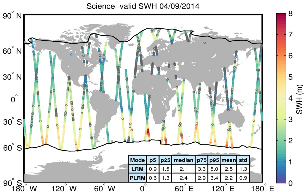
Figure 19. Geographical distribution of science-valid SWH data over oceans and lakes for 04/09/2014. The statistical values shown in the table refer to the SWH in m and are calculated separately for LRM and PLRM regions. The black lines mark the outer limit of the Arctic and Antarctic polar polygons. Gray circles denote records that have been rejected based on the editing criteria described in Table 3.
