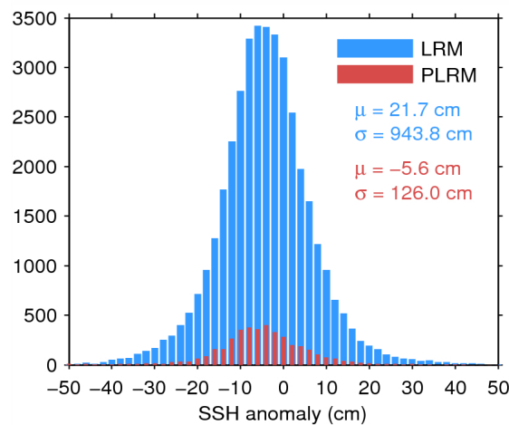
Figure 7. Histogram of flag-valid SSH anomaly over oceans and lakes for LRM (blue) and PLRM (red) for 04/09/2014. The mean ( \mu ) and standard deviation ( \sigma ) are also shown. Note that values outside [-50\ 50] cm are excluded from the histogram for the sake of readability but not from the computation of \mu and \sigma .
