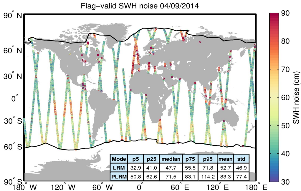
Figure 18. Geographical distribution of flag-valid 20-Hz SWH measurement noise over oceans and lakes for 04/09/2014. The statistical values shown in the table refer to the SWH noise and are calculated separately for LRM and PLRM regions. Measurements taken over polar polygons have been excluded from the computation of the statistical values. The black lines mark the outer limit of the Arctic and Antarctic polar polygons.
