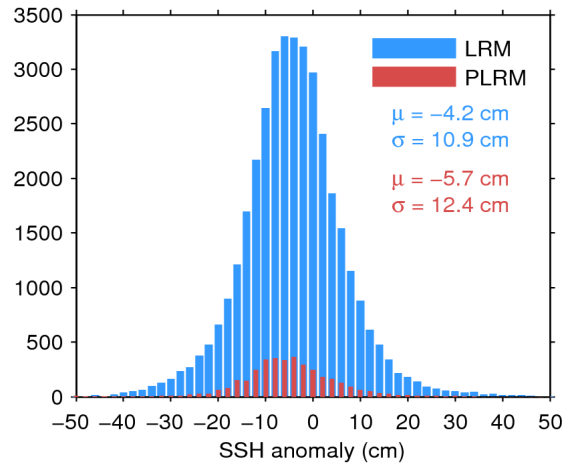
Figure 11. Histogram of science-valid SSH anomaly over oceans and lakes for LRM (blue) and PLRM (red) for 04/09/2014. The mean ( \mu ) and standard deviation ( \sigma ) are also shown. Note that values outside [-50\ 50] cm are excluded from the histogram for the sake of readability but not from the computation of \mu and \sigma .
