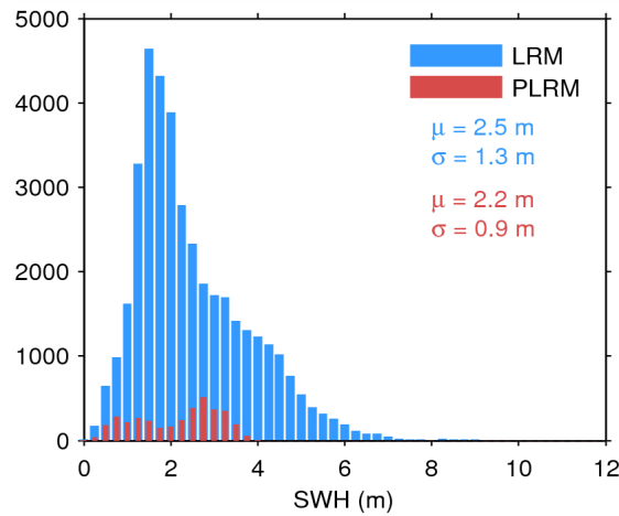
Figure 20. Histogram of science-valid SWH over oceans and lakes for LRM (blue) and PLRM (red) for 04/09/2014. The mean ( \mu ) and standard deviation ( \sigma ) are also shown. Note that values larger than 12 m are excluded from the histogram for the sake of readability but not from the computation of \mu and \sigma .
