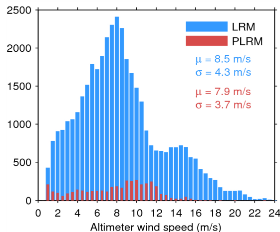
Figure 35. Histogram of science-valid wind over oceans and lakes for LRM (blue) and PLRM (red) for 04/09/2014. The mean ( \mu ) and standard deviation ( \sigma ) are also shown. Note that values larger than 24 m/s are excluded from the histogram for the sake of readability but not from the computation of \mu and \sigma .
