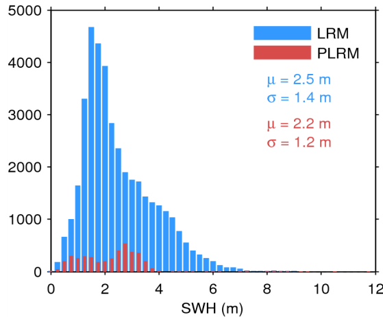
Figure 17. Histogram of flag-valid SWH over oceans and lakes for LRM (blue) and PLRM (red) for 04/09/2014. The mean ( \mu ) and standard deviation ( \sigma ) are also shown. Note that values larger than 12 m are excluded from the histogram for the sake of readability but not from the computation of \mu and \sigma .
