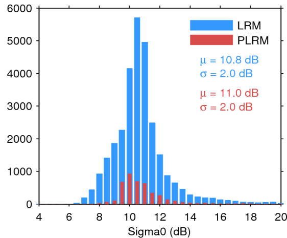
Figure 25. Histogram of flag-valid sigma0 over oceans and lakes for LRM (blue) and PLRM (red) for 03/09/2014. The mean ( \mu ) and standard deviation ( \sigma ) are also shown. Note that values outside [4 20] dB are excluded from the histogram for the sake of readability but not from the computation of \mu and \sigma .
