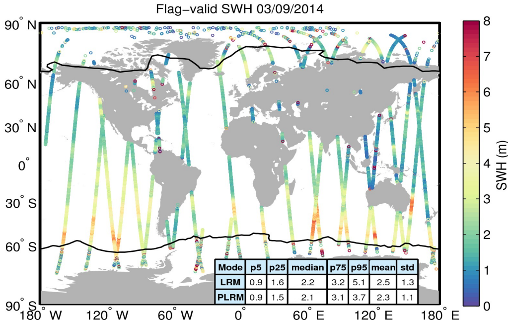
Figure 15. Geographical distribution of flag-valid SWH data over oceans and lakes for 03/09/2014. The statistical values shown in the table refer to the SWH in m and are calculated separately for LRM and PLRM regions. Measurements taken over polar polygons have been excluded from the computation of the statistical values. The black lines mark the outer limit of the Arctic and Antarctic polar polygons.
