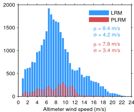
Figure 35. Histogram of science-valid wind over oceans and lakes for LRM (blue) and PLRM (red) for 03/09/2014. The mean ( \mu ) and standard deviation ( \sigma ) are also shown. Note that values larger than 24 m/s are excluded from the histogram for the sake of readability but not from the computation of \mu and \sigma .
