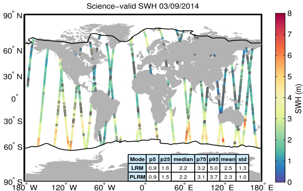
Figure 19. Geographical distribution of science-valid SWH data over oceans and lakes for 03/09/2014. The statistical values shown in the table refer to the SWH in m and are calculated separately for LRM and PLRM regions. The black lines mark the outer limit of the Arctic and Antarctic polar polygons. Gray circles denote records that have been rejected based on the editing criteria described in Table 3.
