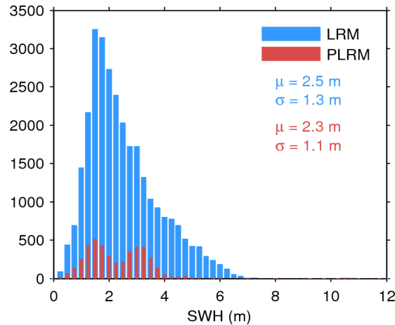
Figure 17. Histogram of flag-valid SWH over oceans and lakes for LRM (blue) and PLRM (red) for 03/09/2014. The mean ( \mu ) and standard deviation ( \sigma ) are also shown. Note that values larger than 12 m are excluded from the histogram for the sake of readability but not from the computation of \mu and \sigma .
