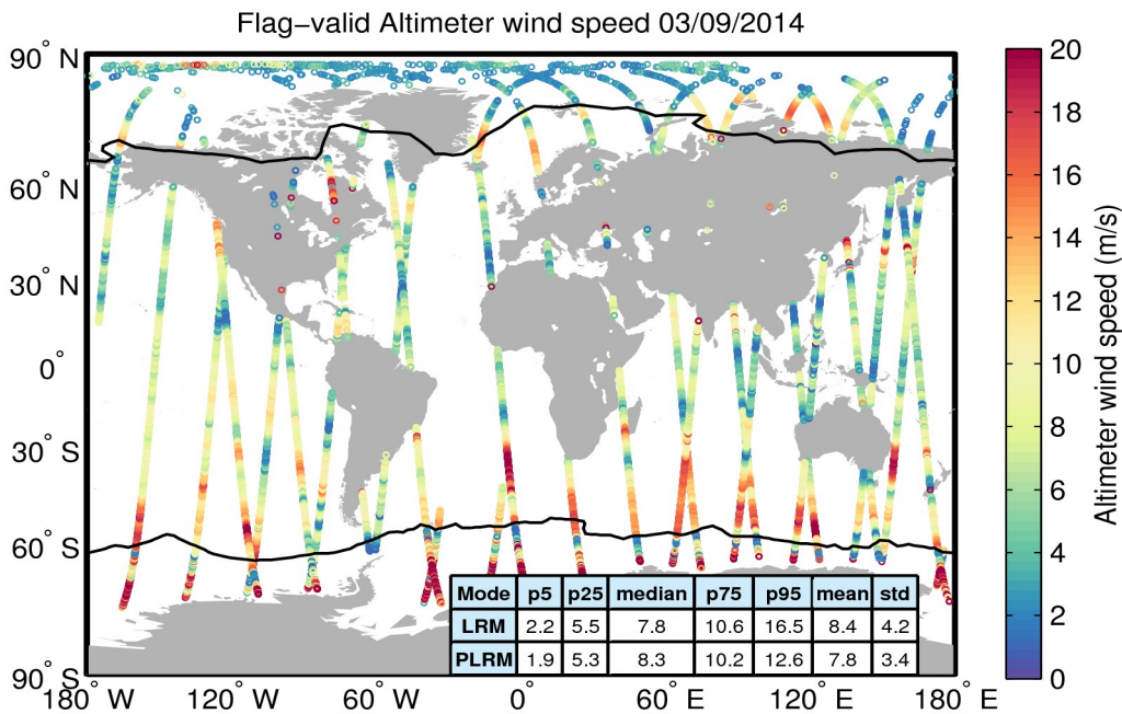
Figure 31. Geographical distribution of flag-valid wind data over oceans and lakes for 03/09/2014. The statistical values shown in the table refer to the wind in m/s and are calculated separately for LRM and PLRM regions. Measurements taken over polar polygons have been excluded from the computation of the statistical values. The black lines mark the outer limit of the Arctic and Antarctic polar polygons.
