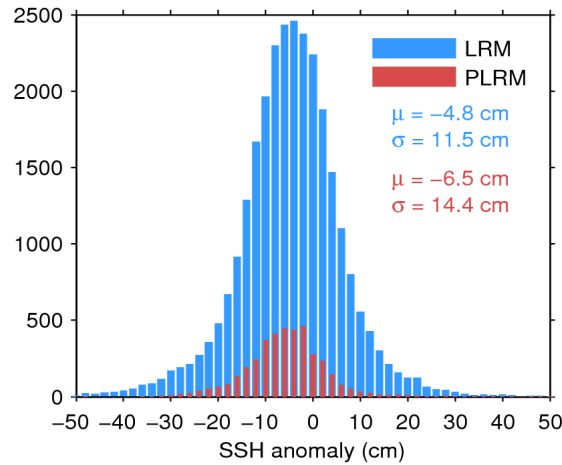
Figure 11. Histogram of science-valid SSH anomaly over oceans and lakes for LRM (blue) and PLRM (red) for 03/09/2014. The mean ( \mu ) and standard deviation ( \sigma ) are also shown. Note that values outside [-50 50] cm are excluded from the histogram for the sake of readability but not from the computation of \mu and \sigma .
