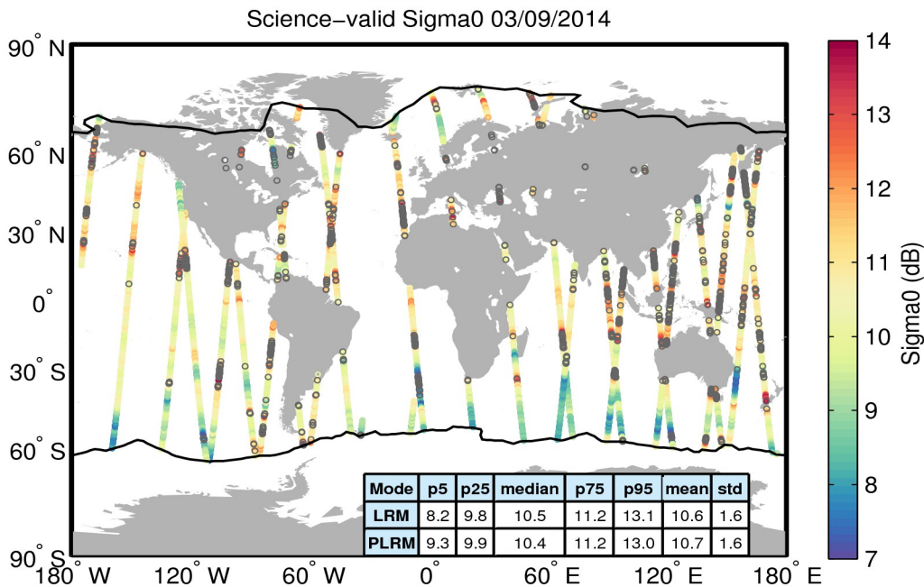
Figure 27. Geographical distribution of science-valid sigma0 data over oceans and lakes for 03/09/2014. The statistical values shown in the table refer to the sigma0 in dB and are calculated separately for LRM and PLRM regions. The black lines mark the outer limit of the Arctic and Antarctic polar polygons. Gray circles denote records that have been rejected based on the editing criteria described in Table 4.
