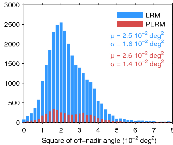
Figure 39. Histogram of flag-valid mispointing over oceans and lakes for LRM (blue) and PLRM (red) for 03/09/2014. Only positive values have been considered. The mean ( \mu ) and standard deviation ( \sigma ) are also shown. Note that values larger than 8 \cdot 10^{-2} \text{ deg}^2 are excluded from the histogram for the sake of readability but not from the computation of \mu and \sigma .
