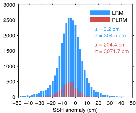
Figure 7. Histogram of flag-valid SSH anomaly over oceans and lakes for LRM (blue) and PLRM (red) for 03/09/2014. The mean ( \mu ) and standard deviation ( \sigma ) are also shown. Note that values outside [-50 \ 50] cm are excluded from the histogram for the sake of readability but not from the computation of \mu and \sigma .
