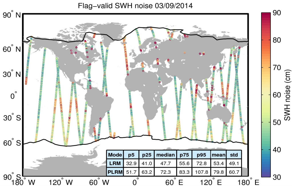
Figure 18. Geographical distribution of flag-valid 20-Hz SWH measurement noise over oceans and lakes for 03/09/2014. The statistical values shown in the table refer to the SWH noise and are calculated separately for LRM and PLRM regions. Measurements taken over polar polygons have been excluded from the computation of the statistical values. The black lines mark the outer limit of the Arctic and Antarctic polar polygons.
