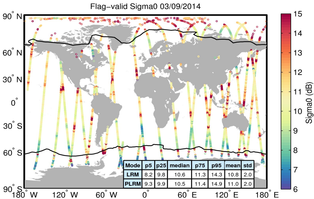
Figure 23. Geographical distribution of flag-valid sigma0 data over oceans and lakes for 03/09/2014. The statistical values shown in the table refer to the sigma0 in dB and are calculated separately for LRM and PLRM regions. Measurements taken over polar polygons have been excluded from the computation of the statistical values. The black lines mark the outer limit of the Arctic and Antarctic polar polygons.
