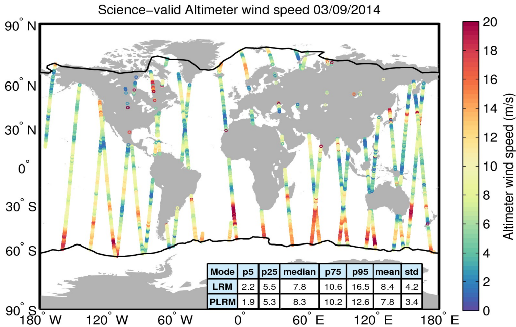
Figure 34. Geographical distribution of science-valid wind data over oceans and lakes for 03/09/2014. The statistical values shown in the table refer to the wind in m/s and are calculated separately for LRM and PLRM regions. The black lines mark the outer limit of the Arctic and Antarctic polar polygons. Gray circles denote records that have been rejected based on the editing criteria described in Table 5.
