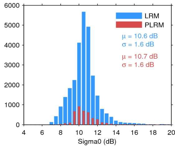
Figure 28. Histogram of science-valid sigma0 over oceans and lakes for LRM (blue) and PLRM (red) for 03/09/2014. The mean ( \mu ) and standard deviation ( \sigma ) are also shown. Note that values outside [4 20] dB are excluded from the histogram for the sake of readability but not from the computation of \mu and \sigma .
