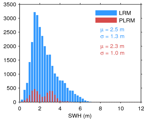
Figure 20. Histogram of science-valid SWH over oceans and lakes for LRM (blue) and PLRM (red) for 03/09/2014. The mean ( \mu ) and standard deviation ( \sigma ) are also shown. Note that values larger than 12 m are excluded from the histogram for the sake of readability but not from the computation of \mu and \sigma .
