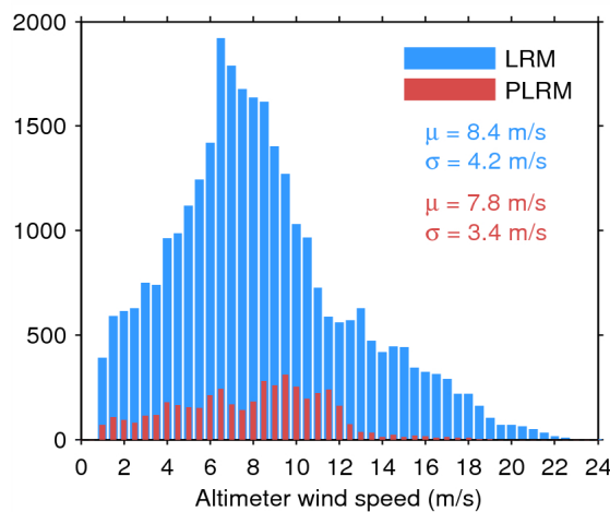
Figure 33. Histogram of flag-valid wind over oceans and lakes for LRM (blue) and PLRM (red) for 03/09/2014. The mean ( \mu ) and standard deviation ( \sigma ) are also shown. Note that values larger than 24 m/s are excluded from the histogram for the sake of readability but not from the computation of \mu and \sigma .
