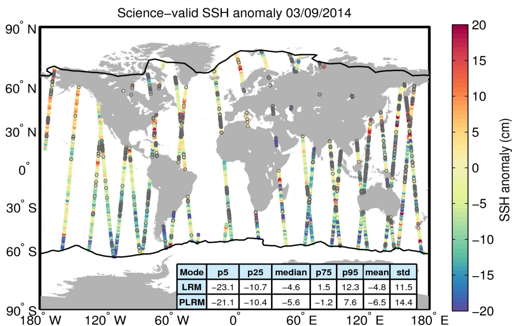
Figure 10. Geographical distribution of science-valid SSH anomaly data over oceans and lakes for 03/09/2014. The statistical values shown in the table refer to the SSH anomaly in cm and are calculated separately for LRM and PLRM regions. The black lines mark the outer limit of the Arctic and Antarctic polar polygons. Gray circles denote records that have been rejected based on the editing criteria described in Table 2.
