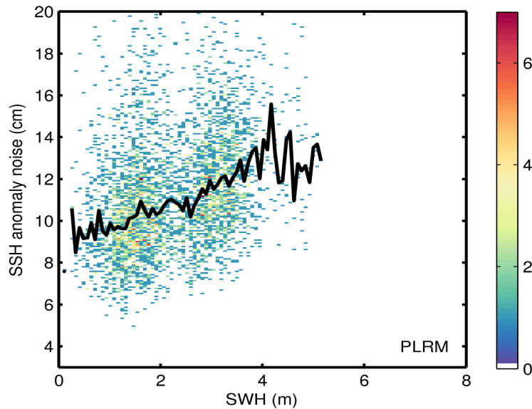
Figure 9. 2D histogram showing flag-valid SSH anomaly noise as a function of SWH for LRM (top) and PLRM (bottom) for 03/09/2014. The black line denotes the median SSH anomaly as a function of SWH.
