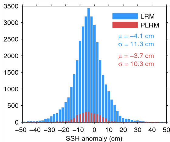
Figure 11. Histogram of science-valid SSH anomaly over oceans and lakes for LRM (blue) and PLRM (red) for 02/09/2014. The mean ( \mu ) and standard deviation ( \sigma ) are also shown. Note that values outside [-50 \ 50] cm are excluded from the histogram for the sake of readability but not from the computation of \mu and \sigma .
