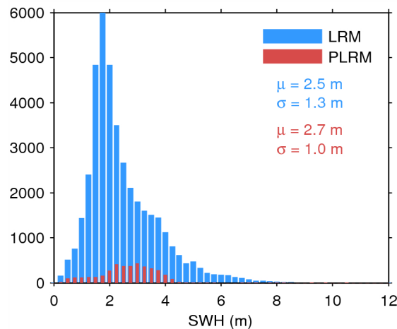
Figure 17. Histogram of flag-valid SWH over oceans and lakes for LRM (blue) and PLRM (red) for 02/09/2014. The mean ( \mu ) and standard deviation ( \sigma ) are also shown. Note that values larger than 12 m are excluded from the histogram for the sake of readability but not from the computation of \mu and \sigma .
