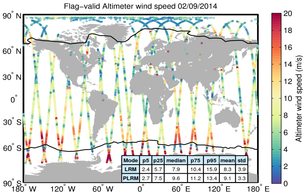
Figure 31. Geographical distribution of flag-valid wind data over oceans and lakes for 02/09/2014. The statistical values shown in the table refer to the wind in m/s and are calculated separately for LRM and PLRM regions. Measurements taken over polar polygons have been excluded from the computation of the statistical values. The black lines mark the outer limit of the Arctic and Antarctic polar polygons.
