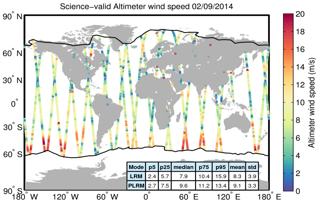
Figure 34. Geographical distribution of science-valid wind data over oceans and lakes for 02/09/2014. The statistical values shown in the table refer to the wind in m/s and are calculated separately for LRM and PLRM regions. The black lines mark the outer limit of the Arctic and Antarctic polar polygons. Gray circles denote records that have been rejected based on the editing criteria described in Table 5.
