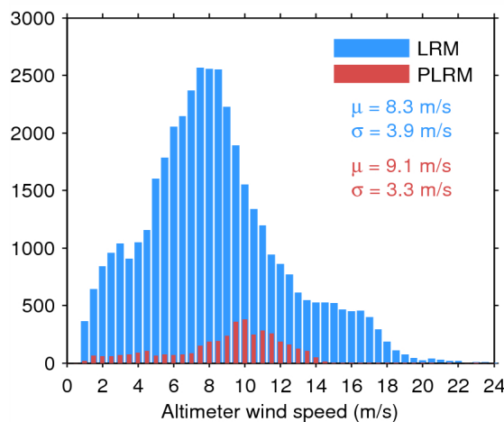
Figure 35. Histogram of science-valid wind over oceans and lakes for LRM (blue) and PLRM (red) for 02/09/2014. The mean ( \mu ) and standard deviation ( \sigma ) are also shown. Note that values larger than 24 m/s are excluded from the histogram for the sake of readability but not from the computation of \mu and \sigma .
