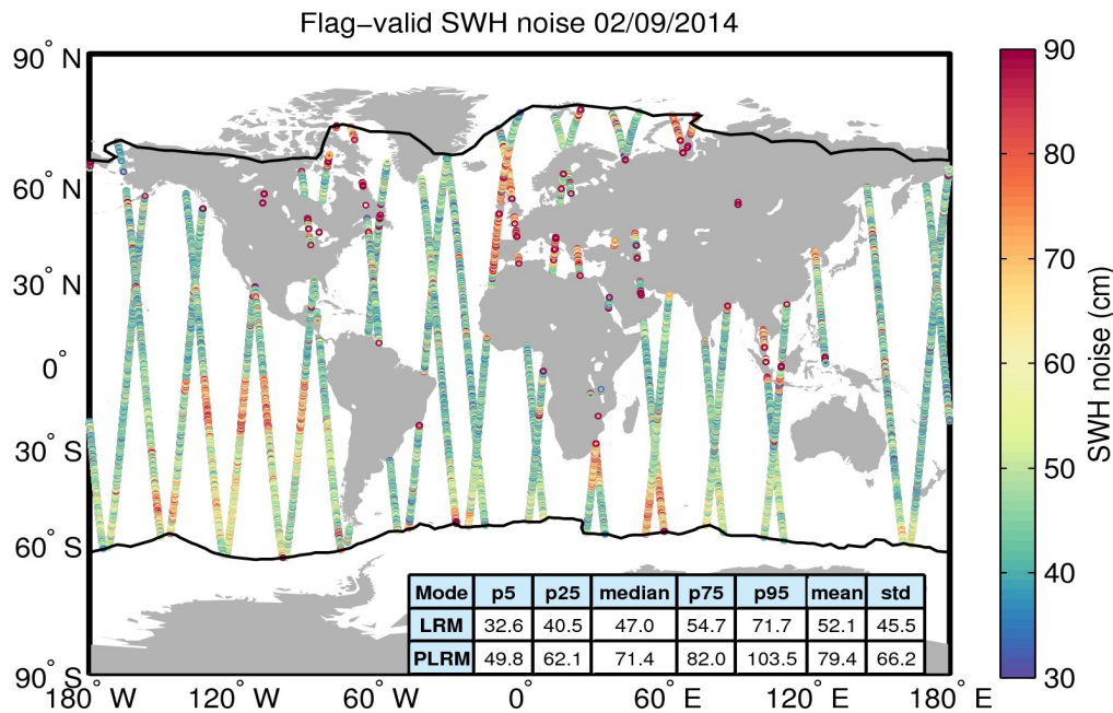
Figure 18. Geographical distribution of flag-valid 20-Hz SWH measurement noise over oceans and lakes for 02/09/2014. The statistical values shown in the table refer to the SWH noise and are calculated separately for LRM and PLRM regions. Measurements taken over polar polygons have been excluded from the computation of the statistical values. The black lines mark the outer limit of the Arctic and Antarctic polar polygons.
