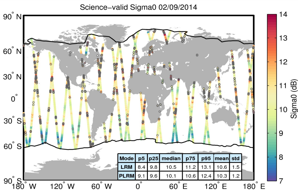
Figure 27. Geographical distribution of science-valid sigma0 data over oceans and lakes for 02/09/2014. The statistical values shown in the table refer to the sigma0 in dB and are calculated separately for LRM and PLRM regions. The black lines mark the outer limit of the Arctic and Antarctic polar polygons. Gray circles denote records that have been rejected based on the editing criteria described in Table 4.
