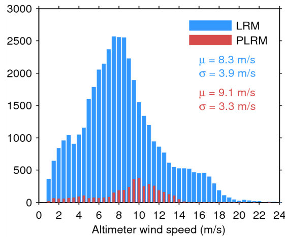
Figure 33. Histogram of flag-valid wind over oceans and lakes for LRM (blue) and PLRM (red) for 02/09/2014. The mean ( \mu ) and standard deviation ( \sigma ) are also shown. Note that values larger than 24 m/s are excluded from the histogram for the sake of readability but not from the computation of \mu and \sigma .
