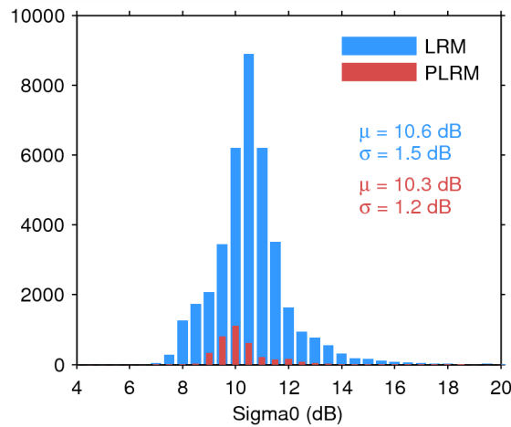
Figure 28. Histogram of science-valid sigma0 over oceans and lakes for LRM (blue) and PLRM (red) for 02/09/2014. The mean ( \mu ) and standard deviation ( \sigma ) are also shown. Note that values outside [4 20] dB are excluded from the histogram for the sake of readability but not from the computation of \mu and \sigma .
