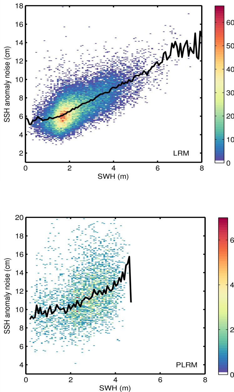
Figure 9. 2D histogram showing flag-valid SSH anomaly noise as a function of SWH for LRM (top) and PLRM (bottom) for 02/09/2014. The black line denotes the median SSH anomaly as a function of SWH.
