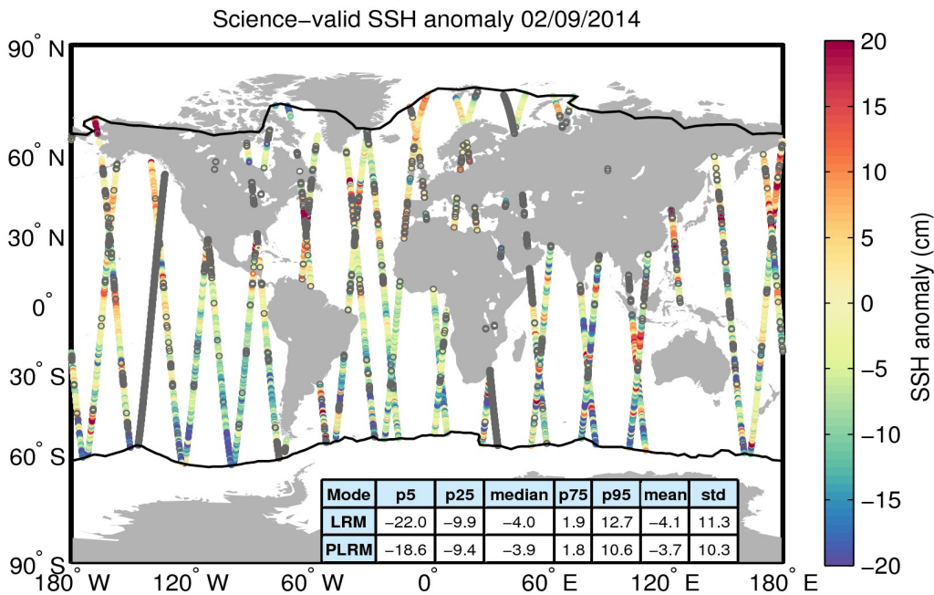
Figure 10. Geographical distribution of science-valid SSH anomaly data over oceans and lakes for 02/09/2014. The statistical values shown in the table refer to the SSH anomaly in cm and are calculated separately for LRM and PLRM regions. The black lines mark the outer limit of the Arctic and Antarctic polar polygons. Gray circles denote records that have been rejected based on the editing criteria described in Table 2.
