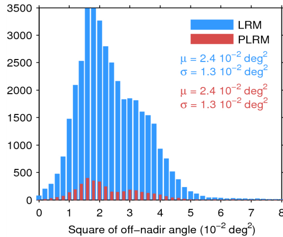
Figure 39. Histogram of flag-valid mispointing over oceans and lakes for LRM (blue) and PLRM (red) for 02/09/2014. Only positive values have been considered. The mean ( \mu ) and standard deviation ( \sigma ) are also shown. Note that values larger than 8 \cdot 10^{-2} \text{ deg}^2 are excluded from the histogram for the sake of readability but not from the computation of \mu and \sigma .
