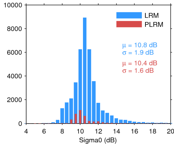
Figure 25. Histogram of flag-valid sigma0 over oceans and lakes for LRM (blue) and PLRM (red) for 02/09/2014. The mean ( \mu ) and standard deviation ( \sigma ) are also shown. Note that values outside [4 20] dB are excluded from the histogram for the sake of readability but not from the computation of \mu and \sigma .
