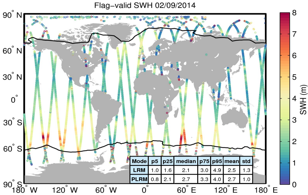
Figure 15. Geographical distribution of flag-valid SWH data over oceans and lakes for 02/09/2014. The statistical values shown in the table refer to the SWH in m and are calculated separately for LRM and PLRM regions. Measurements taken over polar polygons have been excluded from the computation of the statistical values. The black lines mark the outer limit of the Arctic and Antarctic polar polygons.
