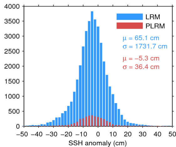
Figure 7. Histogram of flag-valid SSH anomaly over oceans and lakes for LRM (blue) and PLRM (red) for 02/09/2014. The mean ( \mu ) and standard deviation ( \sigma ) are also shown. Note that values outside [-50 \ 50] cm are excluded from the histogram for the sake of readability but not from the computation of \mu and \sigma .
