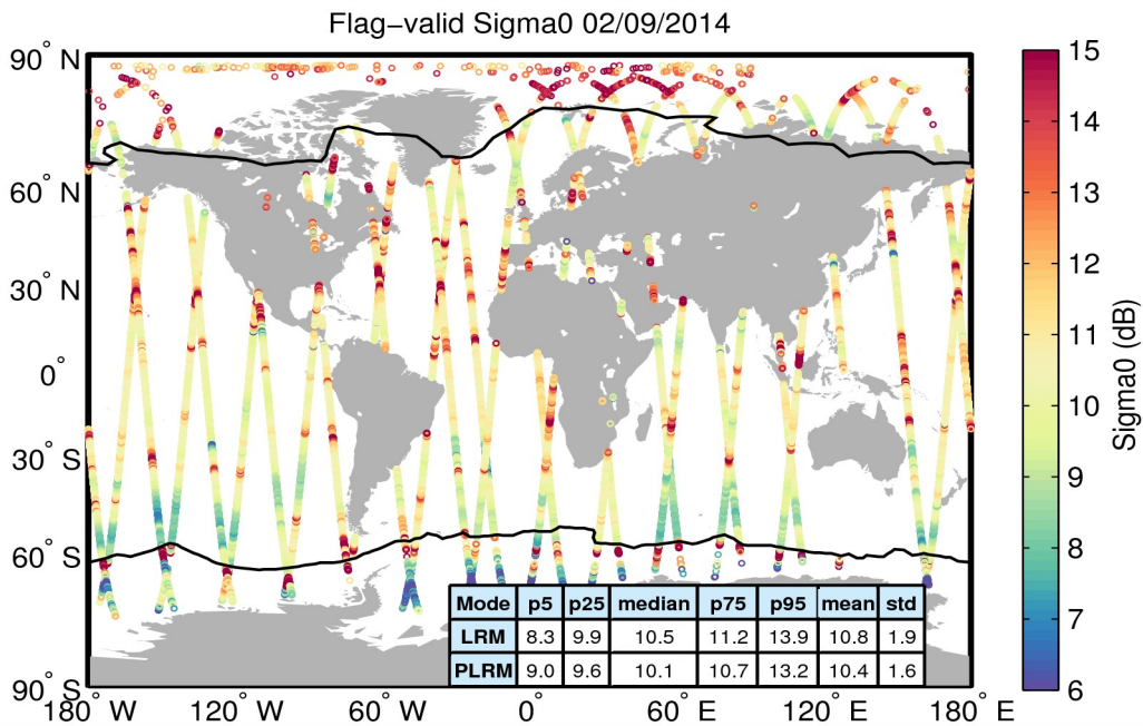
Figure 23. Geographical distribution of flag-valid sigma0 data over oceans and lakes for 02/09/2014. The statistical values shown in the table refer to the sigma0 in dB and are calculated separately for LRM and PLRM regions. Measurements taken over polar polygons have been excluded from the computation of the statistical values. The black lines mark the outer limit of the Arctic and Antarctic polar polygons.
