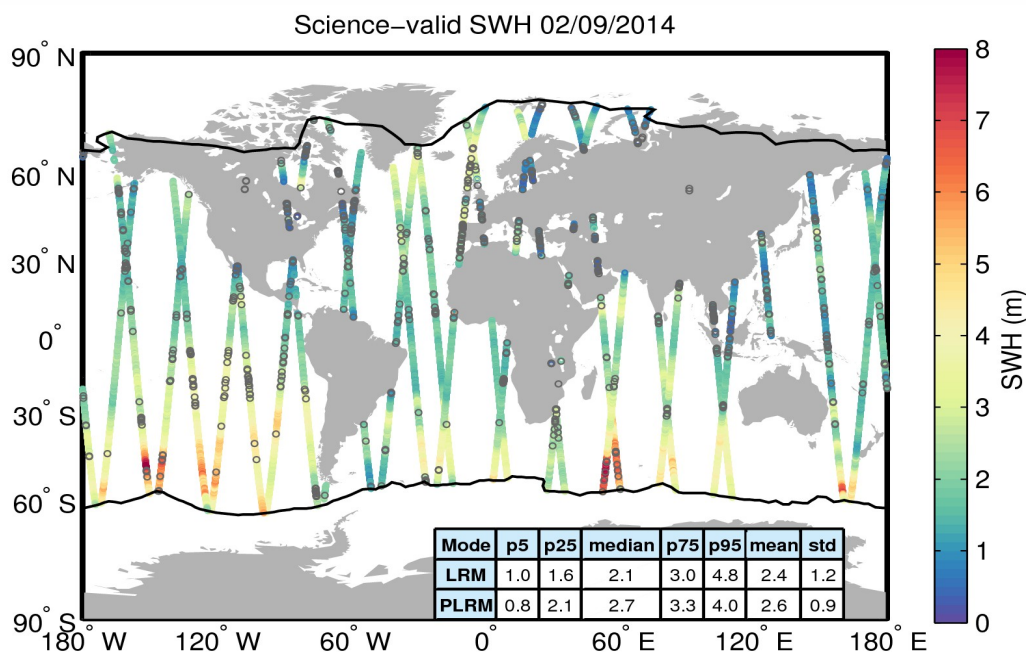
Figure 19. Geographical distribution of science-valid SWH data over oceans and lakes for 02/09/2014. The statistical values shown in the table refer to the SWH in m and are calculated separately for LRM and PLRM regions. The black lines mark the outer limit of the Arctic and Antarctic polar polygons. Gray circles denote records that have been rejected based on the editing criteria described in Table 3.
