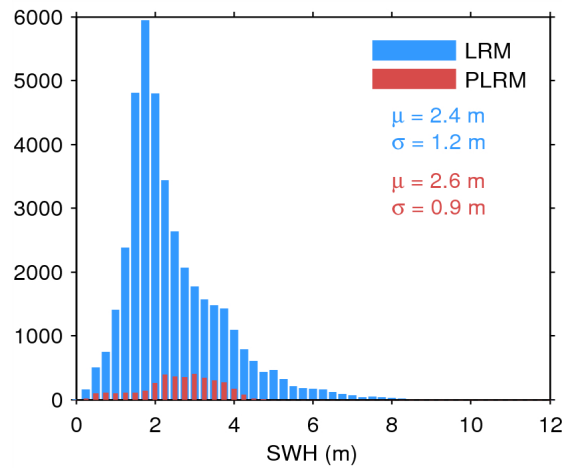
Figure 20. Histogram of science-valid SWH over oceans and lakes for LRM (blue) and PLRM (red) for 02/09/2014. The mean ( \mu ) and standard deviation ( \sigma ) are also shown. Note that values larger than 12 m are excluded from the histogram for the sake of readability but not from the computation of \mu and \sigma .
