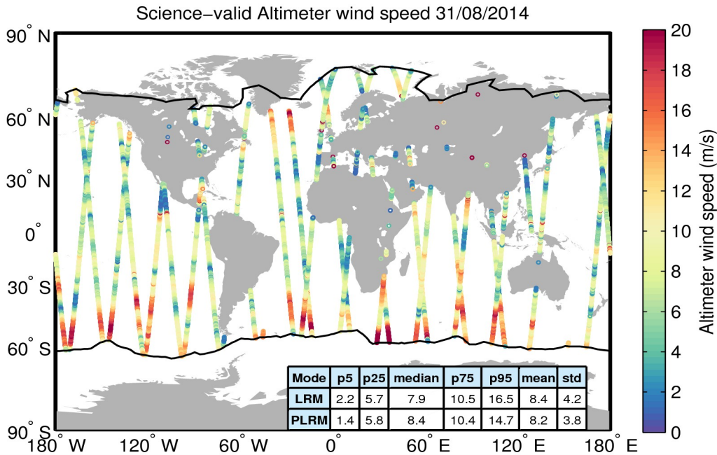
Figure 34. Geographical distribution of science-valid wind data over oceans and lakes for 31/08/2014. The statistical values shown in the table refer to the wind in m/s and are calculated separately for LRM and PLRM regions. The black lines mark the outer limit of the Arctic and Antarctic polar polygons. Gray circles denote records that have been rejected based on the editing criteria described in Table 5.
