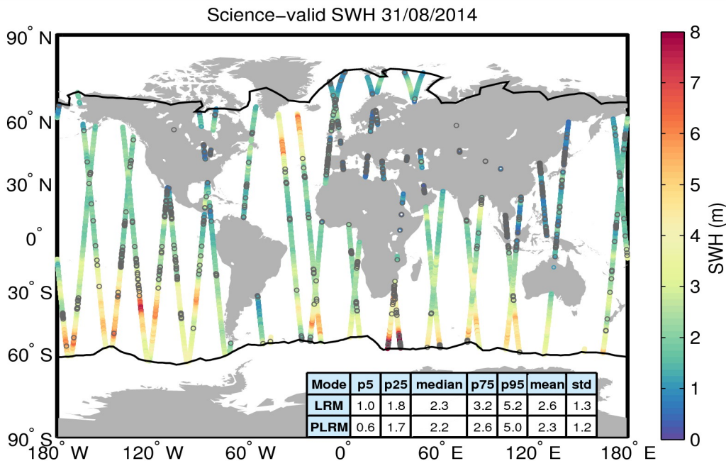
Figure 19. Geographical distribution of science-valid SWH data over oceans and lakes for 31/08/2014. The statistical values shown in the table refer to the SWH in m and are calculated separately for LRM and PLRM regions. The black lines mark the outer limit of the Arctic and Antarctic polar polygons. Gray circles denote records that have been rejected based on the editing criteria described in Table 3.
