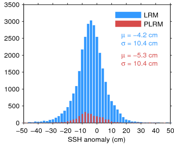
Figure 11. Histogram of science-valid SSH anomaly over oceans and lakes for LRM (blue) and PLRM (red) for 31/08/2014. The mean ( \mu ) and standard deviation ( \sigma ) are also shown. Note that values outside [-50\ 50] cm are excluded from the histogram for the sake of readability but not from the computation of \mu and \sigma .
