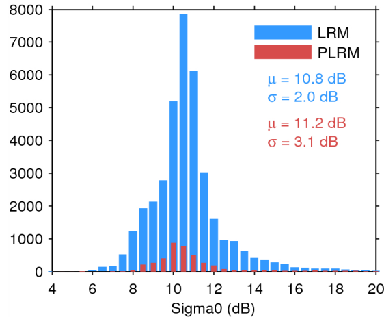
Figure 25. Histogram of flag-valid sigma0 over oceans and lakes for LRM (blue) and PLRM (red) for 31/08/2014. The mean ( \mu ) and standard deviation ( \sigma ) are also shown. Note that values outside [4 20] dB are excluded from the histogram for the sake of readability but not from the computation of \mu and \sigma .
