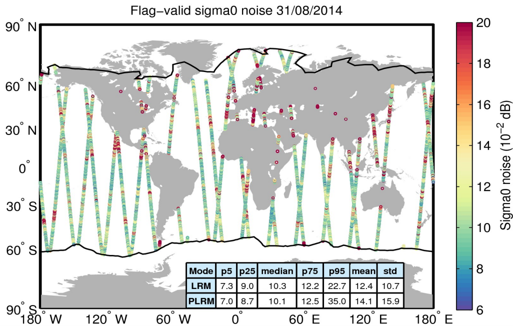
Figure 26. Geographical distribution of flag-valid 20-Hz sigma0 measurement noise over oceans and lakes for 31/08/2014. The statistical values shown in the table refer to the sigma0 noise and are calculated separately for LRM and PLRM regions. Measurements taken over polar polygons have been excluded from the computation of the statistical values. The black lines mark the outer limit of the Arctic and Antarctic polar polygons.
