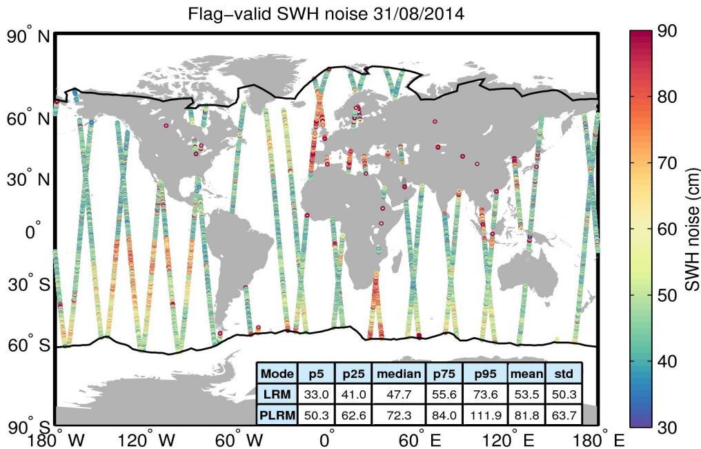
Figure 18. Geographical distribution of flag-valid 20-Hz SWH measurement noise over oceans and lakes for 31/08/2014. The statistical values shown in the table refer to the SWH noise and are calculated separately for LRM and PLRM regions. Measurements taken over polar polygons have been excluded from the computation of the statistical values. The black lines mark the outer limit of the Arctic and Antarctic polar polygons.
