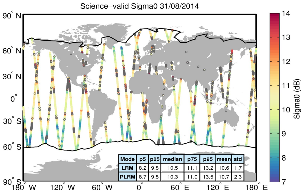
Figure 27. Geographical distribution of science-valid sigma0 data over oceans and lakes for 31/08/2014. The statistical values shown in the table refer to the sigma0 in dB and are calculated separately for LRM and PLRM regions. The black lines mark the outer limit of the Arctic and Antarctic polar polygons. Gray circles denote records that have been rejected based on the editing criteria described in Table 4.
