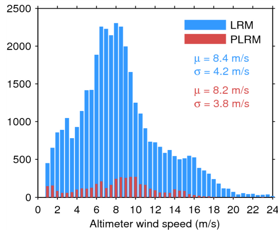
Figure 33. Histogram of flag-valid wind over oceans and lakes for LRM (blue) and PLRM (red) for 31/08/2014. The mean ( \mu ) and standard deviation ( \sigma ) are also shown. Note that values larger than 24 m/s are excluded from the histogram for the sake of readability but not from the computation of \mu and \sigma .
