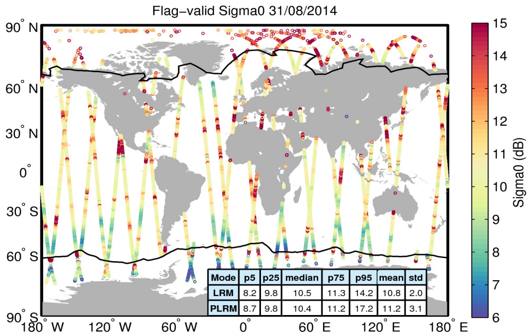
Figure 23. Geographical distribution of flag-valid sigma0 data over oceans and lakes for 31/08/2014. The statistical values shown in the table refer to the sigma0 in dB and are calculated separately for LRM and PLRM regions. Measurements taken over polar polygons have been excluded from the computation of the statistical values. The black lines mark the outer limit of the Arctic and Antarctic polar polygons.
