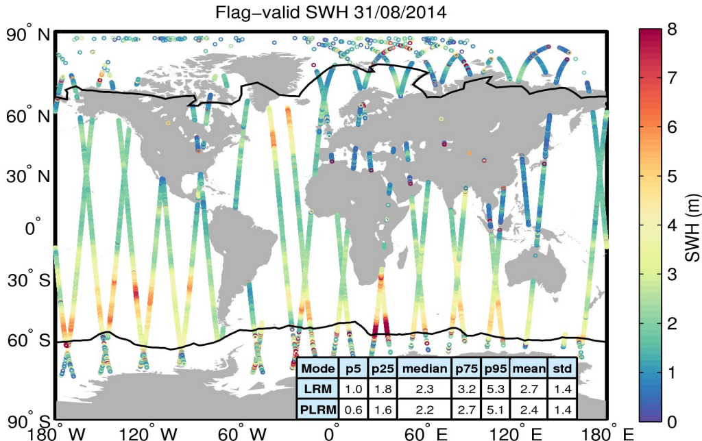
Figure 15. Geographical distribution of flag-valid SWH data over oceans and lakes for 31/08/2014. The statistical values shown in the table refer to the SWH in m and are calculated separately for LRM and PLRM regions. Measurements taken over polar polygons have been excluded from the computation of the statistical values. The black lines mark the outer limit of the Arctic and Antarctic polar polygons.
