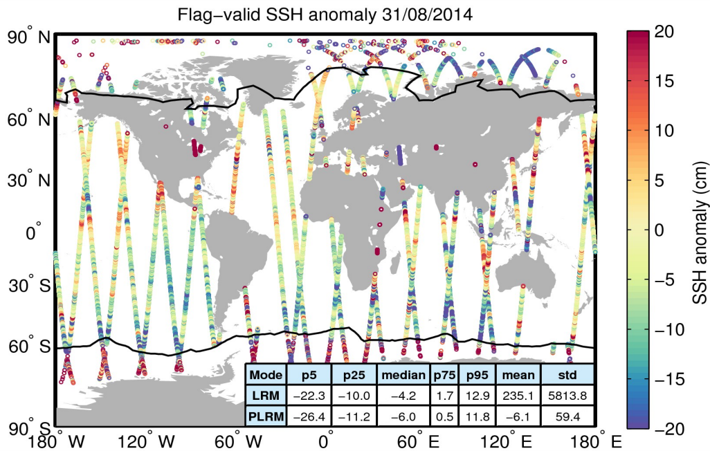
Figure 5. Geographical distribution of flag-valid 1-Hz SSH anomaly data over oceans and lakes for 31/08/2014. The statistical values shown in the table refer to the SSH anomaly in cm and are calculated separately for LRM and PLRM regions. Measurements taken over polar polygons have been excluded from the computation of the statistical values. The black lines mark the outer limit of the Arctic and Antarctic polar polygons.
