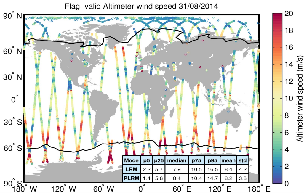
Figure 31. Geographical distribution of flag-valid wind data over oceans and lakes for 31/08/2014. The statistical values shown in the table refer to the wind in m/s and are calculated separately for LRM and PLRM regions. Measurements taken over polar polygons have been excluded from the computation of the statistical values. The black lines mark the outer limit of the Arctic and Antarctic polar polygons.
