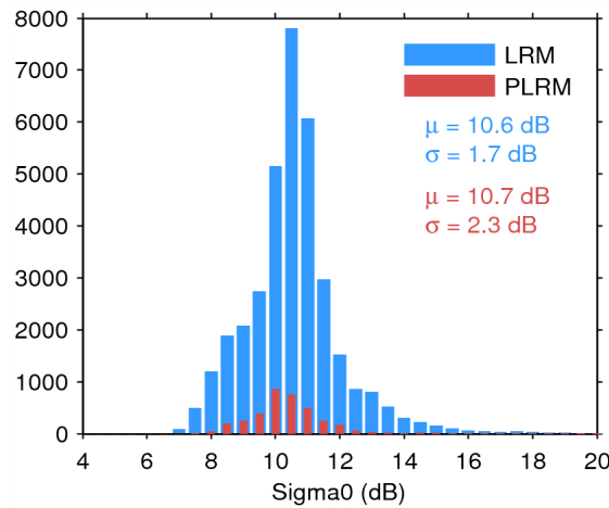
Figure 28. Histogram of science-valid sigma0 over oceans and lakes for LRM (blue) and PLRM (red) for 31/08/2014. The mean ( \mu ) and standard deviation ( \sigma ) are also shown. Note that values outside [4 20] dB are excluded from the histogram for the sake of readability but not from the computation of \mu and \sigma .
