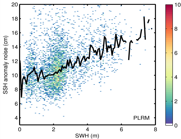
Figure 9. 2D histogram showing flag-valid SSH anomaly noise as a function of SWH for LRM (top) and PLRM (bottom) for 31/08/2014. The black line denotes the median SSH anomaly as a function of SWH.
