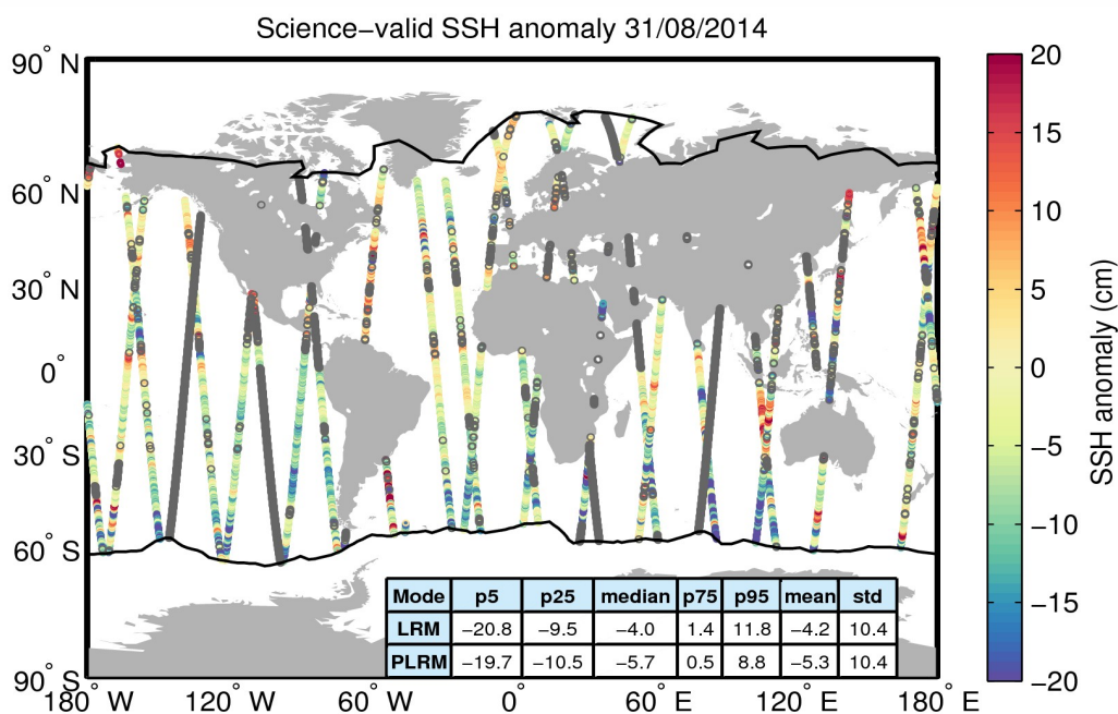
Figure 10. Geographical distribution of science-valid SSH anomaly data over oceans and lakes for 31/08/2014. The statistical values shown in the table refer to the SSH anomaly in cm and are calculated separately for LRM and PLRM regions. The black lines mark the outer limit of the Arctic and Antarctic polar polygons. Gray circles denote records that have been rejected based on the editing criteria described in Table 2.
