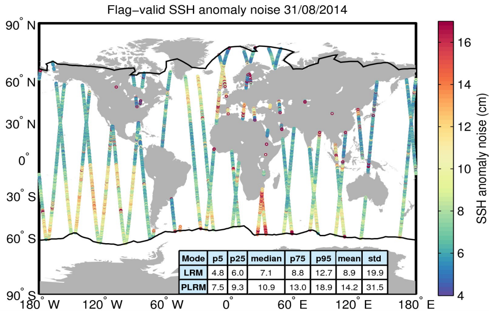
Figure 8. Geographical distribution of flag-valid 20-Hz SSH anomaly measurement noise over oceans and lakes for 31/08/2014. The statistical values shown in the table refer to the SSH anomaly noise and are calculated separately for LRM and PLRM regions. Measurements taken over polar polygons have been excluded from the computation of the statistical values. The black lines mark the outer limit of the Arctic and Antarctic polar polygons.
