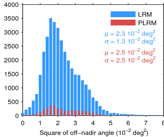
Figure 39. Histogram of flag-valid mispointing over oceans and lakes for LRM (blue) and PLRM (red) for 31/08/2014. Only positive values have been considered. The mean ( \mu ) and standard deviation ( \sigma ) are also shown. Note that values larger than 8 \cdot 10^{-2} \text{ deg}^2 are excluded from the histogram for the sake of readability but not from the computation of \mu and \sigma .
