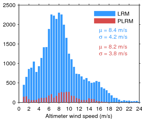
Figure 35. Histogram of science-valid wind over oceans and lakes for LRM (blue) and PLRM (red) for 31/08/2014. The mean ( \mu ) and standard deviation ( \sigma ) are also shown. Note that values larger than 24 m/s are excluded from the histogram for the sake of readability but not from the computation of \mu and \sigma .
