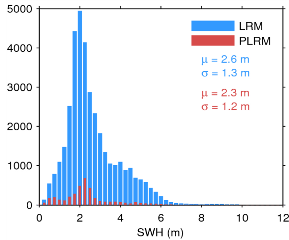
Figure 20. Histogram of science-valid SWH over oceans and lakes for LRM (blue) and PLRM (red) for 31/08/2014. The mean ( \mu ) and standard deviation ( \sigma ) are also shown. Note that values larger than 12 m are excluded from the histogram for the sake of readability but not from the computation of \mu and \sigma .
