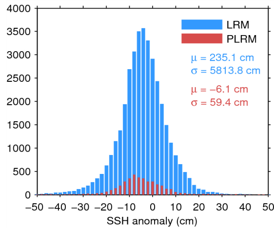
Figure 7. Histogram of flag-valid SSH anomaly over oceans and lakes for LRM (blue) and PLRM (red) for 31/08/2014. The mean ( \mu ) and standard deviation ( \sigma ) are also shown. Note that values outside [-50\ 50] cm are excluded from the histogram for the sake of readability but not from the computation of \mu and \sigma .
