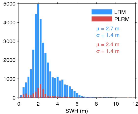
Figure 17. Histogram of flag-valid SWH over oceans and lakes for LRM (blue) and PLRM (red) for 31/08/2014. The mean ( \mu ) and standard deviation ( \sigma ) are also shown. Note that values larger than 12 m are excluded from the histogram for the sake of readability but not from the computation of \mu and \sigma .
