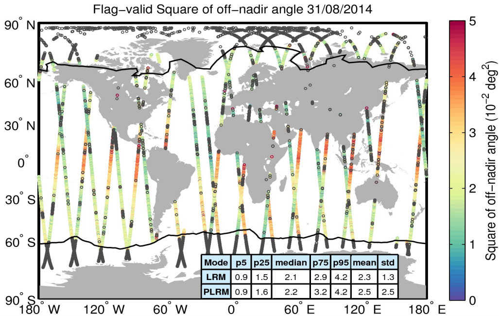
Figure 37. Geographical distribution of flag-valid mispointing data over oceans and lakes for 31/08/2014. The statistical values shown in the table refer to the mispointing in 10^{-2} \text{ deg}^2 and are calculated separately for LRM and PLRM regions. Measurements taken over polar polygons have been excluded from the computation of the statistical values. The black lines mark the outer limit of the Arctic and Antarctic polar polygons. Gray circles denote negative values.
