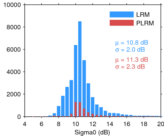
Figure 25. Histogram of flag-valid sigma0 over oceans and lakes for LRM (blue) and PLRM (red) for 30/08/2014. The mean ( \mu ) and standard deviation ( \sigma ) are also shown. Note that values outside [4 20] dB are excluded from the histogram for the sake of readability but not from the computation of \mu and \sigma .
