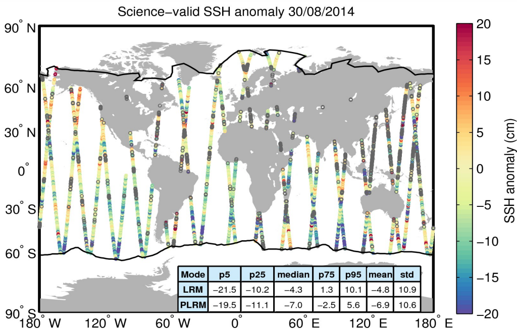
Figure 10. Geographical distribution of science-valid SSH anomaly data over oceans and lakes for 30/08/2014. The statistical values shown in the table refer to the SSH anomaly in cm and are calculated separately for LRM and PLRM regions. The black lines mark the outer limit of the Arctic and Antarctic polar polygons. Gray circles denote records that have been rejected based on the editing criteria described in Table 2.
