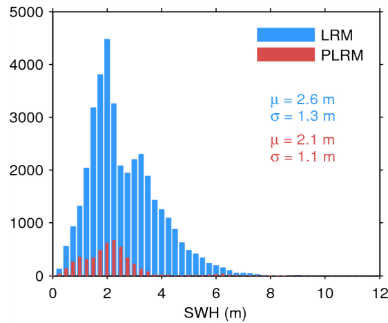
Figure 20. Histogram of science-valid SWH over oceans and lakes for LRM (blue) and PLRM (red) for 30/08/2014. The mean ( \mu ) and standard deviation ( \sigma ) are also shown. Note that values larger than 12 m are excluded from the histogram for the sake of readability but not from the computation of \mu and \sigma .
