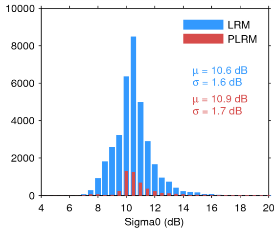
Figure 28. Histogram of science-valid sigma0 over oceans and lakes for LRM (blue) and PLRM (red) for 30/08/2014. The mean ( \mu ) and standard deviation ( \sigma ) are also shown. Note that values outside [4 20] dB are excluded from the histogram for the sake of readability but not from the computation of \mu and \sigma .
