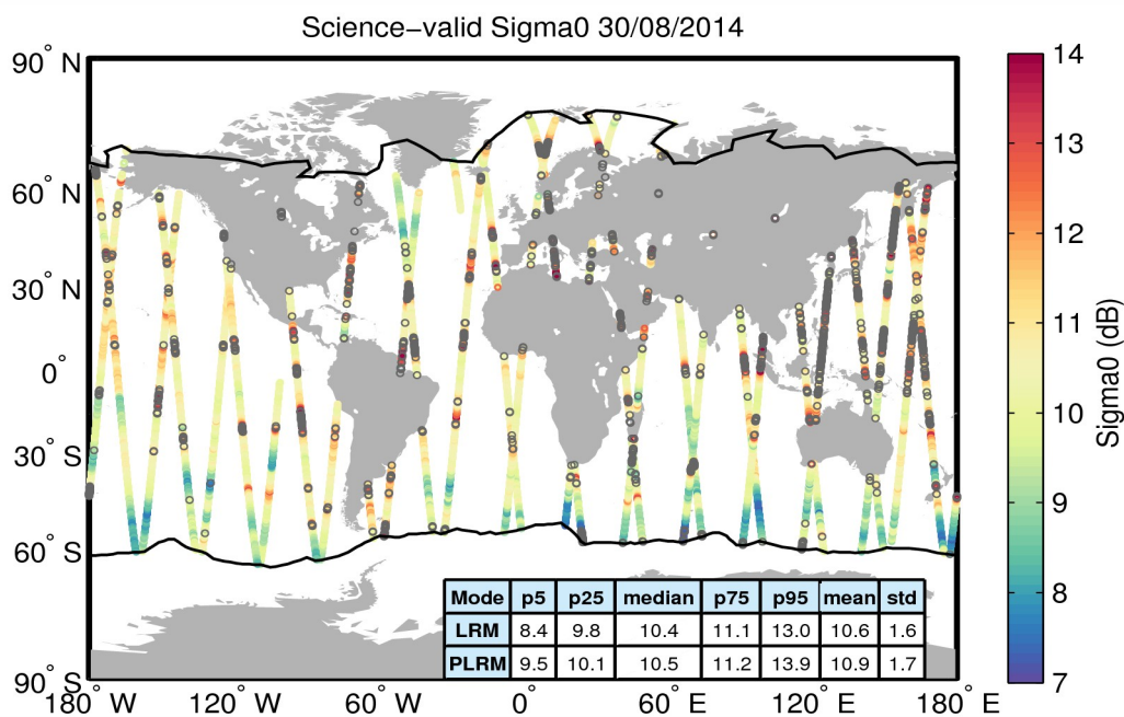
Figure 27. Geographical distribution of science-valid sigma0 data over oceans and lakes for 30/08/2014. The statistical values shown in the table refer to the sigma0 in dB and are calculated separately for LRM and PLRM regions. The black lines mark the outer limit of the Arctic and Antarctic polar polygons. Gray circles denote records that have been rejected based on the editing criteria described in Table 4.
