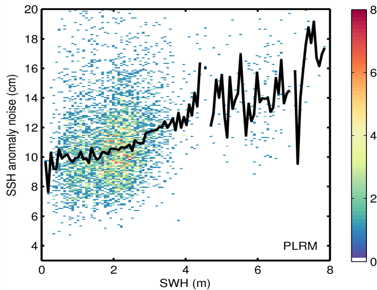
Figure 9. 2D histogram showing flag-valid SSH anomaly noise as a function of SWH for LRM (top) and PLRM (bottom) for 30/08/2014. The black line denotes the median SSH anomaly as a function of SWH.
