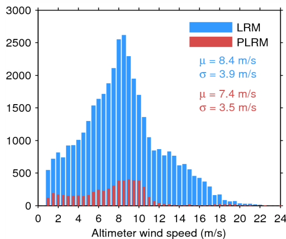
Figure 35. Histogram of science-valid wind over oceans and lakes for LRM (blue) and PLRM (red) for 30/08/2014. The mean ( \mu ) and standard deviation ( \sigma ) are also shown. Note that values larger than 24 m/s are excluded from the histogram for the sake of readability but not from the computation of \mu and \sigma .
