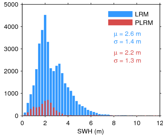
Figure 17. Histogram of flag-valid SWH over oceans and lakes for LRM (blue) and PLRM (red) for 30/08/2014. The mean ( \mu ) and standard deviation ( \sigma ) are also shown. Note that values larger than 12 m are excluded from the histogram for the sake of readability but not from the computation of \mu and \sigma .
