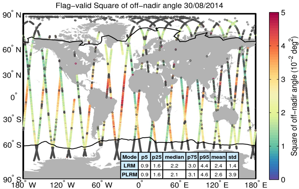
Figure 37. Geographical distribution of flag-valid mispointing data over oceans and lakes for 30/08/2014. The statistical values shown in the table refer to the mispointing in 10^{-2} \text{ deg}^2 and are calculated separately for LRM and PLRM regions. Measurements taken over polar polygons have been excluded from the computation of the statistical values. The black lines mark the outer limit of the Arctic and Antarctic polar polygons. Gray circles denote negative values.
