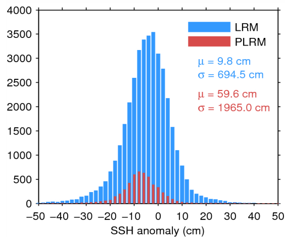
Figure 7. Histogram of flag-valid SSH anomaly over oceans and lakes for LRM (blue) and PLRM (red) for 30/08/2014. The mean ( \mu ) and standard deviation ( \sigma ) are also shown. Note that values outside [-50\ 50] cm are excluded from the histogram for the sake of readability but not from the computation of \mu and \sigma .
