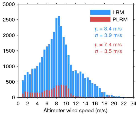
Figure 33. Histogram of flag-valid wind over oceans and lakes for LRM (blue) and PLRM (red) for 30/08/2014. The mean ( \mu ) and standard deviation ( \sigma ) are also shown. Note that values larger than 24 m/s are excluded from the histogram for the sake of readability but not from the computation of \mu and \sigma .
