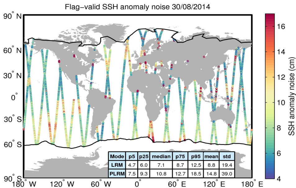
Figure 8. Geographical distribution of flag-valid 20-Hz SSH anomaly measurement noise over oceans and lakes for 30/08/2014. The statistical values shown in the table refer to the SSH anomaly noise and are calculated separately for LRM and PLRM regions. Measurements taken over polar polygons have been excluded from the computation of the statistical values. The black lines mark the outer limit of the Arctic and Antarctic polar polygons.
