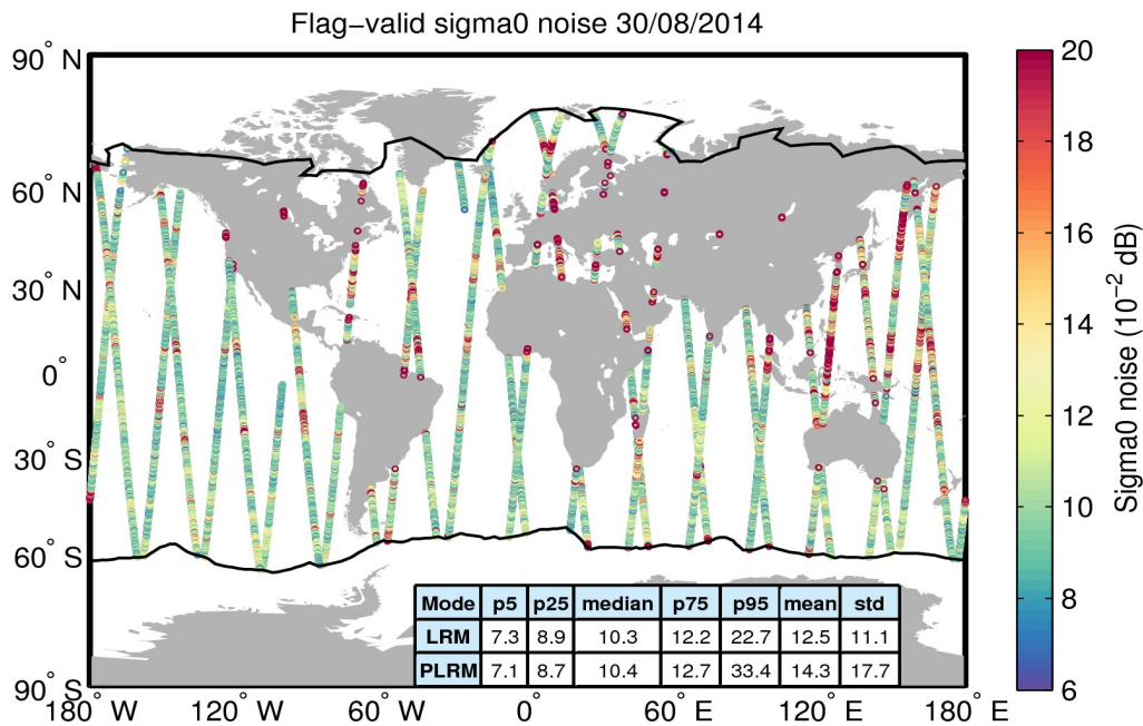
Figure 26. Geographical distribution of flag-valid 20-Hz sigma0 measurement noise over oceans and lakes for 30/08/2014. The statistical values shown in the table refer to the sigma0 noise and are calculated separately for LRM and PLRM regions. Measurements taken over polar polygons have been excluded from the computation of the statistical values. The black lines mark the outer limit of the Arctic and Antarctic polar polygons.
