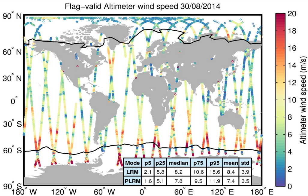
Figure 31. Geographical distribution of flag-valid wind data over oceans and lakes for 30/08/2014. The statistical values shown in the table refer to the wind in m/s and are calculated separately for LRM and PLRM regions. Measurements taken over polar polygons have been excluded from the computation of the statistical values. The black lines mark the outer limit of the Arctic and Antarctic polar polygons.
