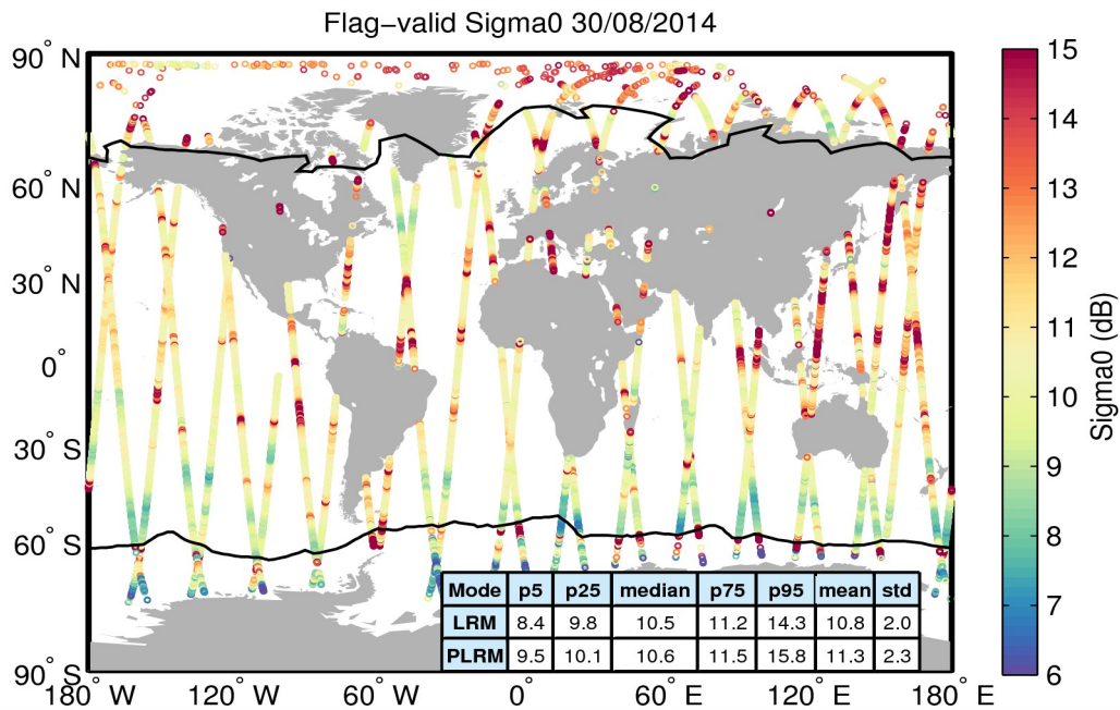
Figure 23. Geographical distribution of flag-valid sigma0 data over oceans and lakes for 30/08/2014. The statistical values shown in the table refer to the sigma0 in dB and are calculated separately for LRM and PLRM regions. Measurements taken over polar polygons have been excluded from the computation of the statistical values. The black lines mark the outer limit of the Arctic and Antarctic polar polygons.
