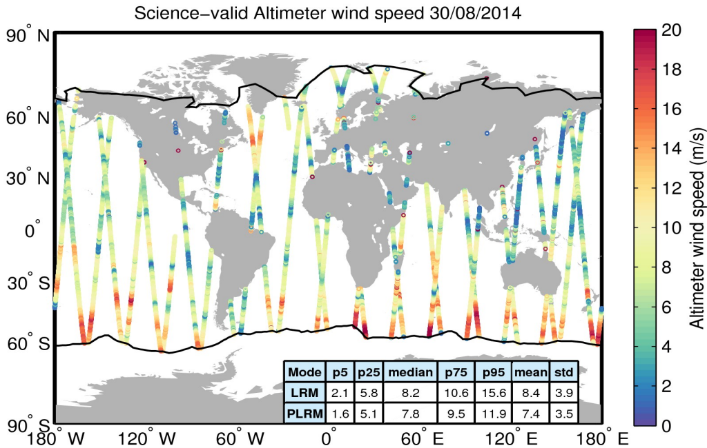
Figure 34. Geographical distribution of science-valid wind data over oceans and lakes for 30/08/2014. The statistical values shown in the table refer to the wind in m/s and are calculated separately for LRM and PLRM regions. The black lines mark the outer limit of the Arctic and Antarctic polar polygons. Gray circles denote records that have been rejected based on the editing criteria described in Table 5.
