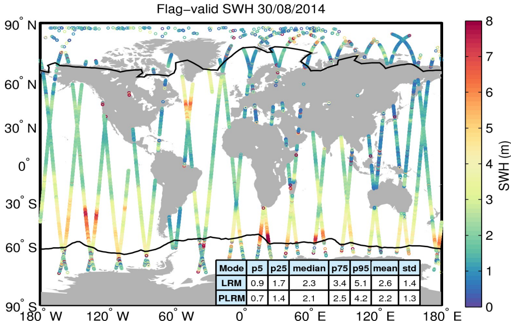
Figure 15. Geographical distribution of flag-valid SWH data over oceans and lakes for 30/08/2014. The statistical values shown in the table refer to the SWH in m and are calculated separately for LRM and PLRM regions. Measurements taken over polar polygons have been excluded from the computation of the statistical values. The black lines mark the outer limit of the Arctic and Antarctic polar polygons.
