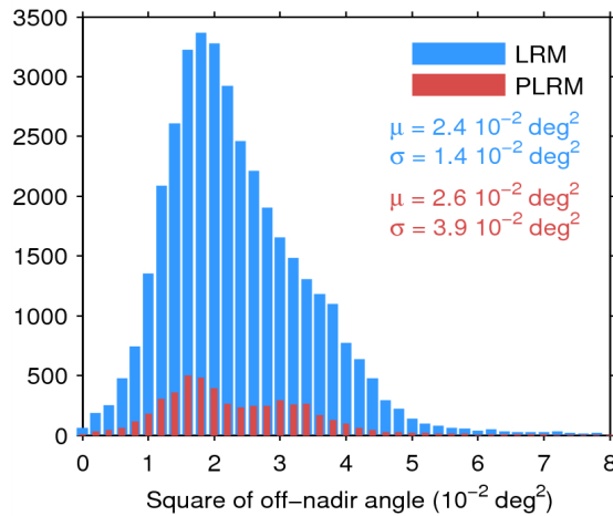
Figure 39. Histogram of flag-valid mispointing over oceans and lakes for LRM (blue) and PLRM (red) for 30/08/2014. Only positive values have been considered. The mean ( \mu ) and standard deviation ( \sigma ) are also shown. Note that values larger than 8 \cdot 10^{-2} \text{ deg}^2 are excluded from the histogram for the sake of readability but not from the computation of \mu and \sigma .
