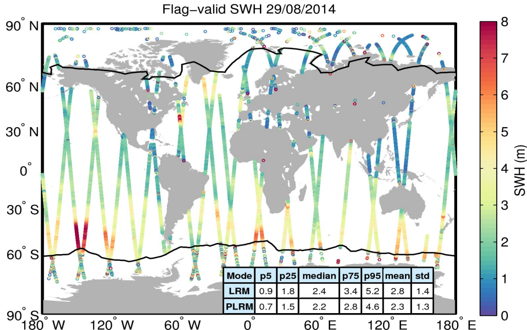
Figure 15. Geographical distribution of flag-valid SWH data over oceans and lakes for 29/08/2014. The statistical values shown in the table refer to the SWH in m and are calculated separately for LRM and PLRM regions. Measurements taken over polar polygons have been excluded from the computation of the statistical values. The black lines mark the outer limit of the Arctic and Antarctic polar polygons.
