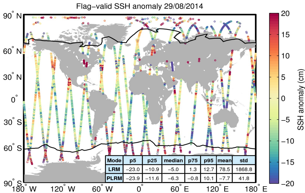
Figure 5. Geographical distribution of flag-valid 1-Hz SSH anomaly data over oceans and lakes for 29/08/2014. The statistical values shown in the table refer to the SSH anomaly in cm and are calculated separately for LRM and PLRM regions. Measurements taken over polar polygons have been excluded from the computation of the statistical values. The black lines mark the outer limit of the Arctic and Antarctic polar polygons.
