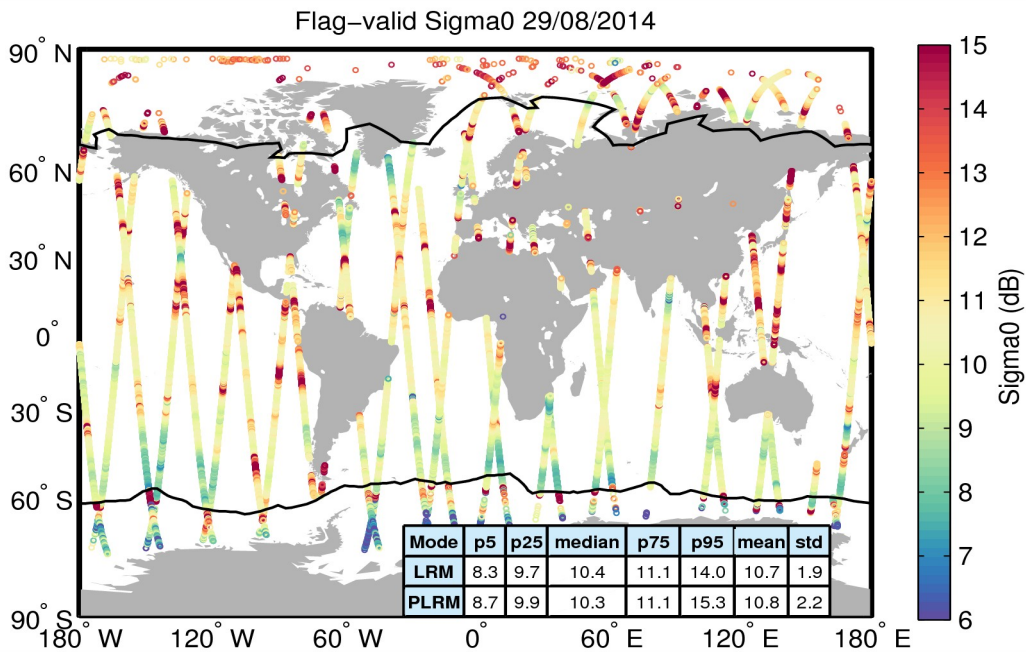
Figure 23. Geographical distribution of flag-valid sigma0 data over oceans and lakes for 29/08/2014. The statistical values shown in the table refer to the sigma0 in dB and are calculated separately for LRM and PLRM regions. Measurements taken over polar polygons have been excluded from the computation of the statistical values. The black lines mark the outer limit of the Arctic and Antarctic polar polygons.
