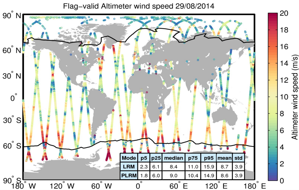
Figure 31. Geographical distribution of flag-valid wind data over oceans and lakes for 29/08/2014. The statistical values shown in the table refer to the wind in m/s and are calculated separately for LRM and PLRM regions. Measurements taken over polar polygons have been excluded from the computation of the statistical values. The black lines mark the outer limit of the Arctic and Antarctic polar polygons.
