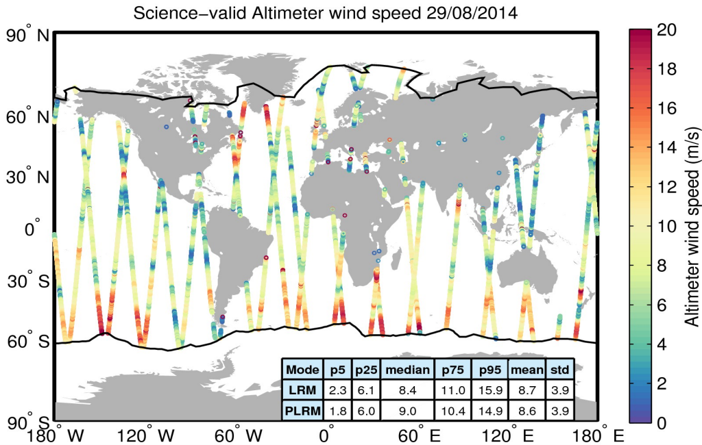
Figure 34. Geographical distribution of science-valid wind data over oceans and lakes for 29/08/2014. The statistical values shown in the table refer to the wind in m/s and are calculated separately for LRM and PLRM regions. The black lines mark the outer limit of the Arctic and Antarctic polar polygons. Gray circles denote records that have been rejected based on the editing criteria described in Table 5.
