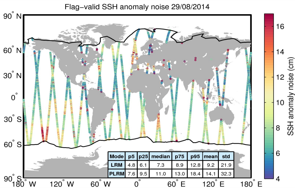
Figure 8. Geographical distribution of flag-valid 20-Hz SSH anomaly measurement noise over oceans and lakes for 29/08/2014. The statistical values shown in the table refer to the SSH anomaly noise and are calculated separately for LRM and PLRM regions. Measurements taken over polar polygons have been excluded from the computation of the statistical values. The black lines mark the outer limit of the Arctic and Antarctic polar polygons.
