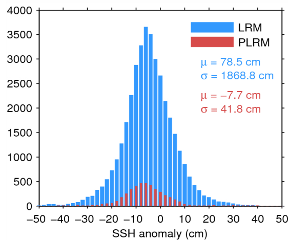
Figure 7. Histogram of flag-valid SSH anomaly over oceans and lakes for LRM (blue) and PLRM (red) for 29/08/2014. The mean ( \mu ) and standard deviation ( \sigma ) are also shown. Note that values outside [-50\ 50] cm are excluded from the histogram for the sake of readability but not from the computation of \mu and \sigma .
