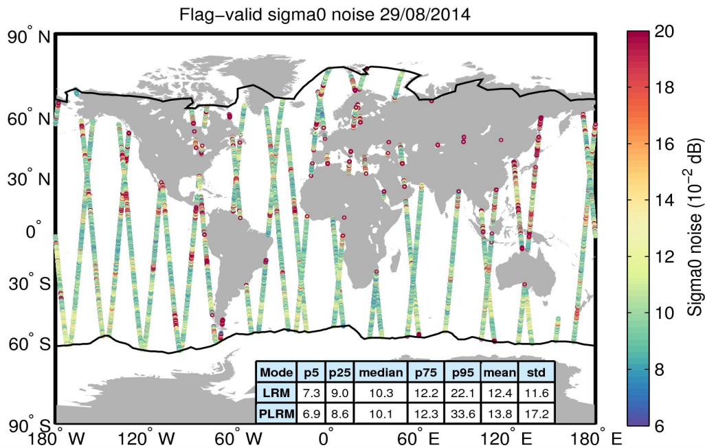
Figure 26. Geographical distribution of flag-valid 20-Hz sigma0 measurement noise over oceans and lakes for 29/08/2014. The statistical values shown in the table refer to the sigma0 noise and are calculated separately for LRM and PLRM regions. Measurements taken over polar polygons have been excluded from the computation of the statistical values. The black lines mark the outer limit of the Arctic and Antarctic polar polygons.
