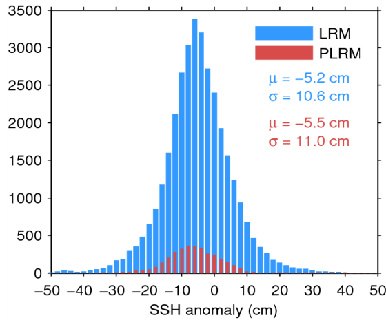
Figure 11. Histogram of science-valid SSH anomaly over oceans and lakes for LRM (blue) and PLRM (red) for 29/08/2014. The mean ( \mu ) and standard deviation ( \sigma ) are also shown. Note that values outside [-50 50] cm are excluded from the histogram for the sake of readability but not from the computation of \mu and \sigma .
