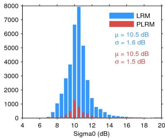
Figure 28. Histogram of science-valid sigma0 over oceans and lakes for LRM (blue) and PLRM (red) for 29/08/2014. The mean ( \mu ) and standard deviation ( \sigma ) are also shown. Note that values outside [4 20] dB are excluded from the histogram for the sake of readability but not from the computation of \mu and \sigma .
