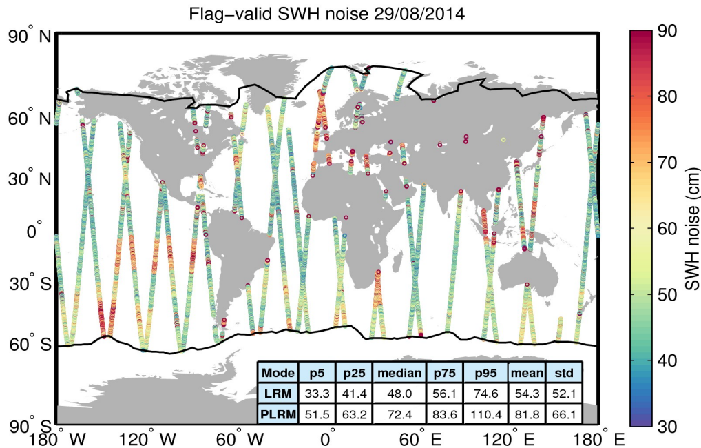
Figure 18. Geographical distribution of flag-valid 20-Hz SWH measurement noise over oceans and lakes for 29/08/2014. The statistical values shown in the table refer to the SWH noise and are calculated separately for LRM and PLRM regions. Measurements taken over polar polygons have been excluded from the computation of the statistical values. The black lines mark the outer limit of the Arctic and Antarctic polar polygons.
