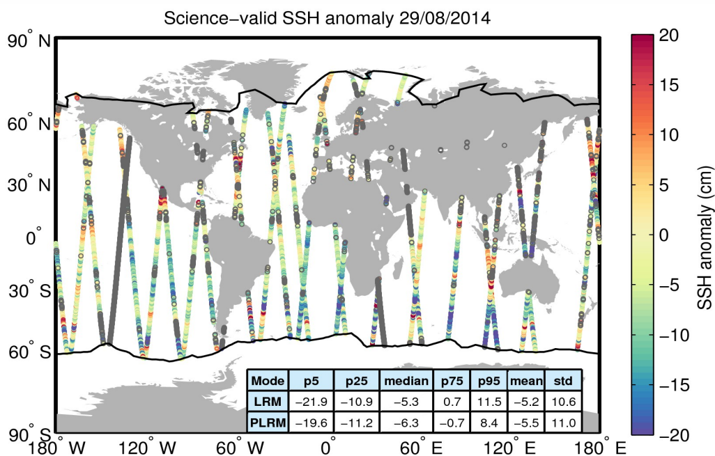
Figure 10. Geographical distribution of science-valid SSH anomaly data over oceans and lakes for 29/08/2014. The statistical values shown in the table refer to the SSH anomaly in cm and are calculated separately for LRM and PLRM regions. The black lines mark the outer limit of the Arctic and Antarctic polar polygons. Gray circles denote records that have been rejected based on the editing criteria described in Table 2.
