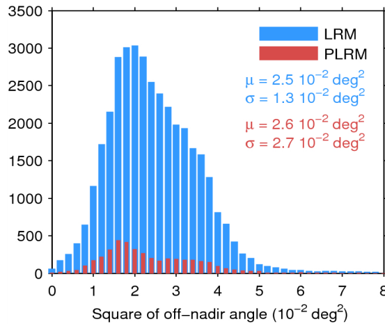
Figure 39. Histogram of flag-valid mispointing over oceans and lakes for LRM (blue) and PLRM (red) for 29/08/2014. Only positive values have been considered. The mean ( \mu ) and standard deviation ( \sigma ) are also shown. Note that values larger than 8 \cdot 10^{-2} \text{ deg}^2 are excluded from the histogram for the sake of readability but not from the computation of \mu and \sigma .
