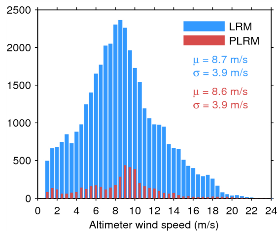
Figure 33. Histogram of flag-valid wind over oceans and lakes for LRM (blue) and PLRM (red) for 29/08/2014. The mean ( \mu ) and standard deviation ( \sigma ) are also shown. Note that values larger than 24 m/s are excluded from the histogram for the sake of readability but not from the computation of \mu and \sigma .
