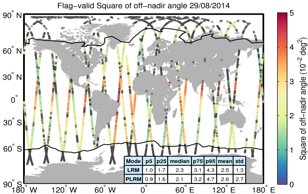
Figure 37. Geographical distribution of flag-valid mispointing data over oceans and lakes for 29/08/2014. The statistical values shown in the table refer to the mispointing in 10^{-2} \text{ deg}^2 and are calculated separately for LRM and PLRM regions. Measurements taken over polar polygons have been excluded from the computation of the statistical values. The black lines mark the outer limit of the Arctic and Antarctic polar polygons. Gray circles denote negative values.
