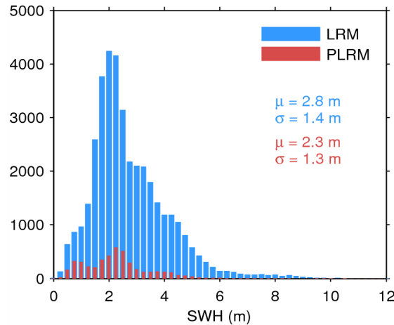
Figure 17. Histogram of flag-valid SWH over oceans and lakes for LRM (blue) and PLRM (red) for 29/08/2014. The mean ( \mu ) and standard deviation ( \sigma ) are also shown. Note that values larger than 12 m are excluded from the histogram for the sake of readability but not from the computation of \mu and \sigma .
