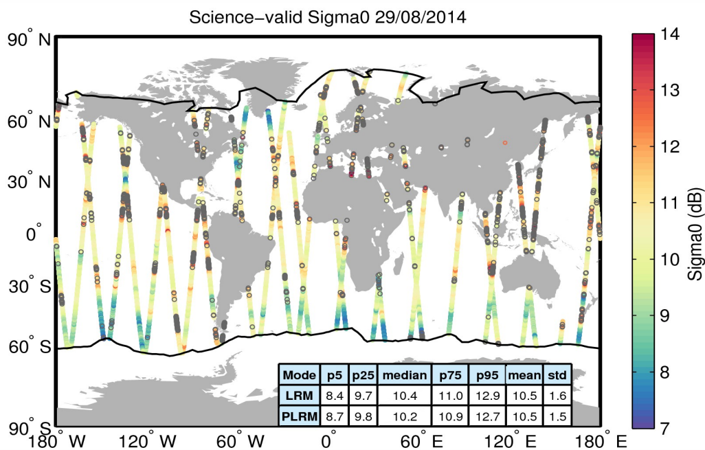
Figure 27. Geographical distribution of science-valid sigma0 data over oceans and lakes for 29/08/2014. The statistical values shown in the table refer to the sigma0 in dB and are calculated separately for LRM and PLRM regions. The black lines mark the outer limit of the Arctic and Antarctic polar polygons. Gray circles denote records that have been rejected based on the editing criteria described in Table 4.
