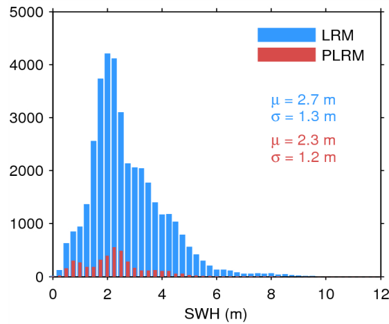
Figure 20. Histogram of science-valid SWH over oceans and lakes for LRM (blue) and PLRM (red) for 29/08/2014. The mean ( \mu ) and standard deviation ( \sigma ) are also shown. Note that values larger than 12 m are excluded from the histogram for the sake of readability but not from the computation of \mu and \sigma .
