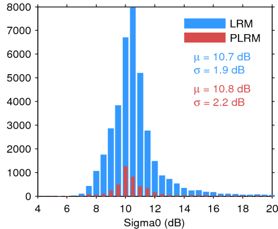
Figure 25. Histogram of flag-valid sigma0 over oceans and lakes for LRM (blue) and PLRM (red) for 29/08/2014. The mean ( \mu ) and standard deviation ( \sigma ) are also shown. Note that values outside [4 20] dB are excluded from the histogram for the sake of readability but not from the computation of \mu and \sigma .
