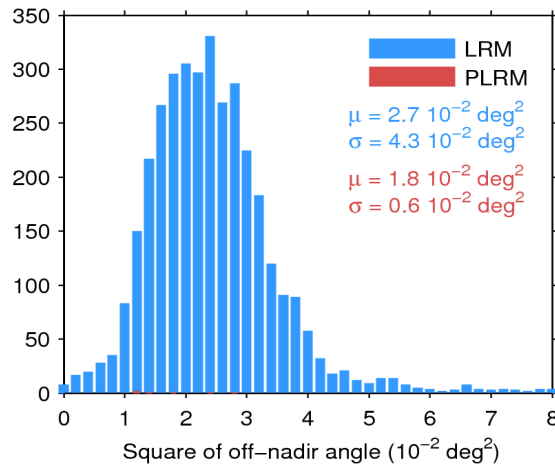
Figure 39. Histogram of flag-valid mispointing over oceans and lakes for LRM (blue) and PLRM (red) for 28/08/2014. Only positive values have been considered. The mean ( \mu ) and standard deviation ( \sigma ) are also shown. Note that values larger than 8 \cdot 10^{-2} \text{ deg}^2 are excluded from the histogram for the sake of readability but not from the computation of \mu and \sigma .
