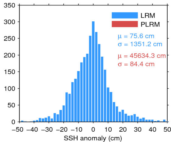
Figure 7. Histogram of flag-valid SSH anomaly over oceans and lakes for LRM (blue) and PLRM (red) for 28/08/2014. The mean ( \mu ) and standard deviation ( \sigma ) are also shown. Note that values outside [-50 \ 50] cm are excluded from the histogram for the sake of readability but not from the computation of \mu and \sigma .
