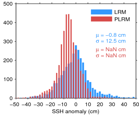
Figure 11. Histogram of science-valid SSH anomaly over oceans and lakes for LRM (blue) and PLRM (red) for 28/08/2014. The mean ( \mu ) and standard deviation ( \sigma ) are also shown. Note that values outside [-50\ 50] cm are excluded from the histogram for the sake of readability but not from the computation of \mu and \sigma .
