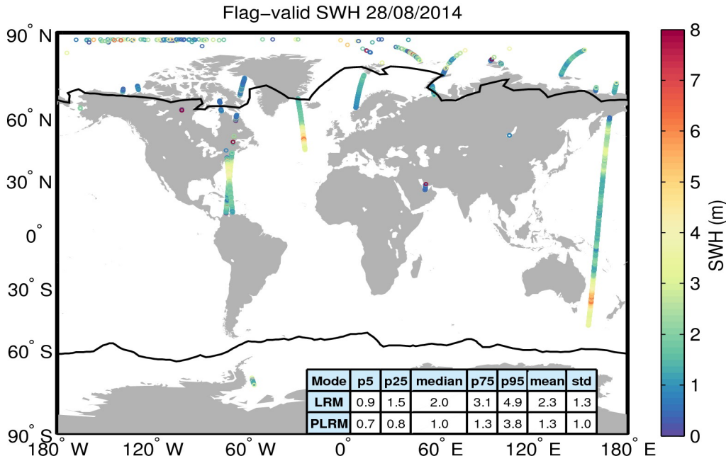
Figure 15. Geographical distribution of flag-valid SWH data over oceans and lakes for 28/08/2014. The statistical values shown in the table refer to the SWH in m and are calculated separately for LRM and PLRM regions. Measurements taken over polar polygons have been excluded from the computation of the statistical values. The black lines mark the outer limit of the Arctic and Antarctic polar polygons.
