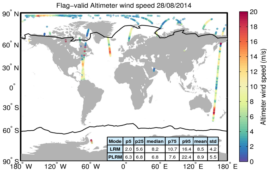
Figure 31. Geographical distribution of flag-valid wind data over oceans and lakes for 28/08/2014. The statistical values shown in the table refer to the wind in m/s and are calculated separately for LRM and PLRM regions. Measurements taken over polar polygons have been excluded from the computation of the statistical values. The black lines mark the outer limit of the Arctic and Antarctic polar polygons.
