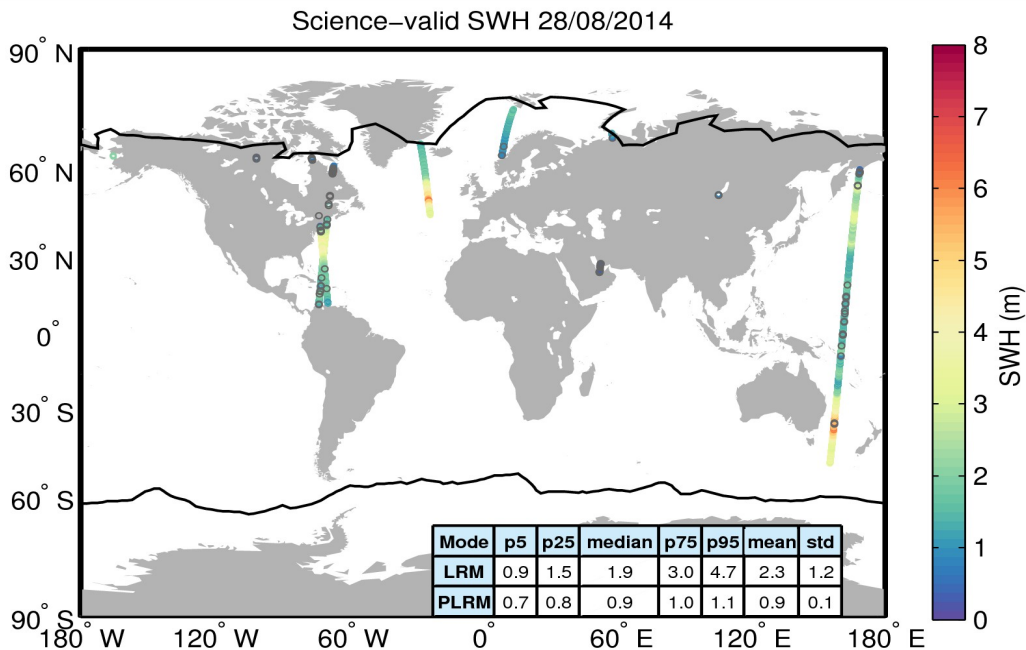
Figure 19. Geographical distribution of science-valid SWH data over oceans and lakes for 28/08/2014. The statistical values shown in the table refer to the SWH in m and are calculated separately for LRM and PLRM regions. The black lines mark the outer limit of the Arctic and Antarctic polar polygons. Gray circles denote records that have been rejected based on the editing criteria described in Table 3.
