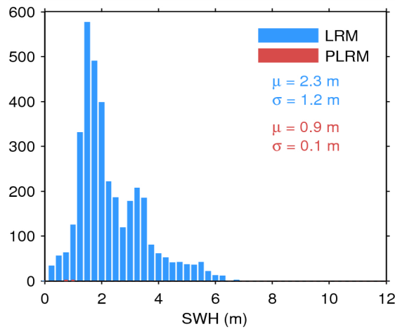
Figure 20. Histogram of science-valid SWH over oceans and lakes for LRM (blue) and PLRM (red) for 28/08/2014. The mean ( \mu ) and standard deviation ( \sigma ) are also shown. Note that values larger than 12 m are excluded from the histogram for the sake of readability but not from the computation of \mu and \sigma .
