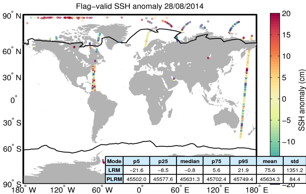
Figure 5. Geographical distribution of flag-valid 1-Hz SSH anomaly data over oceans and lakes for 28/08/2014. The statistical values shown in the table refer to the SSH anomaly in cm and are calculated separately for LRM and PLRM regions. Measurements taken over polar polygons have been excluded from the computation of the statistical values. The black lines mark the outer limit of the Arctic and Antarctic polar polygons.
