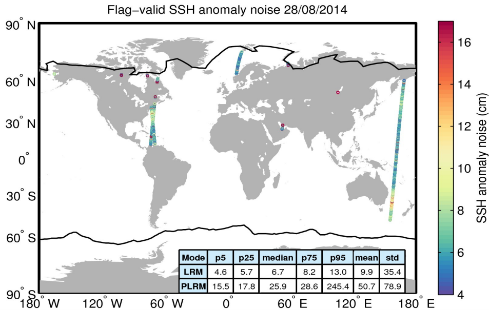
Figure 8. Geographical distribution of flag-valid 20-Hz SSH anomaly measurement noise over oceans and lakes for 28/08/2014. The statistical values shown in the table refer to the SSH anomaly noise and are calculated separately for LRM and PLRM regions. Measurements taken over polar polygons have been excluded from the computation of the statistical values. The black lines mark the outer limit of the Arctic and Antarctic polar polygons.
