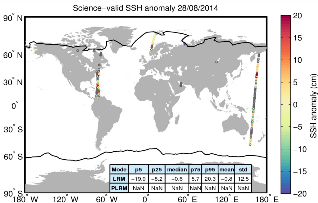
Figure 10. Geographical distribution of science-valid SSH anomaly data over oceans and lakes for 28/08/2014. The statistical values shown in the table refer to the SSH anomaly in cm and are calculated separately for LRM and PLRM regions. The black lines mark the outer limit of the Arctic and Antarctic polar polygons. Gray circles denote records that have been rejected based on the editing criteria described in Table 2.
