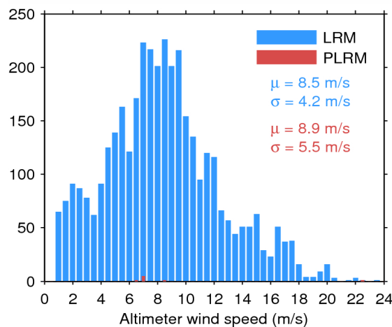
Figure 35. Histogram of science-valid wind over oceans and lakes for LRM (blue) and PLRM (red) for 28/08/2014. The mean ( \mu ) and standard deviation ( \sigma ) are also shown. Note that values larger than 24 m/s are excluded from the histogram for the sake of readability but not from the computation of \mu and \sigma .
