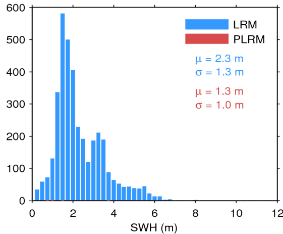
Figure 17. Histogram of flag-valid SWH over oceans and lakes for LRM (blue) and PLRM (red) for 28/08/2014. The mean ( \mu ) and standard deviation ( \sigma ) are also shown. Note that values larger than 12 m are excluded from the histogram for the sake of readability but not from the computation of \mu and \sigma .
