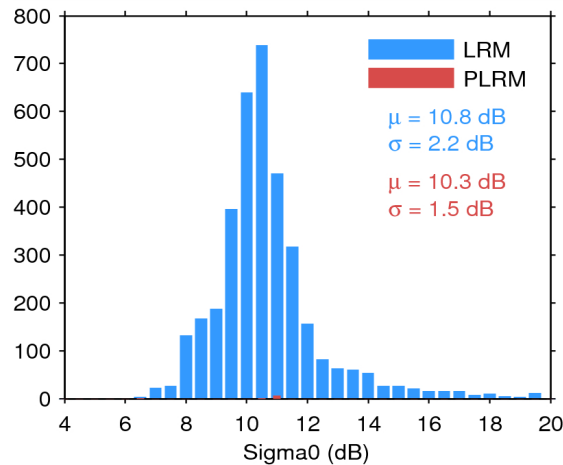
Figure 25. Histogram of flag-valid sigma0 over oceans and lakes for LRM (blue) and PLRM (red) for 28/08/2014. The mean ( \mu ) and standard deviation ( \sigma ) are also shown. Note that values outside [4 20] dB are excluded from the histogram for the sake of readability but not from the computation of \mu and \sigma .
