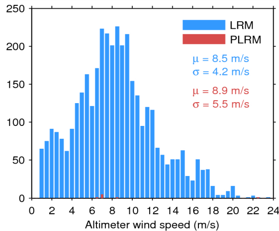
Figure 33. Histogram of flag-valid wind over oceans and lakes for LRM (blue) and PLRM (red) for 28/08/2014. The mean ( \mu ) and standard deviation ( \sigma ) are also shown. Note that values larger than 24 m/s are excluded from the histogram for the sake of readability but not from the computation of \mu and \sigma .
