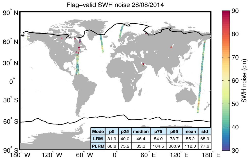
Figure 18. Geographical distribution of flag-valid 20-Hz SWH measurement noise over oceans and lakes for 28/08/2014. The statistical values shown in the table refer to the SWH noise and are calculated separately for LRM and PLRM regions. Measurements taken over polar polygons have been excluded from the computation of the statistical values. The black lines mark the outer limit of the Arctic and Antarctic polar polygons.
