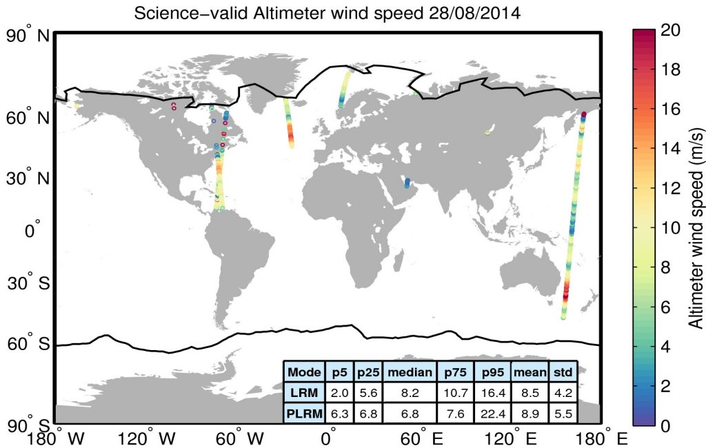
Figure 34. Geographical distribution of science-valid wind data over oceans and lakes for 28/08/2014. The statistical values shown in the table refer to the wind in m/s and are calculated separately for LRM and PLRM regions. The black lines mark the outer limit of the Arctic and Antarctic polar polygons. Gray circles denote records that have been rejected based on the editing criteria described in Table 5.
