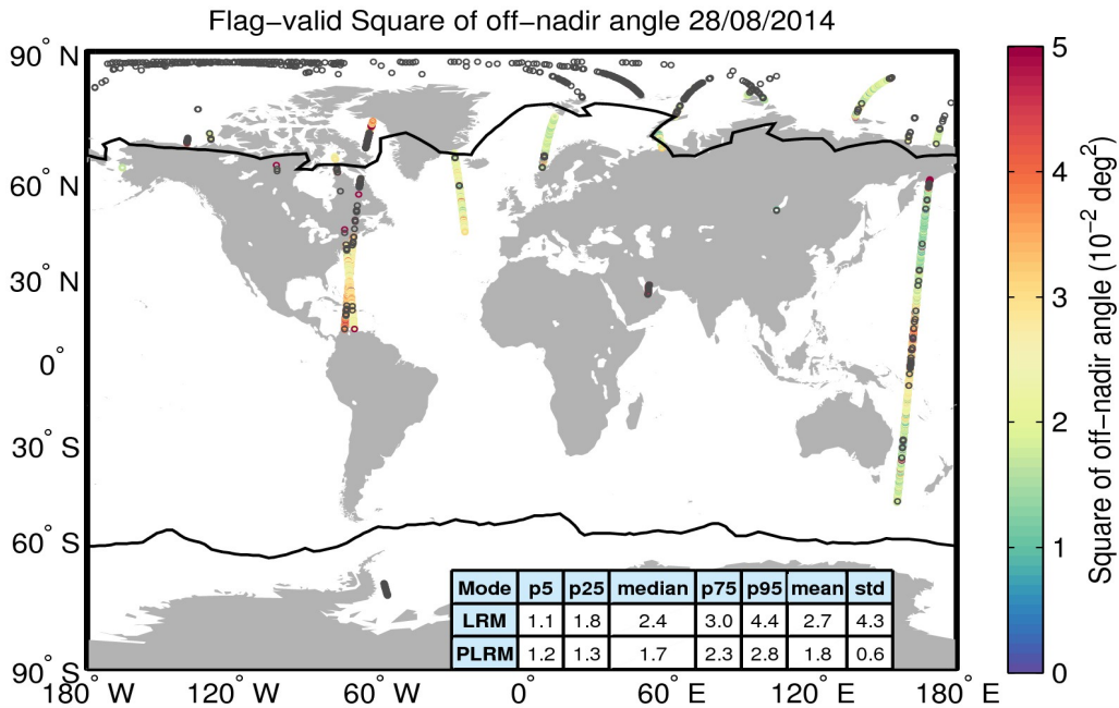
Figure 37. Geographical distribution of flag-valid mispointing data over oceans and lakes for 28/08/2014. The statistical values shown in the table refer to the mispointing in 10^{-2} \text{ deg}^2 and are calculated separately for LRM and PLRM regions. Measurements taken over polar polygons have been excluded from the computation of the statistical values. The black lines mark the outer limit of the Arctic and Antarctic polar polygons. Gray circles denote negative values.
