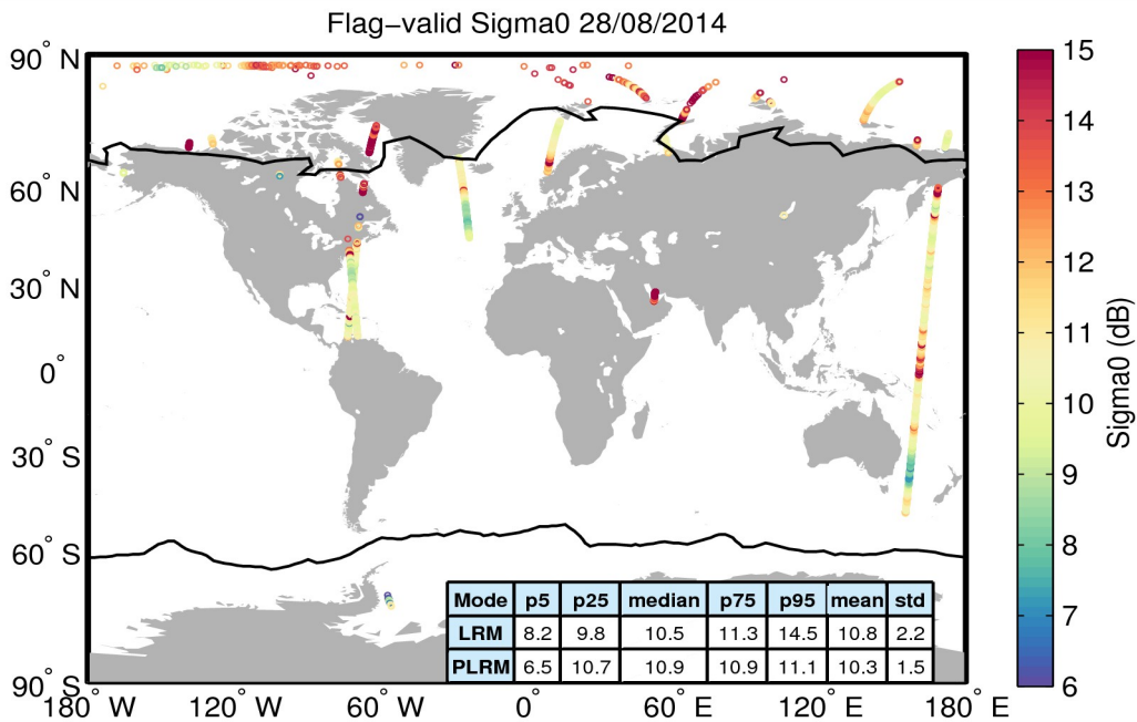
Figure 23. Geographical distribution of flag-valid sigma0 data over oceans and lakes for 28/08/2014. The statistical values shown in the table refer to the sigma0 in dB and are calculated separately for LRM and PLRM regions. Measurements taken over polar polygons have been excluded from the computation of the statistical values. The black lines mark the outer limit of the Arctic and Antarctic polar polygons.
