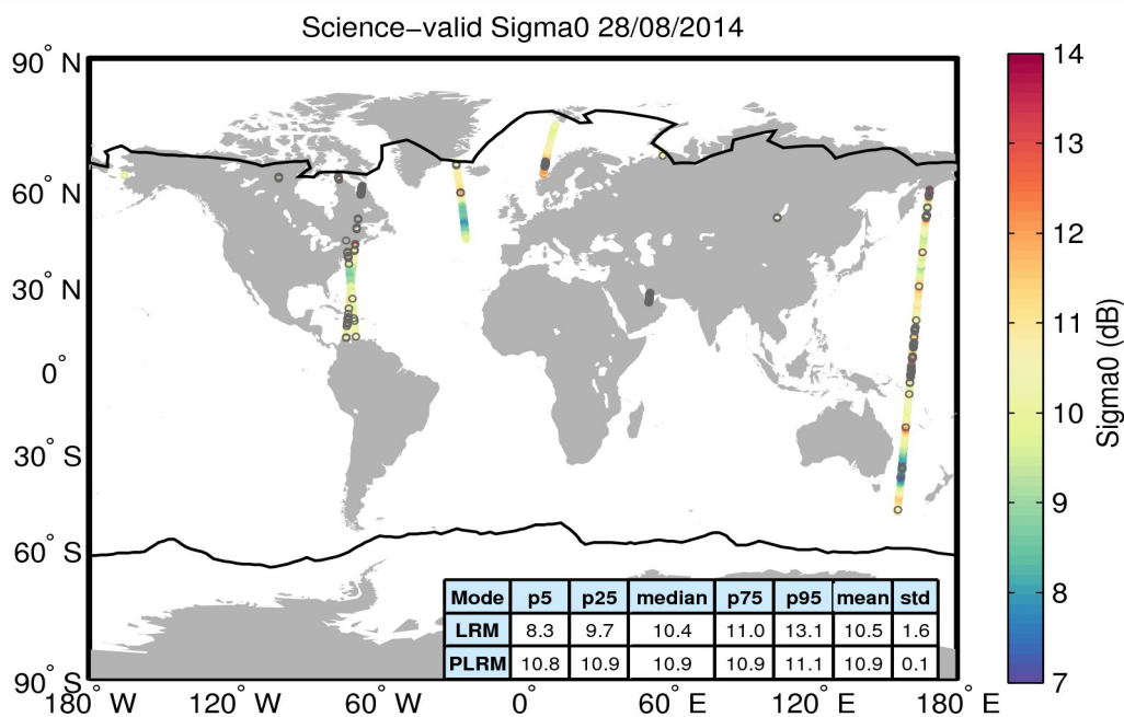
Figure 27. Geographical distribution of science-valid sigma0 data over oceans and lakes for 28/08/2014. The statistical values shown in the table refer to the sigma0 in dB and are calculated separately for LRM and PLRM regions. The black lines mark the outer limit of the Arctic and Antarctic polar polygons. Gray circles denote records that have been rejected based on the editing criteria described in Table 4.
