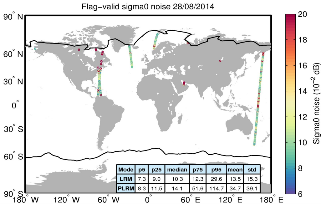
Figure 26. Geographical distribution of flag-valid 20-Hz sigma0 measurement noise over oceans and lakes for 28/08/2014. The statistical values shown in the table refer to the sigma0 noise and are calculated separately for LRM and PLRM regions. Measurements taken over polar polygons have been excluded from the computation of the statistical values. The black lines mark the outer limit of the Arctic and Antarctic polar polygons.
