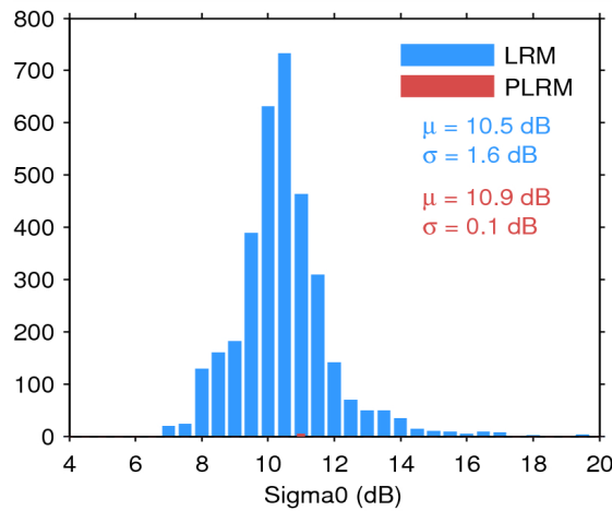
Figure 28. Histogram of science-valid sigma0 over oceans and lakes for LRM (blue) and PLRM (red) for 28/08/2014. The mean ( \mu ) and standard deviation ( \sigma ) are also shown. Note that values outside [4 20] dB are excluded from the histogram for the sake of readability but not from the computation of \mu and \sigma .
