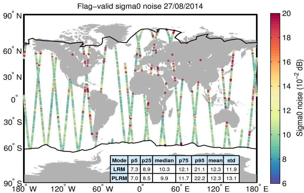
Figure 26. Geographical distribution of flag-valid 20-Hz sigma0 measurement noise over oceans and lakes for 27/08/2014. The statistical values shown in the table refer to the sigma0 noise and are calculated separately for LRM and PLRM regions. Measurements taken over polar polygons have been excluded from the computation of the statistical values. The black lines mark the outer limit of the Arctic and Antarctic polar polygons.
