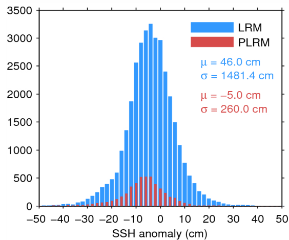
Figure 7. Histogram of flag-valid SSH anomaly over oceans and lakes for LRM (blue) and PLRM (red) for 27/08/2014. The mean ( \mu ) and standard deviation ( \sigma ) are also shown. Note that values outside [-50\ 50] cm are excluded from the histogram for the sake of readability but not from the computation of \mu and \sigma .
