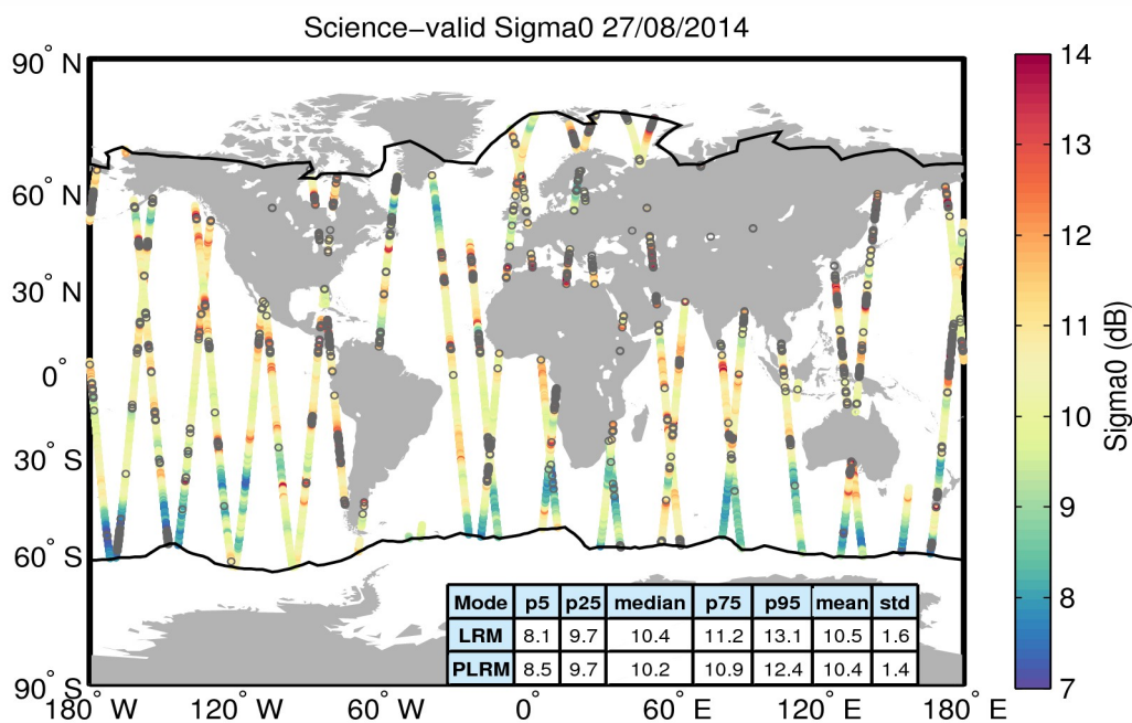
Figure 27. Geographical distribution of science-valid sigma0 data over oceans and lakes for 27/08/2014. The statistical values shown in the table refer to the sigma0 in dB and are calculated separately for LRM and PLRM regions. The black lines mark the outer limit of the Arctic and Antarctic polar polygons. Gray circles denote records that have been rejected based on the editing criteria described in Table 4.
