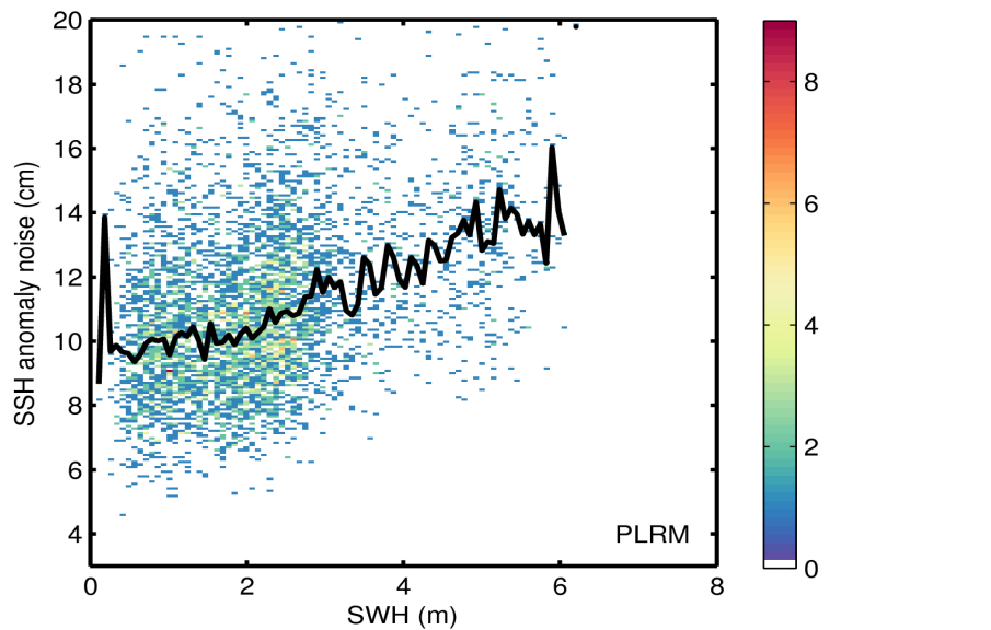
Figure 9. 2D histogram showing flag-valid SSH anomaly noise as a function of SWH for LRM (top) and PLRM (bottom) for 27/08/2014. The black line denotes the median SSH anomaly as a function of SWH.
