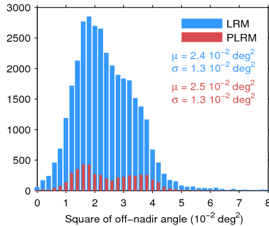
Figure 39. Histogram of flag-valid mispointing over oceans and lakes for LRM (blue) and PLRM (red) for 27/08/2014. Only positive values have been considered. The mean ( \mu ) and standard deviation ( \sigma ) are also shown. Note that values larger than 8 \cdot 10^{-2} \text{ deg}^2 are excluded from the histogram for the sake of readability but not from the computation of \mu and \sigma .
