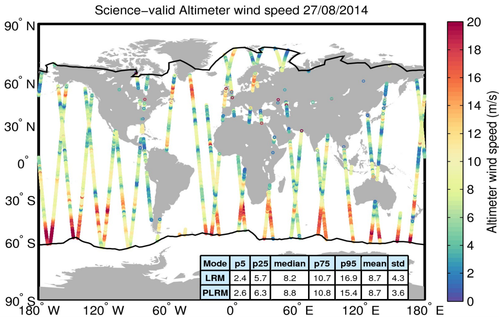
Figure 34. Geographical distribution of science-valid wind data over oceans and lakes for 27/08/2014. The statistical values shown in the table refer to the wind in m/s and are calculated separately for LRM and PLRM regions. The black lines mark the outer limit of the Arctic and Antarctic polar polygons. Gray circles denote records that have been rejected based on the editing criteria described in Table 5.
