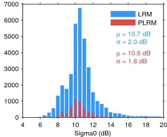
Figure 25. Histogram of flag-valid sigma0 over oceans and lakes for LRM (blue) and PLRM (red) for 27/08/2014. The mean ( \mu ) and standard deviation ( \sigma ) are also shown. Note that values outside [4 20] dB are excluded from the histogram for the sake of readability but not from the computation of \mu and \sigma .
