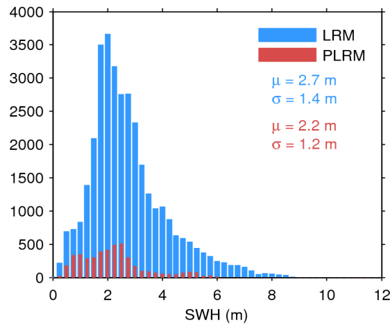
Figure 20. Histogram of science-valid SWH over oceans and lakes for LRM (blue) and PLRM (red) for 27/08/2014. The mean ( \mu ) and standard deviation ( \sigma ) are also shown. Note that values larger than 12 m are excluded from the histogram for the sake of readability but not from the computation of \mu and \sigma .
