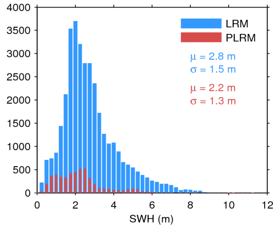
Figure 17. Histogram of flag-valid SWH over oceans and lakes for LRM (blue) and PLRM (red) for 27/08/2014. The mean ( \mu ) and standard deviation ( \sigma ) are also shown. Note that values larger than 12 m are excluded from the histogram for the sake of readability but not from the computation of \mu and \sigma .
