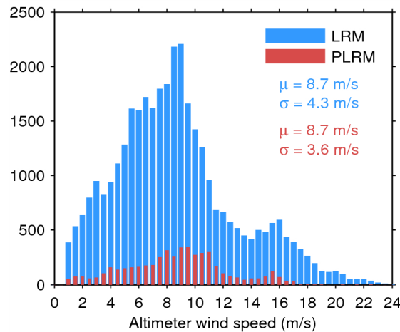
Figure 33. Histogram of flag-valid wind over oceans and lakes for LRM (blue) and PLRM (red) for 27/08/2014. The mean ( \mu ) and standard deviation ( \sigma ) are also shown. Note that values larger than 24 m/s are excluded from the histogram for the sake of readability but not from the computation of \mu and \sigma .
