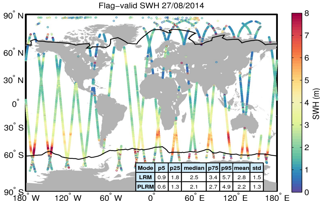
Figure 15. Geographical distribution of flag-valid SWH data over oceans and lakes for 27/08/2014. The statistical values shown in the table refer to the SWH in m and are calculated separately for LRM and PLRM regions. Measurements taken over polar polygons have been excluded from the computation of the statistical values. The black lines mark the outer limit of the Arctic and Antarctic polar polygons.
