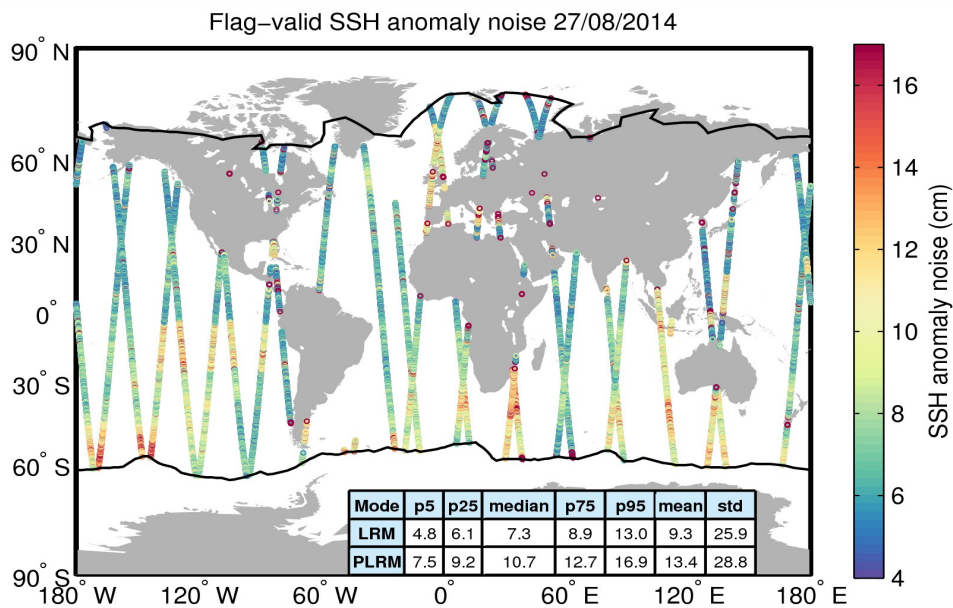
Figure 8. Geographical distribution of flag-valid 20-Hz SSH anomaly measurement noise over oceans and lakes for 27/08/2014. The statistical values shown in the table refer to the SSH anomaly noise and are calculated separately for LRM and PLRM regions. Measurements taken over polar polygons have been excluded from the computation of the statistical values. The black lines mark the outer limit of the Arctic and Antarctic polar polygons.
