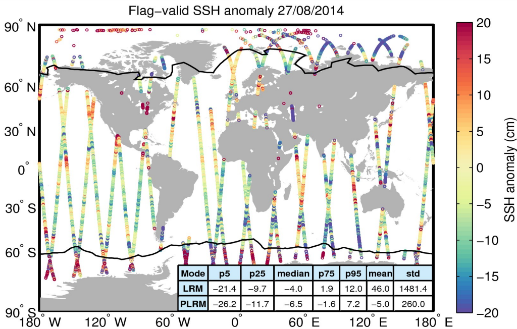
Figure 5. Geographical distribution of flag-valid 1-Hz SSH anomaly data over oceans and lakes for 27/08/2014. The statistical values shown in the table refer to the SSH anomaly in cm and are calculated separately for LRM and PLRM regions. Measurements taken over polar polygons have been excluded from the computation of the statistical values. The black lines mark the outer limit of the Arctic and Antarctic polar polygons.
