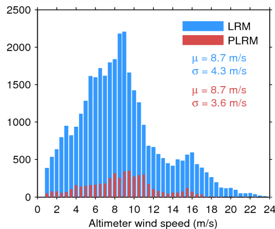
Figure 35. Histogram of science-valid wind over oceans and lakes for LRM (blue) and PLRM (red) for 27/08/2014. The mean ( \mu ) and standard deviation ( \sigma ) are also shown. Note that values larger than 24 m/s are excluded from the histogram for the sake of readability but not from the computation of \mu and \sigma .
