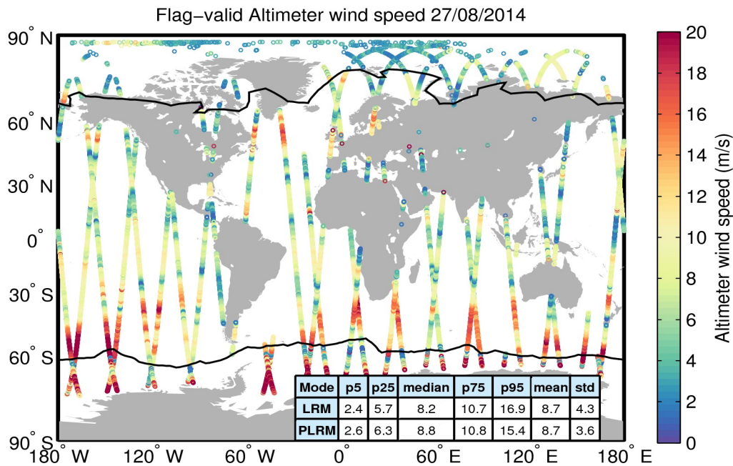
Figure 31. Geographical distribution of flag-valid wind data over oceans and lakes for 27/08/2014. The statistical values shown in the table refer to the wind in m/s and are calculated separately for LRM and PLRM regions. Measurements taken over polar polygons have been excluded from the computation of the statistical values. The black lines mark the outer limit of the Arctic and Antarctic polar polygons.
