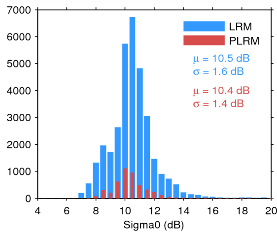
Figure 28. Histogram of science-valid sigma0 over oceans and lakes for LRM (blue) and PLRM (red) for 27/08/2014. The mean ( \mu ) and standard deviation ( \sigma ) are also shown. Note that values outside [4 20] dB are excluded from the histogram for the sake of readability but not from the computation of \mu and \sigma .
