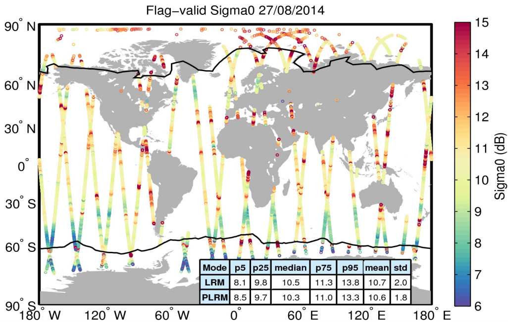
Figure 23. Geographical distribution of flag-valid sigma0 data over oceans and lakes for 27/08/2014. The statistical values shown in the table refer to the sigma0 in dB and are calculated separately for LRM and PLRM regions. Measurements taken over polar polygons have been excluded from the computation of the statistical values. The black lines mark the outer limit of the Arctic and Antarctic polar polygons.
