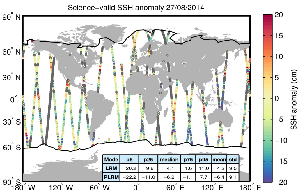
Figure 10. Geographical distribution of science-valid SSH anomaly data over oceans and lakes for 27/08/2014. The statistical values shown in the table refer to the SSH anomaly in cm and are calculated separately for LRM and PLRM regions. The black lines mark the outer limit of the Arctic and Antarctic polar polygons. Gray circles denote records that have been rejected based on the editing criteria described in Table 2.
