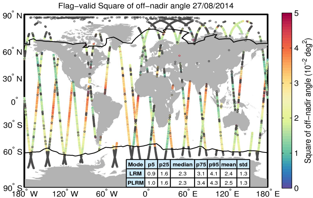
Figure 37. Geographical distribution of flag-valid mispointing data over oceans and lakes for 27/08/2014. The statistical values shown in the table refer to the mispointing in 10^{-2} \text{ deg}^2 and are calculated separately for LRM and PLRM regions. Measurements taken over polar polygons have been excluded from the computation of the statistical values. The black lines mark the outer limit of the Arctic and Antarctic polar polygons. Gray circles denote negative values.
