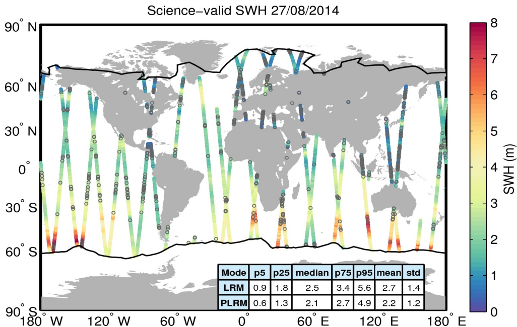
Figure 19. Geographical distribution of science-valid SWH data over oceans and lakes for 27/08/2014. The statistical values shown in the table refer to the SWH in m and are calculated separately for LRM and PLRM regions. The black lines mark the outer limit of the Arctic and Antarctic polar polygons. Gray circles denote records that have been rejected based on the editing criteria described in Table 3.
