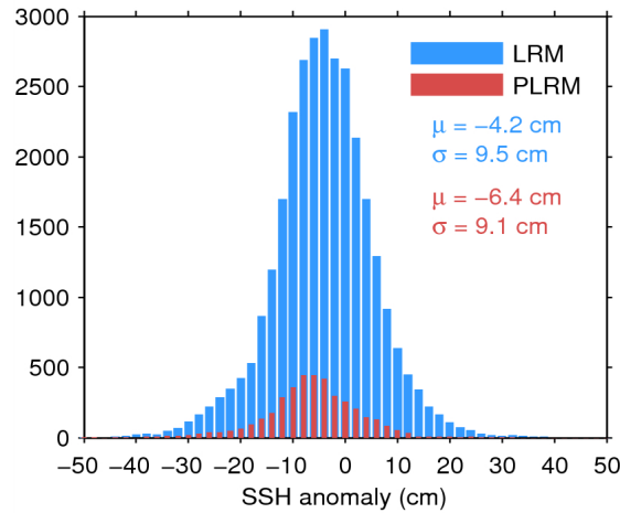
Figure 11. Histogram of science-valid SSH anomaly over oceans and lakes for LRM (blue) and PLRM (red) for 27/08/2014. The mean ( \mu ) and standard deviation ( \sigma ) are also shown. Note that values outside [-50 50] cm are excluded from the histogram for the sake of readability but not from the computation of \mu and \sigma .
