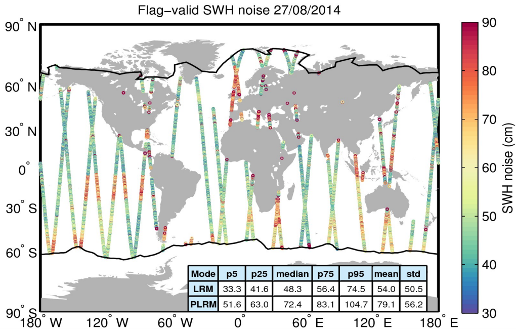
Figure 18. Geographical distribution of flag-valid 20-Hz SWH measurement noise over oceans and lakes for 27/08/2014. The statistical values shown in the table refer to the SWH noise and are calculated separately for LRM and PLRM regions. Measurements taken over polar polygons have been excluded from the computation of the statistical values. The black lines mark the outer limit of the Arctic and Antarctic polar polygons.
