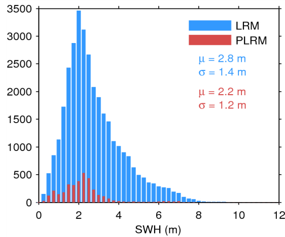
Figure 20. Histogram of science-valid SWH over oceans and lakes for LRM (blue) and PLRM (red) for 26/08/2014. The mean ( \mu ) and standard deviation ( \sigma ) are also shown. Note that values larger than 12 m are excluded from the histogram for the sake of readability but not from the computation of \mu and \sigma .
