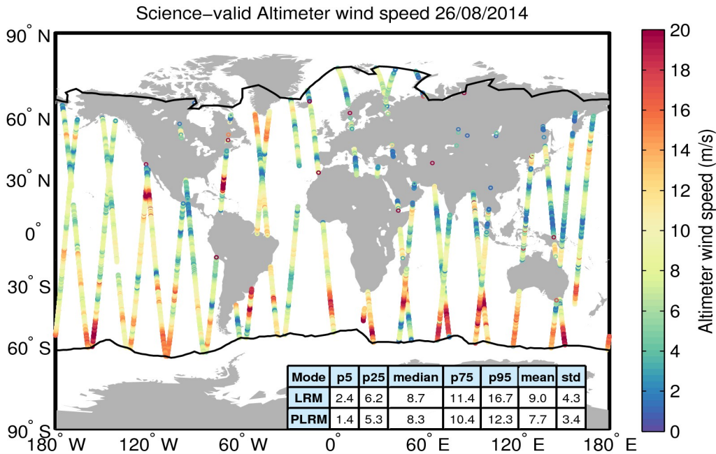
Figure 34. Geographical distribution of science-valid wind data over oceans and lakes for 26/08/2014. The statistical values shown in the table refer to the wind in m/s and are calculated separately for LRM and PLRM regions. The black lines mark the outer limit of the Arctic and Antarctic polar polygons. Gray circles denote records that have been rejected based on the editing criteria described in Table 5.
