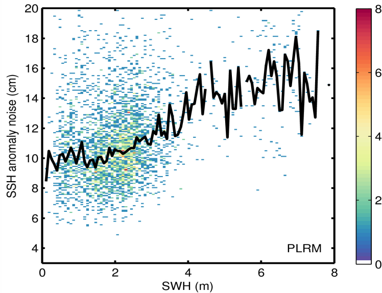
Figure 9. 2D histogram showing flag-valid SSH anomaly noise as a function of SWH for LRM (top) and PLRM (bottom) for 26/08/2014. The black line denotes the median SSH anomaly as a function of SWH.
