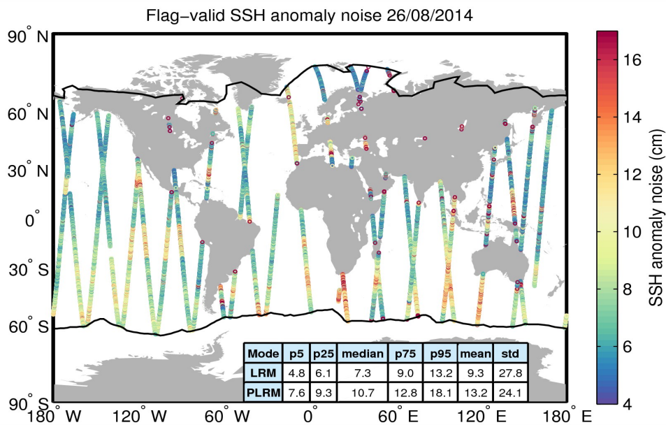
Figure 8. Geographical distribution of flag-valid 20-Hz SSH anomaly measurement noise over oceans and lakes for 26/08/2014. The statistical values shown in the table refer to the SSH anomaly noise and are calculated separately for LRM and PLRM regions. Measurements taken over polar polygons have been excluded from the computation of the statistical values. The black lines mark the outer limit of the Arctic and Antarctic polar polygons.
