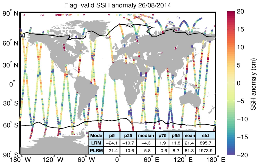
Figure 5. Geographical distribution of flag-valid 1-Hz SSH anomaly data over oceans and lakes for 26/08/2014. The statistical values shown in the table refer to the SSH anomaly in cm and are calculated separately for LRM and PLRM regions. Measurements taken over polar polygons have been excluded from the computation of the statistical values. The black lines mark the outer limit of the Arctic and Antarctic polar polygons.
