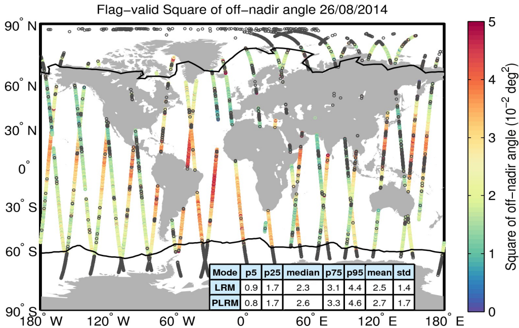
Figure 37. Geographical distribution of flag-valid mispointing data over oceans and lakes for 26/08/2014. The statistical values shown in the table refer to the mispointing in 10^{-2} deg 2 and are calculated separately for LRM and PLRM regions. Measurements taken over polar polygons have been excluded from the computation of the statistical values. The black lines mark the outer limit of the Arctic and Antarctic polar polygons. Gray circles denote negative values.
