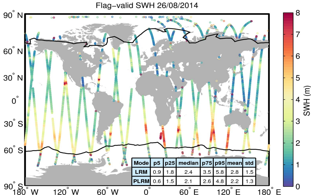
Figure 15. Geographical distribution of flag-valid SWH data over oceans and lakes for 26/08/2014. The statistical values shown in the table refer to the SWH in m and are calculated separately for LRM and PLRM regions. Measurements taken over polar polygons have been excluded from the computation of the statistical values. The black lines mark the outer limit of the Arctic and Antarctic polar polygons.
