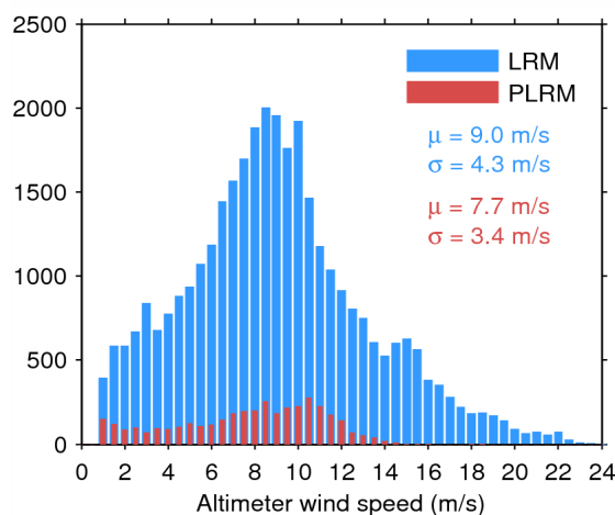
Figure 33. Histogram of flag-valid wind over oceans and lakes for LRM (blue) and PLRM (red) for 26/08/2014. The mean ( \mu ) and standard deviation ( \sigma ) are also shown. Note that values larger than 24 m/s are excluded from the histogram for the sake of readability but not from the computation of \mu and \sigma .
