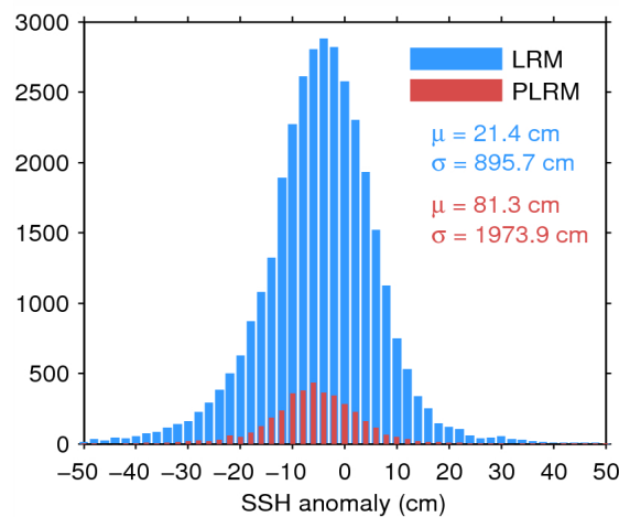
Figure 7. Histogram of flag-valid SSH anomaly over oceans and lakes for LRM (blue) and PLRM (red) for 26/08/2014. The mean ( \mu ) and standard deviation ( \sigma ) are also shown. Note that values outside [-50\ 50] cm are excluded from the histogram for the sake of readability but not from the computation of \mu and \sigma .
