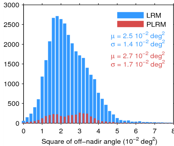
Figure 39. Histogram of flag-valid mispointing over oceans and lakes for LRM (blue) and PLRM (red) for 26/08/2014. Only positive values have been considered. The mean ( \mu ) and standard deviation ( \sigma ) are also shown. Note that values larger than 8 \cdot 10^{-2} \text{ deg}^2 are excluded from the histogram for the sake of readability but not from the computation of \mu and \sigma .
