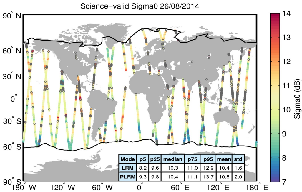
Figure 27. Geographical distribution of science-valid sigma0 data over oceans and lakes for 26/08/2014. The statistical values shown in the table refer to the sigma0 in dB and are calculated separately for LRM and PLRM regions. The black lines mark the outer limit of the Arctic and Antarctic polar polygons. Gray circles denote records that have been rejected based on the editing criteria described in Table 4.
