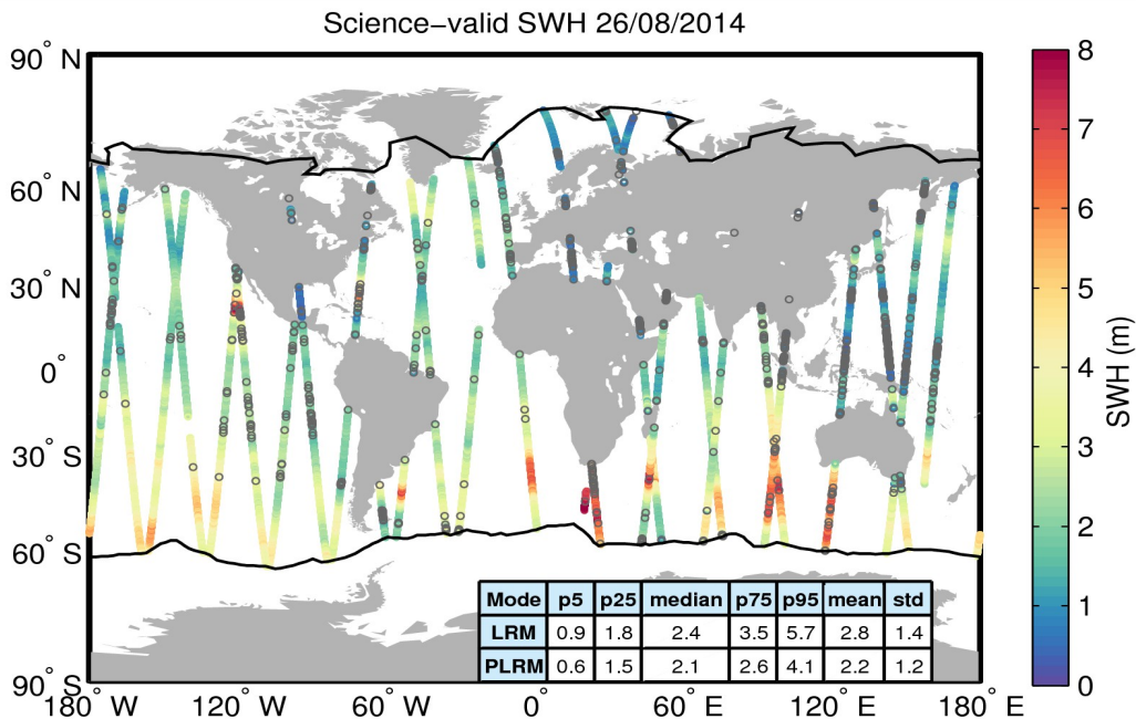
Figure 19. Geographical distribution of science-valid SWH data over oceans and lakes for 26/08/2014. The statistical values shown in the table refer to the SWH in m and are calculated separately for LRM and PLRM regions. The black lines mark the outer limit of the Arctic and Antarctic polar polygons. Gray circles denote records that have been rejected based on the editing criteria described in Table 3.
