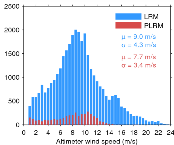
Figure 35. Histogram of science-valid wind over oceans and lakes for LRM (blue) and PLRM (red) for 26/08/2014. The mean ( \mu ) and standard deviation ( \sigma ) are also shown. Note that values larger than 24 m/s are excluded from the histogram for the sake of readability but not from the computation of \mu and \sigma .
