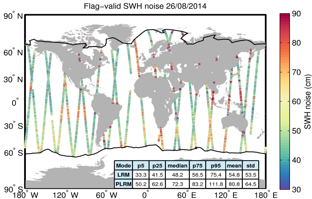
Figure 18. Geographical distribution of flag-valid 20-Hz SWH measurement noise over oceans and lakes for 26/08/2014. The statistical values shown in the table refer to the SWH noise and are calculated separately for LRM and PLRM regions. Measurements taken over polar polygons have been excluded from the computation of the statistical values. The black lines mark the outer limit of the Arctic and Antarctic polar polygons.
