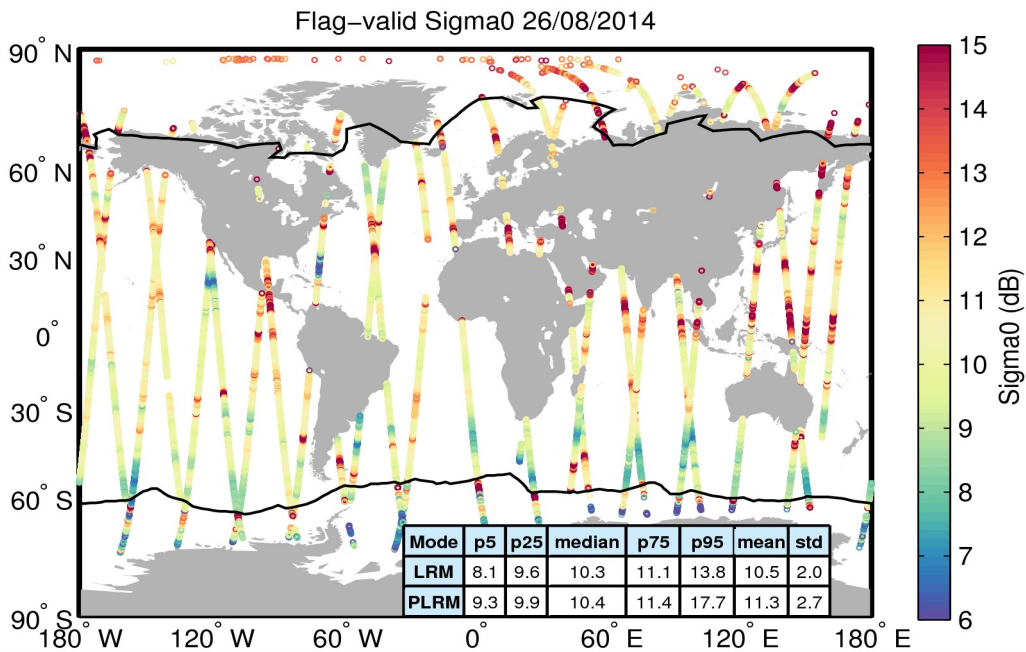
Figure 23. Geographical distribution of flag-valid sigma0 data over oceans and lakes for 26/08/2014. The statistical values shown in the table refer to the sigma0 in dB and are calculated separately for LRM and PLRM regions. Measurements taken over polar polygons have been excluded from the computation of the statistical values. The black lines mark the outer limit of the Arctic and Antarctic polar polygons.
