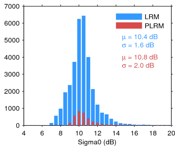
Figure 28. Histogram of science-valid sigma0 over oceans and lakes for LRM (blue) and PLRM (red) for 26/08/2014. The mean ( \mu ) and standard deviation ( \sigma ) are also shown. Note that values outside [4 20] dB are excluded from the histogram for the sake of readability but not from the computation of \mu and \sigma .
