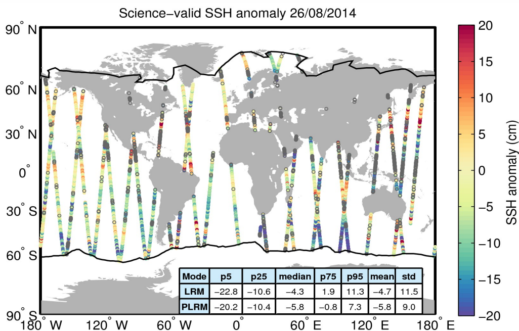
Figure 10. Geographical distribution of science-valid SSH anomaly data over oceans and lakes for 26/08/2014. The statistical values shown in the table refer to the SSH anomaly in cm and are calculated separately for LRM and PLRM regions. The black lines mark the outer limit of the Arctic and Antarctic polar polygons. Gray circles denote records that have been rejected based on the editing criteria described in Table 2.
