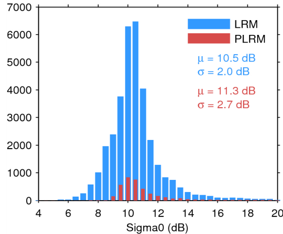
Figure 25. Histogram of flag-valid sigma0 over oceans and lakes for LRM (blue) and PLRM (red) for 26/08/2014. The mean ( \mu ) and standard deviation ( \sigma ) are also shown. Note that values outside [4 20] dB are excluded from the histogram for the sake of readability but not from the computation of \mu and \sigma .
