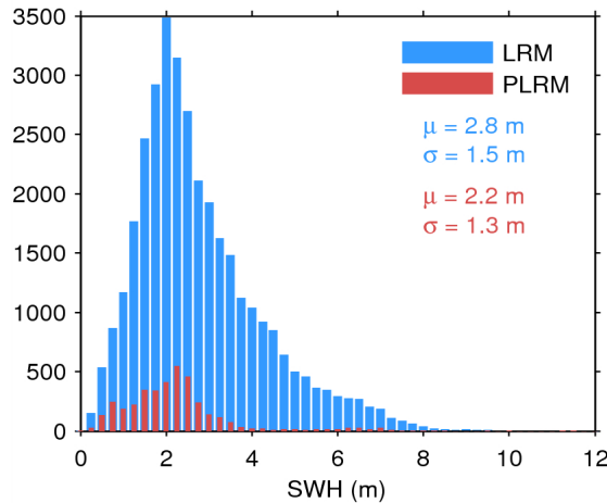
Figure 17. Histogram of flag-valid SWH over oceans and lakes for LRM (blue) and PLRM (red) for 26/08/2014. The mean ( \mu ) and standard deviation ( \sigma ) are also shown. Note that values larger than 12 m are excluded from the histogram for the sake of readability but not from the computation of \mu and \sigma .
