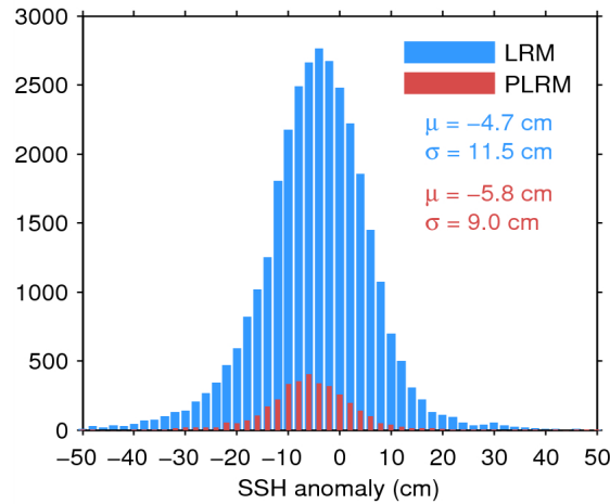
Figure 11. Histogram of science-valid SSH anomaly over oceans and lakes for LRM (blue) and PLRM (red) for 26/08/2014. The mean ( \mu ) and standard deviation ( \sigma ) are also shown. Note that values outside [-50 50] cm are excluded from the histogram for the sake of readability but not from the computation of \mu and \sigma .
