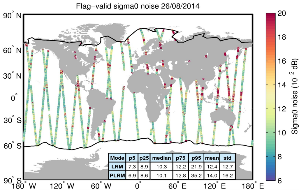
Figure 26. Geographical distribution of flag-valid 20-Hz sigma0 measurement noise over oceans and lakes for 26/08/2014. The statistical values shown in the table refer to the sigma0 noise and are calculated separately for LRM and PLRM regions. Measurements taken over polar polygons have been excluded from the computation of the statistical values. The black lines mark the outer limit of the Arctic and Antarctic polar polygons.
