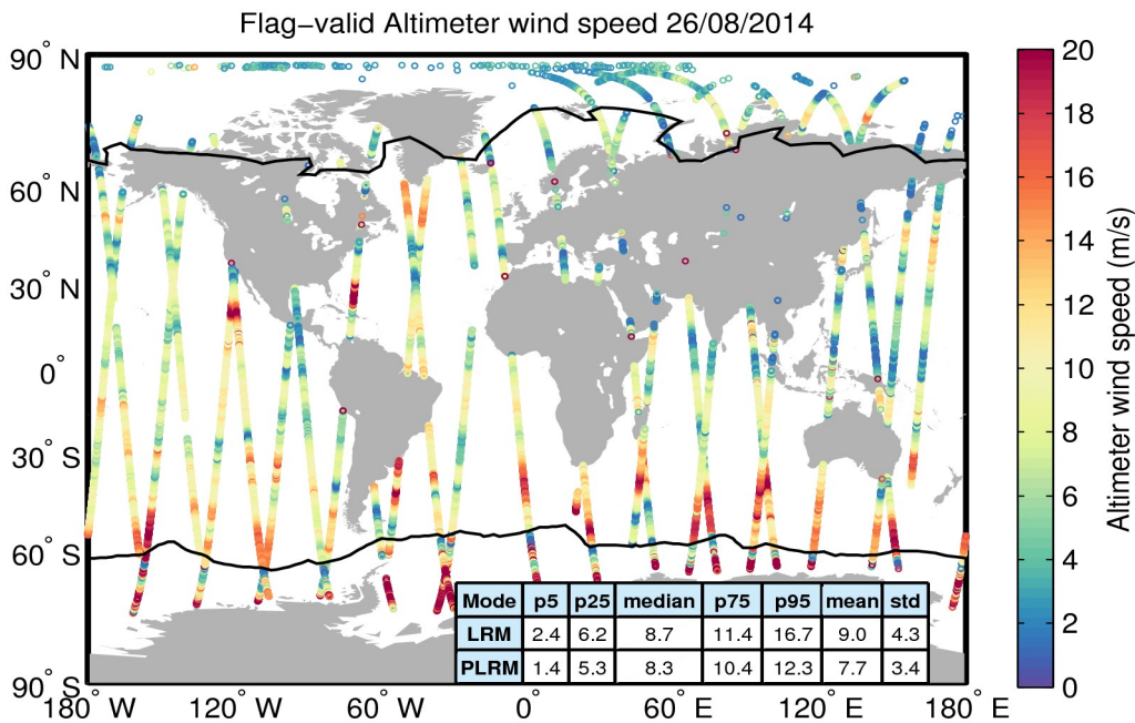
Figure 31. Geographical distribution of flag-valid wind data over oceans and lakes for 26/08/2014. The statistical values shown in the table refer to the wind in m/s and are calculated separately for LRM and PLRM regions. Measurements taken over polar polygons have been excluded from the computation of the statistical values. The black lines mark the outer limit of the Arctic and Antarctic polar polygons.
