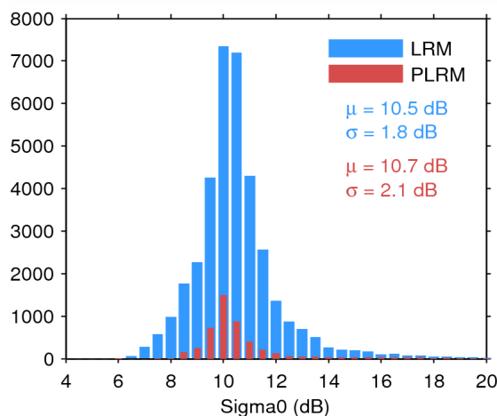
Figure 25. Histogram of flag-valid sigma0 over oceans and lakes for LRM (blue) and PLRM (red) for 25/08/2014. The mean ( \mu ) and standard deviation ( \sigma ) are also shown. Note that values outside [4 20] dB are excluded from the histogram for the sake of readability but not from the computation of \mu and \sigma .
