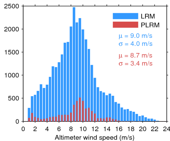
Figure 35. Histogram of science-valid wind over oceans and lakes for LRM (blue) and PLRM (red) for 25/08/2014. The mean ( \mu ) and standard deviation ( \sigma ) are also shown. Note that values larger than 24 m/s are excluded from the histogram for the sake of readability but not from the computation of \mu and \sigma .
