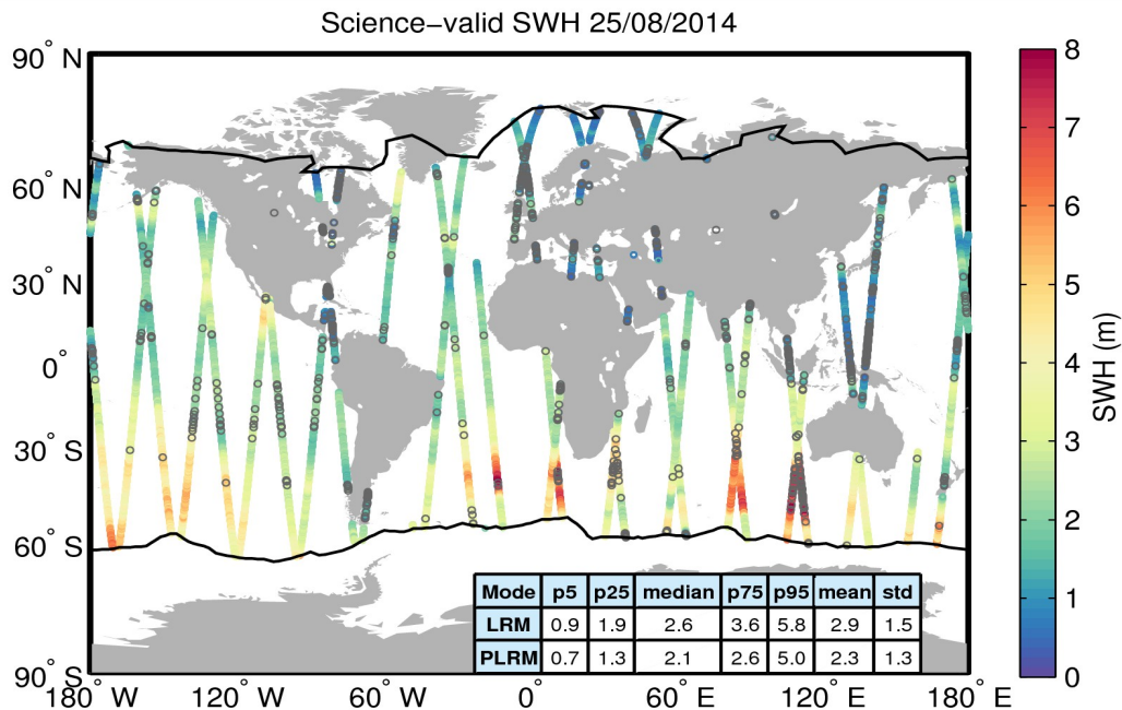
Figure 19. Geographical distribution of science-valid SWH data over oceans and lakes for 25/08/2014. The statistical values shown in the table refer to the SWH in m and are calculated separately for LRM and PLRM regions. The black lines mark the outer limit of the Arctic and Antarctic polar polygons. Gray circles denote records that have been rejected based on the editing criteria described in Table 3.
