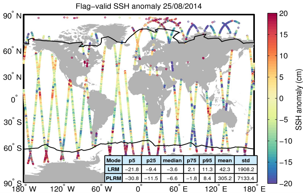
Figure 5. Geographical distribution of flag-valid 1-Hz SSH anomaly data over oceans and lakes for 25/08/2014. The statistical values shown in the table refer to the SSH anomaly in cm and are calculated separately for LRM and PLRM regions. Measurements taken over polar polygons have been excluded from the computation of the statistical values. The black lines mark the outer limit of the Arctic and Antarctic polar polygons.
