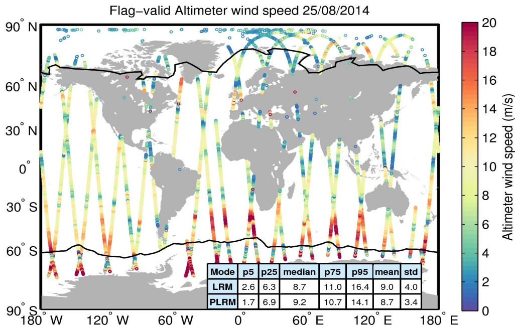
Figure 31. Geographical distribution of flag-valid wind data over oceans and lakes for 25/08/2014. The statistical values shown in the table refer to the wind in m/s and are calculated separately for LRM and PLRM regions. Measurements taken over polar polygons have been excluded from the computation of the statistical values. The black lines mark the outer limit of the Arctic and Antarctic polar polygons.
