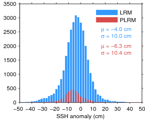
Figure 11. Histogram of science-valid SSH anomaly over oceans and lakes for LRM (blue) and PLRM (red) for 25/08/2014. The mean ( \mu ) and standard deviation ( \sigma ) are also shown. Note that values outside [-50\ 50] cm are excluded from the histogram for the sake of readability but not from the computation of \mu and \sigma .
