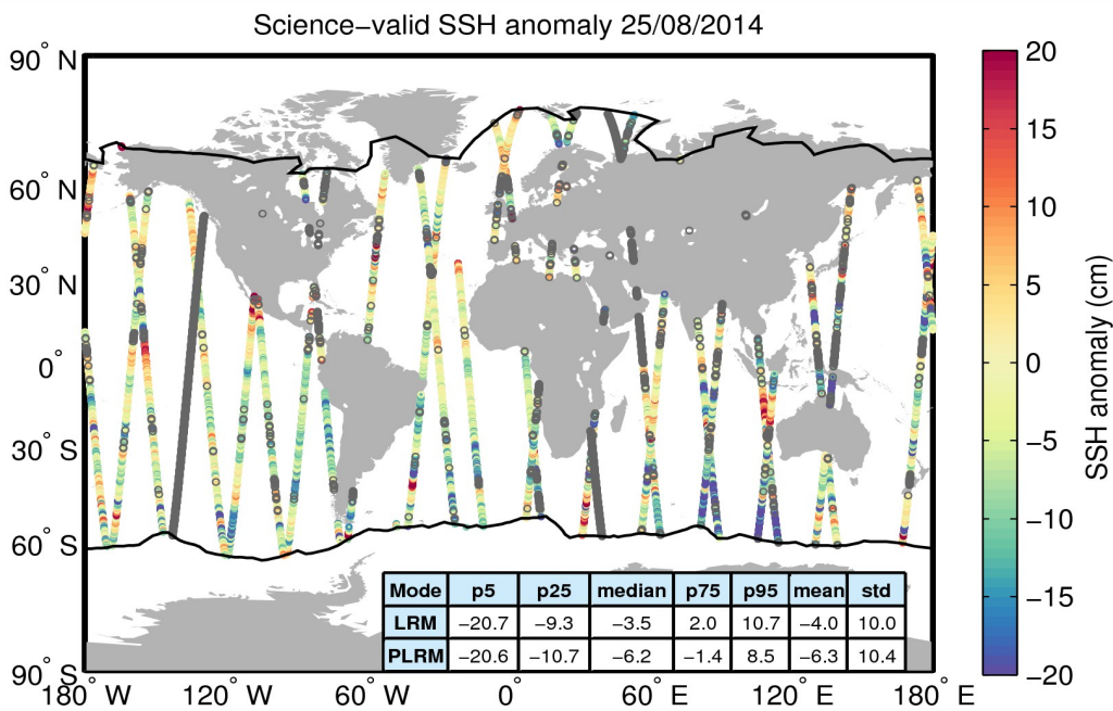
Figure 10. Geographical distribution of science-valid SSH anomaly data over oceans and lakes for 25/08/2014. The statistical values shown in the table refer to the SSH anomaly in cm and are calculated separately for LRM and PLRM regions. The black lines mark the outer limit of the Arctic and Antarctic polar polygons. Gray circles denote records that have been rejected based on the editing criteria described in Table 2.
