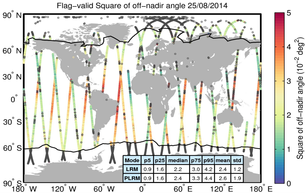
Figure 37. Geographical distribution of flag-valid mispointing data over oceans and lakes for 25/08/2014. The statistical values shown in the table refer to the mispointing in 10^{-2} \text{ deg}^2 and are calculated separately for LRM and PLRM regions. Measurements taken over polar polygons have been excluded from the computation of the statistical values. The black lines mark the outer limit of the Arctic and Antarctic polar polygons. Gray circles denote negative values.
