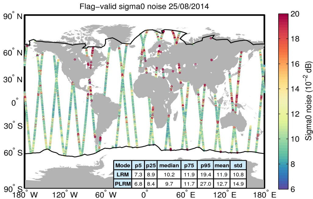
Figure 26. Geographical distribution of flag-valid 20-Hz sigma0 measurement noise over oceans and lakes for 25/08/2014. The statistical values shown in the table refer to the sigma0 noise and are calculated separately for LRM and PLRM regions. Measurements taken over polar polygons have been excluded from the computation of the statistical values. The black lines mark the outer limit of the Arctic and Antarctic polar polygons.
