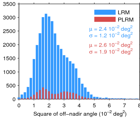
Figure 39. Histogram of flag-valid mispointing over oceans and lakes for LRM (blue) and PLRM (red) for 25/08/2014. Only positive values have been considered. The mean ( \mu ) and standard deviation ( \sigma ) are also shown. Note that values larger than 8 \cdot 10^{-2} \text{ deg}^2 are excluded from the histogram for the sake of readability but not from the computation of \mu and \sigma .
