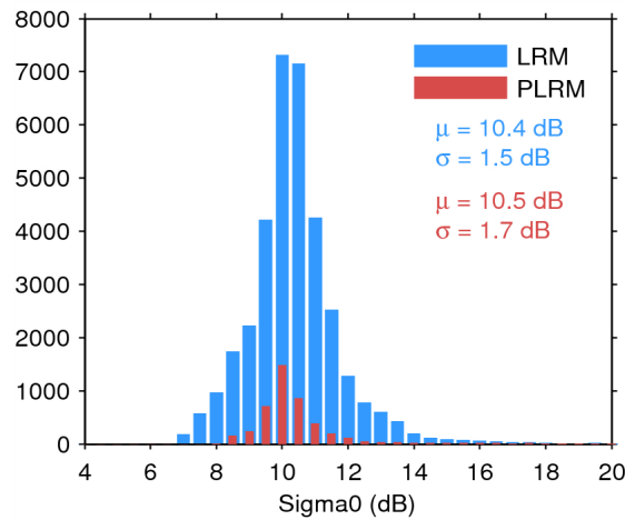
Figure 28. Histogram of science-valid sigma0 over oceans and lakes for LRM (blue) and PLRM (red) for 25/08/2014. The mean ( \mu ) and standard deviation ( \sigma ) are also shown. Note that values outside [4 20] dB are excluded from the histogram for the sake of readability but not from the computation of \mu and \sigma .
