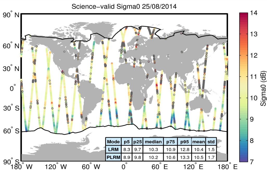
Figure 27. Geographical distribution of science-valid sigma0 data over oceans and lakes for 25/08/2014. The statistical values shown in the table refer to the sigma0 in dB and are calculated separately for LRM and PLRM regions. The black lines mark the outer limit of the Arctic and Antarctic polar polygons. Gray circles denote records that have been rejected based on the editing criteria described in Table 4.
