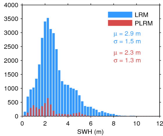
Figure 20. Histogram of science-valid SWH over oceans and lakes for LRM (blue) and PLRM (red) for 25/08/2014. The mean ( \mu ) and standard deviation ( \sigma ) are also shown. Note that values larger than 12 m are excluded from the histogram for the sake of readability but not from the computation of \mu and \sigma .
