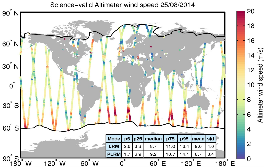
Figure 34. Geographical distribution of science-valid wind data over oceans and lakes for 25/08/2014. The statistical values shown in the table refer to the wind in m/s and are calculated separately for LRM and PLRM regions. The black lines mark the outer limit of the Arctic and Antarctic polar polygons. Gray circles denote records that have been rejected based on the editing criteria described in Table 5.
