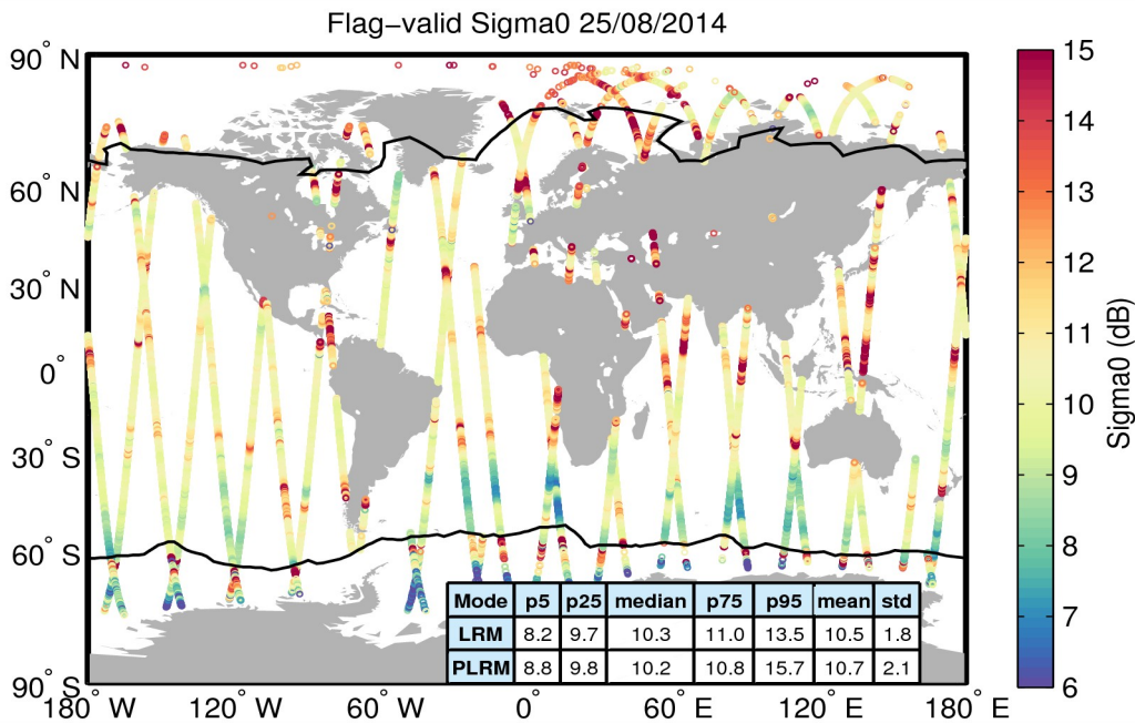
Figure 23. Geographical distribution of flag-valid sigma0 data over oceans and lakes for 25/08/2014. The statistical values shown in the table refer to the sigma0 in dB and are calculated separately for LRM and PLRM regions. Measurements taken over polar polygons have been excluded from the computation of the statistical values. The black lines mark the outer limit of the Arctic and Antarctic polar polygons.
