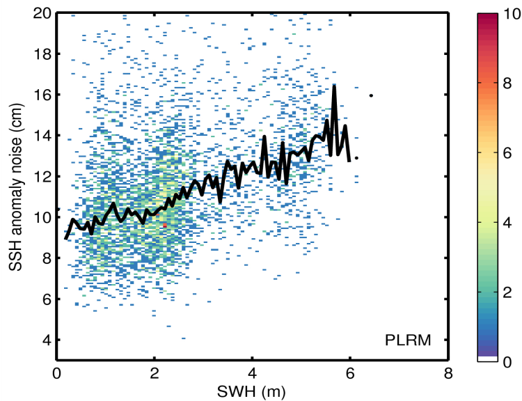
Figure 9. 2D histogram showing flag-valid SSH anomaly noise as a function of SWH for LRM (top) and PLRM (bottom) for 25/08/2014. The black line denotes the median SSH anomaly as a function of SWH.
