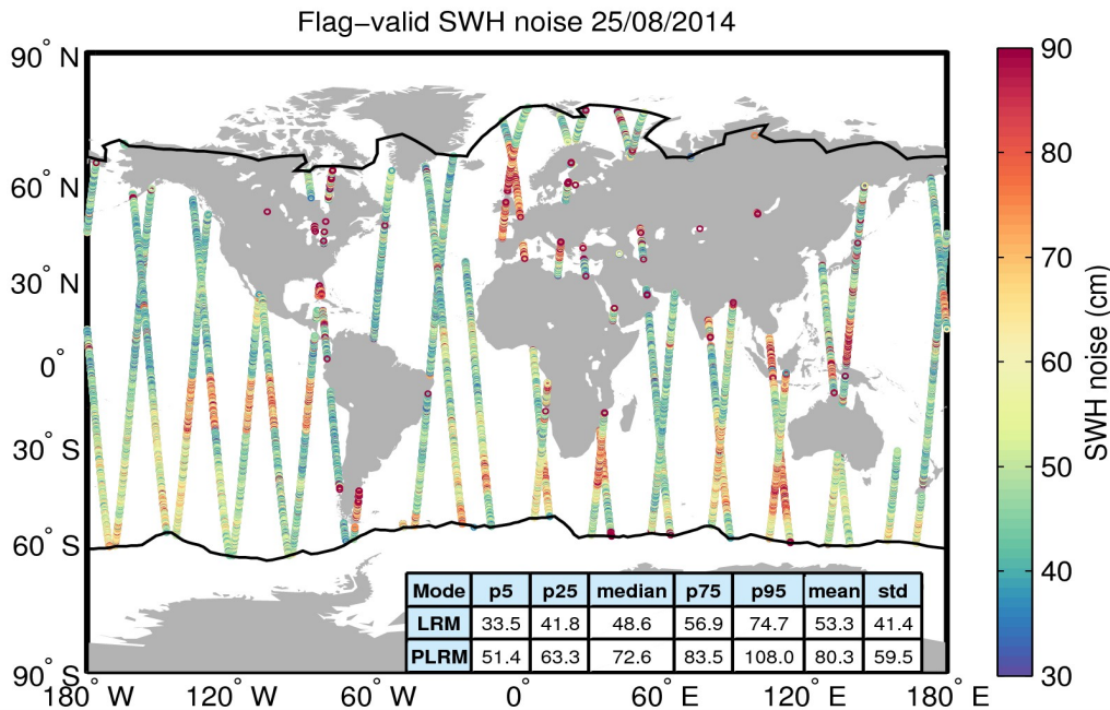
Figure 18. Geographical distribution of flag-valid 20-Hz SWH measurement noise over oceans and lakes for 25/08/2014. The statistical values shown in the table refer to the SWH noise and are calculated separately for LRM and PLRM regions. Measurements taken over polar polygons have been excluded from the computation of the statistical values. The black lines mark the outer limit of the Arctic and Antarctic polar polygons.
