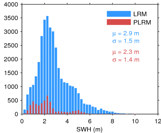
Figure 17. Histogram of flag-valid SWH over oceans and lakes for LRM (blue) and PLRM (red) for 25/08/2014. The mean ( \mu ) and standard deviation ( \sigma ) are also shown. Note that values larger than 12 m are excluded from the histogram for the sake of readability but not from the computation of \mu and \sigma .
