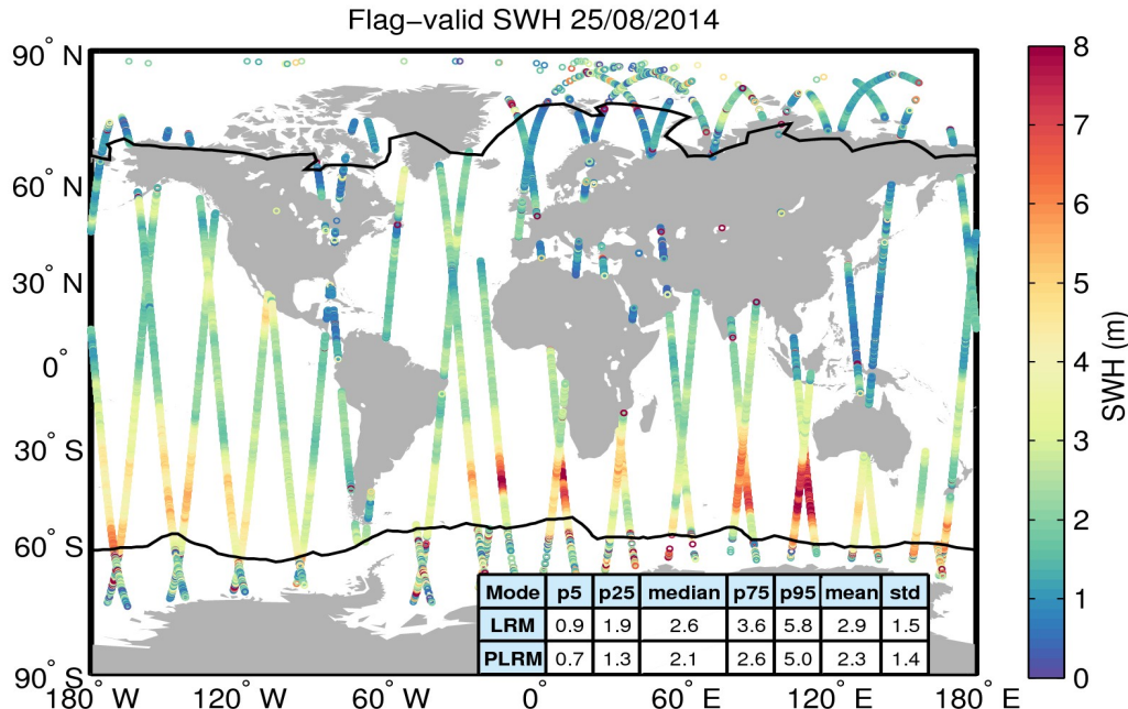
Figure 15. Geographical distribution of flag-valid SWH data over oceans and lakes for 25/08/2014. The statistical values shown in the table refer to the SWH in m and are calculated separately for LRM and PLRM regions. Measurements taken over polar polygons have been excluded from the computation of the statistical values. The black lines mark the outer limit of the Arctic and Antarctic polar polygons.
