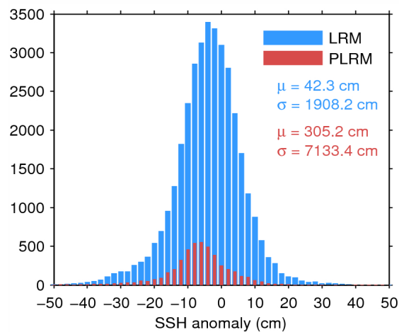
Figure 7. Histogram of flag-valid SSH anomaly over oceans and lakes for LRM (blue) and PLRM (red) for 25/08/2014. The mean ( \mu ) and standard deviation ( \sigma ) are also shown. Note that values outside [-50\ 50] cm are excluded from the histogram for the sake of readability but not from the computation of \mu and \sigma .
