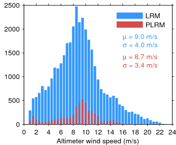
Figure 33. Histogram of flag-valid wind over oceans and lakes for LRM (blue) and PLRM (red) for 25/08/2014. The mean ( \mu ) and standard deviation ( \sigma ) are also shown. Note that values larger than 24 m/s are excluded from the histogram for the sake of readability but not from the computation of \mu and \sigma .
