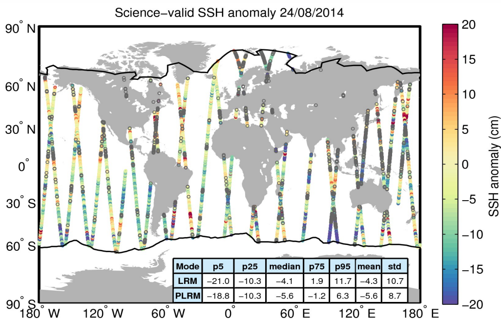
Figure 10. Geographical distribution of science-valid SSH anomaly data over oceans and lakes for 24/08/2014. The statistical values shown in the table refer to the SSH anomaly in cm and are calculated separately for LRM and PLRM regions. The black lines mark the outer limit of the Arctic and Antarctic polar polygons. Gray circles denote records that have been rejected based on the editing criteria described in Table 2.
