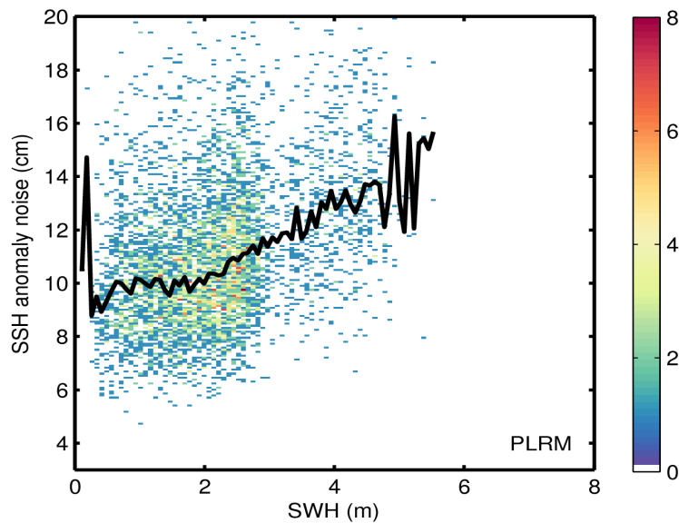
Figure 9. 2D histogram showing flag-valid SSH anomaly noise as a function of SWH for LRM (top) and PLRM (bottom) for 24/08/2014. The black line denotes the median SSH anomaly as a function of SWH.
