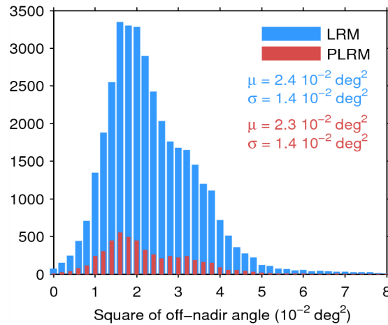
Figure 39. Histogram of flag-valid mispointing over oceans and lakes for LRM (blue) and PLRM (red) for 24/08/2014. Only positive values have been considered. The mean ( \mu ) and standard deviation ( \sigma ) are also shown. Note that values larger than 8 \cdot 10^{-2} \text{ deg}^2 are excluded from the histogram for the sake of readability but not from the computation of \mu and \sigma .
