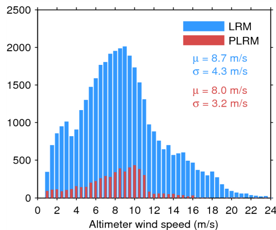
Figure 35. Histogram of science-valid wind over oceans and lakes for LRM (blue) and PLRM (red) for 24/08/2014. The mean ( \mu ) and standard deviation ( \sigma ) are also shown. Note that values larger than 24 m/s are excluded from the histogram for the sake of readability but not from the computation of \mu and \sigma .
