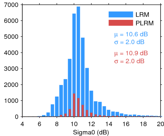
Figure 25. Histogram of flag-valid sigma0 over oceans and lakes for LRM (blue) and PLRM (red) for 24/08/2014. The mean ( \mu ) and standard deviation ( \sigma ) are also shown. Note that values outside [4 20] dB are excluded from the histogram for the sake of readability but not from the computation of \mu and \sigma .
