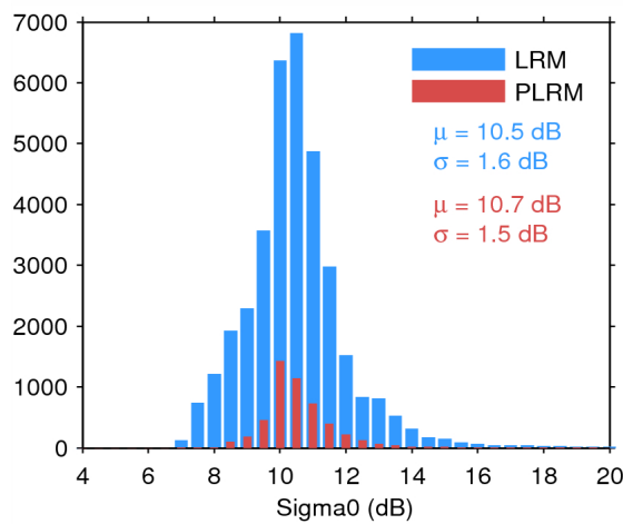
Figure 28. Histogram of science-valid sigma0 over oceans and lakes for LRM (blue) and PLRM (red) for 24/08/2014. The mean ( \mu ) and standard deviation ( \sigma ) are also shown. Note that values outside [4 20] dB are excluded from the histogram for the sake of readability but not from the computation of \mu and \sigma .
