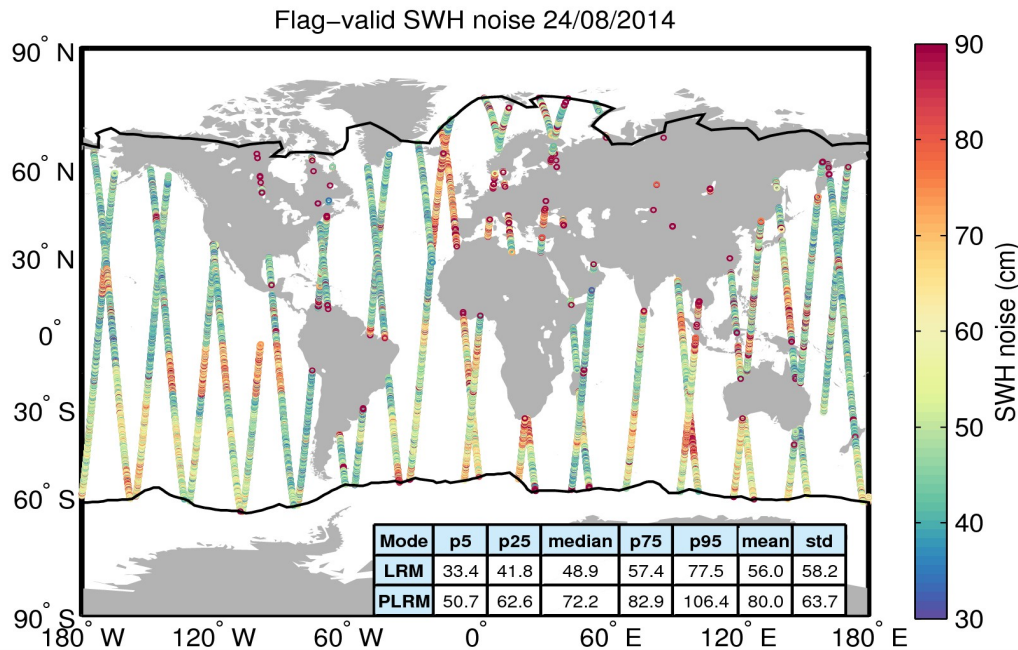
Figure 18. Geographical distribution of flag-valid 20-Hz SWH measurement noise over oceans and lakes for 24/08/2014. The statistical values shown in the table refer to the SWH noise and are calculated separately for LRM and PLRM regions. Measurements taken over polar polygons have been excluded from the computation of the statistical values. The black lines mark the outer limit of the Arctic and Antarctic polar polygons.
