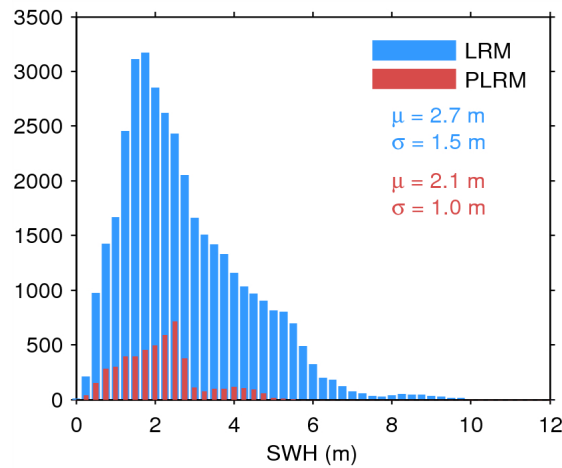
Figure 20. Histogram of science-valid SWH over oceans and lakes for LRM (blue) and PLRM (red) for 24/08/2014. The mean ( \mu ) and standard deviation ( \sigma ) are also shown. Note that values larger than 12 m are excluded from the histogram for the sake of readability but not from the computation of \mu and \sigma .
