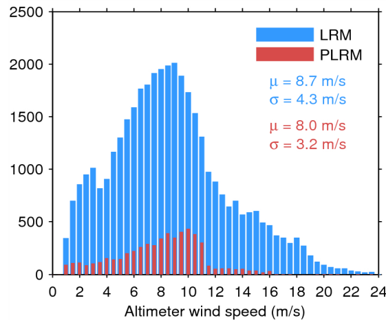
Figure 33. Histogram of flag-valid wind over oceans and lakes for LRM (blue) and PLRM (red) for 24/08/2014. The mean ( \mu ) and standard deviation ( \sigma ) are also shown. Note that values larger than 24 m/s are excluded from the histogram for the sake of readability but not from the computation of \mu and \sigma .
