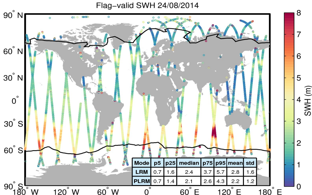
Figure 15. Geographical distribution of flag-valid SWH data over oceans and lakes for 24/08/2014. The statistical values shown in the table refer to the SWH in m and are calculated separately for LRM and PLRM regions. Measurements taken over polar polygons have been excluded from the computation of the statistical values. The black lines mark the outer limit of the Arctic and Antarctic polar polygons.
