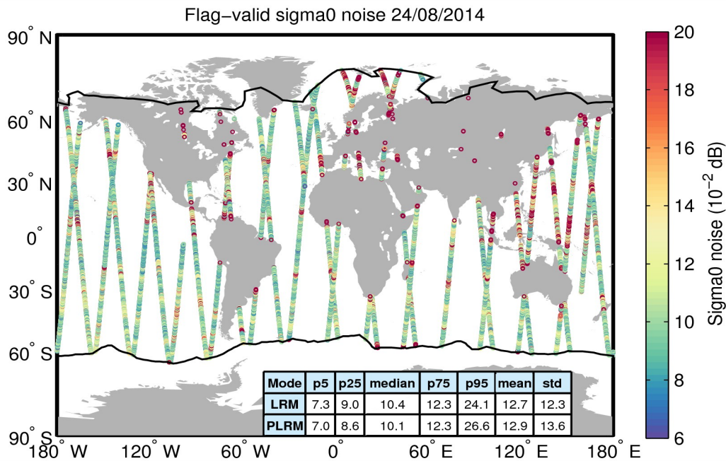
Figure 26. Geographical distribution of flag-valid 20-Hz sigma0 measurement noise over oceans and lakes for 24/08/2014. The statistical values shown in the table refer to the sigma0 noise and are calculated separately for LRM and PLRM regions. Measurements taken over polar polygons have been excluded from the computation of the statistical values. The black lines mark the outer limit of the Arctic and Antarctic polar polygons.
