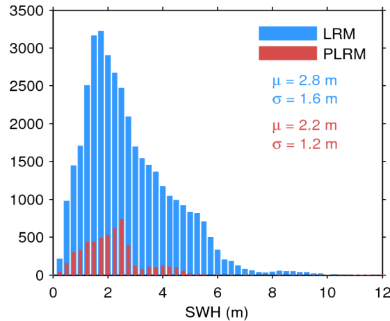
Figure 17. Histogram of flag-valid SWH over oceans and lakes for LRM (blue) and PLRM (red) for 24/08/2014. The mean ( \mu ) and standard deviation ( \sigma ) are also shown. Note that values larger than 12 m are excluded from the histogram for the sake of readability but not from the computation of \mu and \sigma .
