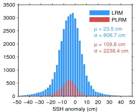
Figure 7. Histogram of flag-valid SSH anomaly over oceans and lakes for LRM (blue) and PLRM (red) for 24/08/2014. The mean ( \mu ) and standard deviation ( \sigma ) are also shown. Note that values outside [-50\ 50] cm are excluded from the histogram for the sake of readability but not from the computation of \mu and \sigma .
