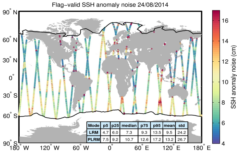
Figure 8. Geographical distribution of flag-valid 20-Hz SSH anomaly measurement noise over oceans and lakes for 24/08/2014. The statistical values shown in the table refer to the SSH anomaly noise and are calculated separately for LRM and PLRM regions. Measurements taken over polar polygons have been excluded from the computation of the statistical values. The black lines mark the outer limit of the Arctic and Antarctic polar polygons.
