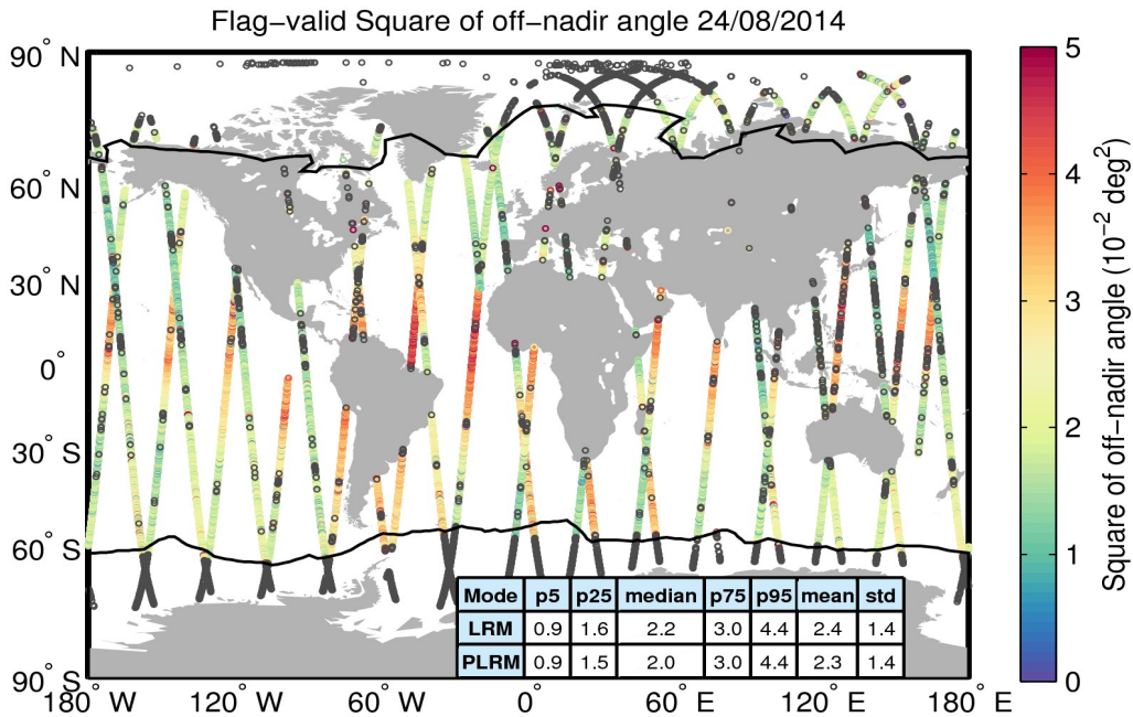
Figure 37. Geographical distribution of flag-valid mispointing data over oceans and lakes for 24/08/2014. The statistical values shown in the table refer to the mispointing in 10^{-2} \text{ deg}^2 and are calculated separately for LRM and PLRM regions. Measurements taken over polar polygons have been excluded from the computation of the statistical values. The black lines mark the outer limit of the Arctic and Antarctic polar polygons. Gray circles denote negative values.
