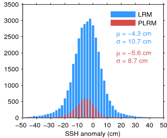
Figure 11. Histogram of science-valid SSH anomaly over oceans and lakes for LRM (blue) and PLRM (red) for 24/08/2014. The mean ( \mu ) and standard deviation ( \sigma ) are also shown. Note that values outside [-50 50] cm are excluded from the histogram for the sake of readability but not from the computation of \mu and \sigma .
