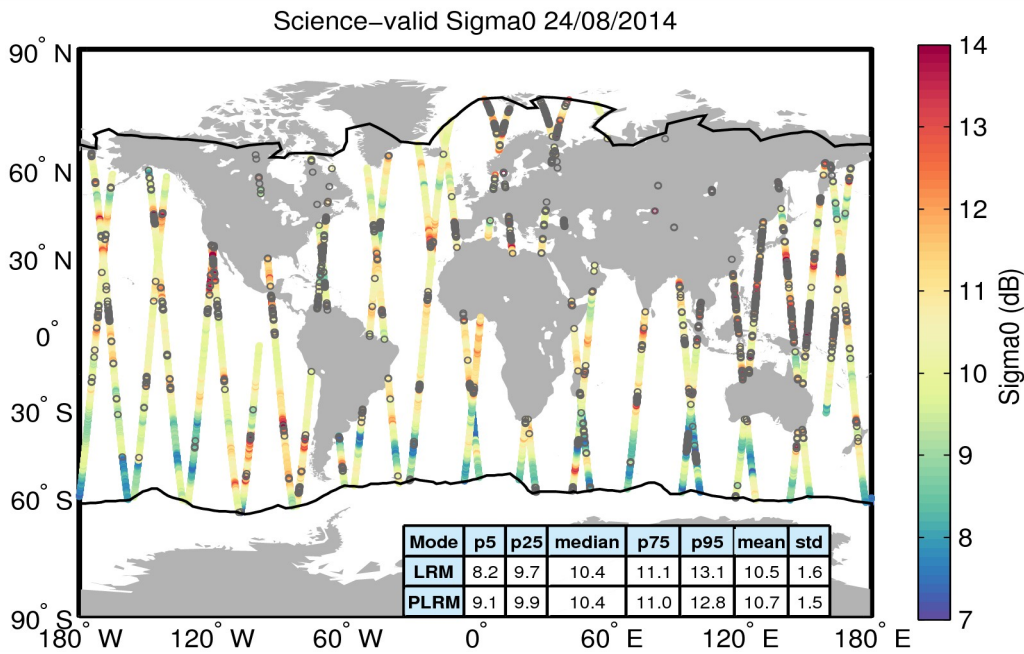
Figure 27. Geographical distribution of science-valid sigma0 data over oceans and lakes for 24/08/2014. The statistical values shown in the table refer to the sigma0 in dB and are calculated separately for LRM and PLRM regions. The black lines mark the outer limit of the Arctic and Antarctic polar polygons. Gray circles denote records that have been rejected based on the editing criteria described in Table 4.
