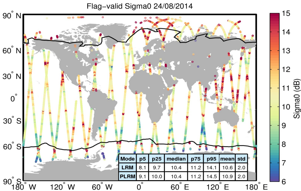
Figure 23. Geographical distribution of flag-valid sigma0 data over oceans and lakes for 24/08/2014. The statistical values shown in the table refer to the sigma0 in dB and are calculated separately for LRM and PLRM regions. Measurements taken over polar polygons have been excluded from the computation of the statistical values. The black lines mark the outer limit of the Arctic and Antarctic polar polygons.
