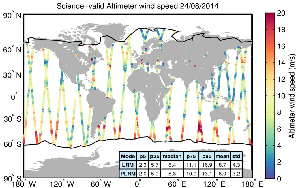
Figure 34. Geographical distribution of science-valid wind data over oceans and lakes for 24/08/2014. The statistical values shown in the table refer to the wind in m/s and are calculated separately for LRM and PLRM regions. The black lines mark the outer limit of the Arctic and Antarctic polar polygons. Gray circles denote records that have been rejected based on the editing criteria described in Table 5.
