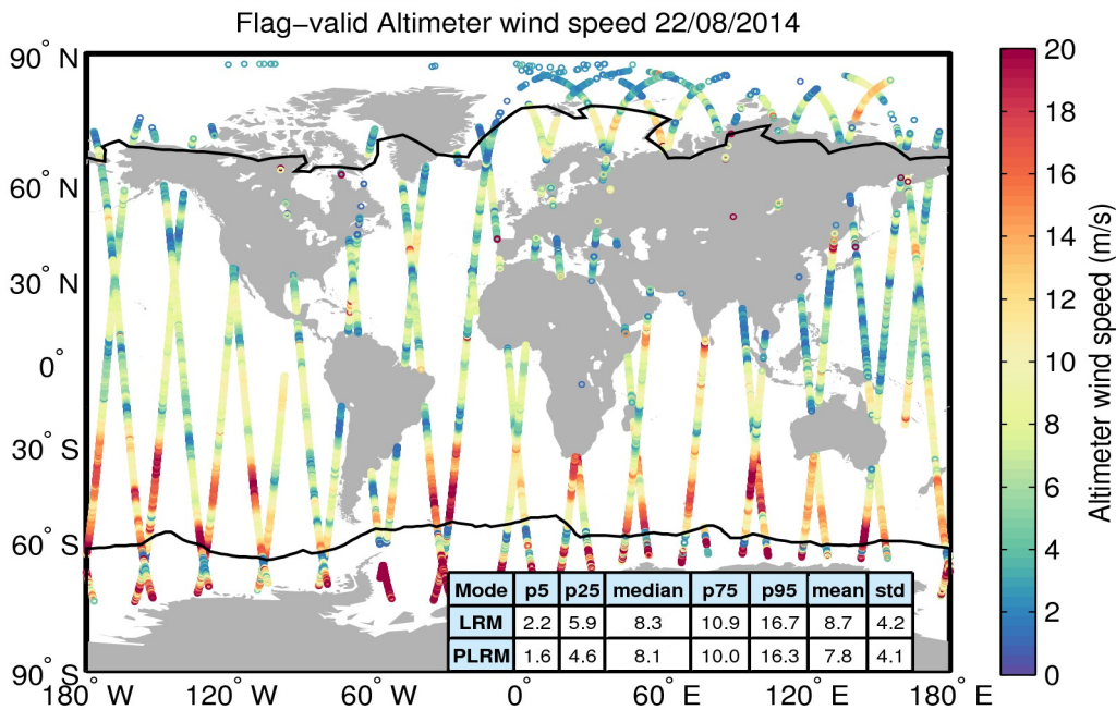
Figure 31. Geographical distribution of flag-valid wind data over oceans and lakes for 22/08/2014. The statistical values shown in the table refer to the wind in m/s and are calculated separately for LRM and PLRM regions. Measurements taken over polar polygons have been excluded from the computation of the statistical values. The black lines mark the outer limit of the Arctic and Antarctic polar polygons.
