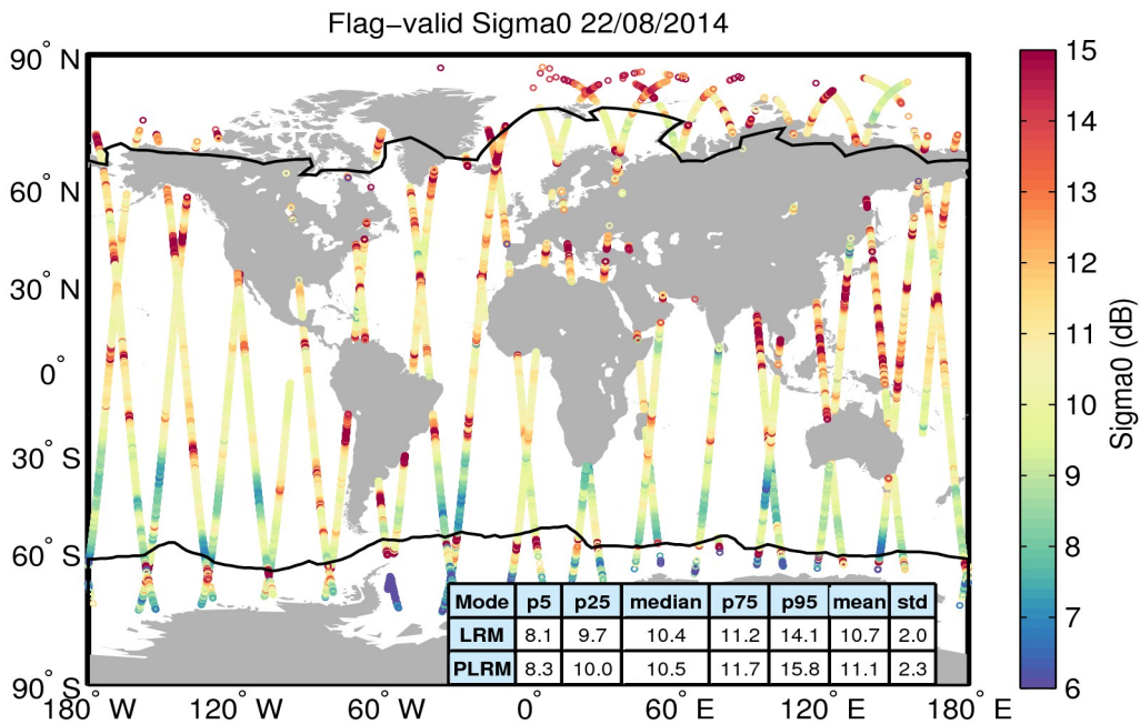
Figure 23. Geographical distribution of flag-valid sigma0 data over oceans and lakes for 22/08/2014. The statistical values shown in the table refer to the sigma0 in dB and are calculated separately for LRM and PLRM regions. Measurements taken over polar polygons have been excluded from the computation of the statistical values. The black lines mark the outer limit of the Arctic and Antarctic polar polygons.
