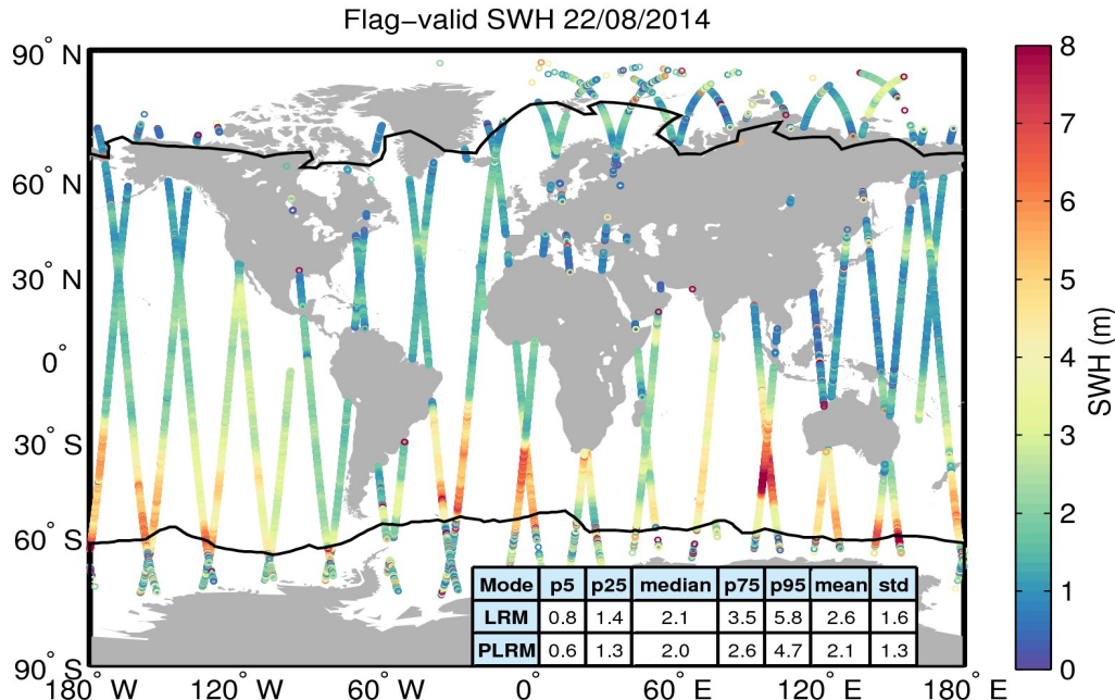
Figure 15. Geographical distribution of flag-valid SWH data over oceans and lakes for 22/08/2014. The statistical values shown in the table refer to the SWH in m and are calculated separately for LRM and PLRM regions. Measurements taken over polar polygons have been excluded from the computation of the statistical values. The black lines mark the outer limit of the Arctic and Antarctic polar polygons.
