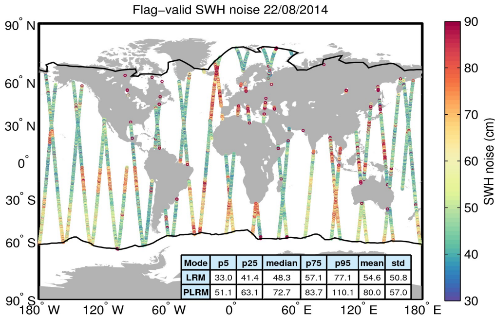
Figure 18. Geographical distribution of flag-valid 20-Hz SWH measurement noise over oceans and lakes for 22/08/2014. The statistical values shown in the table refer to the SWH noise and are calculated separately for LRM and PLRM regions. Measurements taken over polar polygons have been excluded from the computation of the statistical values. The black lines mark the outer limit of the Arctic and Antarctic polar polygons.
