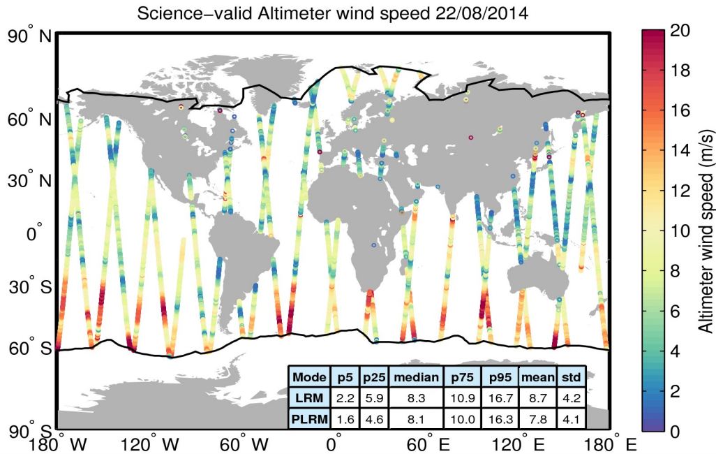
Figure 34. Geographical distribution of science-valid wind data over oceans and lakes for 22/08/2014. The statistical values shown in the table refer to the wind in m/s and are calculated separately for LRM and PLRM regions. The black lines mark the outer limit of the Arctic and Antarctic polar polygons. Gray circles denote records that have been rejected based on the editing criteria described in Table 5.
