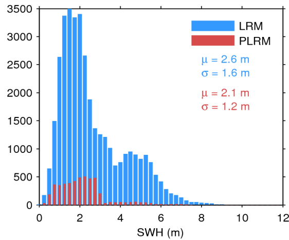
Figure 20. Histogram of science-valid SWH over oceans and lakes for LRM (blue) and PLRM (red) for 22/08/2014. The mean ( \mu ) and standard deviation ( \sigma ) are also shown. Note that values larger than 12 m are excluded from the histogram for the sake of readability but not from the computation of \mu and \sigma .
