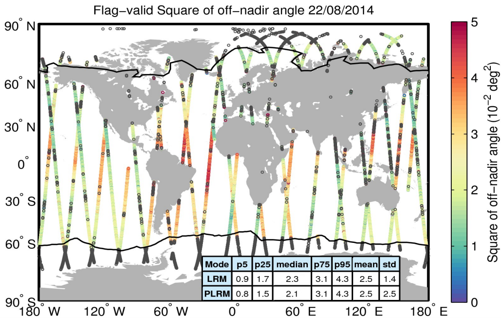
Figure 37. Geographical distribution of flag-valid mispointing data over oceans and lakes for 22/08/2014. The statistical values shown in the table refer to the mispointing in 10^{-2} \text{ deg}^2 and are calculated separately for LRM and PLRM regions. Measurements taken over polar polygons have been excluded from the computation of the statistical values. The black lines mark the outer limit of the Arctic and Antarctic polar polygons. Gray circles denote negative values.
