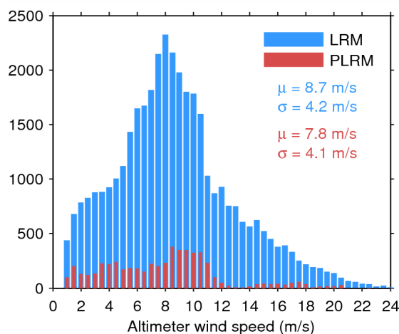
Figure 33. Histogram of flag-valid wind over oceans and lakes for LRM (blue) and PLRM (red) for 22/08/2014. The mean ( \mu ) and standard deviation ( \sigma ) are also shown. Note that values larger than 24 m/s are excluded from the histogram for the sake of readability but not from the computation of \mu and \sigma .
