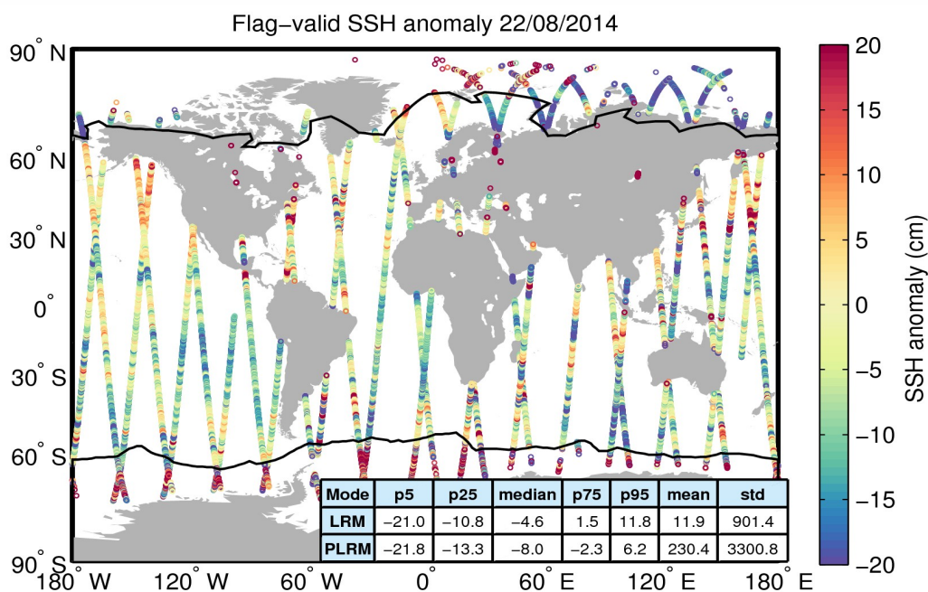
Figure 5. Geographical distribution of flag-valid 1-Hz SSH anomaly data over oceans and lakes for 22/08/2014. The statistical values shown in the table refer to the SSH anomaly in cm and are calculated separately for LRM and PLRM regions. Measurements taken over polar polygons have been excluded from the computation of the statistical values. The black lines mark the outer limit of the Arctic and Antarctic polar polygons.
