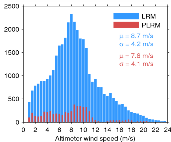
Figure 35. Histogram of science-valid wind over oceans and lakes for LRM (blue) and PLRM (red) for 22/08/2014. The mean ( \mu ) and standard deviation ( \sigma ) are also shown. Note that values larger than 24 m/s are excluded from the histogram for the sake of readability but not from the computation of \mu and \sigma .
