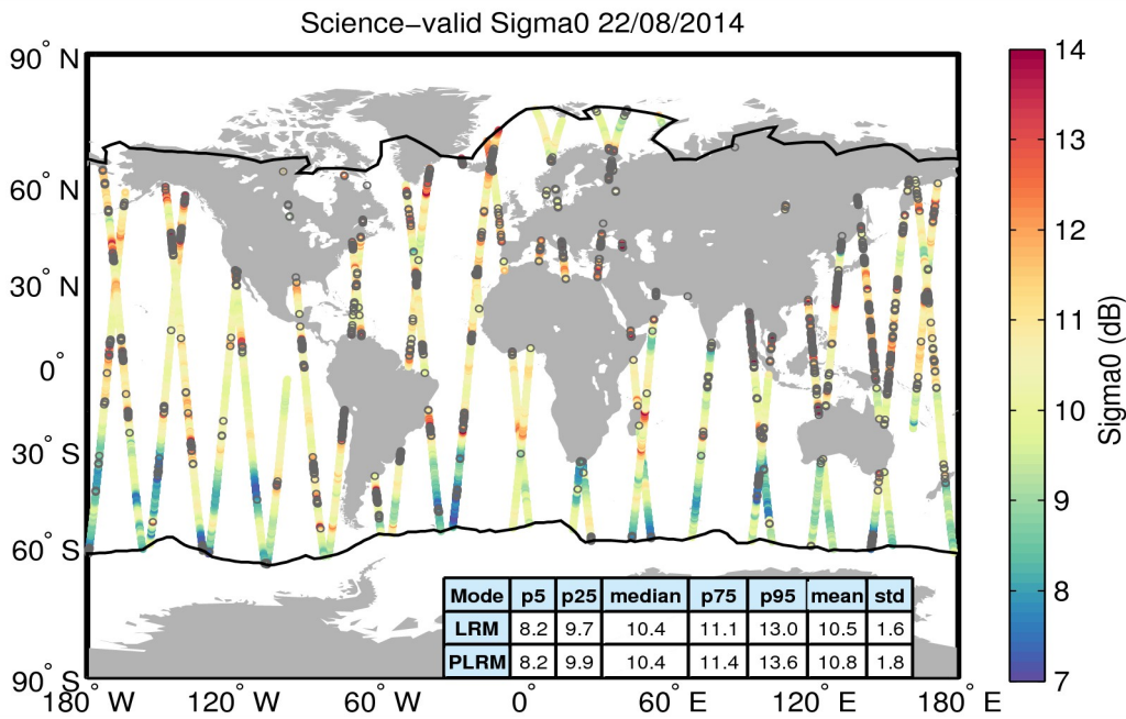
Figure 27. Geographical distribution of science-valid sigma0 data over oceans and lakes for 22/08/2014. The statistical values shown in the table refer to the sigma0 in dB and are calculated separately for LRM and PLRM regions. The black lines mark the outer limit of the Arctic and Antarctic polar polygons. Gray circles denote records that have been rejected based on the editing criteria described in Table 4.
