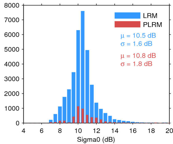
Figure 28. Histogram of science-valid sigma0 over oceans and lakes for LRM (blue) and PLRM (red) for 22/08/2014. The mean ( \mu ) and standard deviation ( \sigma ) are also shown. Note that values outside [4 20] dB are excluded from the histogram for the sake of readability but not from the computation of \mu and \sigma .
