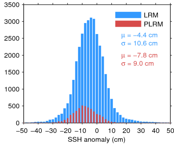
Figure 11. Histogram of science-valid SSH anomaly over oceans and lakes for LRM (blue) and PLRM (red) for 22/08/2014. The mean ( \mu ) and standard deviation ( \sigma ) are also shown. Note that values outside [-50 50] cm are excluded from the histogram for the sake of readability but not from the computation of \mu and \sigma .
