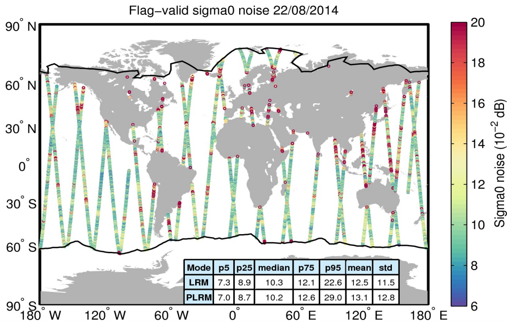
Figure 26. Geographical distribution of flag-valid 20-Hz sigma0 measurement noise over oceans and lakes for 22/08/2014. The statistical values shown in the table refer to the sigma0 noise and are calculated separately for LRM and PLRM regions. Measurements taken over polar polygons have been excluded from the computation of the statistical values. The black lines mark the outer limit of the Arctic and Antarctic polar polygons.
