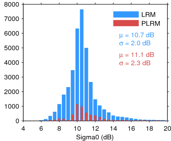
Figure 25. Histogram of flag-valid sigma0 over oceans and lakes for LRM (blue) and PLRM (red) for 22/08/2014. The mean ( \mu ) and standard deviation ( \sigma ) are also shown. Note that values outside [4 20] dB are excluded from the histogram for the sake of readability but not from the computation of \mu and \sigma .
