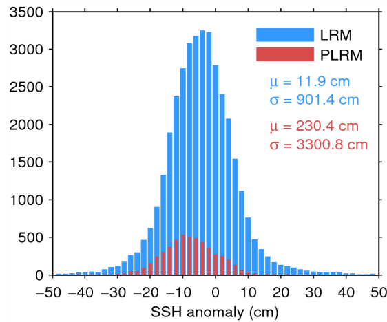
Figure 7. Histogram of flag-valid SSH anomaly over oceans and lakes for LRM (blue) and PLRM (red) for 22/08/2014. The mean ( \mu ) and standard deviation ( \sigma ) are also shown. Note that values outside [-50\ 50] cm are excluded from the histogram for the sake of readability but not from the computation of \mu and \sigma .
