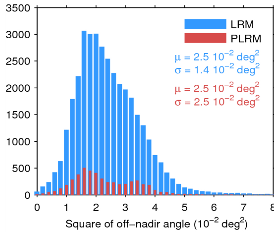
Figure 39. Histogram of flag-valid mispointing over oceans and lakes for LRM (blue) and PLRM (red) for 22/08/2014. Only positive values have been considered. The mean ( \mu ) and standard deviation ( \sigma ) are also shown. Note that values larger than 8 \cdot 10^{-2} \text{ deg}^2 are excluded from the histogram for the sake of readability but not from the computation of \mu and \sigma .
