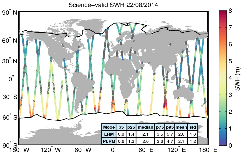
Figure 19. Geographical distribution of science-valid SWH data over oceans and lakes for 22/08/2014. The statistical values shown in the table refer to the SWH in m and are calculated separately for LRM and PLRM regions. The black lines mark the outer limit of the Arctic and Antarctic polar polygons. Gray circles denote records that have been rejected based on the editing criteria described in Table 3.
