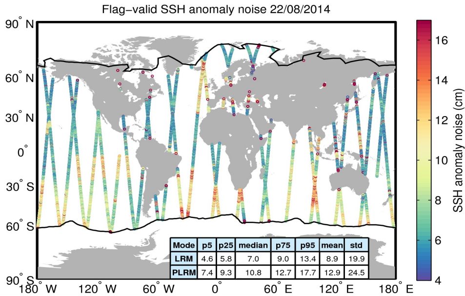
Figure 8. Geographical distribution of flag-valid 20-Hz SSH anomaly measurement noise over oceans and lakes for 22/08/2014. The statistical values shown in the table refer to the SSH anomaly noise and are calculated separately for LRM and PLRM regions. Measurements taken over polar polygons have been excluded from the computation of the statistical values. The black lines mark the outer limit of the Arctic and Antarctic polar polygons.
