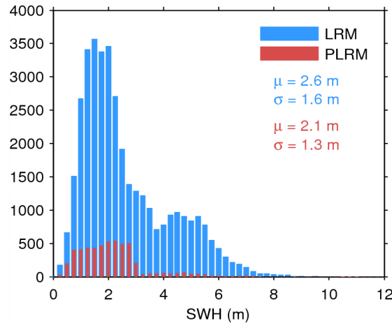
Figure 17. Histogram of flag-valid SWH over oceans and lakes for LRM (blue) and PLRM (red) for 22/08/2014. The mean ( \mu ) and standard deviation ( \sigma ) are also shown. Note that values larger than 12 m are excluded from the histogram for the sake of readability but not from the computation of \mu and \sigma .
