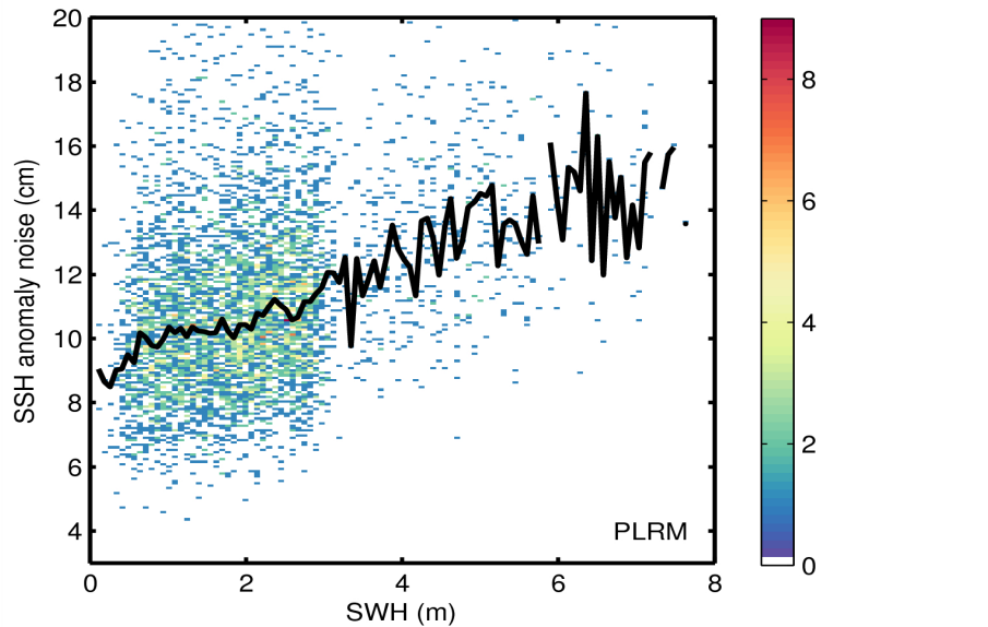
Figure 9. 2D histogram showing flag-valid SSH anomaly noise as a function of SWH for LRM (top) and PLRM (bottom) for 22/08/2014. The black line denotes the median SSH anomaly as a function of SWH.
