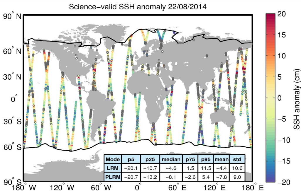
Figure 10. Geographical distribution of science-valid SSH anomaly data over oceans and lakes for 22/08/2014. The statistical values shown in the table refer to the SSH anomaly in cm and are calculated separately for LRM and PLRM regions. The black lines mark the outer limit of the Arctic and Antarctic polar polygons. Gray circles denote records that have been rejected based on the editing criteria described in Table 2.
