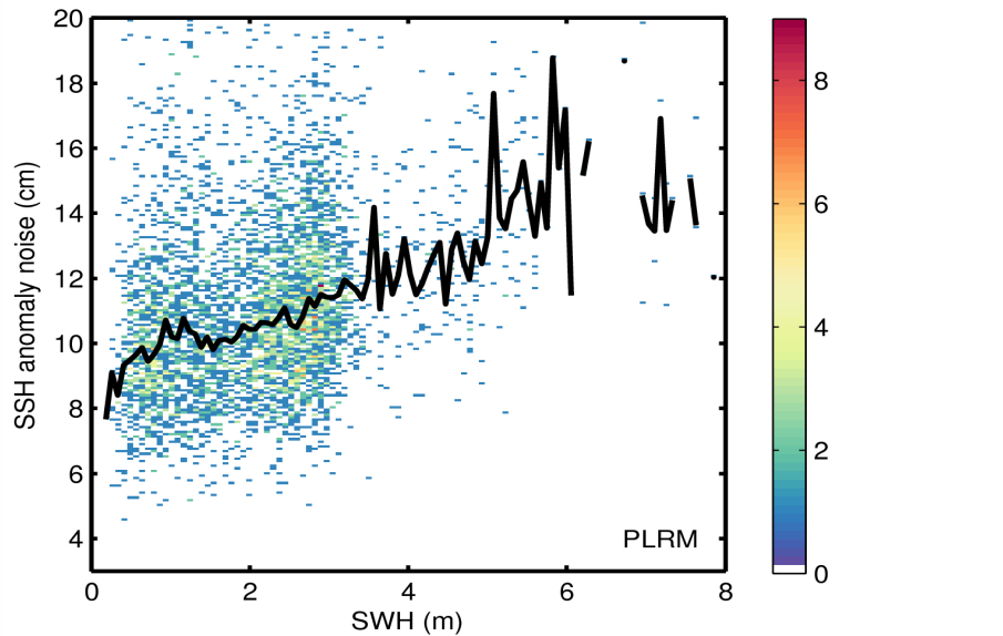
Figure 9. 2D histogram showing flag-valid SSH anomaly noise as a function of SWH for LRM (top) and PLRM (bottom) for 21/08/2014. The black line denotes the median SSH anomaly as a function of SWH.
