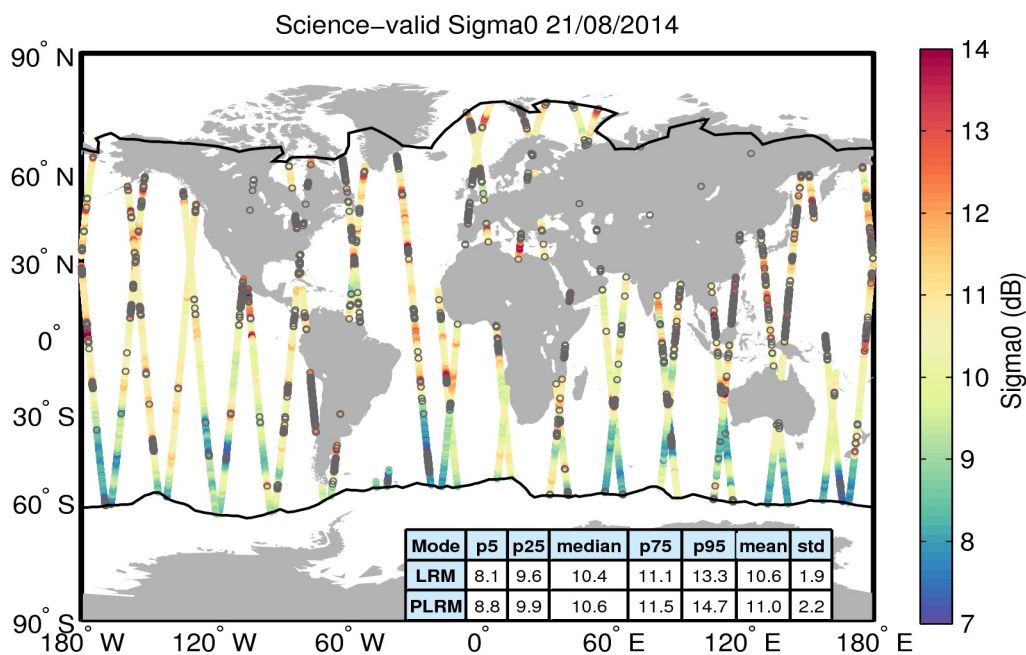
Figure 27. Geographical distribution of science-valid sigma0 data over oceans and lakes for 21/08/2014. The statistical values shown in the table refer to the sigma0 in dB and are calculated separately for LRM and PLRM regions. The black lines mark the outer limit of the Arctic and Antarctic polar polygons. Gray circles denote records that have been rejected based on the editing criteria described in Table 4.
