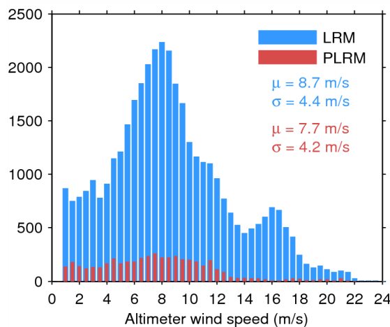
Figure 35. Histogram of science-valid wind over oceans and lakes for LRM (blue) and PLRM (red) for 21/08/2014. The mean ( \mu ) and standard deviation ( \sigma ) are also shown. Note that values larger than 24 m/s are excluded from the histogram for the sake of readability but not from the computation of \mu and \sigma .
