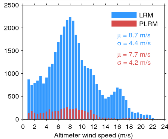
Figure 33. Histogram of flag-valid wind over oceans and lakes for LRM (blue) and PLRM (red) for 21/08/2014. The mean ( \mu ) and standard deviation ( \sigma ) are also shown. Note that values larger than 24 m/s are excluded from the histogram for the sake of readability but not from the computation of \mu and \sigma .
