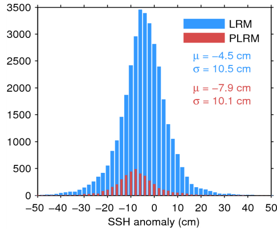
Figure 11. Histogram of science-valid SSH anomaly over oceans and lakes for LRM (blue) and PLRM (red) for 21/08/2014. The mean ( \mu ) and standard deviation ( \sigma ) are also shown. Note that values outside [-50\ 50] cm are excluded from the histogram for the sake of readability but not from the computation of \mu and \sigma .
