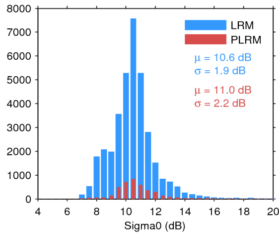
Figure 28. Histogram of science-valid sigma0 over oceans and lakes for LRM (blue) and PLRM (red) for 21/08/2014. The mean ( \mu ) and standard deviation ( \sigma ) are also shown. Note that values outside [4 20] dB are excluded from the histogram for the sake of readability but not from the computation of \mu and \sigma .
