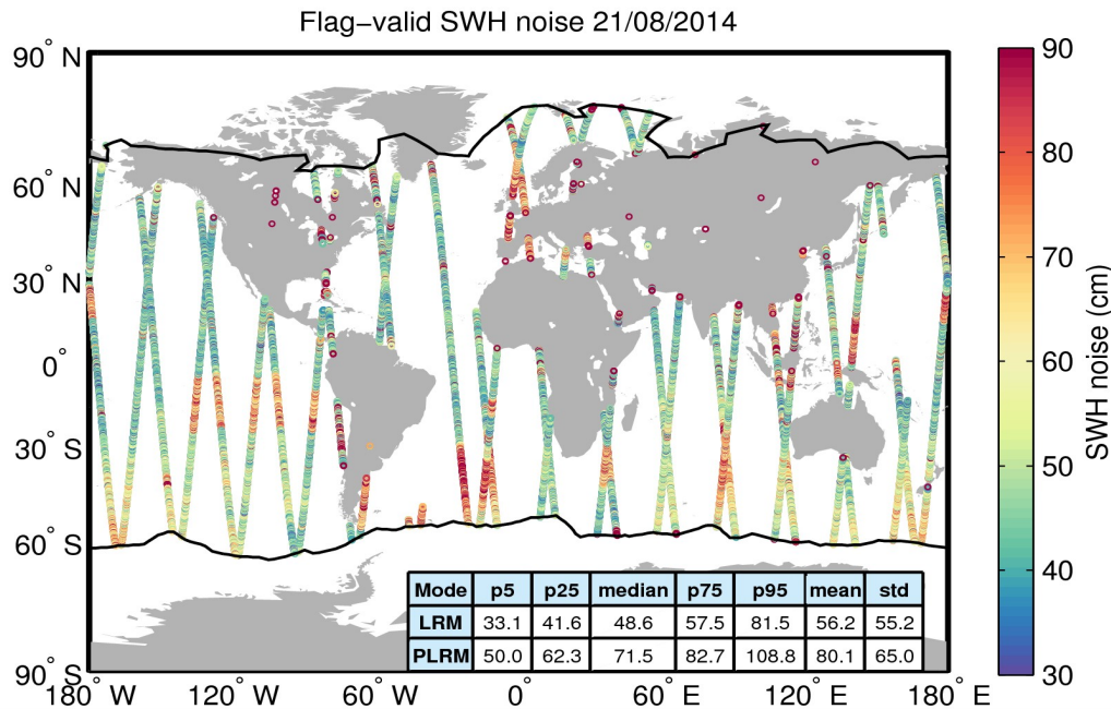
Figure 18. Geographical distribution of flag-valid 20-Hz SWH measurement noise over oceans and lakes for 21/08/2014. The statistical values shown in the table refer to the SWH noise and are calculated separately for LRM and PLRM regions. Measurements taken over polar polygons have been excluded from the computation of the statistical values. The black lines mark the outer limit of the Arctic and Antarctic polar polygons.
