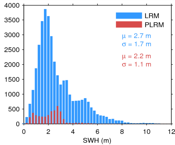
Figure 20. Histogram of science-valid SWH over oceans and lakes for LRM (blue) and PLRM (red) for 21/08/2014. The mean ( \mu ) and standard deviation ( \sigma ) are also shown. Note that values larger than 12 m are excluded from the histogram for the sake of readability but not from the computation of \mu and \sigma .
