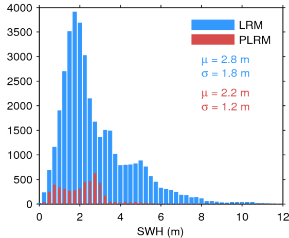
Figure 17. Histogram of flag-valid SWH over oceans and lakes for LRM (blue) and PLRM (red) for 21/08/2014. The mean ( \mu ) and standard deviation ( \sigma ) are also shown. Note that values larger than 12 m are excluded from the histogram for the sake of readability but not from the computation of \mu and \sigma .
