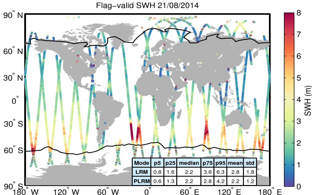
Figure 15. Geographical distribution of flag-valid SWH data over oceans and lakes for 21/08/2014. The statistical values shown in the table refer to the SWH in m and are calculated separately for LRM and PLRM regions. Measurements taken over polar polygons have been excluded from the computation of the statistical values. The black lines mark the outer limit of the Arctic and Antarctic polar polygons.
