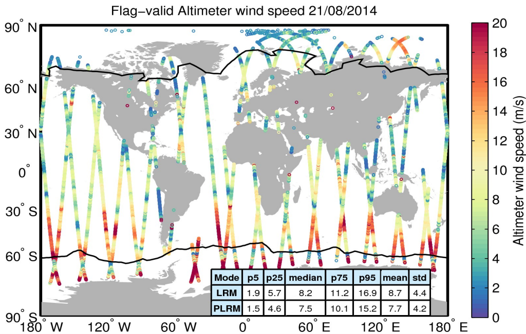
Figure 31. Geographical distribution of flag-valid wind data over oceans and lakes for 21/08/2014. The statistical values shown in the table refer to the wind in m/s and are calculated separately for LRM and PLRM regions. Measurements taken over polar polygons have been excluded from the computation of the statistical values. The black lines mark the outer limit of the Arctic and Antarctic polar polygons.
