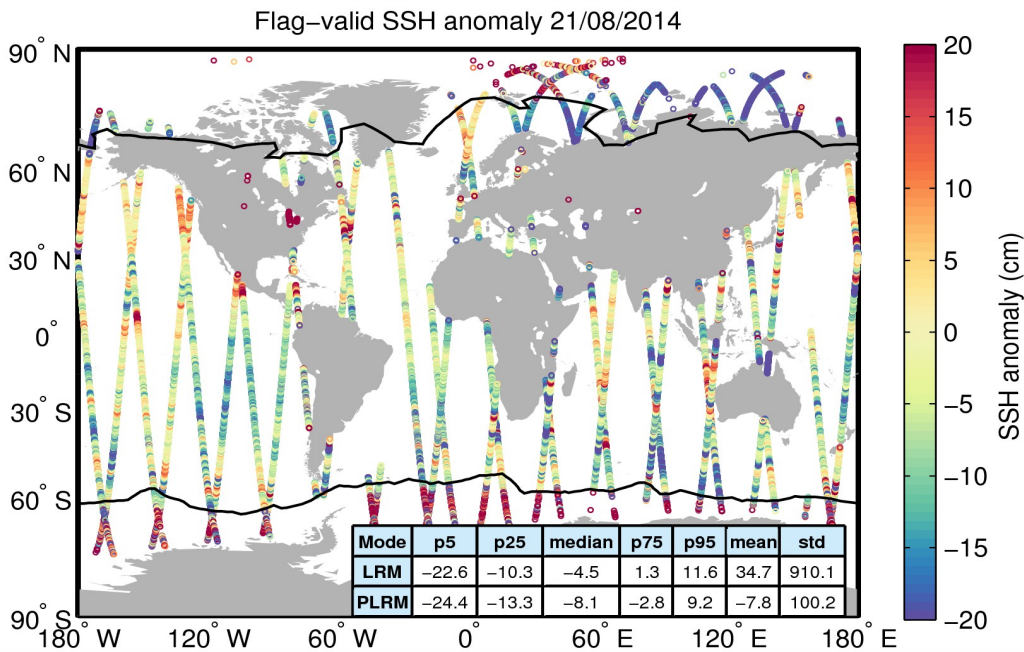
Figure 5. Geographical distribution of flag-valid 1-Hz SSH anomaly data over oceans and lakes for 21/08/2014. The statistical values shown in the table refer to the SSH anomaly in cm and are calculated separately for LRM and PLRM regions. Measurements taken over polar polygons have been excluded from the computation of the statistical values. The black lines mark the outer limit of the Arctic and Antarctic polar polygons.
