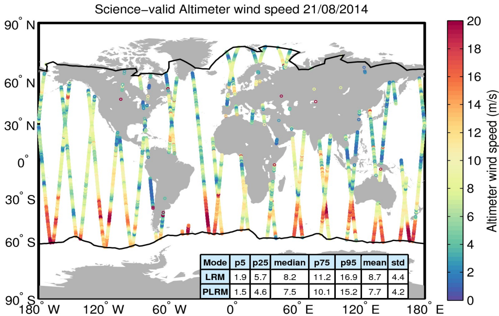
Figure 34. Geographical distribution of science-valid wind data over oceans and lakes for 21/08/2014. The statistical values shown in the table refer to the wind in m/s and are calculated separately for LRM and PLRM regions. The black lines mark the outer limit of the Arctic and Antarctic polar polygons. Gray circles denote records that have been rejected based on the editing criteria described in Table 5.
