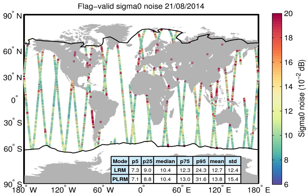
Figure 26. Geographical distribution of flag-valid 20-Hz sigma0 measurement noise over oceans and lakes for 21/08/2014. The statistical values shown in the table refer to the sigma0 noise and are calculated separately for LRM and PLRM regions. Measurements taken over polar polygons have been excluded from the computation of the statistical values. The black lines mark the outer limit of the Arctic and Antarctic polar polygons.
