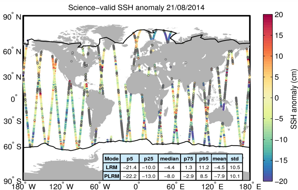
Figure 10. Geographical distribution of science-valid SSH anomaly data over oceans and lakes for 21/08/2014. The statistical values shown in the table refer to the SSH anomaly in cm and are calculated separately for LRM and PLRM regions. The black lines mark the outer limit of the Arctic and Antarctic polar polygons. Gray circles denote records that have been rejected based on the editing criteria described in Table 2.
