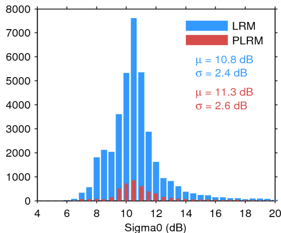
Figure 25. Histogram of flag-valid sigma0 over oceans and lakes for LRM (blue) and PLRM (red) for 21/08/2014. The mean ( \mu ) and standard deviation ( \sigma ) are also shown. Note that values outside [4 20] dB are excluded from the histogram for the sake of readability but not from the computation of \mu and \sigma .
