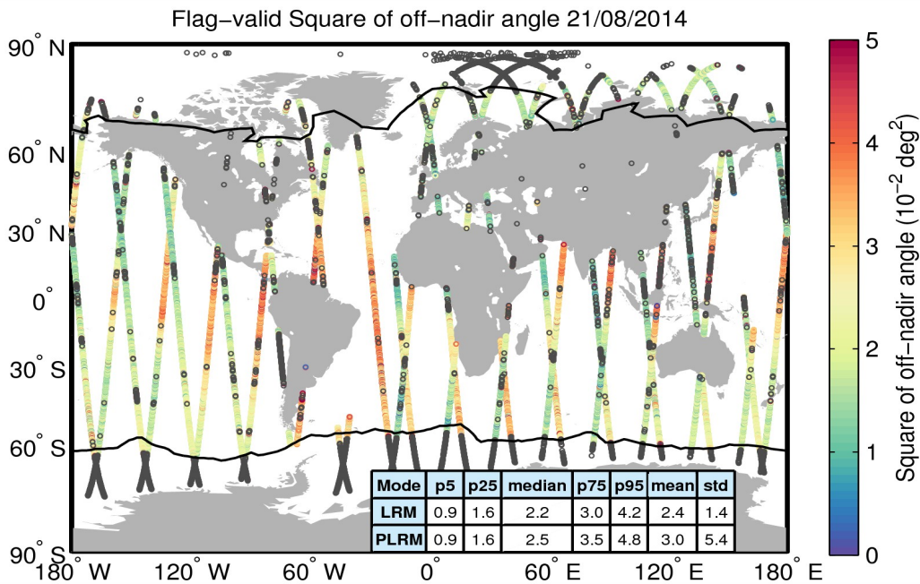
Figure 37. Geographical distribution of flag-valid mispointing data over oceans and lakes for 21/08/2014. The statistical values shown in the table refer to the mispointing in 10^{-2} \text{ deg}^2 and are calculated separately for LRM and PLRM regions. Measurements taken over polar polygons have been excluded from the computation of the statistical values. The black lines mark the outer limit of the Arctic and Antarctic polar polygons. Gray circles denote negative values.
