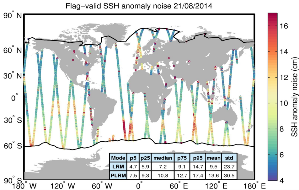
Figure 8. Geographical distribution of flag-valid 20-Hz SSH anomaly measurement noise over oceans and lakes for 21/08/2014. The statistical values shown in the table refer to the SSH anomaly noise and are calculated separately for LRM and PLRM regions. Measurements taken over polar polygons have been excluded from the computation of the statistical values. The black lines mark the outer limit of the Arctic and Antarctic polar polygons.
