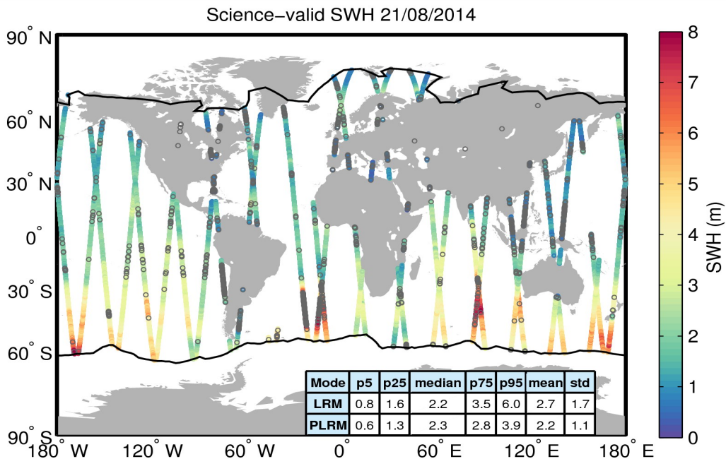
Figure 19. Geographical distribution of science-valid SWH data over oceans and lakes for 21/08/2014. The statistical values shown in the table refer to the SWH in m and are calculated separately for LRM and PLRM regions. The black lines mark the outer limit of the Arctic and Antarctic polar polygons. Gray circles denote records that have been rejected based on the editing criteria described in Table 3.
