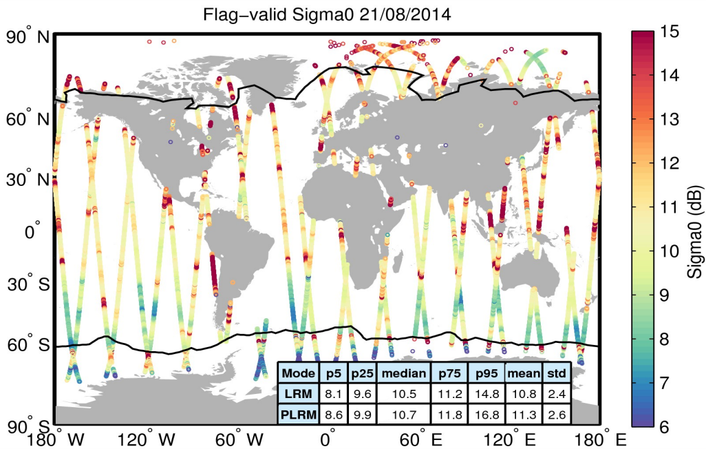
Figure 23. Geographical distribution of flag-valid sigma0 data over oceans and lakes for 21/08/2014. The statistical values shown in the table refer to the sigma0 in dB and are calculated separately for LRM and PLRM regions. Measurements taken over polar polygons have been excluded from the computation of the statistical values. The black lines mark the outer limit of the Arctic and Antarctic polar polygons.
