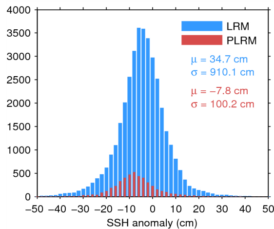
Figure 7. Histogram of flag-valid SSH anomaly over oceans and lakes for LRM (blue) and PLRM (red) for 21/08/2014. The mean ( \mu ) and standard deviation ( \sigma ) are also shown. Note that values outside [-50 50] cm are excluded from the histogram for the sake of readability but not from the computation of \mu and \sigma .
