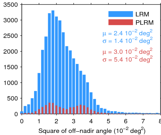
Figure 39. Histogram of flag-valid mispointing over oceans and lakes for LRM (blue) and PLRM (red) for 21/08/2014. Only positive values have been considered. The mean ( \mu ) and standard deviation ( \sigma ) are also shown. Note that values larger than 8 \cdot 10^{-2} \text{ deg}^2 are excluded from the histogram for the sake of readability but not from the computation of \mu and \sigma .
