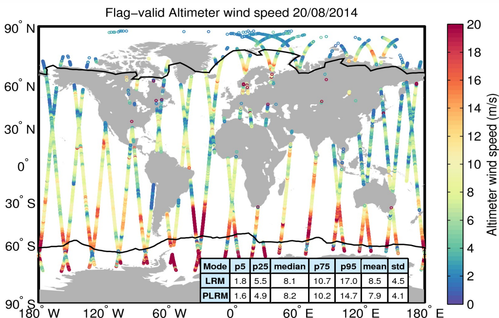
Figure 31. Geographical distribution of flag-valid wind data over oceans and lakes for 20/08/2014. The statistical values shown in the table refer to the wind in m/s and are calculated separately for LRM and PLRM regions. Measurements taken over polar polygons have been excluded from the computation of the statistical values. The black lines mark the outer limit of the Arctic and Antarctic polar polygons.
