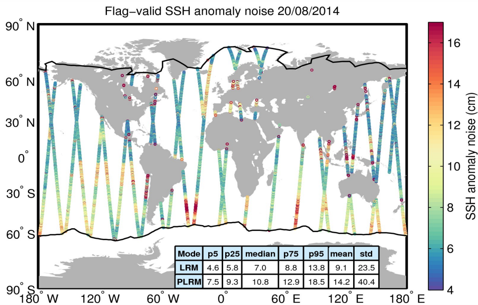
Figure 8. Geographical distribution of flag-valid 20-Hz SSH anomaly measurement noise over oceans and lakes for 20/08/2014. The statistical values shown in the table refer to the SSH anomaly noise and are calculated separately for LRM and PLRM regions. Measurements taken over polar polygons have been excluded from the computation of the statistical values. The black lines mark the outer limit of the Arctic and Antarctic polar polygons.
