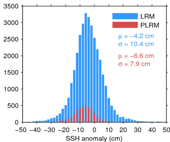
Figure 11. Histogram of science-valid SSH anomaly over oceans and lakes for LRM (blue) and PLRM (red) for 20/08/2014. The mean ( \mu ) and standard deviation ( \sigma ) are also shown. Note that values outside [-50 50] cm are excluded from the histogram for the sake of readability but not from the computation of \mu and \sigma .
