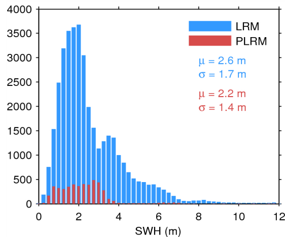
Figure 17. Histogram of flag-valid SWH over oceans and lakes for LRM (blue) and PLRM (red) for 20/08/2014. The mean ( \mu ) and standard deviation ( \sigma ) are also shown. Note that values larger than 12 m are excluded from the histogram for the sake of readability but not from the computation of \mu and \sigma .
