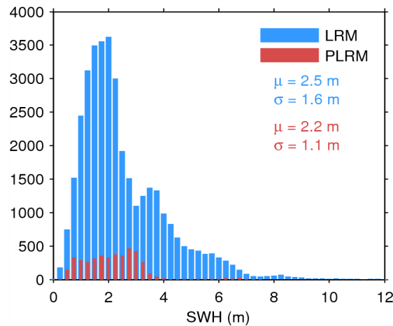
Figure 20. Histogram of science-valid SWH over oceans and lakes for LRM (blue) and PLRM (red) for 20/08/2014. The mean ( \mu ) and standard deviation ( \sigma ) are also shown. Note that values larger than 12 m are excluded from the histogram for the sake of readability but not from the computation of \mu and \sigma .
