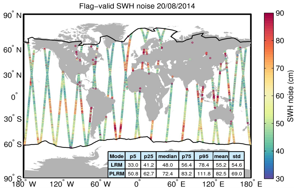
Figure 18. Geographical distribution of flag-valid 20-Hz SWH measurement noise over oceans and lakes for 20/08/2014. The statistical values shown in the table refer to the SWH noise and are calculated separately for LRM and PLRM regions. Measurements taken over polar polygons have been excluded from the computation of the statistical values. The black lines mark the outer limit of the Arctic and Antarctic polar polygons.
