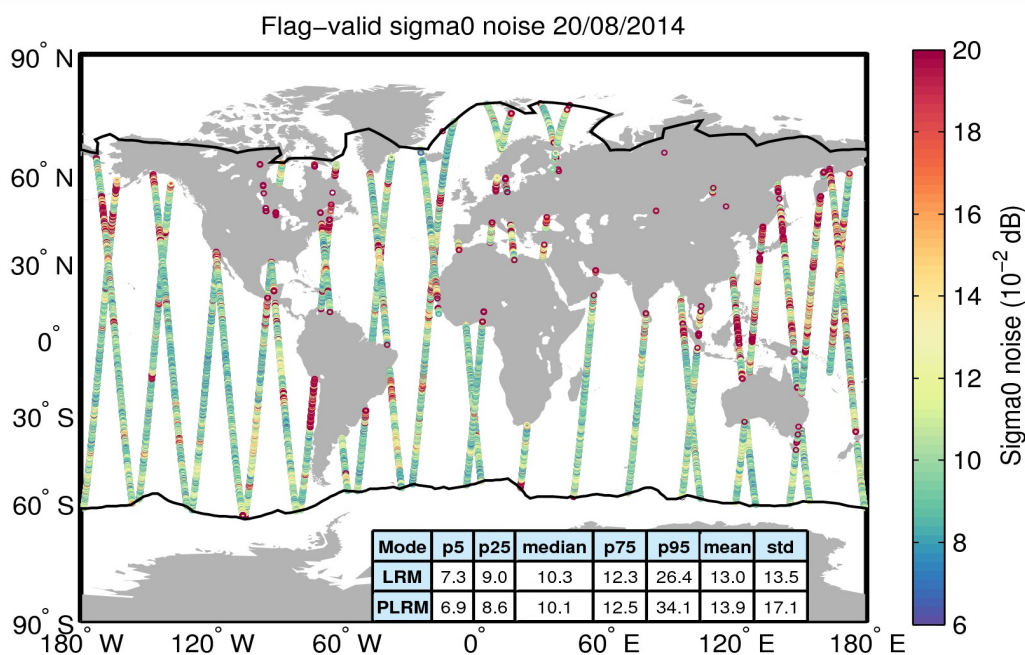
Figure 26. Geographical distribution of flag-valid 20-Hz sigma0 measurement noise over oceans and lakes for 20/08/2014. The statistical values shown in the table refer to the sigma0 noise and are calculated separately for LRM and PLRM regions. Measurements taken over polar polygons have been excluded from the computation of the statistical values. The black lines mark the outer limit of the Arctic and Antarctic polar polygons.
