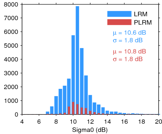
Figure 28. Histogram of science-valid sigma0 over oceans and lakes for LRM (blue) and PLRM (red) for 20/08/2014. The mean ( \mu ) and standard deviation ( \sigma ) are also shown. Note that values outside [4 20] dB are excluded from the histogram for the sake of readability but not from the computation of \mu and \sigma .
