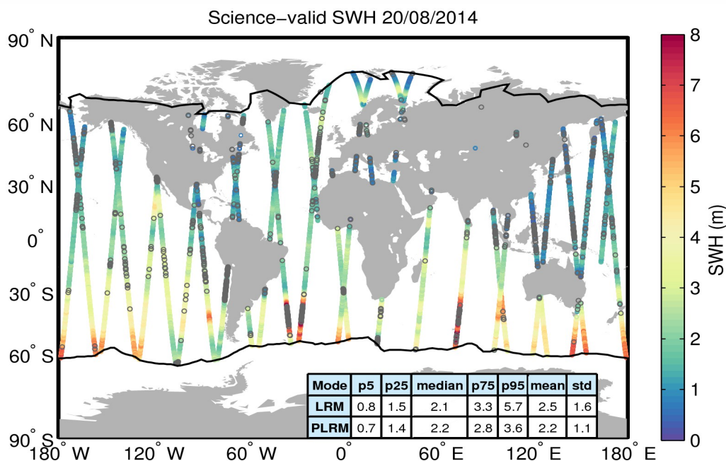
Figure 19. Geographical distribution of science-valid SWH data over oceans and lakes for 20/08/2014. The statistical values shown in the table refer to the SWH in m and are calculated separately for LRM and PLRM regions. The black lines mark the outer limit of the Arctic and Antarctic polar polygons. Gray circles denote records that have been rejected based on the editing criteria described in Table 3.
