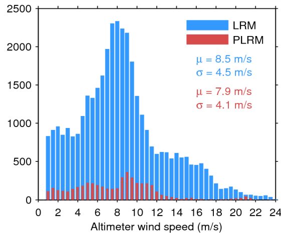
Figure 33. Histogram of flag-valid wind over oceans and lakes for LRM (blue) and PLRM (red) for 20/08/2014. The mean ( \mu ) and standard deviation ( \sigma ) are also shown. Note that values larger than 24 m/s are excluded from the histogram for the sake of readability but not from the computation of \mu and \sigma .
