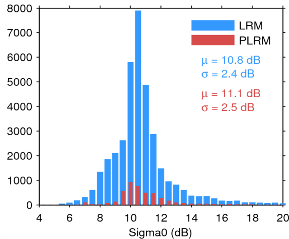
Figure 25. Histogram of flag-valid sigma0 over oceans and lakes for LRM (blue) and PLRM (red) for 20/08/2014. The mean ( \mu ) and standard deviation ( \sigma ) are also shown. Note that values outside [4 20] dB are excluded from the histogram for the sake of readability but not from the computation of \mu and \sigma .
