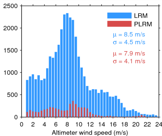
Figure 35. Histogram of science-valid wind over oceans and lakes for LRM (blue) and PLRM (red) for 20/08/2014. The mean ( \mu ) and standard deviation ( \sigma ) are also shown. Note that values larger than 24 m/s are excluded from the histogram for the sake of readability but not from the computation of \mu and \sigma .
