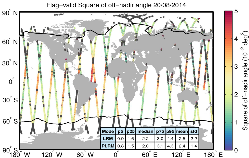
Figure 37. Geographical distribution of flag-valid mispointing data over oceans and lakes for 20/08/2014. The statistical values shown in the table refer to the mispointing in 10^{-2} \text{ deg}^2 and are calculated separately for LRM and PLRM regions. Measurements taken over polar polygons have been excluded from the computation of the statistical values. The black lines mark the outer limit of the Arctic and Antarctic polar polygons. Gray circles denote negative values.
