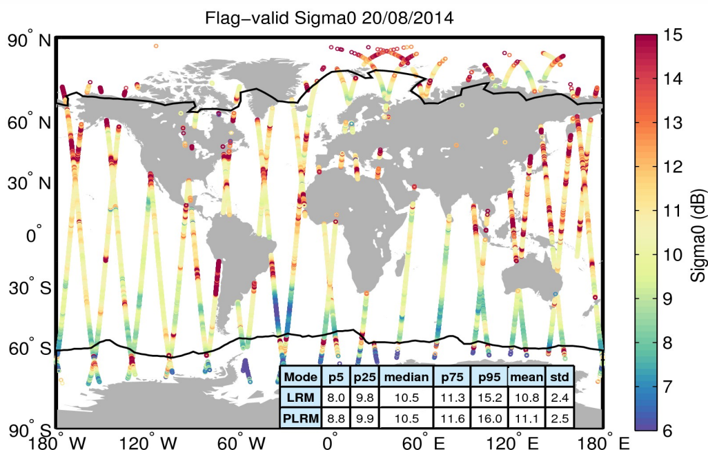
Figure 23. Geographical distribution of flag-valid sigma0 data over oceans and lakes for 20/08/2014. The statistical values shown in the table refer to the sigma0 in dB and are calculated separately for LRM and PLRM regions. Measurements taken over polar polygons have been excluded from the computation of the statistical values. The black lines mark the outer limit of the Arctic and Antarctic polar polygons.
