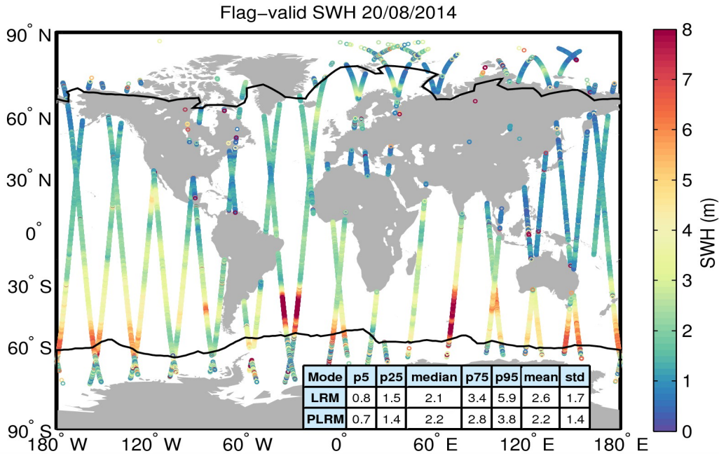
Figure 15. Geographical distribution of flag-valid SWH data over oceans and lakes for 20/08/2014. The statistical values shown in the table refer to the SWH in m and are calculated separately for LRM and PLRM regions. Measurements taken over polar polygons have been excluded from the computation of the statistical values. The black lines mark the outer limit of the Arctic and Antarctic polar polygons.
