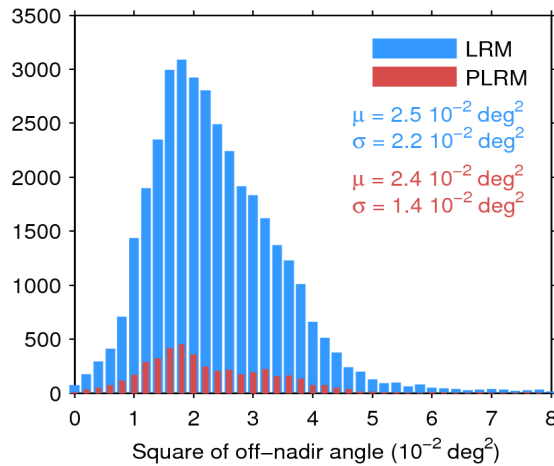
Figure 39. Histogram of flag-valid mispointing over oceans and lakes for LRM (blue) and PLRM (red) for 20/08/2014. Only positive values have been considered. The mean ( \mu ) and standard deviation ( \sigma ) are also shown. Note that values larger than 8 \cdot 10^{-2} \text{ deg}^2 are excluded from the histogram for the sake of readability but not from the computation of \mu and \sigma .
