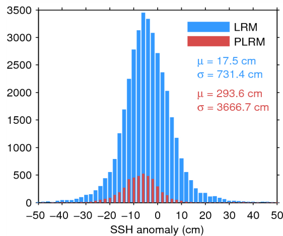
Figure 7. Histogram of flag-valid SSH anomaly over oceans and lakes for LRM (blue) and PLRM (red) for 20/08/2014. The mean ( \mu ) and standard deviation ( \sigma ) are also shown. Note that values outside [-50\ 50] cm are excluded from the histogram for the sake of readability but not from the computation of \mu and \sigma .
