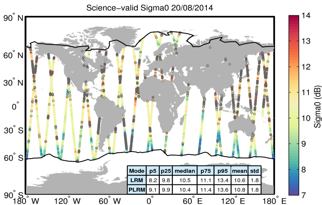
Figure 27. Geographical distribution of science-valid sigma0 data over oceans and lakes for 20/08/2014. The statistical values shown in the table refer to the sigma0 in dB and are calculated separately for LRM and PLRM regions. The black lines mark the outer limit of the Arctic and Antarctic polar polygons. Gray circles denote records that have been rejected based on the editing criteria described in Table 4.
