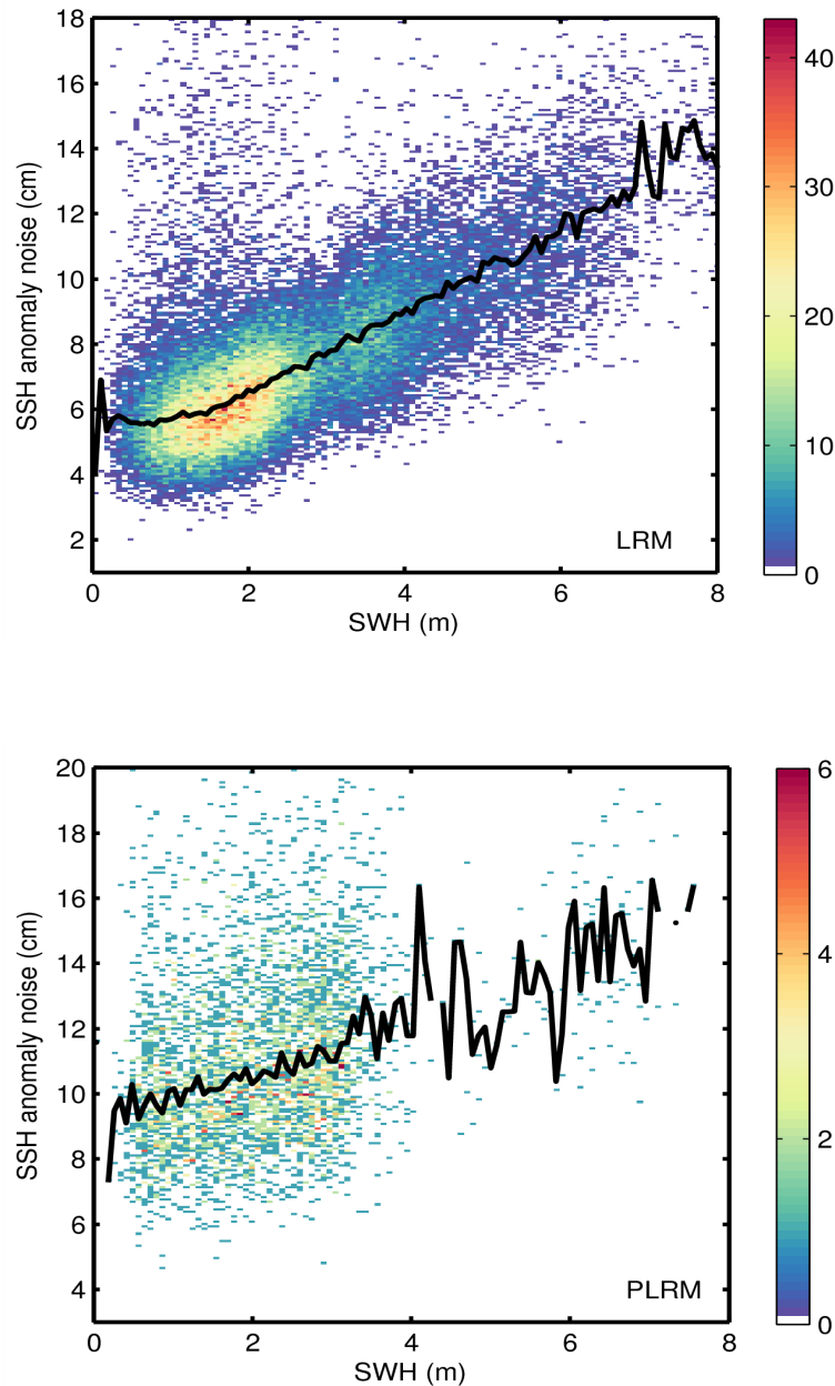
Figure 9. 2D histogram showing flag-valid SSH anomaly noise as a function of SWH for LRM (top) and PLRM (bottom) for 20/08/2014. The black line denotes the median SSH anomaly as a function of SWH.
