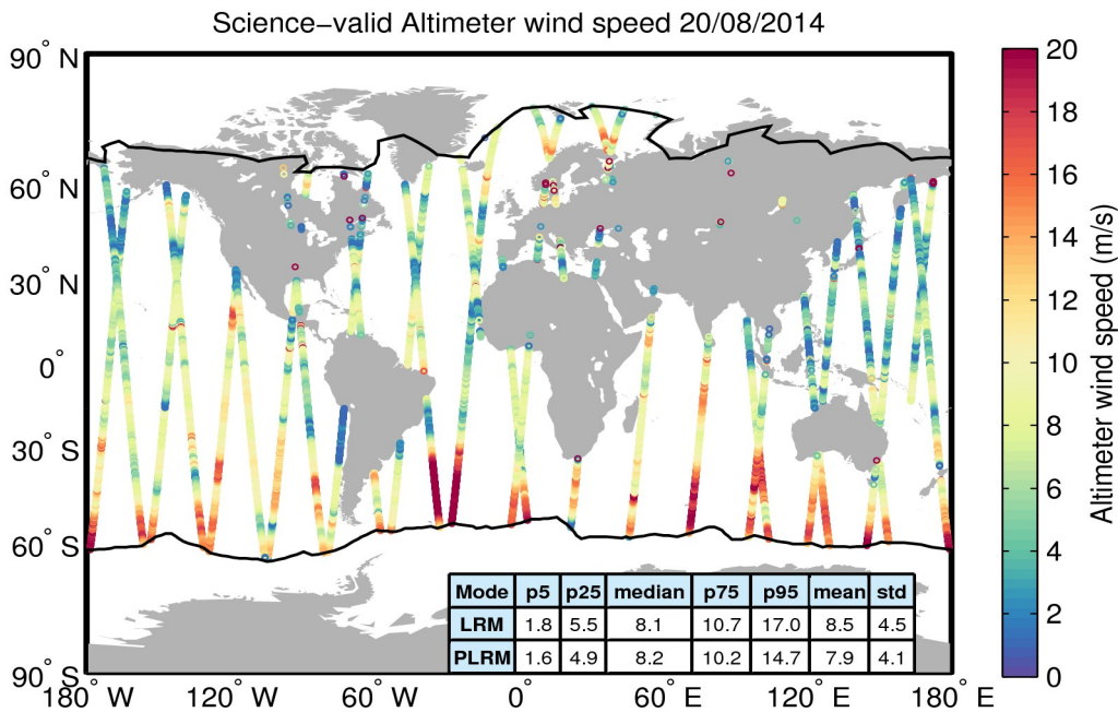
Figure 34. Geographical distribution of science-valid wind data over oceans and lakes for 20/08/2014. The statistical values shown in the table refer to the wind in m/s and are calculated separately for LRM and PLRM regions. The black lines mark the outer limit of the Arctic and Antarctic polar polygons. Gray circles denote records that have been rejected based on the editing criteria described in Table 5.
