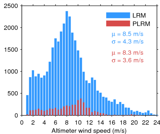
Figure 35. Histogram of science-valid wind over oceans and lakes for LRM (blue) and PLRM (red) for 19/08/2014. The mean ( \mu ) and standard deviation ( \sigma ) are also shown. Note that values larger than 24 m/s are excluded from the histogram for the sake of readability but not from the computation of \mu and \sigma .
