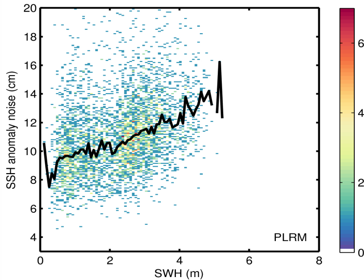
Figure 9. 2D histogram showing flag-valid SSH anomaly noise as a function of SWH for LRM (top) and PLRM (bottom) for 19/08/2014. The black line denotes the median SSH anomaly as a function of SWH.
