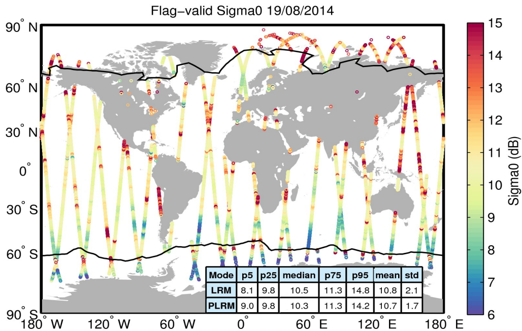
Figure 23. Geographical distribution of flag-valid sigma0 data over oceans and lakes for 19/08/2014. The statistical values shown in the table refer to the sigma0 in dB and are calculated separately for LRM and PLRM regions. Measurements taken over polar polygons have been excluded from the computation of the statistical values. The black lines mark the outer limit of the Arctic and Antarctic polar polygons.
