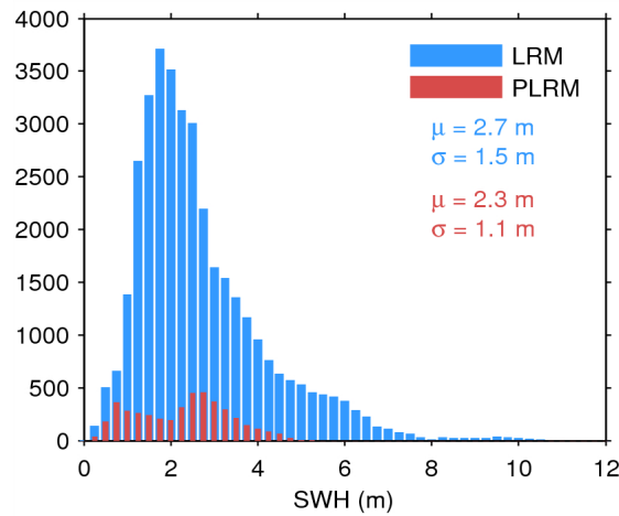
Figure 20. Histogram of science-valid SWH over oceans and lakes for LRM (blue) and PLRM (red) for 19/08/2014. The mean ( \mu ) and standard deviation ( \sigma ) are also shown. Note that values larger than 12 m are excluded from the histogram for the sake of readability but not from the computation of \mu and \sigma .
