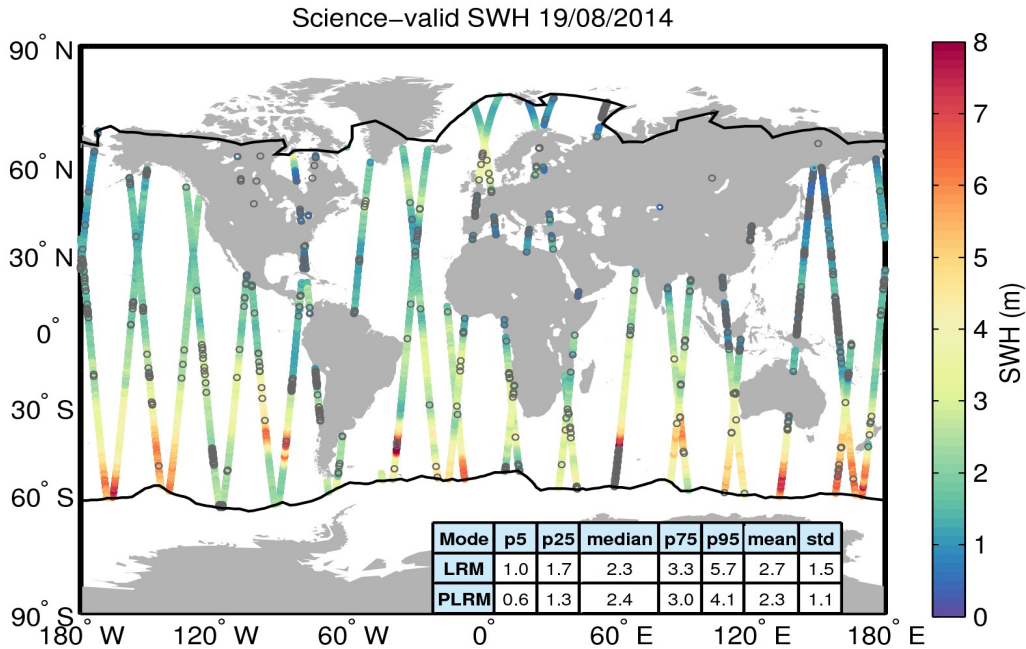
Figure 19. Geographical distribution of science-valid SWH data over oceans and lakes for 19/08/2014. The statistical values shown in the table refer to the SWH in m and are calculated separately for LRM and PLRM regions. The black lines mark the outer limit of the Arctic and Antarctic polar polygons. Gray circles denote records that have been rejected based on the editing criteria described in Table 3.
