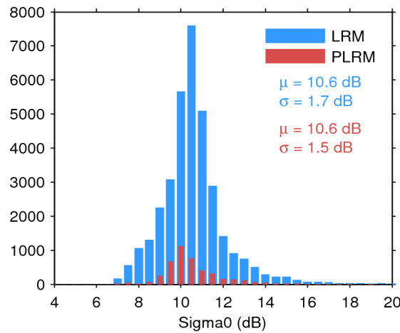
Figure 28. Histogram of science-valid sigma0 over oceans and lakes for LRM (blue) and PLRM (red) for 19/08/2014. The mean ( \mu ) and standard deviation ( \sigma ) are also shown. Note that values outside [4 20] dB are excluded from the histogram for the sake of readability but not from the computation of \mu and \sigma .
