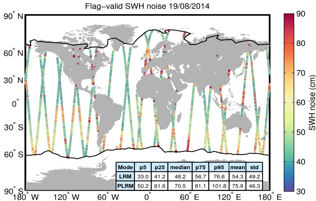
Figure 18. Geographical distribution of flag-valid 20-Hz SWH measurement noise over oceans and lakes for 19/08/2014. The statistical values shown in the table refer to the SWH noise and are calculated separately for LRM and PLRM regions. Measurements taken over polar polygons have been excluded from the computation of the statistical values. The black lines mark the outer limit of the Arctic and Antarctic polar polygons.
