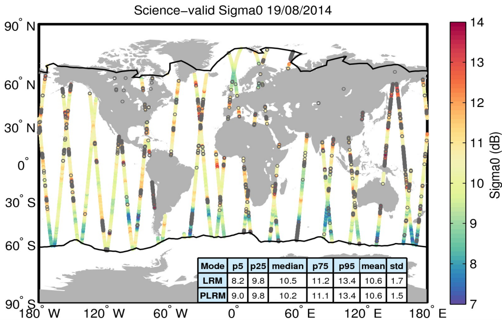
Figure 27. Geographical distribution of science-valid sigma0 data over oceans and lakes for 19/08/2014. The statistical values shown in the table refer to the sigma0 in dB and are calculated separately for LRM and PLRM regions. The black lines mark the outer limit of the Arctic and Antarctic polar polygons. Gray circles denote records that have been rejected based on the editing criteria described in Table 4.
