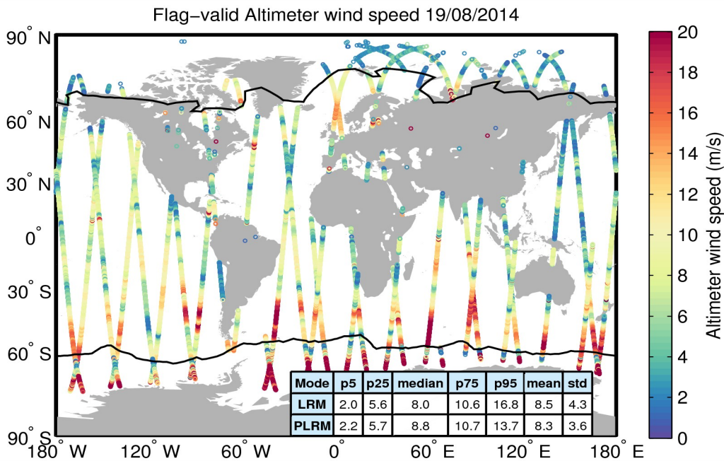
Figure 31. Geographical distribution of flag-valid wind data over oceans and lakes for 19/08/2014. The statistical values shown in the table refer to the wind in m/s and are calculated separately for LRM and PLRM regions. Measurements taken over polar polygons have been excluded from the computation of the statistical values. The black lines mark the outer limit of the Arctic and Antarctic polar polygons.
