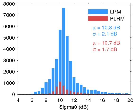
Figure 25. Histogram of flag-valid sigma0 over oceans and lakes for LRM (blue) and PLRM (red) for 19/08/2014. The mean ( \mu ) and standard deviation ( \sigma ) are also shown. Note that values outside [4 20] dB are excluded from the histogram for the sake of readability but not from the computation of \mu and \sigma .
