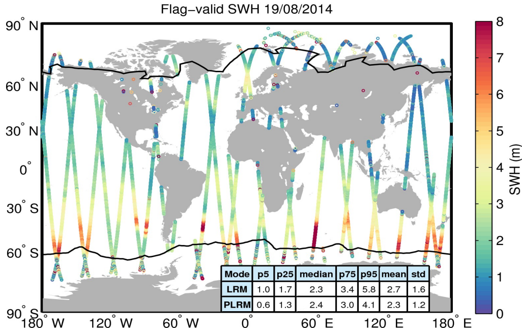
Figure 15. Geographical distribution of flag-valid SWH data over oceans and lakes for 19/08/2014. The statistical values shown in the table refer to the SWH in m and are calculated separately for LRM and PLRM regions. Measurements taken over polar polygons have been excluded from the computation of the statistical values. The black lines mark the outer limit of the Arctic and Antarctic polar polygons.
