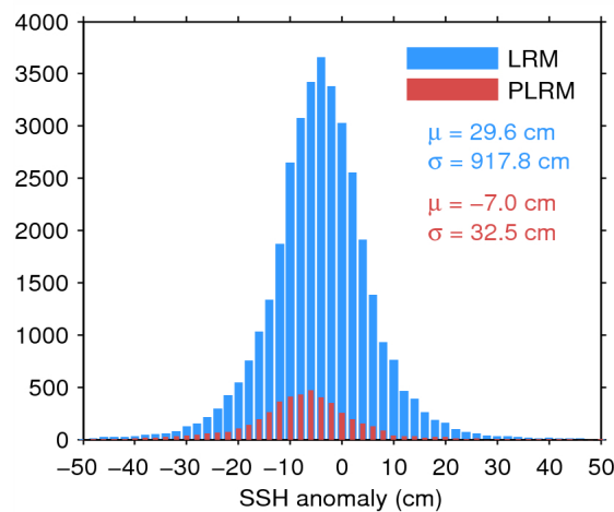
Figure 7. Histogram of flag-valid SSH anomaly over oceans and lakes for LRM (blue) and PLRM (red) for 19/08/2014. The mean ( \mu ) and standard deviation ( \sigma ) are also shown. Note that values outside [-50 50] cm are excluded from the histogram for the sake of readability but not from the computation of \mu and \sigma .
