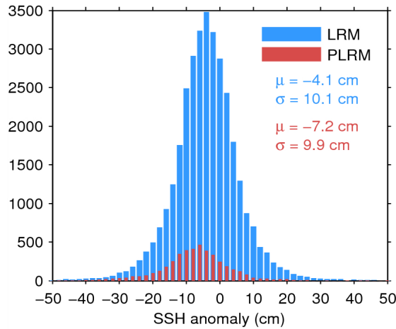
Figure 11. Histogram of science-valid SSH anomaly over oceans and lakes for LRM (blue) and PLRM (red) for 19/08/2014. The mean ( \mu ) and standard deviation ( \sigma ) are also shown. Note that values outside [-50 50] cm are excluded from the histogram for the sake of readability but not from the computation of \mu and \sigma .
