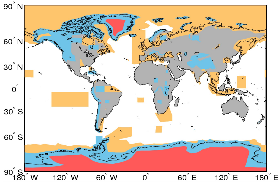
Figure A1. Extent of the regions defining the geographical mode mask for 19/08/2014. The regions where SAR, and SARin are operated are denoted by the orange and blue polygons, respectively. LRM is operated over areas of the continental ice sheets (red polygons) and over oceans and land not covered by other modes.
