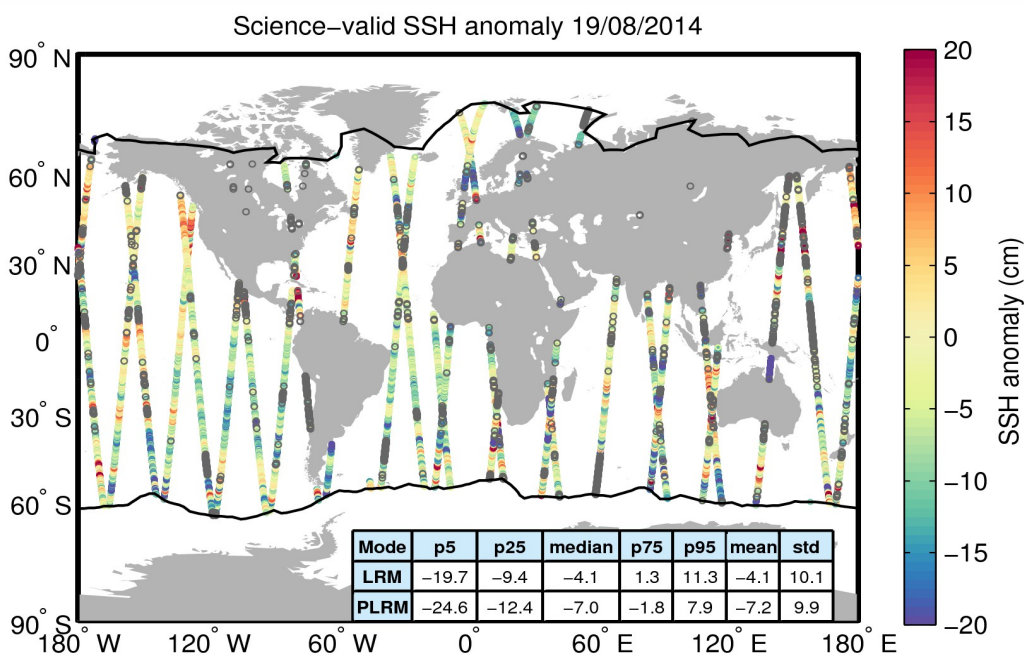
Figure 10. Geographical distribution of science-valid SSH anomaly data over oceans and lakes for 19/08/2014. The statistical values shown in the table refer to the SSH anomaly in cm and are calculated separately for LRM and PLRM regions. The black lines mark the outer limit of the Arctic and Antarctic polar polygons. Gray circles denote records that have been rejected based on the editing criteria described in Table 2.
