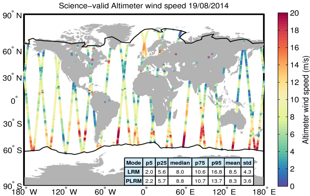
Figure 34. Geographical distribution of science-valid wind data over oceans and lakes for 19/08/2014. The statistical values shown in the table refer to the wind in m/s and are calculated separately for LRM and PLRM regions. The black lines mark the outer limit of the Arctic and Antarctic polar polygons. Gray circles denote records that have been rejected based on the editing criteria described in Table 5.
