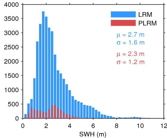
Figure 17. Histogram of flag-valid SWH over oceans and lakes for LRM (blue) and PLRM (red) for 19/08/2014. The mean ( \mu ) and standard deviation ( \sigma ) are also shown. Note that values larger than 12 m are excluded from the histogram for the sake of readability but not from the computation of \mu and \sigma .
