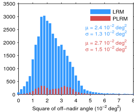
Figure 39. Histogram of flag-valid mispointing over oceans and lakes for LRM (blue) and PLRM (red) for 19/08/2014. Only positive values have been considered. The mean ( \mu ) and standard deviation ( \sigma ) are also shown. Note that values larger than 8 \cdot 10^{-2} \text{ deg}^2 are excluded from the histogram for the sake of readability but not from the computation of \mu and \sigma .
