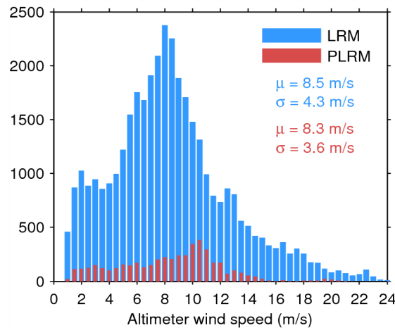
Figure 33. Histogram of flag-valid wind over oceans and lakes for LRM (blue) and PLRM (red) for 19/08/2014. The mean ( \mu ) and standard deviation ( \sigma ) are also shown. Note that values larger than 24 m/s are excluded from the histogram for the sake of readability but not from the computation of \mu and \sigma .
