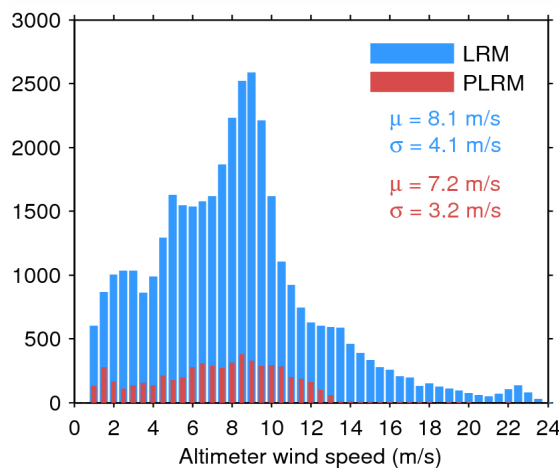
Figure 35. Histogram of science-valid wind over oceans and lakes for LRM (blue) and PLRM (red) for 18/08/2014. The mean ( \mu ) and standard deviation ( \sigma ) are also shown. Note that values larger than 24 m/s are excluded from the histogram for the sake of readability but not from the computation of \mu and \sigma .
