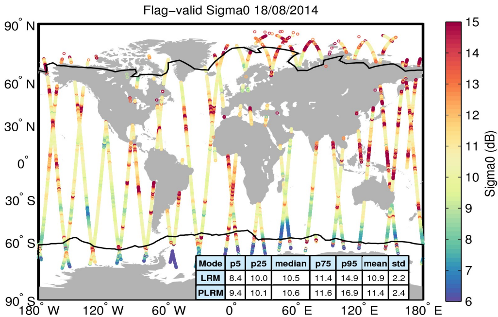
Figure 23. Geographical distribution of flag-valid sigma0 data over oceans and lakes for 18/08/2014. The statistical values shown in the table refer to the sigma0 in dB and are calculated separately for LRM and PLRM regions. Measurements taken over polar polygons have been excluded from the computation of the statistical values. The black lines mark the outer limit of the Arctic and Antarctic polar polygons.
