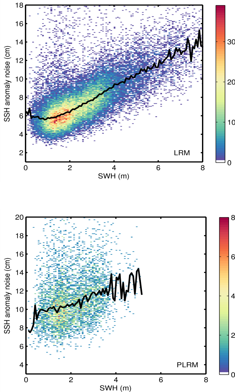
Figure 9. 2D histogram showing flag-valid SSH anomaly noise as a function of SWH for LRM (top) and PLRM (bottom) for 18/08/2014. The black line denotes the median SSH anomaly as a function of SWH.
