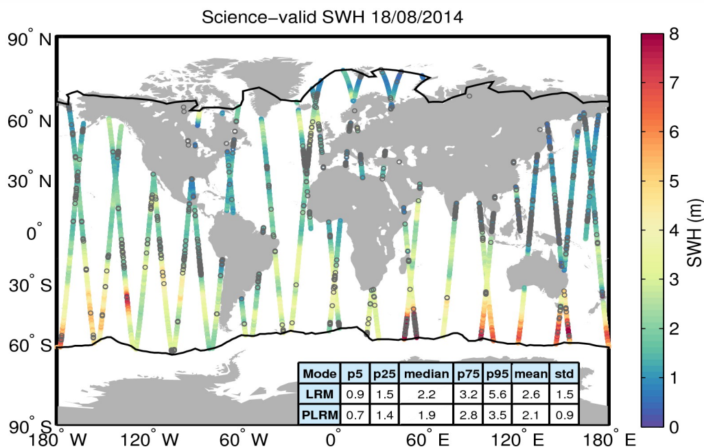
Figure 19. Geographical distribution of science-valid SWH data over oceans and lakes for 18/08/2014. The statistical values shown in the table refer to the SWH in m and are calculated separately for LRM and PLRM regions. The black lines mark the outer limit of the Arctic and Antarctic polar polygons. Gray circles denote records that have been rejected based on the editing criteria described in Table 3.
