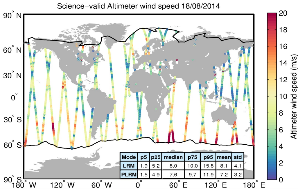
Figure 34. Geographical distribution of science-valid wind data over oceans and lakes for 18/08/2014. The statistical values shown in the table refer to the wind in m/s and are calculated separately for LRM and PLRM regions. The black lines mark the outer limit of the Arctic and Antarctic polar polygons. Gray circles denote records that have been rejected based on the editing criteria described in Table 5.
