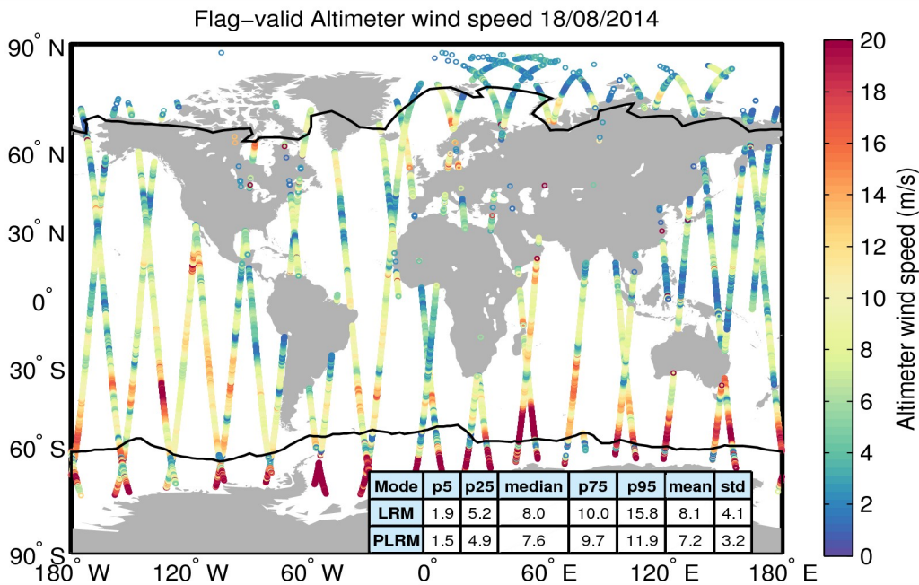
Figure 31. Geographical distribution of flag-valid wind data over oceans and lakes for 18/08/2014. The statistical values shown in the table refer to the wind in m/s and are calculated separately for LRM and PLRM regions. Measurements taken over polar polygons have been excluded from the computation of the statistical values. The black lines mark the outer limit of the Arctic and Antarctic polar polygons.
