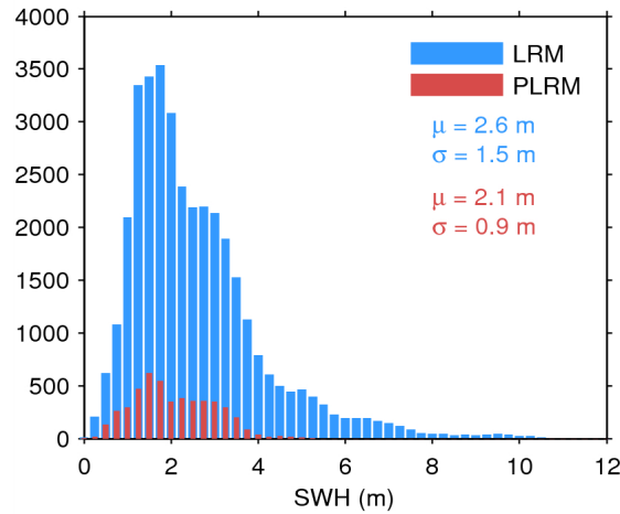
Figure 20. Histogram of science-valid SWH over oceans and lakes for LRM (blue) and PLRM (red) for 18/08/2014. The mean ( \mu ) and standard deviation ( \sigma ) are also shown. Note that values larger than 12 m are excluded from the histogram for the sake of readability but not from the computation of \mu and \sigma .
