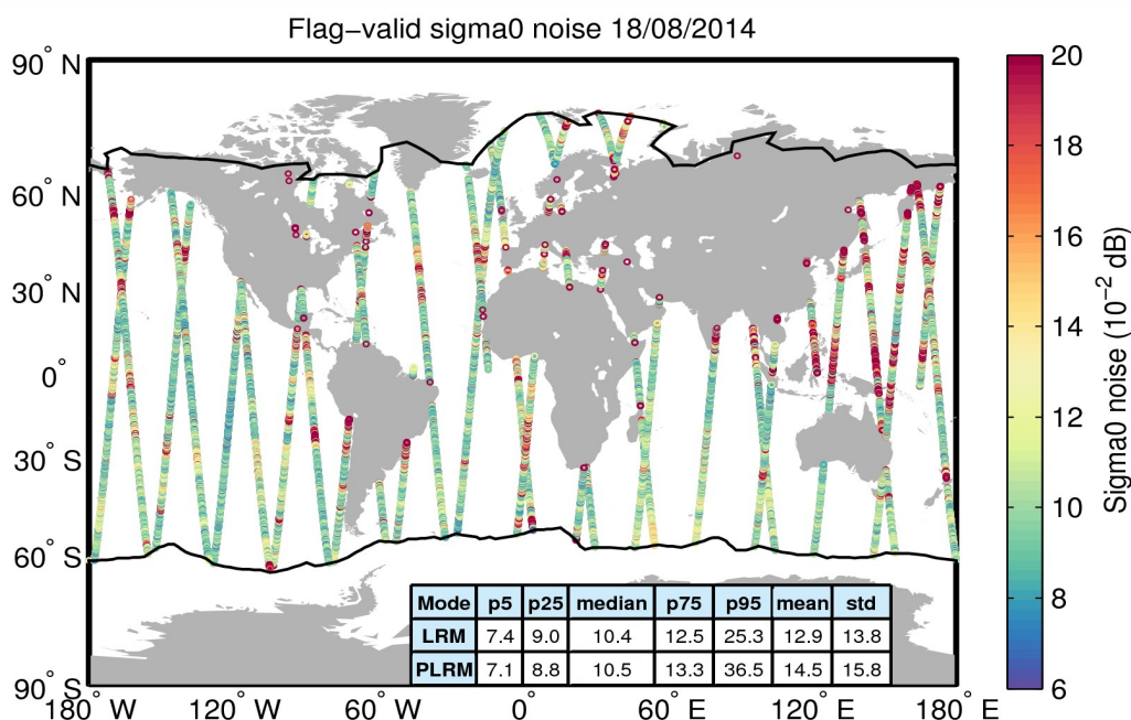
Figure 26. Geographical distribution of flag-valid 20-Hz sigma0 measurement noise over oceans and lakes for 18/08/2014. The statistical values shown in the table refer to the sigma0 noise and are calculated separately for LRM and PLRM regions. Measurements taken over polar polygons have been excluded from the computation of the statistical values. The black lines mark the outer limit of the Arctic and Antarctic polar polygons.
