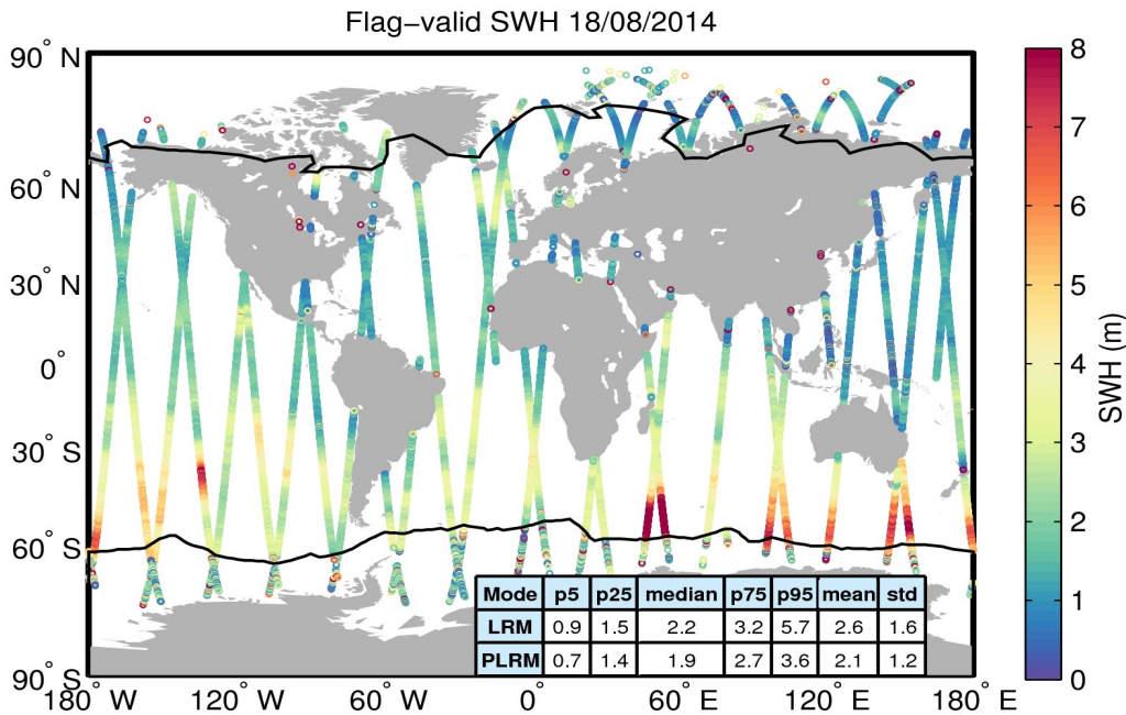
Figure 15. Geographical distribution of flag-valid SWH data over oceans and lakes for 18/08/2014. The statistical values shown in the table refer to the SWH in m and are calculated separately for LRM and PLRM regions. Measurements taken over polar polygons have been excluded from the computation of the statistical values. The black lines mark the outer limit of the Arctic and Antarctic polar polygons.
