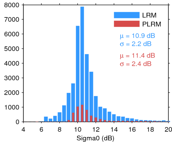
Figure 25. Histogram of flag-valid sigma0 over oceans and lakes for LRM (blue) and PLRM (red) for 18/08/2014. The mean ( \mu ) and standard deviation ( \sigma ) are also shown. Note that values outside [4 20] dB are excluded from the histogram for the sake of readability but not from the computation of \mu and \sigma .
