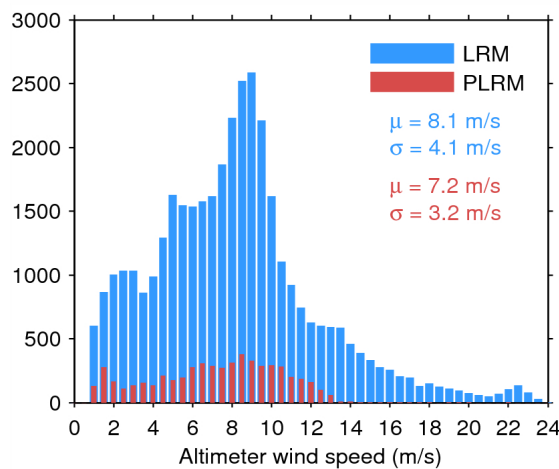
Figure 33. Histogram of flag-valid wind over oceans and lakes for LRM (blue) and PLRM (red) for 18/08/2014. The mean ( \mu ) and standard deviation ( \sigma ) are also shown. Note that values larger than 24 m/s are excluded from the histogram for the sake of readability but not from the computation of \mu and \sigma .
