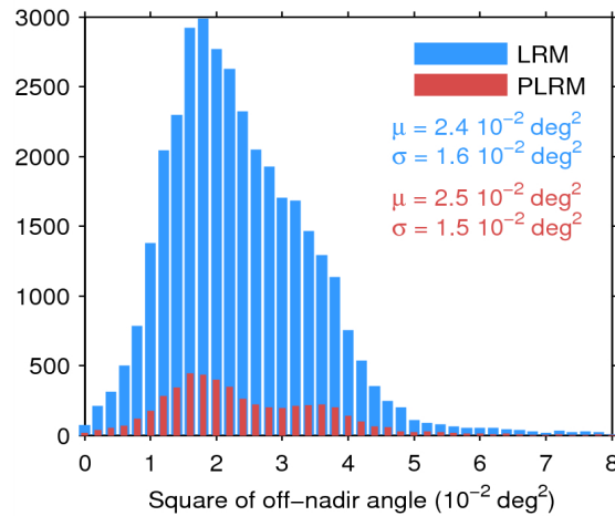
Figure 39. Histogram of flag-valid mispointing over oceans and lakes for LRM (blue) and PLRM (red) for 18/08/2014. Only positive values have been considered. The mean ( \mu ) and standard deviation ( \sigma ) are also shown. Note that values larger than 8 \cdot 10^{-2} \text{ deg}^2 are excluded from the histogram for the sake of readability but not from the computation of \mu and \sigma .
