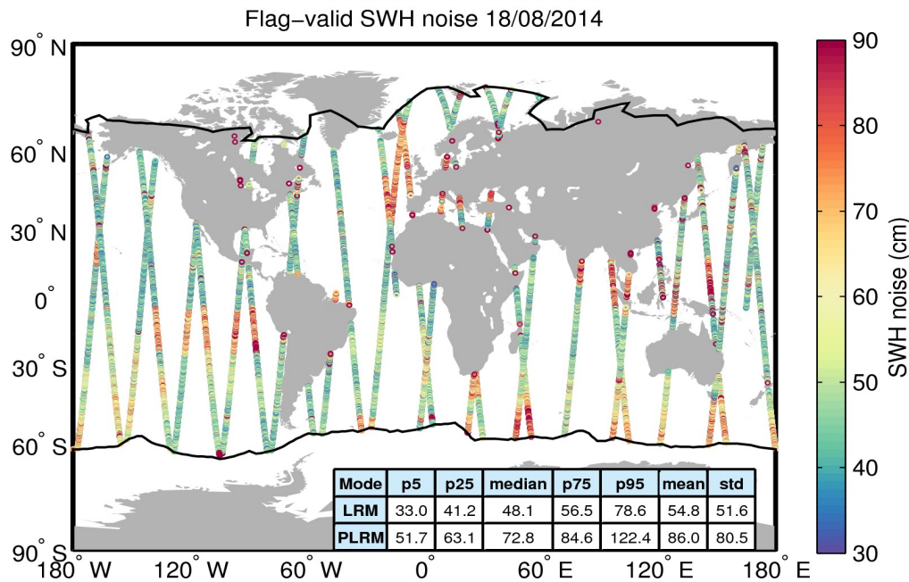
Figure 18. Geographical distribution of flag-valid 20-Hz SWH measurement noise over oceans and lakes for 18/08/2014. The statistical values shown in the table refer to the SWH noise and are calculated separately for LRM and PLRM regions. Measurements taken over polar polygons have been excluded from the computation of the statistical values. The black lines mark the outer limit of the Arctic and Antarctic polar polygons.
