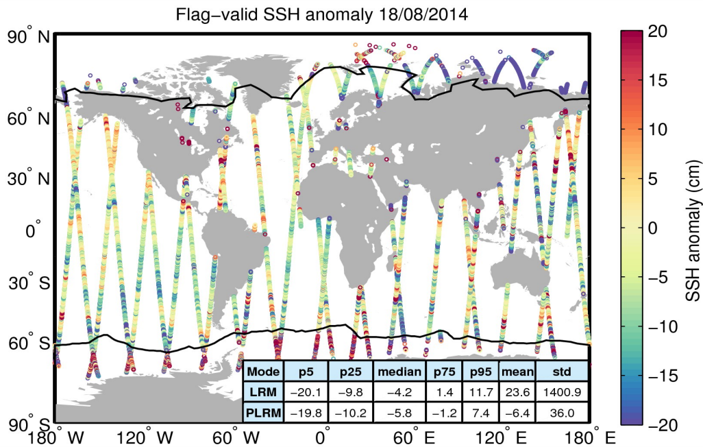
Figure 5. Geographical distribution of flag-valid 1-Hz SSH anomaly data over oceans and lakes for 18/08/2014. The statistical values shown in the table refer to the SSH anomaly in cm and are calculated separately for LRM and PLRM regions. Measurements taken over polar polygons have been excluded from the computation of the statistical values. The black lines mark the outer limit of the Arctic and Antarctic polar polygons.
