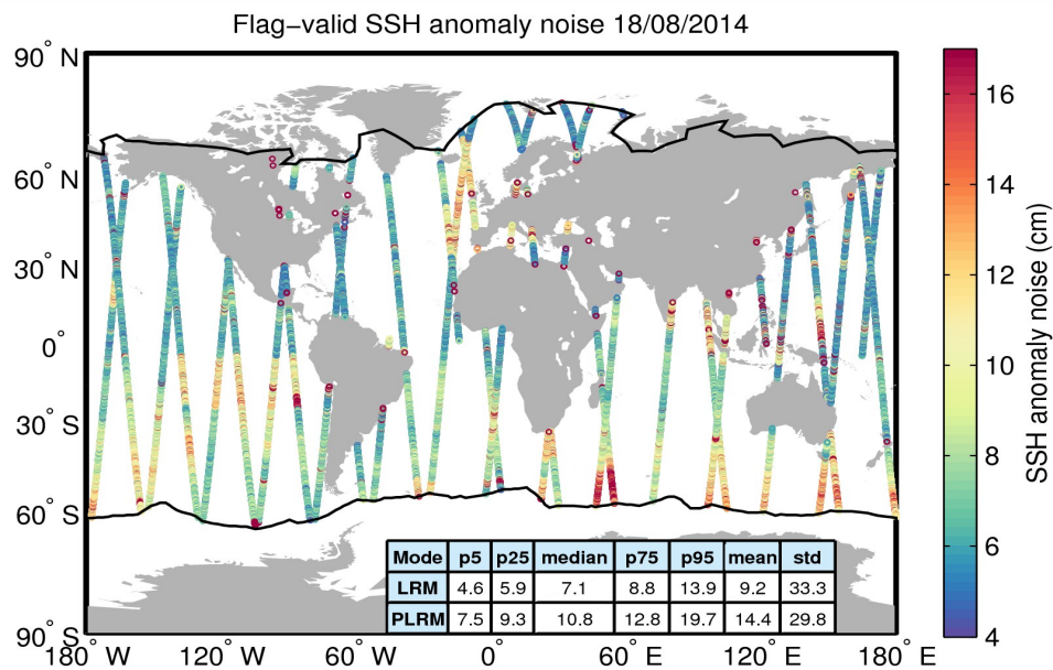
Figure 8. Geographical distribution of flag-valid 20-Hz SSH anomaly measurement noise over oceans and lakes for 18/08/2014. The statistical values shown in the table refer to the SSH anomaly noise and are calculated separately for LRM and PLRM regions. Measurements taken over polar polygons have been excluded from the computation of the statistical values. The black lines mark the outer limit of the Arctic and Antarctic polar polygons.
