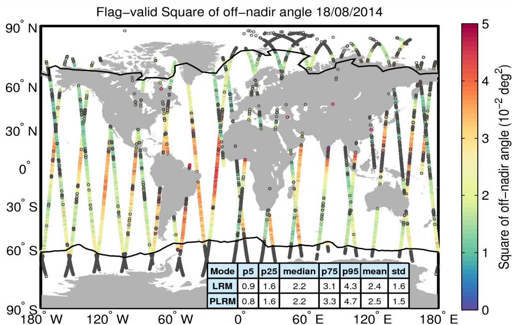
Figure 37. Geographical distribution of flag-valid mispointing data over oceans and lakes for 18/08/2014. The statistical values shown in the table refer to the mispointing in 10^{-2} \text{ deg}^2 and are calculated separately for LRM and PLRM regions. Measurements taken over polar polygons have been excluded from the computation of the statistical values. The black lines mark the outer limit of the Arctic and Antarctic polar polygons. Gray circles denote negative values.
