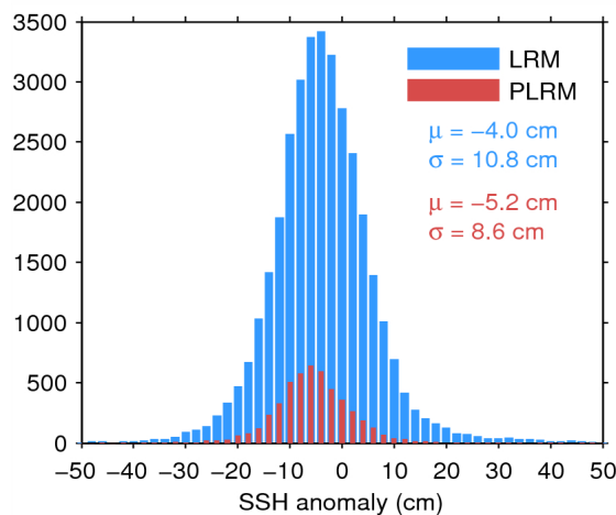
Figure 11. Histogram of science-valid SSH anomaly over oceans and lakes for LRM (blue) and PLRM (red) for 18/08/2014. The mean ( \mu ) and standard deviation ( \sigma ) are also shown. Note that values outside [-50 50] cm are excluded from the histogram for the sake of readability but not from the computation of \mu and \sigma .
