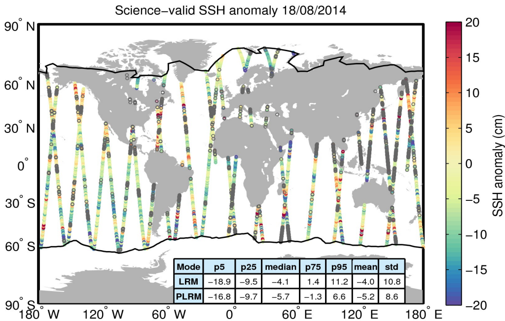
Figure 10. Geographical distribution of science-valid SSH anomaly data over oceans and lakes for 18/08/2014. The statistical values shown in the table refer to the SSH anomaly in cm and are calculated separately for LRM and PLRM regions. The black lines mark the outer limit of the Arctic and Antarctic polar polygons. Gray circles denote records that have been rejected based on the editing criteria described in Table 2.
