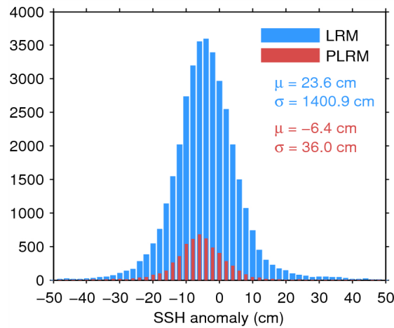
Figure 7. Histogram of flag-valid SSH anomaly over oceans and lakes for LRM (blue) and PLRM (red) for 18/08/2014. The mean ( \mu ) and standard deviation ( \sigma ) are also shown. Note that values outside [-50\ 50] cm are excluded from the histogram for the sake of readability but not from the computation of \mu and \sigma .
