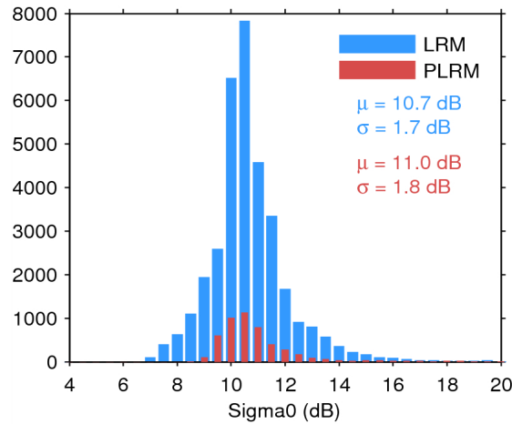
Figure 28. Histogram of science-valid sigma0 over oceans and lakes for LRM (blue) and PLRM (red) for 18/08/2014. The mean ( \mu ) and standard deviation ( \sigma ) are also shown. Note that values outside [4 20] dB are excluded from the histogram for the sake of readability but not from the computation of \mu and \sigma .
