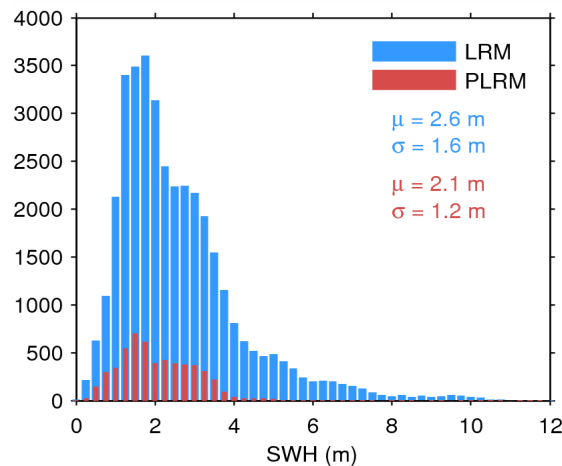
Figure 17. Histogram of flag-valid SWH over oceans and lakes for LRM (blue) and PLRM (red) for 18/08/2014. The mean ( \mu ) and standard deviation ( \sigma ) are also shown. Note that values larger than 12 m are excluded from the histogram for the sake of readability but not from the computation of \mu and \sigma .
