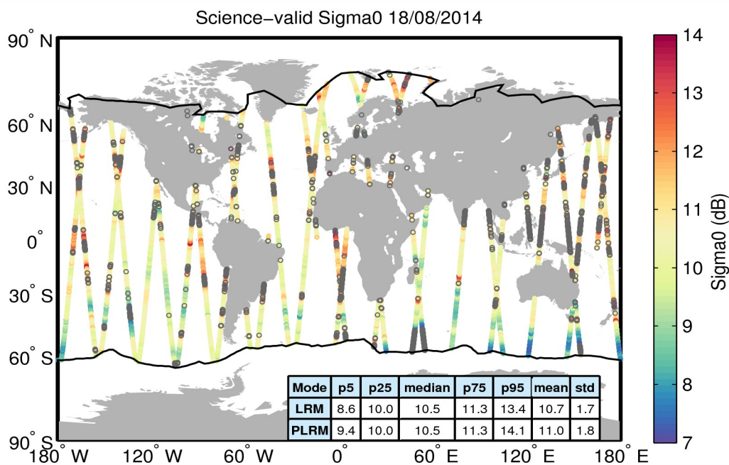
Figure 27. Geographical distribution of science-valid sigma0 data over oceans and lakes for 18/08/2014. The statistical values shown in the table refer to the sigma0 in dB and are calculated separately for LRM and PLRM regions. The black lines mark the outer limit of the Arctic and Antarctic polar polygons. Gray circles denote records that have been rejected based on the editing criteria described in Table 4.
