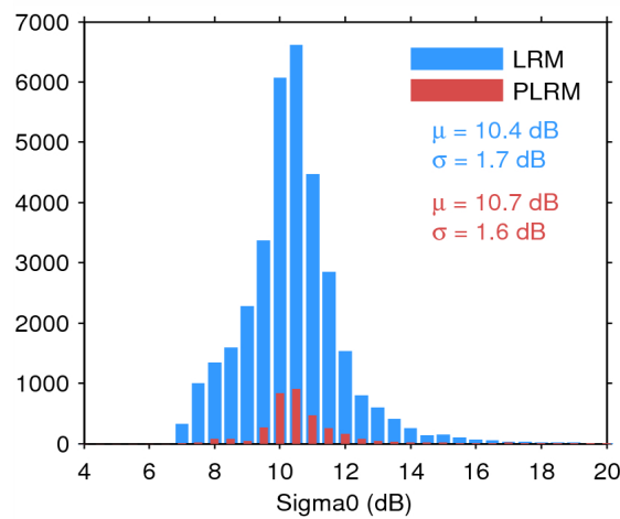
Figure 28. Histogram of science-valid sigma0 over oceans and lakes for LRM (blue) and PLRM (red) for 15/08/2014. The mean ( \mu ) and standard deviation ( \sigma ) are also shown. Note that values outside [4 20] dB are excluded from the histogram for the sake of readability but not from the computation of \mu and \sigma .
