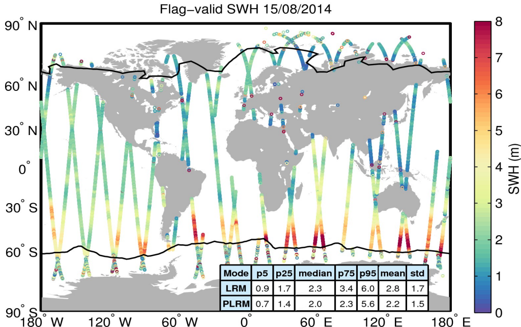
Figure 15. Geographical distribution of flag-valid SWH data over oceans and lakes for 15/08/2014. The statistical values shown in the table refer to the SWH in m and are calculated separately for LRM and PLRM regions. Measurements taken over polar polygons have been excluded from the computation of the statistical values. The black lines mark the outer limit of the Arctic and Antarctic polar polygons.
