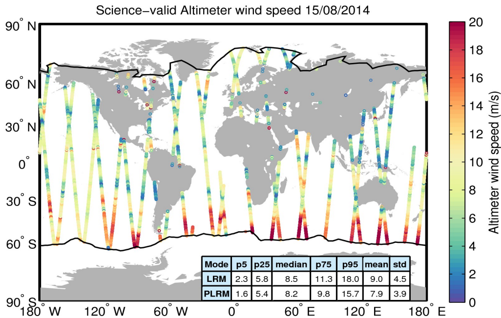
Figure 34. Geographical distribution of science-valid wind data over oceans and lakes for 15/08/2014. The statistical values shown in the table refer to the wind in m/s and are calculated separately for LRM and PLRM regions. The black lines mark the outer limit of the Arctic and Antarctic polar polygons. Gray circles denote records that have been rejected based on the editing criteria described in Table 5.
