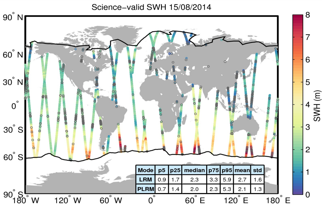
Figure 19. Geographical distribution of science-valid SWH data over oceans and lakes for 15/08/2014. The statistical values shown in the table refer to the SWH in m and are calculated separately for LRM and PLRM regions. The black lines mark the outer limit of the Arctic and Antarctic polar polygons. Gray circles denote records that have been rejected based on the editing criteria described in Table 3.
