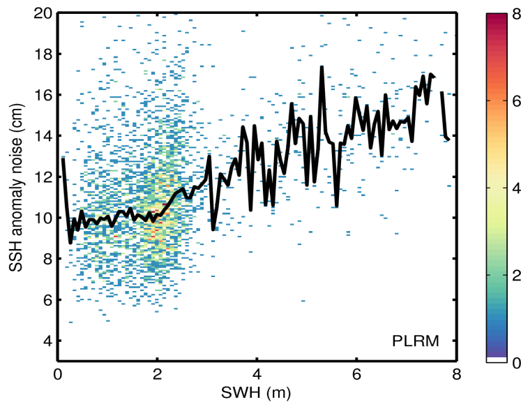
Figure 9. 2D histogram showing flag-valid SSH anomaly noise as a function of SWH for LRM (top) and PLRM (bottom) for 15/08/2014. The black line denotes the median SSH anomaly as a function of SWH.
