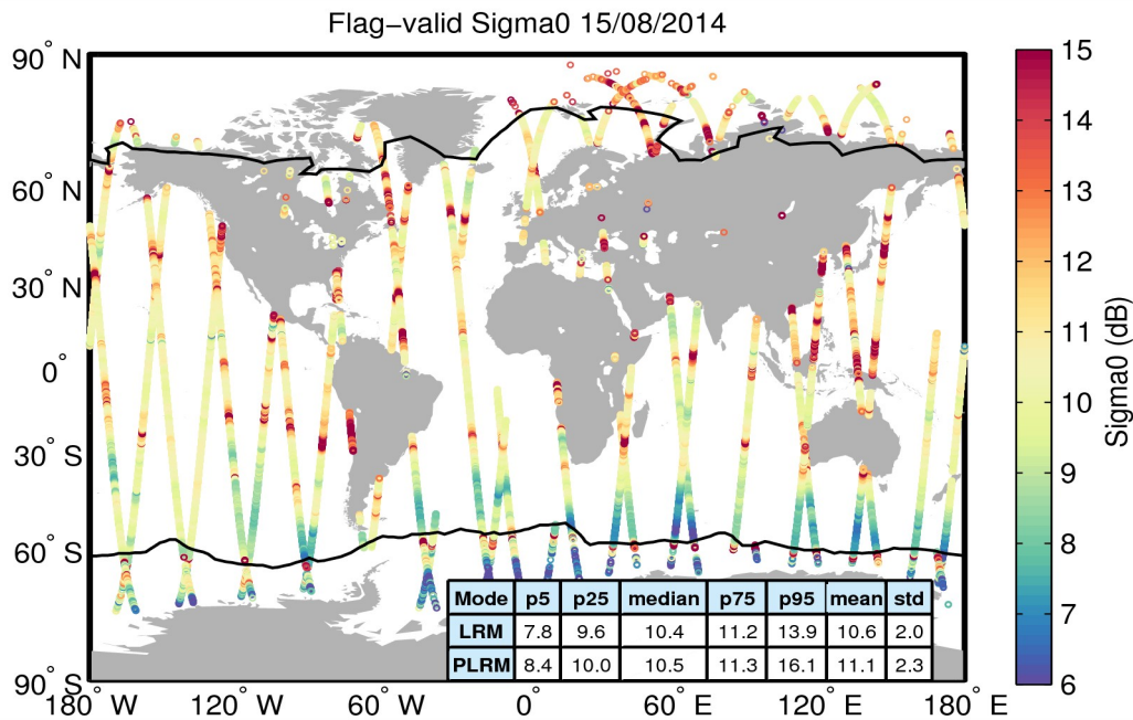
Figure 23. Geographical distribution of flag-valid sigma0 data over oceans and lakes for 15/08/2014. The statistical values shown in the table refer to the sigma0 in dB and are calculated separately for LRM and PLRM regions. Measurements taken over polar polygons have been excluded from the computation of the statistical values. The black lines mark the outer limit of the Arctic and Antarctic polar polygons.
