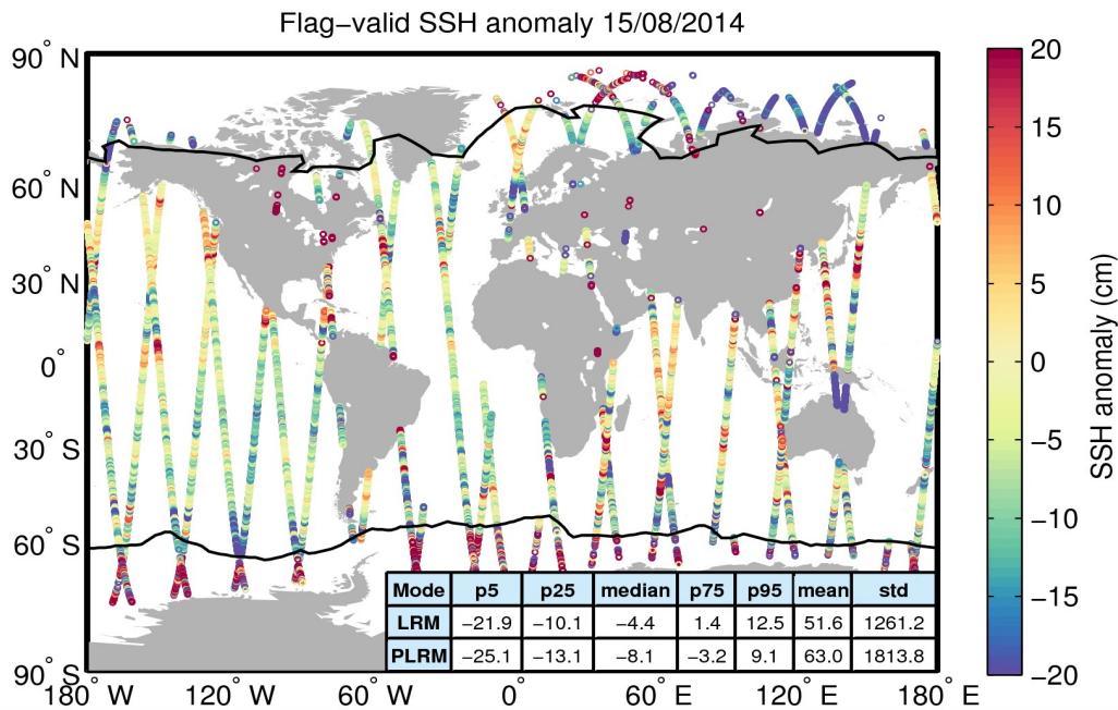
Figure 5. Geographical distribution of flag-valid 1-Hz SSH anomaly data over oceans and lakes for 15/08/2014. The statistical values shown in the table refer to the SSH anomaly in cm and are calculated separately for LRM and PLRM regions. Measurements taken over polar polygons have been excluded from the computation of the statistical values. The black lines mark the outer limit of the Arctic and Antarctic polar polygons.
