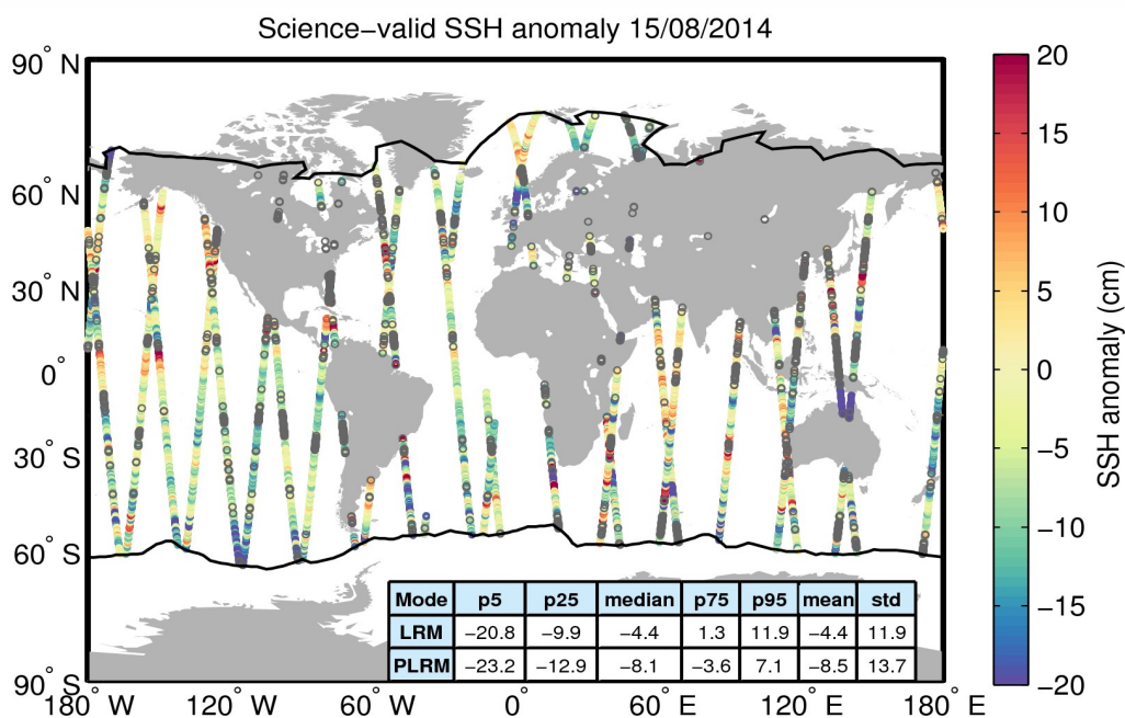
Figure 10. Geographical distribution of science-valid SSH anomaly data over oceans and lakes for 15/08/2014. The statistical values shown in the table refer to the SSH anomaly in cm and are calculated separately for LRM and PLRM regions. The black lines mark the outer limit of the Arctic and Antarctic polar polygons. Gray circles denote records that have been rejected based on the editing criteria described in Table 2.
