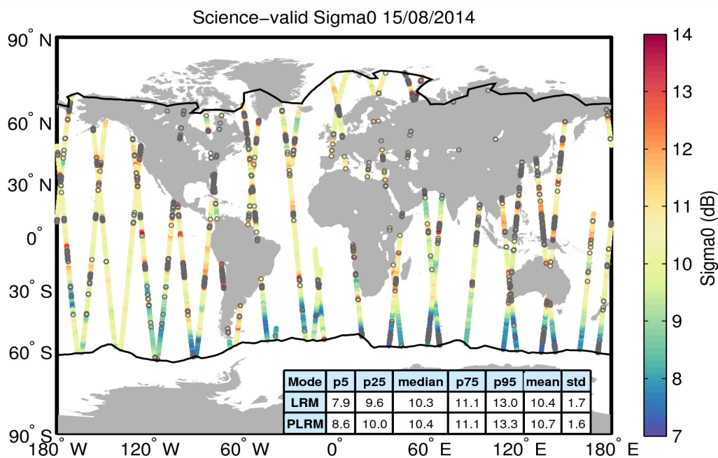
Figure 27. Geographical distribution of science-valid sigma0 data over oceans and lakes for 15/08/2014. The statistical values shown in the table refer to the sigma0 in dB and are calculated separately for LRM and PLRM regions. The black lines mark the outer limit of the Arctic and Antarctic polar polygons. Gray circles denote records that have been rejected based on the editing criteria described in Table 4.
