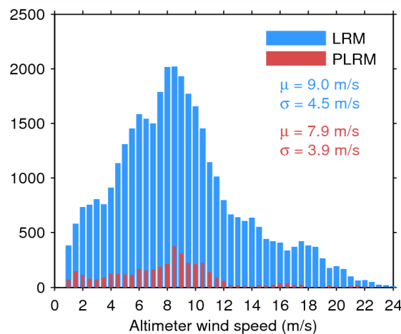
Figure 35. Histogram of science-valid wind over oceans and lakes for LRM (blue) and PLRM (red) for 15/08/2014. The mean ( \mu ) and standard deviation ( \sigma ) are also shown. Note that values larger than 24 m/s are excluded from the histogram for the sake of readability but not from the computation of \mu and \sigma .
