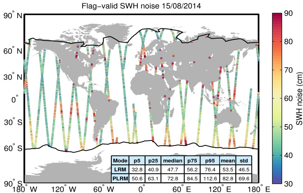
Figure 18. Geographical distribution of flag-valid 20-Hz SWH measurement noise over oceans and lakes for 15/08/2014. The statistical values shown in the table refer to the SWH noise and are calculated separately for LRM and PLRM regions. Measurements taken over polar polygons have been excluded from the computation of the statistical values. The black lines mark the outer limit of the Arctic and Antarctic polar polygons.
