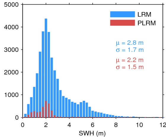
Figure 17. Histogram of flag-valid SWH over oceans and lakes for LRM (blue) and PLRM (red) for 15/08/2014. The mean ( \mu ) and standard deviation ( \sigma ) are also shown. Note that values larger than 12 m are excluded from the histogram for the sake of readability but not from the computation of \mu and \sigma .
