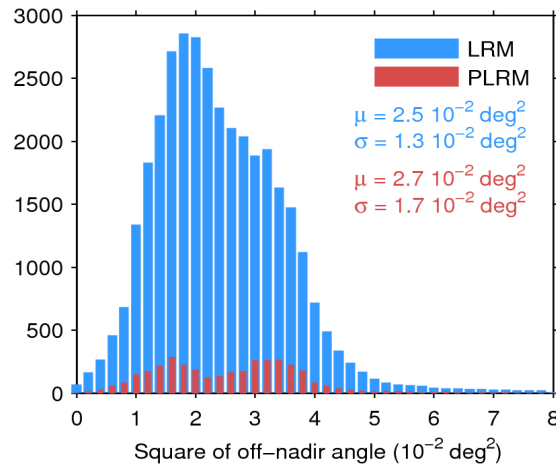
Figure 39. Histogram of flag-valid mispointing over oceans and lakes for LRM (blue) and PLRM (red) for 15/08/2014. Only positive values have been considered. The mean ( \mu ) and standard deviation ( \sigma ) are also shown. Note that values larger than 8 \cdot 10^{-2} \text{ deg}^2 are excluded from the histogram for the sake of readability but not from the computation of \mu and \sigma .
