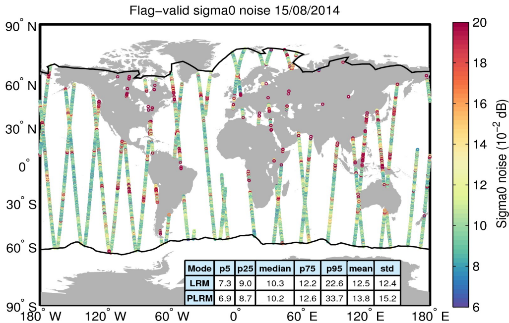
Figure 26. Geographical distribution of flag-valid 20-Hz sigma0 measurement noise over oceans and lakes for 15/08/2014. The statistical values shown in the table refer to the sigma0 noise and are calculated separately for LRM and PLRM regions. Measurements taken over polar polygons have been excluded from the computation of the statistical values. The black lines mark the outer limit of the Arctic and Antarctic polar polygons.
