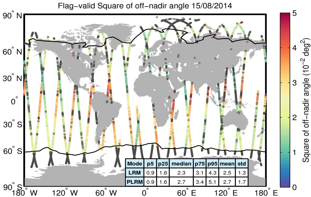
Figure 37. Geographical distribution of flag-valid mispointing data over oceans and lakes for 15/08/2014. The statistical values shown in the table refer to the mispointing in 10^{-2} \text{ deg}^2 and are calculated separately for LRM and PLRM regions. Measurements taken over polar polygons have been excluded from the computation of the statistical values. The black lines mark the outer limit of the Arctic and Antarctic polar polygons. Gray circles denote negative values.
