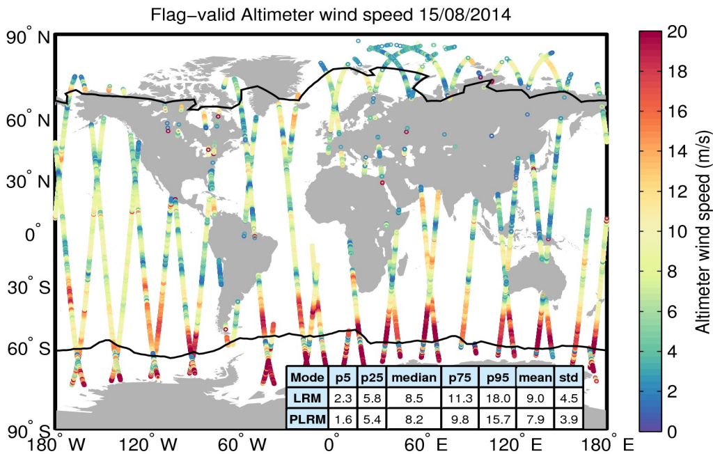
Figure 31. Geographical distribution of flag-valid wind data over oceans and lakes for 15/08/2014. The statistical values shown in the table refer to the wind in m/s and are calculated separately for LRM and PLRM regions. Measurements taken over polar polygons have been excluded from the computation of the statistical values. The black lines mark the outer limit of the Arctic and Antarctic polar polygons.
