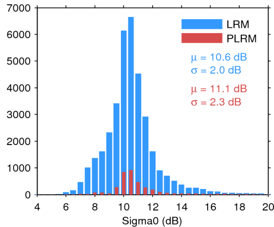
Figure 25. Histogram of flag-valid sigma0 over oceans and lakes for LRM (blue) and PLRM (red) for 15/08/2014. The mean ( \mu ) and standard deviation ( \sigma ) are also shown. Note that values outside [4 20] dB are excluded from the histogram for the sake of readability but not from the computation of \mu and \sigma .
