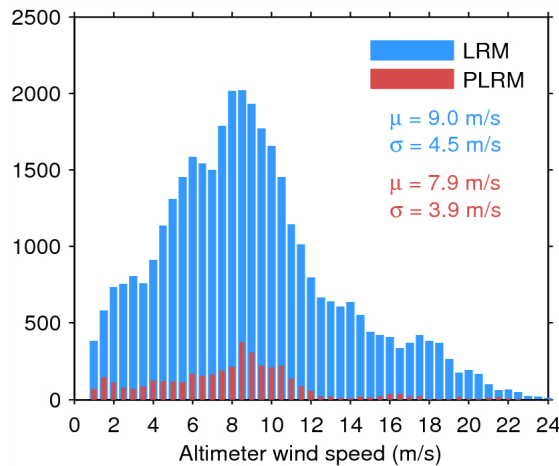
Figure 33. Histogram of flag-valid wind over oceans and lakes for LRM (blue) and PLRM (red) for 15/08/2014. The mean ( \mu ) and standard deviation ( \sigma ) are also shown. Note that values larger than 24 m/s are excluded from the histogram for the sake of readability but not from the computation of \mu and \sigma .
