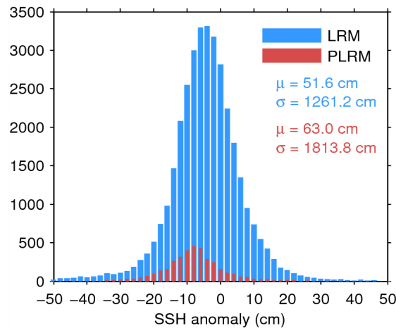
Figure 7. Histogram of flag-valid SSH anomaly over oceans and lakes for LRM (blue) and PLRM (red) for 15/08/2014. The mean ( \mu ) and standard deviation ( \sigma ) are also shown. Note that values outside [-50\ 50] cm are excluded from the histogram for the sake of readability but not from the computation of \mu and \sigma .
