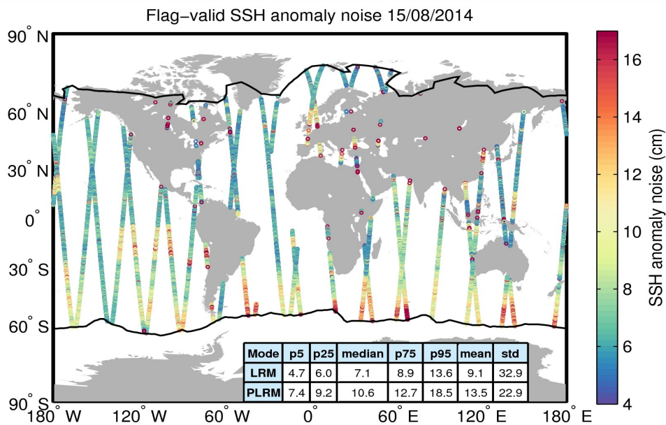
Figure 8. Geographical distribution of flag-valid 20-Hz SSH anomaly measurement noise over oceans and lakes for 15/08/2014. The statistical values shown in the table refer to the SSH anomaly noise and are calculated separately for LRM and PLRM regions. Measurements taken over polar polygons have been excluded from the computation of the statistical values. The black lines mark the outer limit of the Arctic and Antarctic polar polygons.
