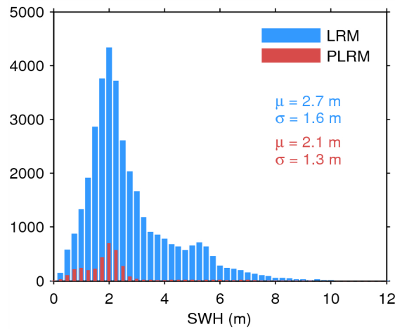
Figure 20. Histogram of science-valid SWH over oceans and lakes for LRM (blue) and PLRM (red) for 15/08/2014. The mean ( \mu ) and standard deviation ( \sigma ) are also shown. Note that values larger than 12 m are excluded from the histogram for the sake of readability but not from the computation of \mu and \sigma .
