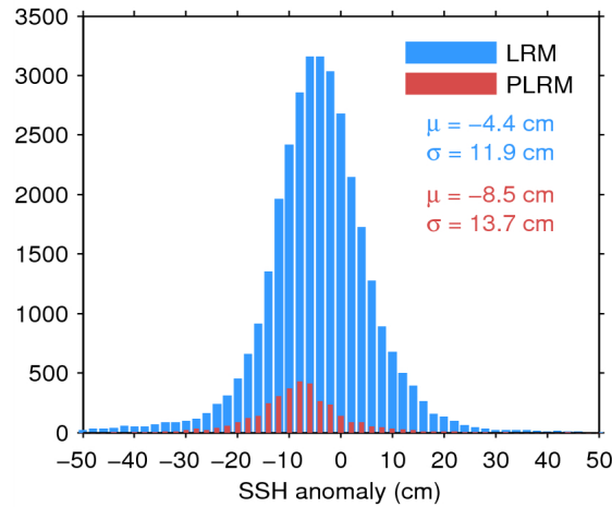
Figure 11. Histogram of science-valid SSH anomaly over oceans and lakes for LRM (blue) and PLRM (red) for 15/08/2014. The mean ( \mu ) and standard deviation ( \sigma ) are also shown. Note that values outside [-50 50] cm are excluded from the histogram for the sake of readability but not from the computation of \mu and \sigma .
