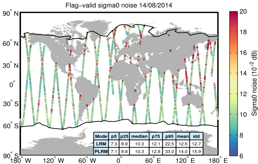
Figure 26. Geographical distribution of flag-valid 20-Hz sigma0 measurement noise over oceans and lakes for 14/08/2014. The statistical values shown in the table refer to the sigma0 noise and are calculated separately for LRM and PLRM regions. Measurements taken over polar polygons have been excluded from the computation of the statistical values. The black lines mark the outer limit of the Arctic and Antarctic polar polygons.
