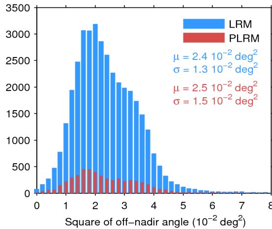
Figure 39. Histogram of flag-valid mispointing over oceans and lakes for LRM (blue) and PLRM (red) for 14/08/2014. Only positive values have been considered. The mean ( \mu ) and standard deviation ( \sigma ) are also shown. Note that values larger than 8 \cdot 10^{-2} \text{ deg}^2 are excluded from the histogram for the sake of readability but not from the computation of \mu and \sigma .
