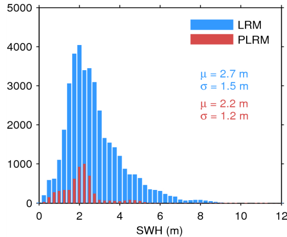
Figure 17. Histogram of flag-valid SWH over oceans and lakes for LRM (blue) and PLRM (red) for 14/08/2014. The mean ( \mu ) and standard deviation ( \sigma ) are also shown. Note that values larger than 12 m are excluded from the histogram for the sake of readability but not from the computation of \mu and \sigma .
