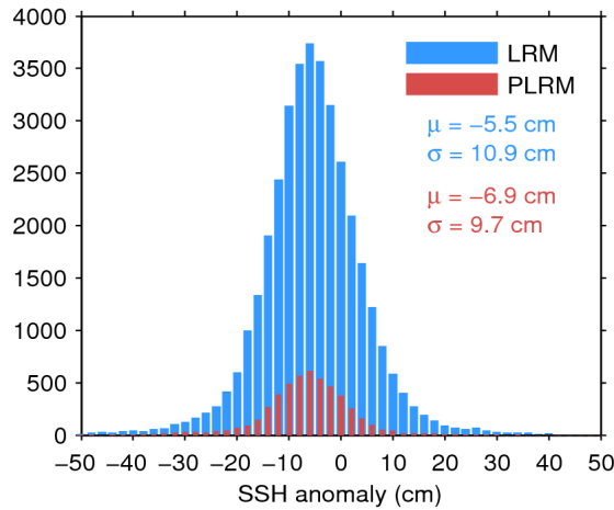
Figure 11. Histogram of science-valid SSH anomaly over oceans and lakes for LRM (blue) and PLRM (red) for 14/08/2014. The mean ( \mu ) and standard deviation ( \sigma ) are also shown. Note that values outside [-50 50] cm are excluded from the histogram for the sake of readability but not from the computation of \mu and \sigma .
