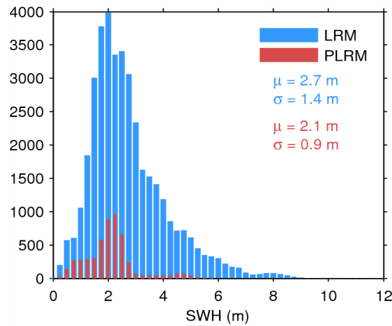
Figure 20. Histogram of science-valid SWH over oceans and lakes for LRM (blue) and PLRM (red) for 14/08/2014. The mean ( \mu ) and standard deviation ( \sigma ) are also shown. Note that values larger than 12 m are excluded from the histogram for the sake of readability but not from the computation of \mu and \sigma .
