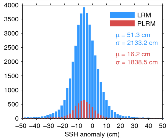
Figure 7. Histogram of flag-valid SSH anomaly over oceans and lakes for LRM (blue) and PLRM (red) for 14/08/2014. The mean ( \mu ) and standard deviation ( \sigma ) are also shown. Note that values outside [-50\ 50] cm are excluded from the histogram for the sake of readability but not from the computation of \mu and \sigma .
