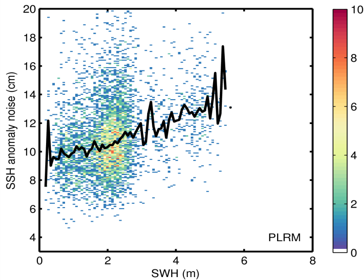
Figure 9. 2D histogram showing flag-valid SSH anomaly noise as a function of SWH for LRM (top) and PLRM (bottom) for 14/08/2014. The black line denotes the median SSH anomaly as a function of SWH.
