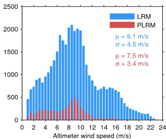
Figure 33. Histogram of flag-valid wind over oceans and lakes for LRM (blue) and PLRM (red) for 14/08/2014. The mean ( \mu ) and standard deviation ( \sigma ) are also shown. Note that values larger than 24 m/s are excluded from the histogram for the sake of readability but not from the computation of \mu and \sigma .
