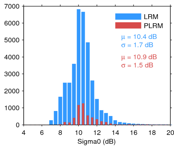
Figure 28. Histogram of science-valid sigma0 over oceans and lakes for LRM (blue) and PLRM (red) for 14/08/2014. The mean ( \mu ) and standard deviation ( \sigma ) are also shown. Note that values outside [4 20] dB are excluded from the histogram for the sake of readability but not from the computation of \mu and \sigma .
