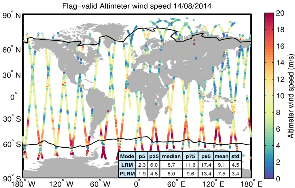
Figure 31. Geographical distribution of flag-valid wind data over oceans and lakes for 14/08/2014. The statistical values shown in the table refer to the wind in m/s and are calculated separately for LRM and PLRM regions. Measurements taken over polar polygons have been excluded from the computation of the statistical values. The black lines mark the outer limit of the Arctic and Antarctic polar polygons.
