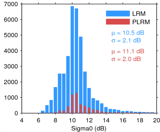
Figure 25. Histogram of flag-valid sigma0 over oceans and lakes for LRM (blue) and PLRM (red) for 14/08/2014. The mean ( \mu ) and standard deviation ( \sigma ) are also shown. Note that values outside [4 20] dB are excluded from the histogram for the sake of readability but not from the computation of \mu and \sigma .
