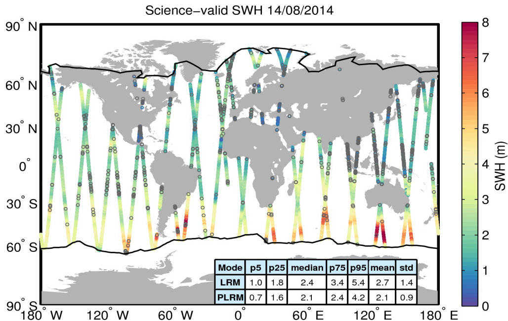
Figure 19. Geographical distribution of science-valid SWH data over oceans and lakes for 14/08/2014. The statistical values shown in the table refer to the SWH in m and are calculated separately for LRM and PLRM regions. The black lines mark the outer limit of the Arctic and Antarctic polar polygons. Gray circles denote records that have been rejected based on the editing criteria described in Table 3.
