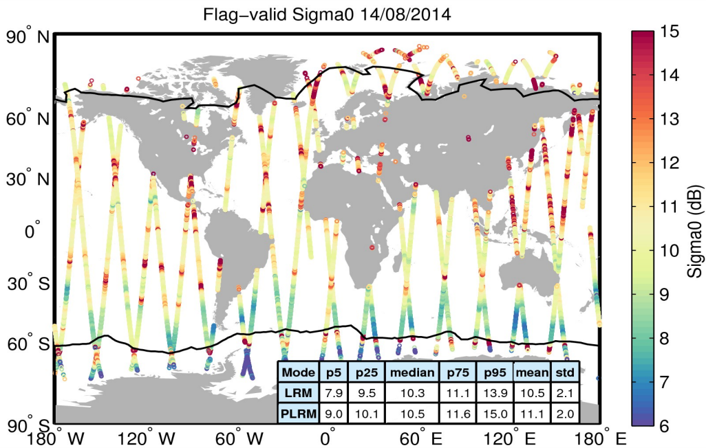
Figure 23. Geographical distribution of flag-valid sigma0 data over oceans and lakes for 14/08/2014. The statistical values shown in the table refer to the sigma0 in dB and are calculated separately for LRM and PLRM regions. Measurements taken over polar polygons have been excluded from the computation of the statistical values. The black lines mark the outer limit of the Arctic and Antarctic polar polygons.
