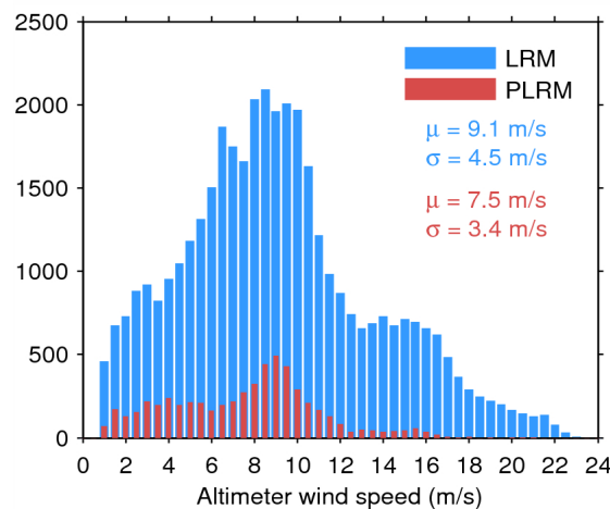
Figure 35. Histogram of science-valid wind over oceans and lakes for LRM (blue) and PLRM (red) for 14/08/2014. The mean ( \mu ) and standard deviation ( \sigma ) are also shown. Note that values larger than 24 m/s are excluded from the histogram for the sake of readability but not from the computation of \mu and \sigma .
