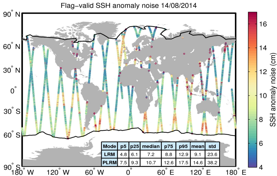
Figure 8. Geographical distribution of flag-valid 20-Hz SSH anomaly measurement noise over oceans and lakes for 14/08/2014. The statistical values shown in the table refer to the SSH anomaly noise and are calculated separately for LRM and PLRM regions. Measurements taken over polar polygons have been excluded from the computation of the statistical values. The black lines mark the outer limit of the Arctic and Antarctic polar polygons.
