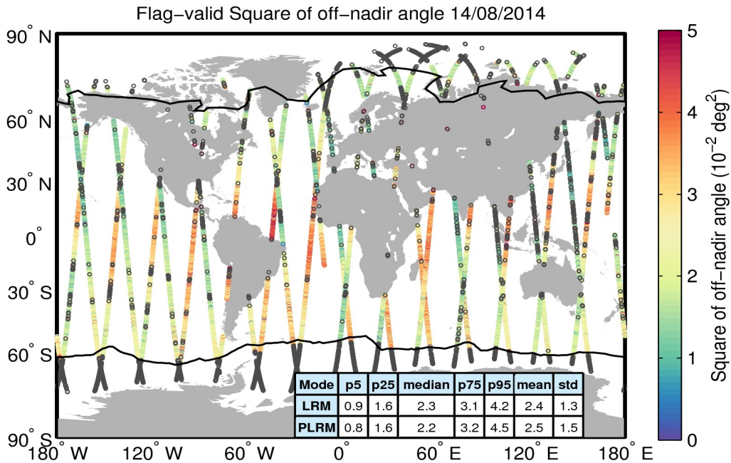
Figure 37. Geographical distribution of flag-valid mispointing data over oceans and lakes for 14/08/2014. The statistical values shown in the table refer to the mispointing in 10^{-2} \text{ deg}^2 and are calculated separately for LRM and PLRM regions. Measurements taken over polar polygons have been excluded from the computation of the statistical values. The black lines mark the outer limit of the Arctic and Antarctic polar polygons. Gray circles denote negative values.
