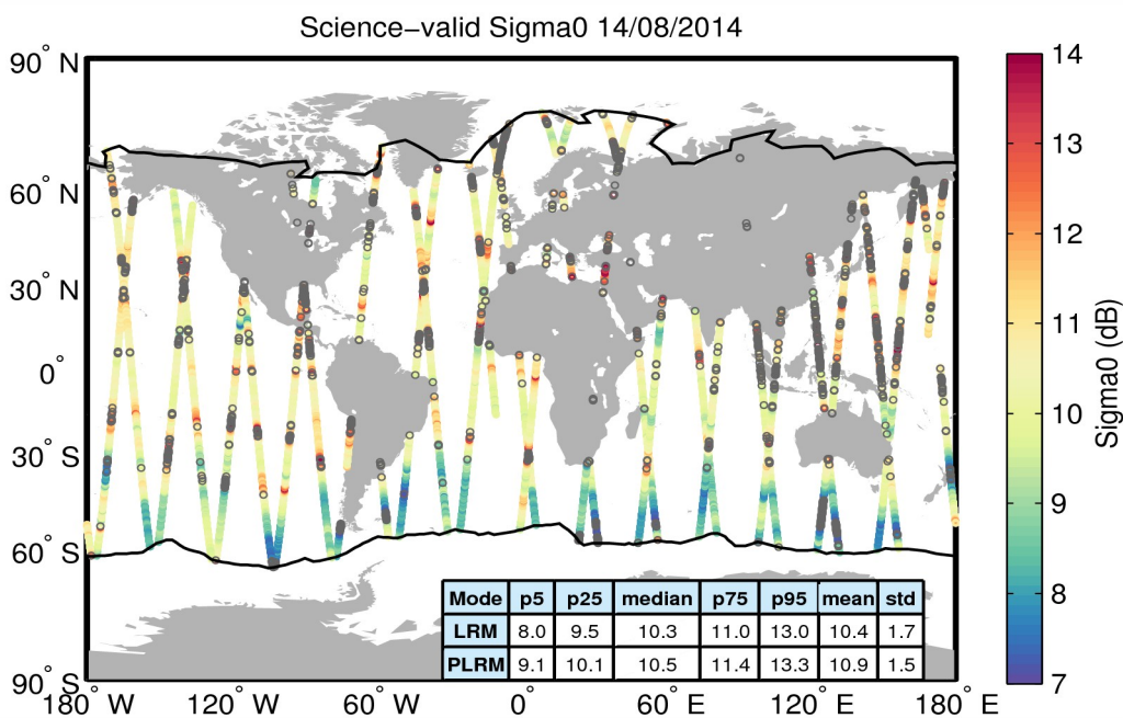
Figure 27. Geographical distribution of science-valid sigma0 data over oceans and lakes for 14/08/2014. The statistical values shown in the table refer to the sigma0 in dB and are calculated separately for LRM and PLRM regions. The black lines mark the outer limit of the Arctic and Antarctic polar polygons. Gray circles denote records that have been rejected based on the editing criteria described in Table 4.
