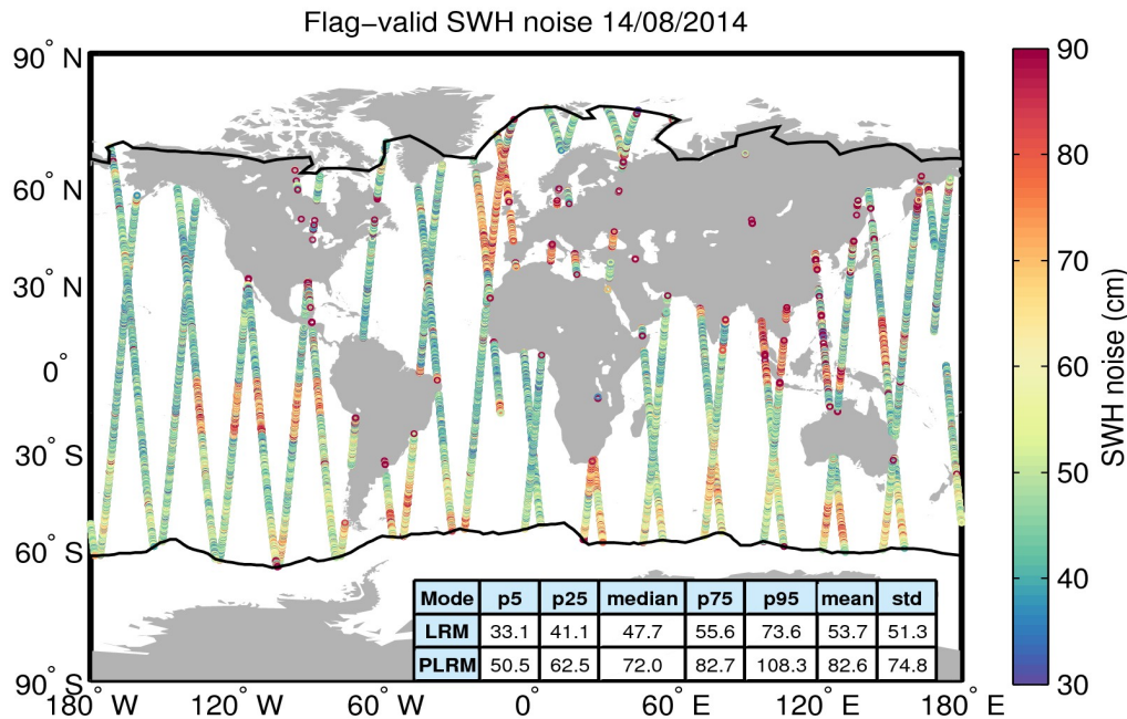
Figure 18. Geographical distribution of flag-valid 20-Hz SWH measurement noise over oceans and lakes for 14/08/2014. The statistical values shown in the table refer to the SWH noise and are calculated separately for LRM and PLRM regions. Measurements taken over polar polygons have been excluded from the computation of the statistical values. The black lines mark the outer limit of the Arctic and Antarctic polar polygons.
