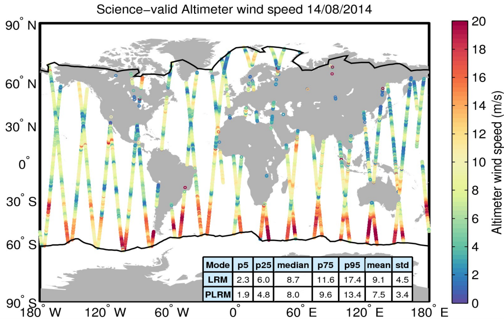
Figure 34. Geographical distribution of science-valid wind data over oceans and lakes for 14/08/2014. The statistical values shown in the table refer to the wind in m/s and are calculated separately for LRM and PLRM regions. The black lines mark the outer limit of the Arctic and Antarctic polar polygons. Gray circles denote records that have been rejected based on the editing criteria described in Table 5.
