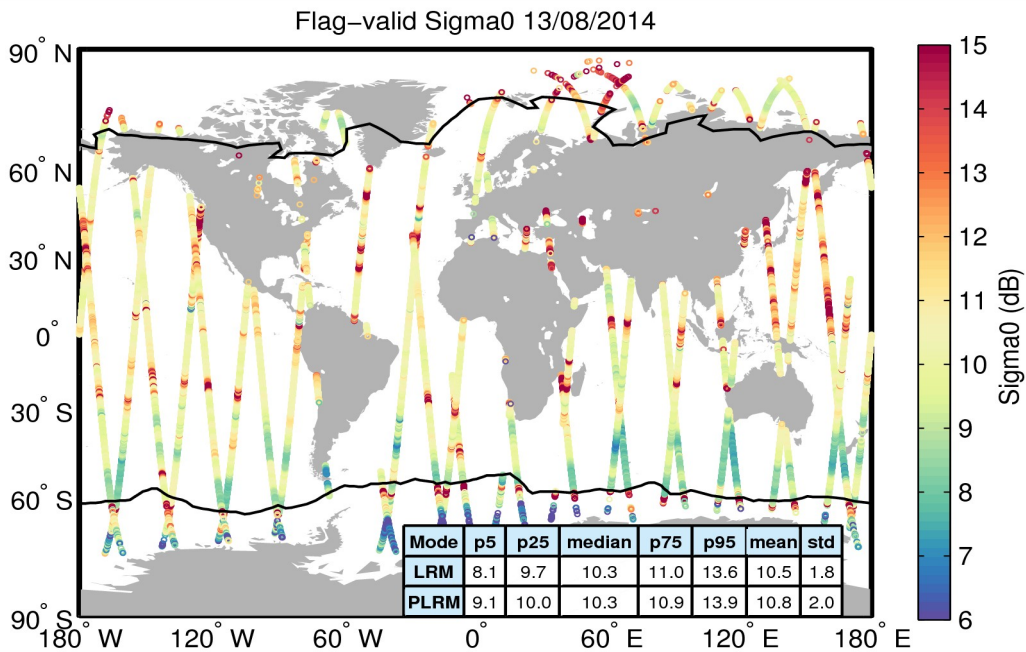
Figure 23. Geographical distribution of flag-valid sigma0 data over oceans and lakes for 13/08/2014. The statistical values shown in the table refer to the sigma0 in dB and are calculated separately for LRM and PLRM regions. Measurements taken over polar polygons have been excluded from the computation of the statistical values. The black lines mark the outer limit of the Arctic and Antarctic polar polygons.
