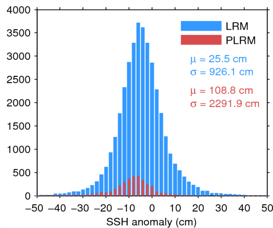
Figure 7. Histogram of flag-valid SSH anomaly over oceans and lakes for LRM (blue) and PLRM (red) for 13/08/2014. The mean ( \mu ) and standard deviation ( \sigma ) are also shown. Note that values outside [-50\ 50] cm are excluded from the histogram for the sake of readability but not from the computation of \mu and \sigma .
