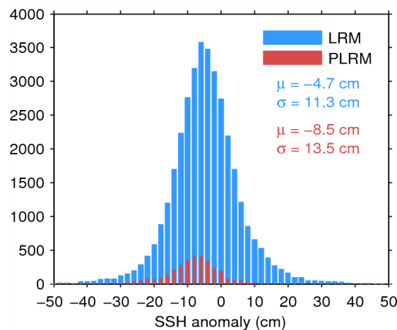
Figure 11. Histogram of science-valid SSH anomaly over oceans and lakes for LRM (blue) and PLRM (red) for 13/08/2014. The mean ( \mu ) and standard deviation ( \sigma ) are also shown. Note that values outside [-50 50] cm are excluded from the histogram for the sake of readability but not from the computation of \mu and \sigma .
