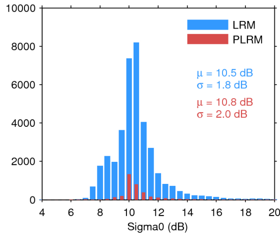
Figure 25. Histogram of flag-valid sigma0 over oceans and lakes for LRM (blue) and PLRM (red) for 13/08/2014. The mean ( \mu ) and standard deviation ( \sigma ) are also shown. Note that values outside [4 20] dB are excluded from the histogram for the sake of readability but not from the computation of \mu and \sigma .
