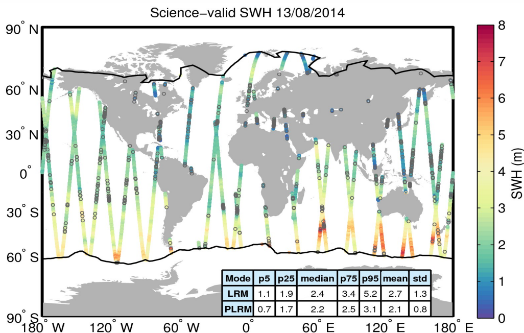
Figure 19. Geographical distribution of science-valid SWH data over oceans and lakes for 13/08/2014. The statistical values shown in the table refer to the SWH in m and are calculated separately for LRM and PLRM regions. The black lines mark the outer limit of the Arctic and Antarctic polar polygons. Gray circles denote records that have been rejected based on the editing criteria described in Table 3.
