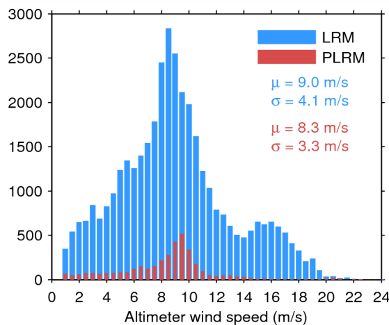
Figure 35. Histogram of science-valid wind over oceans and lakes for LRM (blue) and PLRM (red) for 13/08/2014. The mean ( \mu ) and standard deviation ( \sigma ) are also shown. Note that values larger than 24 m/s are excluded from the histogram for the sake of readability but not from the computation of \mu and \sigma .
