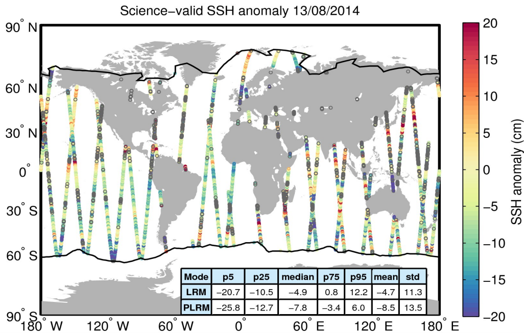
Figure 10. Geographical distribution of science-valid SSH anomaly data over oceans and lakes for 13/08/2014. The statistical values shown in the table refer to the SSH anomaly in cm and are calculated separately for LRM and PLRM regions. The black lines mark the outer limit of the Arctic and Antarctic polar polygons. Gray circles denote records that have been rejected based on the editing criteria described in Table 2.
