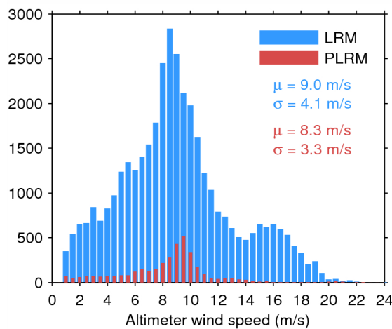
Figure 33. Histogram of flag-valid wind over oceans and lakes for LRM (blue) and PLRM (red) for 13/08/2014. The mean ( \mu ) and standard deviation ( \sigma ) are also shown. Note that values larger than 24 m/s are excluded from the histogram for the sake of readability but not from the computation of \mu and \sigma .
