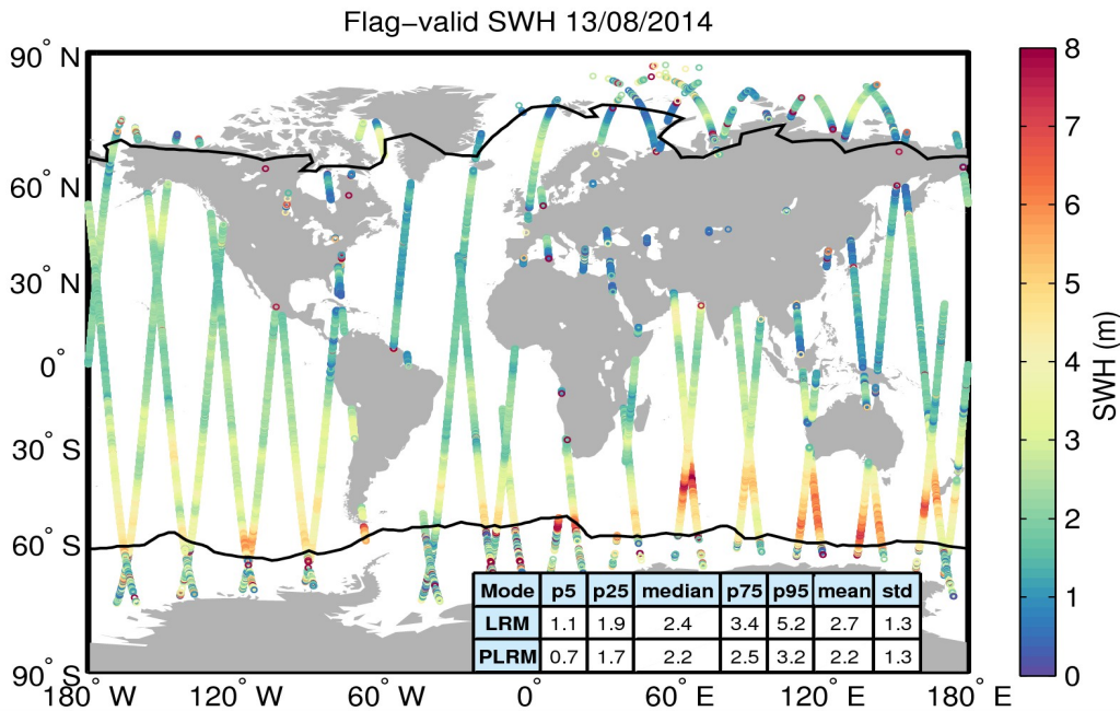
Figure 15. Geographical distribution of flag-valid SWH data over oceans and lakes for 13/08/2014. The statistical values shown in the table refer to the SWH in m and are calculated separately for LRM and PLRM regions. Measurements taken over polar polygons have been excluded from the computation of the statistical values. The black lines mark the outer limit of the Arctic and Antarctic polar polygons.
