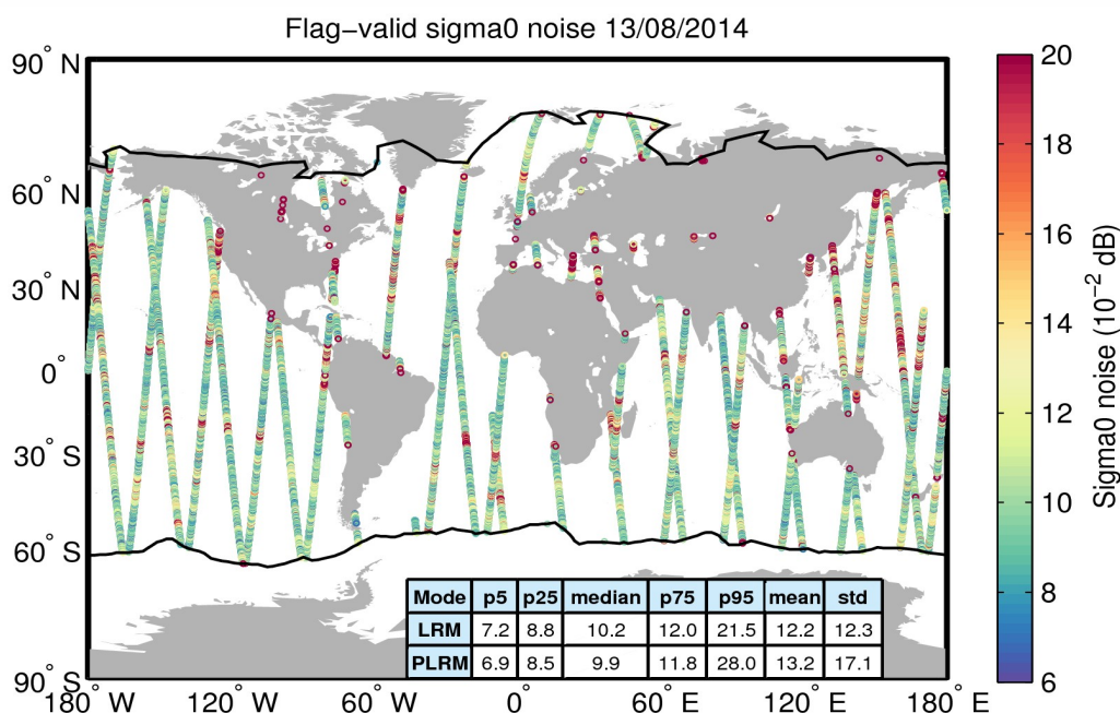
Figure 26. Geographical distribution of flag-valid 20-Hz sigma0 measurement noise over oceans and lakes for 13/08/2014. The statistical values shown in the table refer to the sigma0 noise and are calculated separately for LRM and PLRM regions. Measurements taken over polar polygons have been excluded from the computation of the statistical values. The black lines mark the outer limit of the Arctic and Antarctic polar polygons.
