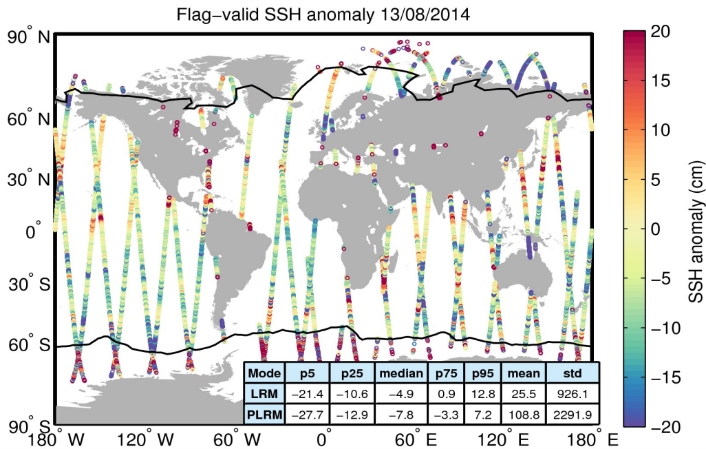
Figure 5. Geographical distribution of flag-valid 1-Hz SSH anomaly data over oceans and lakes for 13/08/2014. The statistical values shown in the table refer to the SSH anomaly in cm and are calculated separately for LRM and PLRM regions. Measurements taken over polar polygons have been excluded from the computation of the statistical values. The black lines mark the outer limit of the Arctic and Antarctic polar polygons.
