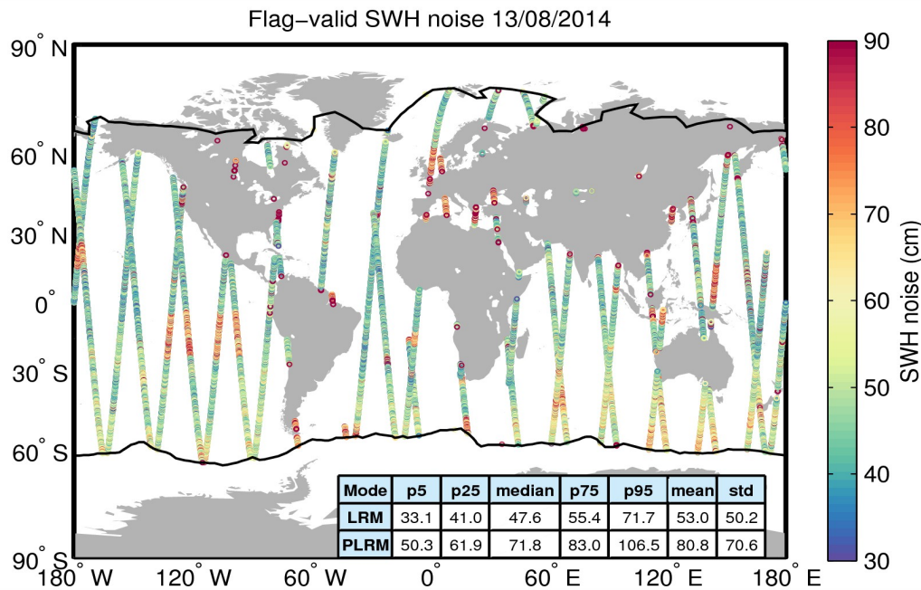
Figure 18. Geographical distribution of flag-valid 20-Hz SWH measurement noise over oceans and lakes for 13/08/2014. The statistical values shown in the table refer to the SWH noise and are calculated separately for LRM and PLRM regions. Measurements taken over polar polygons have been excluded from the computation of the statistical values. The black lines mark the outer limit of the Arctic and Antarctic polar polygons.
