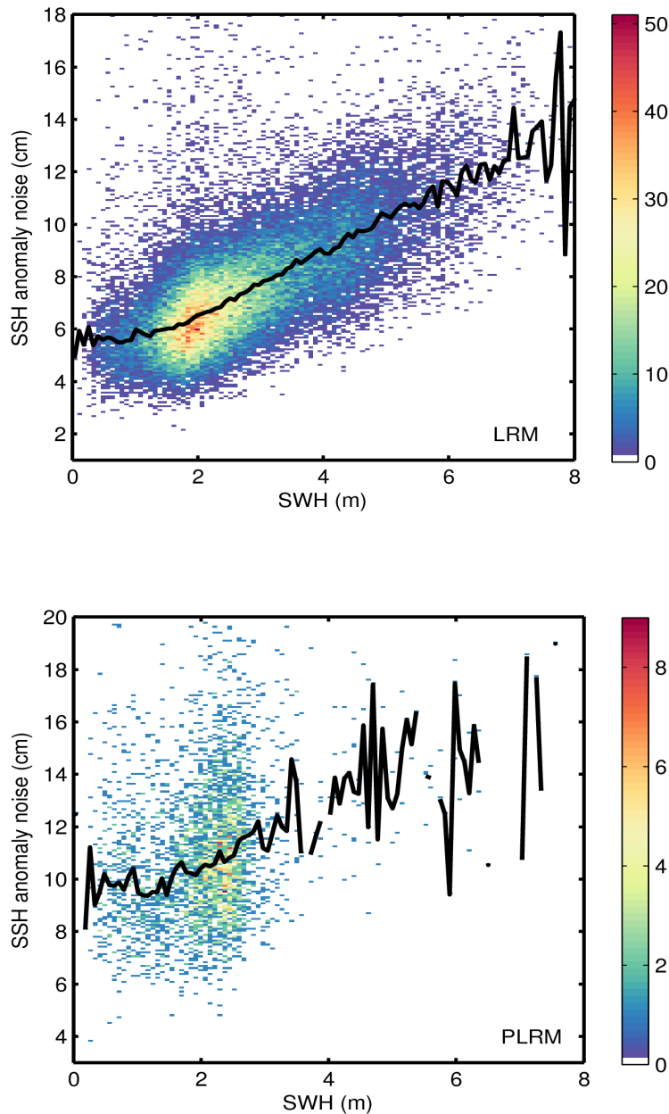
Figure 9. 2D histogram showing flag-valid SSH anomaly noise as a function of SWH for LRM (top) and PLRM (bottom) for 13/08/2014. The black line denotes the median SSH anomaly as a function of SWH.
