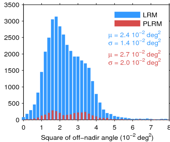
Figure 39. Histogram of flag-valid mispointing over oceans and lakes for LRM (blue) and PLRM (red) for 13/08/2014. Only positive values have been considered. The mean ( \mu ) and standard deviation ( \sigma ) are also shown. Note that values larger than 8 \cdot 10^{-2} \text{ deg}^2 are excluded from the histogram for the sake of readability but not from the computation of \mu and \sigma .
