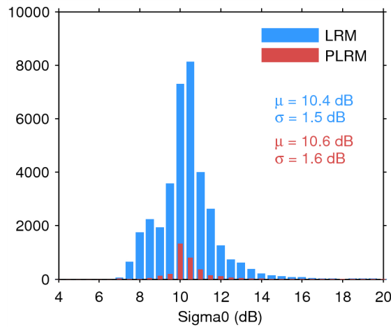
Figure 28. Histogram of science-valid sigma0 over oceans and lakes for LRM (blue) and PLRM (red) for 13/08/2014. The mean ( \mu ) and standard deviation ( \sigma ) are also shown. Note that values outside [4 20] dB are excluded from the histogram for the sake of readability but not from the computation of \mu and \sigma .
