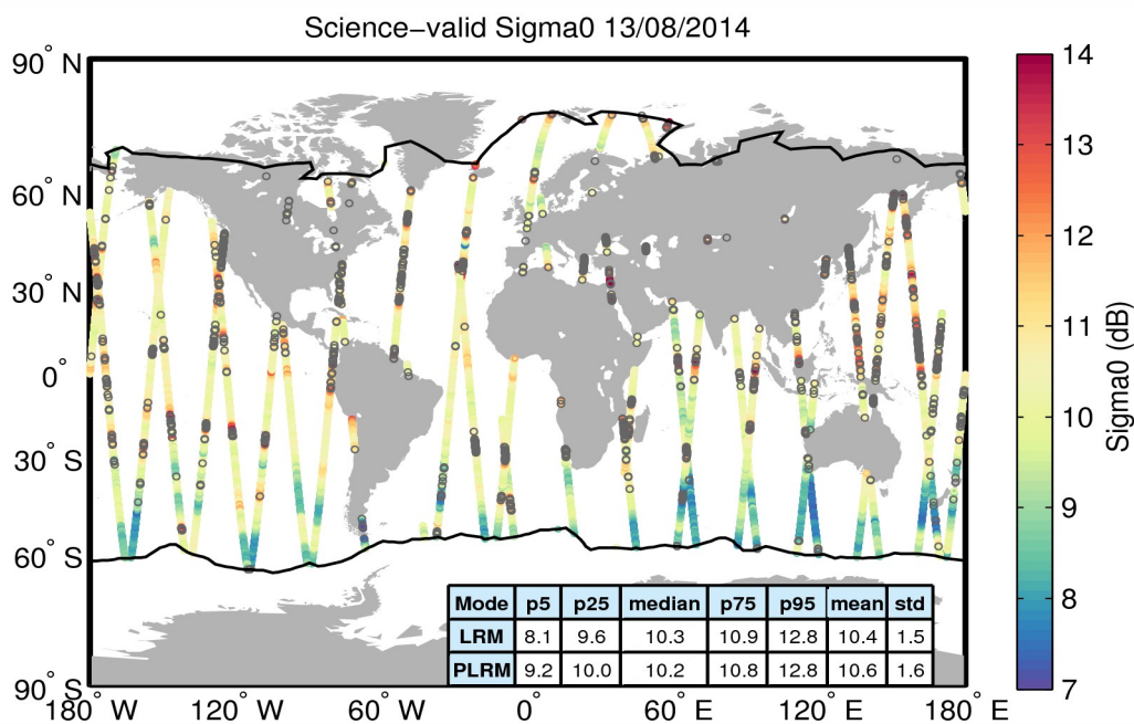
Figure 27. Geographical distribution of science-valid sigma0 data over oceans and lakes for 13/08/2014. The statistical values shown in the table refer to the sigma0 in dB and are calculated separately for LRM and PLRM regions. The black lines mark the outer limit of the Arctic and Antarctic polar polygons. Gray circles denote records that have been rejected based on the editing criteria described in Table 4.
