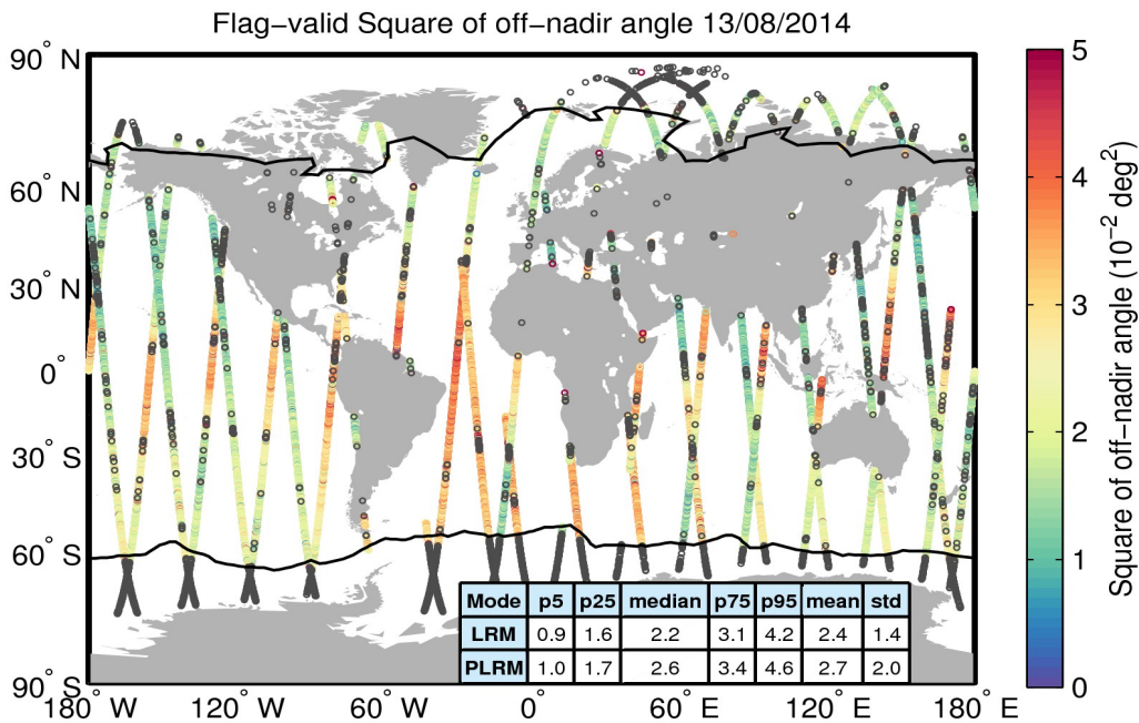
Figure 37. Geographical distribution of flag-valid mispointing data over oceans and lakes for 13/08/2014. The statistical values shown in the table refer to the mispointing in 10^{-2} deg 2 and are calculated separately for LRM and PLRM regions. Measurements taken over polar polygons have been excluded from the computation of the statistical values. The black lines mark the outer limit of the Arctic and Antarctic polar polygons. Gray circles denote negative values.
