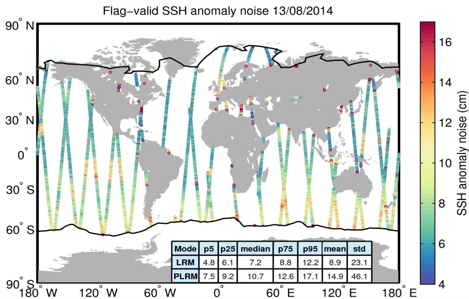
Figure 8. Geographical distribution of flag-valid 20-Hz SSH anomaly measurement noise over oceans and lakes for 13/08/2014. The statistical values shown in the table refer to the SSH anomaly noise and are calculated separately for LRM and PLRM regions. Measurements taken over polar polygons have been excluded from the computation of the statistical values. The black lines mark the outer limit of the Arctic and Antarctic polar polygons.
