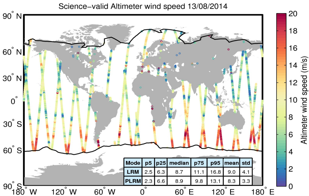
Figure 34. Geographical distribution of science-valid wind data over oceans and lakes for 13/08/2014. The statistical values shown in the table refer to the wind in m/s and are calculated separately for LRM and PLRM regions. The black lines mark the outer limit of the Arctic and Antarctic polar polygons. Gray circles denote records that have been rejected based on the editing criteria described in Table 5.
