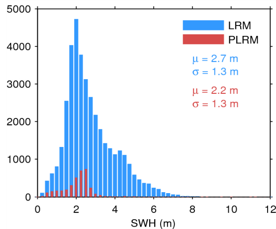
Figure 17. Histogram of flag-valid SWH over oceans and lakes for LRM (blue) and PLRM (red) for 13/08/2014. The mean ( \mu ) and standard deviation ( \sigma ) are also shown. Note that values larger than 12 m are excluded from the histogram for the sake of readability but not from the computation of \mu and \sigma .
