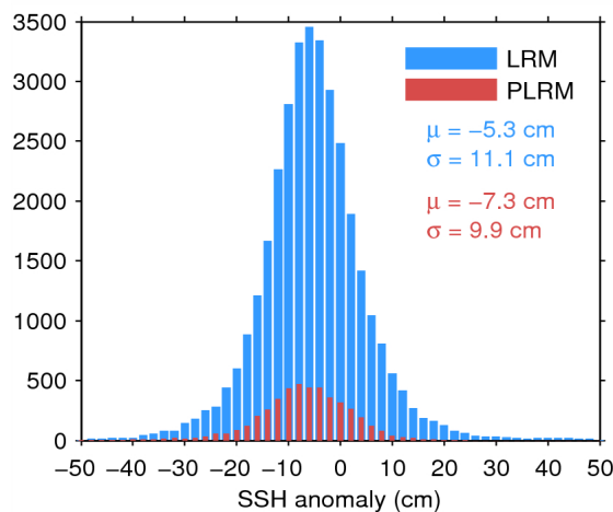
Figure 11. Histogram of science-valid SSH anomaly over oceans and lakes for LRM (blue) and PLRM (red) for 12/08/2014. The mean ( \mu ) and standard deviation ( \sigma ) are also shown. Note that values outside [-50 \ 50] cm are excluded from the histogram for the sake of readability but not from the computation of \mu and \sigma .
