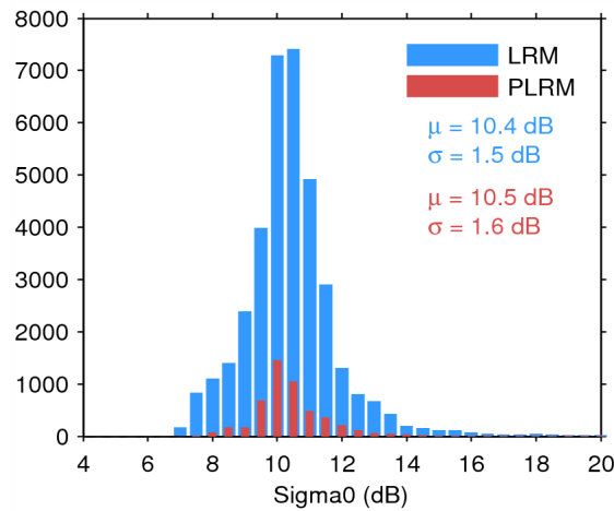
Figure 28. Histogram of science-valid sigma0 over oceans and lakes for LRM (blue) and PLRM (red) for 12/08/2014. The mean ( \mu ) and standard deviation ( \sigma ) are also shown. Note that values outside [4 20] dB are excluded from the histogram for the sake of readability but not from the computation of \mu and \sigma .
