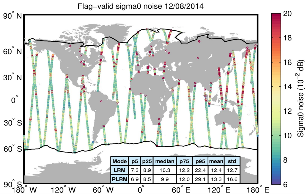
Figure 26. Geographical distribution of flag-valid 20-Hz sigma0 measurement noise over oceans and lakes for 12/08/2014. The statistical values shown in the table refer to the sigma0 noise and are calculated separately for LRM and PLRM regions. Measurements taken over polar polygons have been excluded from the computation of the statistical values. The black lines mark the outer limit of the Arctic and Antarctic polar polygons.
