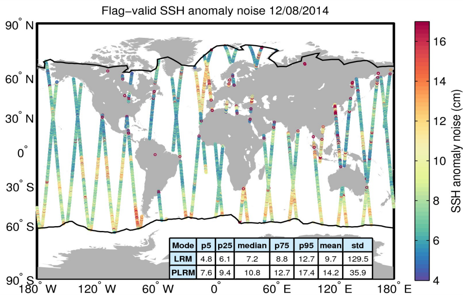
Figure 8. Geographical distribution of flag-valid 20-Hz SSH anomaly measurement noise over oceans and lakes for 12/08/2014. The statistical values shown in the table refer to the SSH anomaly noise and are calculated separately for LRM and PLRM regions. Measurements taken over polar polygons have been excluded from the computation of the statistical values. The black lines mark the outer limit of the Arctic and Antarctic polar polygons.
