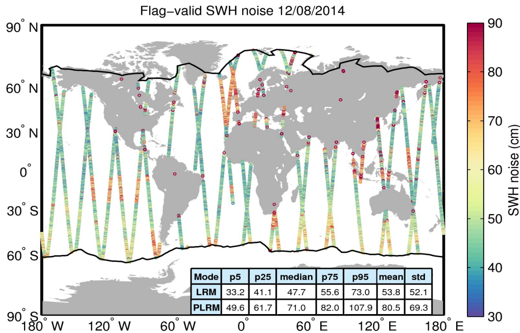
Figure 18. Geographical distribution of flag-valid 20-Hz SWH measurement noise over oceans and lakes for 12/08/2014. The statistical values shown in the table refer to the SWH noise and are calculated separately for LRM and PLRM regions. Measurements taken over polar polygons have been excluded from the computation of the statistical values. The black lines mark the outer limit of the Arctic and Antarctic polar polygons.
