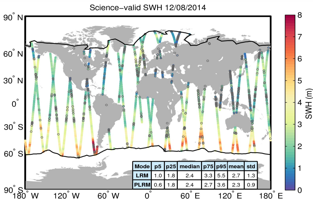
Figure 19. Geographical distribution of science-valid SWH data over oceans and lakes for 12/08/2014. The statistical values shown in the table refer to the SWH in m and are calculated separately for LRM and PLRM regions. The black lines mark the outer limit of the Arctic and Antarctic polar polygons. Gray circles denote records that have been rejected based on the editing criteria described in Table 3.
