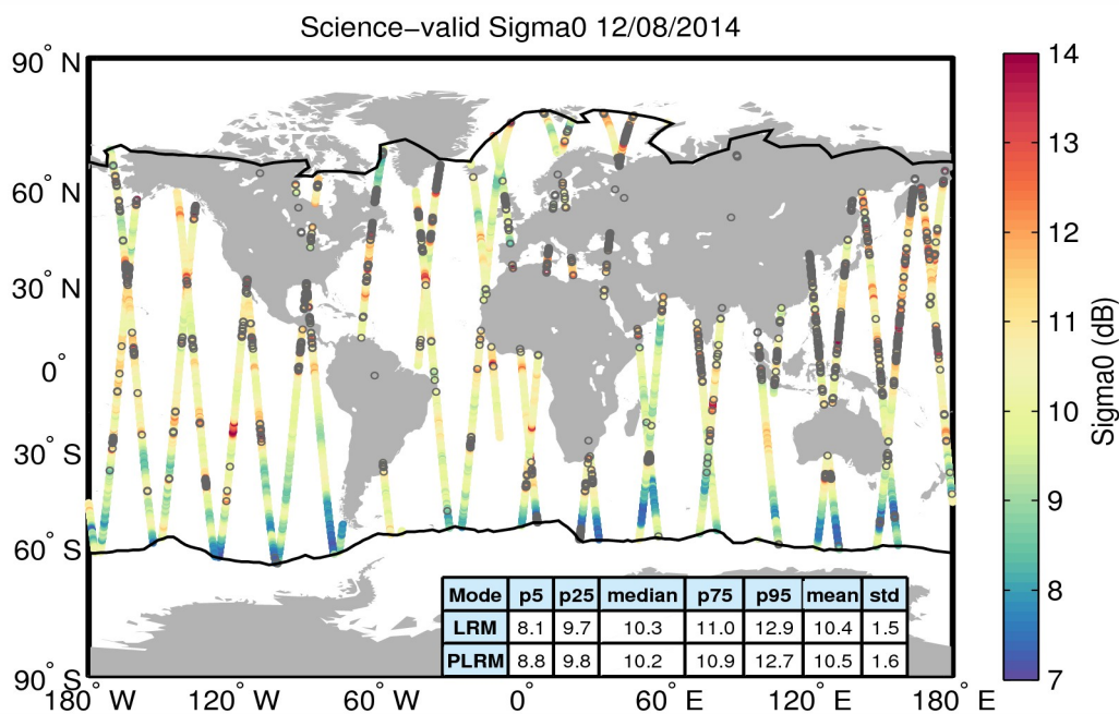
Figure 27. Geographical distribution of science-valid sigma0 data over oceans and lakes for 12/08/2014. The statistical values shown in the table refer to the sigma0 in dB and are calculated separately for LRM and PLRM regions. The black lines mark the outer limit of the Arctic and Antarctic polar polygons. Gray circles denote records that have been rejected based on the editing criteria described in Table 4.
