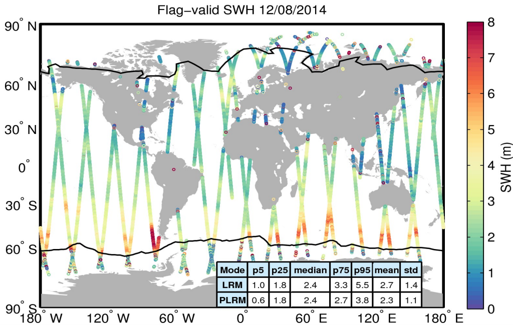
Figure 15. Geographical distribution of flag-valid SWH data over oceans and lakes for 12/08/2014. The statistical values shown in the table refer to the SWH in m and are calculated separately for LRM and PLRM regions. Measurements taken over polar polygons have been excluded from the computation of the statistical values. The black lines mark the outer limit of the Arctic and Antarctic polar polygons.
