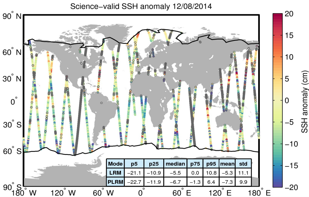
Figure 10. Geographical distribution of science-valid SSH anomaly data over oceans and lakes for 12/08/2014. The statistical values shown in the table refer to the SSH anomaly in cm and are calculated separately for LRM and PLRM regions. The black lines mark the outer limit of the Arctic and Antarctic polar polygons. Gray circles denote records that have been rejected based on the editing criteria described in Table 2.
