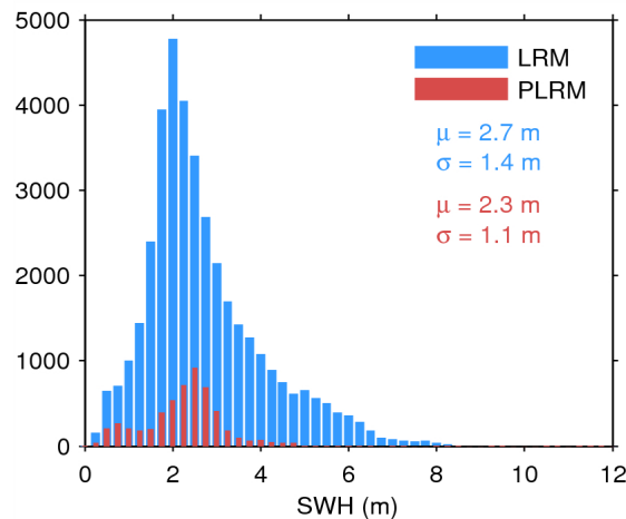
Figure 17. Histogram of flag-valid SWH over oceans and lakes for LRM (blue) and PLRM (red) for 12/08/2014. The mean ( \mu ) and standard deviation ( \sigma ) are also shown. Note that values larger than 12 m are excluded from the histogram for the sake of readability but not from the computation of \mu and \sigma .
