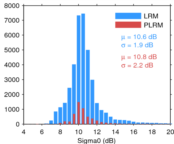
Figure 25. Histogram of flag-valid sigma0 over oceans and lakes for LRM (blue) and PLRM (red) for 12/08/2014. The mean ( \mu ) and standard deviation ( \sigma ) are also shown. Note that values outside [4 20] dB are excluded from the histogram for the sake of readability but not from the computation of \mu and \sigma .
