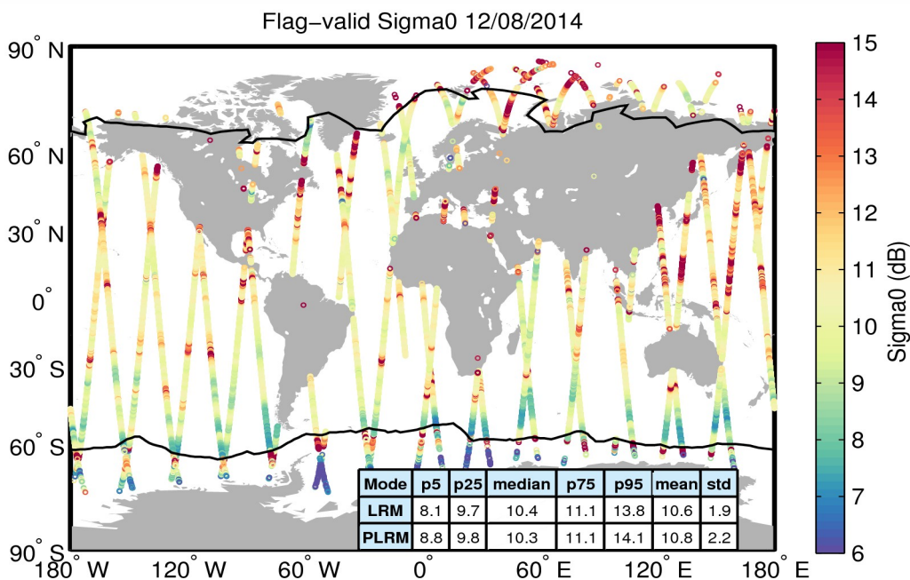
Figure 23. Geographical distribution of flag-valid sigma0 data over oceans and lakes for 12/08/2014. The statistical values shown in the table refer to the sigma0 in dB and are calculated separately for LRM and PLRM regions. Measurements taken over polar polygons have been excluded from the computation of the statistical values. The black lines mark the outer limit of the Arctic and Antarctic polar polygons.
