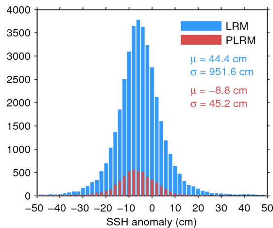
Figure 7. Histogram of flag-valid SSH anomaly over oceans and lakes for LRM (blue) and PLRM (red) for 12/08/2014. The mean ( \mu ) and standard deviation ( \sigma ) are also shown. Note that values outside [-50\ 50] cm are excluded from the histogram for the sake of readability but not from the computation of \mu and \sigma .
