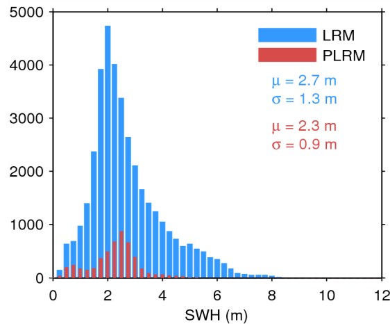
Figure 20. Histogram of science-valid SWH over oceans and lakes for LRM (blue) and PLRM (red) for 12/08/2014. The mean ( \mu ) and standard deviation ( \sigma ) are also shown. Note that values larger than 12 m are excluded from the histogram for the sake of readability but not from the computation of \mu and \sigma .
