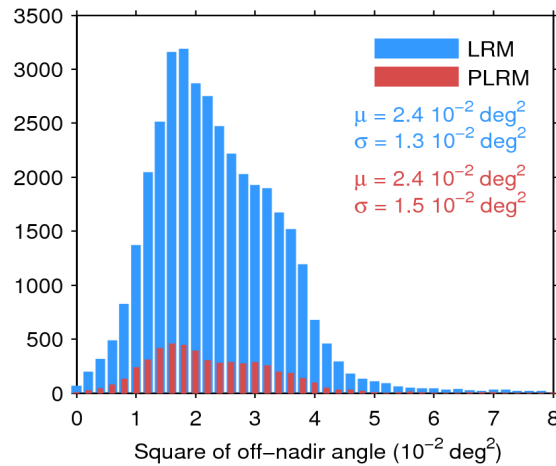
Figure 39. Histogram of flag-valid mispointing over oceans and lakes for LRM (blue) and PLRM (red) for 12/08/2014. Only positive values have been considered. The mean ( \mu ) and standard deviation ( \sigma ) are also shown. Note that values larger than 8 \cdot 10^{-2} \text{ deg}^2 are excluded from the histogram for the sake of readability but not from the computation of \mu and \sigma .
