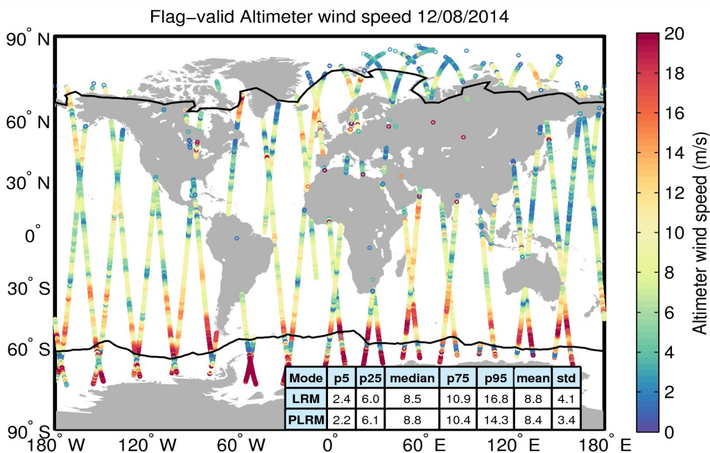
Figure 31. Geographical distribution of flag-valid wind data over oceans and lakes for 12/08/2014. The statistical values shown in the table refer to the wind in m/s and are calculated separately for LRM and PLRM regions. Measurements taken over polar polygons have been excluded from the computation of the statistical values. The black lines mark the outer limit of the Arctic and Antarctic polar polygons.
