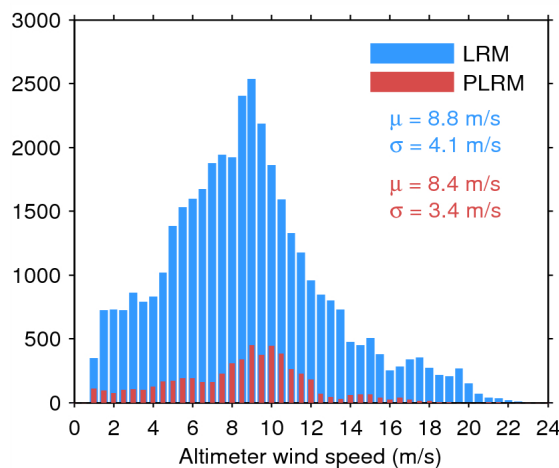
Figure 35. Histogram of science-valid wind over oceans and lakes for LRM (blue) and PLRM (red) for 12/08/2014. The mean ( \mu ) and standard deviation ( \sigma ) are also shown. Note that values larger than 24 m/s are excluded from the histogram for the sake of readability but not from the computation of \mu and \sigma .
