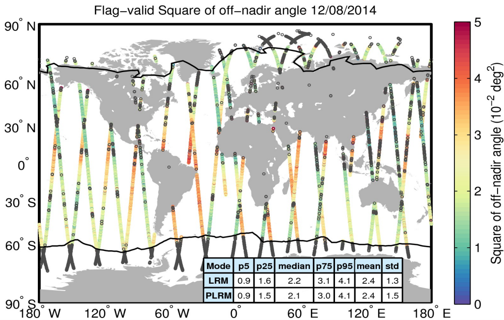
Figure 37. Geographical distribution of flag-valid mispointing data over oceans and lakes for 12/08/2014. The statistical values shown in the table refer to the mispointing in 10^{-2} \text{ deg}^2 and are calculated separately for LRM and PLRM regions. Measurements taken over polar polygons have been excluded from the computation of the statistical values. The black lines mark the outer limit of the Arctic and Antarctic polar polygons. Gray circles denote negative values.
