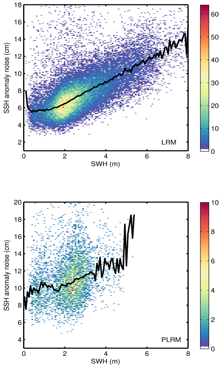
Figure 9. 2D histogram showing flag-valid SSH anomaly noise as a function of SWH for LRM (top) and PLRM (bottom) for 12/08/2014. The black line denotes the median SSH anomaly as a function of SWH.
