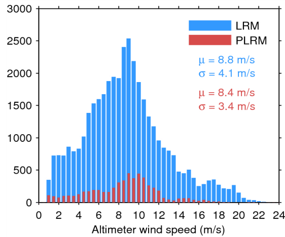
Figure 33. Histogram of flag-valid wind over oceans and lakes for LRM (blue) and PLRM (red) for 12/08/2014. The mean ( \mu ) and standard deviation ( \sigma ) are also shown. Note that values larger than 24 m/s are excluded from the histogram for the sake of readability but not from the computation of \mu and \sigma .
