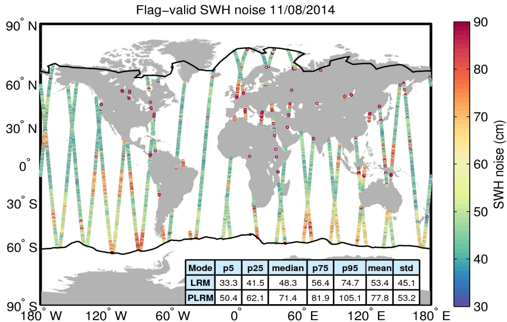
Figure 18. Geographical distribution of flag-valid 20-Hz SWH measurement noise over oceans and lakes for 11/08/2014. The statistical values shown in the table refer to the SWH noise and are calculated separately for LRM and PLRM regions. Measurements taken over polar polygons have been excluded from the computation of the statistical values. The black lines mark the outer limit of the Arctic and Antarctic polar polygons.
