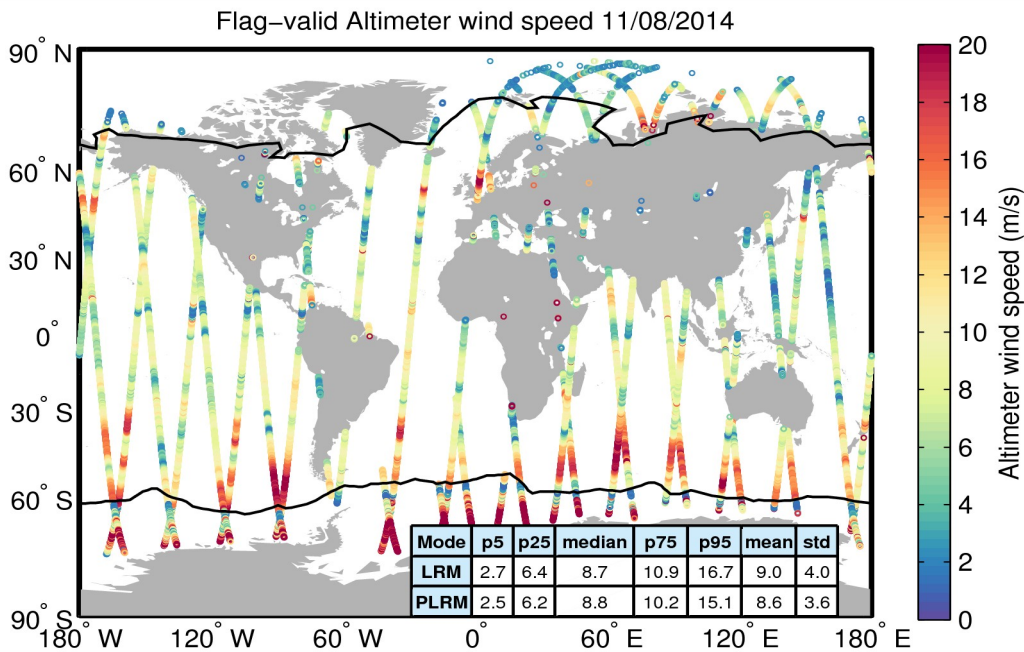
Figure 31. Geographical distribution of flag-valid wind data over oceans and lakes for 11/08/2014. The statistical values shown in the table refer to the wind in m/s and are calculated separately for LRM and PLRM regions. Measurements taken over polar polygons have been excluded from the computation of the statistical values. The black lines mark the outer limit of the Arctic and Antarctic polar polygons.
