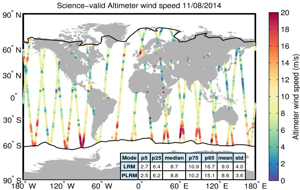
Figure 34. Geographical distribution of science-valid wind data over oceans and lakes for 11/08/2014. The statistical values shown in the table refer to the wind in m/s and are calculated separately for LRM and PLRM regions. The black lines mark the outer limit of the Arctic and Antarctic polar polygons. Gray circles denote records that have been rejected based on the editing criteria described in Table 5.
