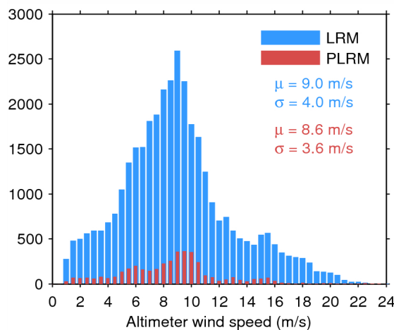
Figure 35. Histogram of science-valid wind over oceans and lakes for LRM (blue) and PLRM (red) for 11/08/2014. The mean ( \mu ) and standard deviation ( \sigma ) are also shown. Note that values larger than 24 m/s are excluded from the histogram for the sake of readability but not from the computation of \mu and \sigma .
