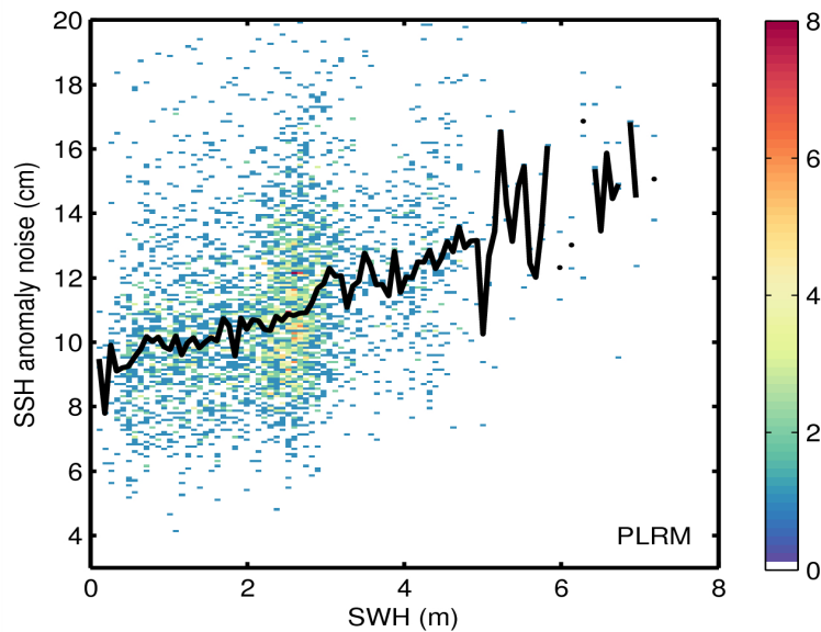
Figure 9. 2D histogram showing flag-valid SSH anomaly noise as a function of SWH for LRM (top) and PLRM (bottom) for 11/08/2014. The black line denotes the median SSH anomaly as a function of SWH.
