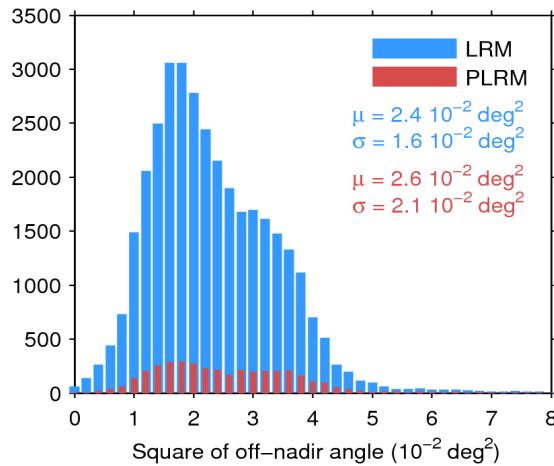
Figure 39. Histogram of flag-valid mispointing over oceans and lakes for LRM (blue) and PLRM (red) for 11/08/2014. Only positive values have been considered. The mean ( \mu ) and standard deviation ( \sigma ) are also shown. Note that values 8 \cdot 10^{-2} \text{ deg}^2 are excluded from the histogram for the sake of readability but not from the computation of \mu and \sigma .
