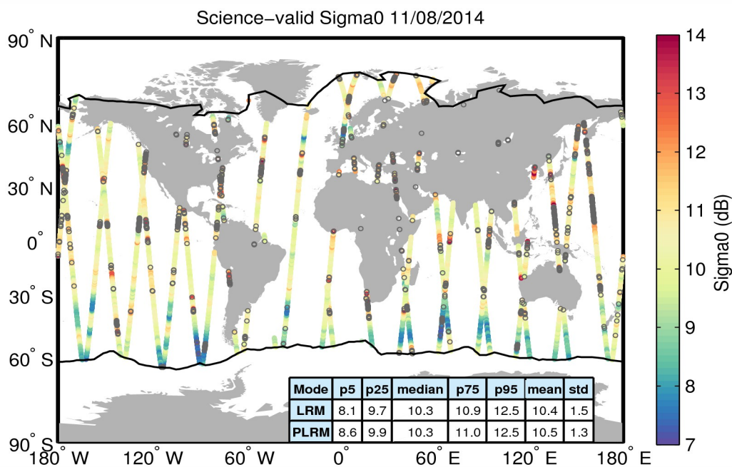
Figure 27. Geographical distribution of science-valid sigma0 data over oceans and lakes for 11/08/2014. The statistical values shown in the table refer to the sigma0 in dB and are calculated separately for LRM and PLRM regions. The black lines mark the outer limit of the Arctic and Antarctic polar polygons. Gray circles denote records that have been rejected based on the editing criteria described in Table 4.
