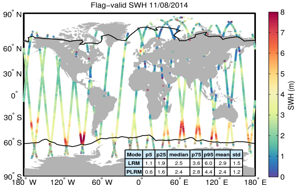
Figure 15. Geographical distribution of flag-valid SWH data over oceans and lakes for 11/08/2014. The statistical values shown in the table refer to the SWH in m and are calculated separately for LRM and PLRM regions. Measurements taken over polar polygons have been excluded from the computation of the statistical values. The black lines mark the outer limit of the Arctic and Antarctic polar polygons.
