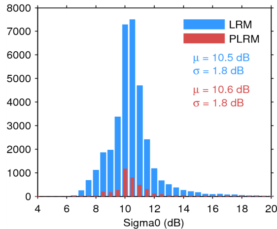
Figure 25. Histogram of flag-valid sigma0 over oceans and lakes for LRM (blue) and PLRM (red) for 11/08/2014. The mean ( \mu ) and standard deviation ( \sigma ) are also shown. Note that values outside [4 20] dB are excluded from the histogram for the sake of readability but not from the computation of \mu and \sigma .
