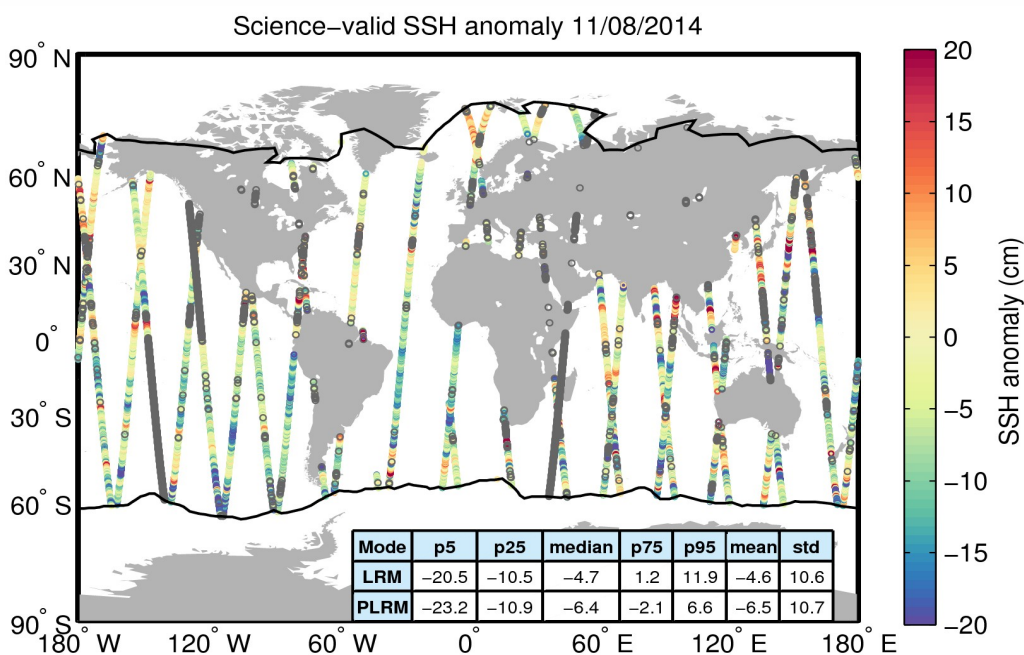
Figure 10. Geographical distribution of science-valid SSH anomaly data over oceans and lakes for 11/08/2014. The statistical values shown in the table refer to the SSH anomaly in cm and are calculated separately for LRM and PLRM regions. The black lines mark the outer limit of the Arctic and Antarctic polar polygons. Gray circles denote records that have been rejected based on the editing criteria described in Table 2.
