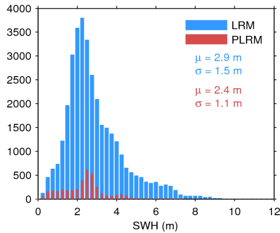
Figure 20. Histogram of science-valid SWH over oceans and lakes for LRM (blue) and PLRM (red) for 11/08/2014. The mean ( \mu ) and standard deviation ( \sigma ) are also shown. Note that values larger than 12 m are excluded from the histogram for the sake of readability but not from the computation of \mu and \sigma .
