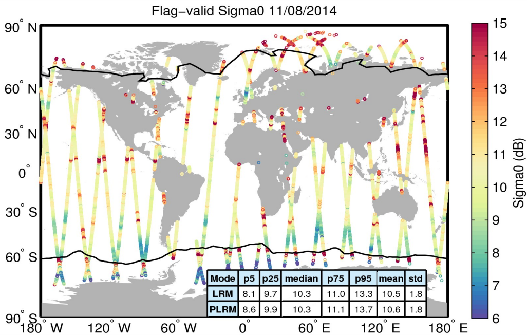
Figure 23. Geographical distribution of flag-valid sigma0 data over oceans and lakes for 11/08/2014. The statistical values shown in the table refer to the sigma0 in dB and are calculated separately for LRM and PLRM regions. Measurements taken over polar polygons have been excluded from the computation of the statistical values. The black lines mark the outer limit of the Arctic and Antarctic polar polygons.
