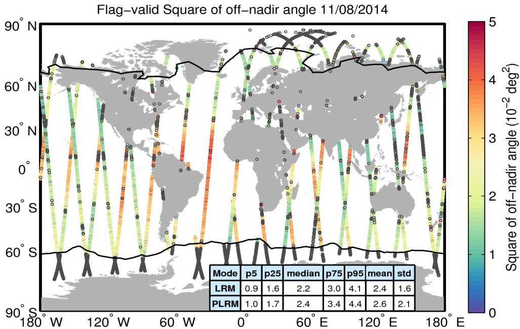
Figure 37. Geographical distribution of flag-valid mispointing data over oceans and lakes for 11/08/2014. The statistical values shown in the table refer to the mispointing in 10^{-2} \text{ deg}^2 and are calculated separately for LRM and PLRM regions. Measurements taken over polar polygons have been excluded from the computation of the statistical values. The black lines mark the outer limit of the Arctic and Antarctic polar polygons. Gray circles denote negative values.
