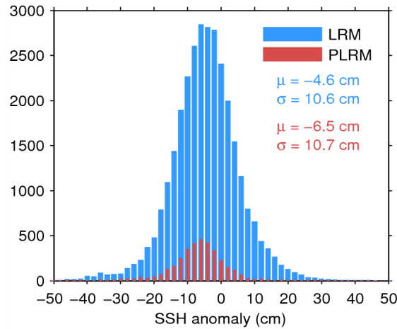
Figure 11. Histogram of science-valid SSH anomaly over oceans and lakes for LRM (blue) and PLRM (red) for 11/08/2014. The mean ( \mu ) and standard deviation ( \sigma ) are also shown. Note that values outside [-50\ 50] cm are excluded from the histogram for the sake of readability but not from the computation of \mu and \sigma .
