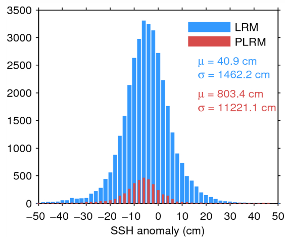
Figure 7. Histogram of flag-valid SSH anomaly over oceans and lakes for LRM (blue) and PLRM (red) for 11/08/2014. The mean ( \mu ) and standard deviation ( \sigma ) are also shown. Note that values outside [-50\ 50] cm are excluded from the histogram for the sake of readability but not from the computation of \mu and \sigma .
