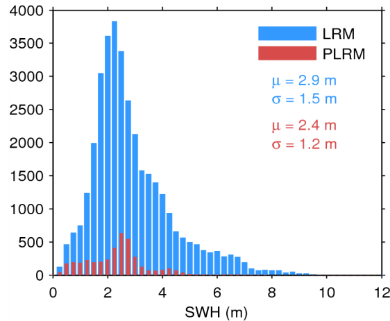
Figure 17. Histogram of flag-valid SWH over oceans and lakes for LRM (blue) and PLRM (red) for 11/08/2014. The mean ( \mu ) and standard deviation ( \sigma ) are also shown. Note that values larger than 12 m are excluded from the histogram for the sake of readability but not from the computation of \mu and \sigma .
