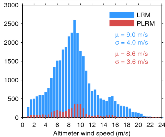
Figure 33. Histogram of flag-valid wind over oceans and lakes for LRM (blue) and PLRM (red) for 11/08/2014. The mean ( \mu ) and standard deviation ( \sigma ) are also shown. Note that values larger than 24 m/s are excluded from the histogram for the sake of readability but not from the computation of \mu and \sigma .
