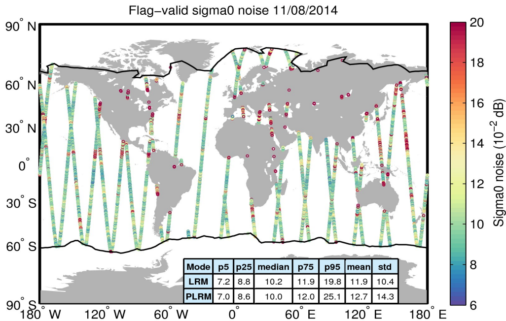
Figure 26. Geographical distribution of flag-valid 20-Hz sigma0 measurement noise over oceans and lakes for 11/08/2014. The statistical values shown in the table refer to the sigma0 noise and are calculated separately for LRM and PLRM regions. Measurements taken over polar polygons have been excluded from the computation of the statistical values. The black lines mark the outer limit of the Arctic and Antarctic polar polygons.
