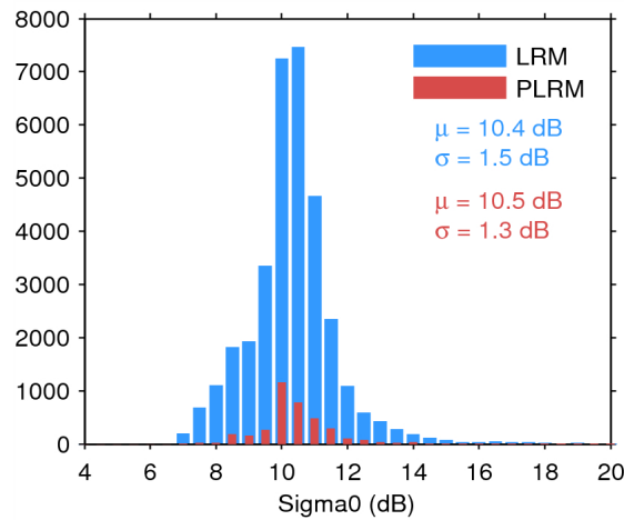
Figure 28. Histogram of science-valid sigma0 over oceans and lakes for LRM (blue) and PLRM (red) for 11/08/2014. The mean ( \mu ) and standard deviation ( \sigma ) are also shown. Note that values outside [4 20] dB are excluded from the histogram for the sake of readability but not from the computation of \mu and \sigma .
