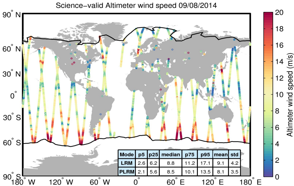
Figure 34. Geographical distribution of science-valid wind data over oceans and lakes for 09/08/2014. The statistical values shown in the table refer to the wind in m/s and are calculated separately for LRM and PLRM regions. The black lines mark the outer limit of the Arctic and Antarctic polar polygons. Gray circles denote records that have been rejected based on the editing criteria described in Table 5.
