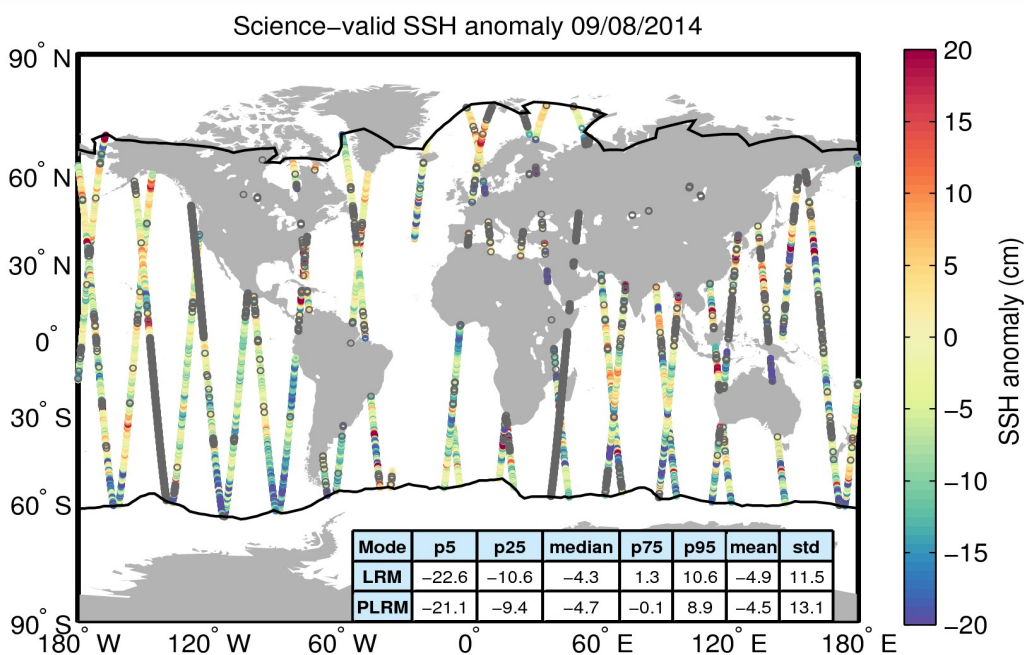
Figure 10. Geographical distribution of science-valid SSH anomaly data over oceans and lakes for 09/08/2014. The statistical values shown in the table refer to the SSH anomaly in cm and are calculated separately for LRM and PLRM regions. The black lines mark the outer limit of the Arctic and Antarctic polar polygons. Gray circles denote records that have been rejected based on the editing criteria described in Table 2.
