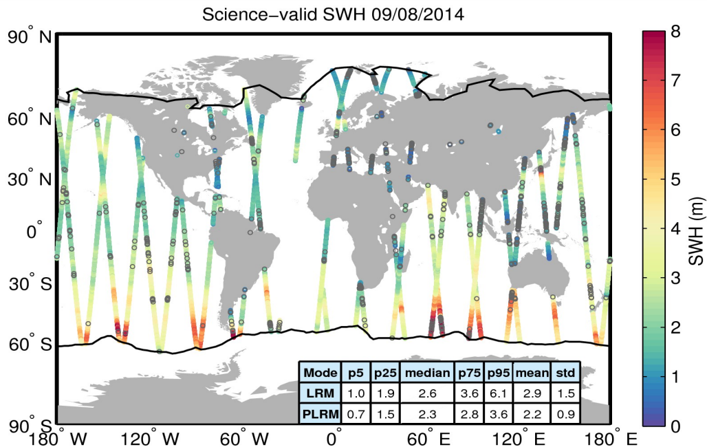
Figure 19. Geographical distribution of science-valid SWH data over oceans and lakes for 09/08/2014. The statistical values shown in the table refer to the SWH in m and are calculated separately for LRM and PLRM regions. The black lines mark the outer limit of the Arctic and Antarctic polar polygons. Gray circles denote records that have been rejected based on the editing criteria described in Table 3.
