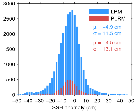
Figure 11. Histogram of science-valid SSH anomaly over oceans and lakes for LRM (blue) and PLRM (red) for 09/08/2014. The mean ( \mu ) and standard deviation ( \sigma ) are also shown. Note that values outside [-50\ 50] cm are excluded from the histogram for the sake of readability but not from the computation of \mu and \sigma .
