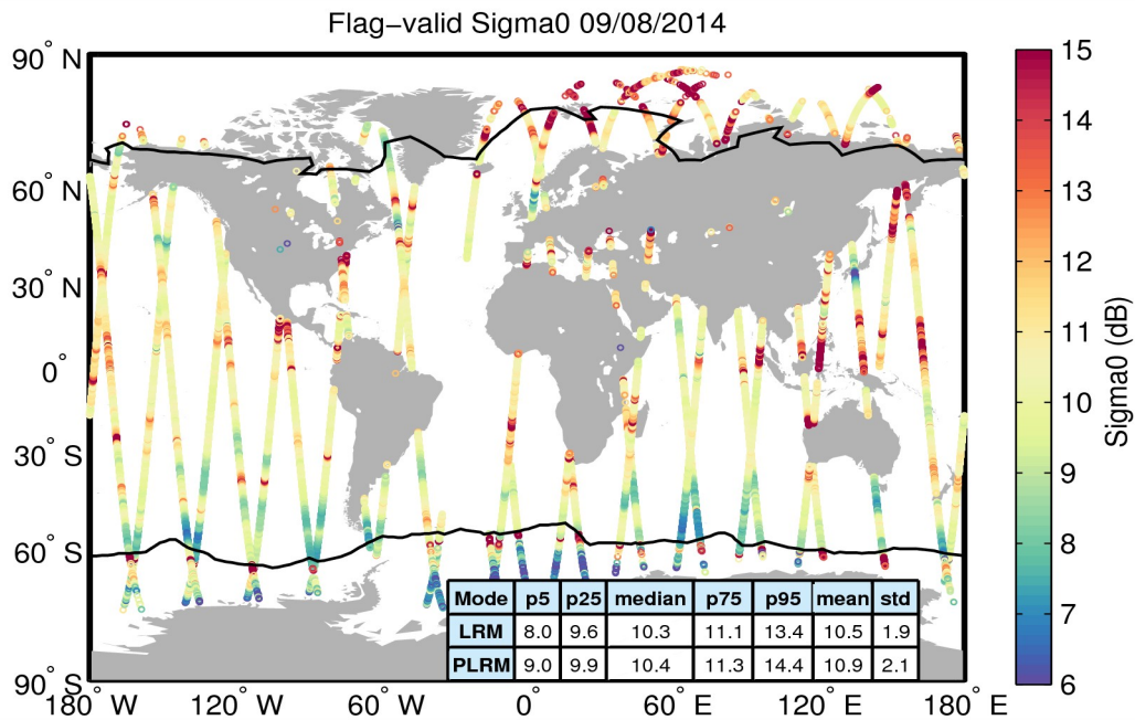
Figure 23. Geographical distribution of flag-valid sigma0 data over oceans and lakes for 09/08/2014. The statistical values shown in the table refer to the sigma0 in dB and are calculated separately for LRM and PLRM regions. Measurements taken over polar polygons have been excluded from the computation of the statistical values. The black lines mark the outer limit of the Arctic and Antarctic polar polygons.
