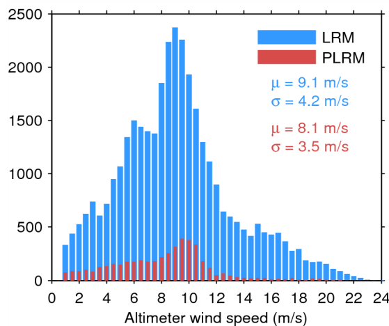
Figure 35. Histogram of science-valid wind over oceans and lakes for LRM (blue) and PLRM (red) for 09/08/2014. The mean ( \mu ) and standard deviation ( \sigma ) are also shown. Note that values larger than 24 m/s are excluded from the histogram for the sake of readability but not from the computation of \mu and \sigma .
