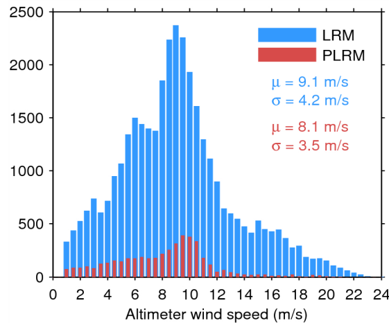
Figure 33. Histogram of flag-valid wind over oceans and lakes for LRM (blue) and PLRM (red) for 09/08/2014. The mean ( \mu ) and standard deviation ( \sigma ) are also shown. Note that values larger than 24 m/s are excluded from the histogram for the sake of readability but not from the computation of \mu and \sigma .
