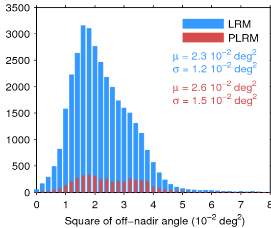
Figure 39. Histogram of flag-valid mispointing over oceans and lakes for LRM (blue) and PLRM (red) for 09/08/2014. Only positive values have been considered. The mean ( \mu ) and standard deviation ( \sigma ) are also shown. Note that values 8 \cdot 10^{-2} \text{ deg}^2 are excluded from the histogram for the sake of readability but not from the computation of \mu and \sigma .
