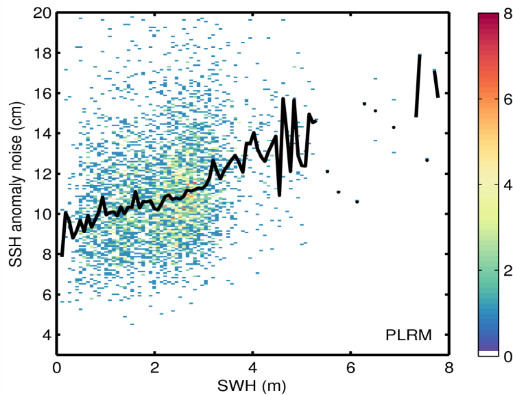
Figure 9. 2D histogram showing flag-valid SSH anomaly noise as a function of SWH for LRM (top) and PLRM (bottom) for 09/08/2014. The black line denotes the median SSH anomaly as a function of SWH.
