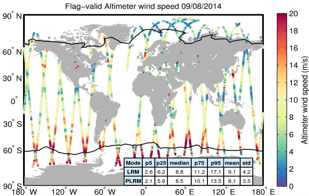
Figure 31. Geographical distribution of flag-valid wind data over oceans and lakes for 09/08/2014. The statistical values shown in the table refer to the wind in m/s and are calculated separately for LRM and PLRM regions. Measurements taken over polar polygons have been excluded from the computation of the statistical values. The black lines mark the outer limit of the Arctic and Antarctic polar polygons.
