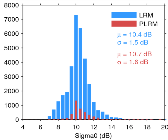
Figure 28. Histogram of science-valid sigma0 over oceans and lakes for LRM (blue) and PLRM (red) for 09/08/2014. The mean ( \mu ) and standard deviation ( \sigma ) are also shown. Note that values outside [4 20] dB are excluded from the histogram for the sake of readability but not from the computation of \mu and \sigma .
