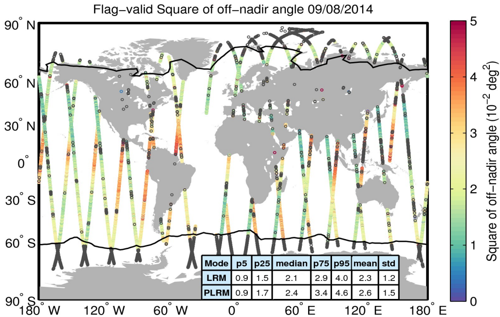
Figure 37. Geographical distribution of flag-valid mispointing data over oceans and lakes for 09/08/2014. The statistical values shown in the table refer to the mispointing in 10^{-2} \text{ deg}^2 and are calculated separately for LRM and PLRM regions. Measurements taken over polar polygons have been excluded from the computation of the statistical values. The black lines mark the outer limit of the Arctic and Antarctic polar polygons. Gray circles denote negative values.
