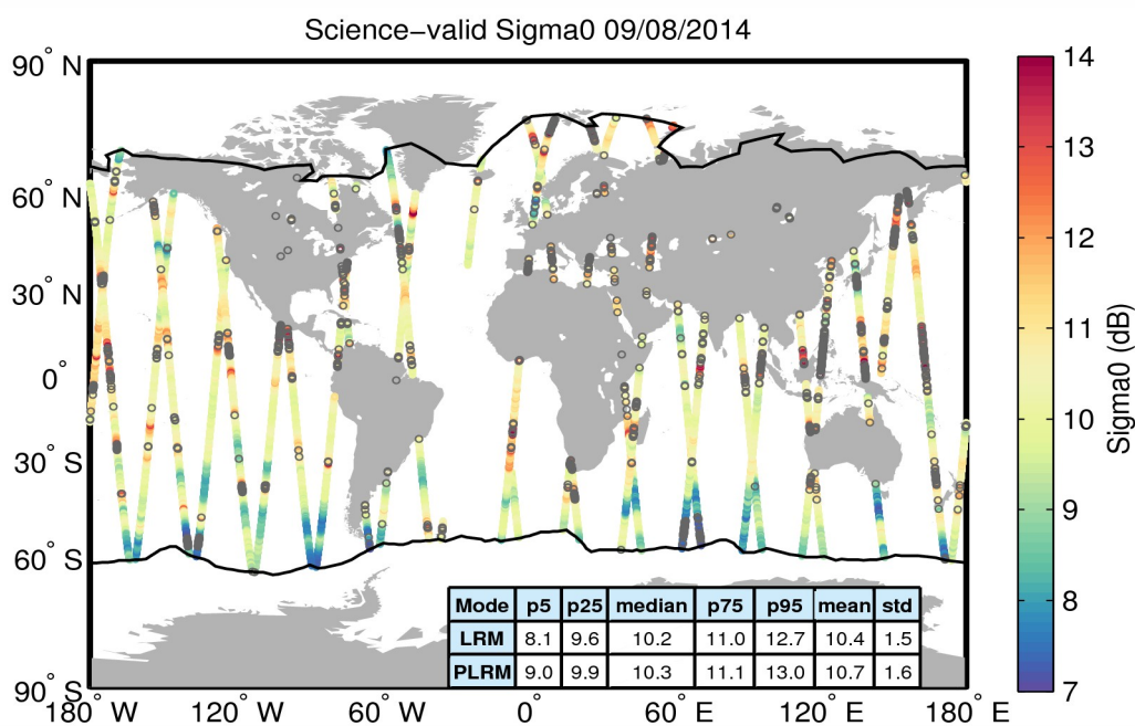
Figure 27. Geographical distribution of science-valid sigma0 data over oceans and lakes for 09/08/2014. The statistical values shown in the table refer to the sigma0 in dB and are calculated separately for LRM and PLRM regions. The black lines mark the outer limit of the Arctic and Antarctic polar polygons. Gray circles denote records that have been rejected based on the editing criteria described in Table 4.
