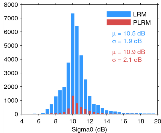
Figure 25. Histogram of flag-valid sigma0 over oceans and lakes for LRM (blue) and PLRM (red) for 09/08/2014. The mean ( \mu ) and standard deviation ( \sigma ) are also shown. Note that values outside [4 20] dB are excluded from the histogram for the sake of readability but not from the computation of \mu and \sigma .
