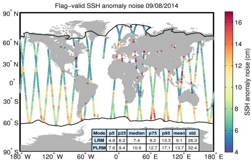
Figure 8. Geographical distribution of flag-valid 20-Hz SSH anomaly measurement noise over oceans and lakes for 09/08/2014. The statistical values shown in the table refer to the SSH anomaly noise and are calculated separately for LRM and PLRM regions. Measurements taken over polar polygons have been excluded from the computation of the statistical values. The black lines mark the outer limit of the Arctic and Antarctic polar polygons.
