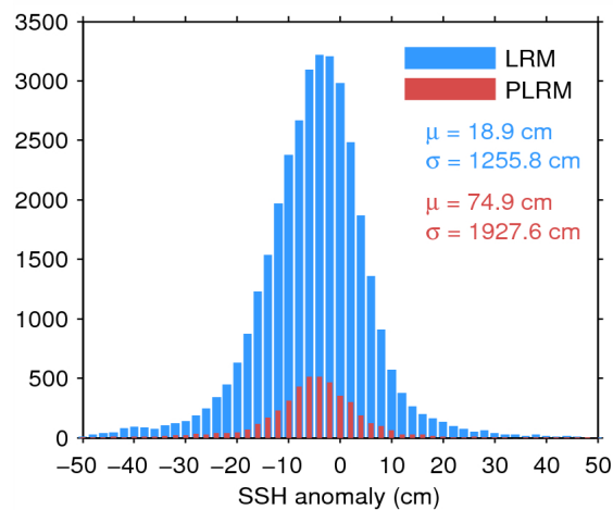
Figure 7. Histogram of flag-valid SSH anomaly over oceans and lakes for LRM (blue) and PLRM (red) for 09/08/2014. The mean ( \mu ) and standard deviation ( \sigma ) are also shown. Note that values outside [-50\ 50] cm are excluded from the histogram for the sake of readability but not from the computation of \mu and \sigma .
