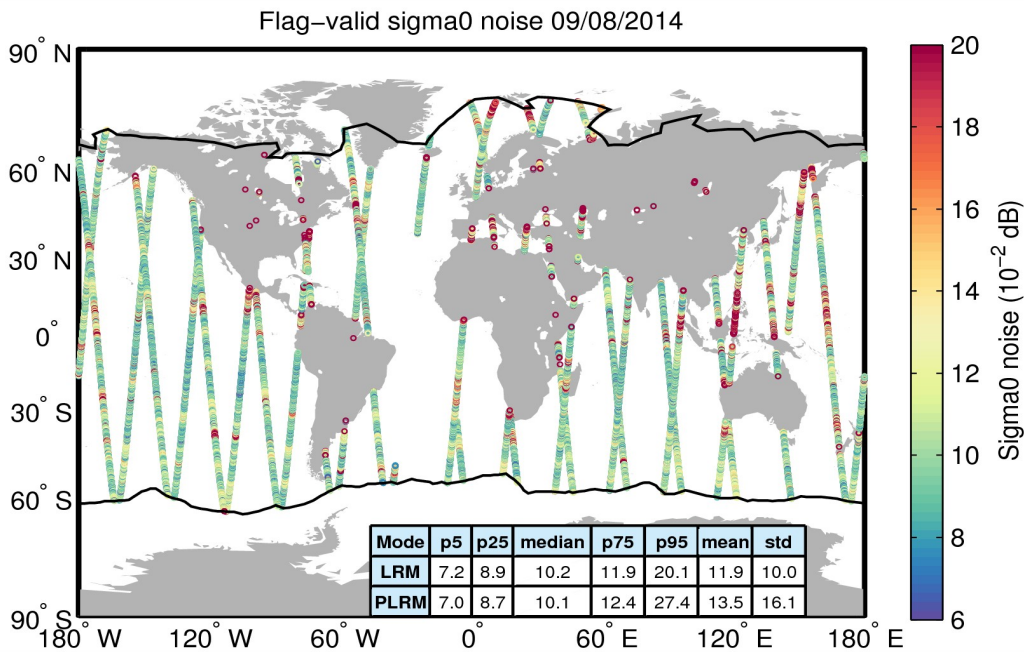
Figure 26. Geographical distribution of flag-valid 20-Hz sigma0 measurement noise over oceans and lakes for 09/08/2014. The statistical values shown in the table refer to the sigma0 noise and are calculated separately for LRM and PLRM regions. Measurements taken over polar polygons have been excluded from the computation of the statistical values. The black lines mark the outer limit of the Arctic and Antarctic polar polygons.
