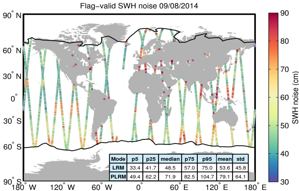
Figure 18. Geographical distribution of flag-valid 20-Hz SWH measurement noise over oceans and lakes for 09/08/2014. The statistical values shown in the table refer to the SWH noise and are calculated separately for LRM and PLRM regions. Measurements taken over polar polygons have been excluded from the computation of the statistical values. The black lines mark the outer limit of the Arctic and Antarctic polar polygons.
