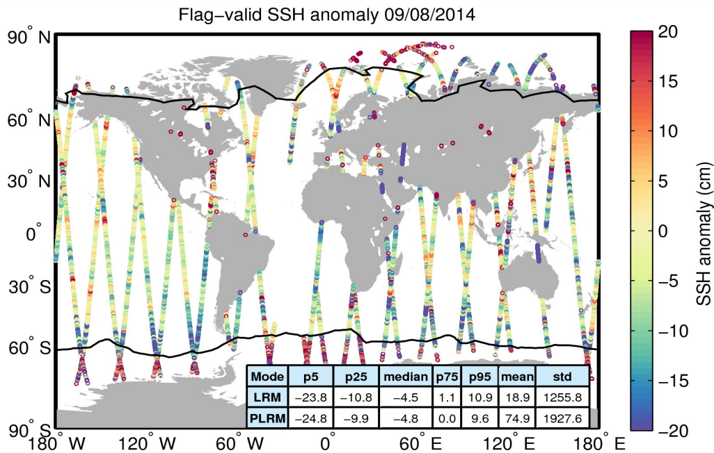
Figure 5. Geographical distribution of flag-valid 1-Hz SSH anomaly data over oceans and lakes for 09/08/2014. The statistical values shown in the table refer to the SSH anomaly in cm and are calculated separately for LRM and PLRM regions. Measurements taken over polar polygons have been excluded from the computation of the statistical values. The black lines mark the outer limit of the Arctic and Antarctic polar polygons.
