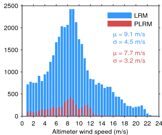
Figure 35. Histogram of science-valid wind over oceans and lakes for LRM (blue) and PLRM (red) for 08/08/2014. The mean ( \mu ) and standard deviation ( \sigma ) are also shown. Note that values larger than 24 m/s are excluded from the histogram for the sake of readability but not from the computation of \mu and \sigma .
