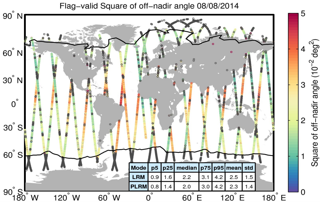
Figure 37. Geographical distribution of flag-valid mispointing data over oceans and lakes for 08/08/2014. The statistical values shown in the table refer to the mispointing in 10^{-2} deg 2 and are calculated separately for LRM and PLRM regions. Measurements taken over polar polygons have been excluded from the computation of the statistical values. The black lines mark the outer limit of the Arctic and Antarctic polar polygons. Gray circles denote negative values.
