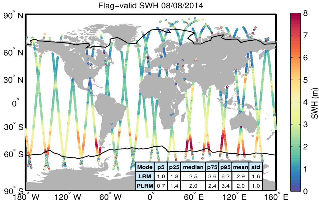
Figure 15. Geographical distribution of flag-valid SWH data over oceans and lakes for 08/08/2014. The statistical values shown in the table refer to the SWH in m and are calculated separately for LRM and PLRM regions. Measurements taken over polar polygons have been excluded from the computation of the statistical values. The black lines mark the outer limit of the Arctic and Antarctic polar polygons.
