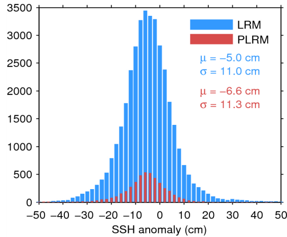
Figure 11. Histogram of science-valid SSH anomaly over oceans and lakes for LRM (blue) and PLRM (red) for 08/08/2014. The mean ( \mu ) and standard deviation ( \sigma ) are also shown. Note that values outside [-50\ 50] cm are excluded from the histogram for the sake of readability but not from the computation of \mu and \sigma .
