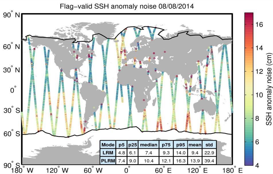
Figure 8. Geographical distribution of flag-valid 20-Hz SSH anomaly measurement noise over oceans and lakes for 08/08/2014. The statistical values shown in the table refer to the SSH anomaly noise and are calculated separately for LRM and PLRM regions. Measurements taken over polar polygons have been excluded from the computation of the statistical values. The black lines mark the outer limit of the Arctic and Antarctic polar polygons.
