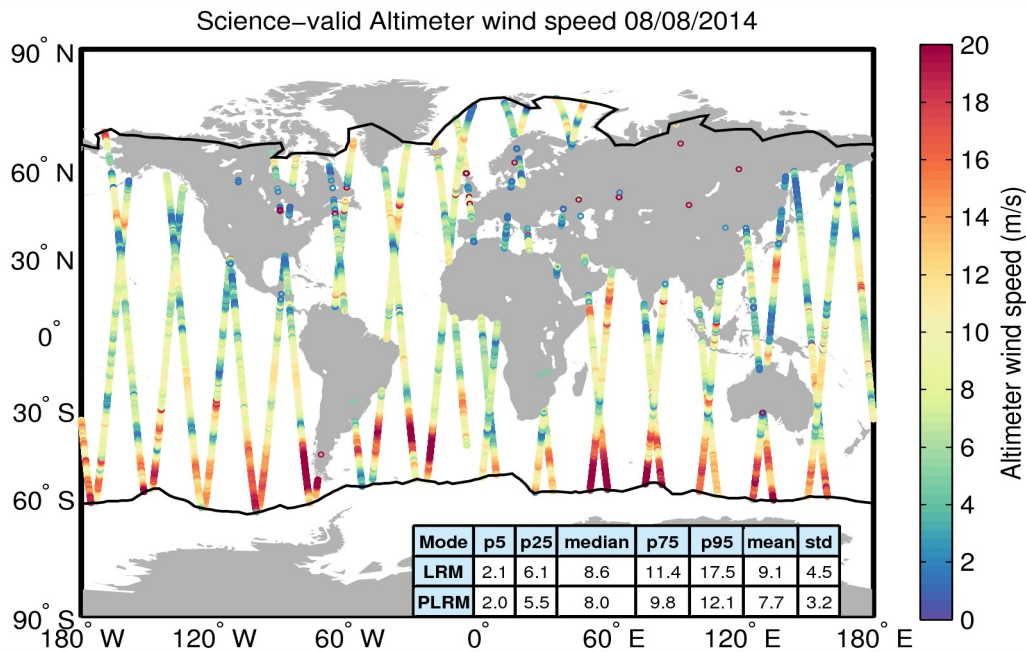
Figure 34. Geographical distribution of science-valid wind data over oceans and lakes for 08/08/2014. The statistical values shown in the table refer to the wind in m/s and are calculated separately for LRM and PLRM regions. The black lines mark the outer limit of the Arctic and Antarctic polar polygons. Gray circles denote records that have been rejected based on the editing criteria described in Table 5.
