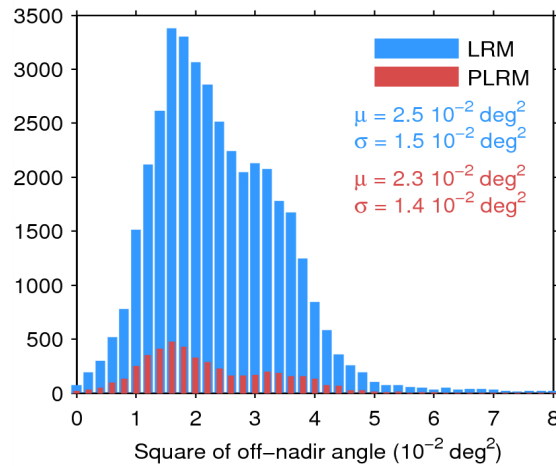
Figure 39. Histogram of flag-valid mispointing over oceans and lakes for LRM (blue) and PLRM (red) for 08/08/2014. Only positive values have been considered. The mean ( \mu ) and standard deviation ( \sigma ) are also shown. Note that values 8 \cdot 10^{-2} \text{ deg}^2 are excluded from the histogram for the sake of readability but not from the computation of \mu and \sigma .
