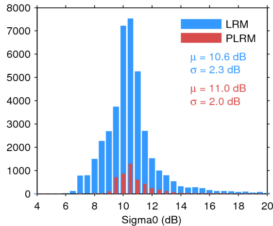
Figure 25. Histogram of flag-valid sigma0 over oceans and lakes for LRM (blue) and PLRM (red) for 08/08/2014. The mean ( \mu ) and standard deviation ( \sigma ) are also shown. Note that values outside [4 20] dB are excluded from the histogram for the sake of readability but not from the computation of \mu and \sigma .
