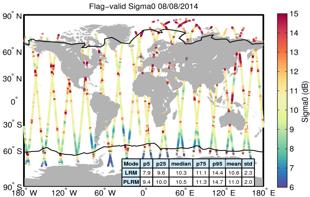
Figure 23. Geographical distribution of flag-valid sigma0 data over oceans and lakes for 08/08/2014. The statistical values shown in the table refer to the sigma0 in dB and are calculated separately for LRM and PLRM regions. Measurements taken over polar polygons have been excluded from the computation of the statistical values. The black lines mark the outer limit of the Arctic and Antarctic polar polygons.
