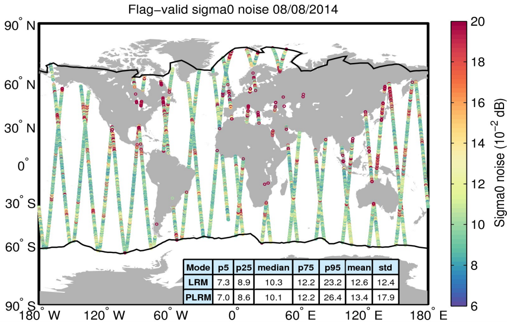
Figure 26. Geographical distribution of flag-valid 20-Hz sigma0 measurement noise over oceans and lakes for 08/08/2014. The statistical values shown in the table refer to the sigma0 noise and are calculated separately for LRM and PLRM regions. Measurements taken over polar polygons have been excluded from the computation of the statistical values. The black lines mark the outer limit of the Arctic and Antarctic polar polygons.
