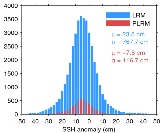
Figure 7. Histogram of flag-valid SSH anomaly over oceans and lakes for LRM (blue) and PLRM (red) for 08/08/2014. The mean ( \mu ) and standard deviation ( \sigma ) are also shown. Note that values outside [-50\ 50] cm are excluded from the histogram for the sake of readability but not from the computation of \mu and \sigma .
