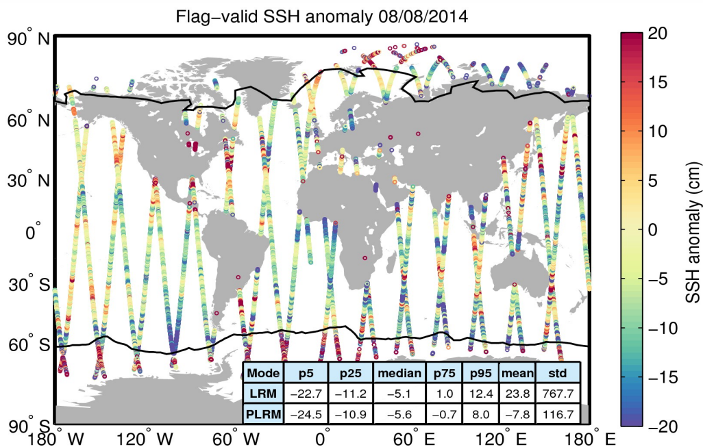
Figure 5. Geographical distribution of flag-valid 1-Hz SSH anomaly data over oceans and lakes for 08/08/2014. The statistical values shown in the table refer to the SSH anomaly in cm and are calculated separately for LRM and PLRM regions. Measurements taken over polar polygons have been excluded from the computation of the statistical values. The black lines mark the outer limit of the Arctic and Antarctic polar polygons.
