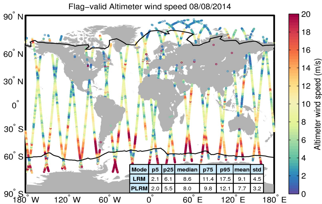
Figure 31. Geographical distribution of flag-valid wind data over oceans and lakes for 08/08/2014. The statistical values shown in the table refer to the wind in m/s and are calculated separately for LRM and PLRM regions. Measurements taken over polar polygons have been excluded from the computation of the statistical values. The black lines mark the outer limit of the Arctic and Antarctic polar polygons.
