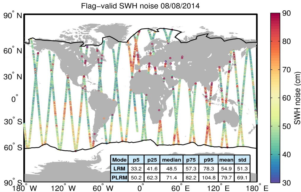
Figure 18. Geographical distribution of flag-valid 20-Hz SWH measurement noise over oceans and lakes for 08/08/2014. The statistical values shown in the table refer to the SWH noise and are calculated separately for LRM and PLRM regions. Measurements taken over polar polygons have been excluded from the computation of the statistical values. The black lines mark the outer limit of the Arctic and Antarctic polar polygons.
