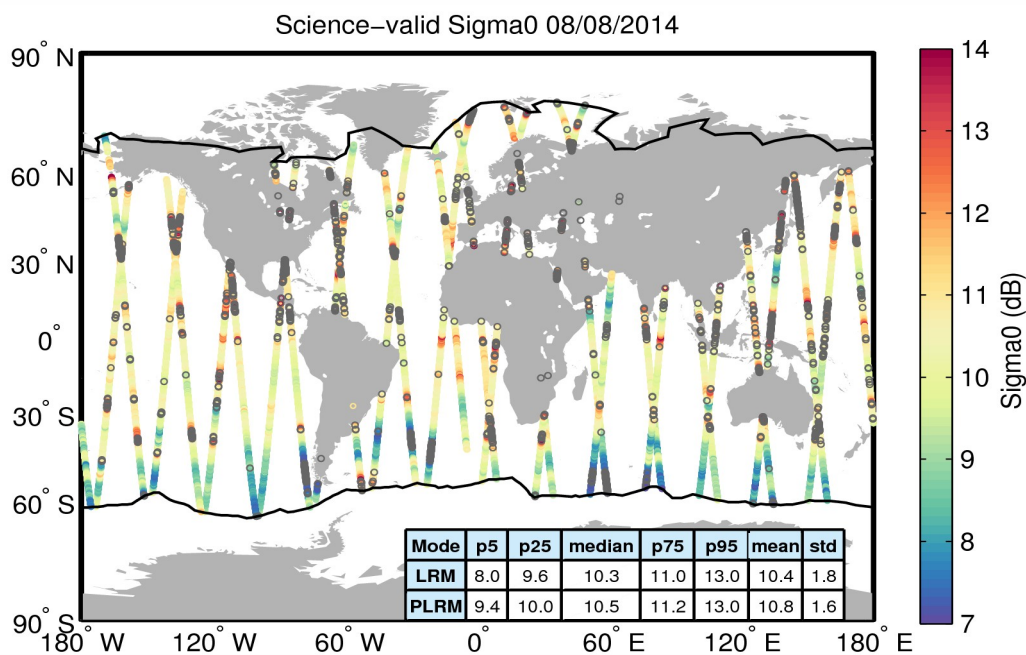
Figure 27. Geographical distribution of science-valid sigma0 data over oceans and lakes for 08/08/2014. The statistical values shown in the table refer to the sigma0 in dB and are calculated separately for LRM and PLRM regions. The black lines mark the outer limit of the Arctic and Antarctic polar polygons. Gray circles denote records that have been rejected based on the editing criteria described in Table 4.
