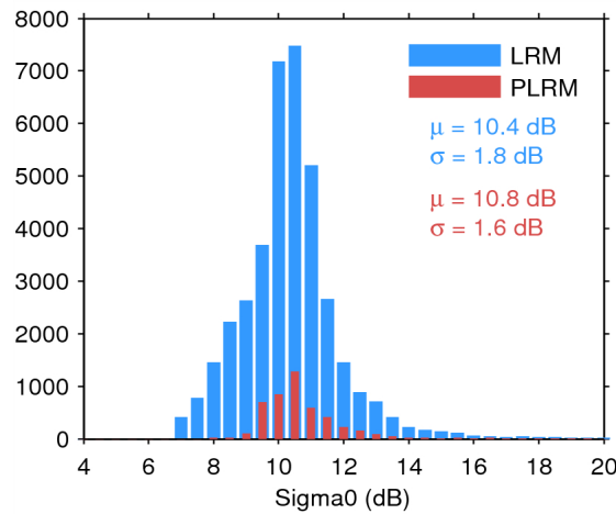
Figure 28. Histogram of science-valid sigma0 over oceans and lakes for LRM (blue) and PLRM (red) for 08/08/2014. The mean ( \mu ) and standard deviation ( \sigma ) are also shown. Note that values outside [4 20] dB are excluded from the histogram for the sake of readability but not from the computation of \mu and \sigma .
