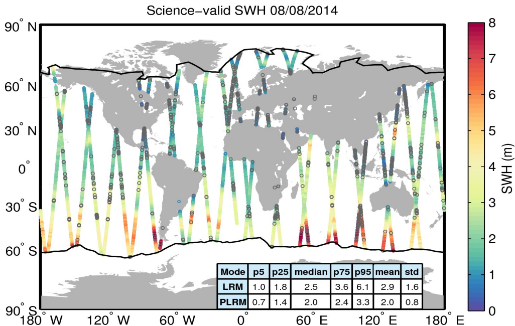
Figure 19. Geographical distribution of science-valid SWH data over oceans and lakes for 08/08/2014. The statistical values shown in the table refer to the SWH in m and are calculated separately for LRM and PLRM regions. The black lines mark the outer limit of the Arctic and Antarctic polar polygons. Gray circles denote records that have been rejected based on the editing criteria described in Table 3.
