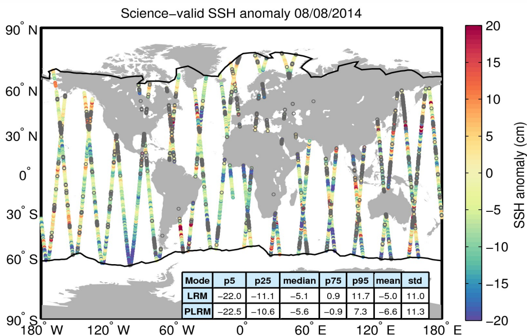
Figure 10. Geographical distribution of science-valid SSH anomaly data over oceans and lakes for 08/08/2014. The statistical values shown in the table refer to the SSH anomaly in cm and are calculated separately for LRM and PLRM regions. The black lines mark the outer limit of the Arctic and Antarctic polar polygons. Gray circles denote records that have been rejected based on the editing criteria described in Table 2.
