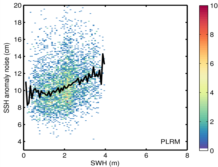
Figure 9. 2D histogram showing flag-valid SSH anomaly noise as a function of SWH for LRM (top) and PLRM (bottom) for 08/08/2014. The black line denotes the median SSH anomaly as a function of SWH.
