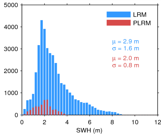
Figure 20. Histogram of science-valid SWH over oceans and lakes for LRM (blue) and PLRM (red) for 08/08/2014. The mean ( \mu ) and standard deviation ( \sigma ) are also shown. Note that values larger than 12 m are excluded from the histogram for the sake of readability but not from the computation of \mu and \sigma .
