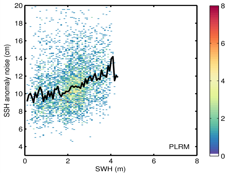
Figure 9. 2D histogram showing flag-valid SSH anomaly noise as a function of SWH for LRM (top) and PLRM (bottom) for 07/08/2014. The black line denotes the median SSH anomaly as a function of SWH.
