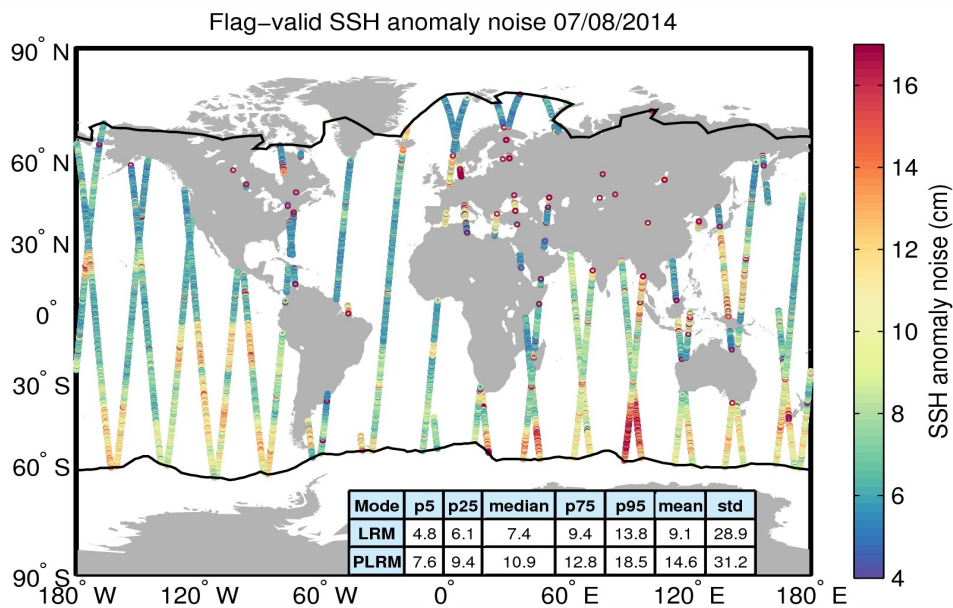
Figure 8. Geographical distribution of flag-valid 20-Hz SSH anomaly measurement noise over oceans and lakes for 07/08/2014. The statistical values shown in the table refer to the SSH anomaly noise and are calculated separately for LRM and PLRM regions. Measurements taken over polar polygons have been excluded from the computation of the statistical values. The black lines mark the outer limit of the Arctic and Antarctic polar polygons.
