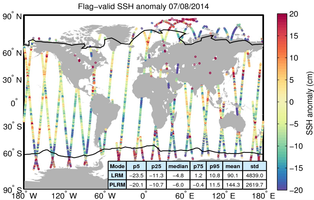
Figure 5. Geographical distribution of flag-valid 1-Hz SSH anomaly data over oceans and lakes for 07/08/2014. The statistical values shown in the table refer to the SSH anomaly in cm and are calculated separately for LRM and PLRM regions. Measurements taken over polar polygons have been excluded from the computation of the statistical values. The black lines mark the outer limit of the Arctic and Antarctic polar polygons.
