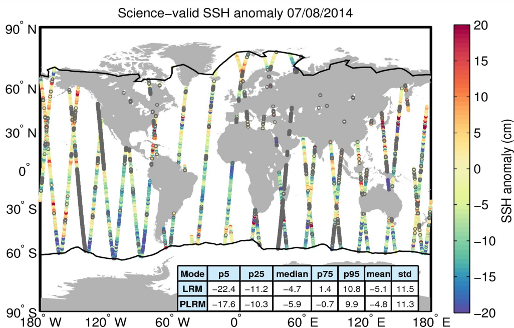
Figure 10. Geographical distribution of science-valid SSH anomaly data over oceans and lakes for 07/08/2014. The statistical values shown in the table refer to the SSH anomaly in cm and are calculated separately for LRM and PLRM regions. The black lines mark the outer limit of the Arctic and Antarctic polar polygons. Gray circles denote records that have been rejected based on the editing criteria described in Table 2.
