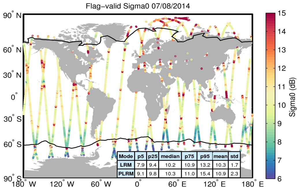
Figure 23. Geographical distribution of flag-valid sigma0 data over oceans and lakes for 07/08/2014. The statistical values shown in the table refer to the sigma0 in dB and are calculated separately for LRM and PLRM regions. Measurements taken over polar polygons have been excluded from the computation of the statistical values. The black lines mark the outer limit of the Arctic and Antarctic polar polygons.
