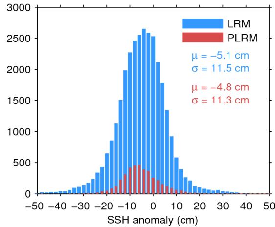
Figure 11. Histogram of science-valid SSH anomaly over oceans and lakes for LRM (blue) and PLRM (red) for 07/08/2014. The mean ( \mu ) and standard deviation ( \sigma ) are also shown. Note that values outside [-50\ 50] cm are excluded from the histogram for the sake of readability but not from the computation of \mu and \sigma .
