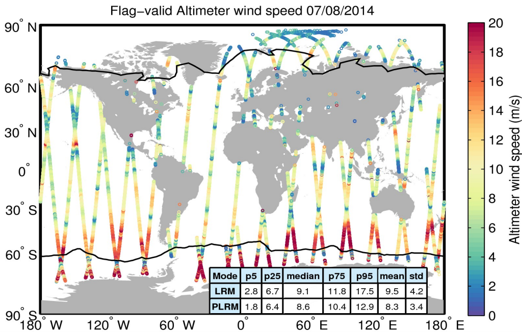
Figure 31. Geographical distribution of flag-valid wind data over oceans and lakes for 07/08/2014. The statistical values shown in the table refer to the wind in m/s and are calculated separately for LRM and PLRM regions. Measurements taken over polar polygons have been excluded from the computation of the statistical values. The black lines mark the outer limit of the Arctic and Antarctic polar polygons.
