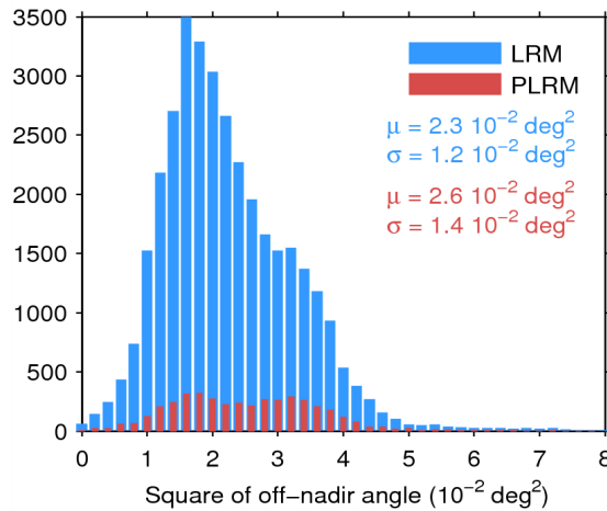
Figure 39. Histogram of flag-valid mispointing over oceans and lakes for LRM (blue) and PLRM (red) for 07/08/2014. Only positive values have been considered. The mean ( \mu ) and standard deviation ( \sigma ) are also shown. Note that values 8 \cdot 10^{-2} \text{ deg}^2 are excluded from the histogram for the sake of readability but not from the computation of \mu and \sigma .
