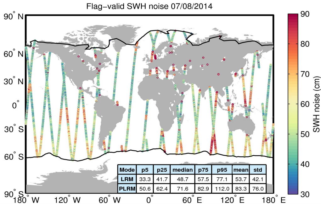
Figure 18. Geographical distribution of flag-valid 20-Hz SWH measurement noise over oceans and lakes for 07/08/2014. The statistical values shown in the table refer to the SWH noise and are calculated separately for LRM and PLRM regions. Measurements taken over polar polygons have been excluded from the computation of the statistical values. The black lines mark the outer limit of the Arctic and Antarctic polar polygons.
