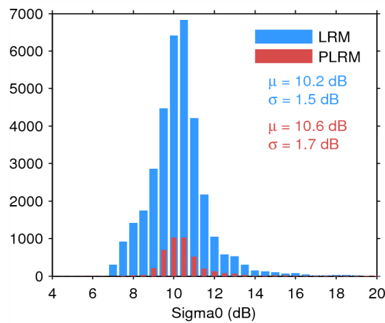
Figure 28. Histogram of science-valid sigma0 over oceans and lakes for LRM (blue) and PLRM (red) for 07/08/2014. The mean ( \mu ) and standard deviation ( \sigma ) are also shown. Note that values outside [4 20] dB are excluded from the histogram for the sake of readability but not from the computation of \mu and \sigma .
