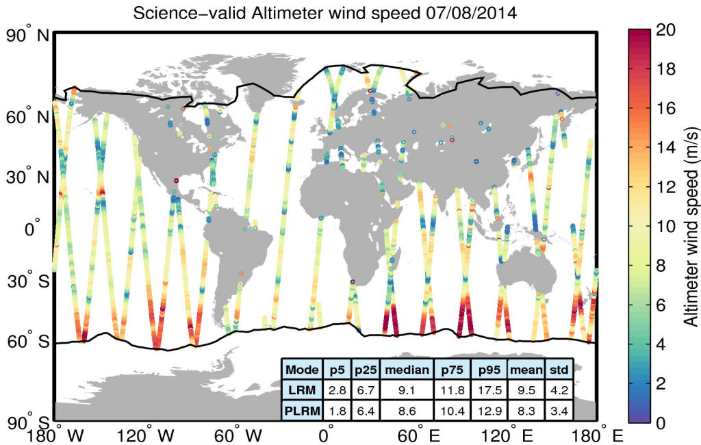
Figure 34. Geographical distribution of science-valid wind data over oceans and lakes for 07/08/2014. The statistical values shown in the table refer to the wind in m/s and are calculated separately for LRM and PLRM regions. The black lines mark the outer limit of the Arctic and Antarctic polar polygons. Gray circles denote records that have been rejected based on the editing criteria described in Table 5.
