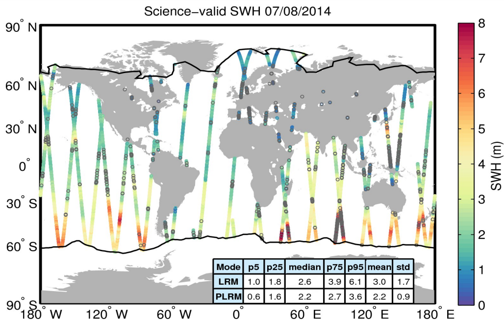
Figure 19. Geographical distribution of science-valid SWH data over oceans and lakes for 07/08/2014. The statistical values shown in the table refer to the SWH in m and are calculated separately for LRM and PLRM regions. The black lines mark the outer limit of the Arctic and Antarctic polar polygons. Gray circles denote records that have been rejected based on the editing criteria described in Table 3.
