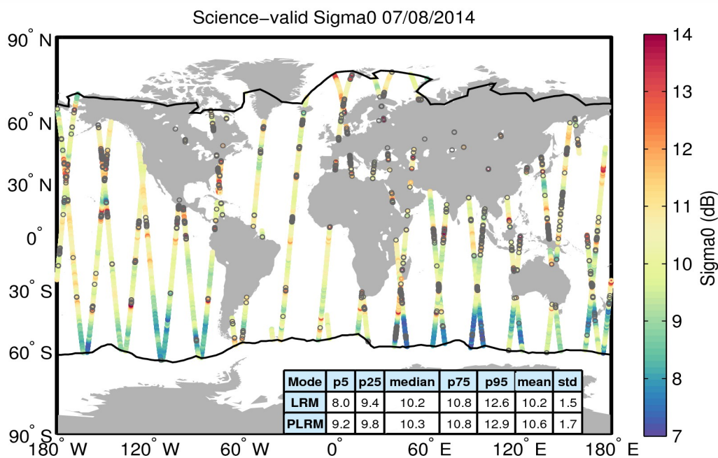
Figure 27. Geographical distribution of science-valid sigma0 data over oceans and lakes for 07/08/2014. The statistical values shown in the table refer to the sigma0 in dB and are calculated separately for LRM and PLRM regions. The black lines mark the outer limit of the Arctic and Antarctic polar polygons. Gray circles denote records that have been rejected based on the editing criteria described in Table 4.
