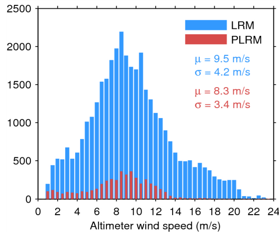
Figure 33. Histogram of flag-valid wind over oceans and lakes for LRM (blue) and PLRM (red) for 07/08/2014. The mean ( \mu ) and standard deviation ( \sigma ) are also shown. Note that values larger than 24 m/s are excluded from the histogram for the sake of readability but not from the computation of \mu and \sigma .
