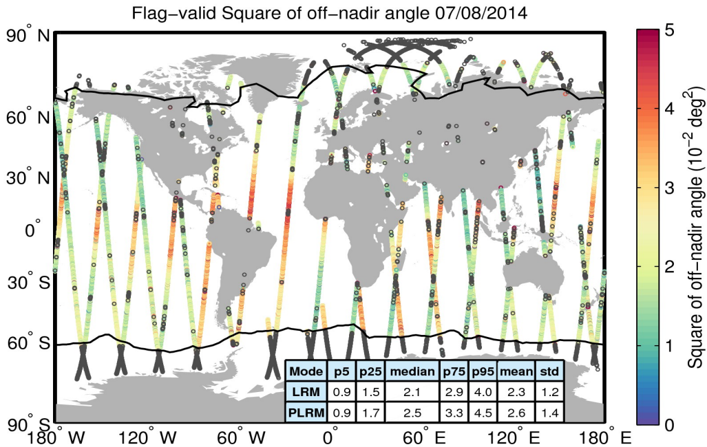
Figure 37. Geographical distribution of flag-valid mispointing data over oceans and lakes for 07/08/2014. The statistical values shown in the table refer to the mispointing in 10^{-2} \text{ deg}^2 and are calculated separately for LRM and PLRM regions. Measurements taken over polar polygons have been excluded from the computation of the statistical values. The black lines mark the outer limit of the Arctic and Antarctic polar polygons. Gray circles denote negative values.
