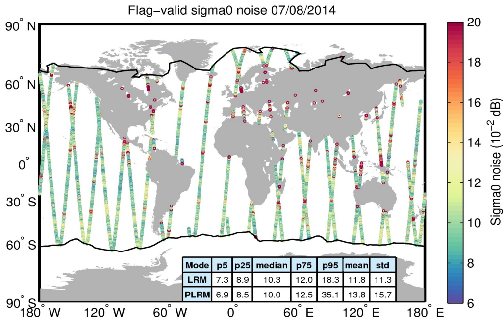
Figure 26. Geographical distribution of flag-valid 20-Hz sigma0 measurement noise over oceans and lakes for 07/08/2014. The statistical values shown in the table refer to the sigma0 noise and are calculated separately for LRM and PLRM regions. Measurements taken over polar polygons have been excluded from the computation of the statistical values. The black lines mark the outer limit of the Arctic and Antarctic polar polygons.
