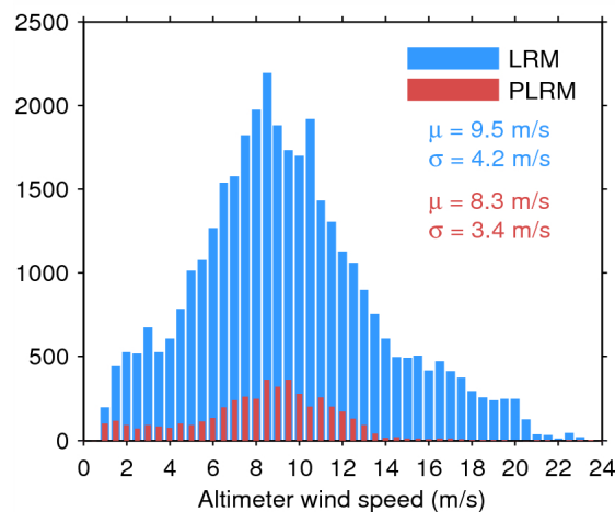
Figure 35. Histogram of science-valid wind over oceans and lakes for LRM (blue) and PLRM (red) for 07/08/2014. The mean ( \mu ) and standard deviation ( \sigma ) are also shown. Note that values larger than 24 m/s are excluded from the histogram for the sake of readability but not from the computation of \mu and \sigma .
