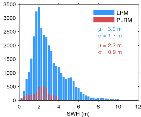
Figure 20. Histogram of science-valid SWH over oceans and lakes for LRM (blue) and PLRM (red) for 07/08/2014. The mean ( \mu ) and standard deviation ( \sigma ) are also shown. Note that values larger than 12 m are excluded from the histogram for the sake of readability but not from the computation of \mu and \sigma .
