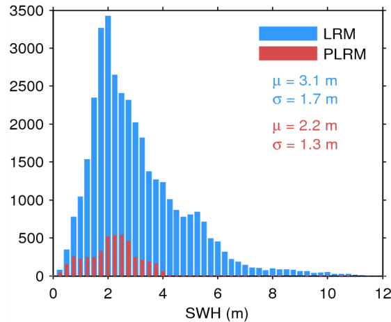
Figure 17. Histogram of flag-valid SWH over oceans and lakes for LRM (blue) and PLRM (red) for 07/08/2014. The mean ( \mu ) and standard deviation ( \sigma ) are also shown. Note that values larger than 12 m are excluded from the histogram for the sake of readability but not from the computation of \mu and \sigma .
