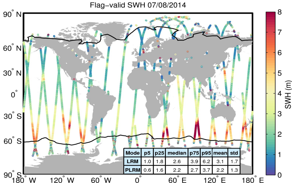
Figure 15. Geographical distribution of flag-valid SWH data over oceans and lakes for 07/08/2014. The statistical values shown in the table refer to the SWH in m and are calculated separately for LRM and PLRM regions. Measurements taken over polar polygons have been excluded from the computation of the statistical values. The black lines mark the outer limit of the Arctic and Antarctic polar polygons.
