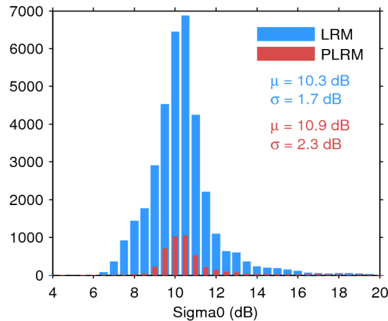
Figure 25. Histogram of flag-valid sigma0 over oceans and lakes for LRM (blue) and PLRM (red) for 07/08/2014. The mean ( \mu ) and standard deviation ( \sigma ) are also shown. Note that values outside [4 20] dB are excluded from the histogram for the sake of readability but not from the computation of \mu and \sigma .
