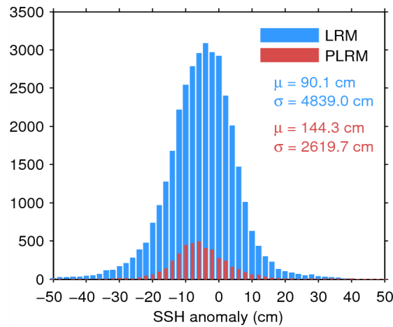
Figure 7. Histogram of flag-valid SSH anomaly over oceans and lakes for LRM (blue) and PLRM (red) for 07/08/2014. The mean ( \mu ) and standard deviation ( \sigma ) are also shown. Note that values outside [-50\ 50] cm are excluded from the histogram for the sake of readability but not from the computation of \mu and \sigma .
