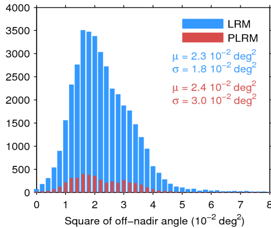
Figure 39. Histogram of flag-valid mispointing over oceans and lakes for LRM (blue) and PLRM (red) for 06/08/2014. Only positive values have been considered. The mean ( \mu ) and standard deviation ( \sigma ) are also shown. Note that values 8 \cdot 10^{-2} \text{ deg}^2 are excluded from the histogram for the sake of readability but not from the computation of \mu and \sigma .
