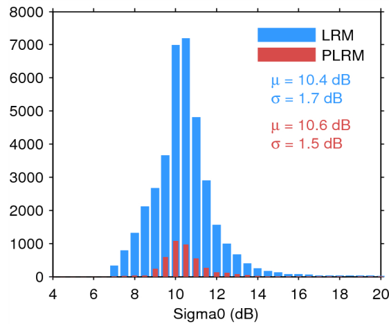
Figure 28. Histogram of science-valid sigma0 over oceans and lakes for LRM (blue) and PLRM (red) for 06/08/2014. The mean ( \mu ) and standard deviation ( \sigma ) are also shown. Note that values outside [4 20] dB are excluded from the histogram for the sake of readability but not from the computation of \mu and \sigma .
