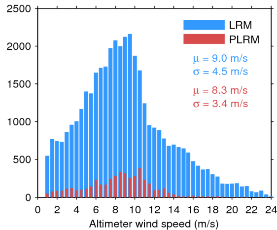
Figure 33. Histogram of flag-valid wind over oceans and lakes for LRM (blue) and PLRM (red) for 06/08/2014. The mean ( \mu ) and standard deviation ( \sigma ) are also shown. Note that values larger than 24 m/s are excluded from the histogram for the sake of readability but not from the computation of \mu and \sigma .
