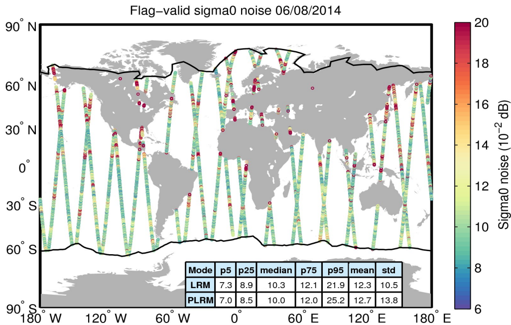
Figure 26. Geographical distribution of flag-valid 20-Hz sigma0 measurement noise over oceans and lakes for 06/08/2014. The statistical values shown in the table refer to the sigma0 noise and are calculated separately for LRM and PLRM regions. Measurements taken over polar polygons have been excluded from the computation of the statistical values. The black lines mark the outer limit of the Arctic and Antarctic polar polygons.
