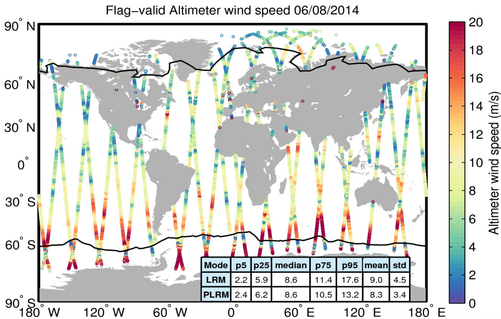
Figure 31. Geographical distribution of flag-valid wind data over oceans and lakes for 06/08/2014. The statistical values shown in the table refer to the wind in m/s and are calculated separately for LRM and PLRM regions. Measurements taken over polar polygons have been excluded from the computation of the statistical values. The black lines mark the outer limit of the Arctic and Antarctic polar polygons.
