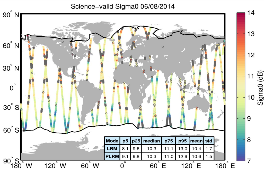
Figure 27. Geographical distribution of science-valid sigma0 data over oceans and lakes for 06/08/2014. The statistical values shown in the table refer to the sigma0 in dB and are calculated separately for LRM and PLRM regions. The black lines mark the outer limit of the Arctic and Antarctic polar polygons. Gray circles denote records that have been rejected based on the editing criteria described in Table 4.
