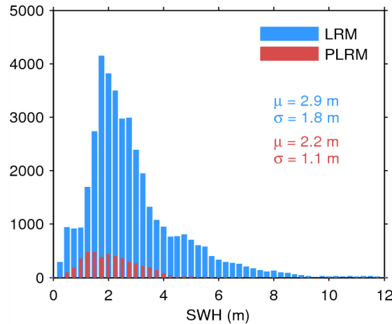
Figure 17. Histogram of flag-valid SWH over oceans and lakes for LRM (blue) and PLRM (red) for 06/08/2014. The mean ( \mu ) and standard deviation ( \sigma ) are also shown. Note that values larger than 12 m are excluded from the histogram for the sake of readability but not from the computation of \mu and \sigma .
