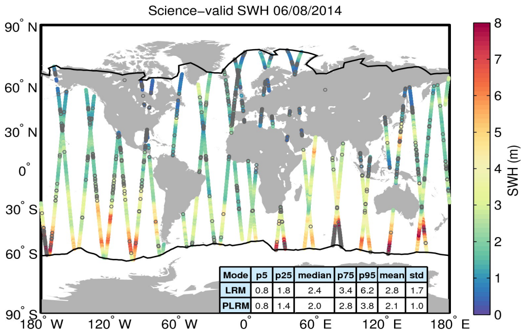
Figure 19. Geographical distribution of science-valid SWH data over oceans and lakes for 06/08/2014. The statistical values shown in the table refer to the SWH in m and are calculated separately for LRM and PLRM regions. The black lines mark the outer limit of the Arctic and Antarctic polar polygons. Gray circles denote records that have been rejected based on the editing criteria described in Table 3.
