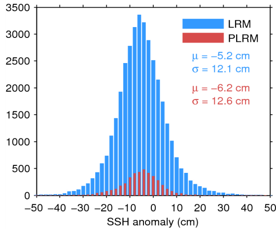
Figure 11. Histogram of science-valid SSH anomaly over oceans and lakes for LRM (blue) and PLRM (red) for 06/08/2014. The mean ( \mu ) and standard deviation ( \sigma ) are also shown. Note that values outside [-50 50] cm are excluded from the histogram for the sake of readability but not from the computation of \mu and \sigma .
