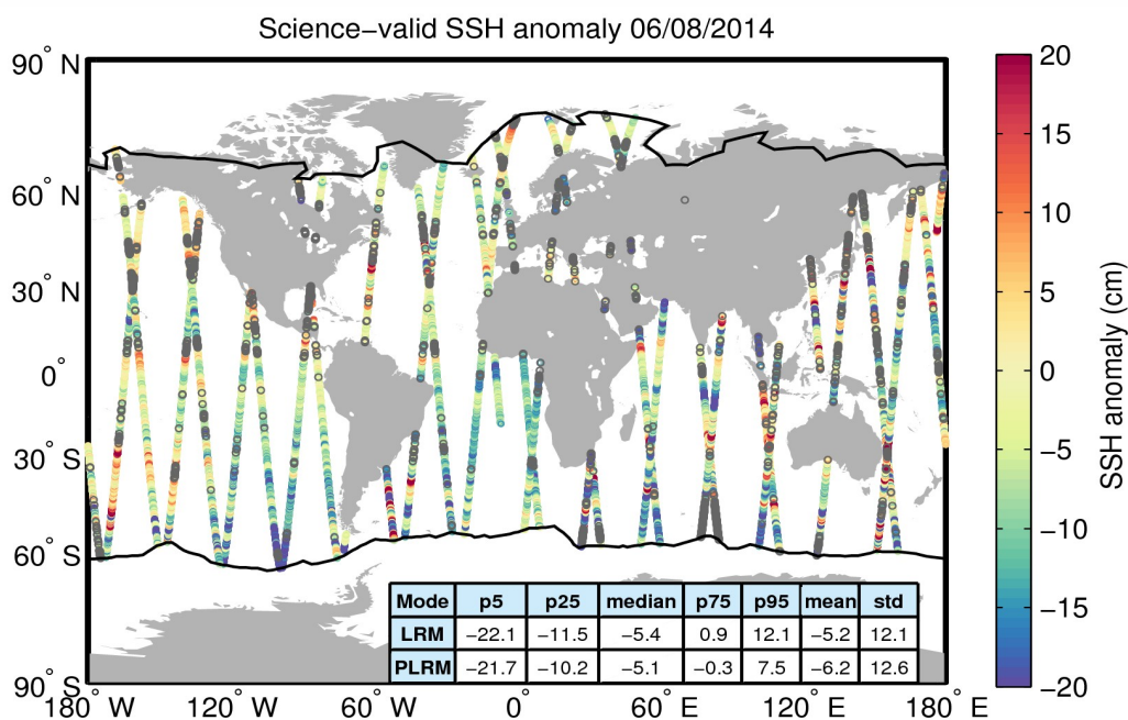
Figure 10. Geographical distribution of science-valid SSH anomaly data over oceans and lakes for 06/08/2014. The statistical values shown in the table refer to the SSH anomaly in cm and are calculated separately for LRM and PLRM regions. The black lines mark the outer limit of the Arctic and Antarctic polar polygons. Gray circles denote records that have been rejected based on the editing criteria described in Table 2.
