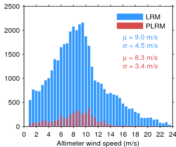
Figure 35. Histogram of science-valid wind over oceans and lakes for LRM (blue) and PLRM (red) for 06/08/2014. The mean ( \mu ) and standard deviation ( \sigma ) are also shown. Note that values larger than 24 m/s are excluded from the histogram for the sake of readability but not from the computation of \mu and \sigma .
