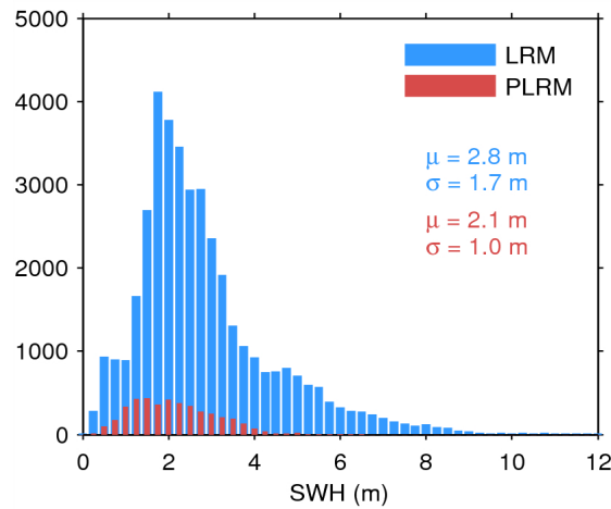
Figure 20. Histogram of science-valid SWH over oceans and lakes for LRM (blue) and PLRM (red) for 06/08/2014. The mean ( \mu ) and standard deviation ( \sigma ) are also shown. Note that values larger than 12 m are excluded from the histogram for the sake of readability but not from the computation of \mu and \sigma .
