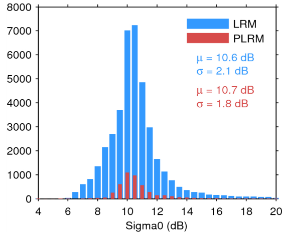
Figure 25. Histogram of flag-valid sigma0 over oceans and lakes for LRM (blue) and PLRM (red) for 06/08/2014. The mean ( \mu ) and standard deviation ( \sigma ) are also shown. Note that values outside [4 20] dB are excluded from the histogram for the sake of readability but not from the computation of \mu and \sigma .
