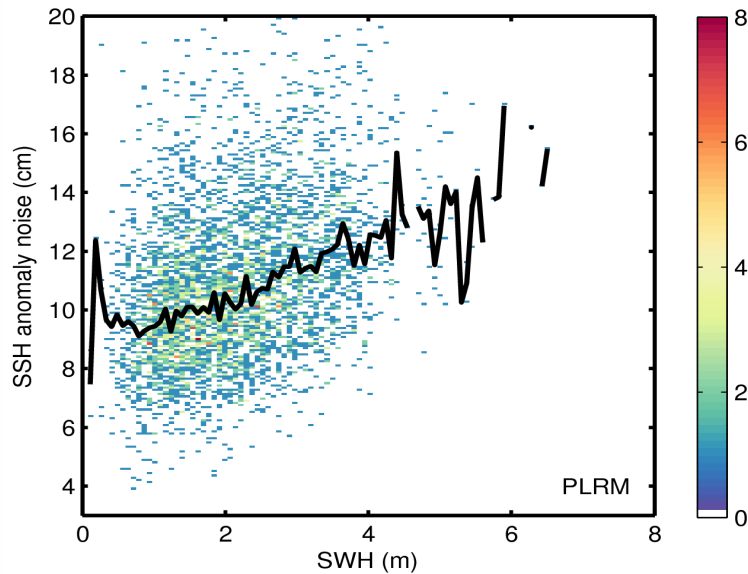
Figure 9. 2D histogram showing flag-valid SSH anomaly noise as a function of SWH for LRM (top) and PLRM (bottom) for 06/08/2014. The black line denotes the median SSH anomaly as a function of SWH.
