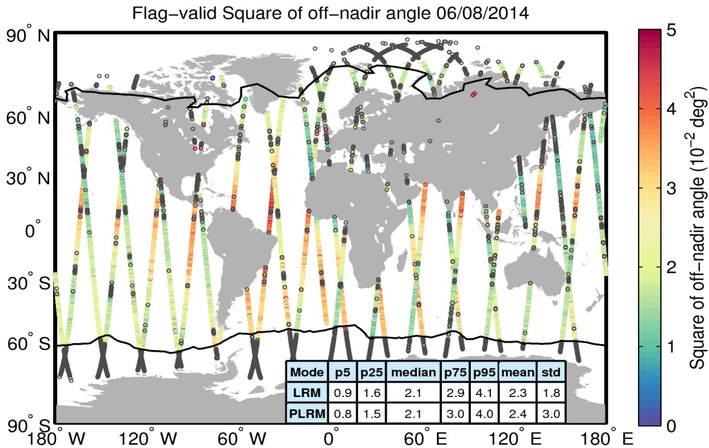
Figure 37. Geographical distribution of flag-valid mispointing data over oceans and lakes for 06/08/2014. The statistical values shown in the table refer to the mispointing in 10^{-2} \text{ deg}^2 and are calculated separately for LRM and PLRM regions. Measurements taken over polar polygons have been excluded from the computation of the statistical values. The black lines mark the outer limit of the Arctic and Antarctic polar polygons. Gray circles denote negative values.
