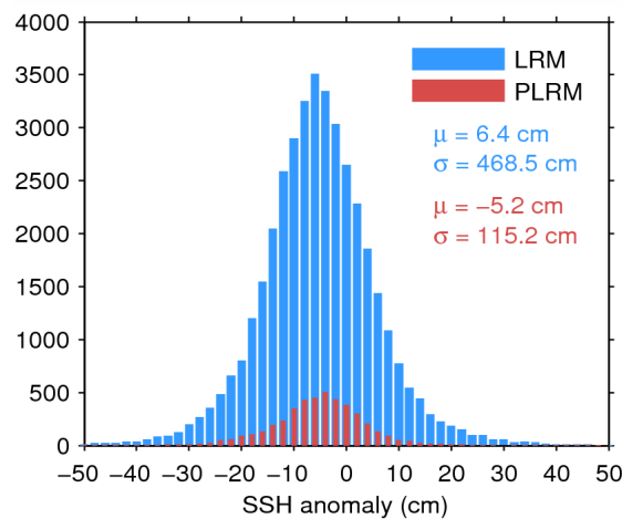
Figure 7. Histogram of flag-valid SSH anomaly over oceans and lakes for LRM (blue) and PLRM (red) for 06/08/2014. The mean ( \mu ) and standard deviation ( \sigma ) are also shown. Note that values outside [-50\ 50] cm are excluded from the histogram for the sake of readability but not from the computation of \mu and \sigma .
