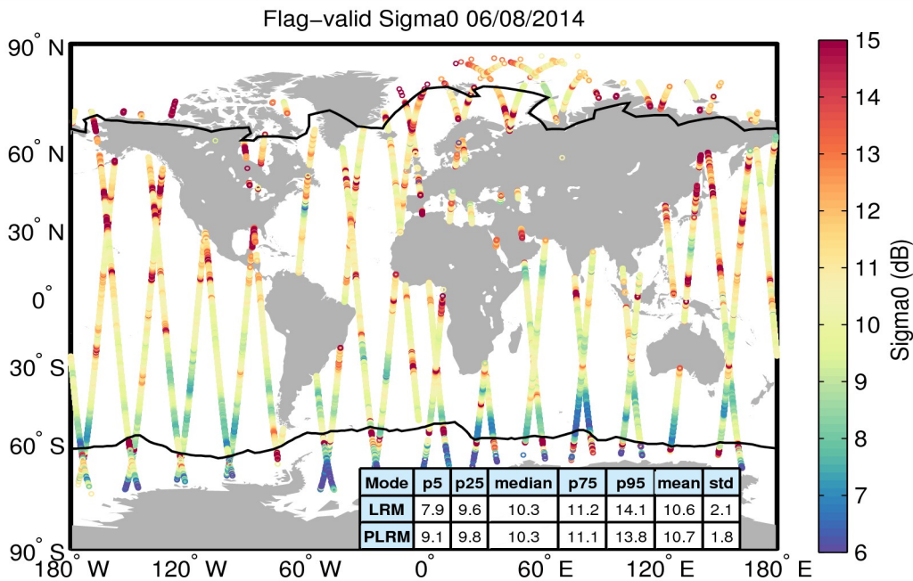
Figure 23. Geographical distribution of flag-valid sigma0 data over oceans and lakes for 06/08/2014. The statistical values shown in the table refer to the sigma0 in dB and are calculated separately for LRM and PLRM regions. Measurements taken over polar polygons have been excluded from the computation of the statistical values. The black lines mark the outer limit of the Arctic and Antarctic polar polygons.
