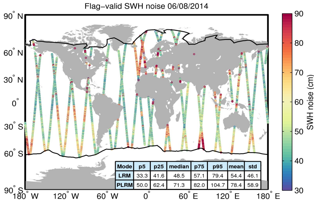
Figure 18. Geographical distribution of flag-valid 20-Hz SWH measurement noise over oceans and lakes for 06/08/2014. The statistical values shown in the table refer to the SWH noise and are calculated separately for LRM and PLRM regions. Measurements taken over polar polygons have been excluded from the computation of the statistical values. The black lines mark the outer limit of the Arctic and Antarctic polar polygons.
