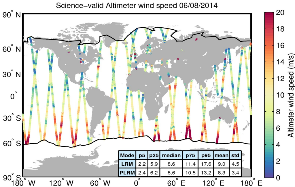
Figure 34. Geographical distribution of science-valid wind data over oceans and lakes for 06/08/2014. The statistical values shown in the table refer to the wind in m/s and are calculated separately for LRM and PLRM regions. The black lines mark the outer limit of the Arctic and Antarctic polar polygons. Gray circles denote records that have been rejected based on the editing criteria described in Table 5.
