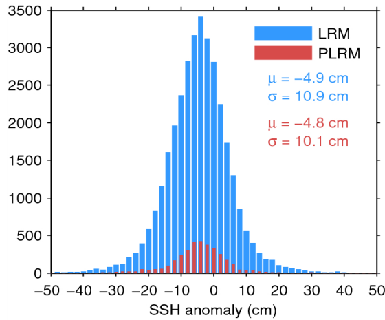
Figure 11. Histogram of science-valid SSH anomaly over oceans and lakes for LRM (blue) and PLRM (red) for 03/08/2014. The mean ( \mu ) and standard deviation ( \sigma ) are also shown. Note that values outside [-50 50] cm are excluded from the histogram for the sake of readability but not from the computation of \mu and \sigma .
