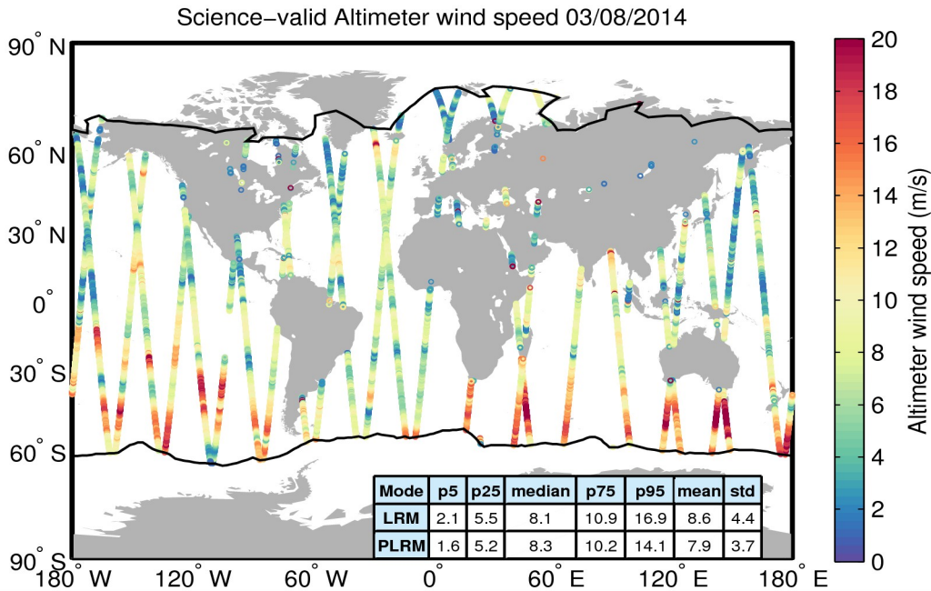
Figure 34. Geographical distribution of science-valid wind data over oceans and lakes for 03/08/2014. The statistical values shown in the table refer to the wind in m/s and are calculated separately for LRM and PLRM regions. The black lines mark the outer limit of the Arctic and Antarctic polar polygons. Gray circles denote records that have been rejected based on the editing criteria described in Table 5.
