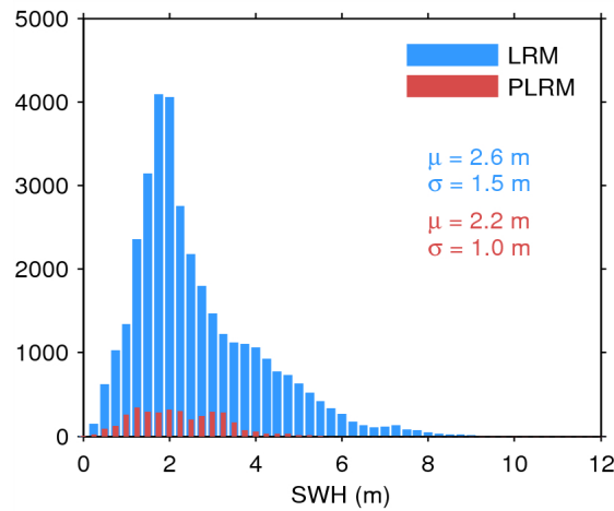
Figure 20. Histogram of science-valid SWH over oceans and lakes for LRM (blue) and PLRM (red) for 03/08/2014. The mean ( \mu ) and standard deviation ( \sigma ) are also shown. Note that values larger than 12 m are excluded from the histogram for the sake of readability but not from the computation of \mu and \sigma .
