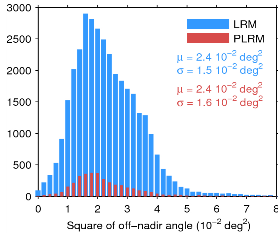
Figure 39. Histogram of flag-valid mispointing over oceans and lakes for LRM (blue) and PLRM (red) for 03/08/2014. Only positive values have been considered. The mean ( \mu ) and standard deviation ( \sigma ) are also shown. Note that values 8 \cdot 10^{-2} \text{ deg}^2 are excluded from the histogram for the sake of readability but not from the computation of \mu and \sigma .
