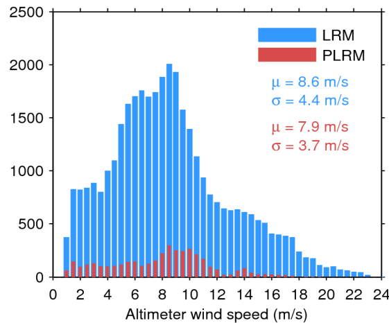
Figure 33. Histogram of flag-valid wind over oceans and lakes for LRM (blue) and PLRM (red) for 03/08/2014. The mean ( \mu ) and standard deviation ( \sigma ) are also shown. Note that values larger than 24 m/s are excluded from the histogram for the sake of readability but not from the computation of \mu and \sigma .
