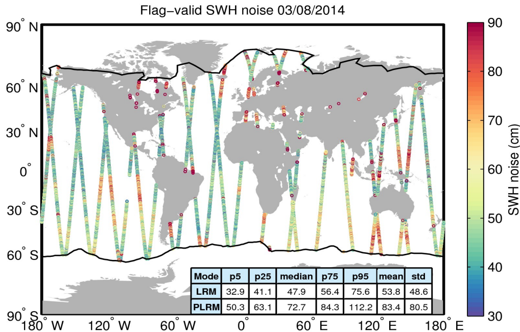
Figure 18. Geographical distribution of flag-valid 20-Hz SWH measurement noise over oceans and lakes for 03/08/2014. The statistical values shown in the table refer to the SWH noise and are calculated separately for LRM and PLRM regions. Measurements taken over polar polygons have been excluded from the computation of the statistical values. The black lines mark the outer limit of the Arctic and Antarctic polar polygons.
