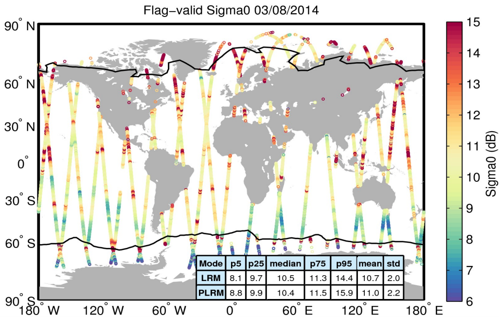
Figure 23. Geographical distribution of flag-valid sigma0 data over oceans and lakes for 03/08/2014. The statistical values shown in the table refer to the sigma0 in dB and are calculated separately for LRM and PLRM regions. Measurements taken over polar polygons have been excluded from the computation of the statistical values. The black lines mark the outer limit of the Arctic and Antarctic polar polygons.
