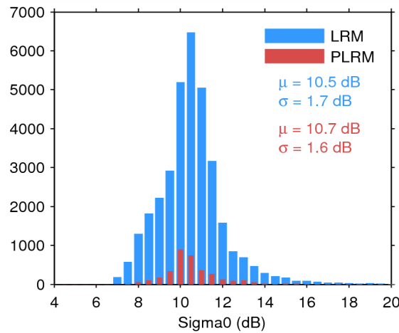
Figure 28. Histogram of science-valid sigma0 over oceans and lakes for LRM (blue) and PLRM (red) for 03/08/2014. The mean ( \mu ) and standard deviation ( \sigma ) are also shown. Note that values outside [4 20] dB are excluded from the histogram for the sake of readability but not from the computation of \mu and \sigma .
