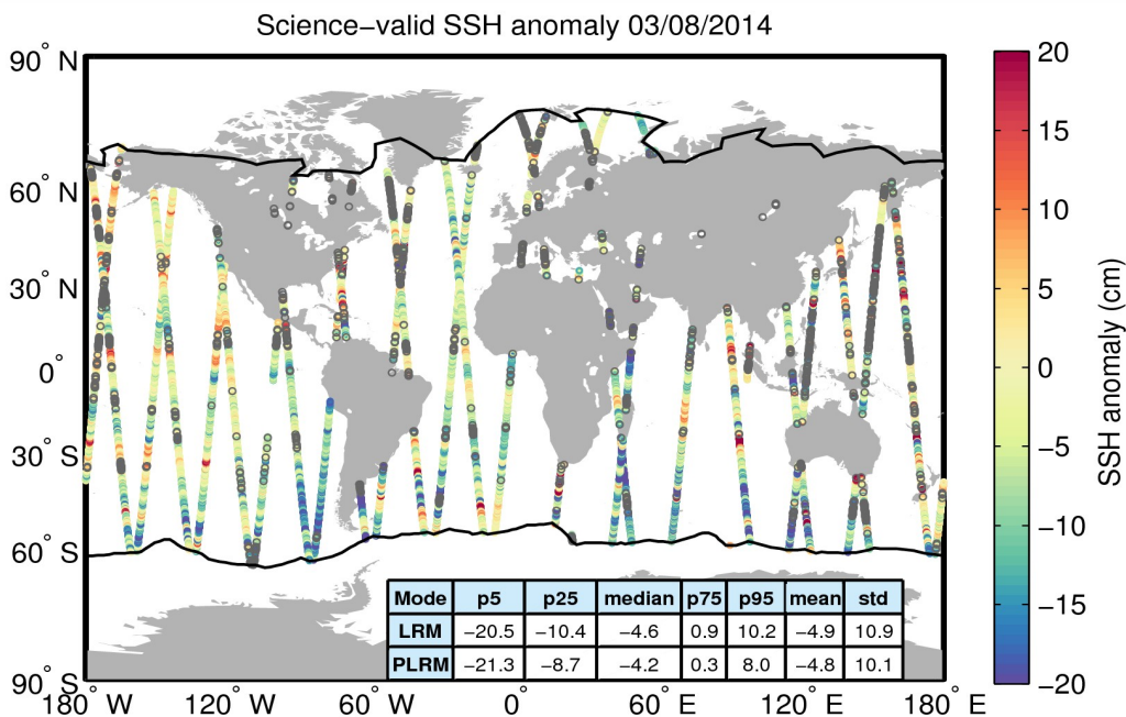
Figure 10. Geographical distribution of science-valid SSH anomaly data over oceans and lakes for 03/08/2014. The statistical values shown in the table refer to the SSH anomaly in cm and are calculated separately for LRM and PLRM regions. The black lines mark the outer limit of the Arctic and Antarctic polar polygons. Gray circles denote records that have been rejected based on the editing criteria described in Table 2.
