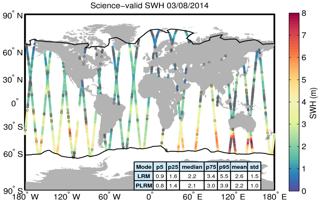
Figure 19. Geographical distribution of science-valid SWH data over oceans and lakes for 03/08/2014. The statistical values shown in the table refer to the SWH in m and are calculated separately for LRM and PLRM regions. The black lines mark the outer limit of the Arctic and Antarctic polar polygons. Gray circles denote records that have been rejected based on the editing criteria described in Table 3.
