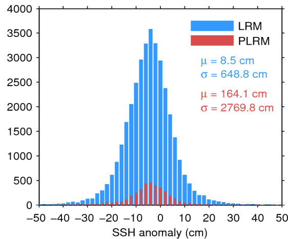
Figure 7. Histogram of flag-valid SSH anomaly over oceans and lakes for LRM (blue) and PLRM (red) for 03/08/2014. The mean ( \mu ) and standard deviation ( \sigma ) are also shown. Note that values outside [-50\ 50] cm are excluded from the histogram for the sake of readability but not from the computation of \mu and \sigma .
