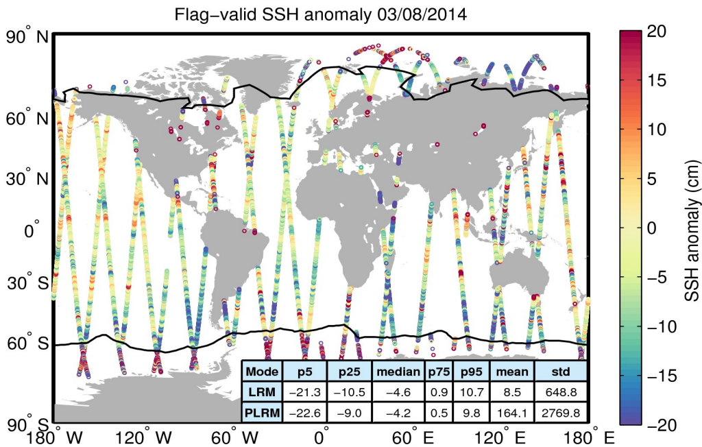
Figure 5. Geographical distribution of flag-valid 1-Hz SSH anomaly data over oceans and lakes for 03/08/2014. The statistical values shown in the table refer to the SSH anomaly in cm and are calculated separately for LRM and PLRM regions. Measurements taken over polar polygons have been excluded from the computation of the statistical values. The black lines mark the outer limit of the Arctic and Antarctic polar polygons.
