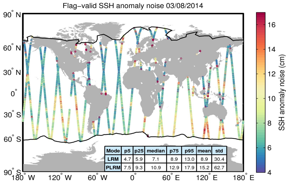
Figure 8. Geographical distribution of flag-valid 20-Hz SSH anomaly measurement noise over oceans and lakes for 03/08/2014. The statistical values shown in the table refer to the SSH anomaly noise and are calculated separately for LRM and PLRM regions. Measurements taken over polar polygons have been excluded from the computation of the statistical values. The black lines mark the outer limit of the Arctic and Antarctic polar polygons.
