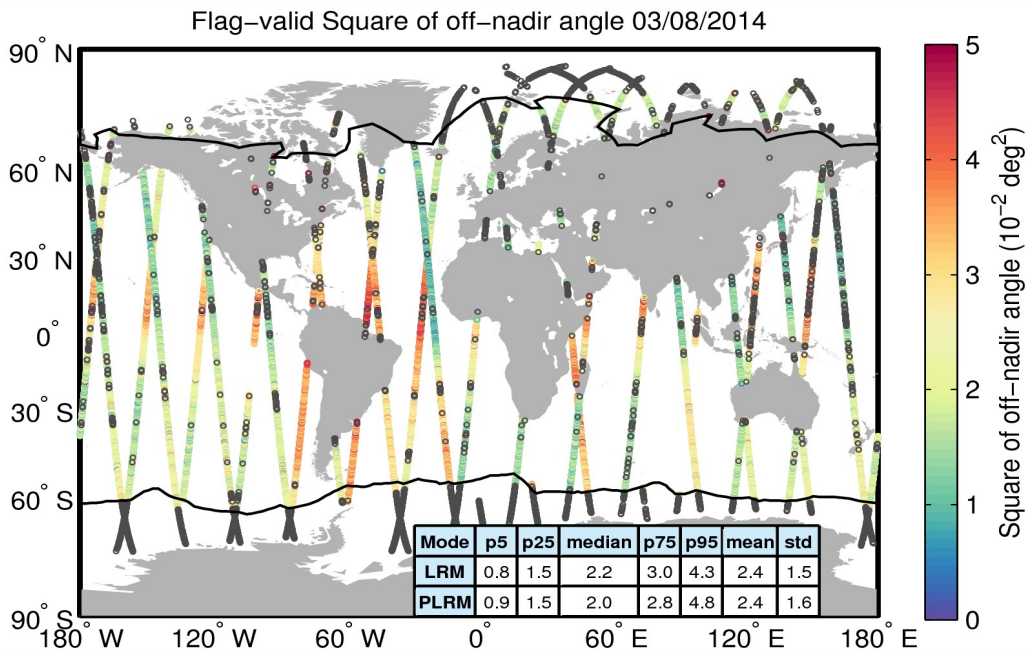
Figure 37. Geographical distribution of flag-valid mispointing data over oceans and lakes for 03/08/2014. The statistical values shown in the table refer to the mispointing in 10^{-2} \text{ deg}^2 and are calculated separately for LRM and PLRM regions. Measurements taken over polar polygons have been excluded from the computation of the statistical values. The black lines mark the outer limit of the Arctic and Antarctic polar polygons. Gray circles denote negative values.
