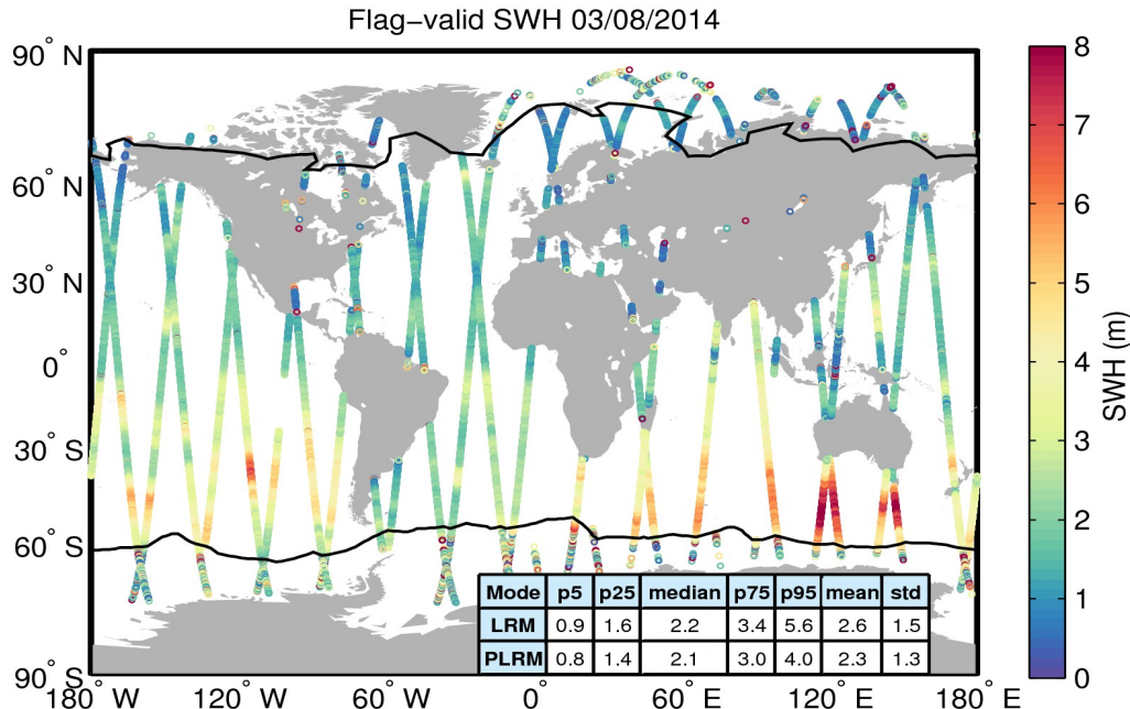
Figure 15. Geographical distribution of flag-valid SWH data over oceans and lakes for 03/08/2014. The statistical values shown in the table refer to the SWH in m and are calculated separately for LRM and PLRM regions. Measurements taken over polar polygons have been excluded from the computation of the statistical values. The black lines mark the outer limit of the Arctic and Antarctic polar polygons.
