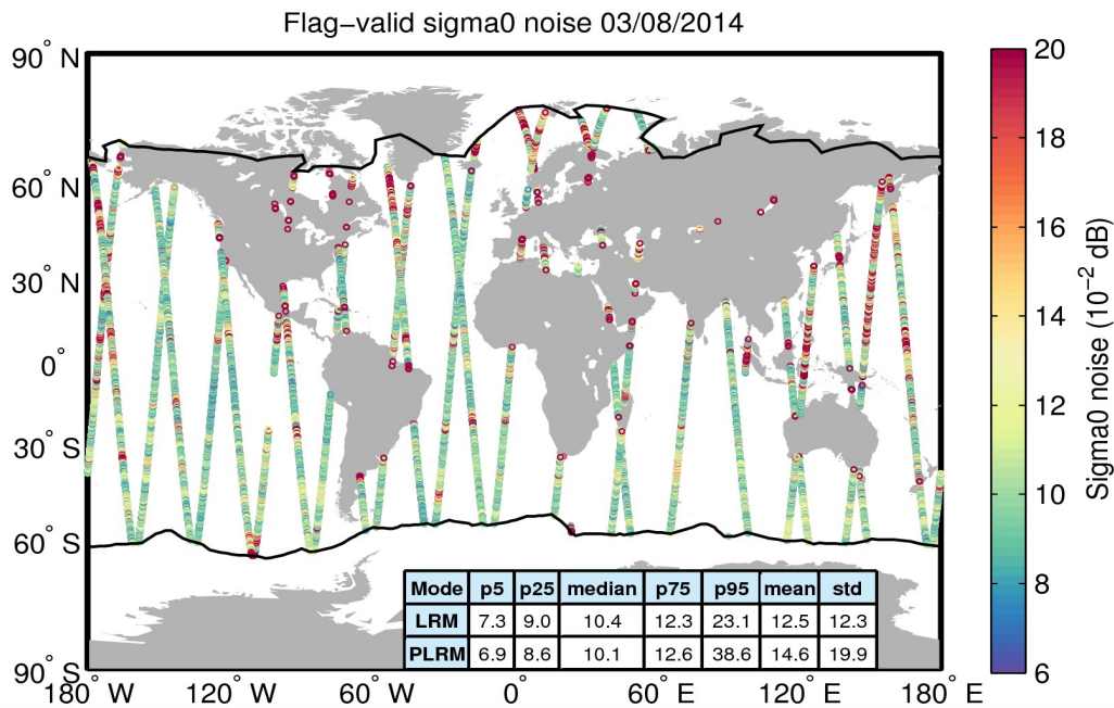
Figure 26. Geographical distribution of flag-valid 20-Hz sigma0 measurement noise over oceans and lakes for 03/08/2014. The statistical values shown in the table refer to the sigma0 noise and are calculated separately for LRM and PLRM regions. Measurements taken over polar polygons have been excluded from the computation of the statistical values. The black lines mark the outer limit of the Arctic and Antarctic polar polygons.
