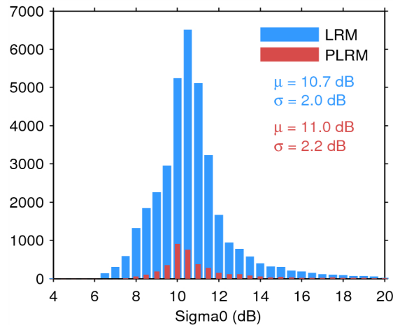
Figure 25. Histogram of flag-valid sigma0 over oceans and lakes for LRM (blue) and PLRM (red) for 03/08/2014. The mean ( \mu ) and standard deviation ( \sigma ) are also shown. Note that values outside [4 20] dB are excluded from the histogram for the sake of readability but not from the computation of \mu and \sigma .
