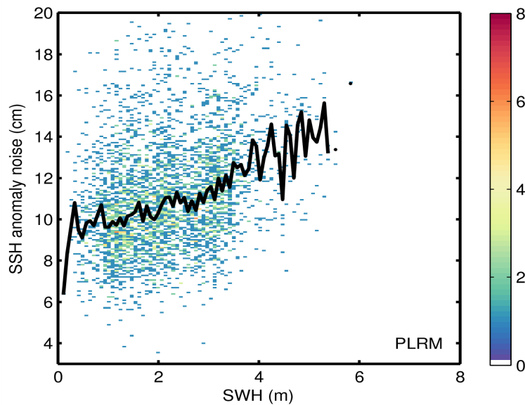
Figure 9. 2D histogram showing flag-valid SSH anomaly noise as a function of SWH for LRM (top) and PLRM (bottom) for 03/08/2014. The black line denotes the median SSH anomaly as a function of SWH.
