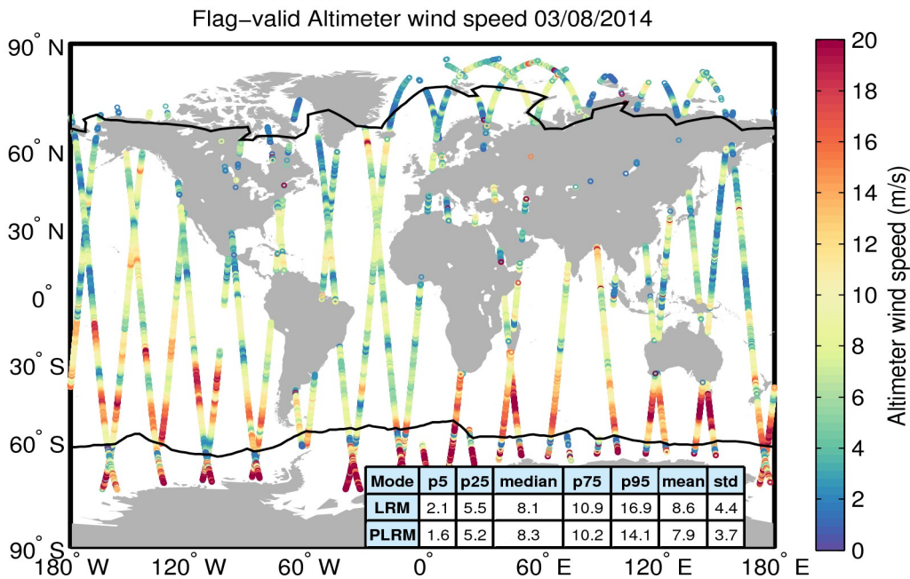
Figure 31. Geographical distribution of flag-valid wind data over oceans and lakes for 03/08/2014. The statistical values shown in the table refer to the wind in m/s and are calculated separately for LRM and PLRM regions. Measurements taken over polar polygons have been excluded from the computation of the statistical values. The black lines mark the outer limit of the Arctic and Antarctic polar polygons.
