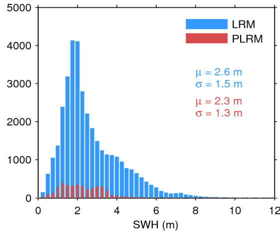
Figure 17. Histogram of flag-valid SWH over oceans and lakes for LRM (blue) and PLRM (red) for 03/08/2014. The mean ( \mu ) and standard deviation ( \sigma ) are also shown. Note that values larger than 12 m are excluded from the histogram for the sake of readability but not from the computation of \mu and \sigma .
