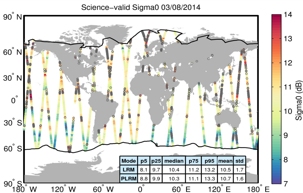
Figure 27. Geographical distribution of science-valid sigma0 data over oceans and lakes for 03/08/2014. The statistical values shown in the table refer to the sigma0 in dB and are calculated separately for LRM and PLRM regions. The black lines mark the outer limit of the Arctic and Antarctic polar polygons. Gray circles denote records that have been rejected based on the editing criteria described in Table 4.
