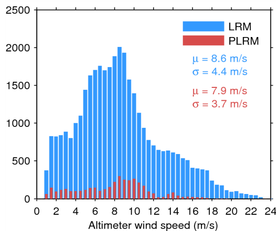
Figure 35. Histogram of science-valid wind over oceans and lakes for LRM (blue) and PLRM (red) for 03/08/2014. The mean ( \mu ) and standard deviation ( \sigma ) are also shown. Note that values larger than 24 m/s are excluded from the histogram for the sake of readability but not from the computation of \mu and \sigma .
